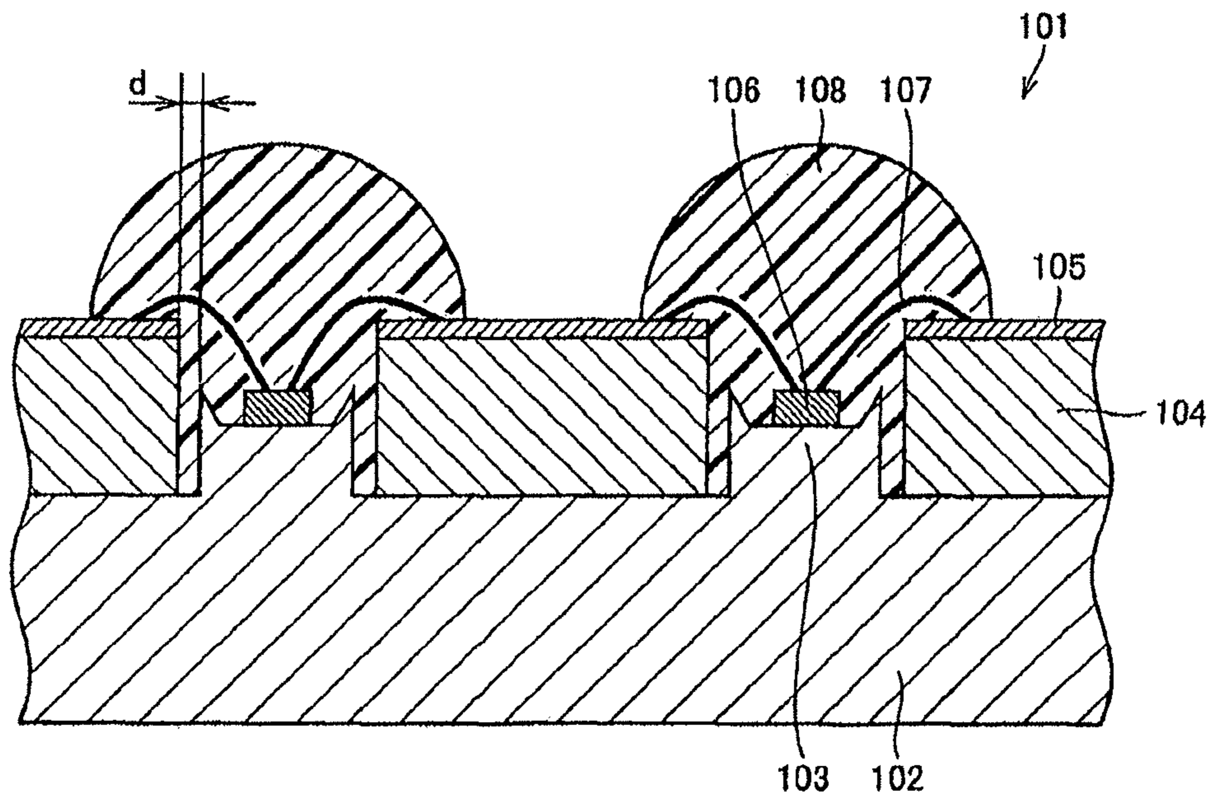
FIG.14 PRIOR ART
