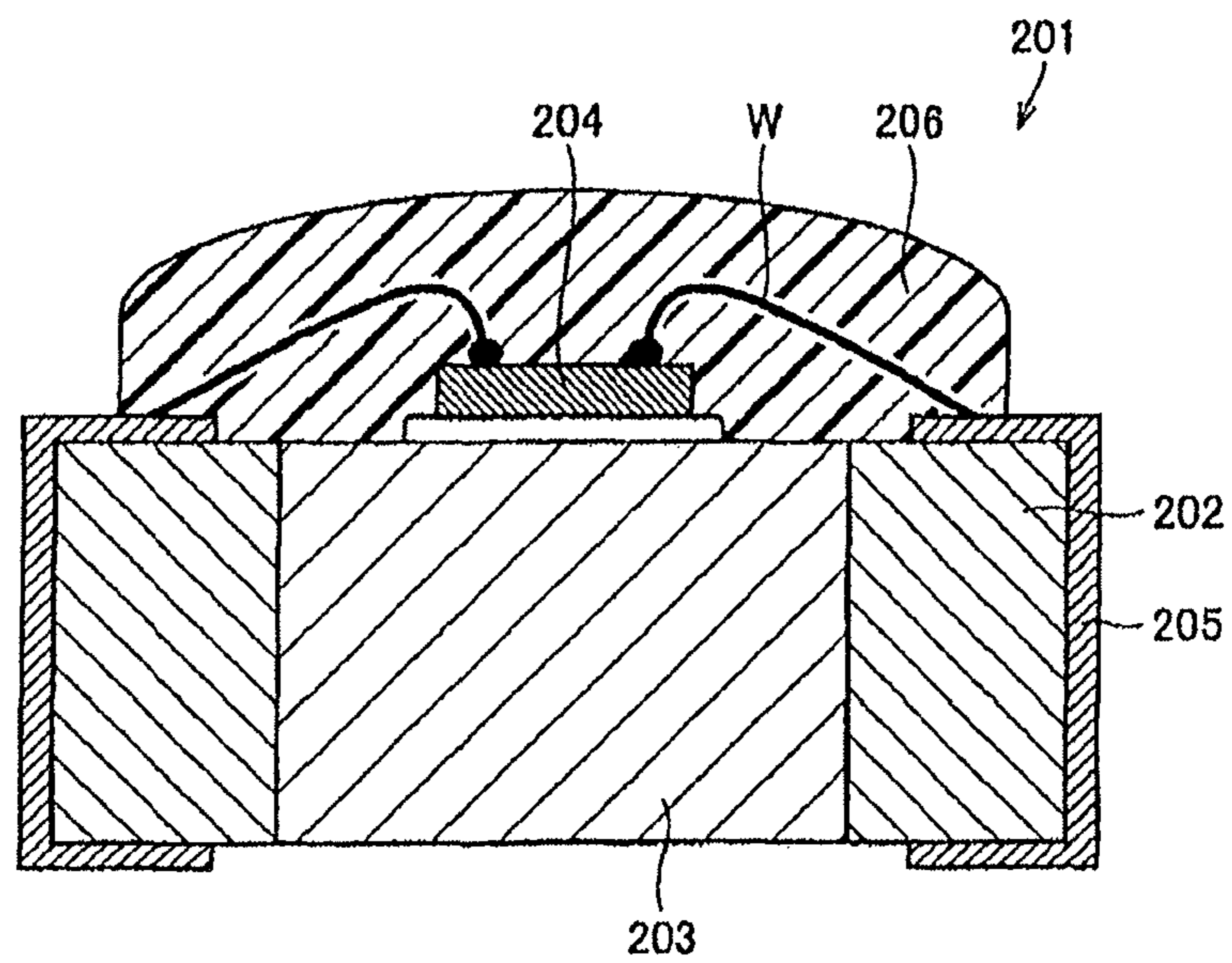
FIG.15 PRIOR ART
