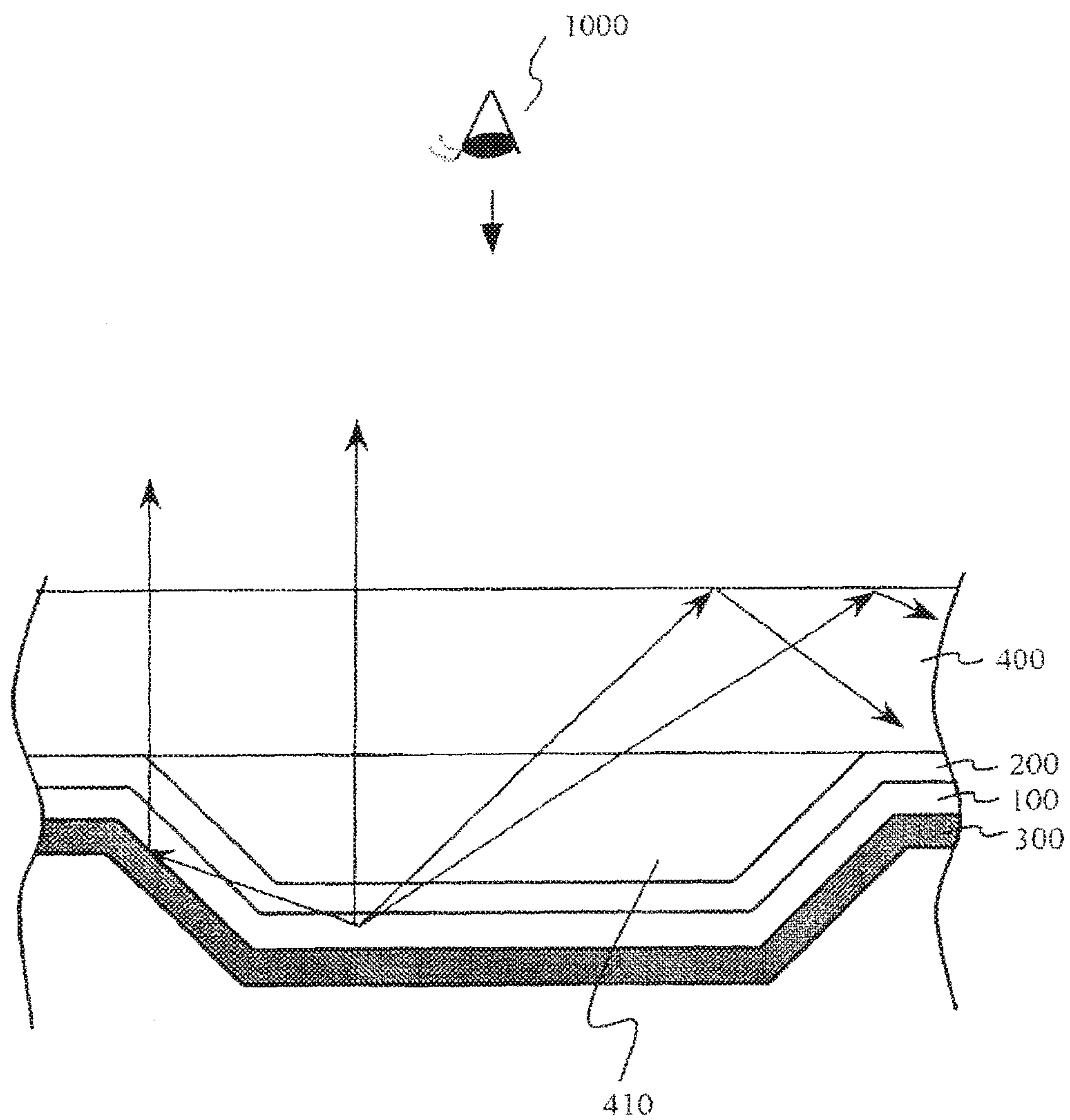
FIG. 34 PRIOR ART
