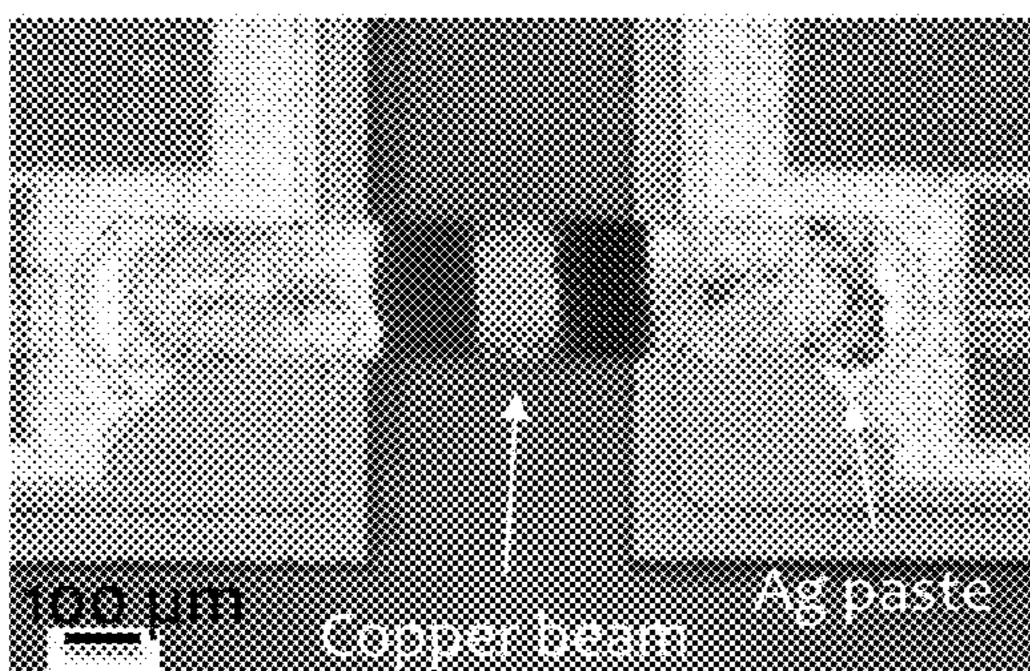
b) Close up view of single interconnect attached with silver paste
