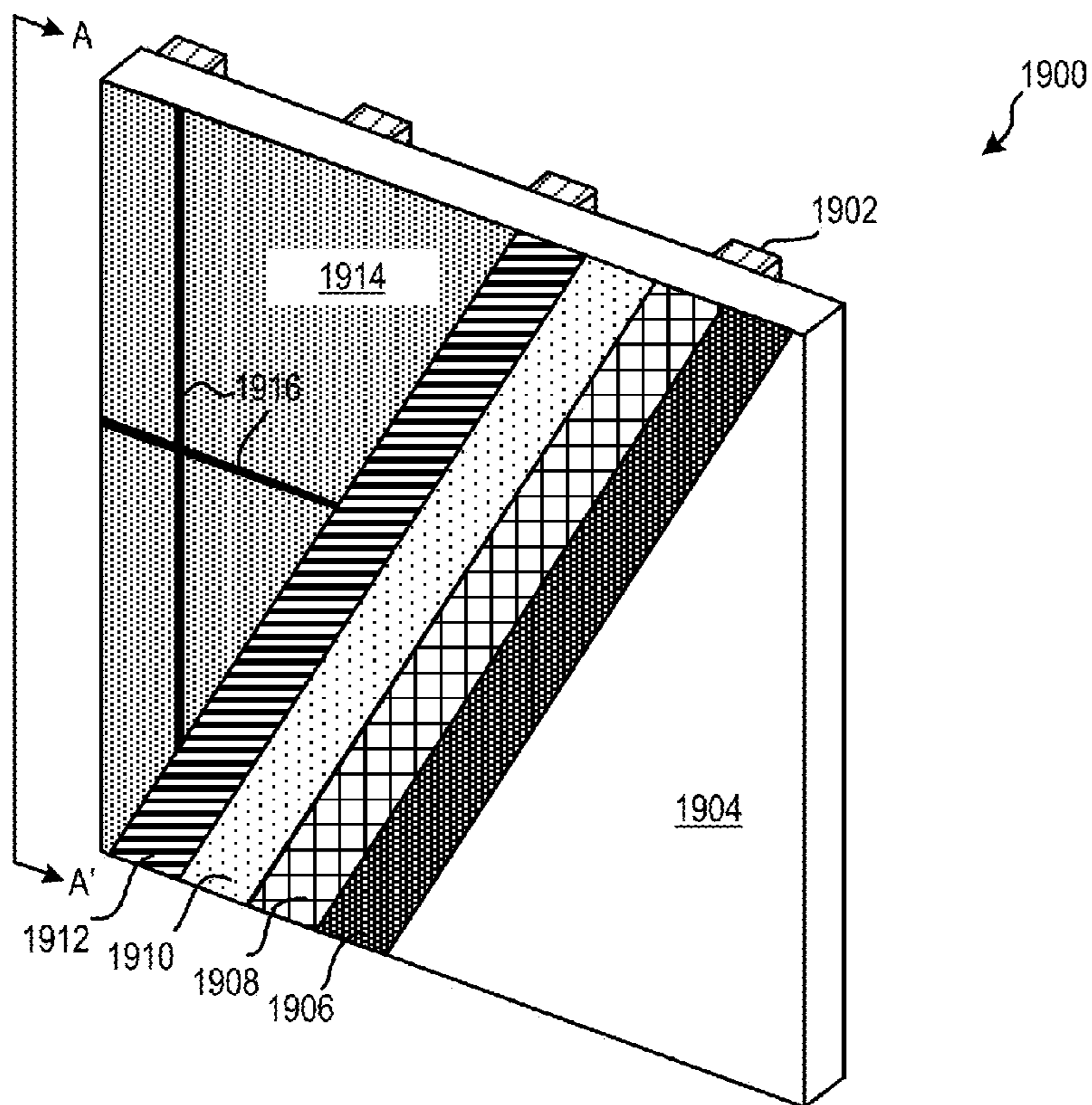
FIG. 19 (PRIOR ART)
