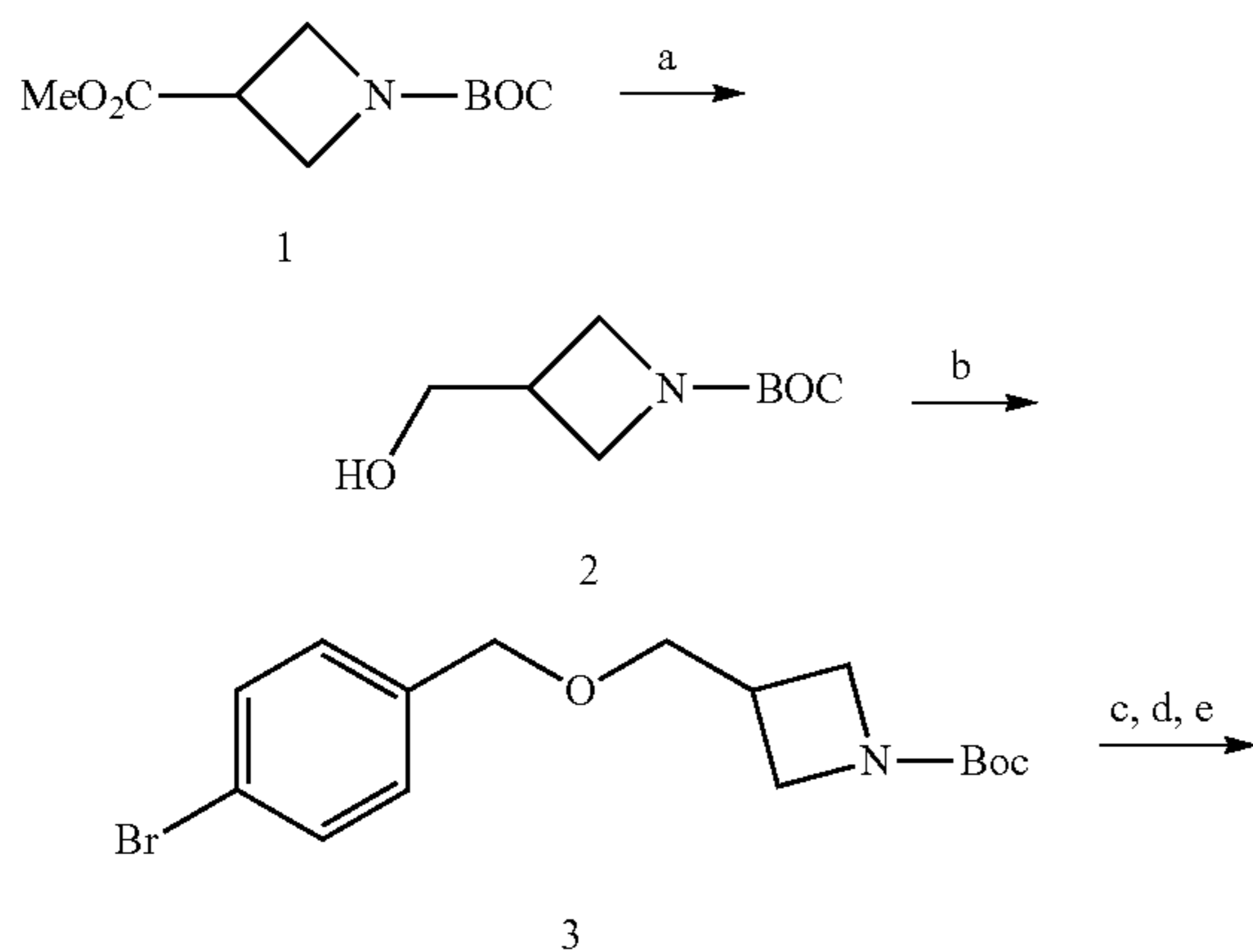
Scheme 15:
