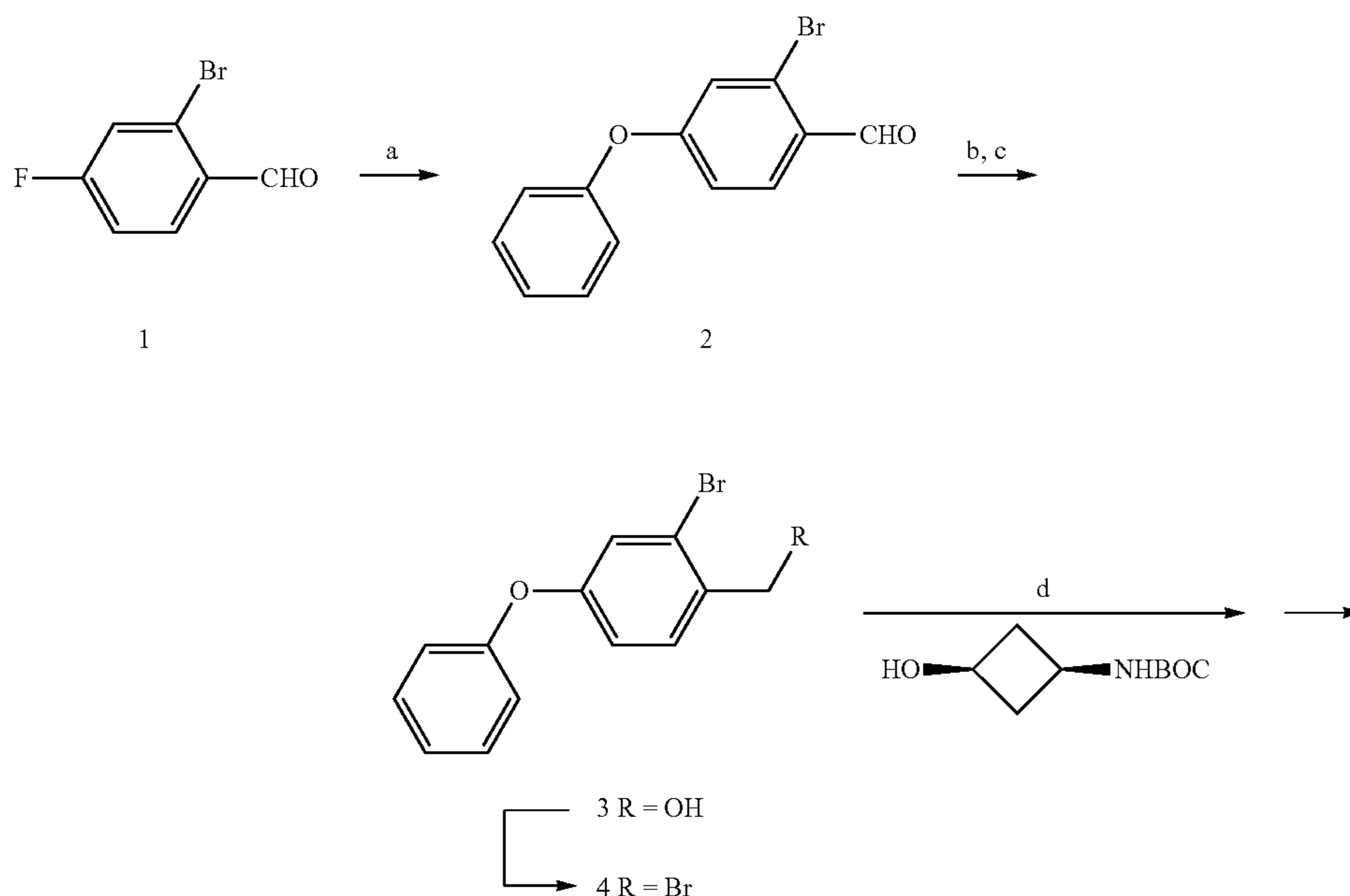
Scheme 8:
