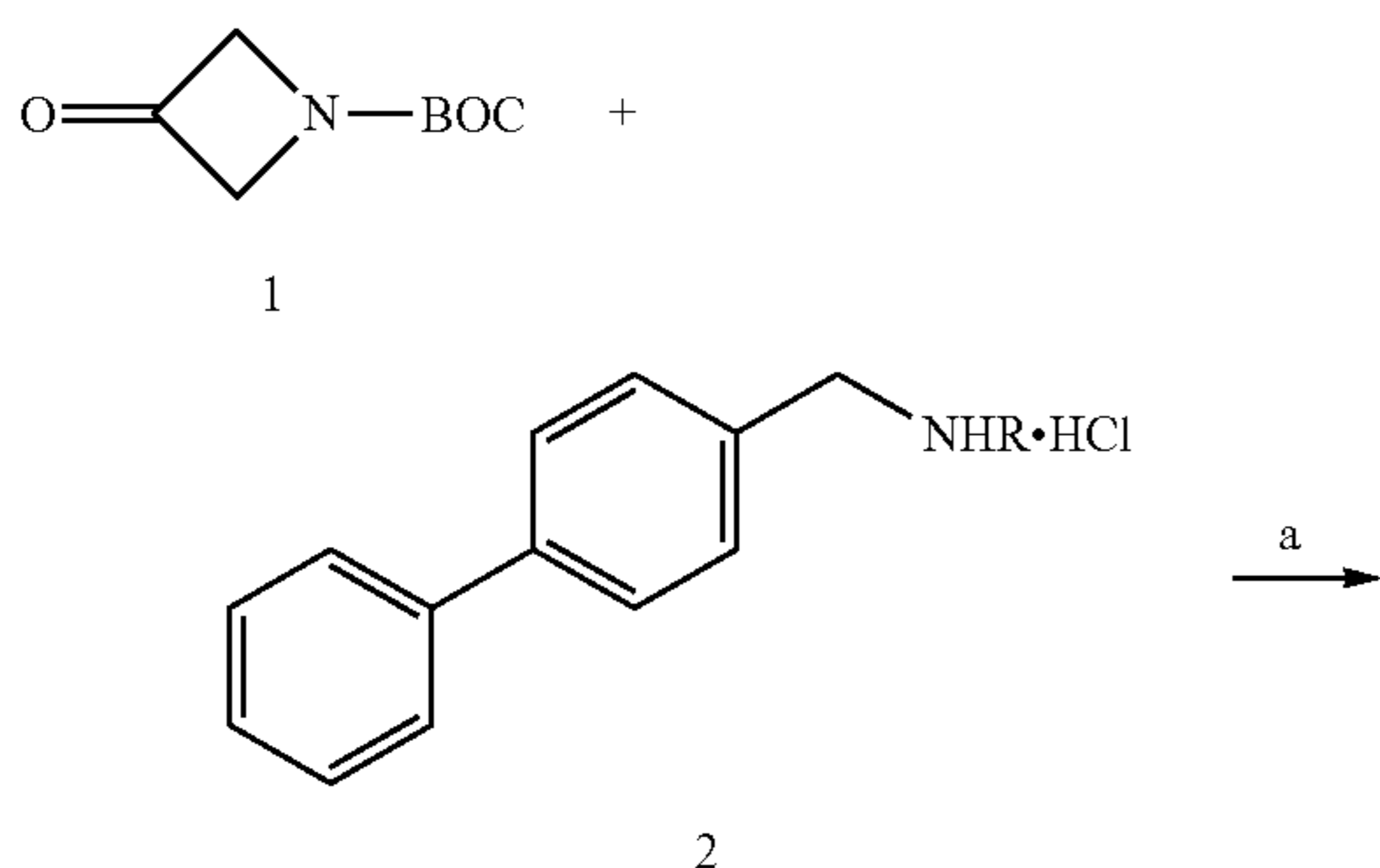
Scheme 19:
