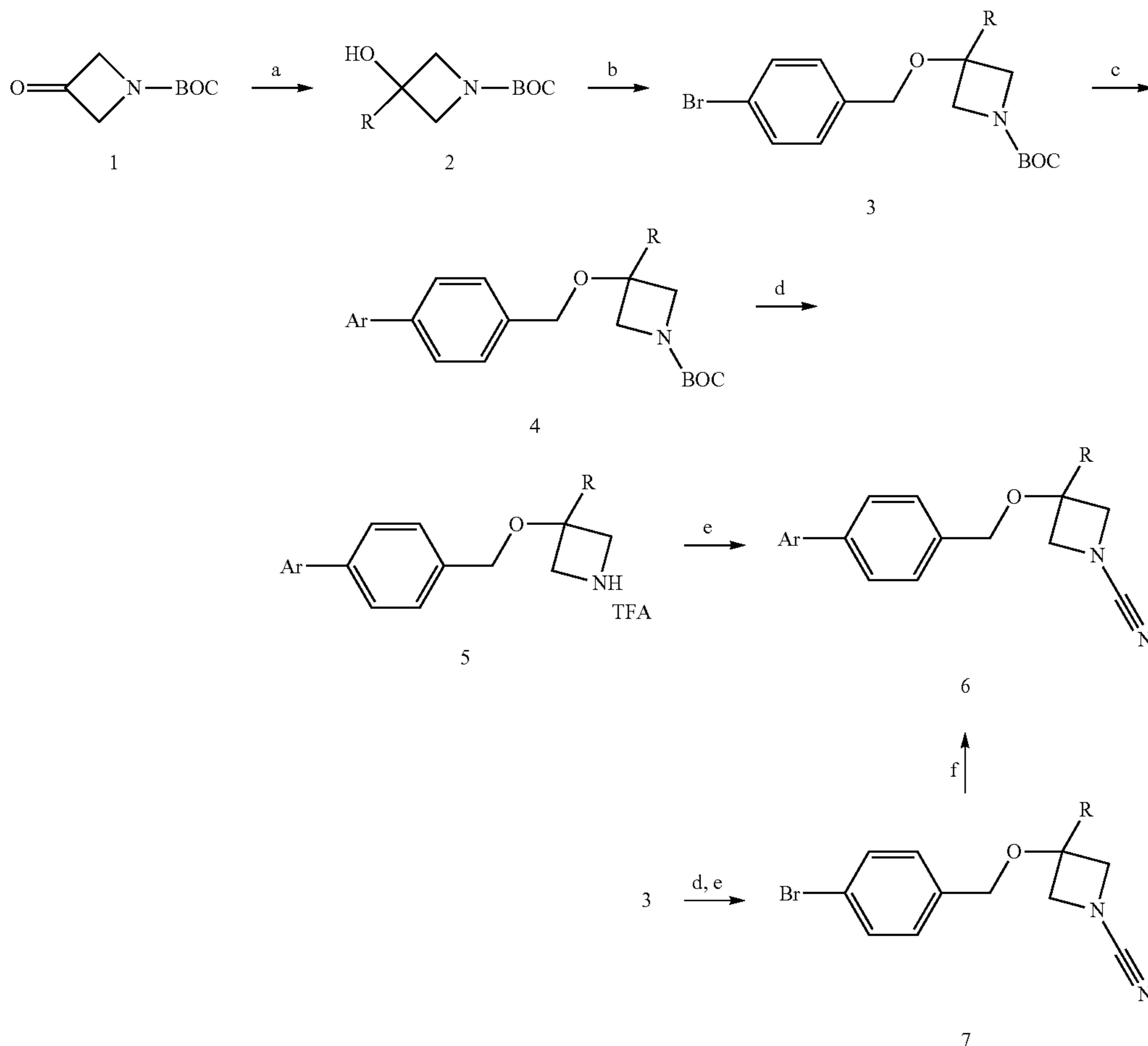
Scheme 17:
