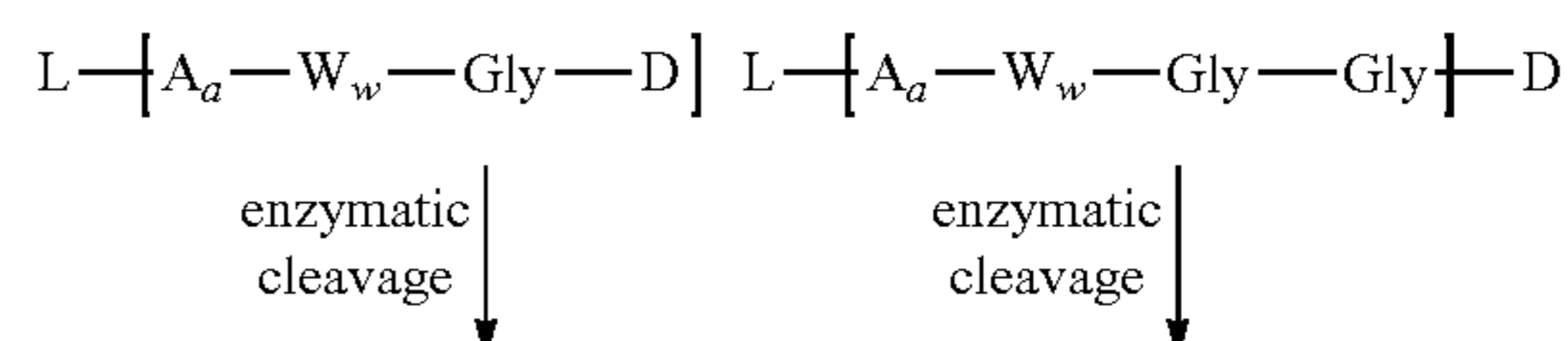
Scheme 1
