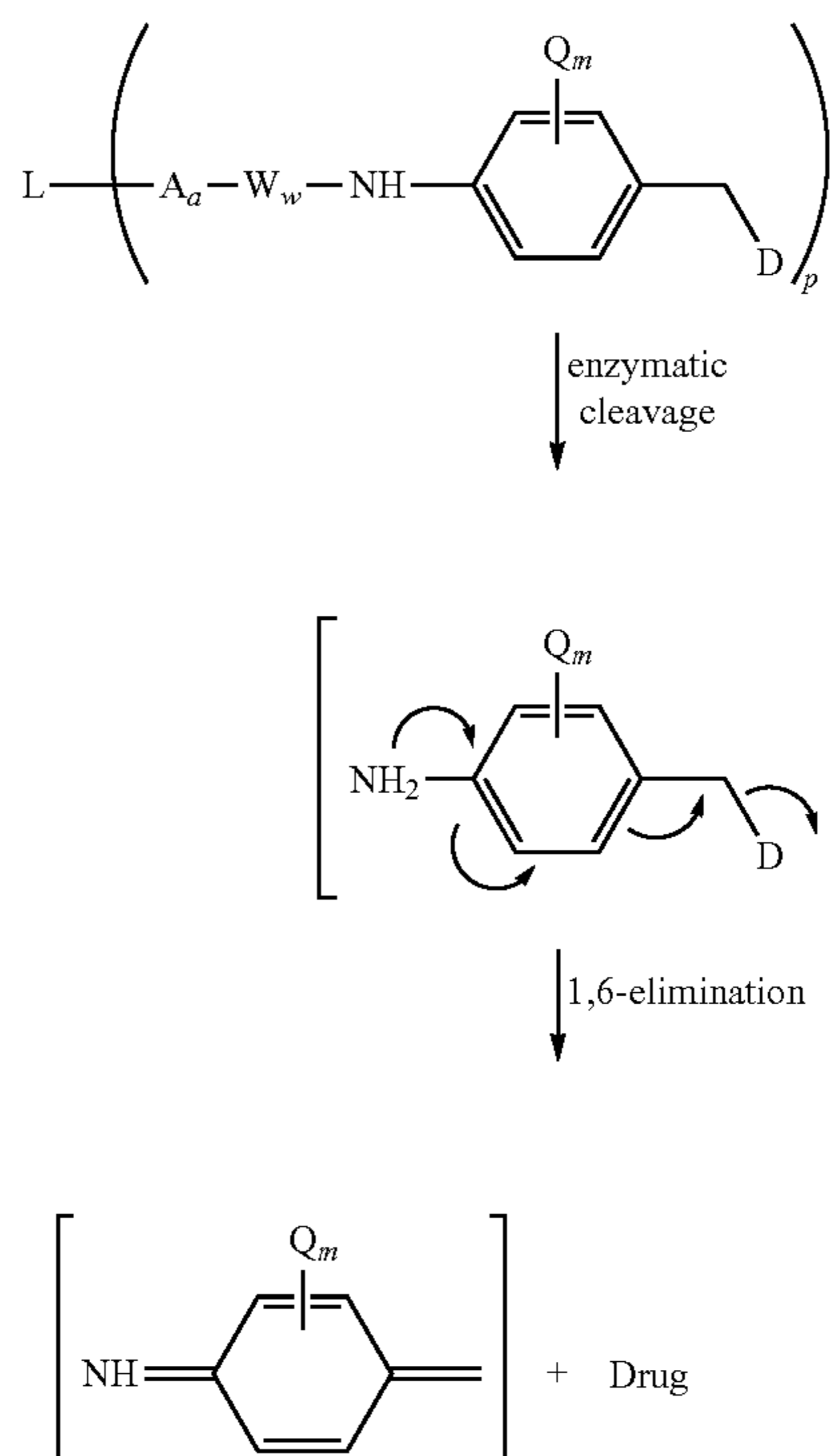
Scheme 3
