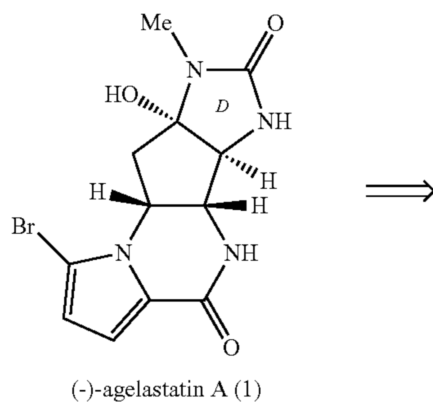
Scheme 2. An early approach toward (-)-agelastatin A (1).
