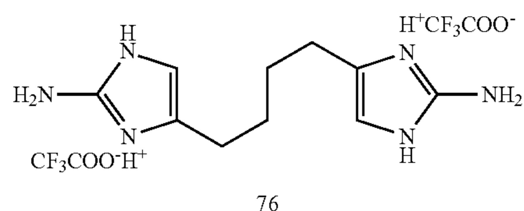
4,4'-(Butane-1,4-diyl)bis(2-amino-1H-imidazol-3-ium) 2,2,2-trifluoroacetate (76)
