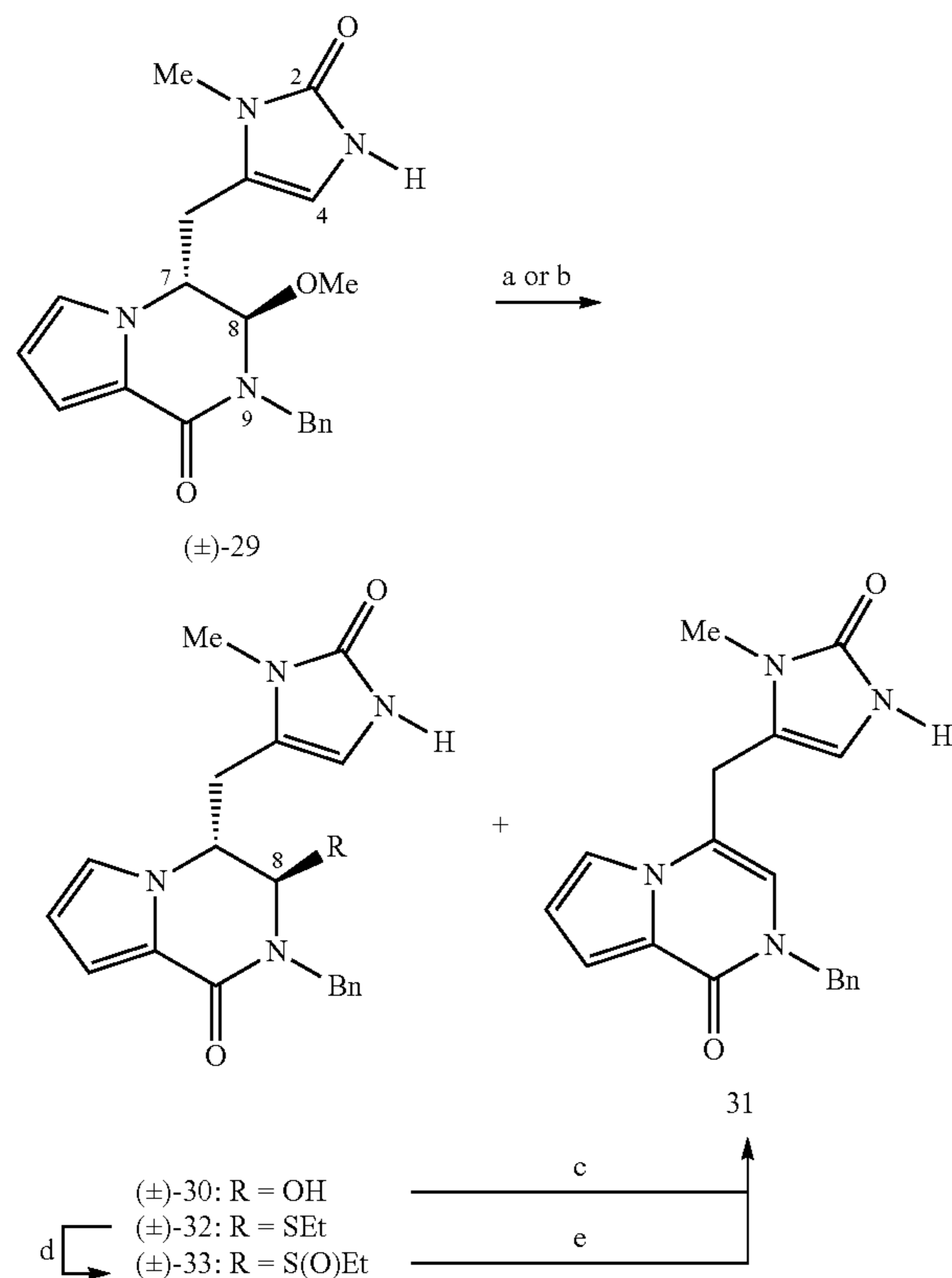
Scheme 6. Formation of pyrrolopyrazinone 31 under various conditions.
