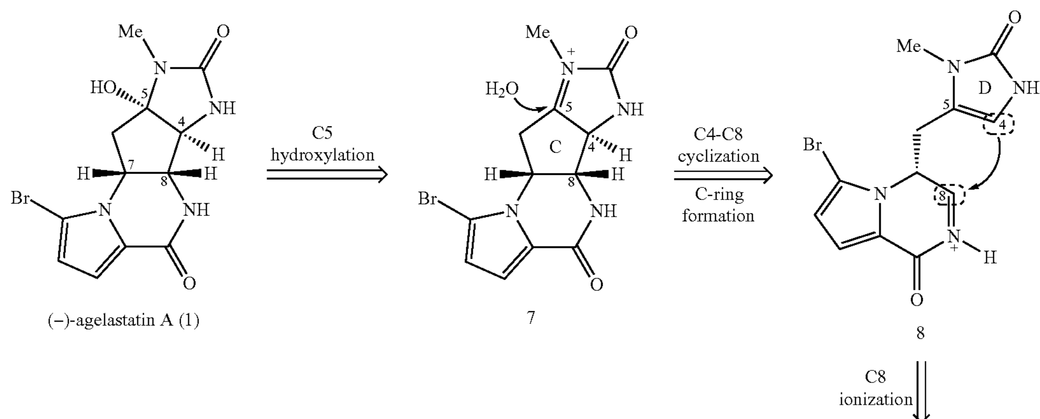
Scheme 1. Retrosynthetic analysis of (-)-agelastatin A (1).
