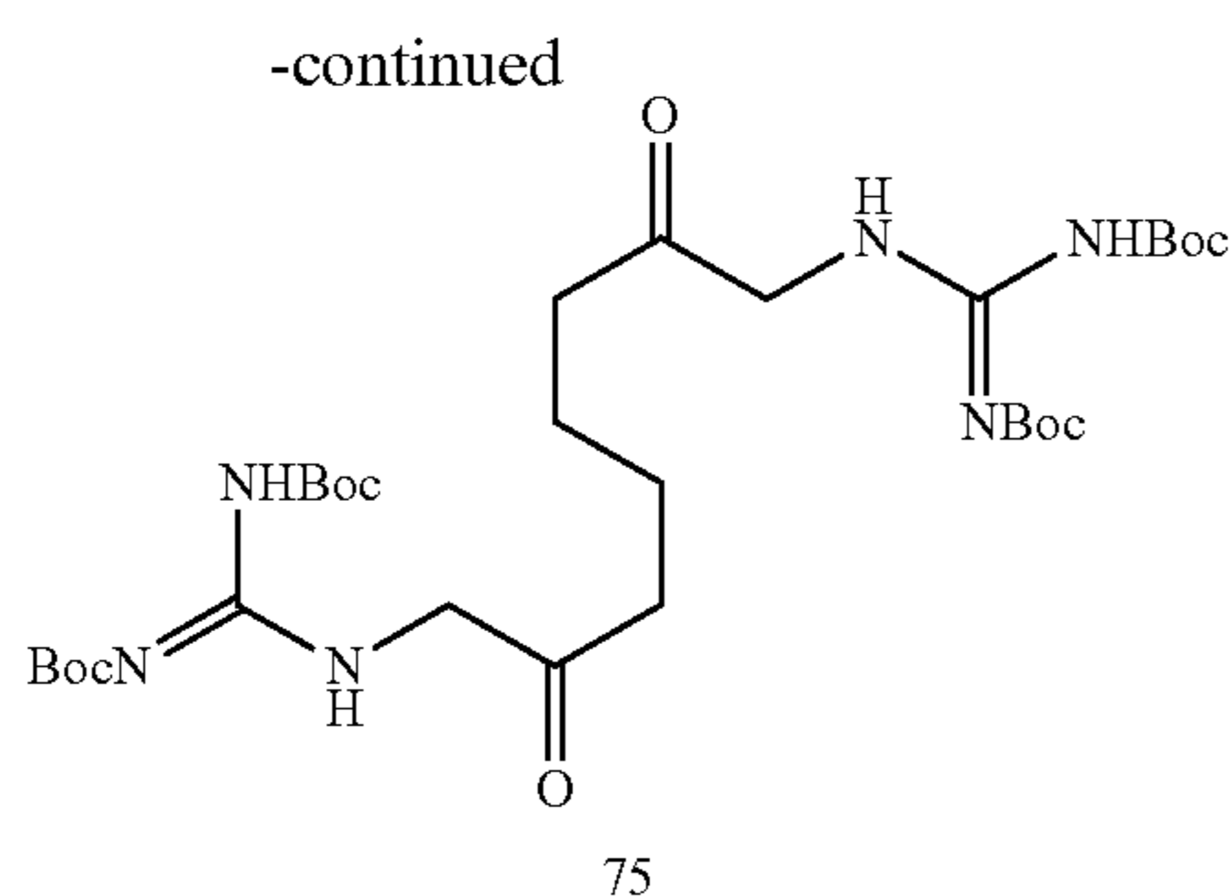
(E,E)-1,1'-(2,7-Dioxooctane-1,8-diyl)bis(2',3-di-bocguanidine) (75)
