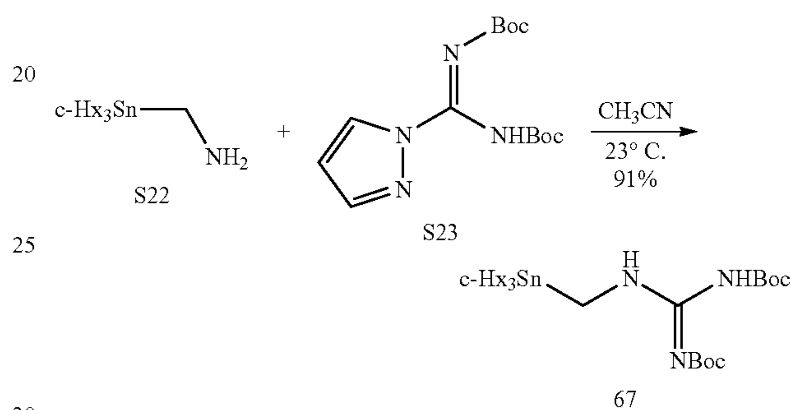
1-((Tricyclohexylstannyl)methyl)-N,N'-di-tert-butylcarbamoylguanidine (67)
