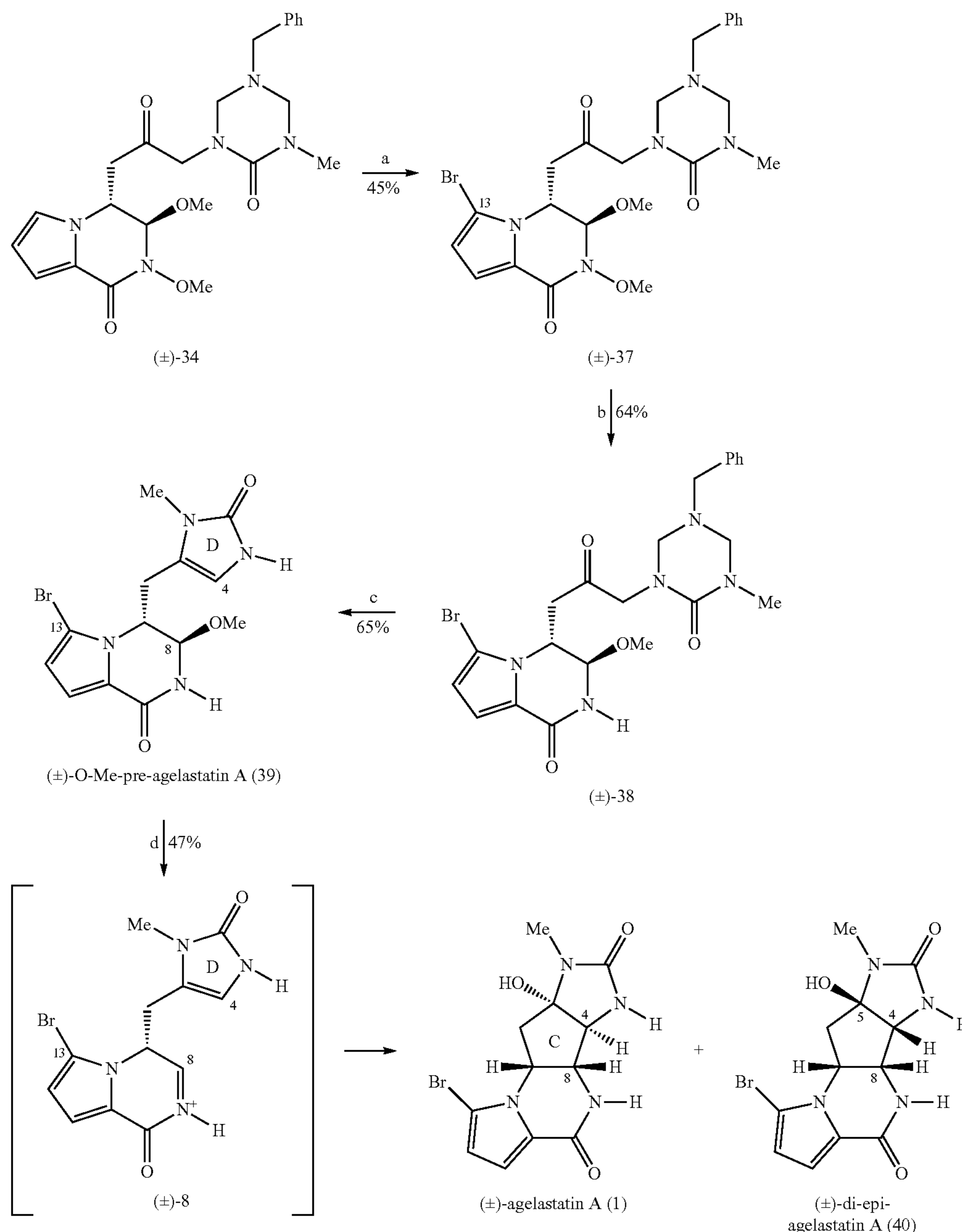
Scheme 8. First generation total synthesis of (±)-agelastatin A (1).
