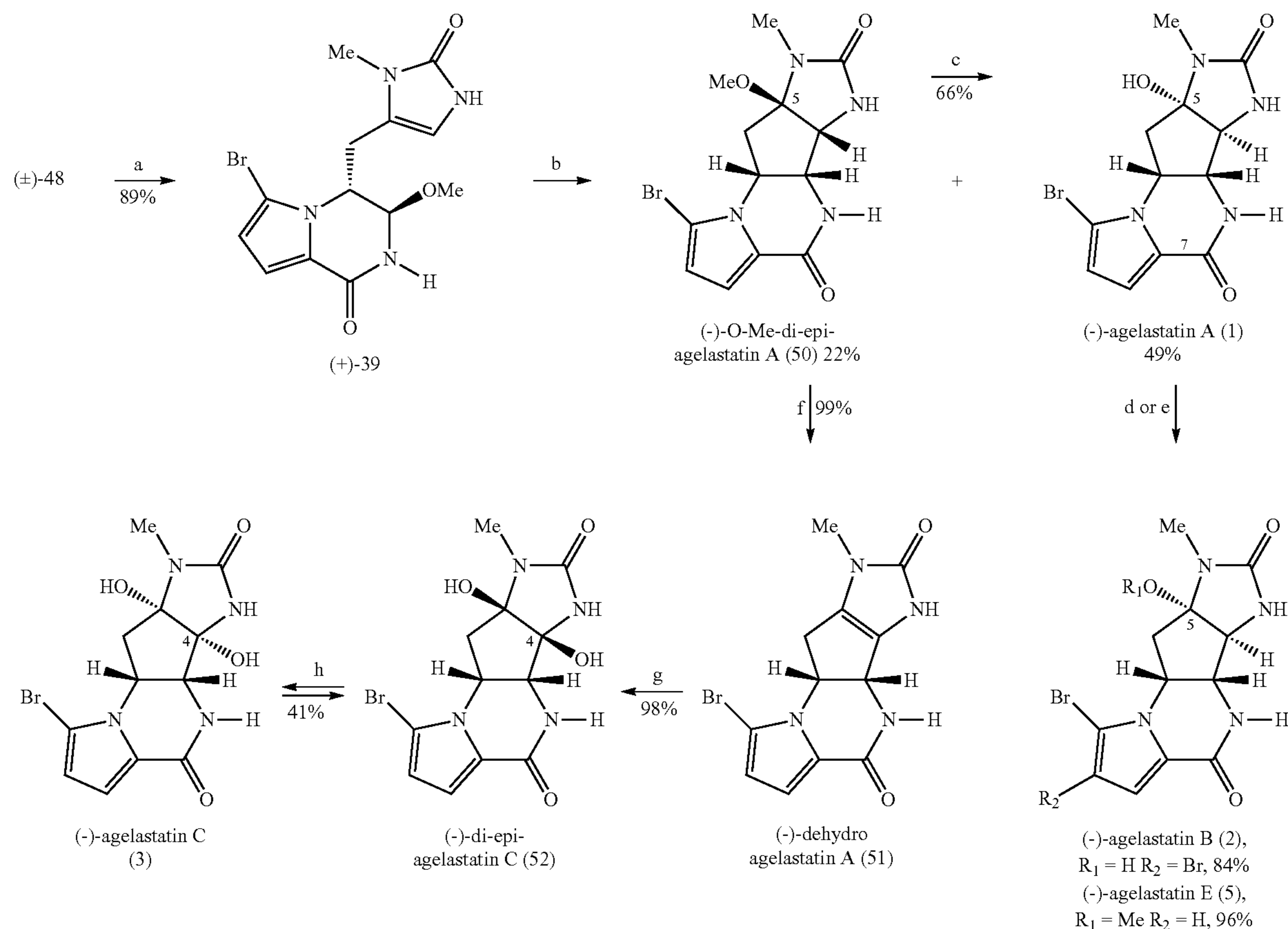
Scheme 11. Enantioselective synthesis of (-)-agelastatins A-C (1-3) and E (5).
