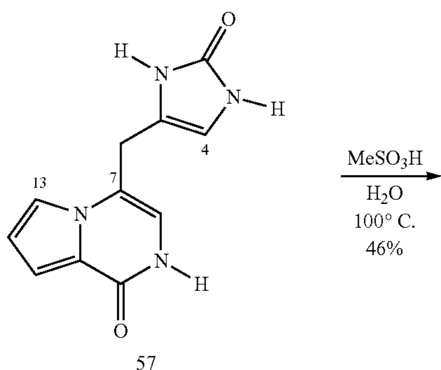
Scheme 13. Formation of the C4-C13 bond upon acidic treatment of enamide 57.
