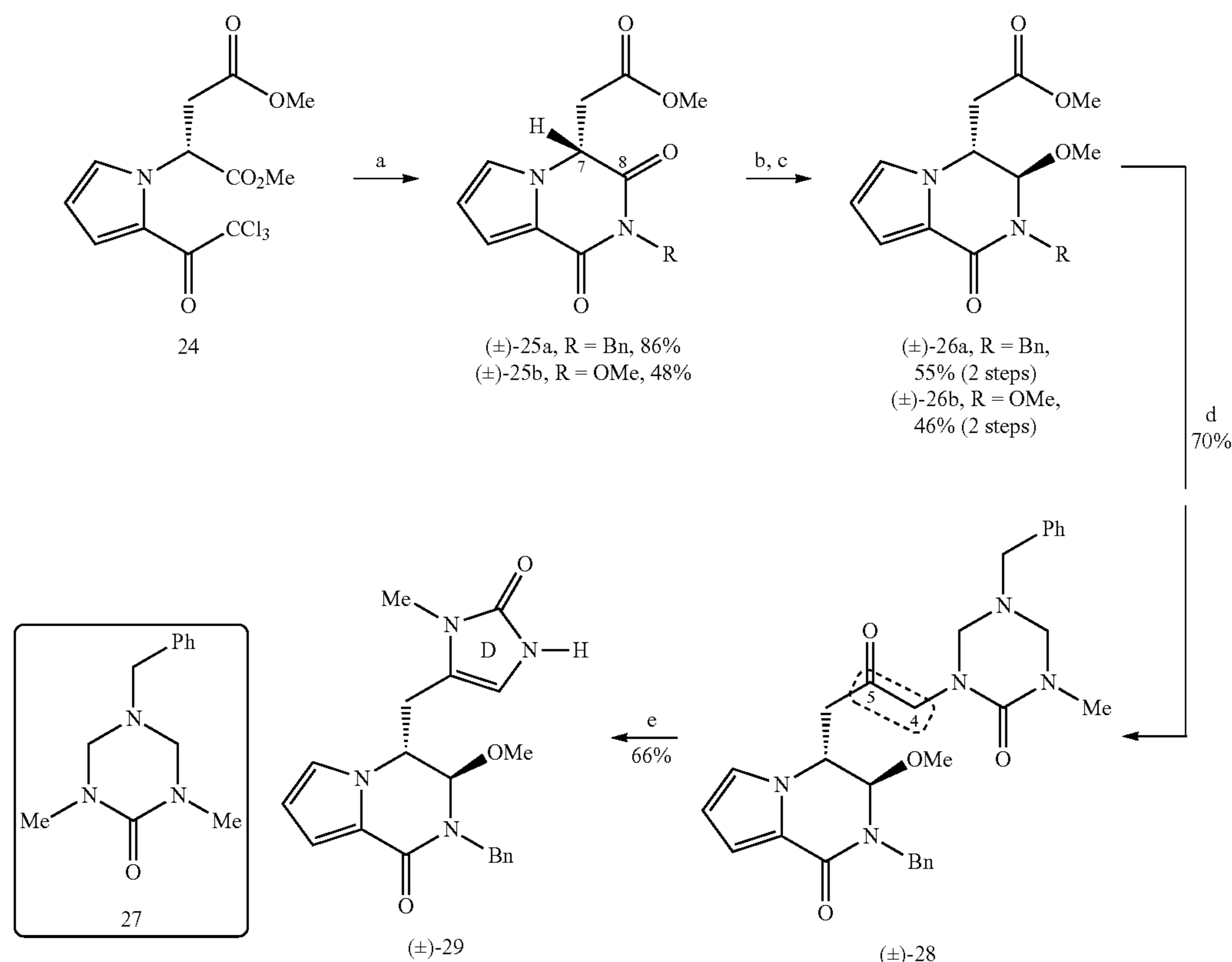
Scheme 5. Synthesis of imidazolone ( \pm )-29.
