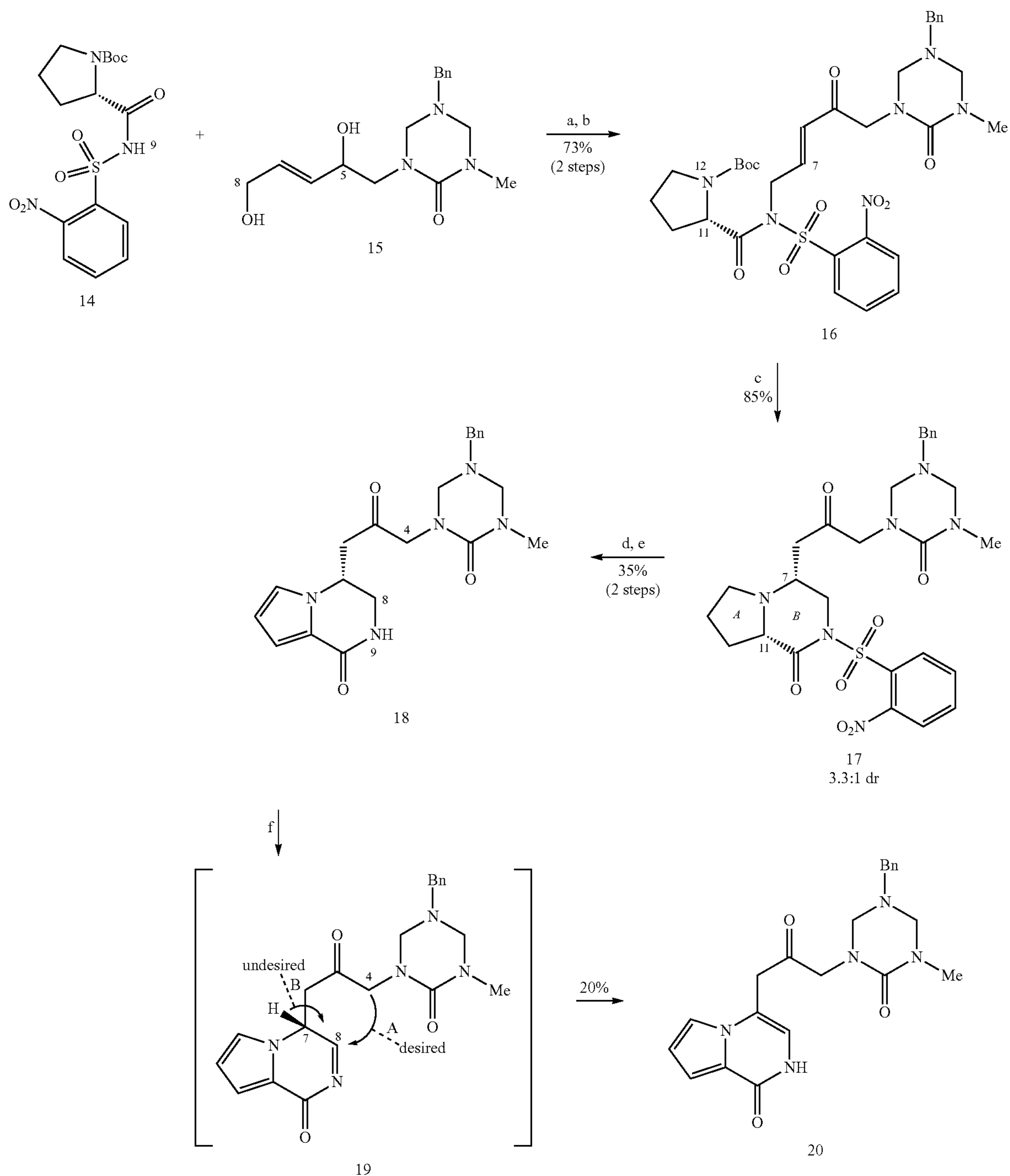
Scheme 3. Synthesis of key bicycle 18 and attempted oxidation-cyclization.
