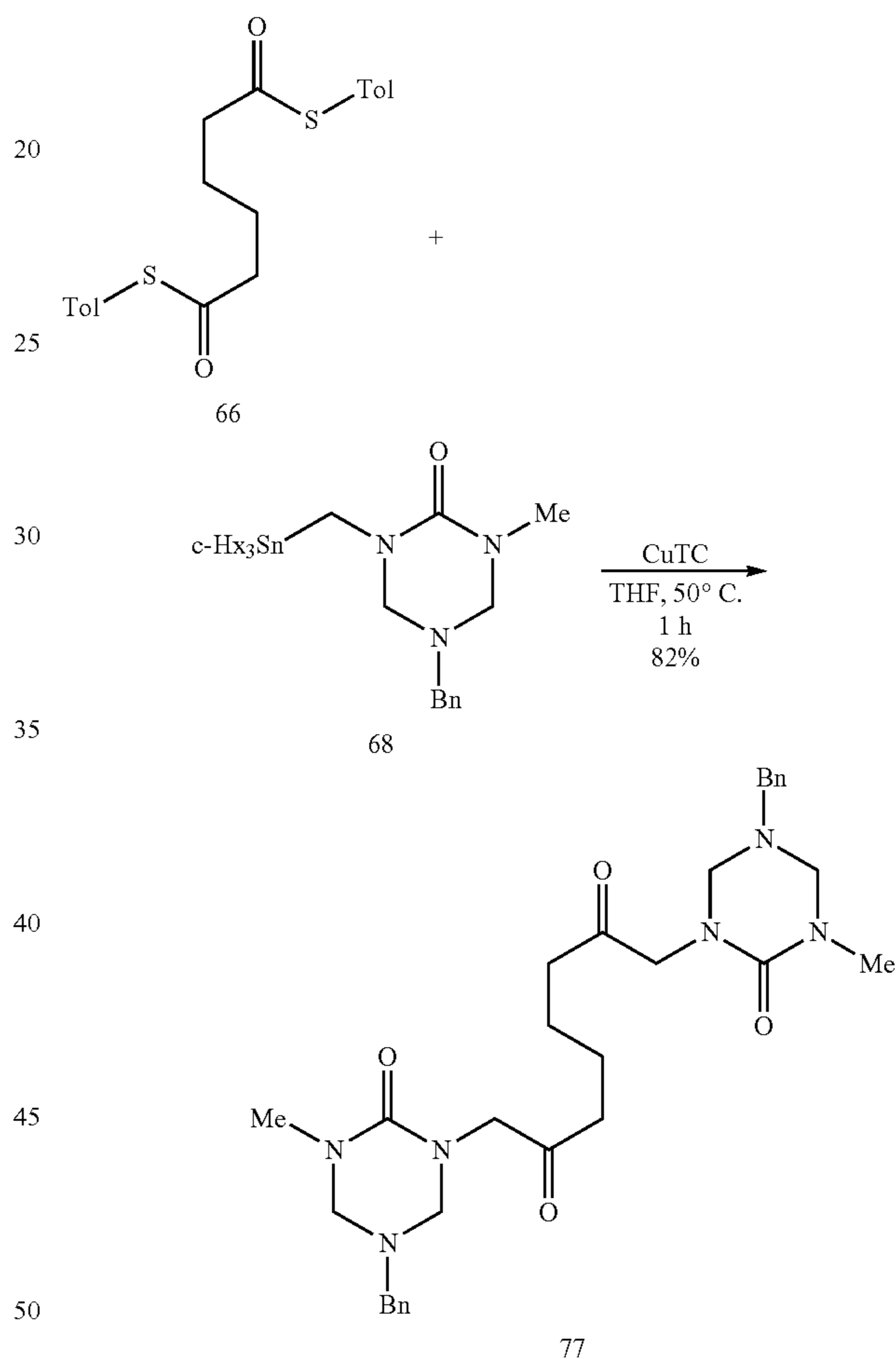
1,8-Bis(5-benzyl-3-methyl-2-oxo-1,3,5-triazinan-1-yl)octane-2,7-dione (77)
