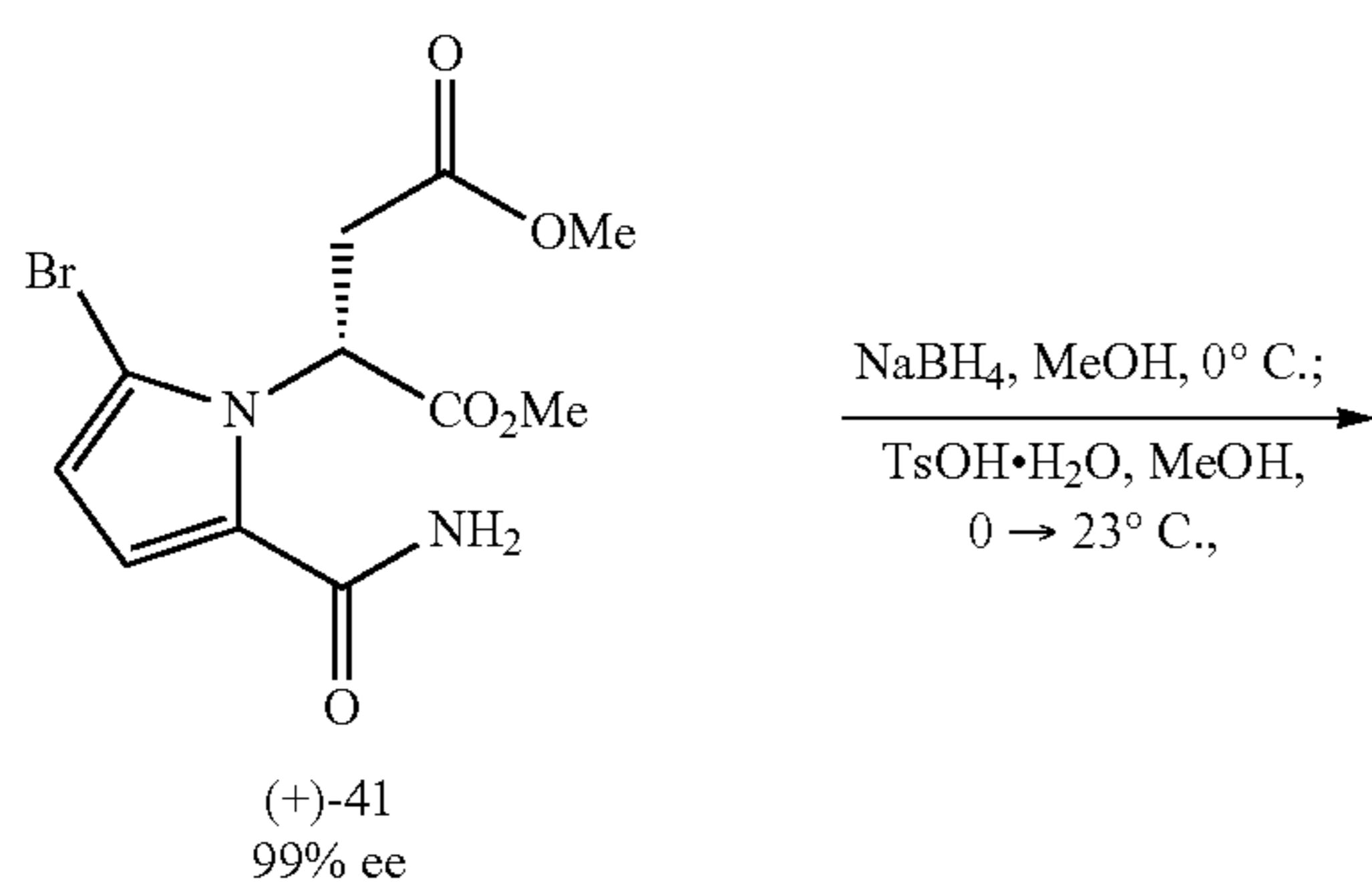
Scheme 10. Synthesis of bicycle (+)-44.
