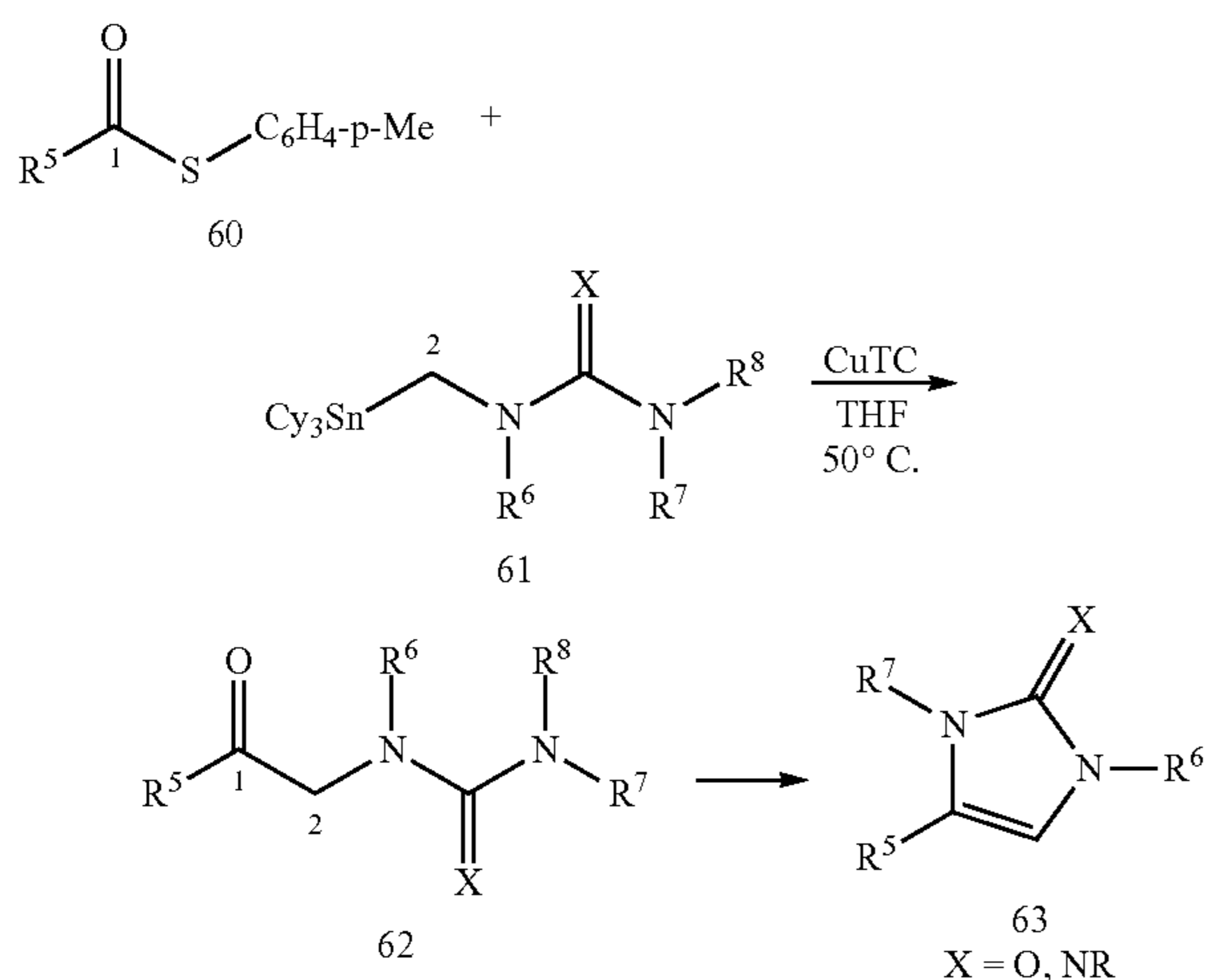
Scheme 15. A versatile synthesis of azaheterocycle 63.
