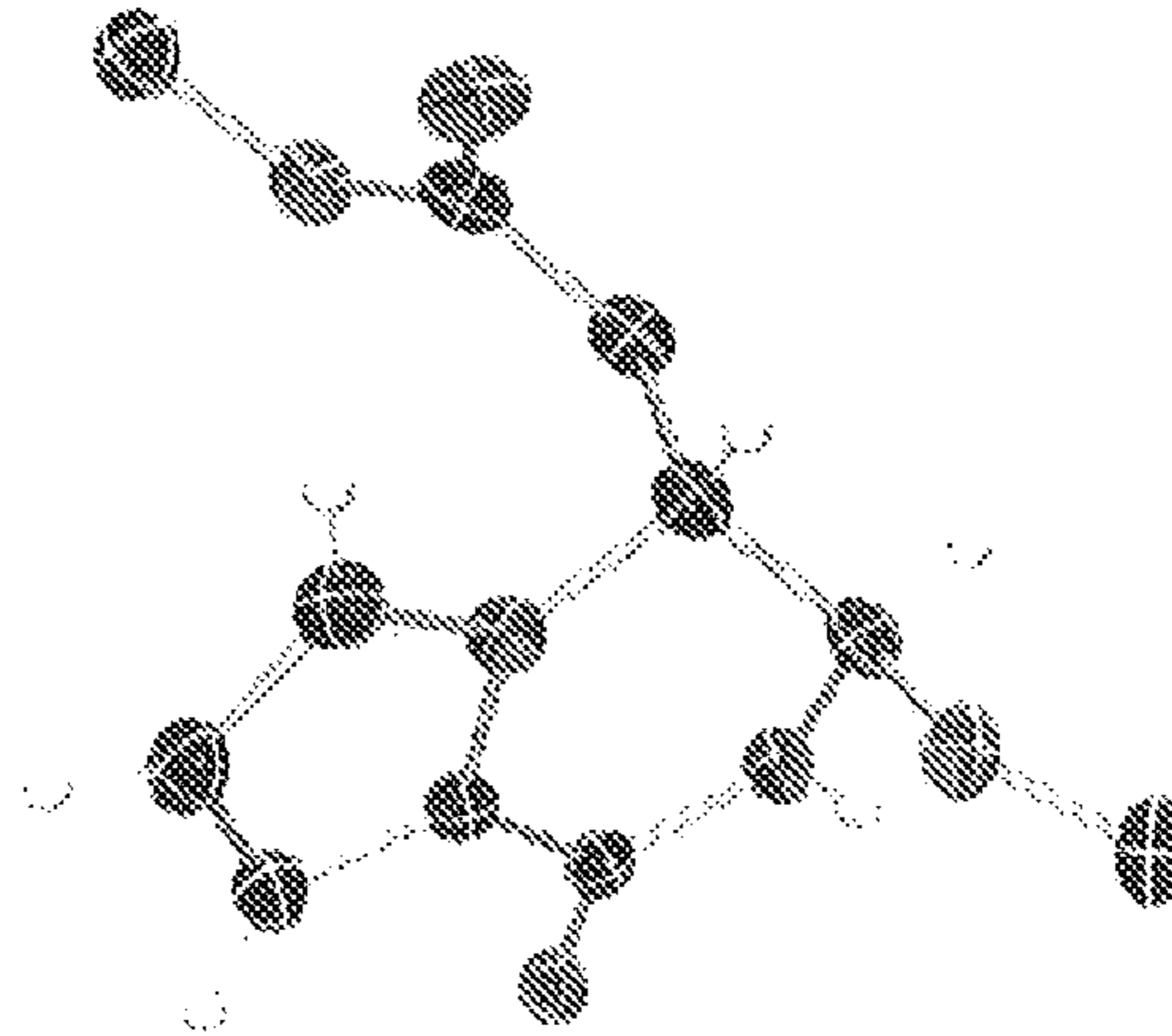
View 3:
