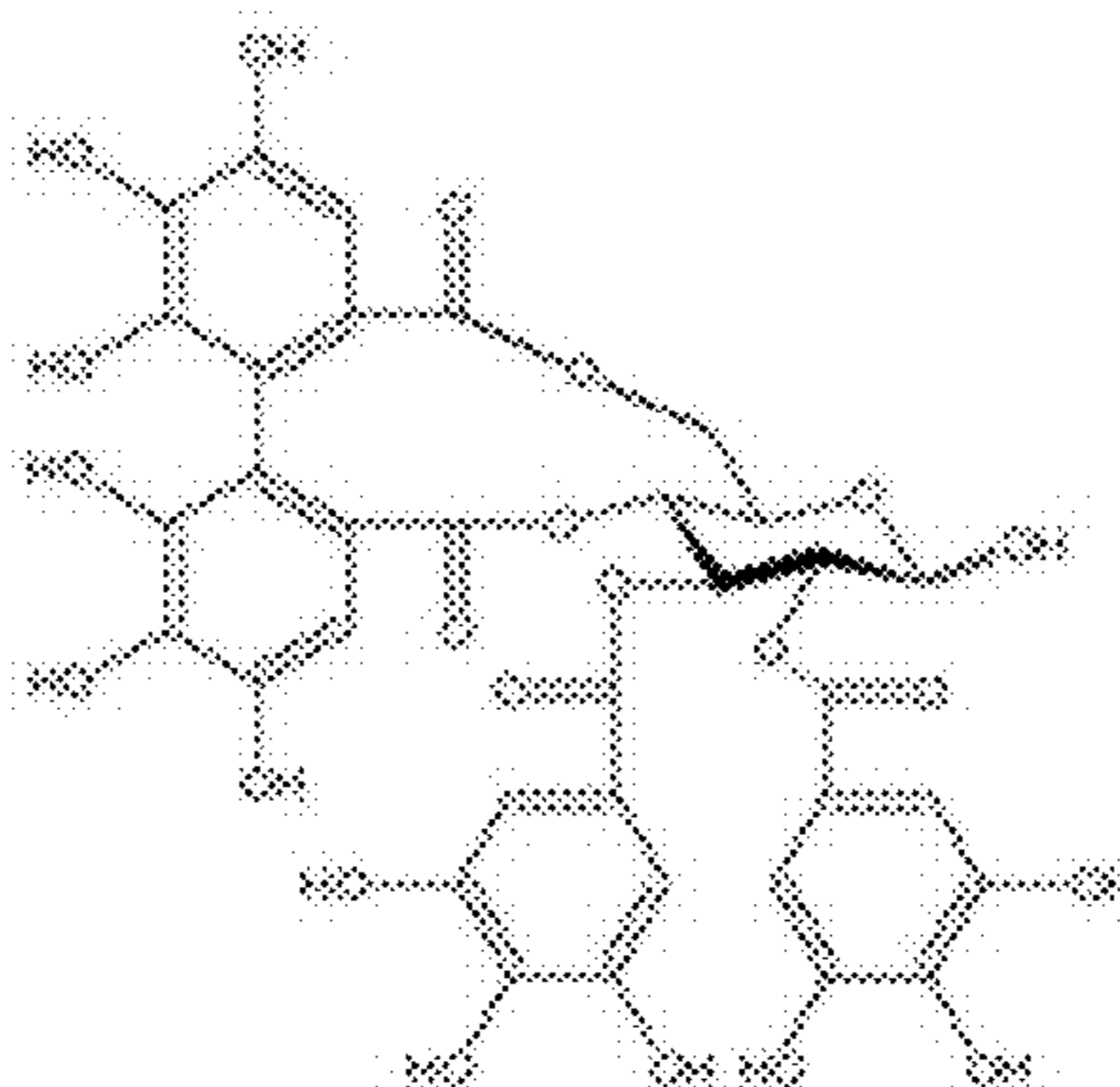
Tellimagrandin (TL)
