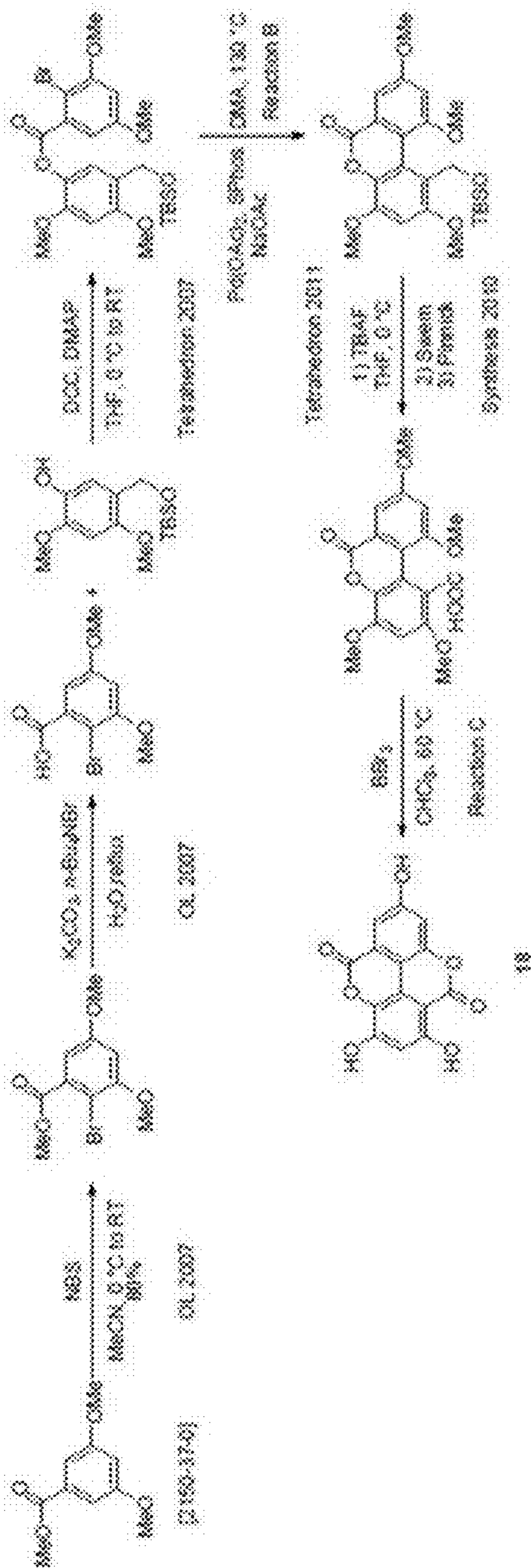
Compounds 17 & 18 (cont.)
