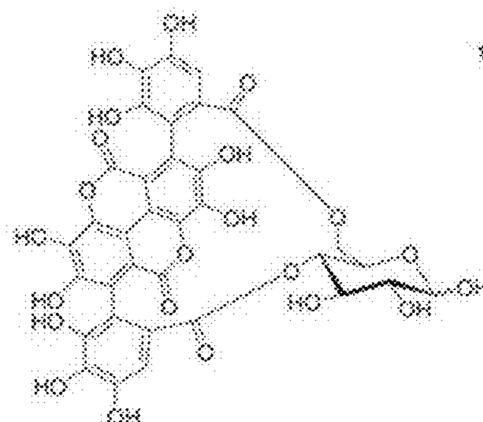
Punicalin (PB)
