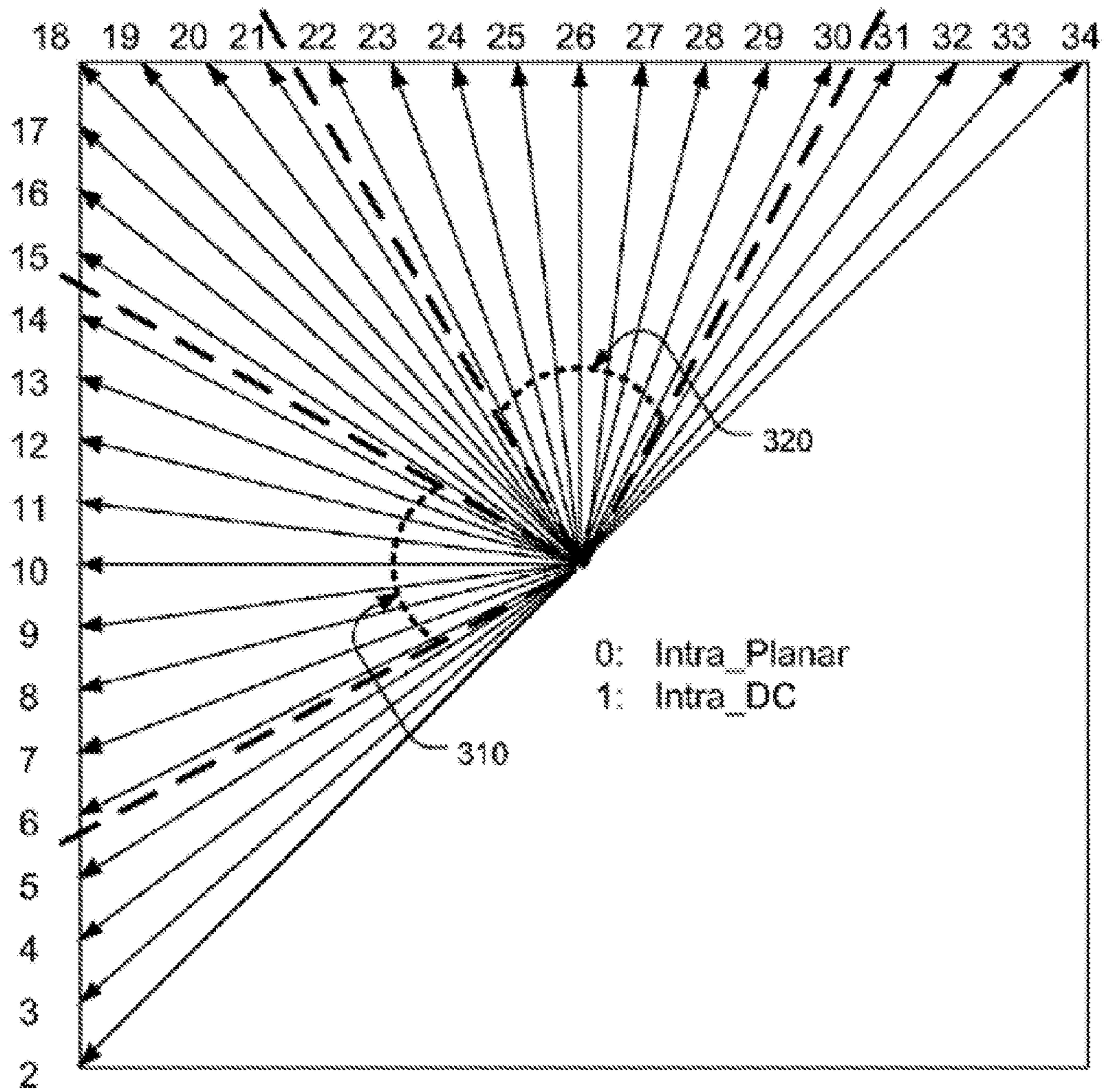
Fig. 3 (PRIOR ART)
