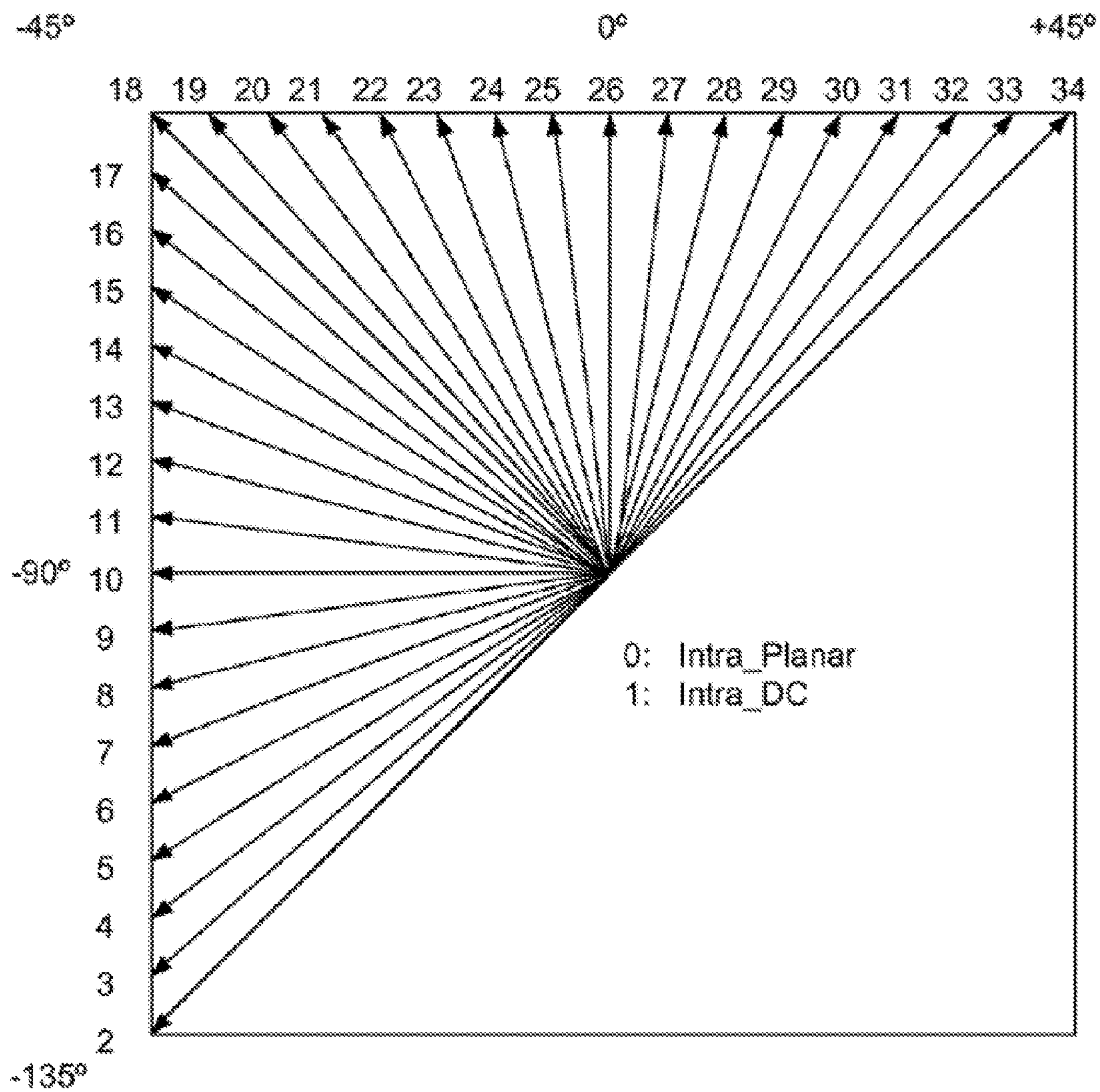
Fig. 1 (PRIOR ART)
