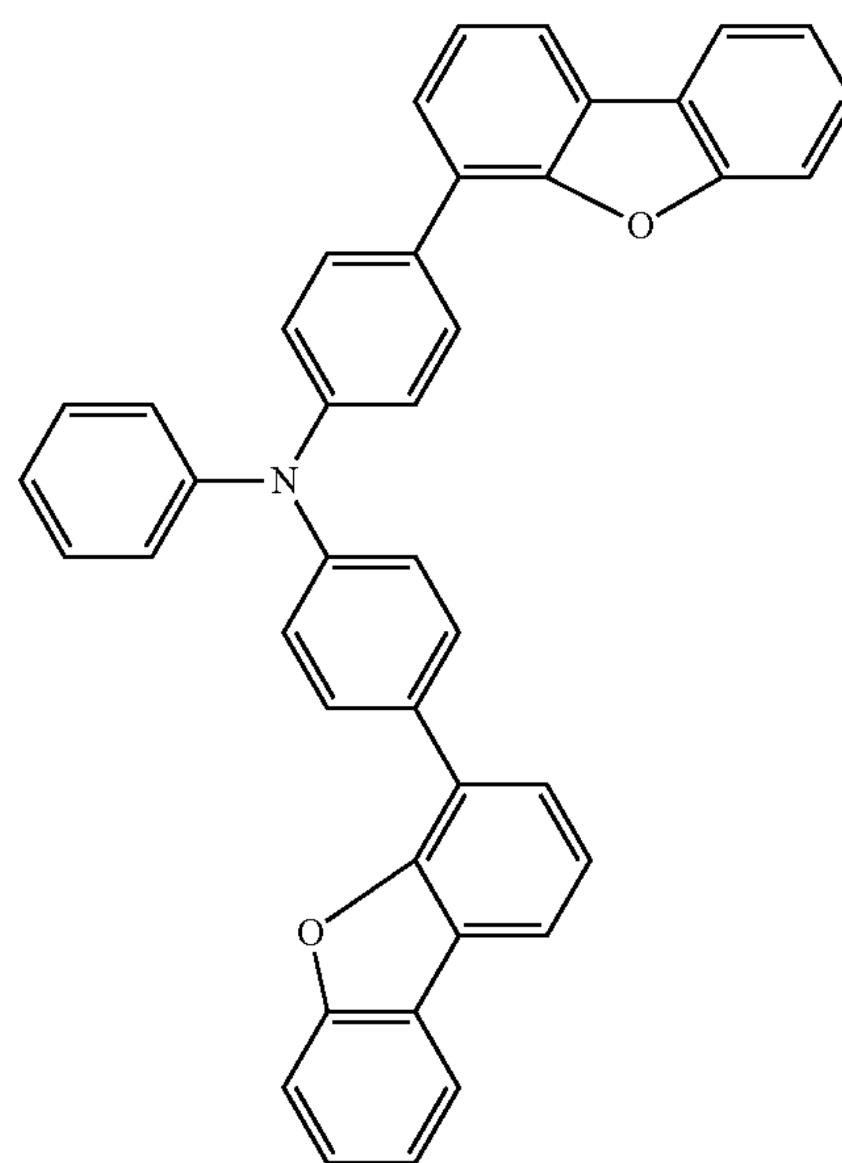
Chemical Formula 1-3
