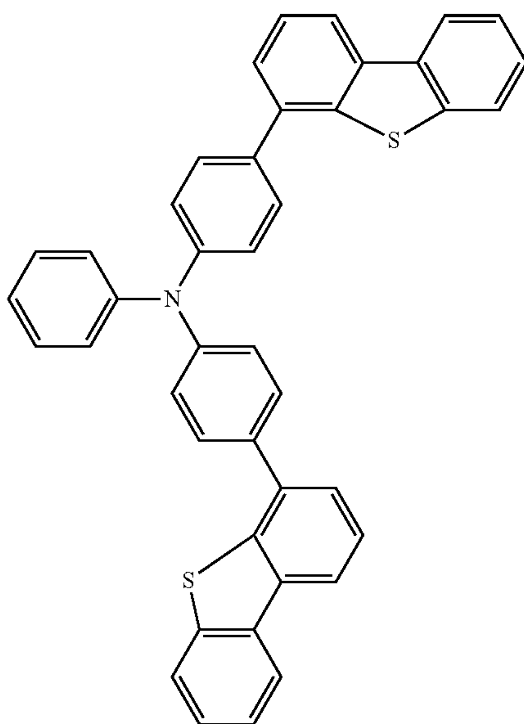
Chemical Formula 1-6
