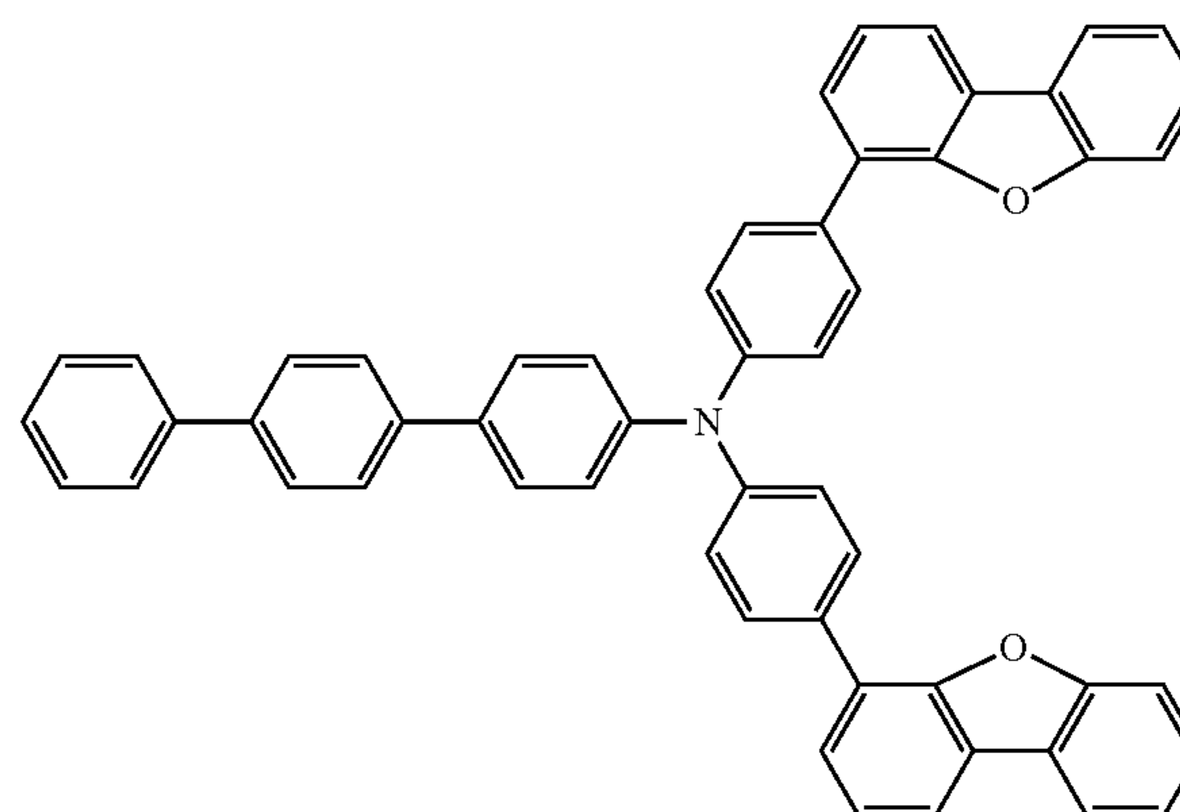
Chemical Formula 2-1
