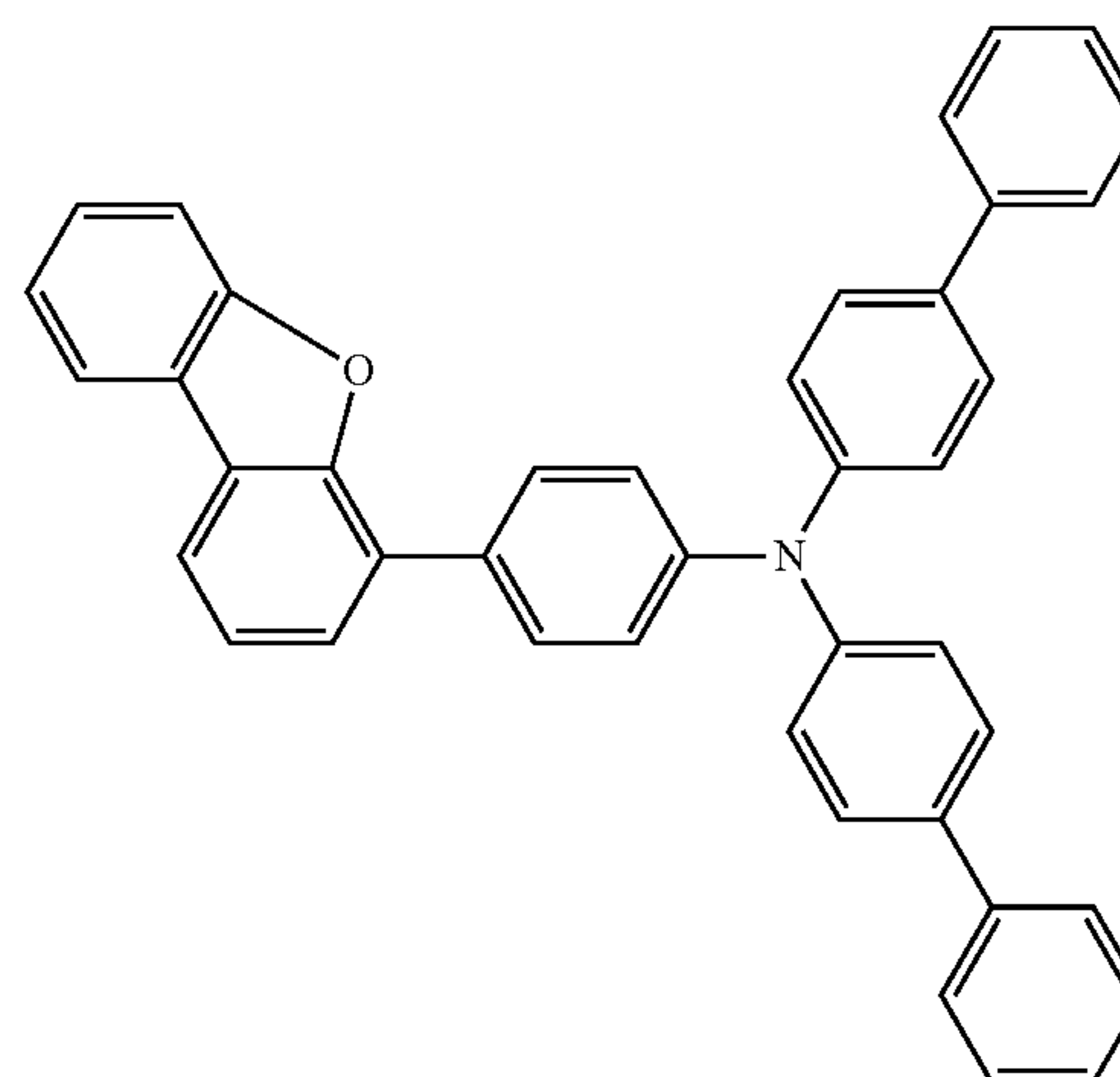
Chemical Formula 1-3
