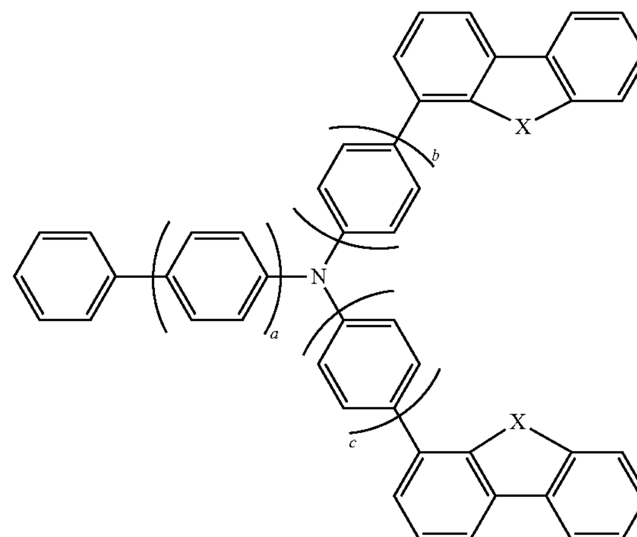
Chemical Formula 2
