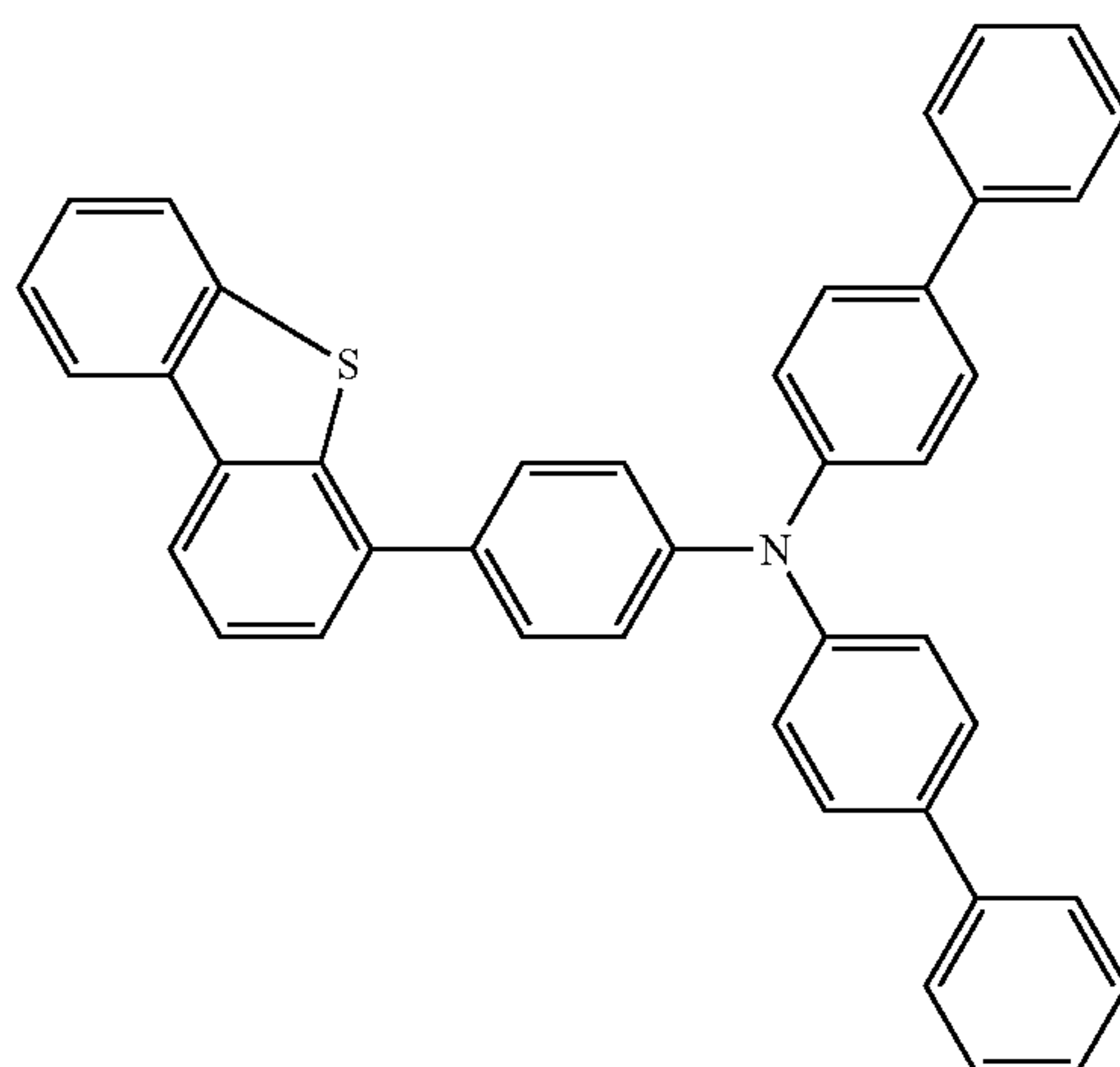
Chemical Formula 1-6
