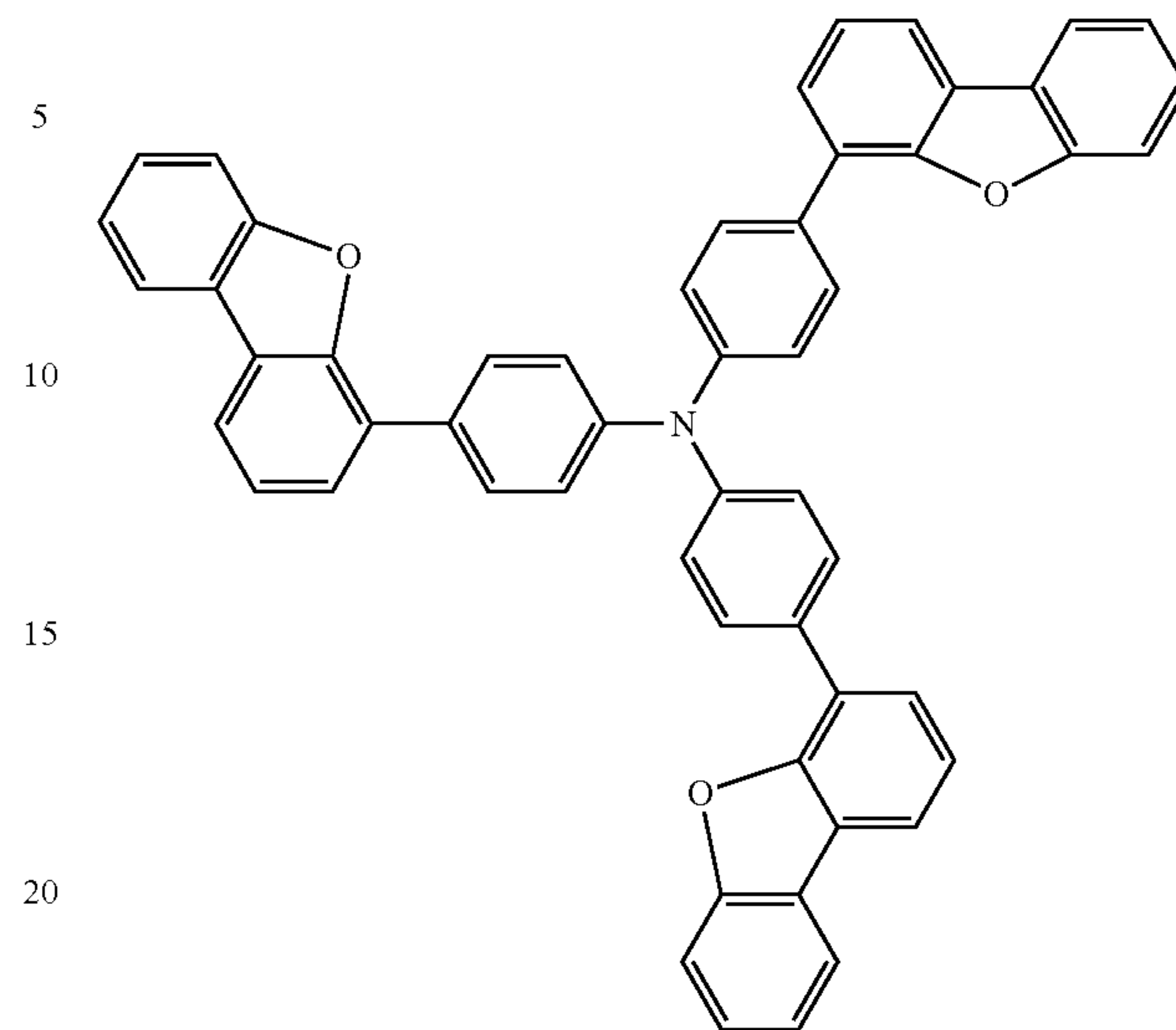
Chemical Formula 2-6
