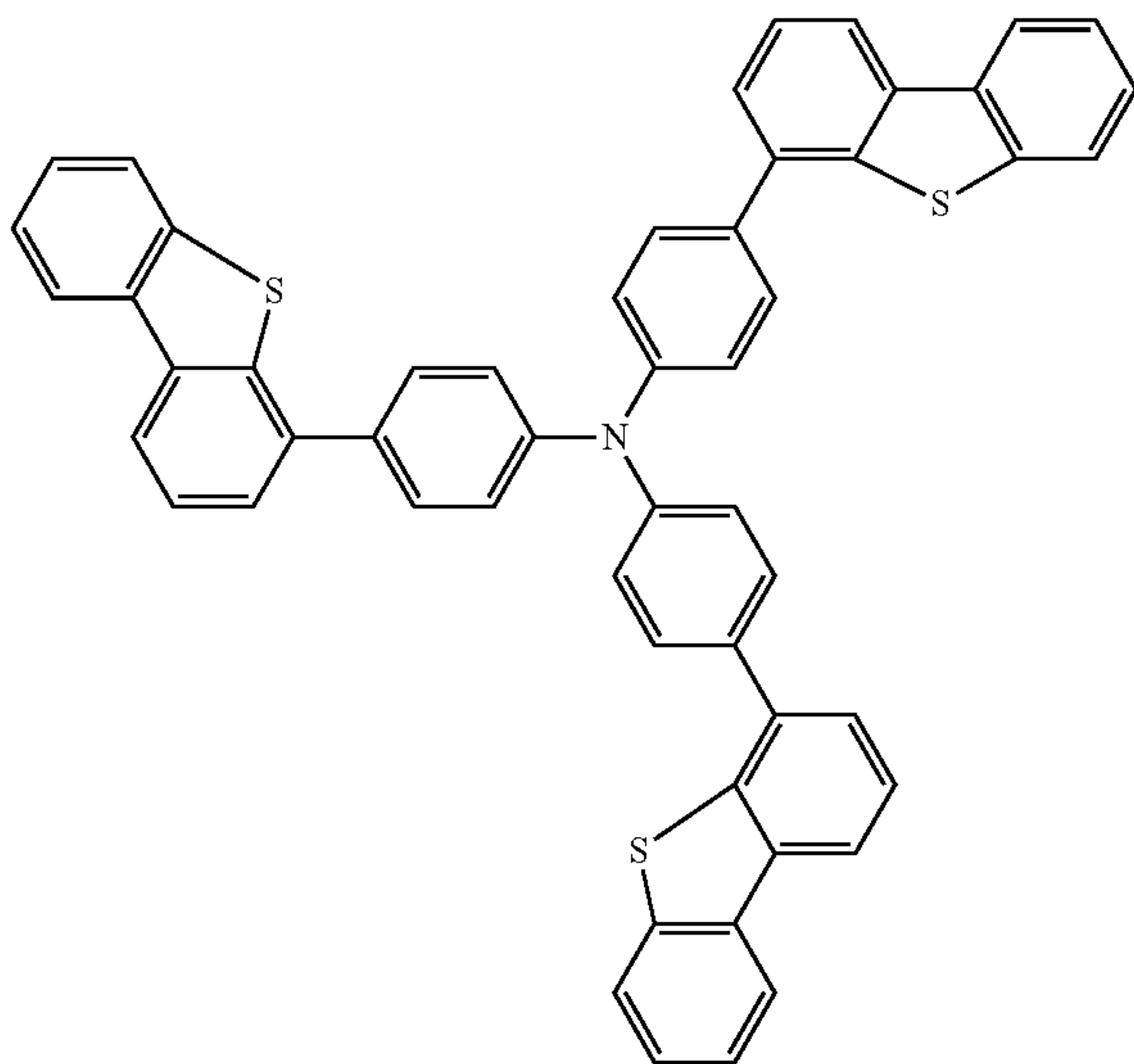
Chemical Formula 1-5
