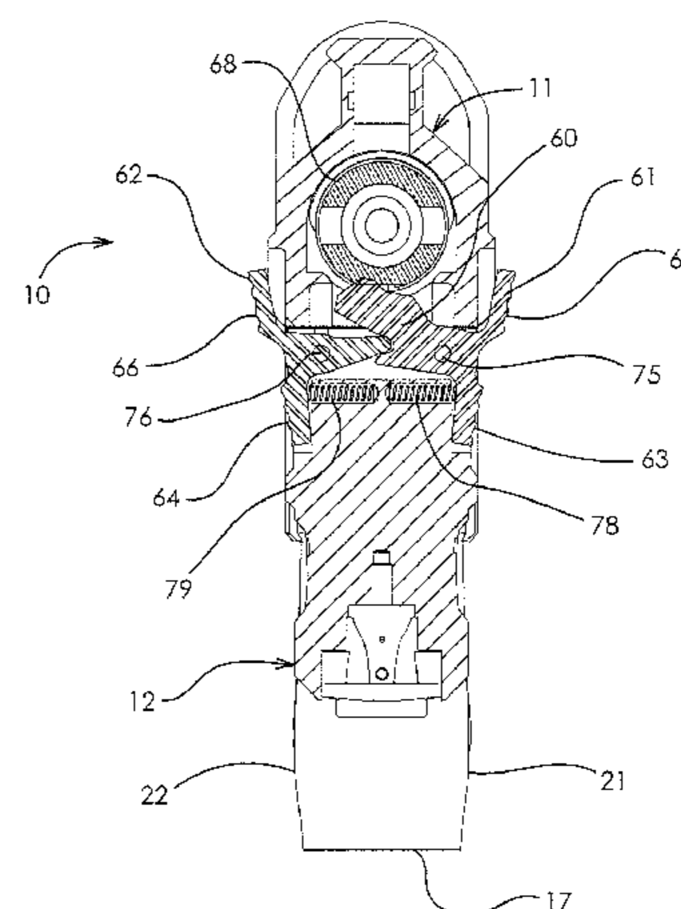
DETAIL D W/BOLT CATCH ENGAGED
