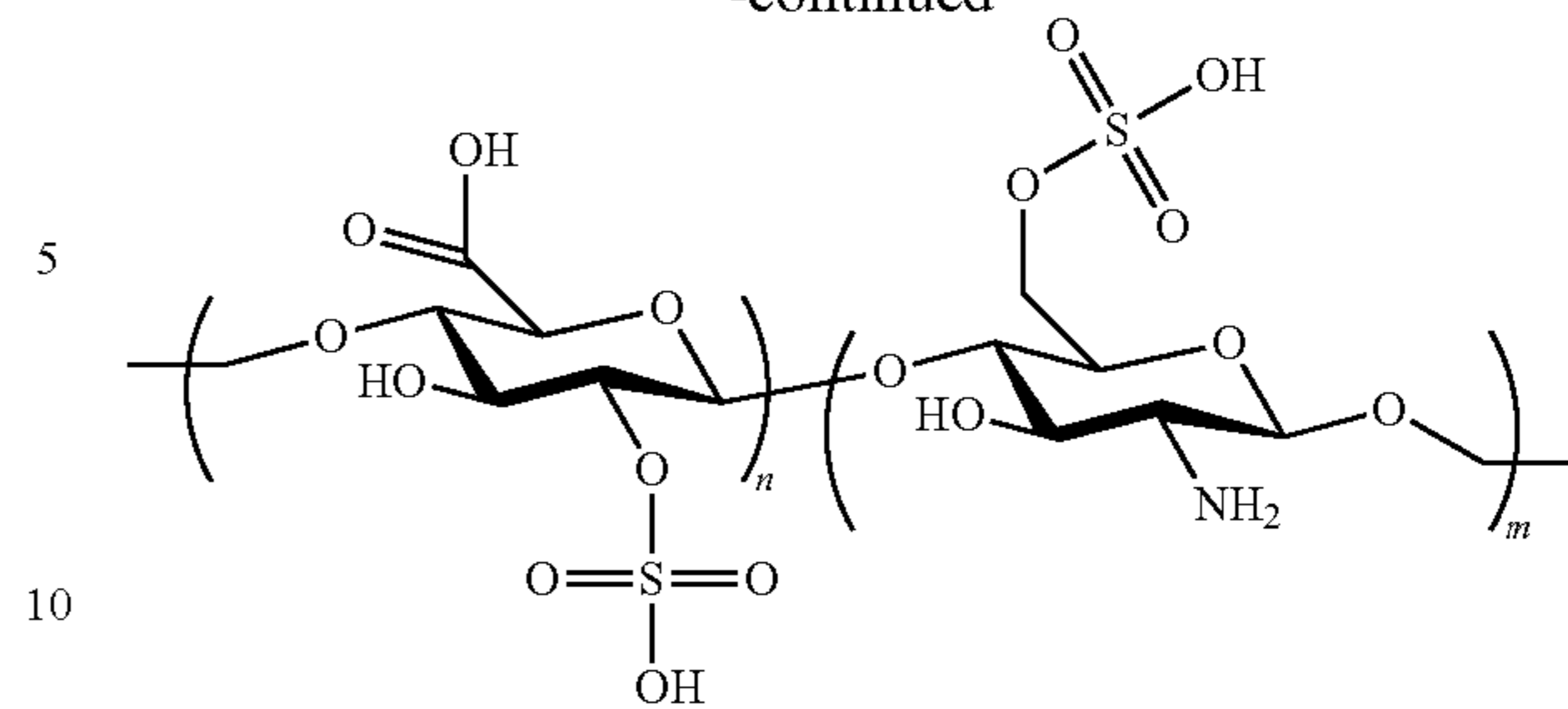
Heparin Amine
