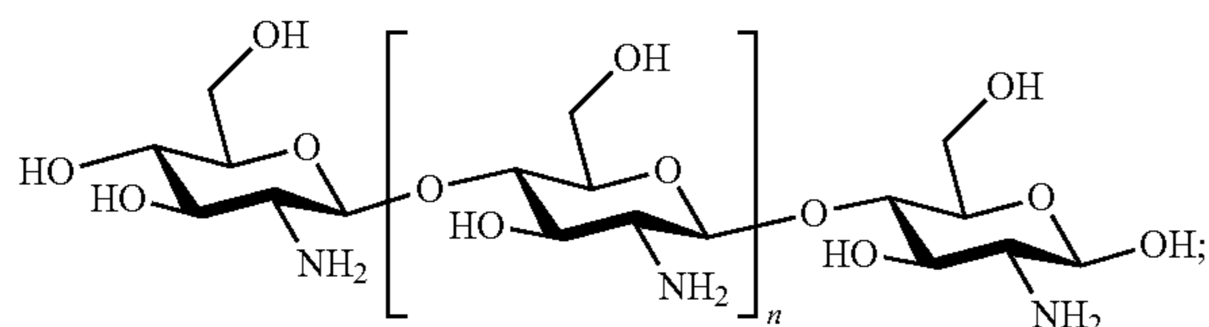
Chitosan
