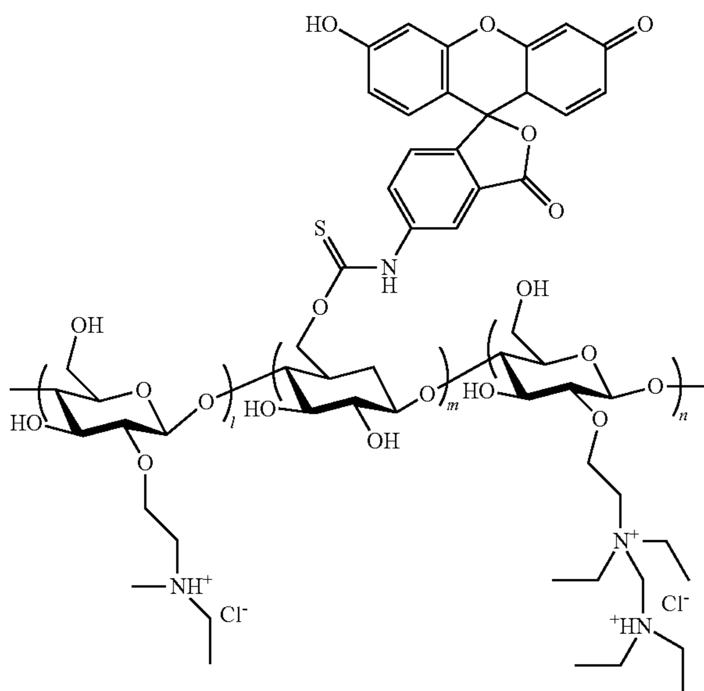
Dextran Fluorescein
