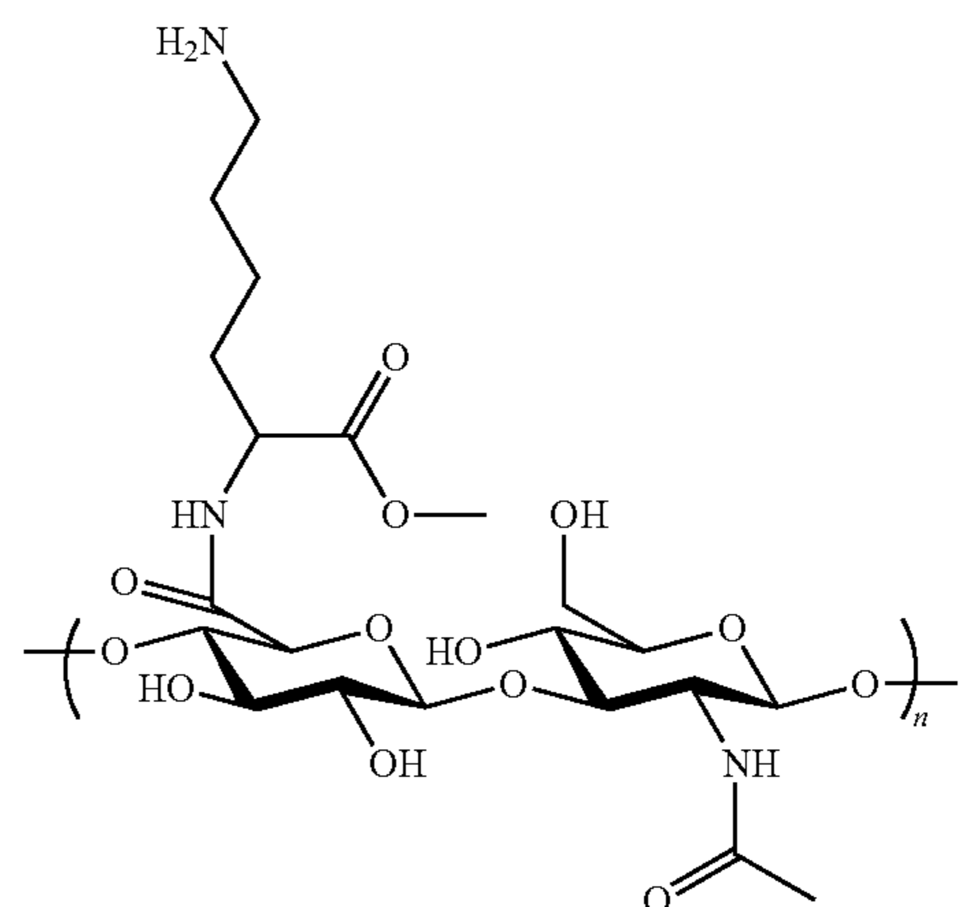
Hyaluronate Amine
