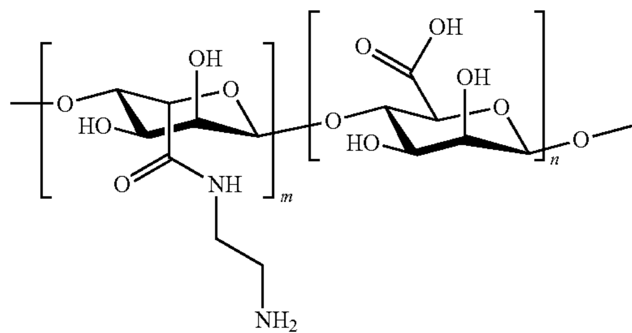
Alginate Amine
