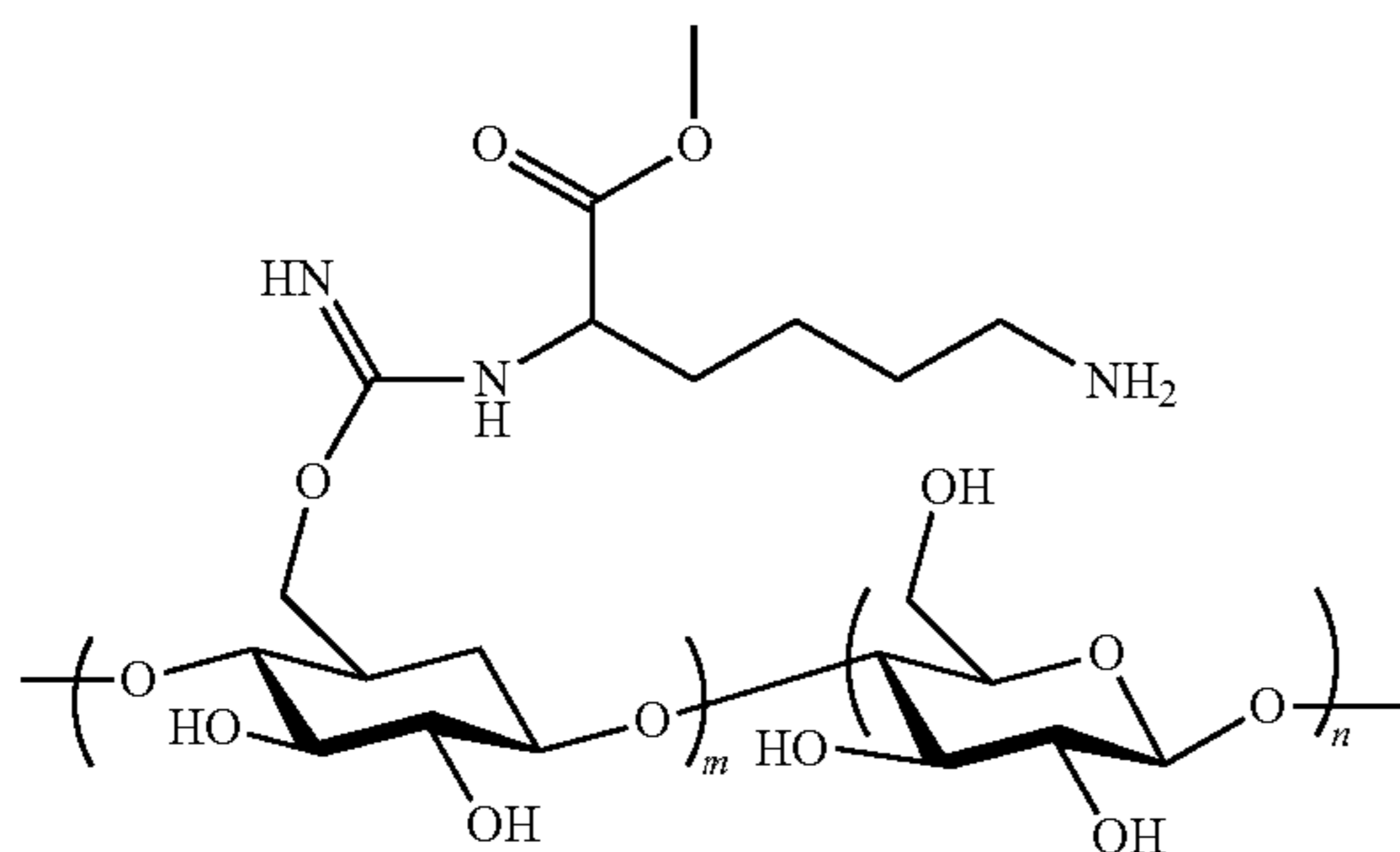
Dextran Amine
