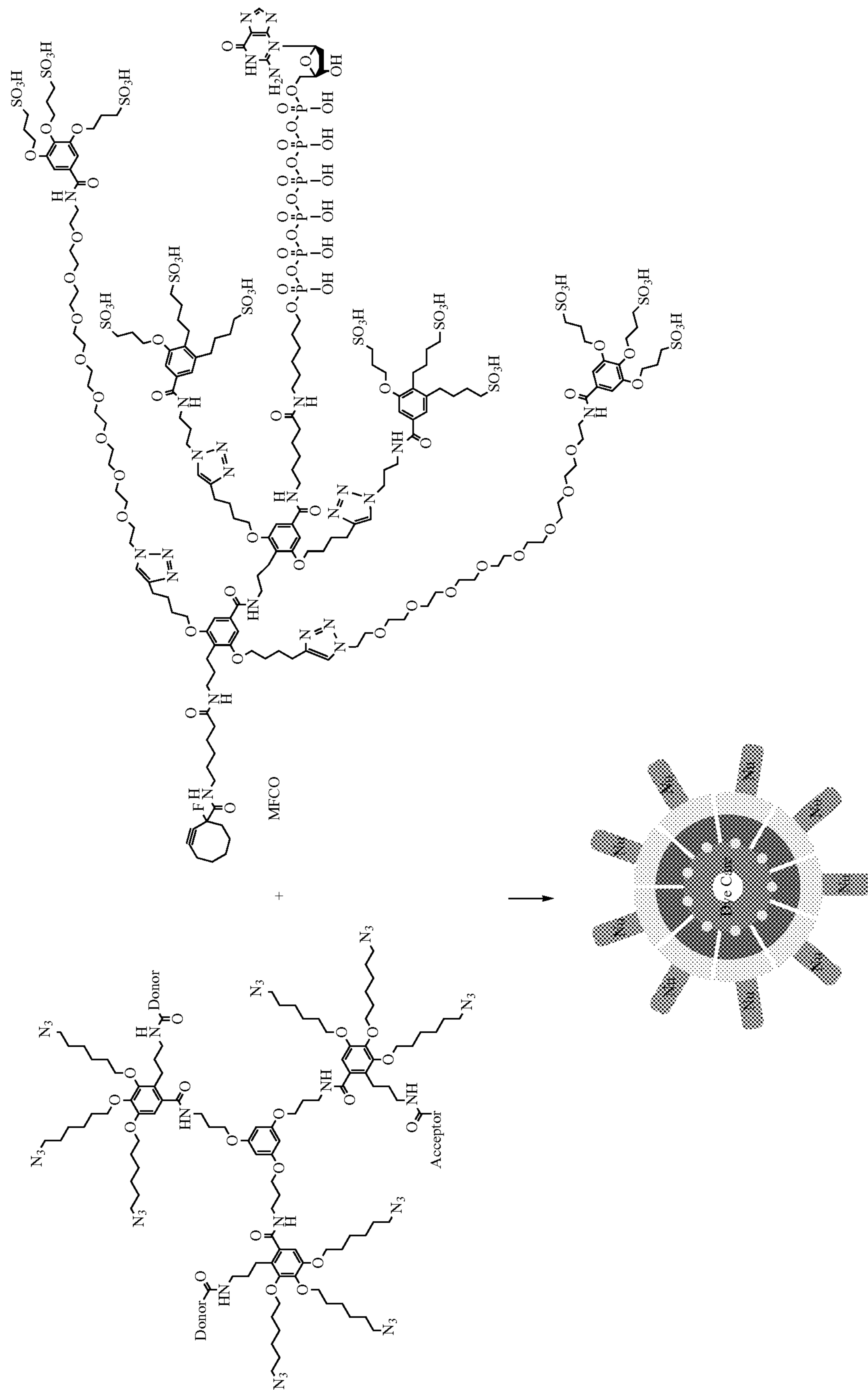
Scheme 17
