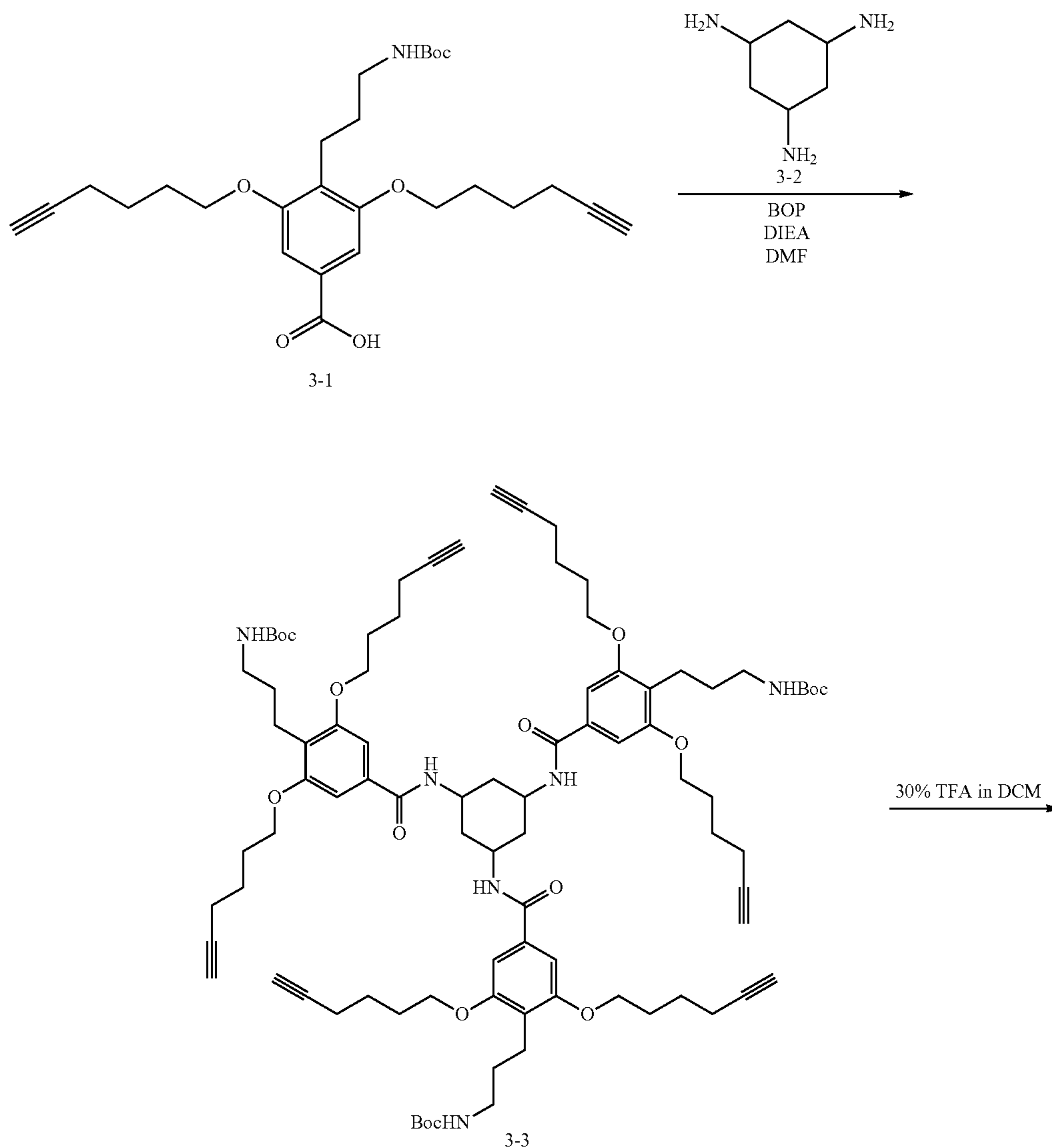
Scheme 25
