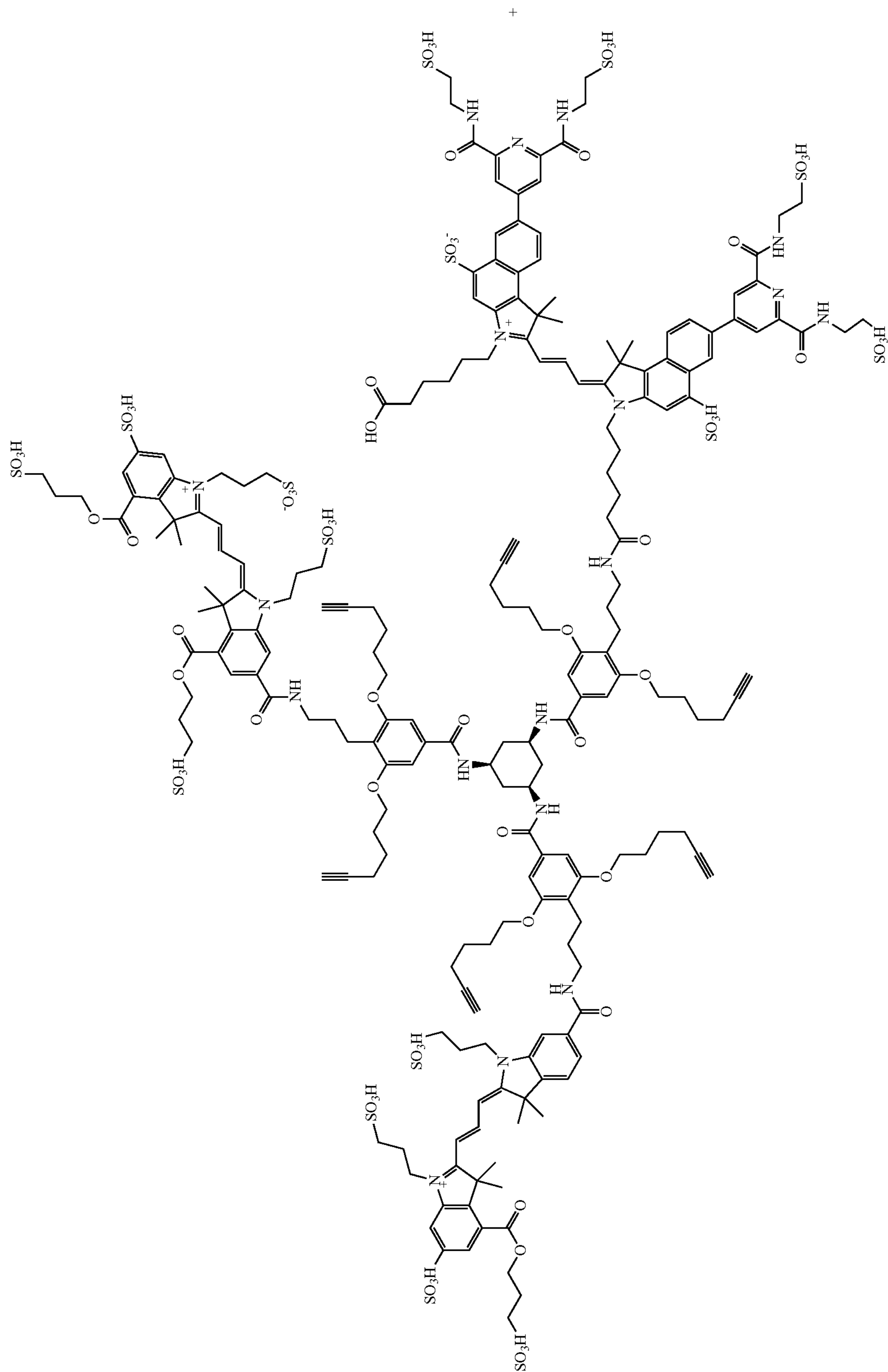
Scheme 26
