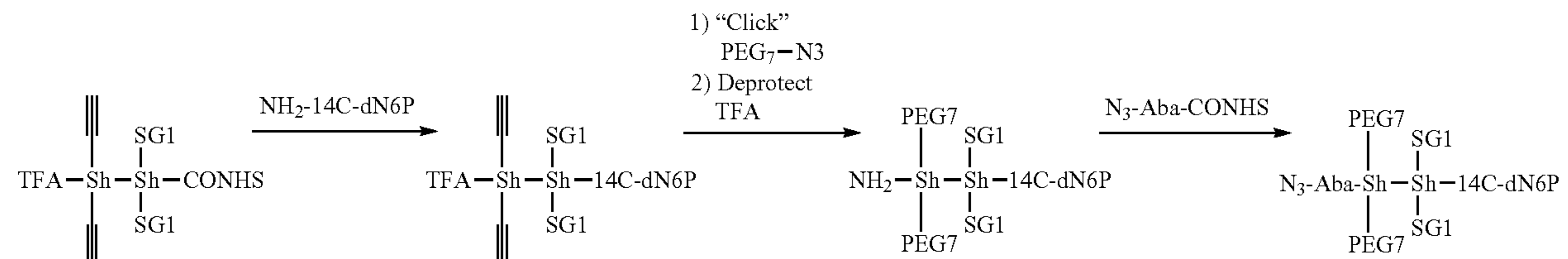
Scheme 7-1
