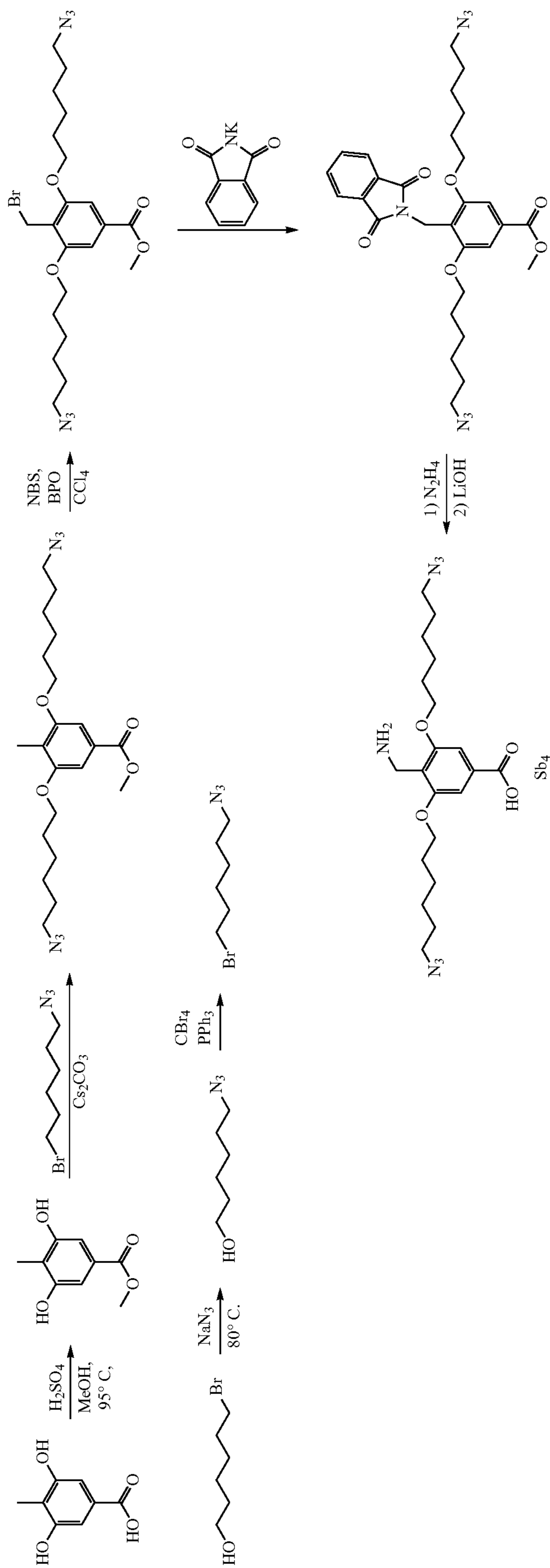
Scheme 13
