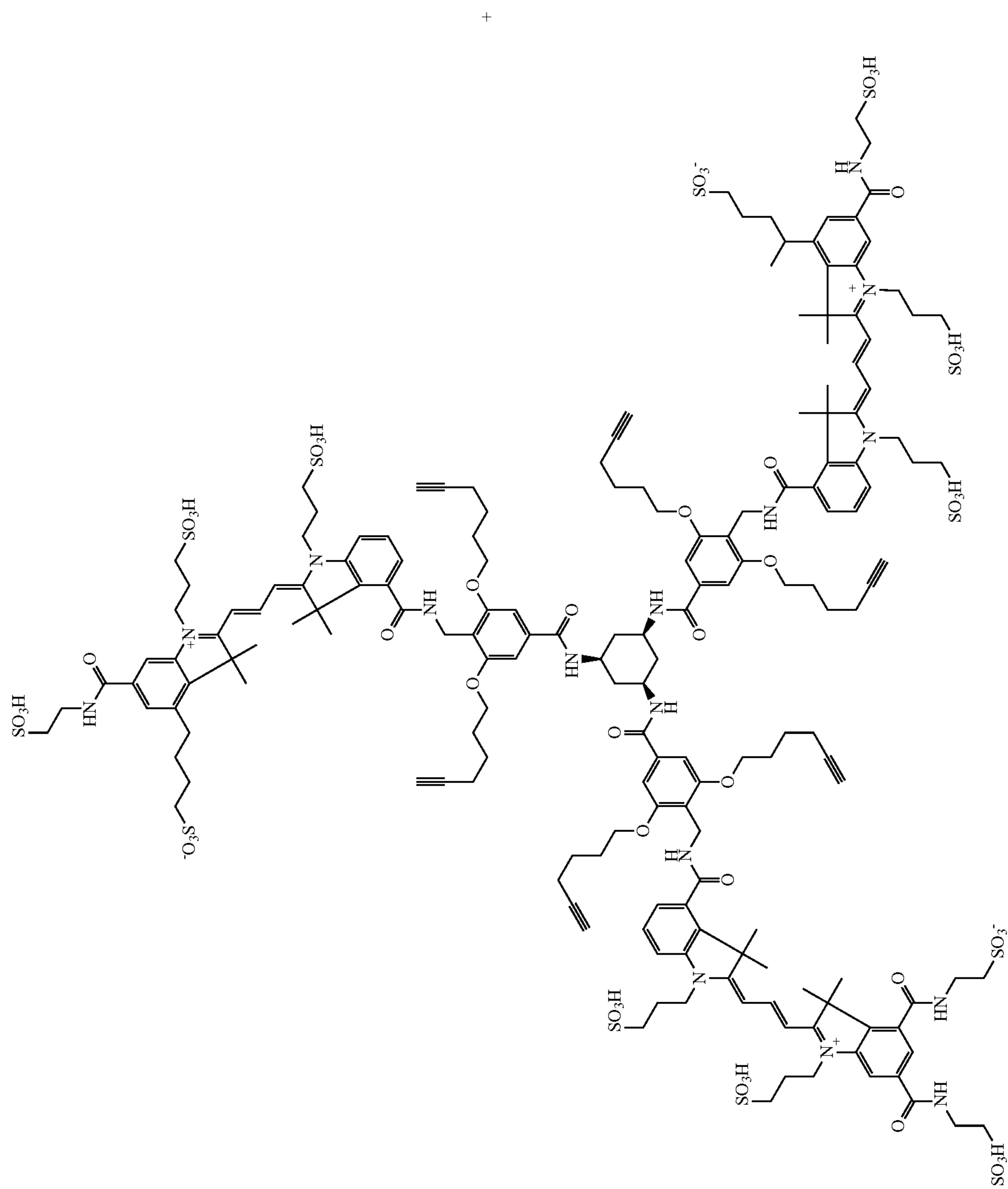
Scheme 9
