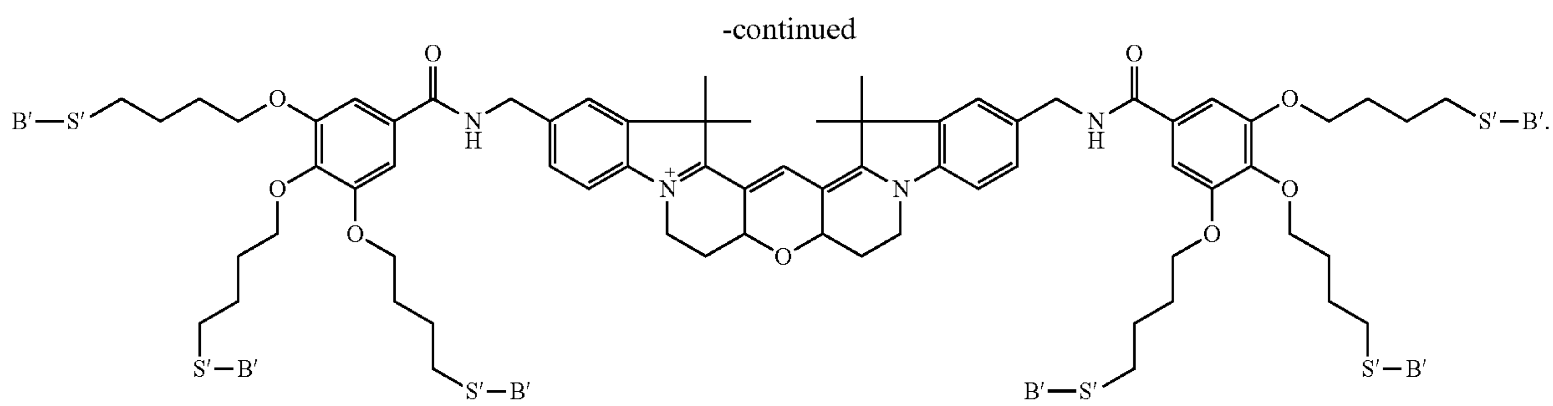
D012-(Gal) 2 (Hexavalent)
