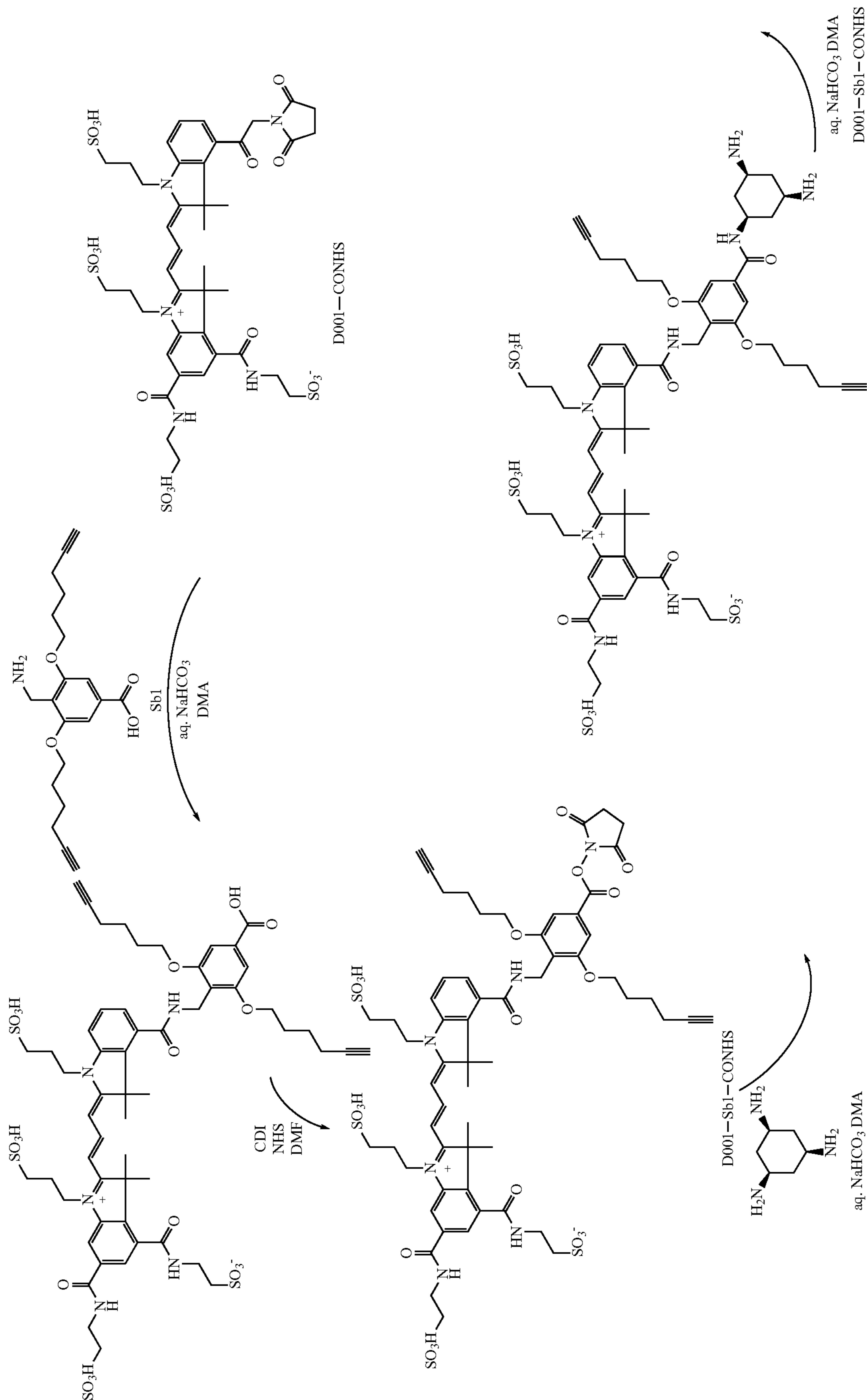
Scheme 2
