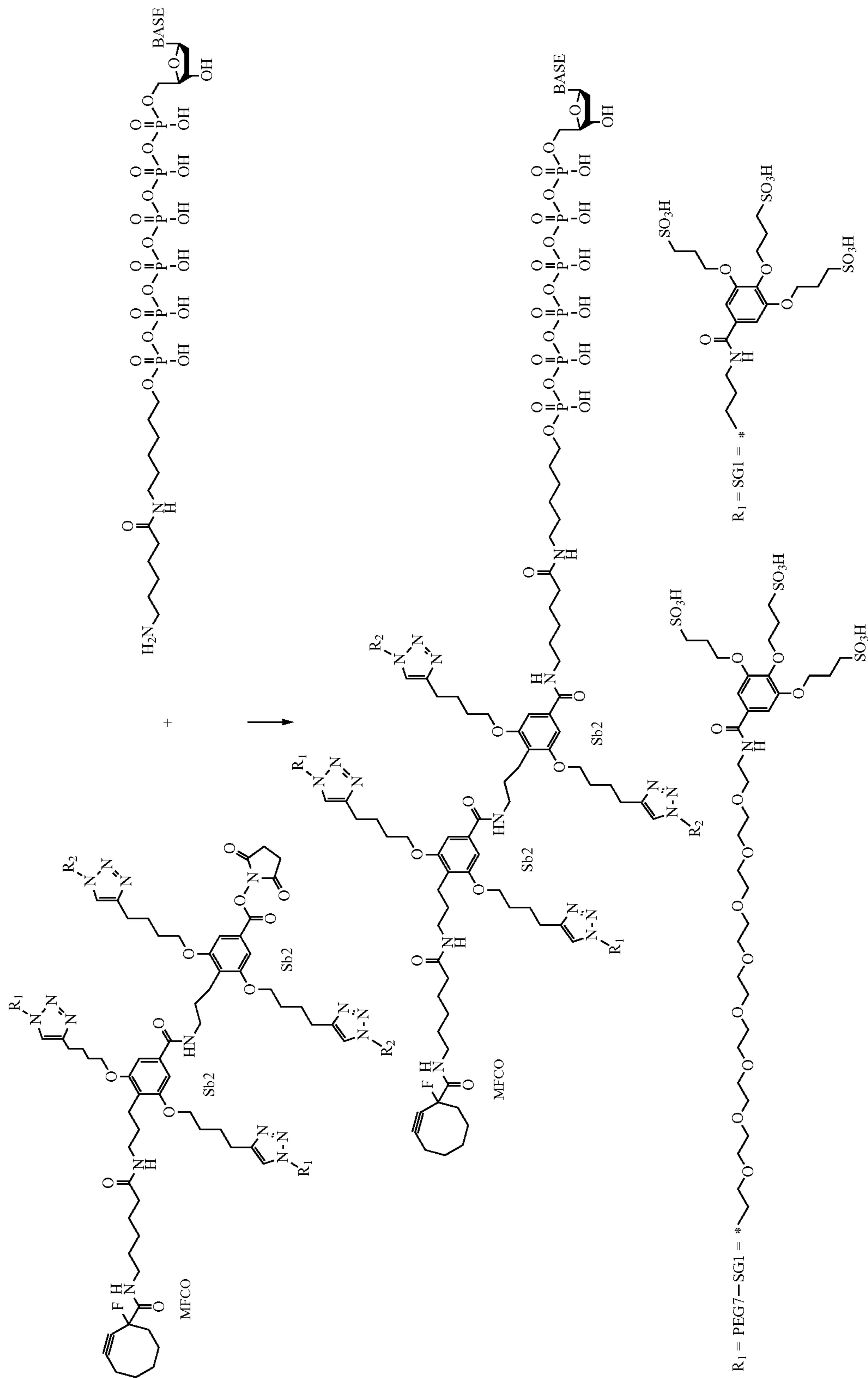
Scheme 15-2
