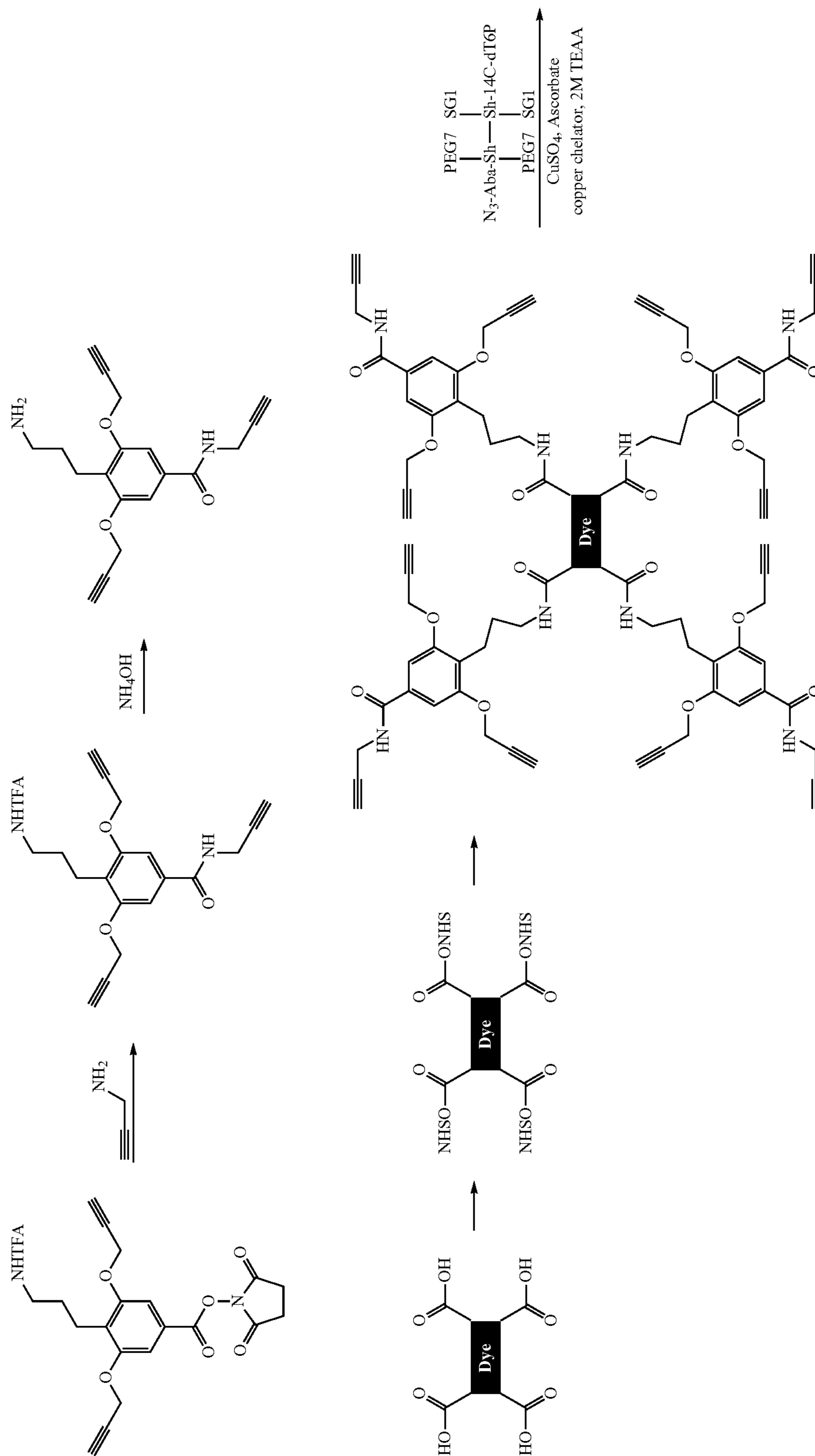
Scheme 20
