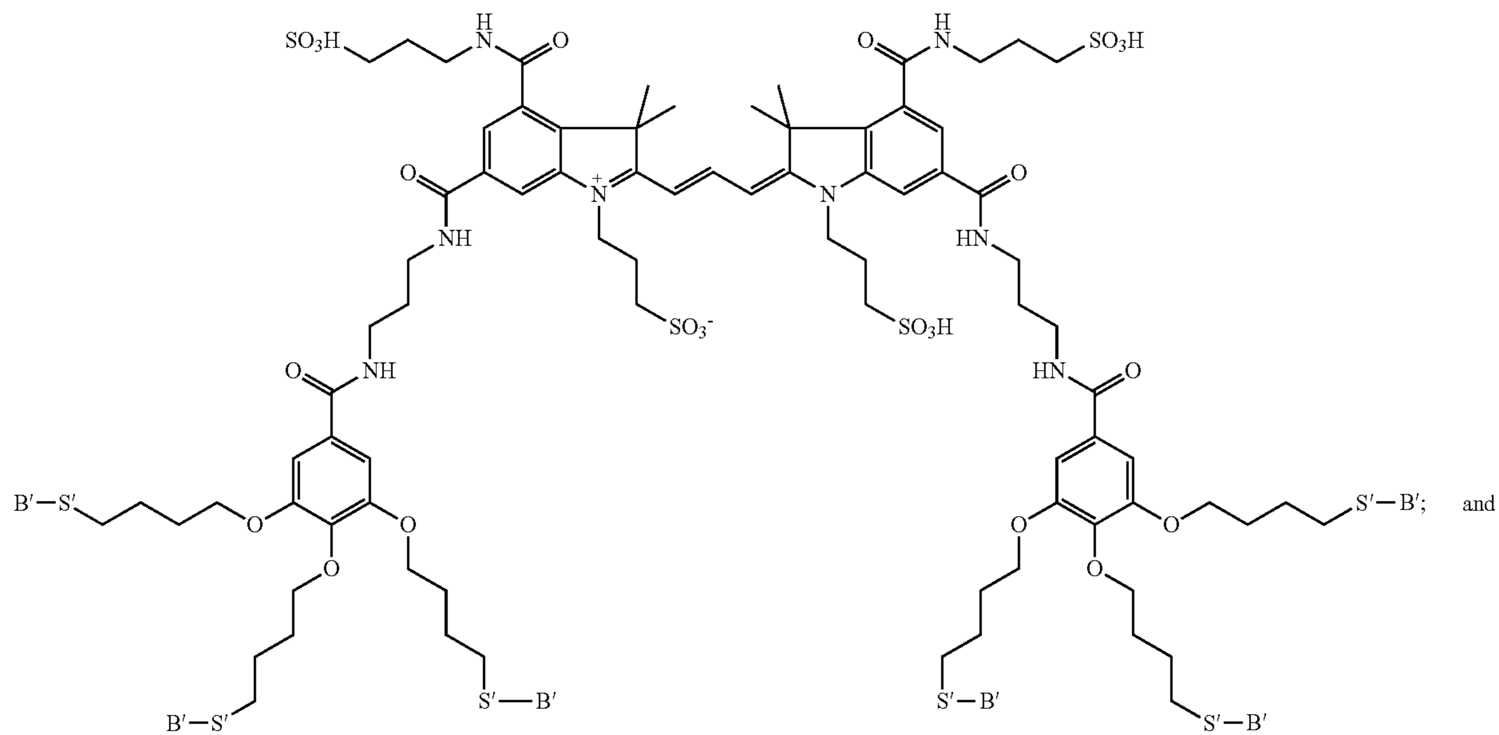
D009(PD-Gal) 2 (Hexavalent)
