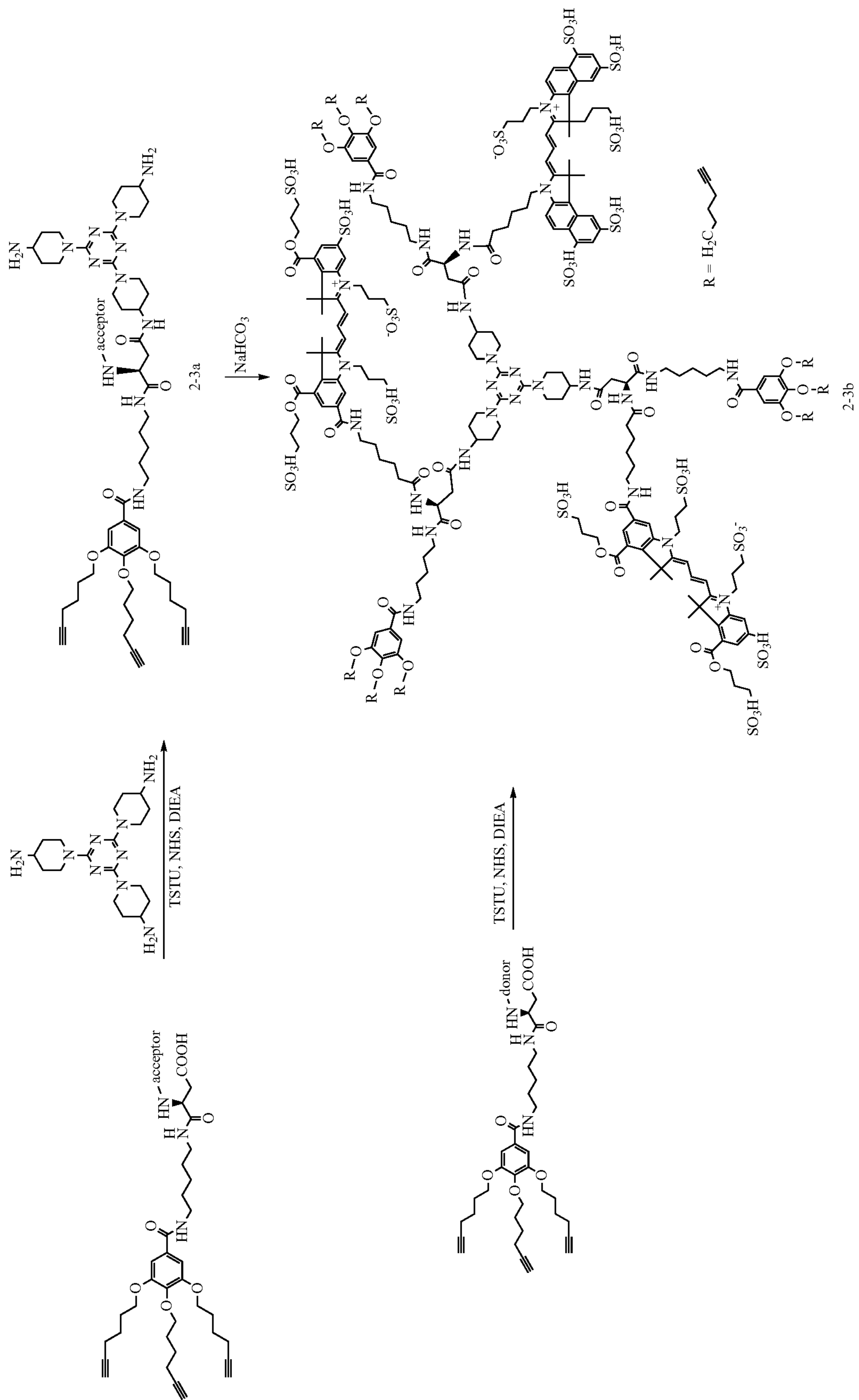
Scheme 23
