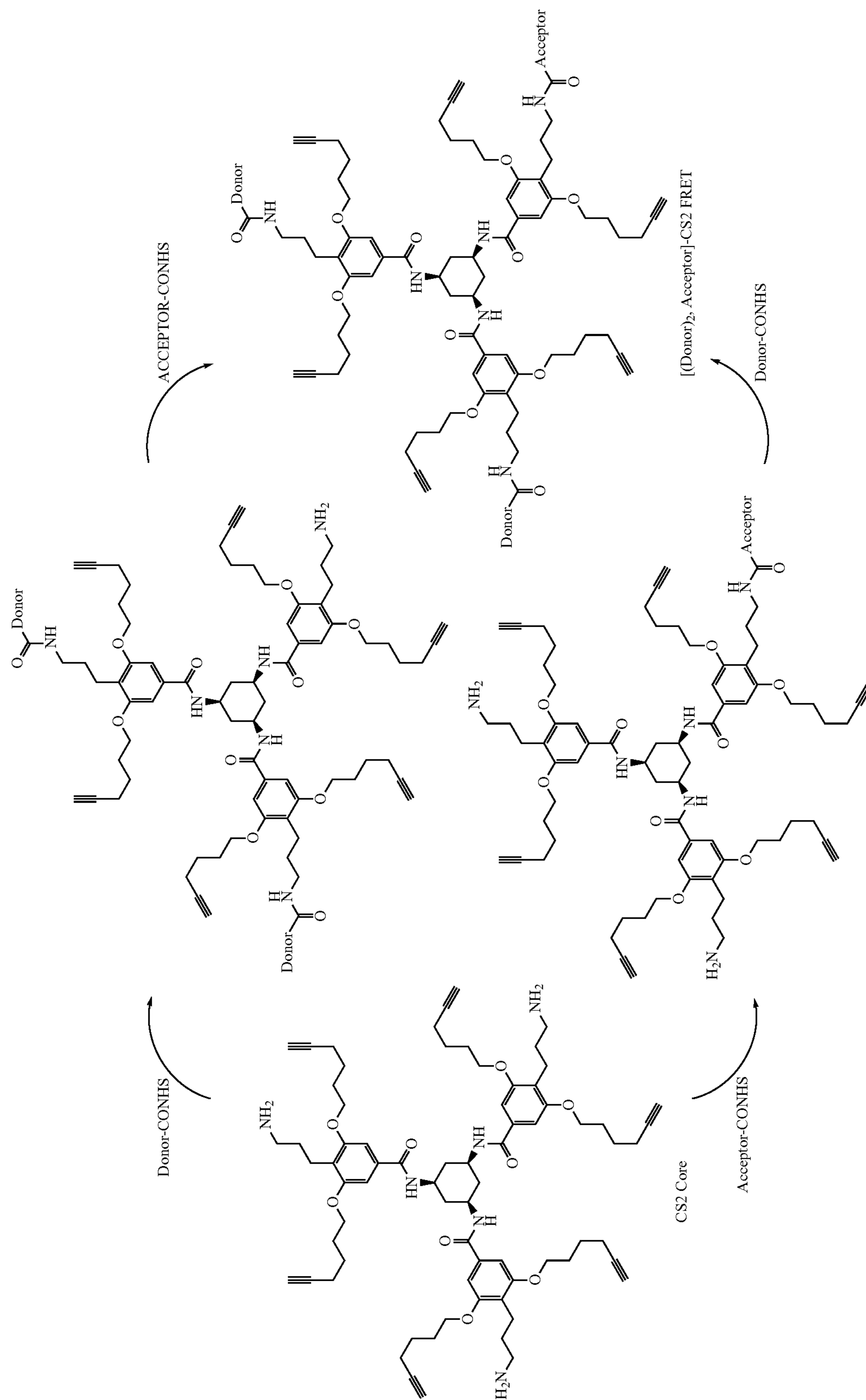
Scheme 4
