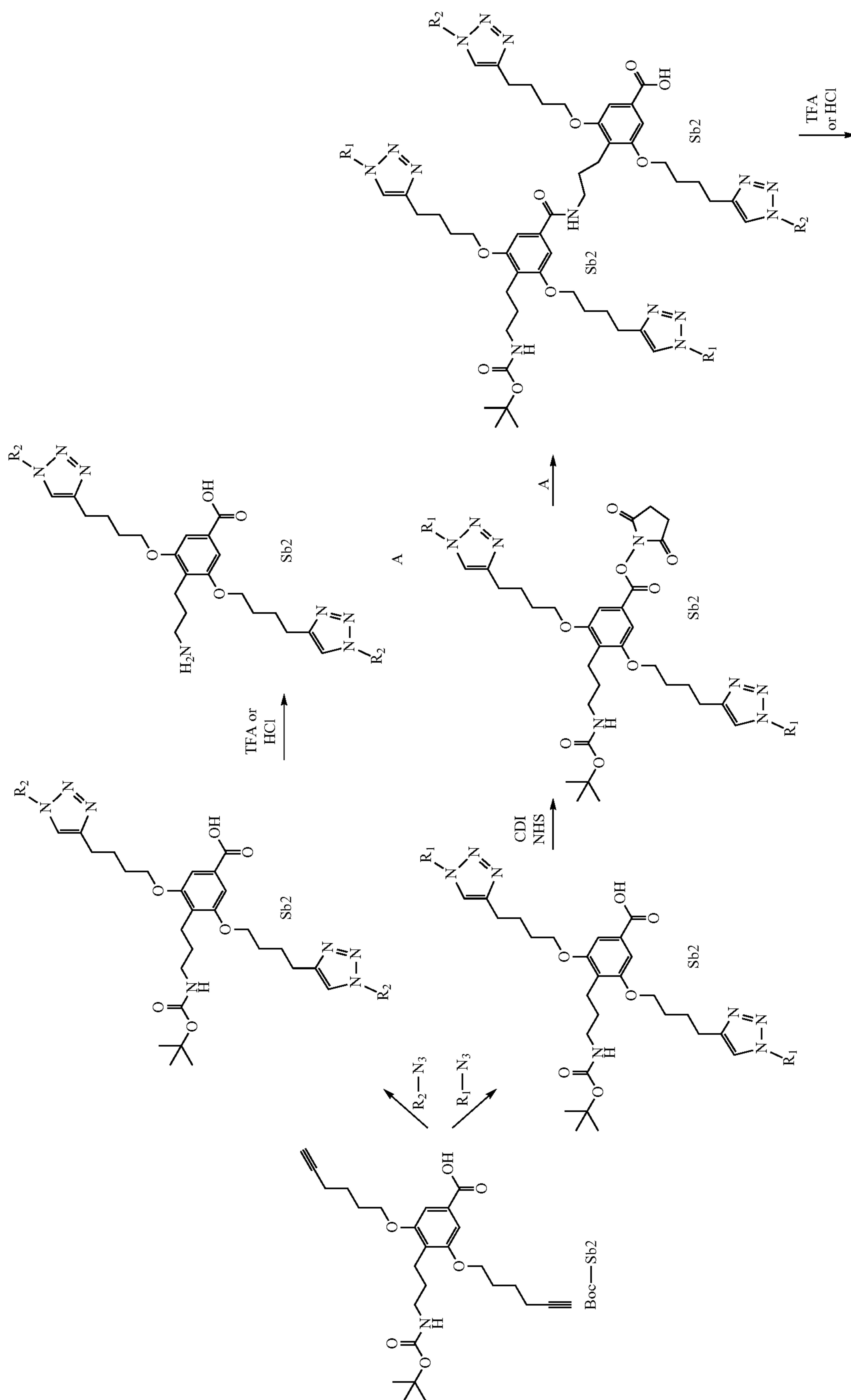
Scheme 15-1
