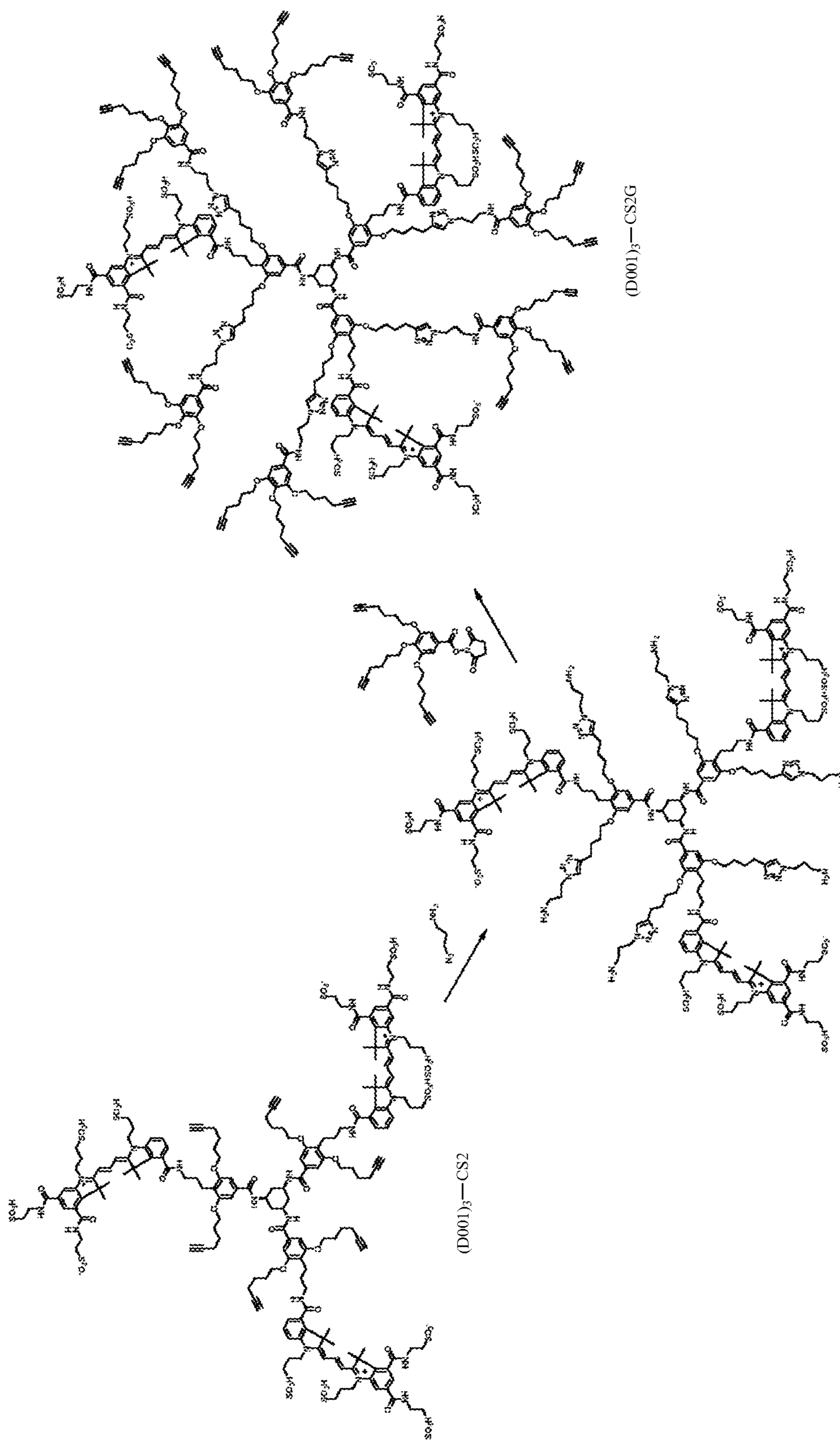
Scheme 5
