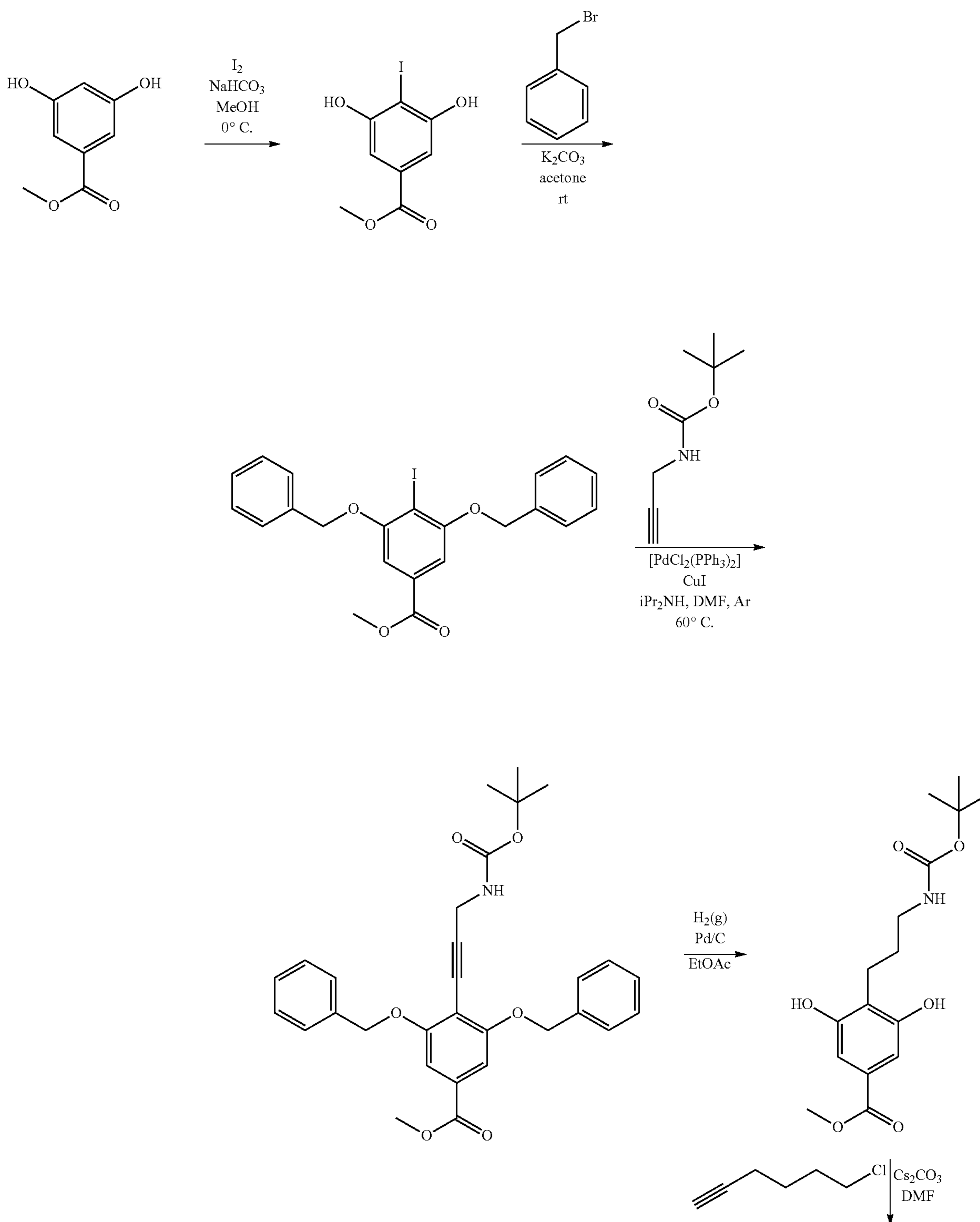
Scheme 16-1
