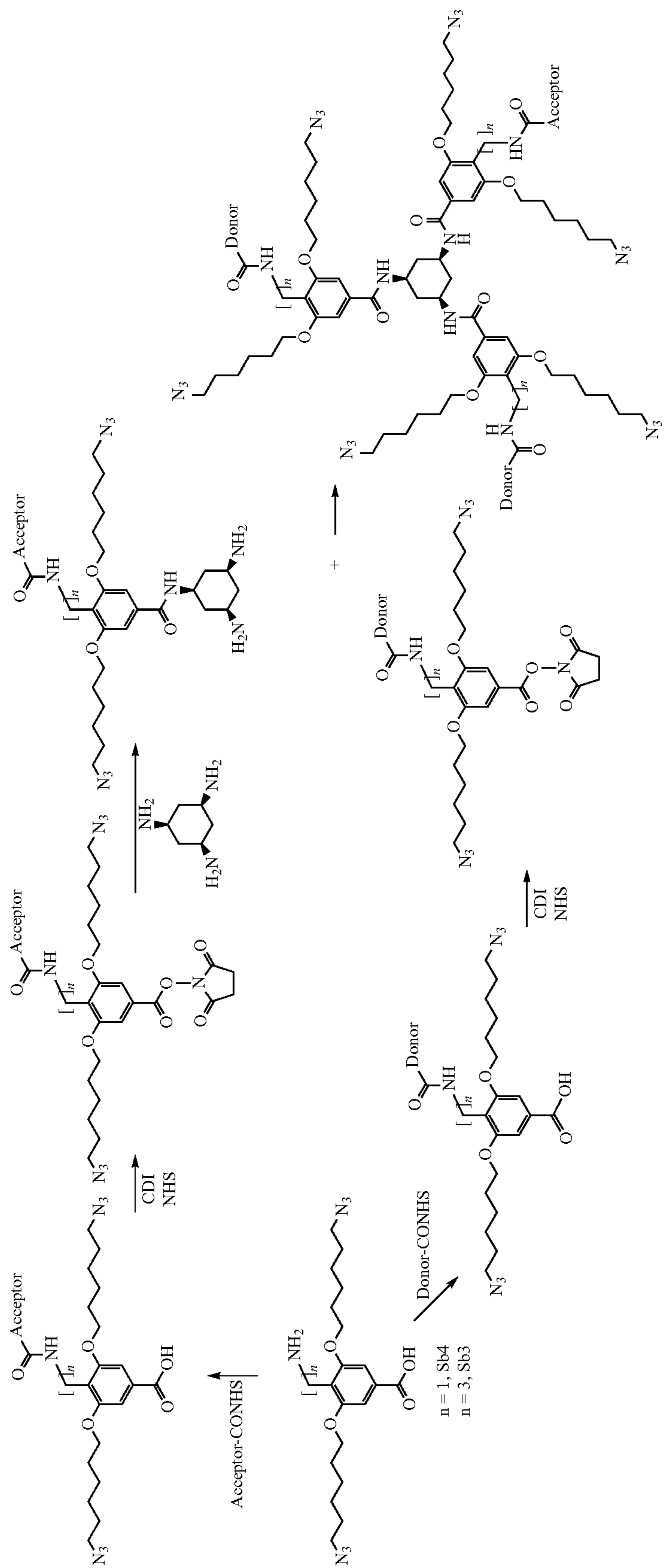
Scheme 11
