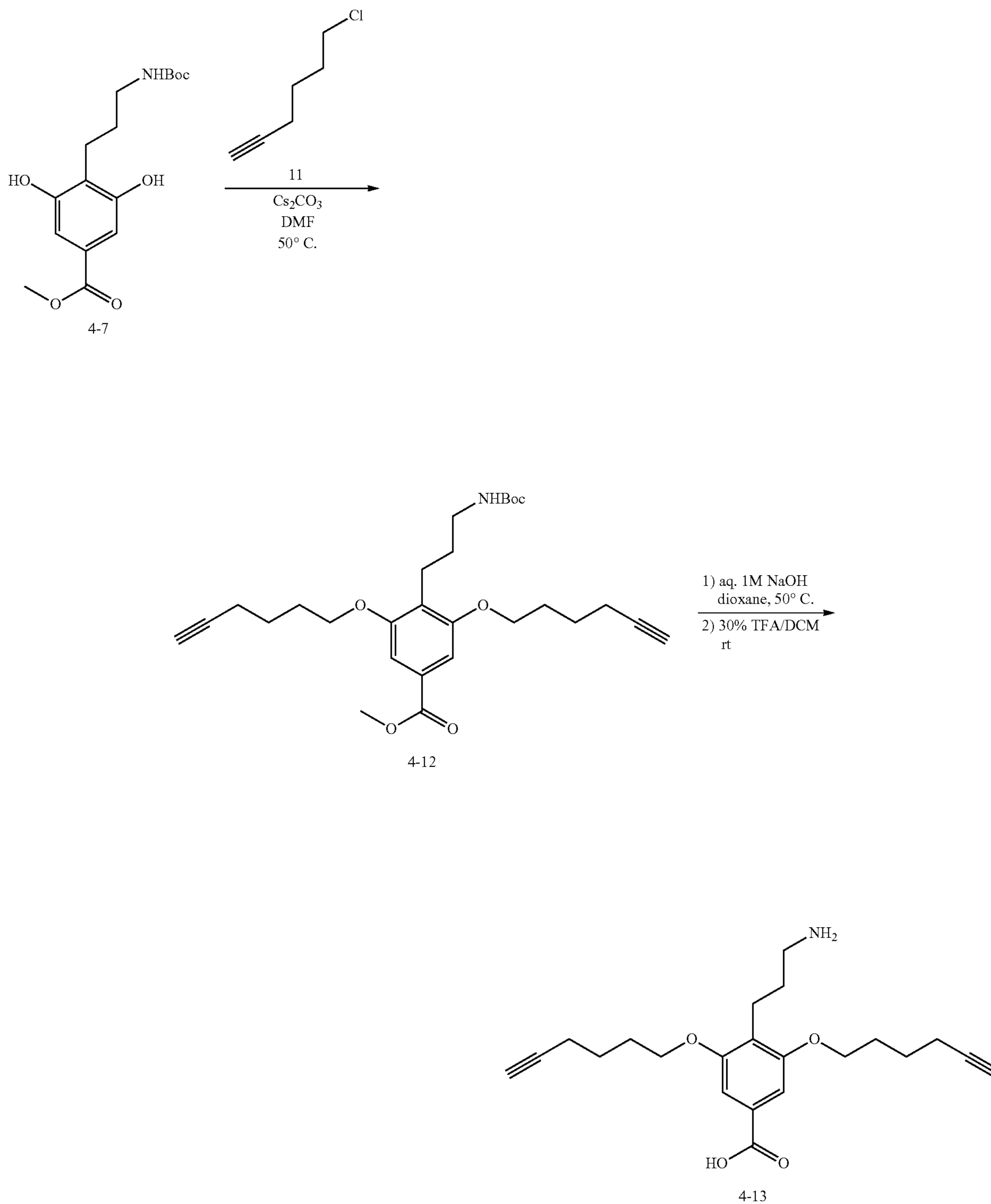
Scheme 28
