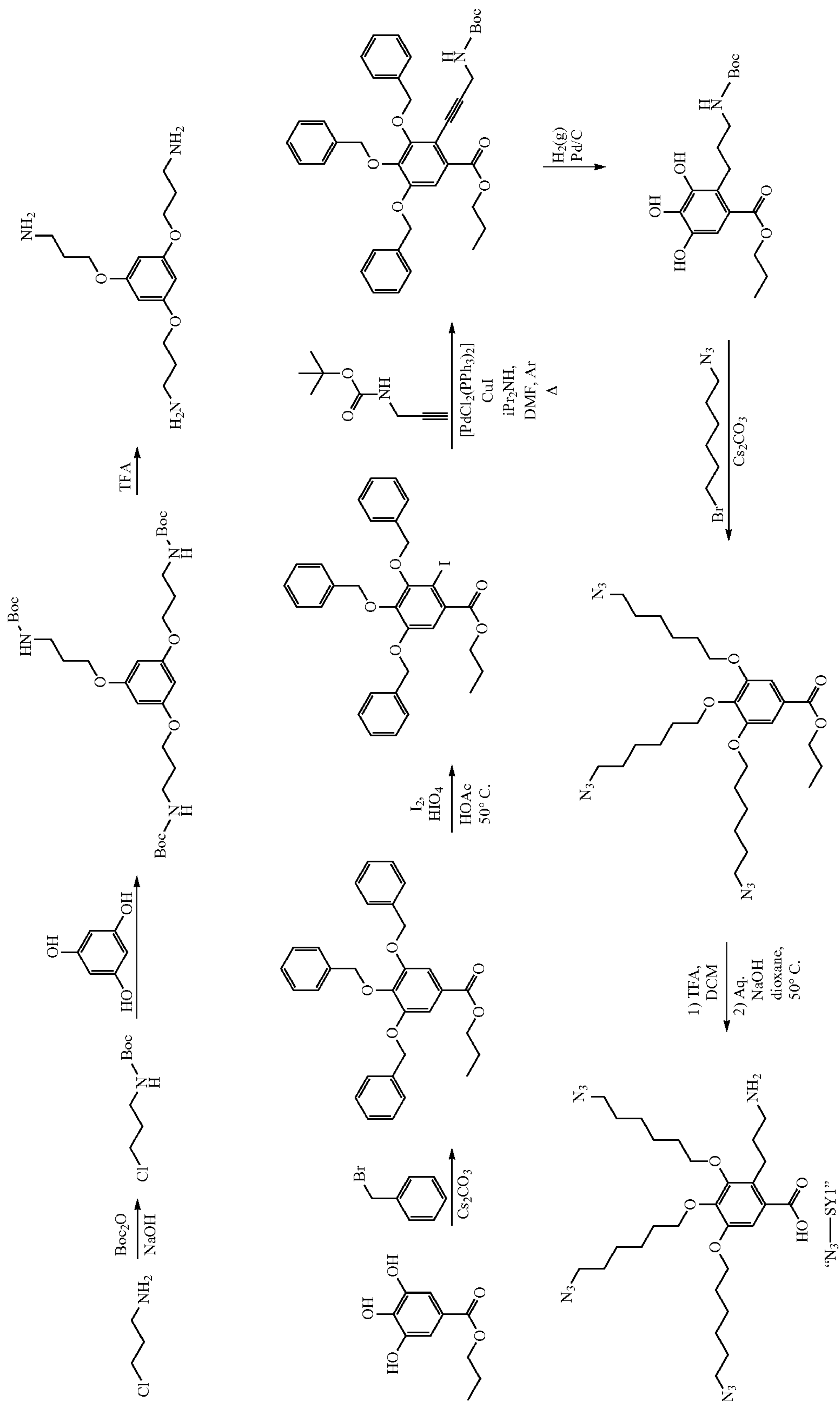
Scheme 14
