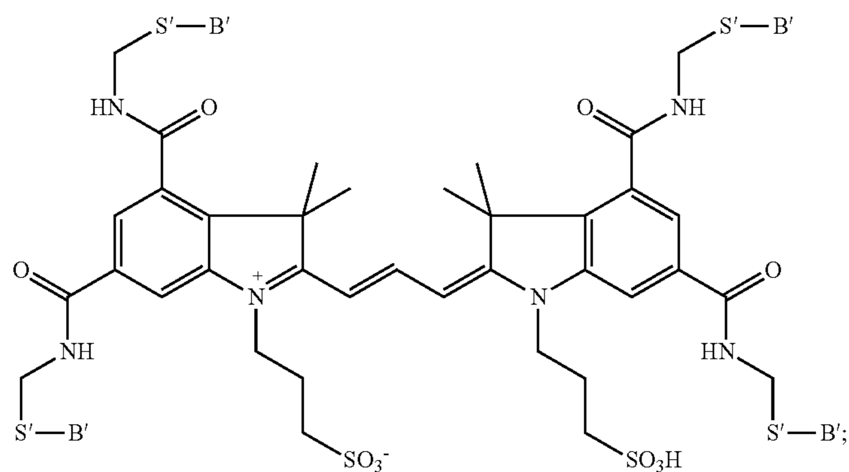
D010 (Tetravalent)
