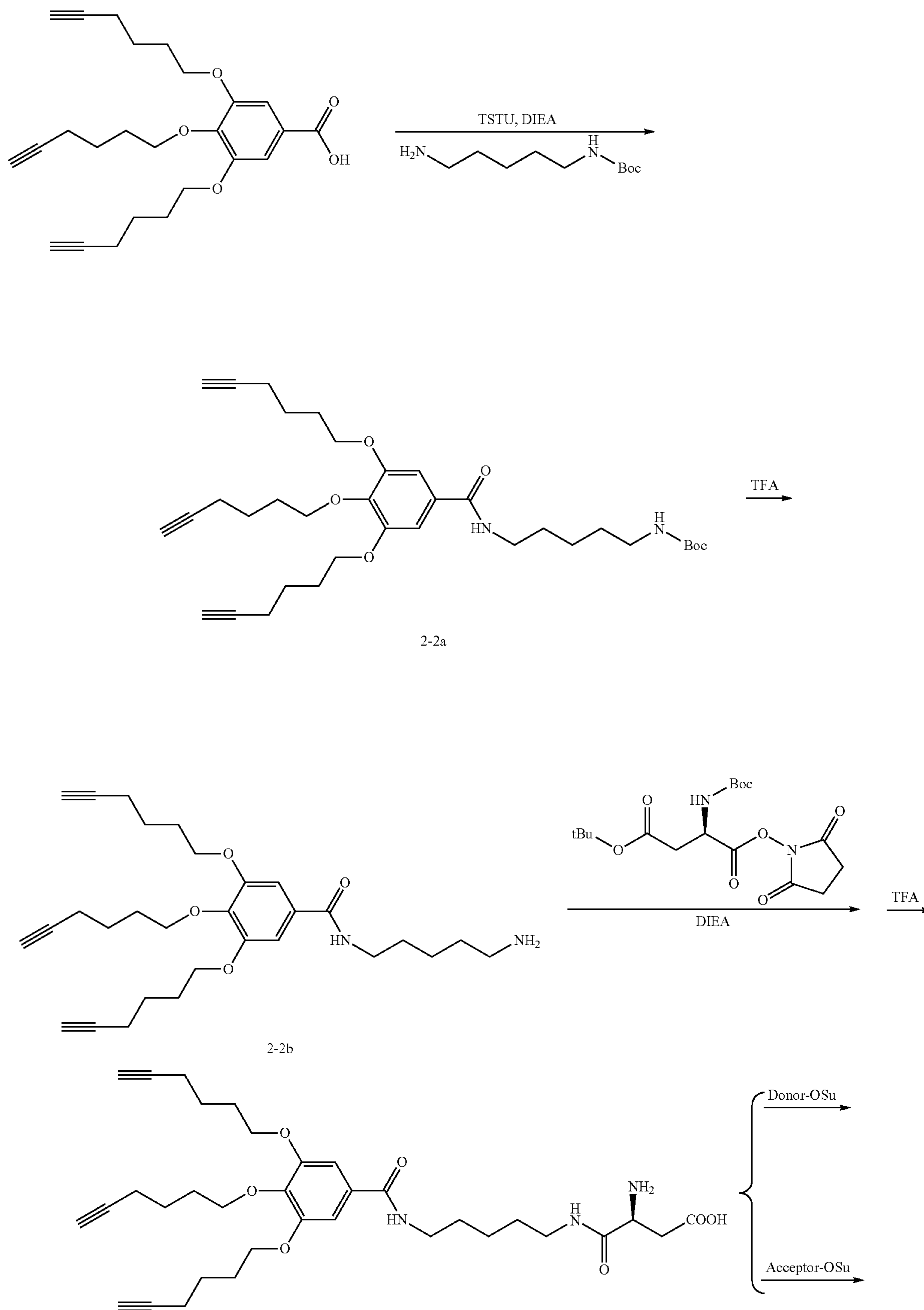
Scheme 22
