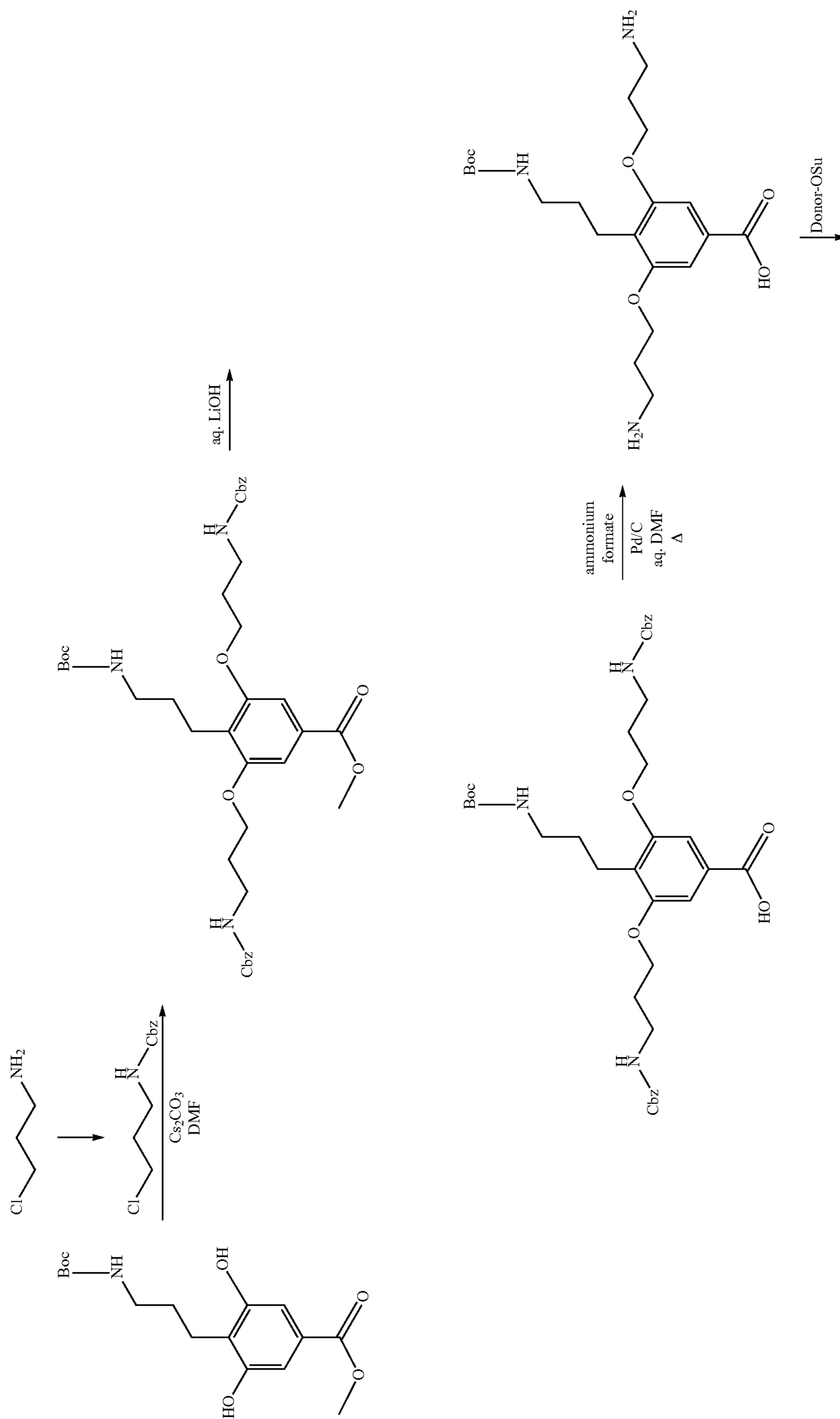
Scheme 10
