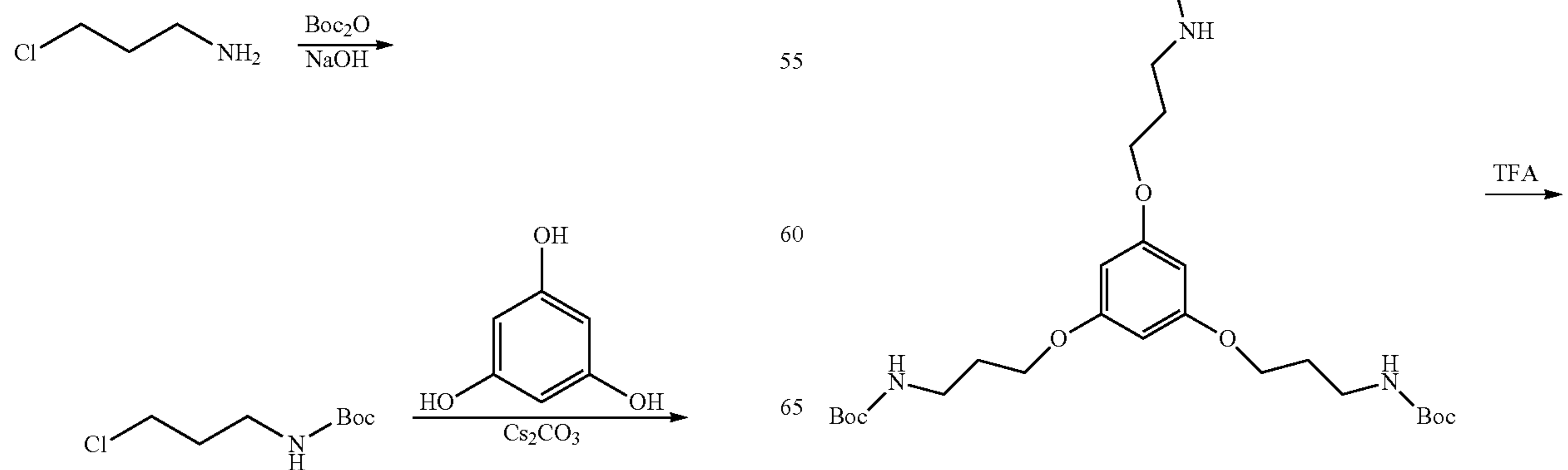
Scheme 6-3
