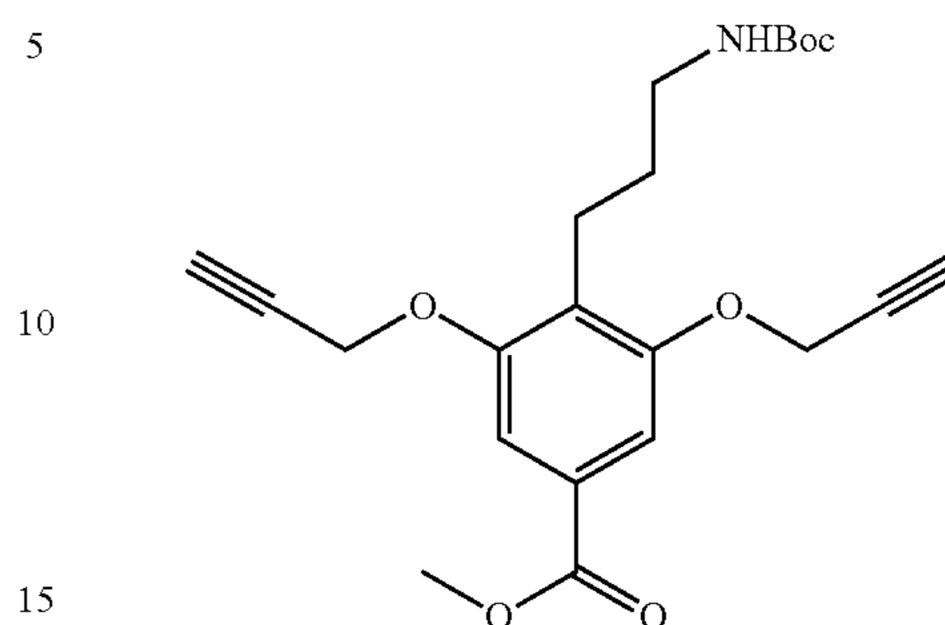
Methyl 4-(3-[[tert-butoxy]carbonyl]amino)propyl)-3,5-bis(prop-2-yn-1-yloxy)benzoate (4-9)
