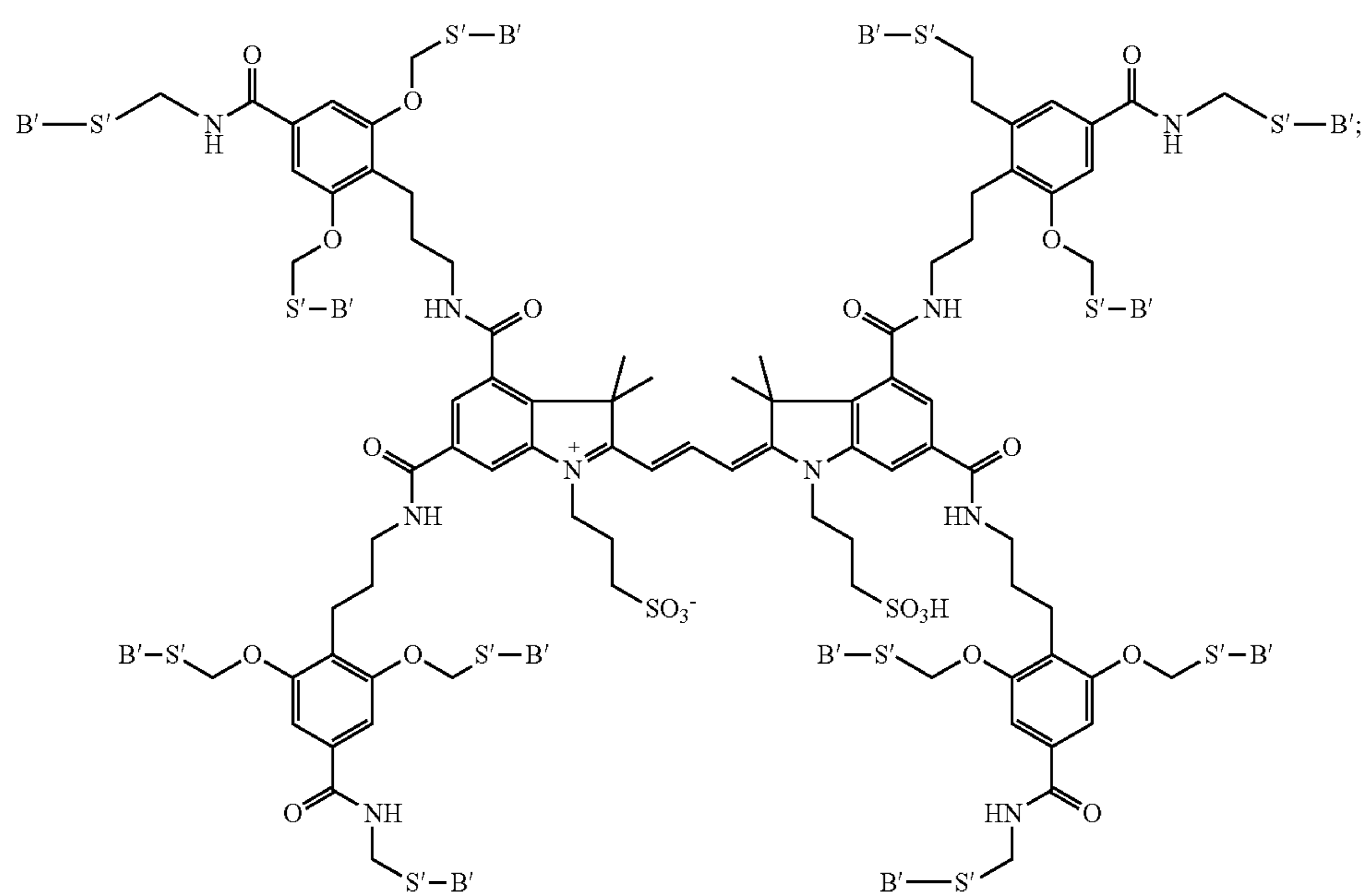
D010(Sh) 4 (Dodecavalent)
