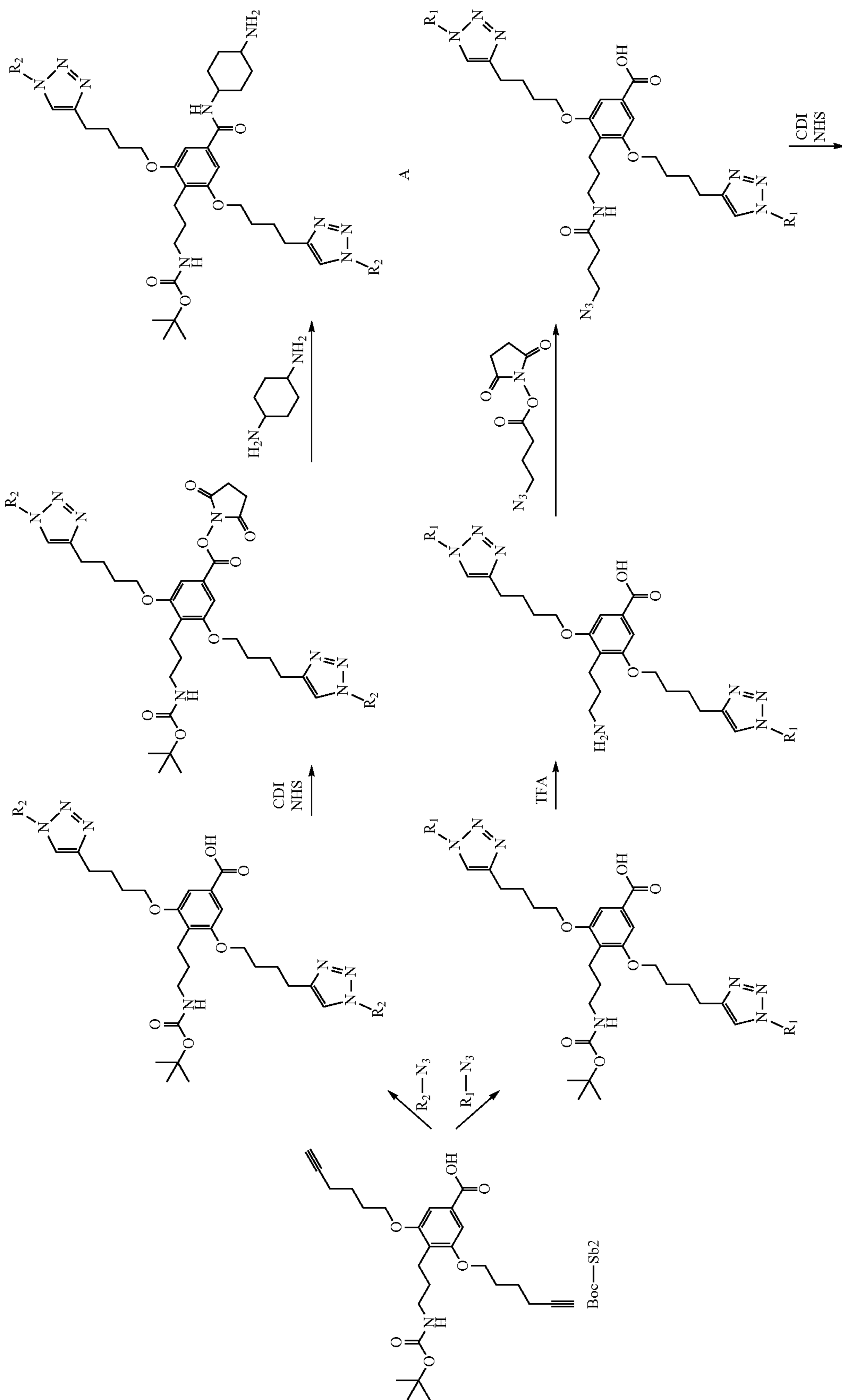
Scheme 7-5
