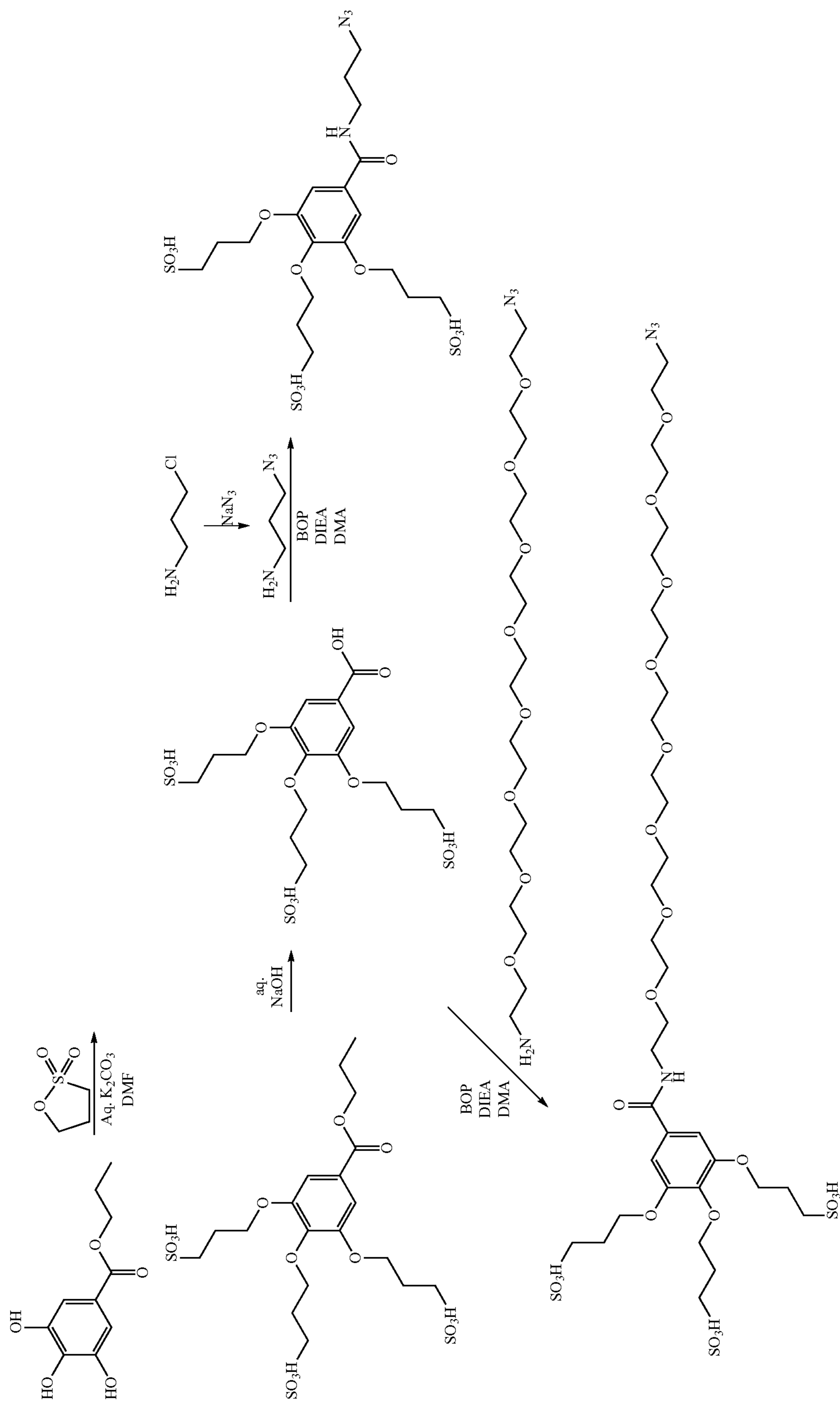
Scheme 16-2
