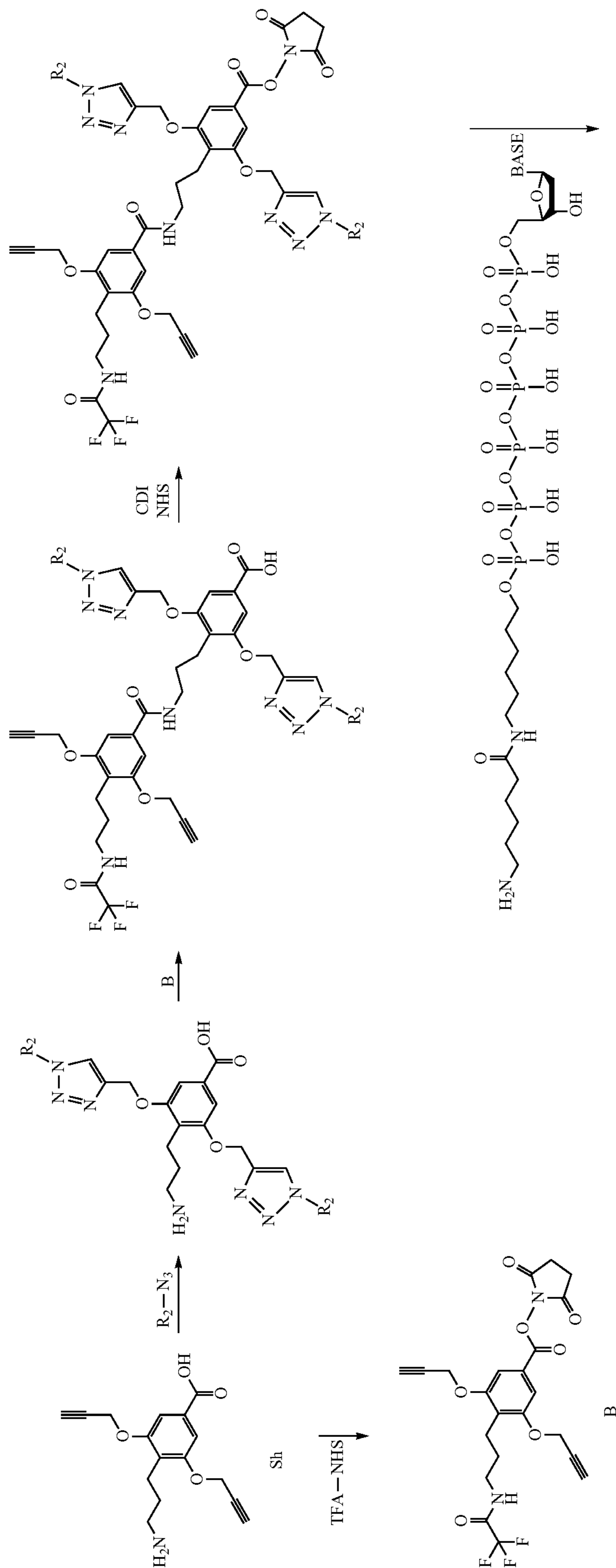
Scheme 7-3
