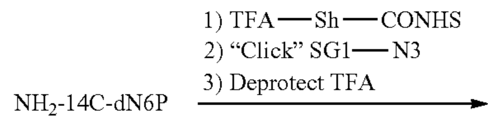
Scheme 7-1
