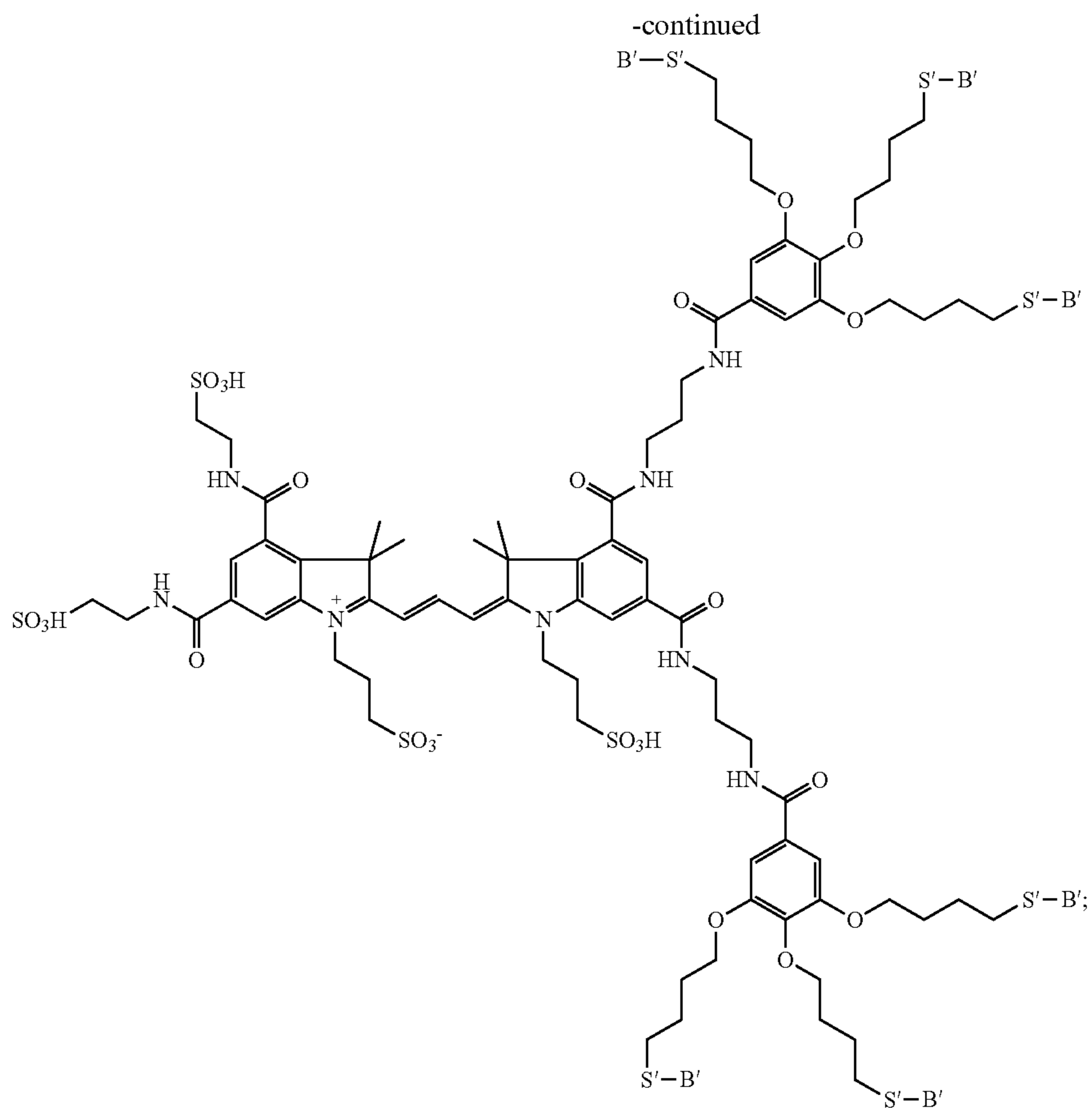
D011(PD-Gal) 2 (Hexavalent)
