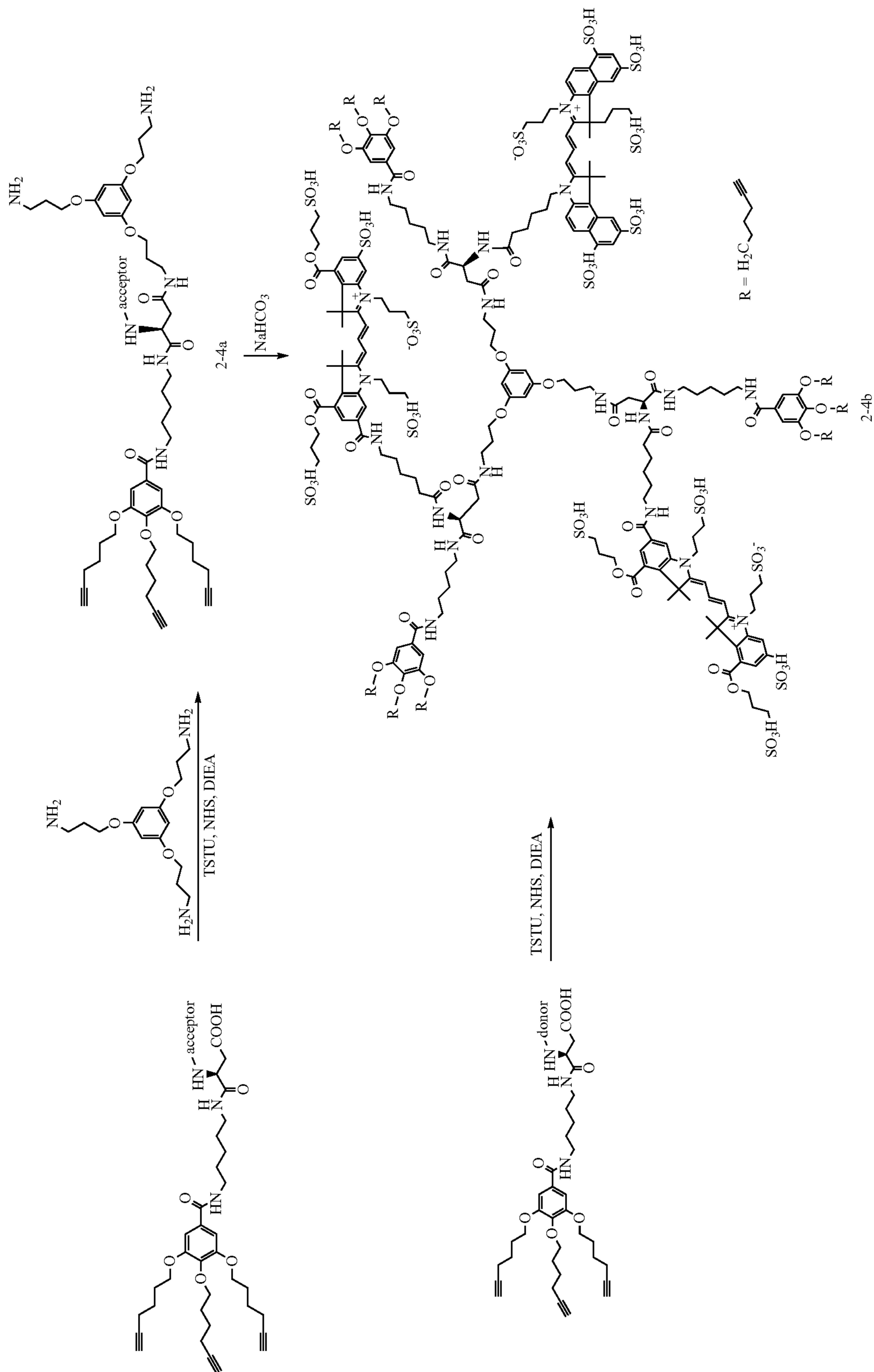
Scheme 24
