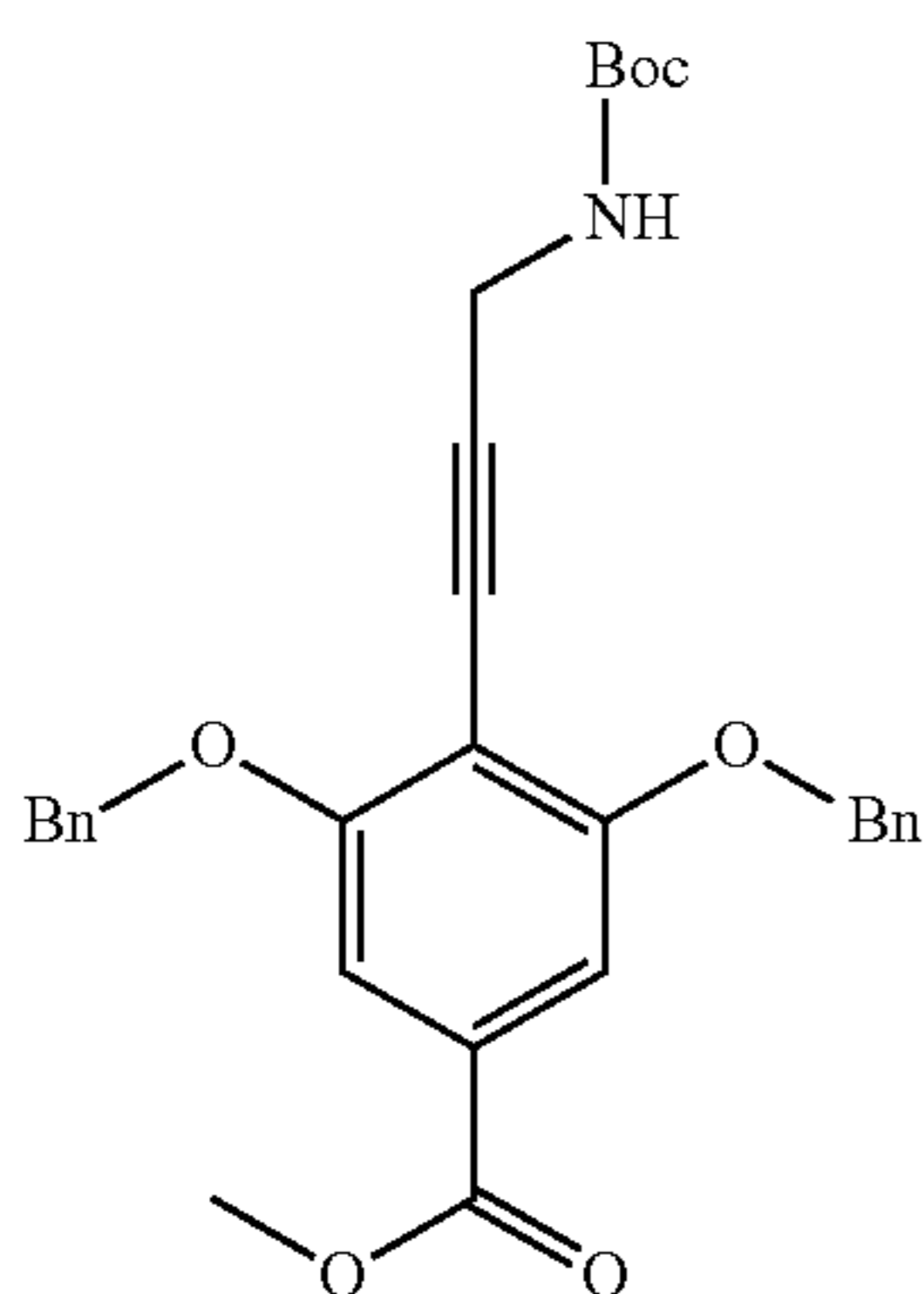
Methyl 3,5-bis(benzyloxy)-4-(3-[[tert-butoxy]carbonyl]amino)prop-1-yn-1-yl)benzoate (4-6)
