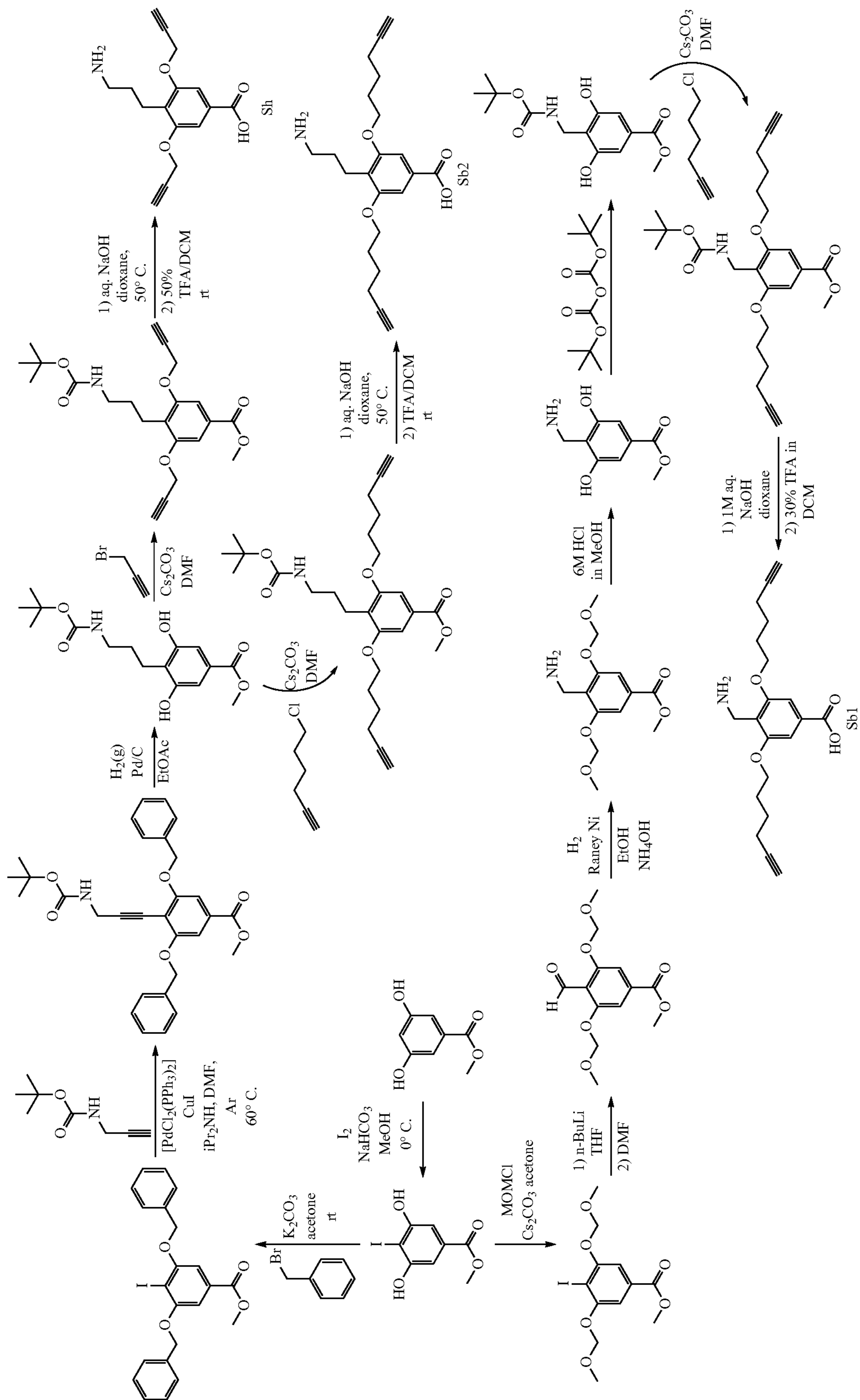
Scheme 1
