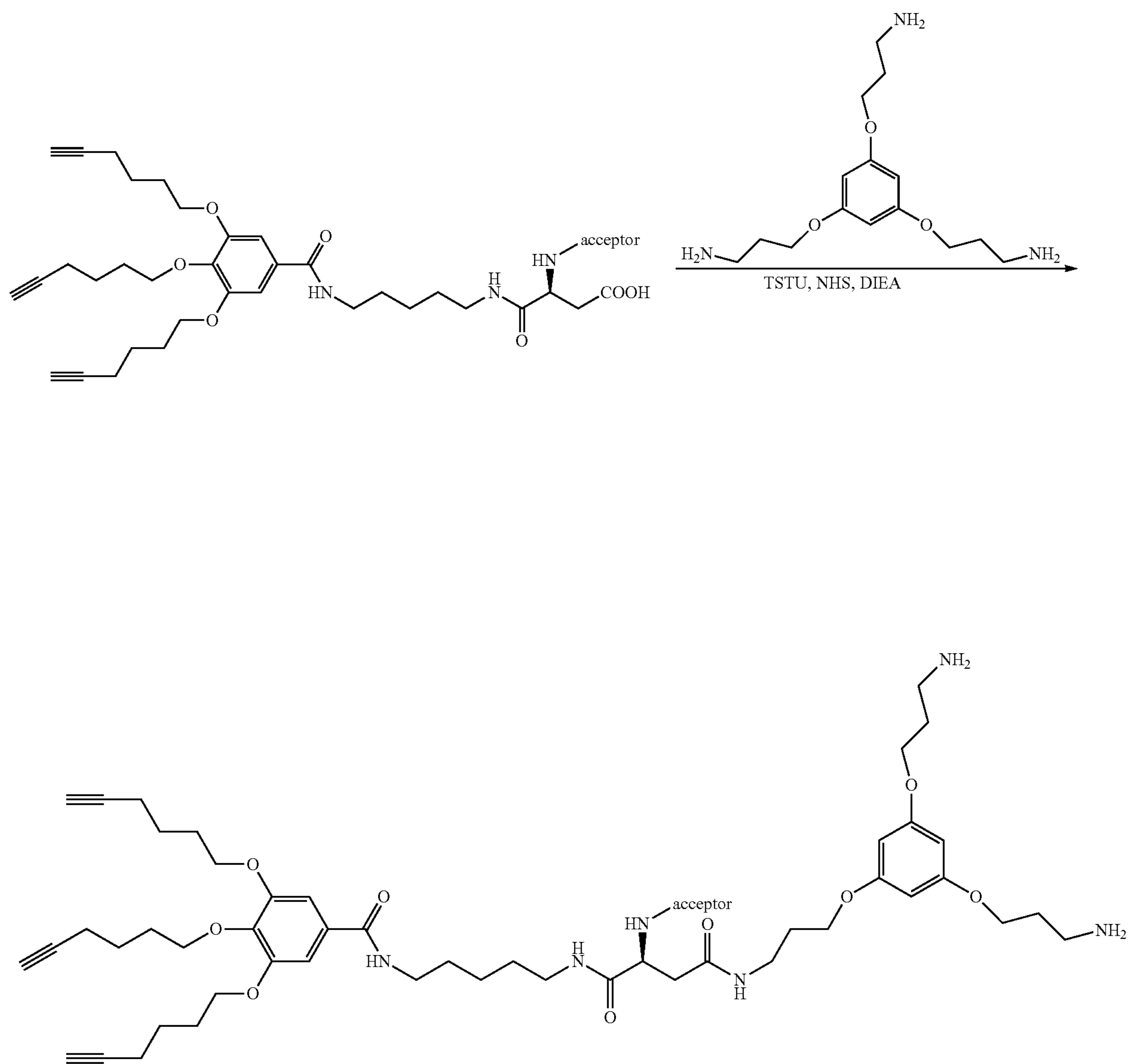
Scheme 6-4;
