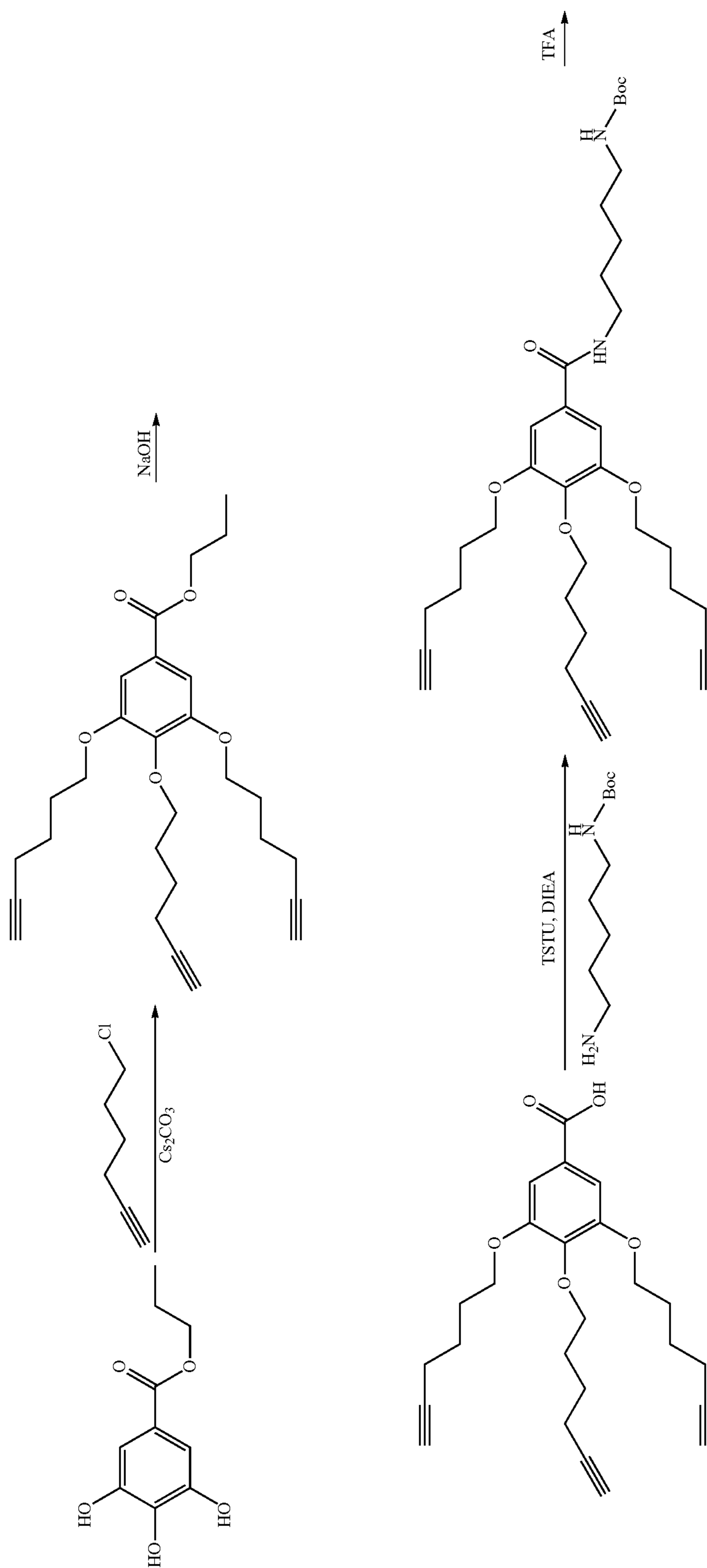
Scheme 6-1
