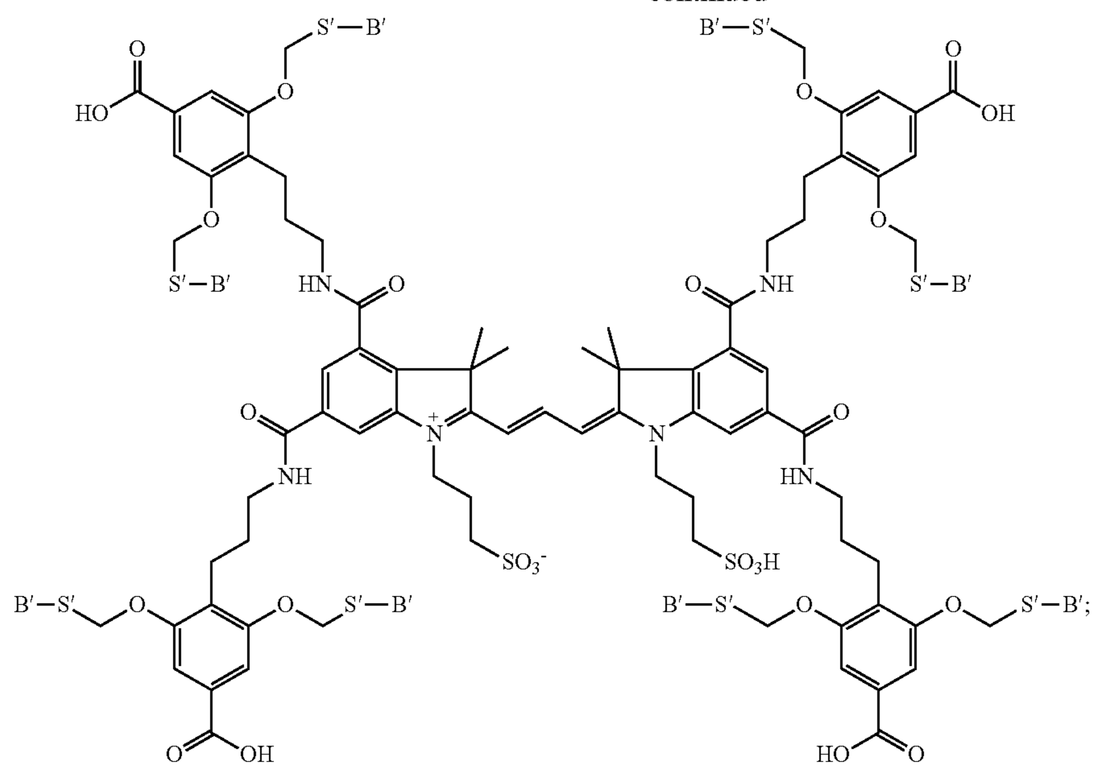
D010(Sh) 4 (Octavalent)
