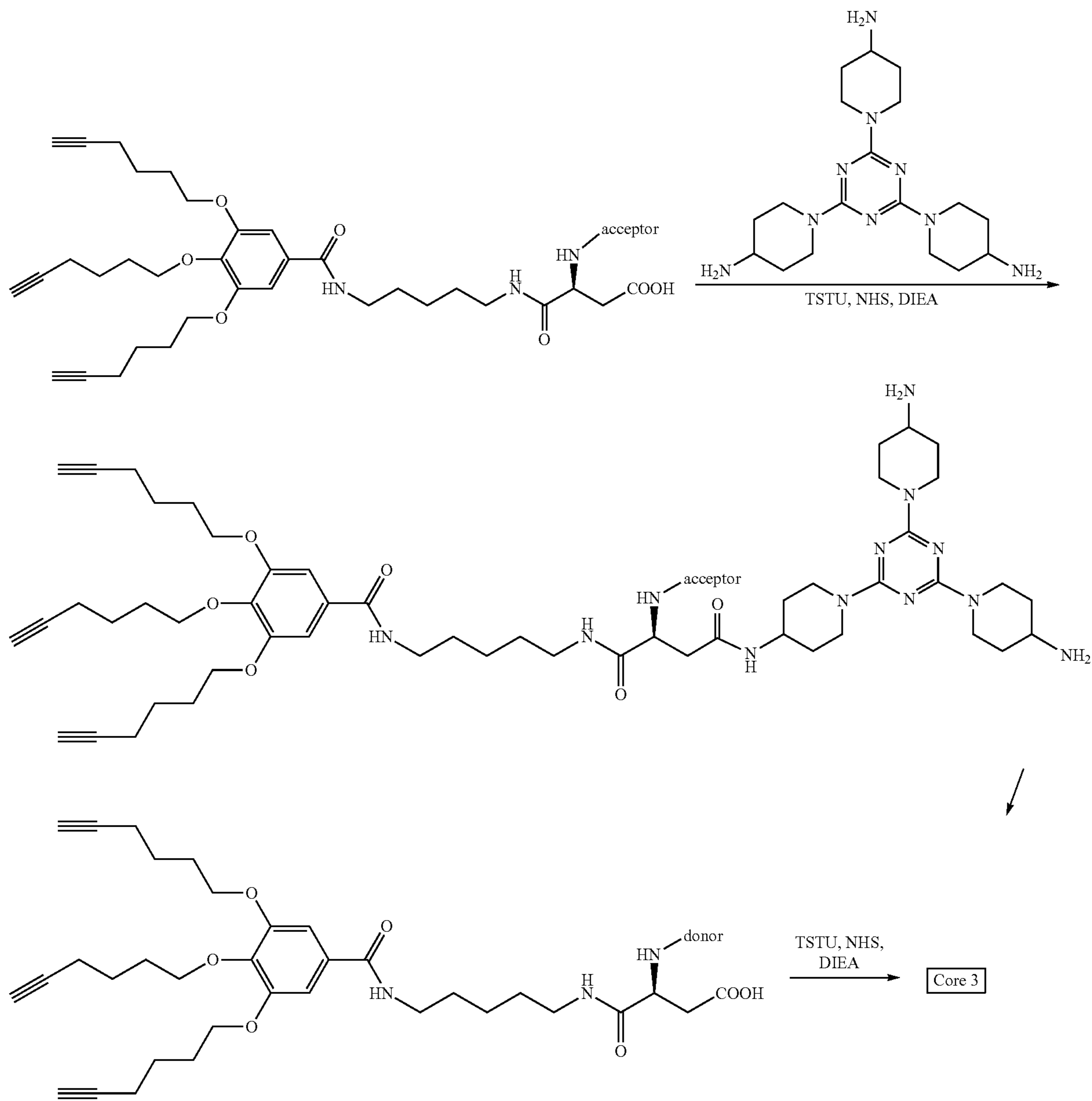
Scheme 6-2
