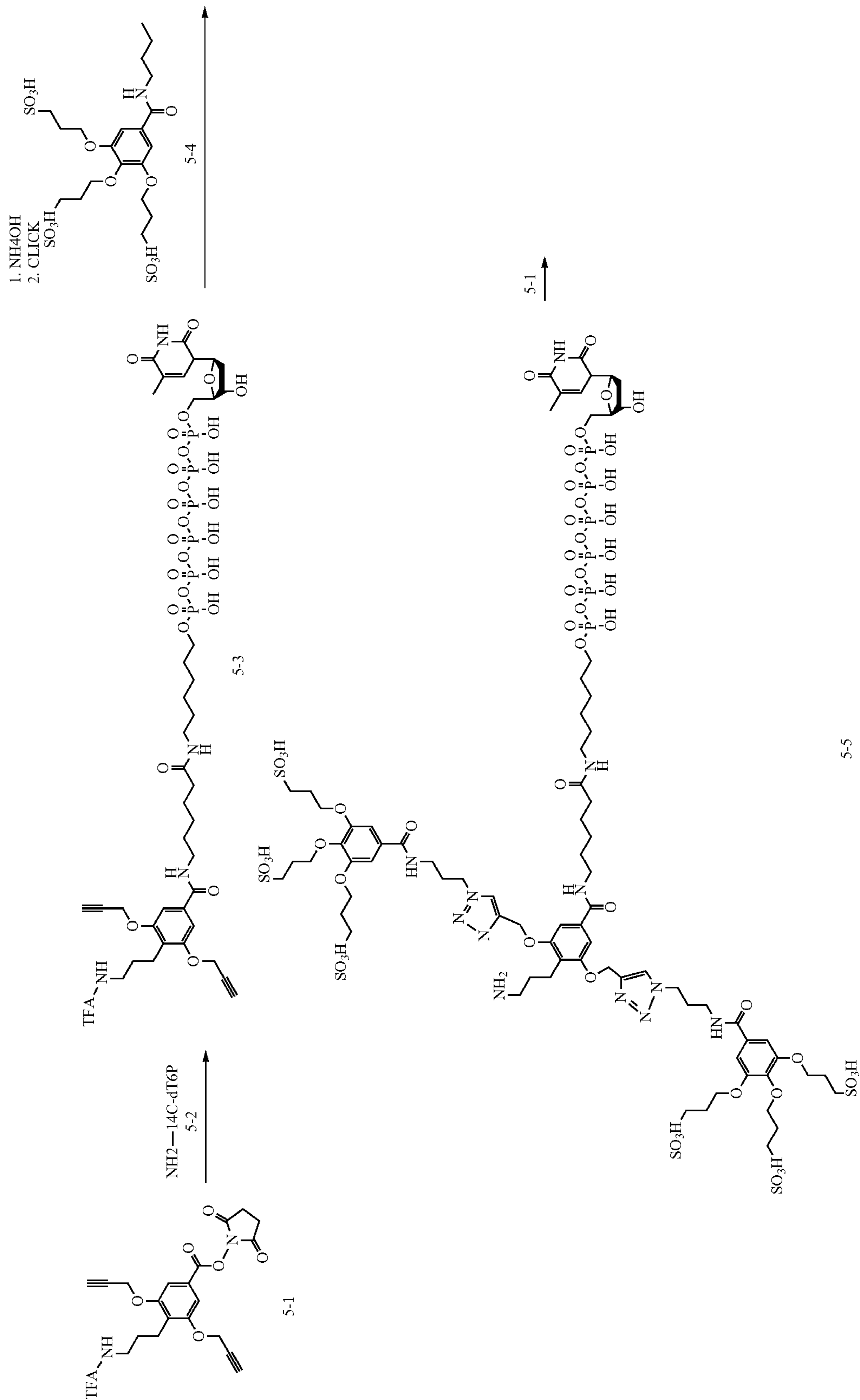
Scheme 29
