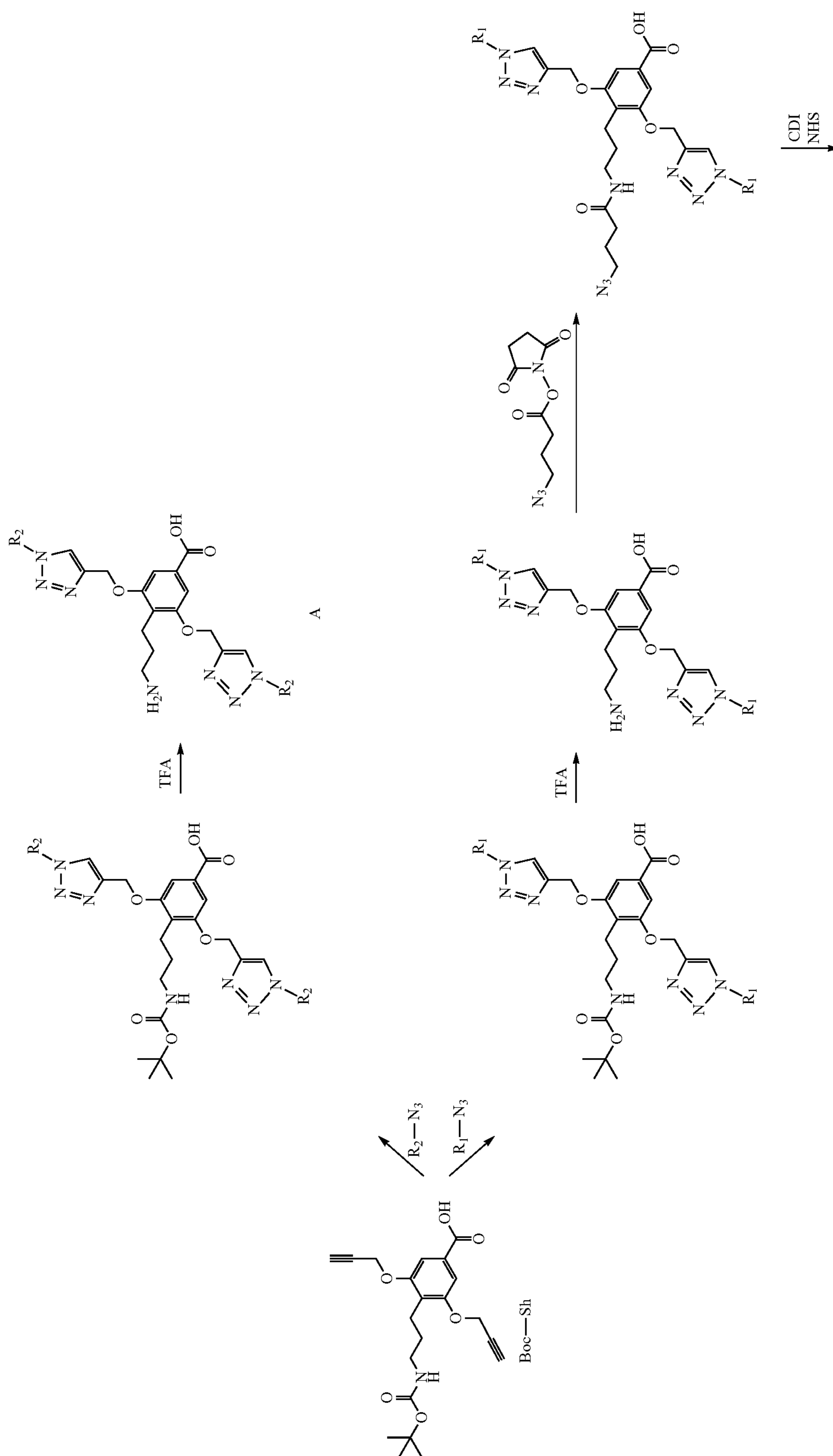
Scheme 7-4
