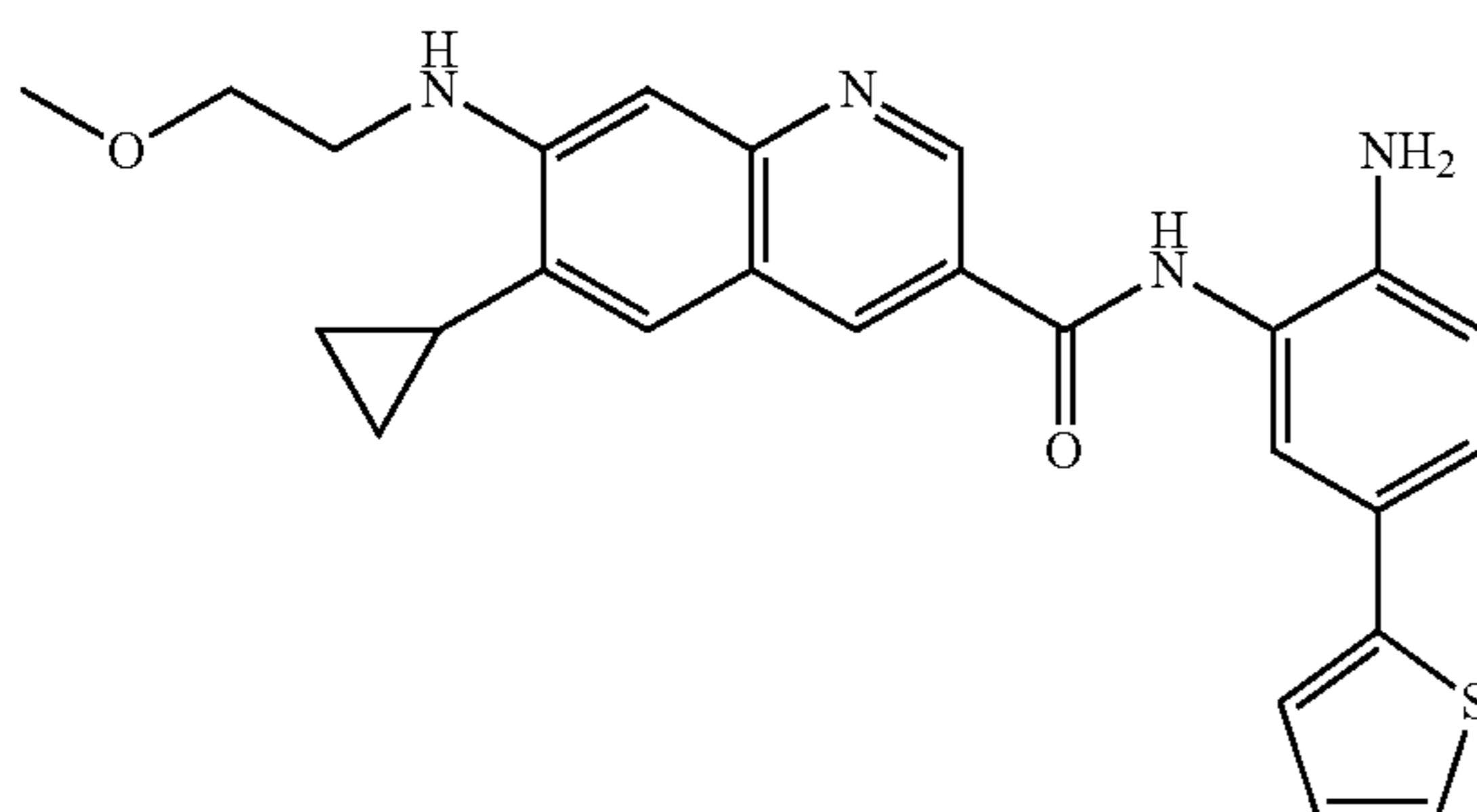
N-(2-amino-5-(thiophen-2-yl)phenyl)-6-cyclopropyl-7-((2-methoxyethyl)amino)quinoline-3-carboxamide
