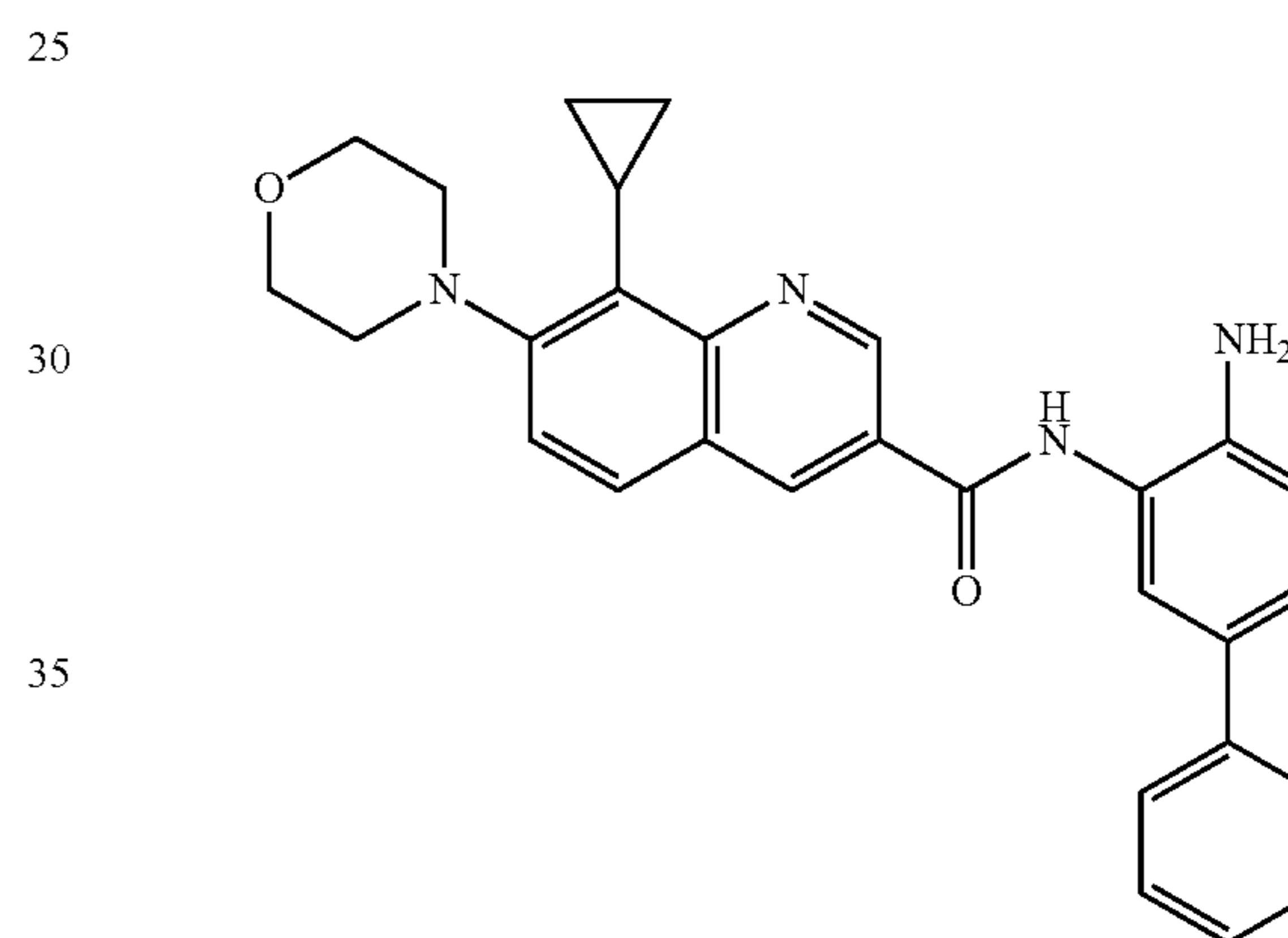
N-(4-amino-[1,1'-biphenyl]-3-yl)-8-cyclopropyl-7-morpholinoquinoline-3-carboxamide
