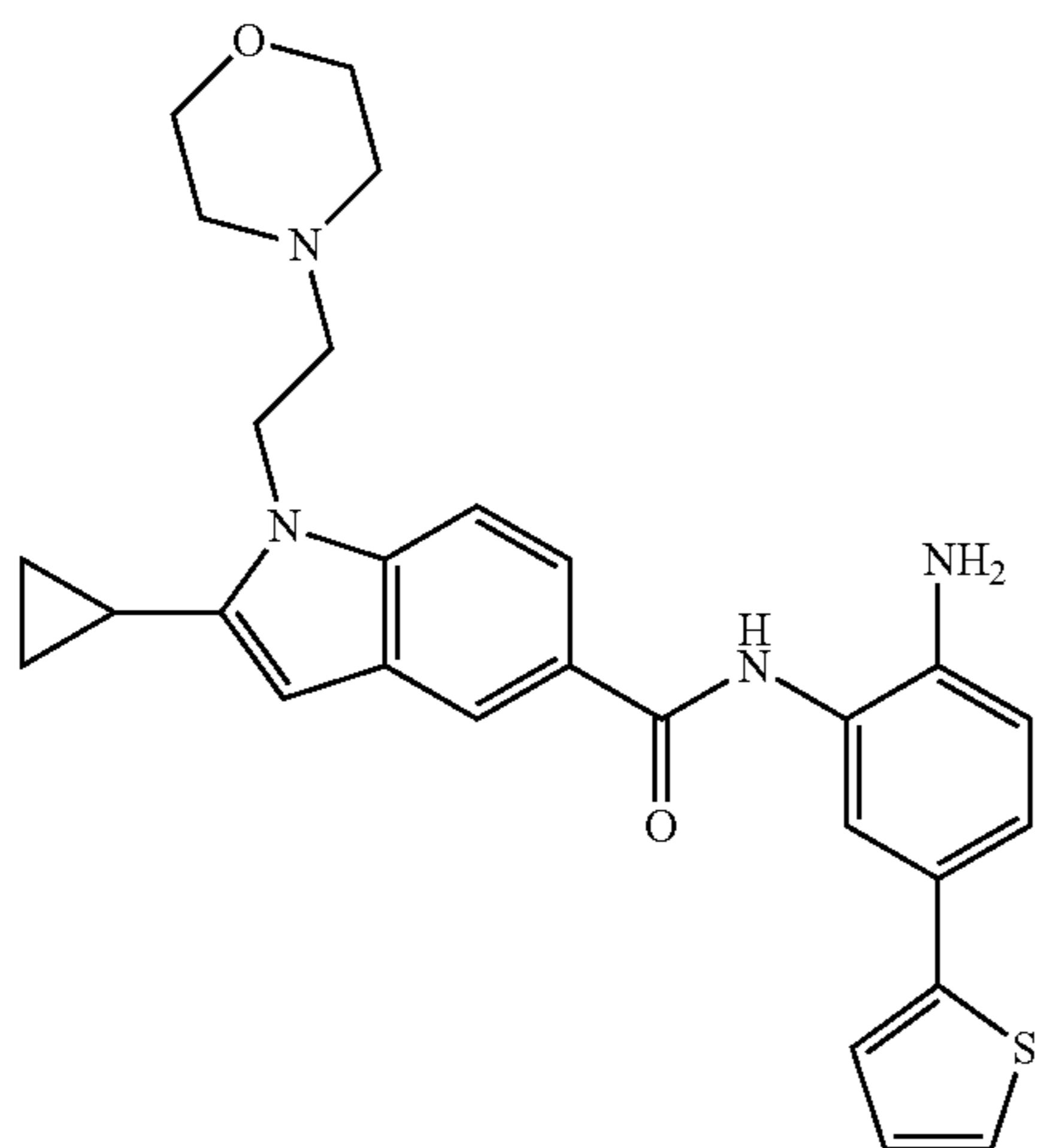
N-(2-amino-5-(thiophen-2-yl)phenyl)-2-cyclopropyl-1-(2-morpholinoethyl)-1H-indole-5-carboxamide
