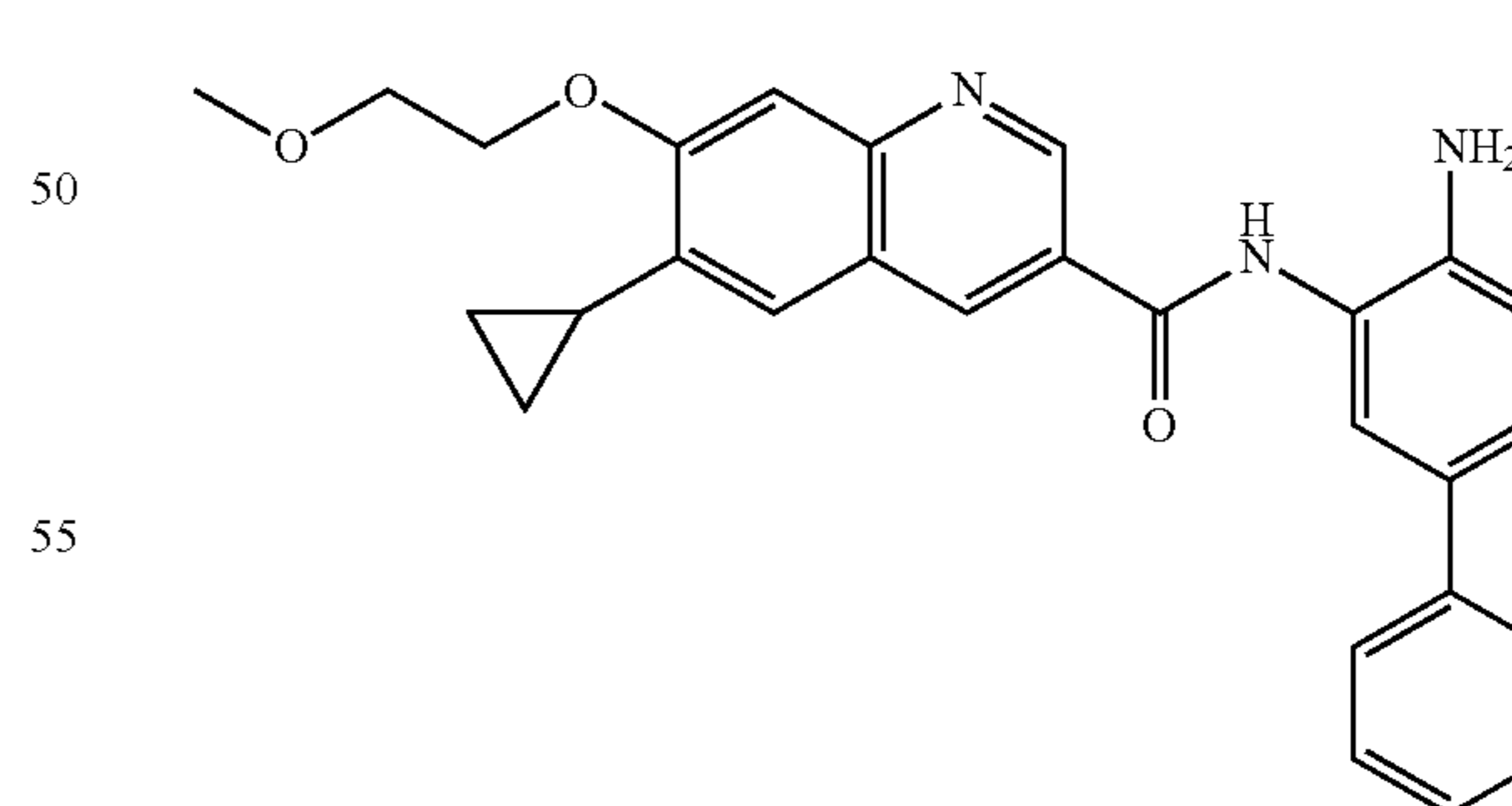
N-(4-amino-[1,1'-biphenyl]-3-yl)-6-cyclopropyl-7-(2-methoxyethoxy)quinoline-3-carboxamide
