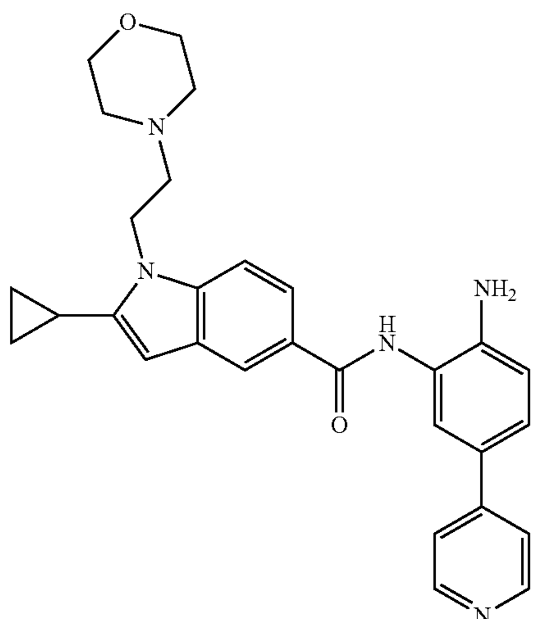
N-(2-amino-5-(pyridin-4-yl)phenyl)-2-cyclopropyl-1-(2-morpholinoethyl)-1H-indole-5-carboxamide, Compound 004
