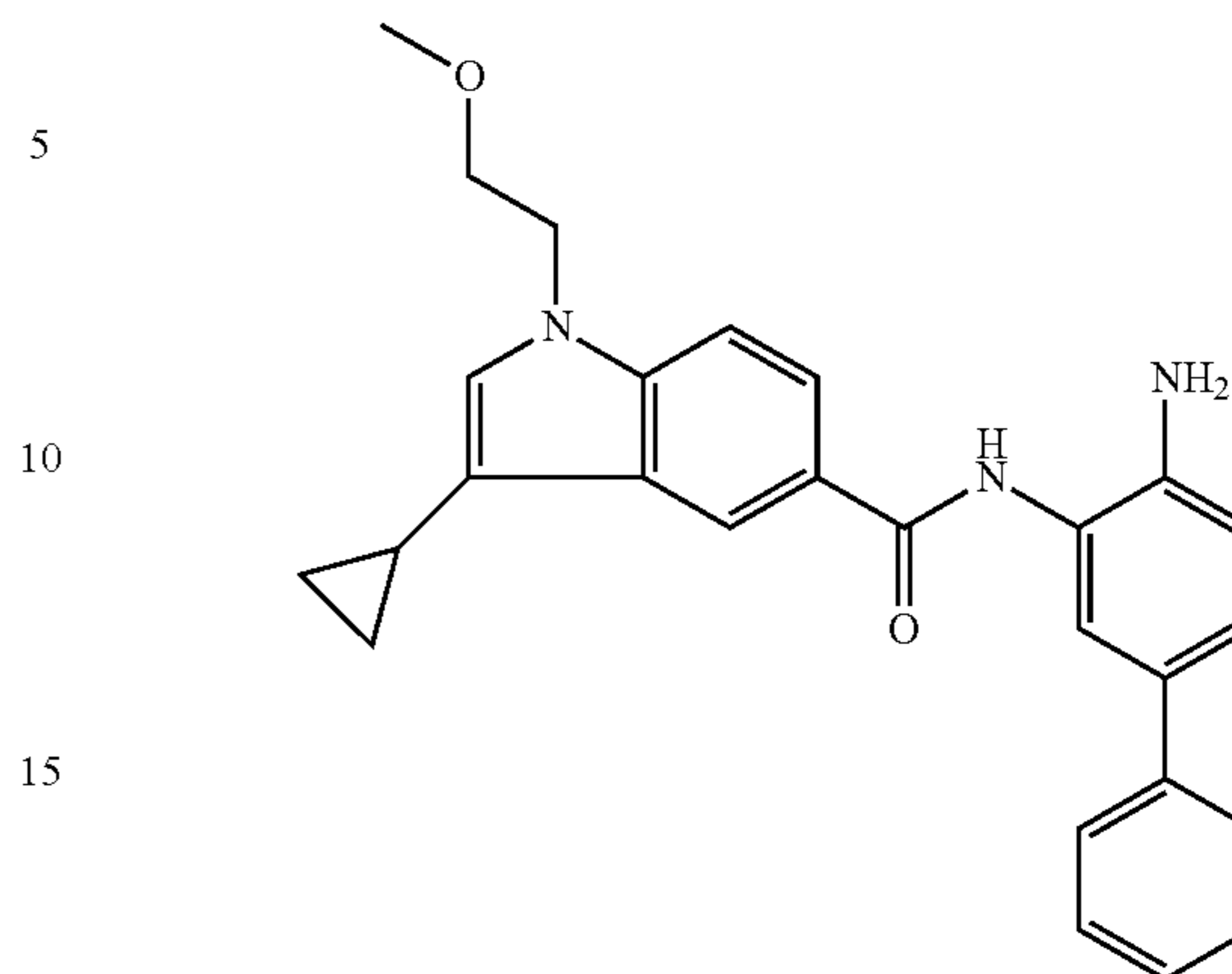
N-(4-amino-[1,1'-biphenyl]-3-yl)-3-cyclopropyl-1-(2-methoxyethyl)-1H-indole-5-carboxamide
