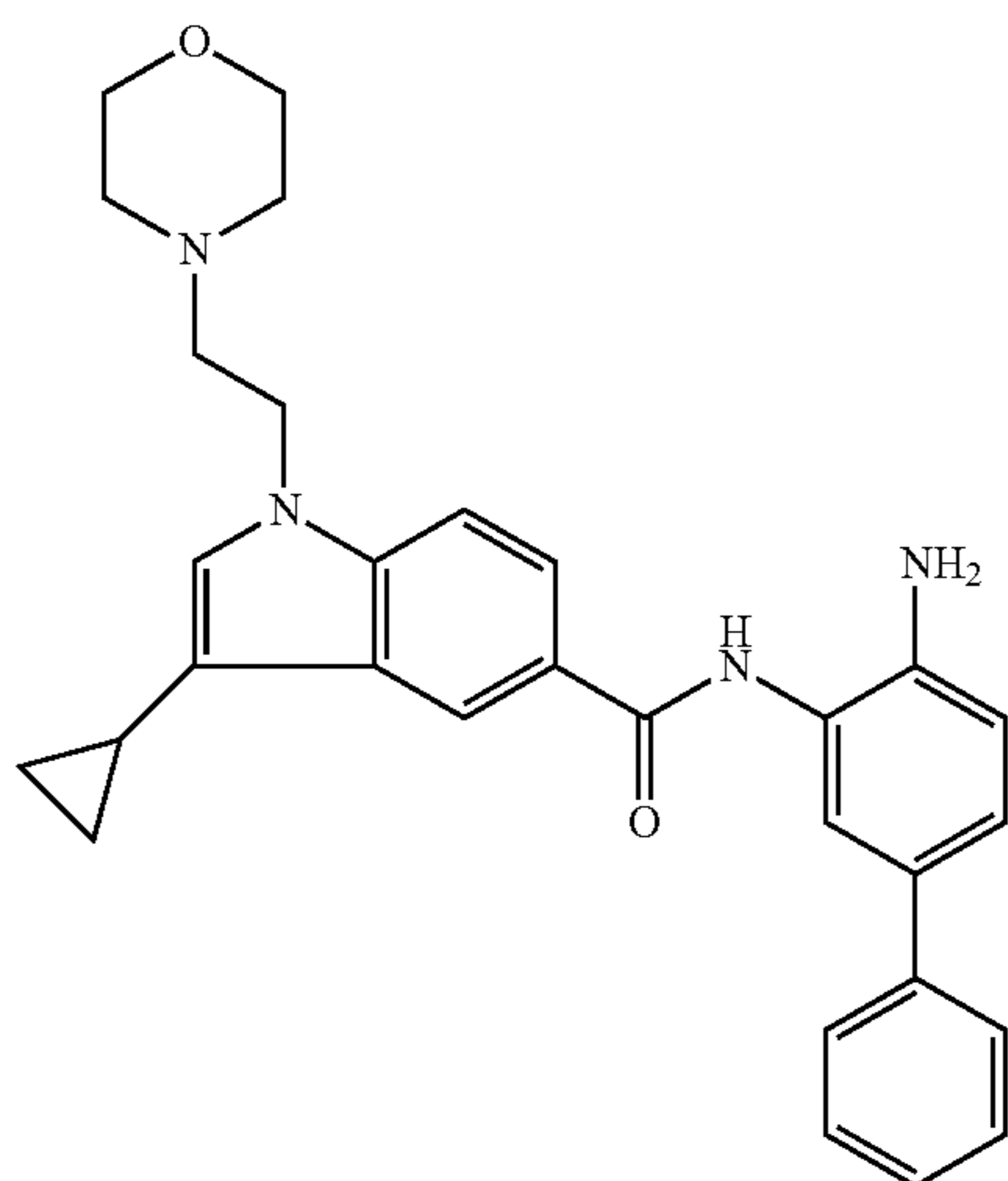
N-(4-amino-[1,1'-biphenyl]-3-yl)-3-cyclopropyl-1-(2-morpholinoethyl)-1H-indole-5-carboxamide
