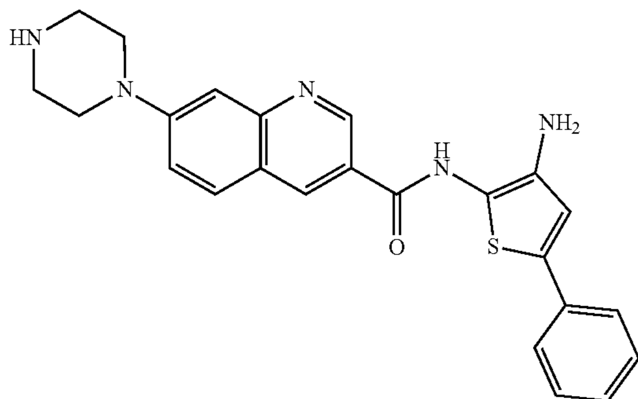
N-(3-amino-5-phenylthiophen-2-yl)-7-(piperazin-1-yl)quinoline-3-carboxamide
