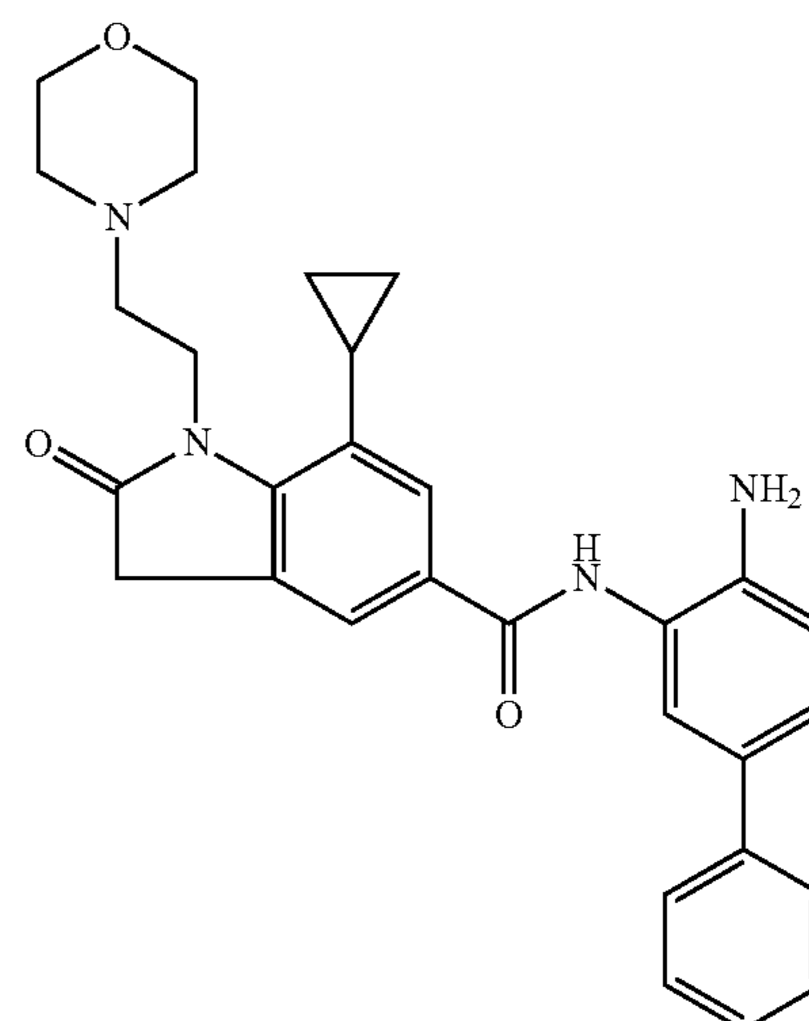
N-(4-amino-[1,1'-biphenyl]-3-yl)-7-cyclopropyl-1-(2-morpholinoethyl)-2-oxindoline-5-carboxamide
