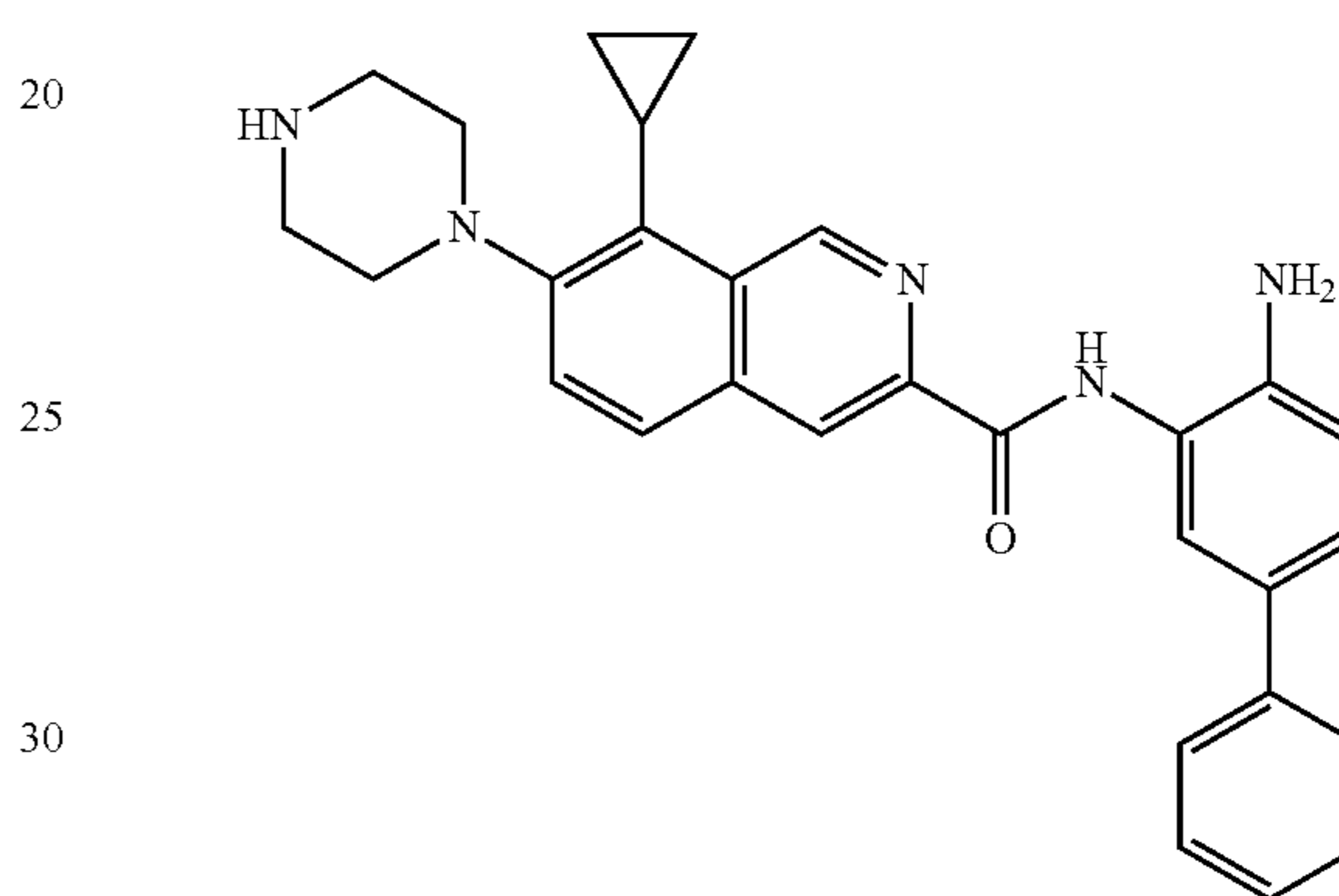
N-(4-amino-[1,1'-biphenyl]-3-yl)-8-cyclopropyl-7-(piperazin-1-yl)isoquinoline-3-carboxamide
