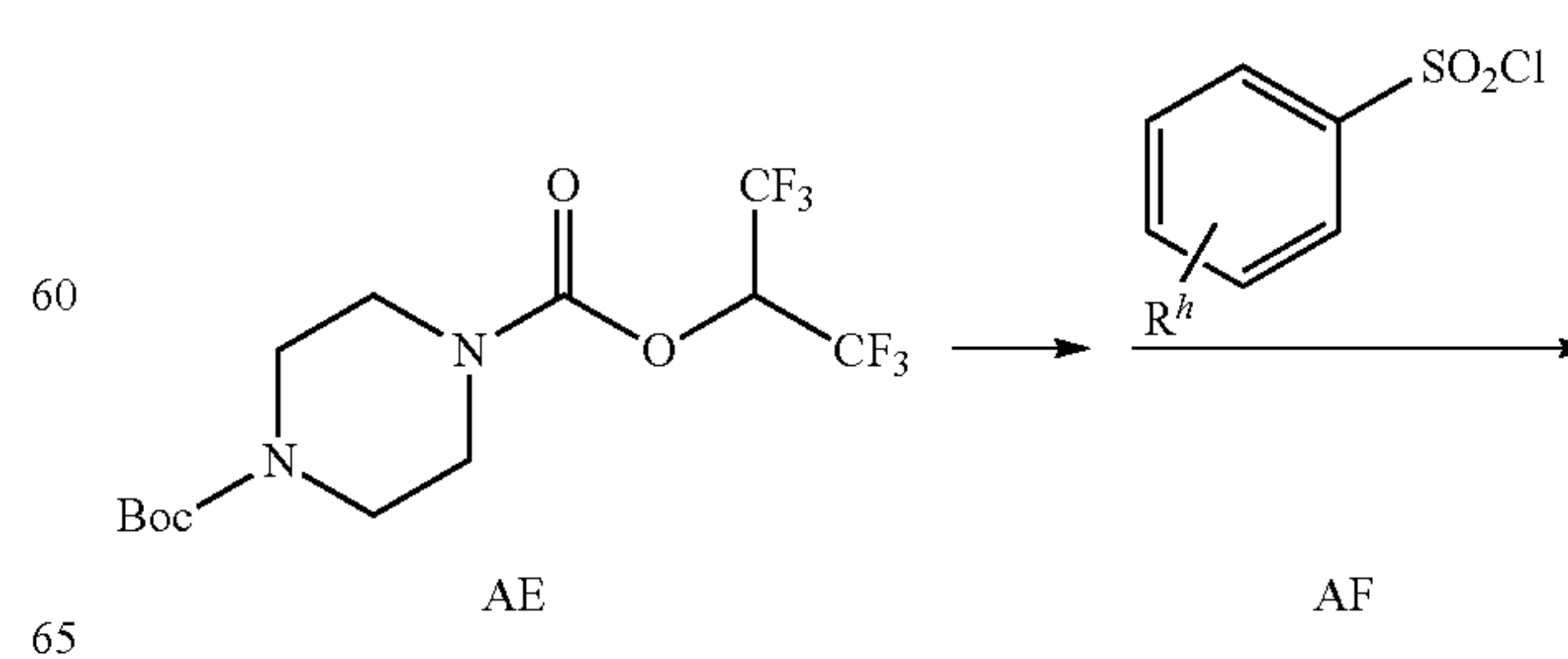
SCHEME 7
