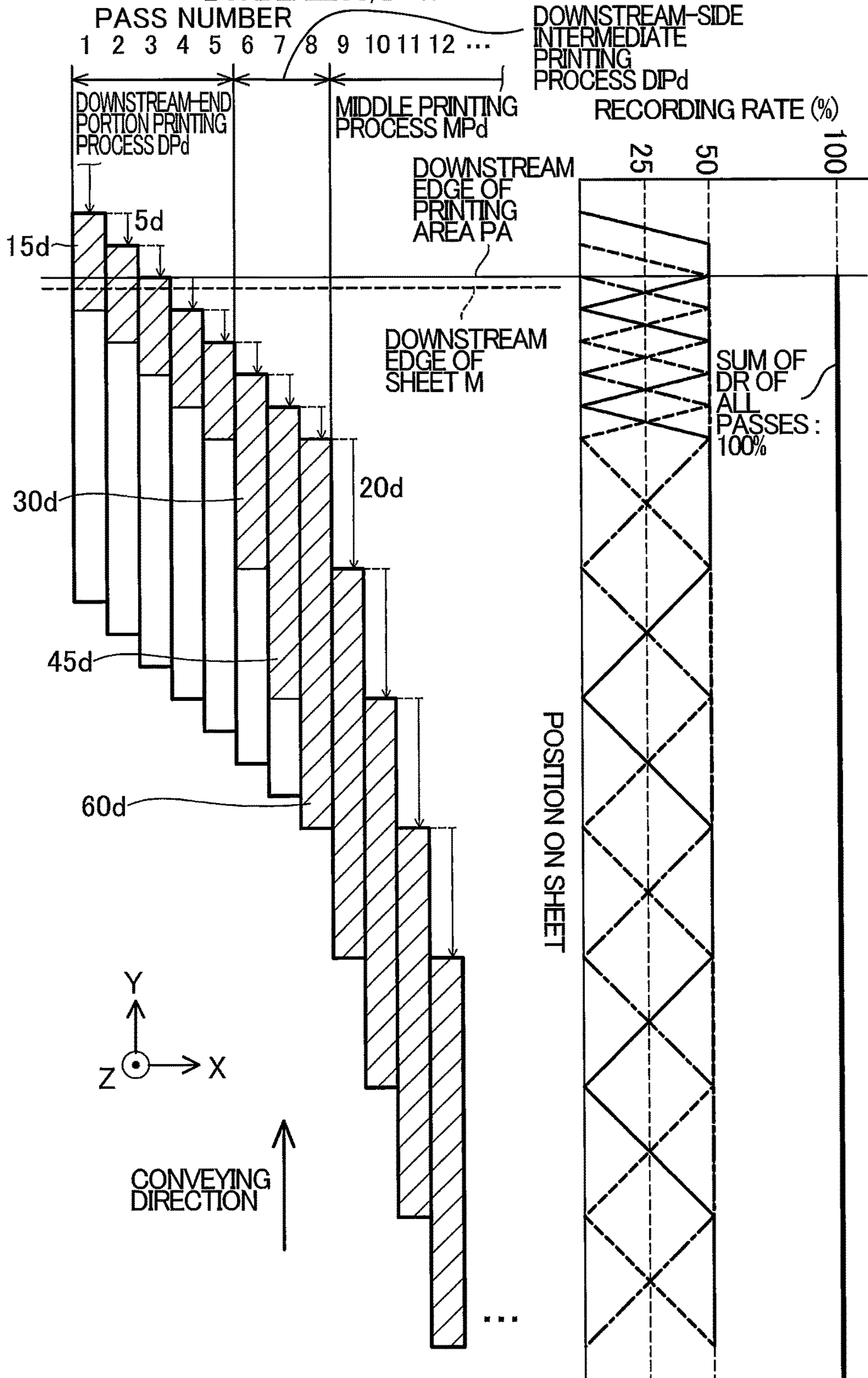
FIG. 22 THIRD EMBODIMENT 3-PASS PRINTING, NORMAL CONTROL, BORDERLESS, DOWNSTREAM EDGE → MIDDLE SECTION
