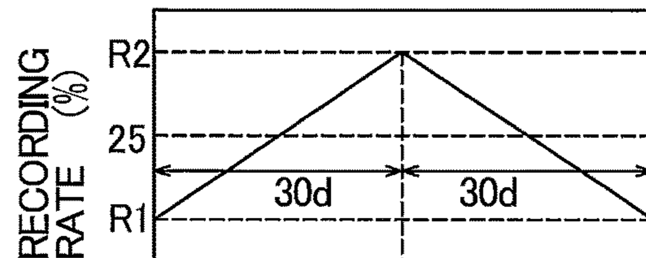
(E) GRADED RECORDING RATE DR (10)~DR (14)
