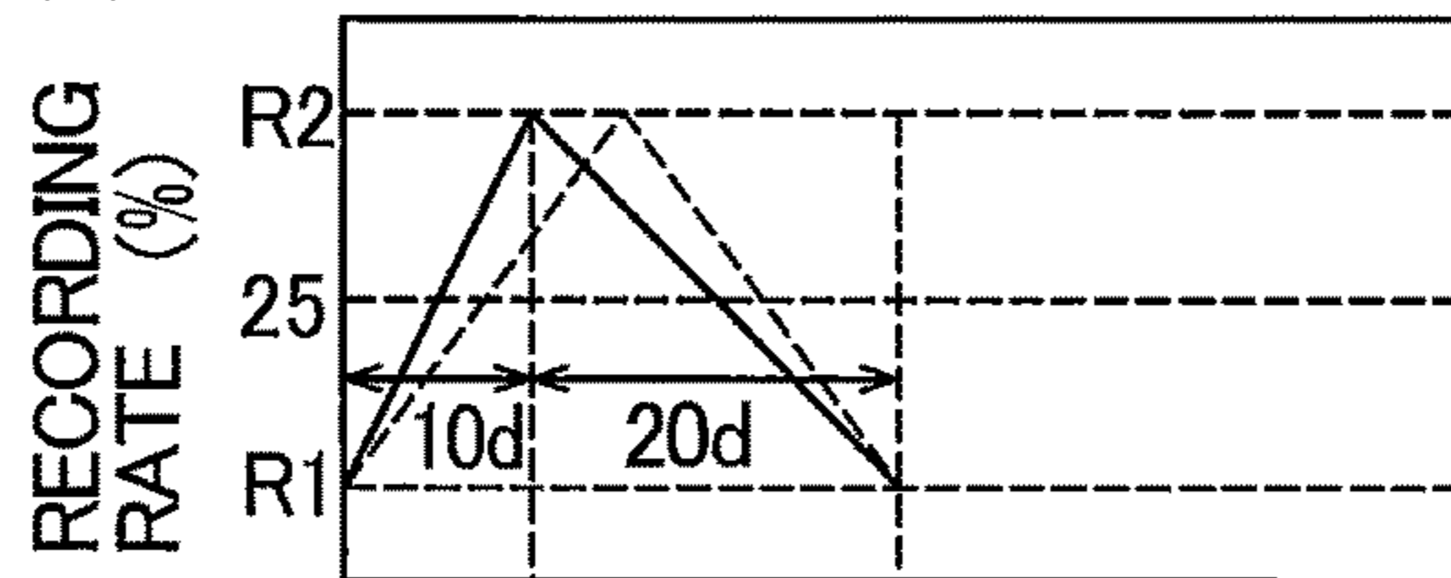
(B) GRADED RECORDING RATE DR (7)
