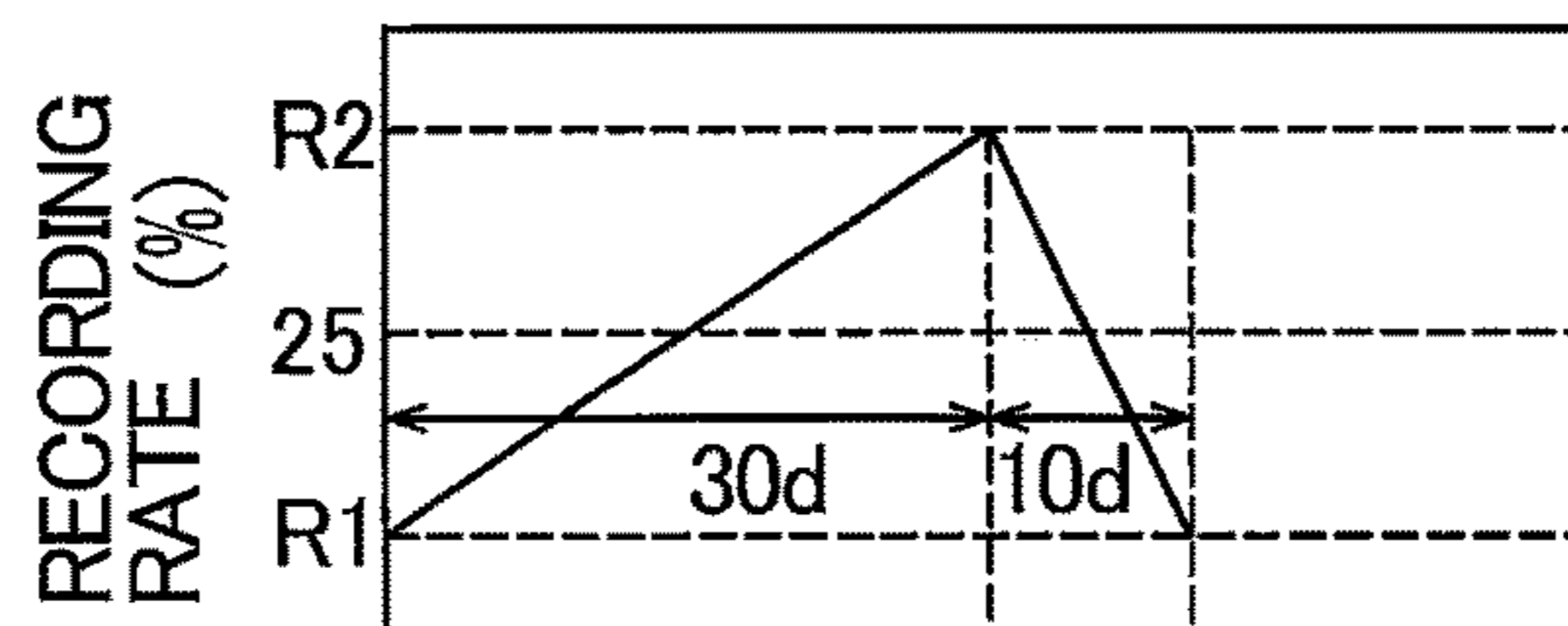
(C) GRADED RECORDING RATE DR (19)
