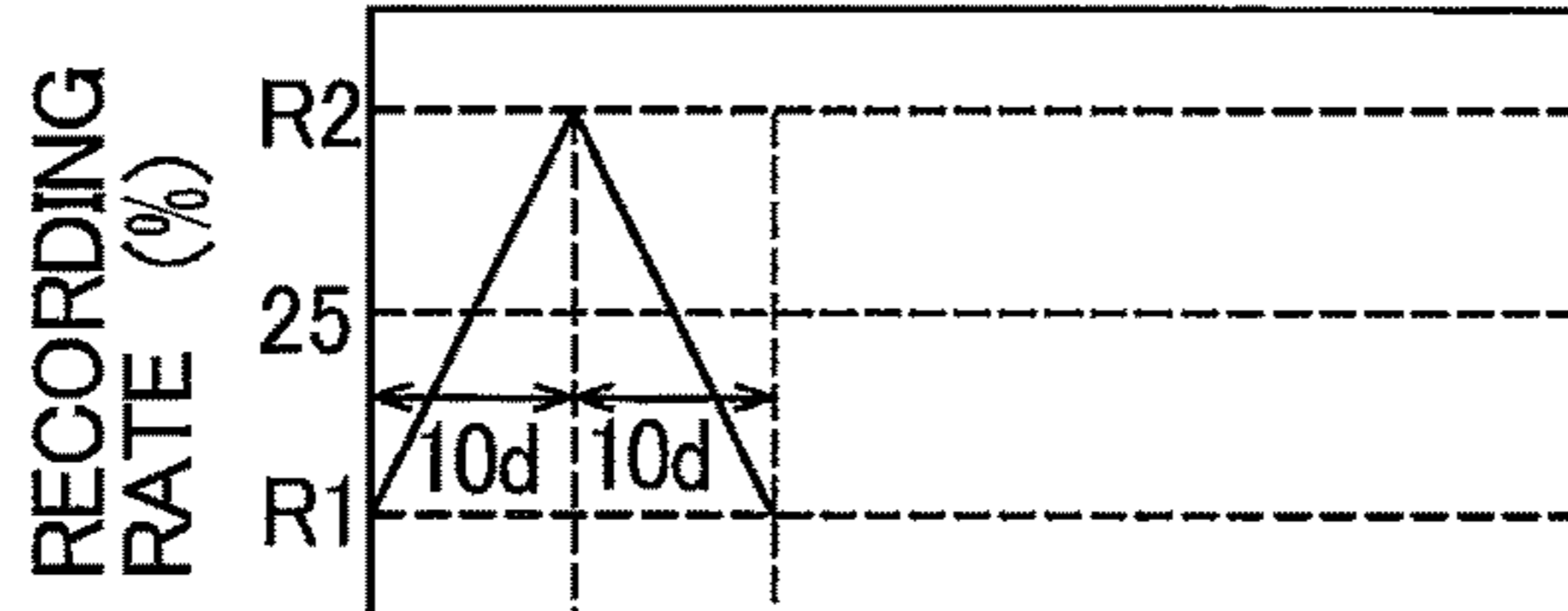
(A) GRADED RECORDING RATE DR (1)~DR (6)
