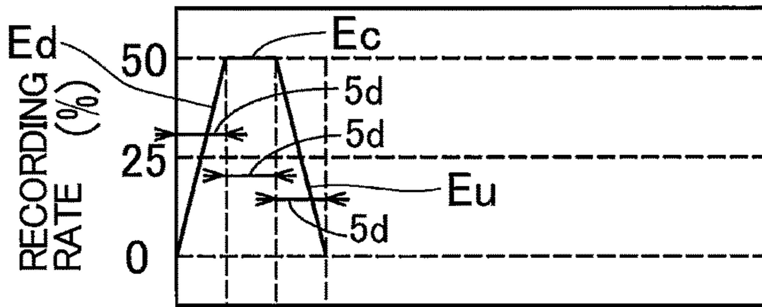
(A) GRADED RECORDING RATE DR (1)~DR (5)
