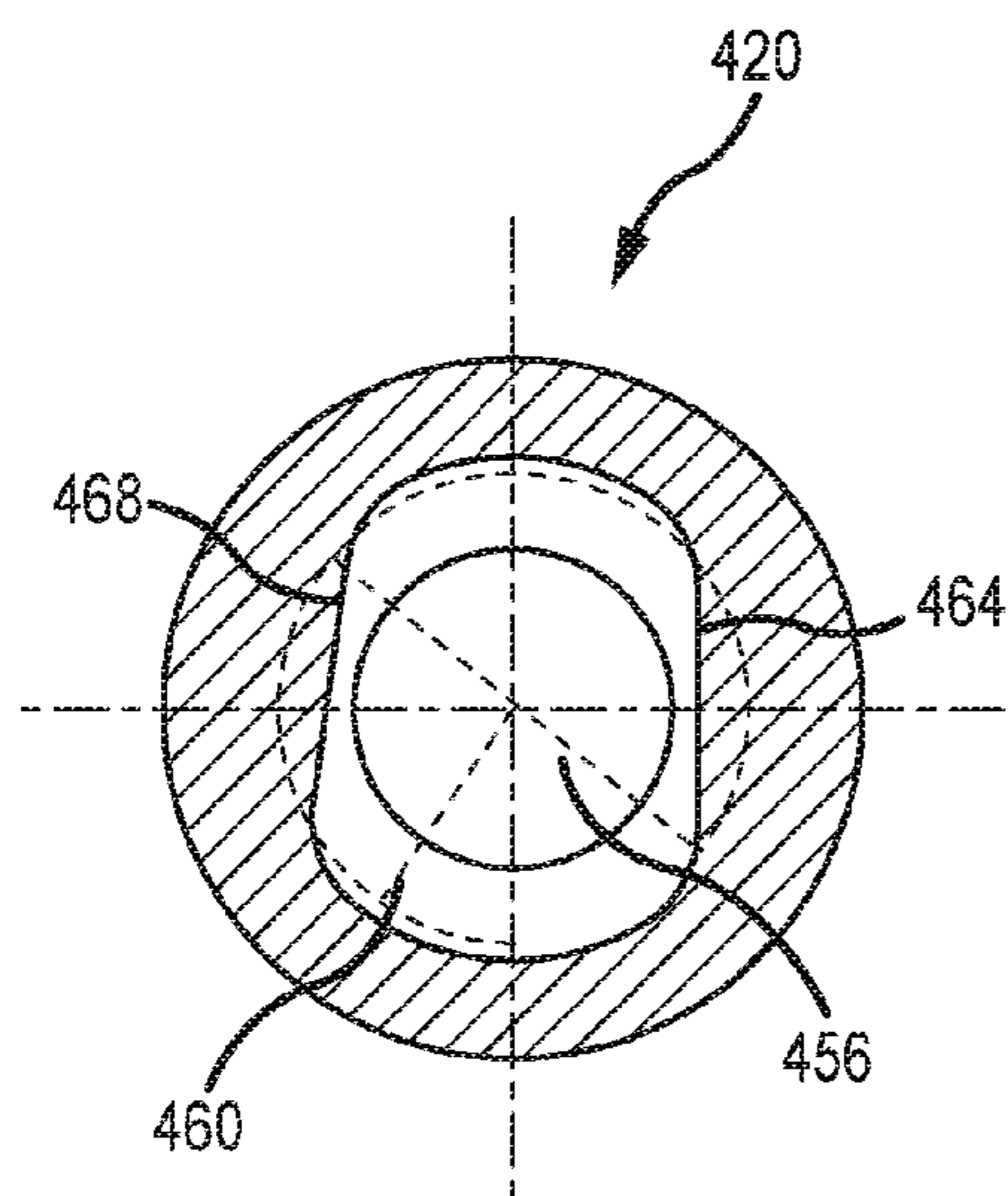
SECTION E-E
