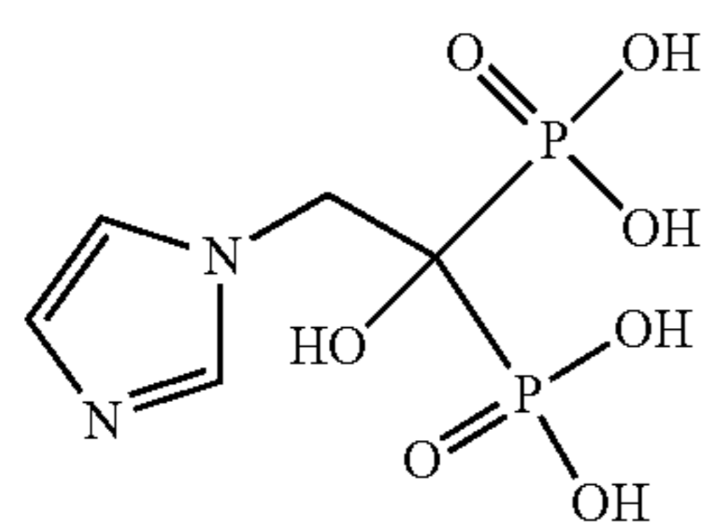
Zoledronic acid
