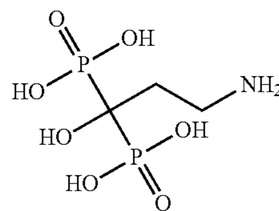
pamidronic acid
