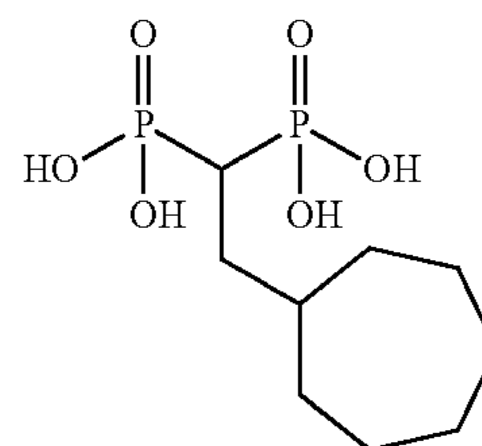
cimadronic acid
