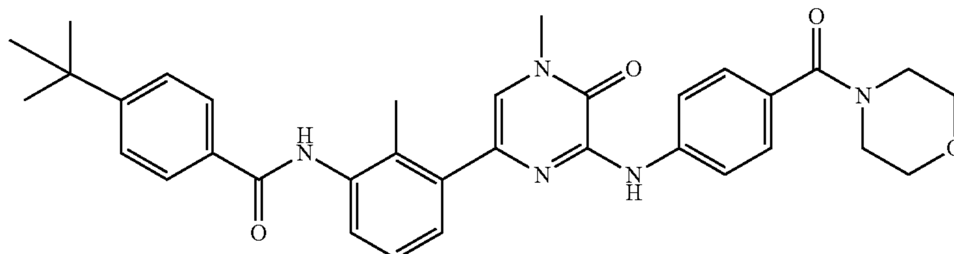
CGI-1746
