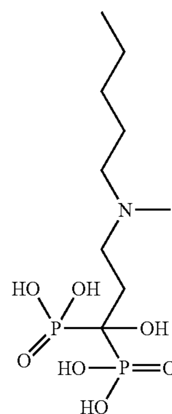
ibandronic acid
