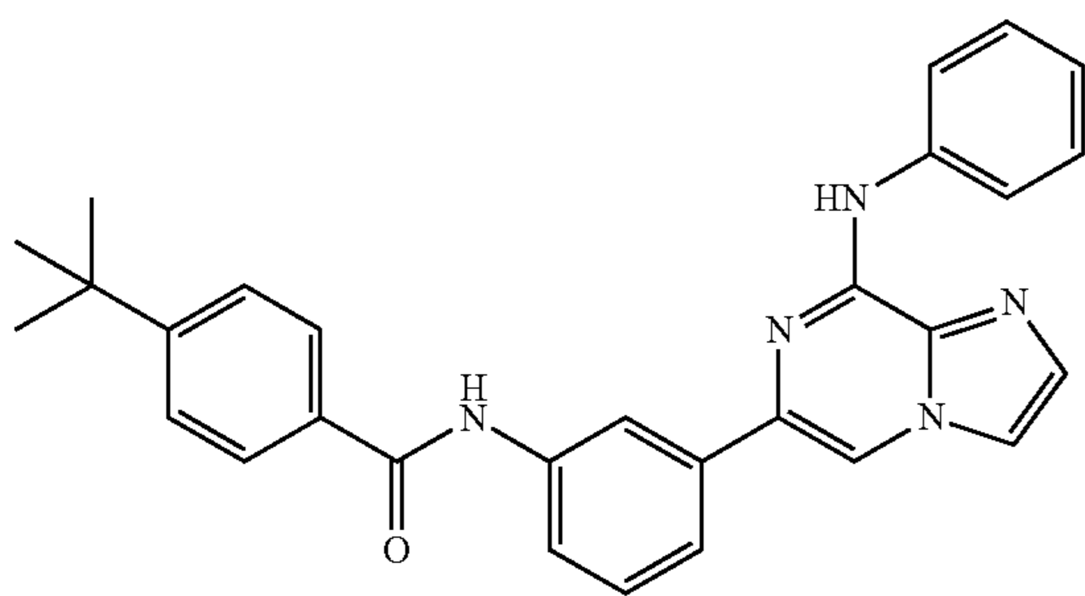
CGI-560
