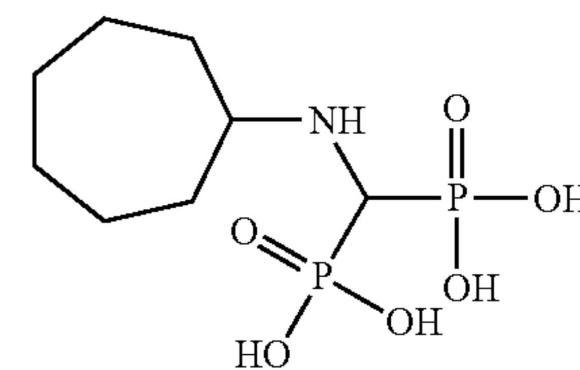
incadronic acid
