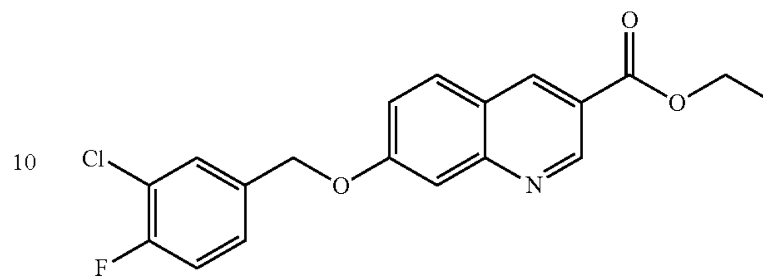
Example 15. Ethyl 7-((3,5-difluorobenzyl)oxy)quinoline-3-carboxylate
