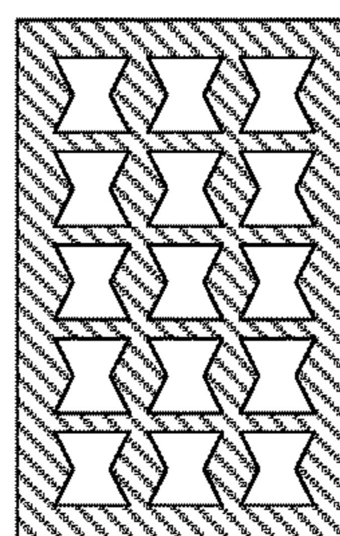
CONCAVE-SHAPED MOLD TRAY (TOP VIEW) FIG. 34
