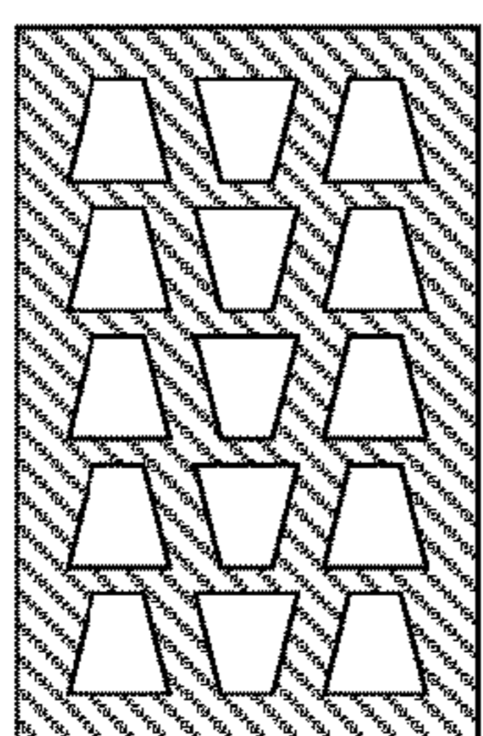
TRAPEZOIDAL- SHAPED MOLD TRAY (TOP VIEW) FIG. 33
