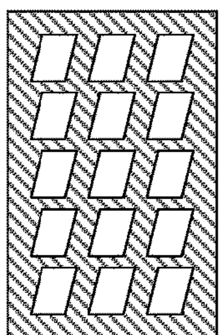
PARALLELOGRAM- SHAPED MOLD TRAY (TOP VIEW) FIG. 35
