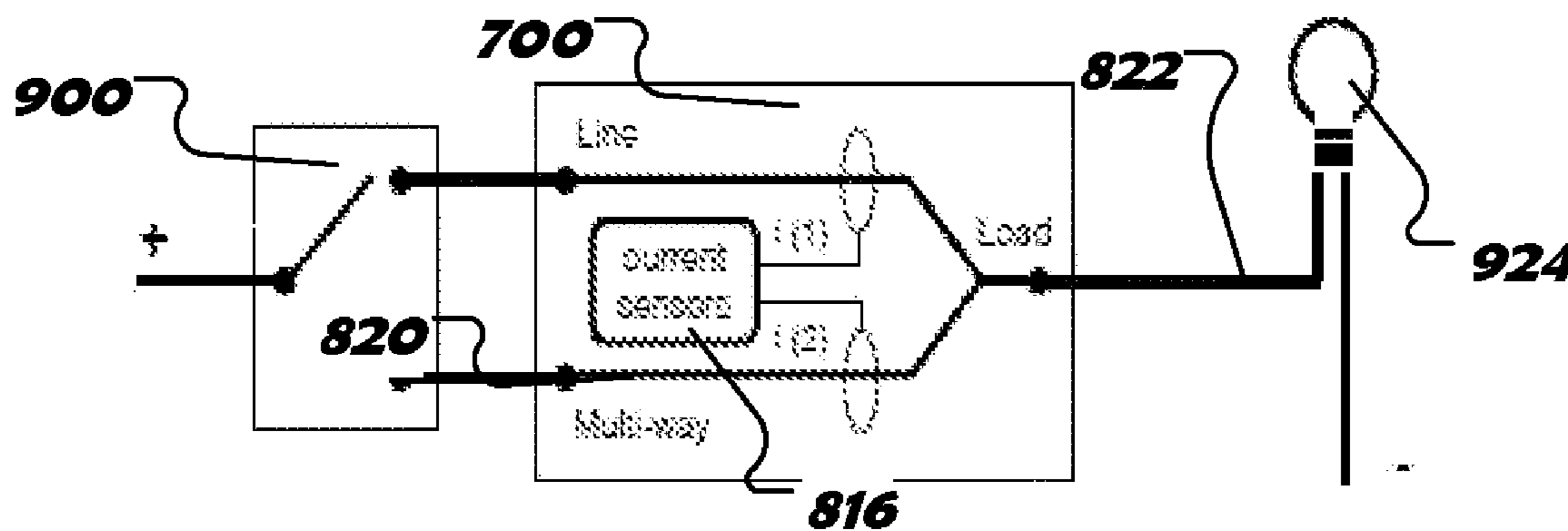
3-way w/ 3rd-party switch sourcing 3-way switch
