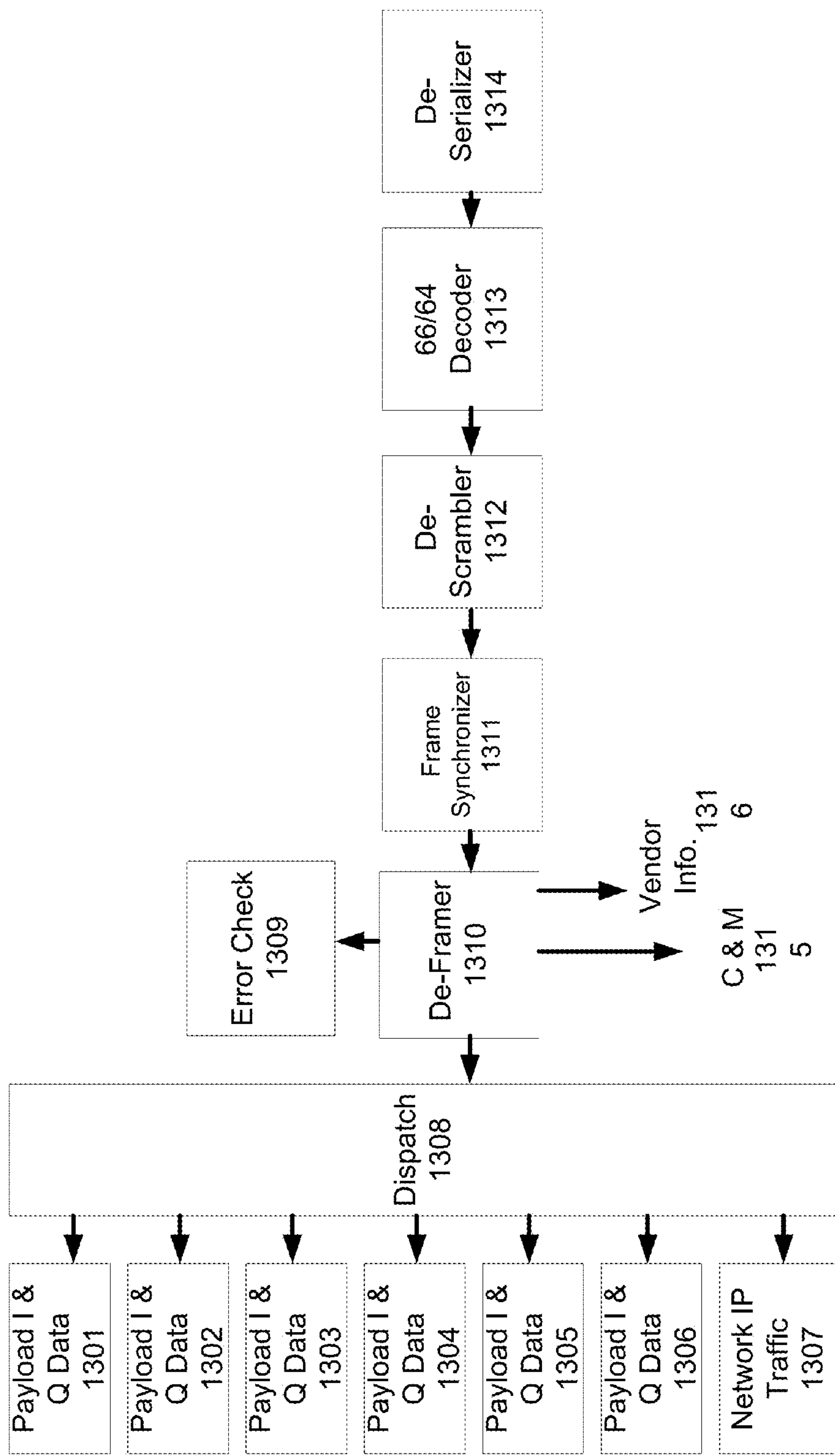
Figure 13. Decoding Data for DAU Uplink Path and DRU Downlink Path
