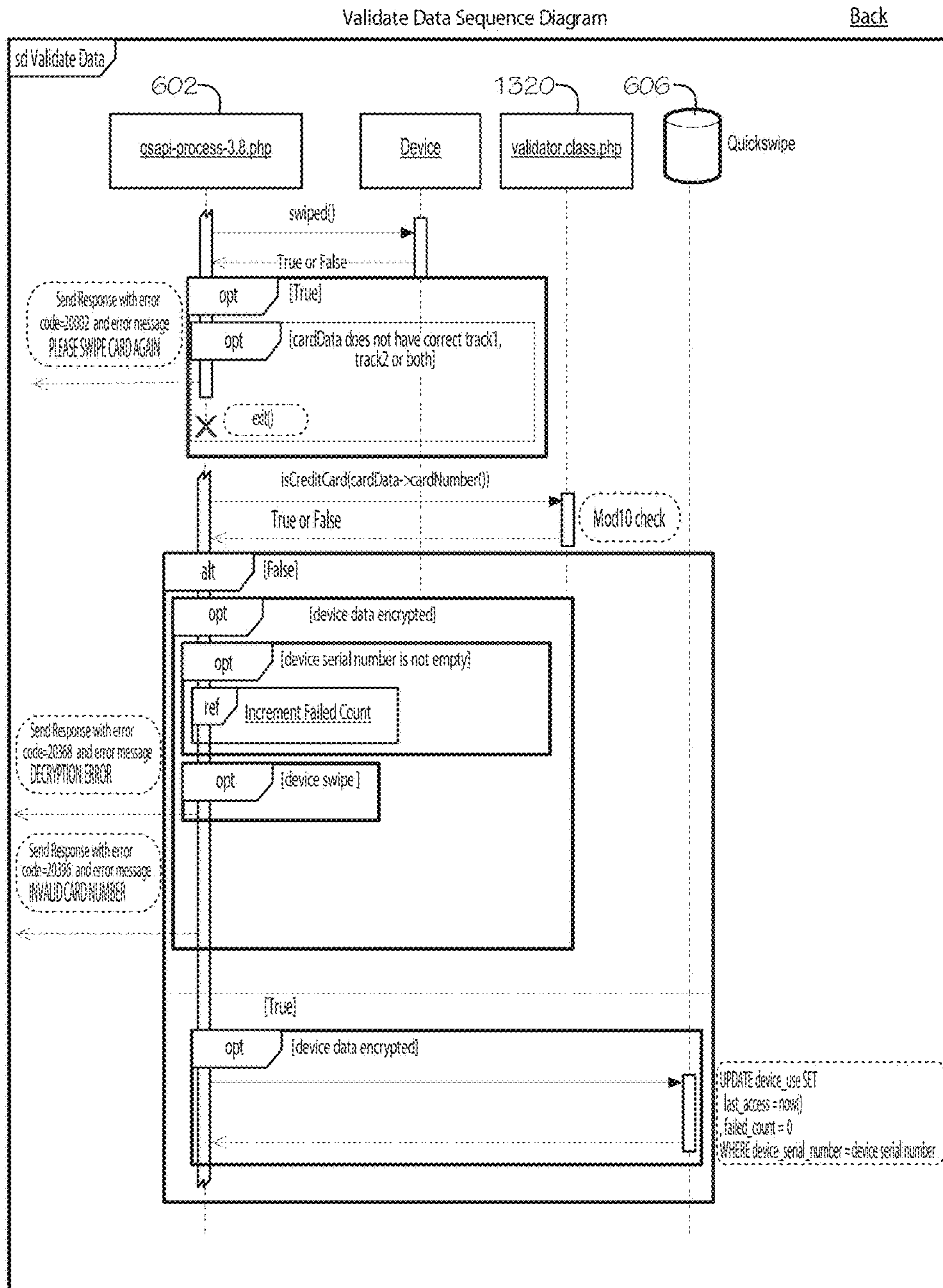
UML OF EXEMPLARY VALIDATION SEQUENCE
