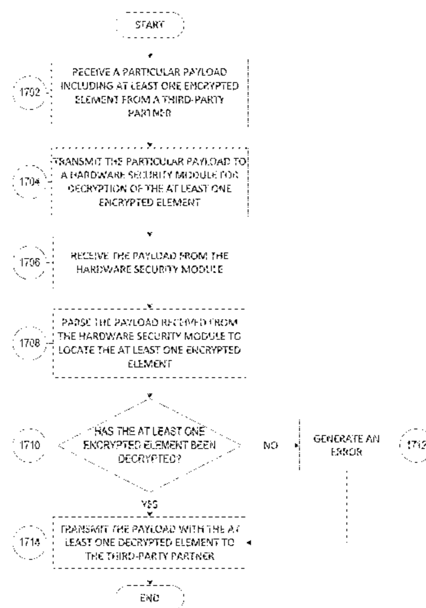
EXEMPLARY DECRYPTION VERIFICATION PROCESS
