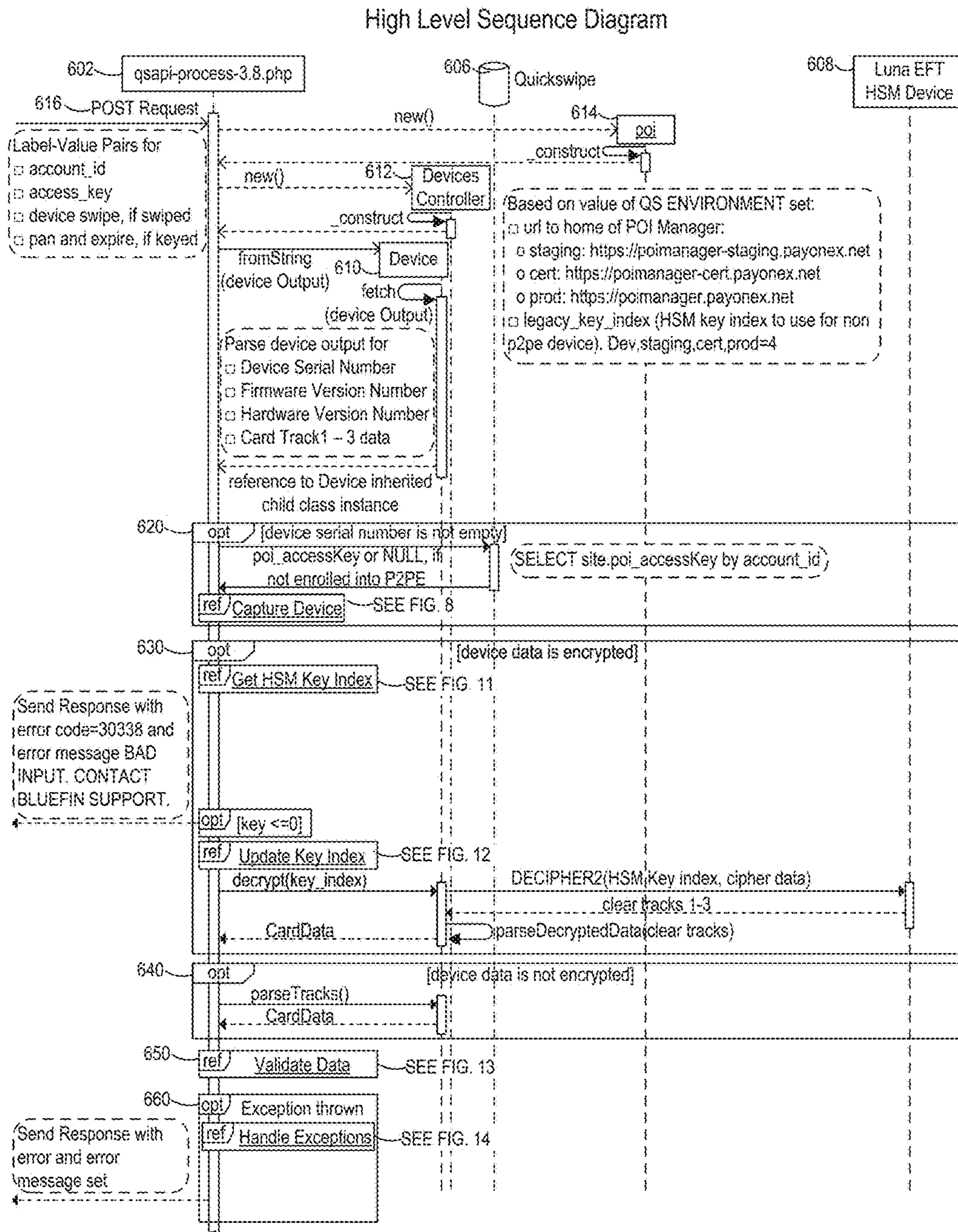
FIG. 6 : UML OF EXEMPLARY OVERALL SEQUENCE
