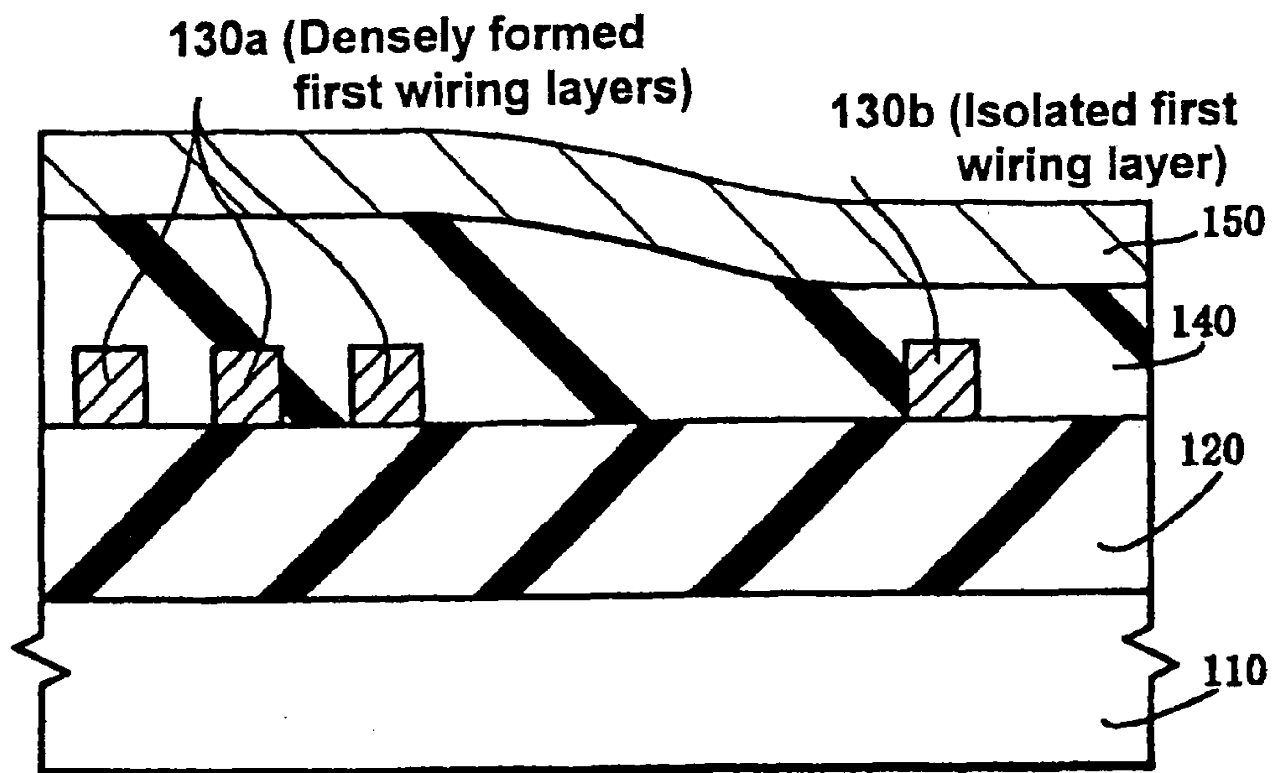
Fig. 18 (Prior Art)
