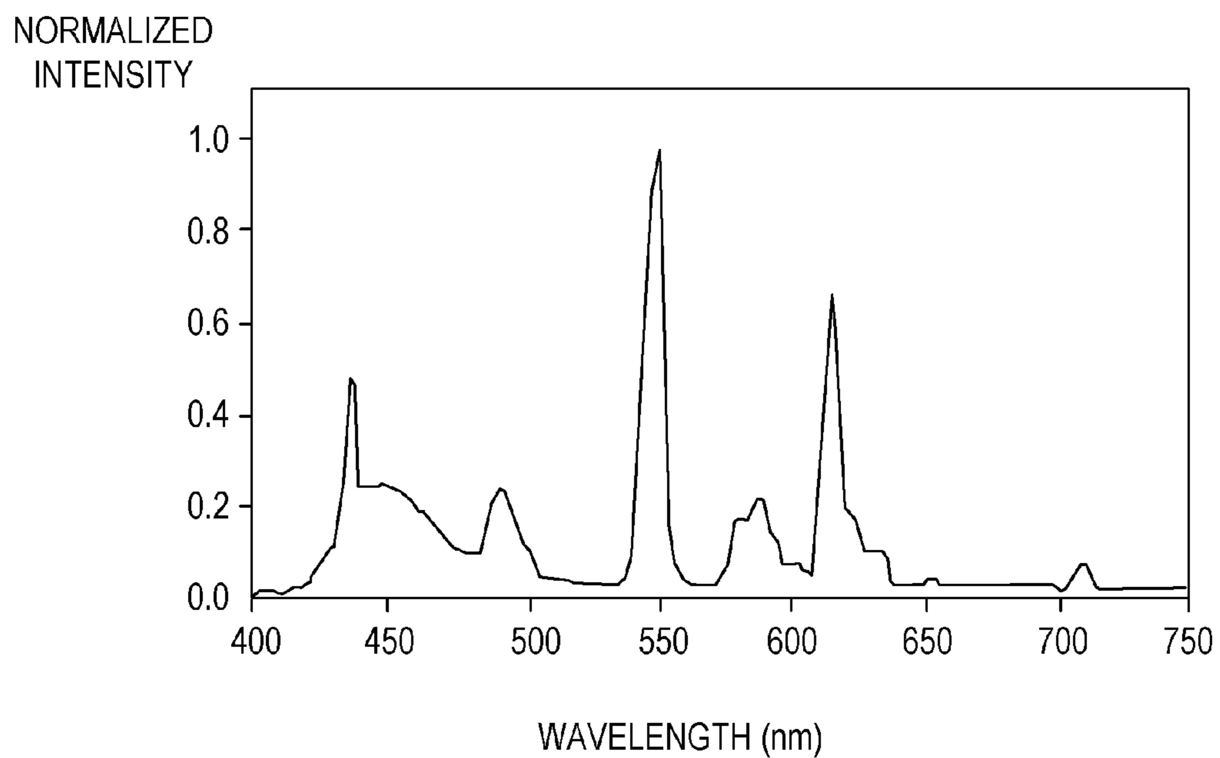
FIG. 3 (PRIOR ART)
