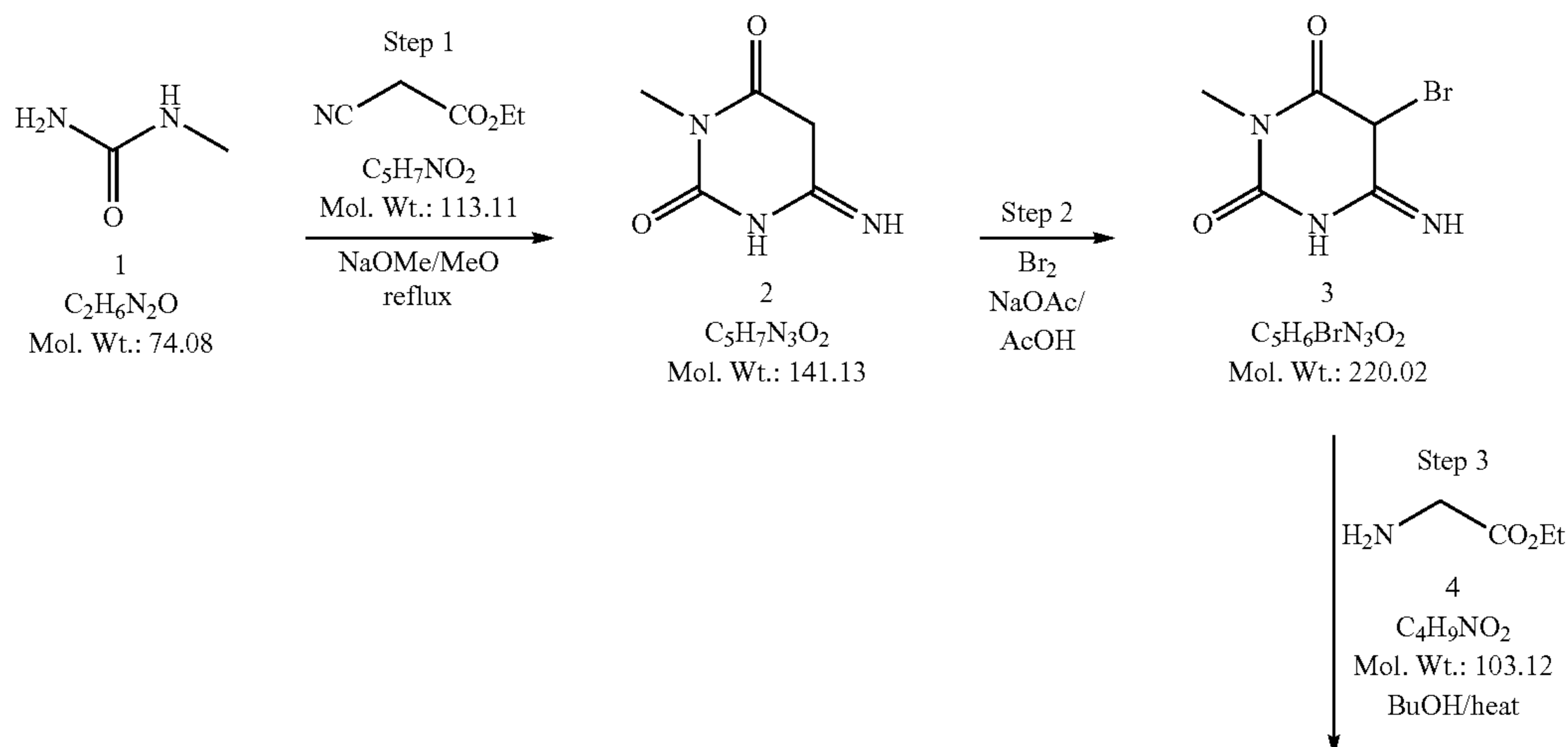
Scheme 2
