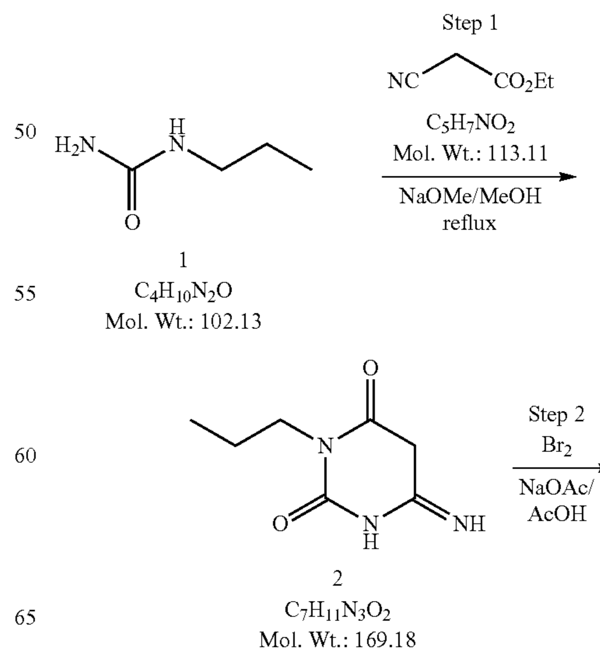
Scheme 1
