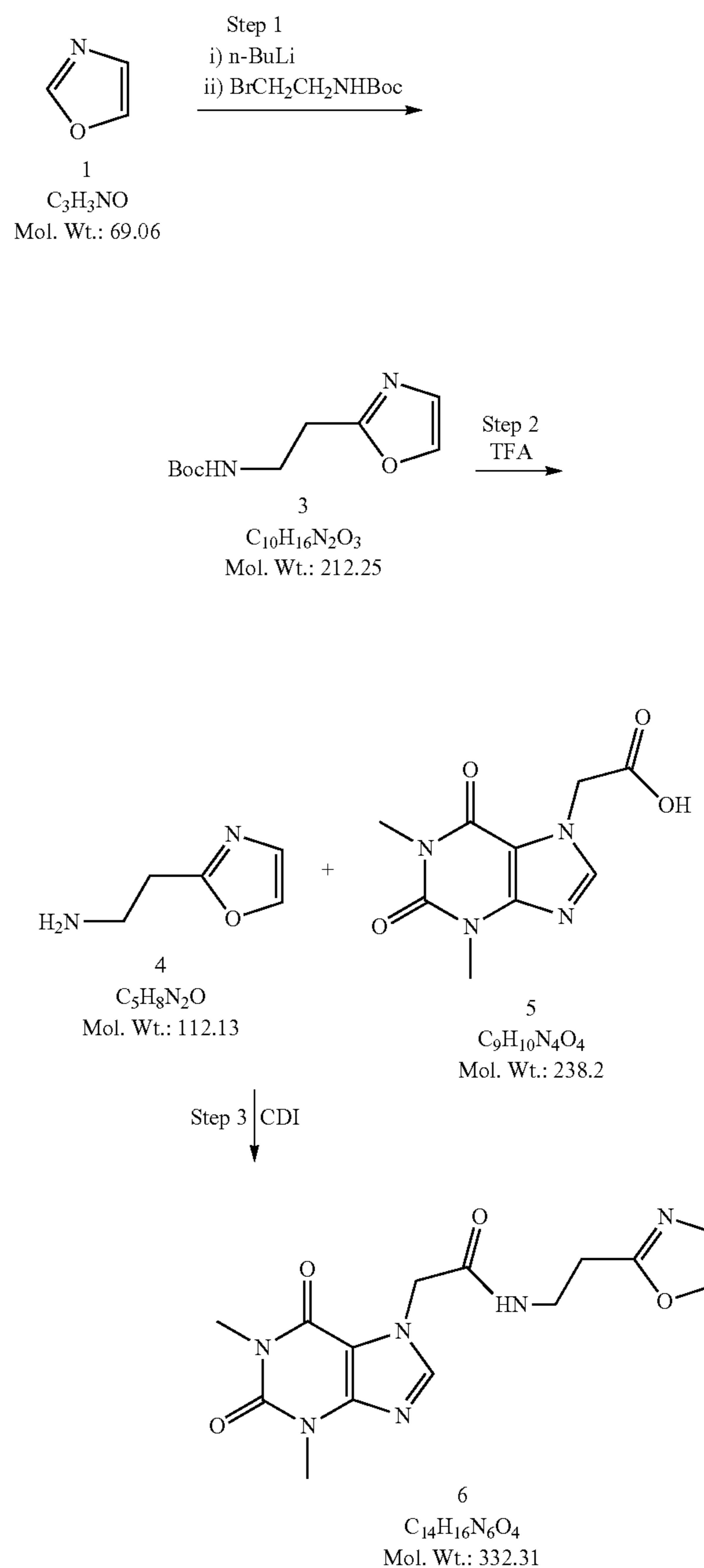
Scheme 11
