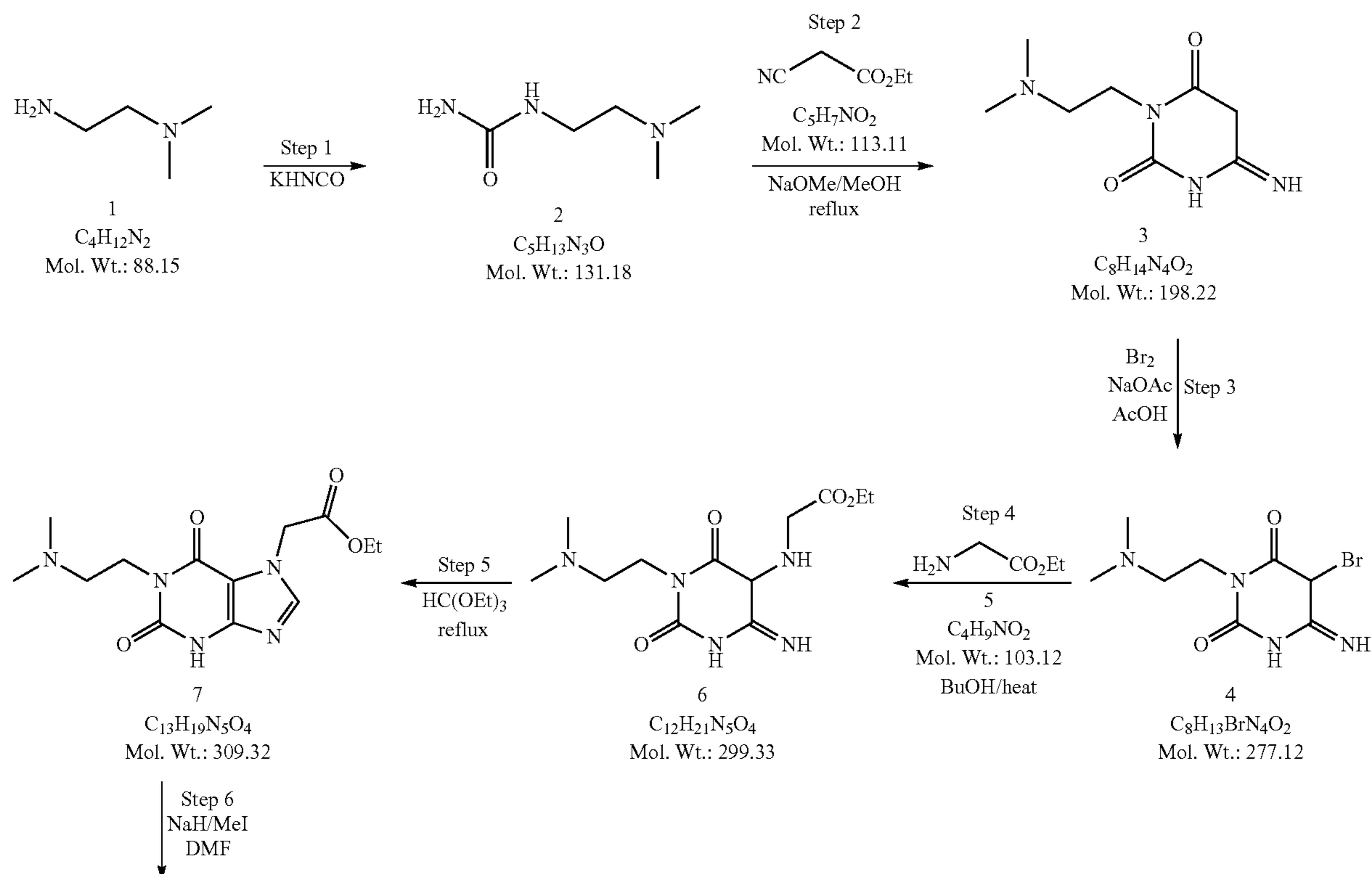
Scheme 3
