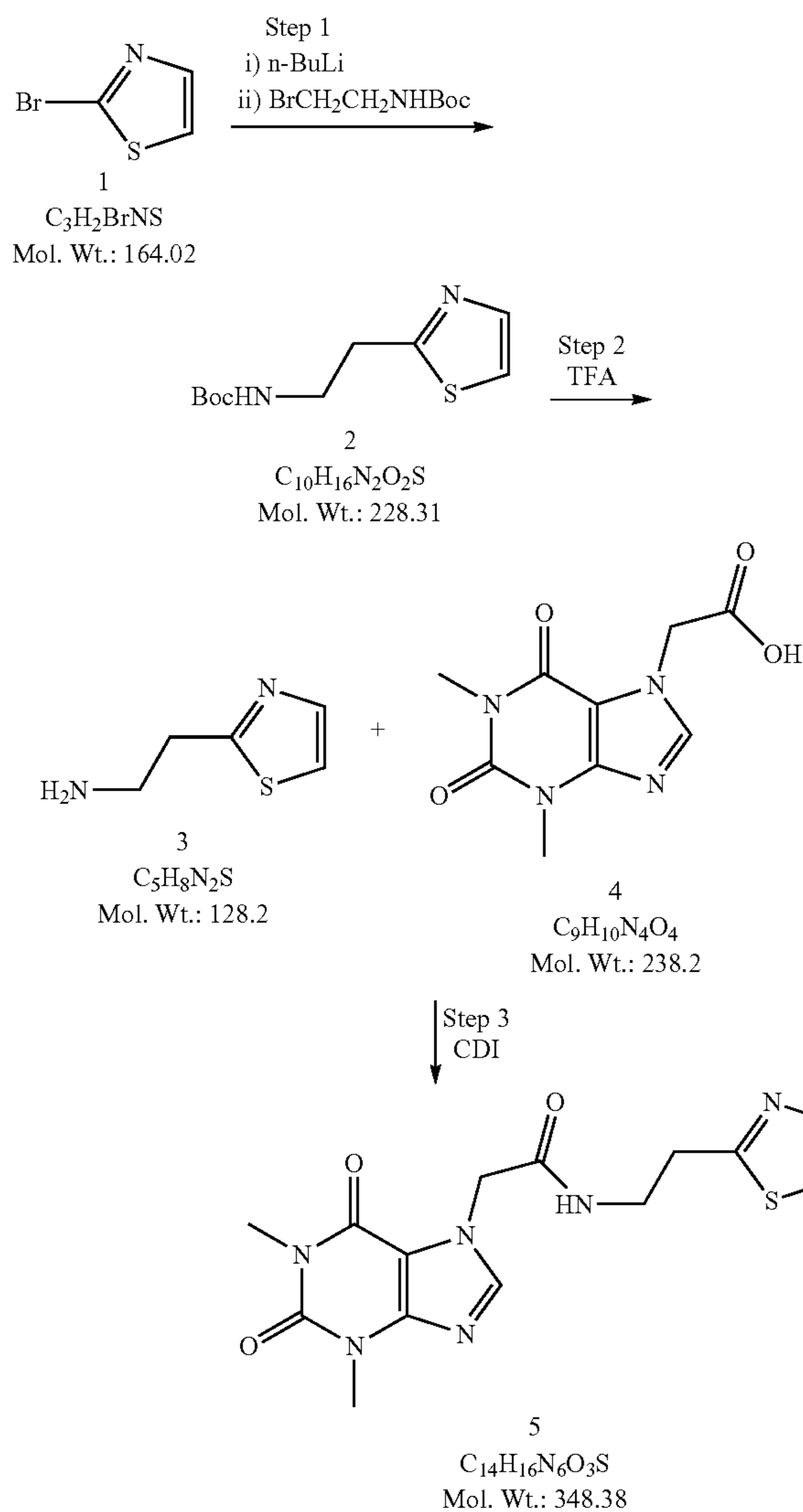
Scheme 9
