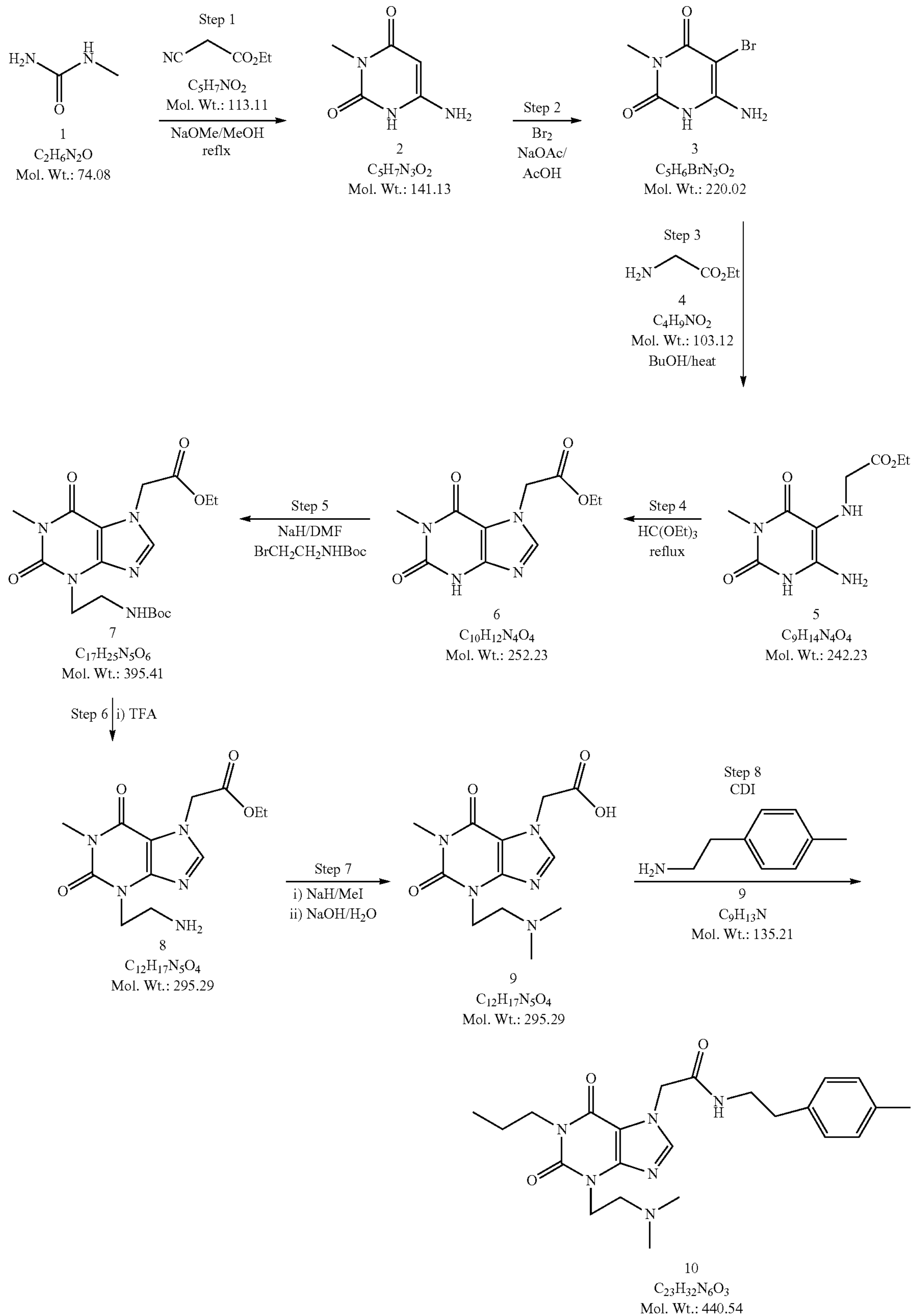
Scheme 12
