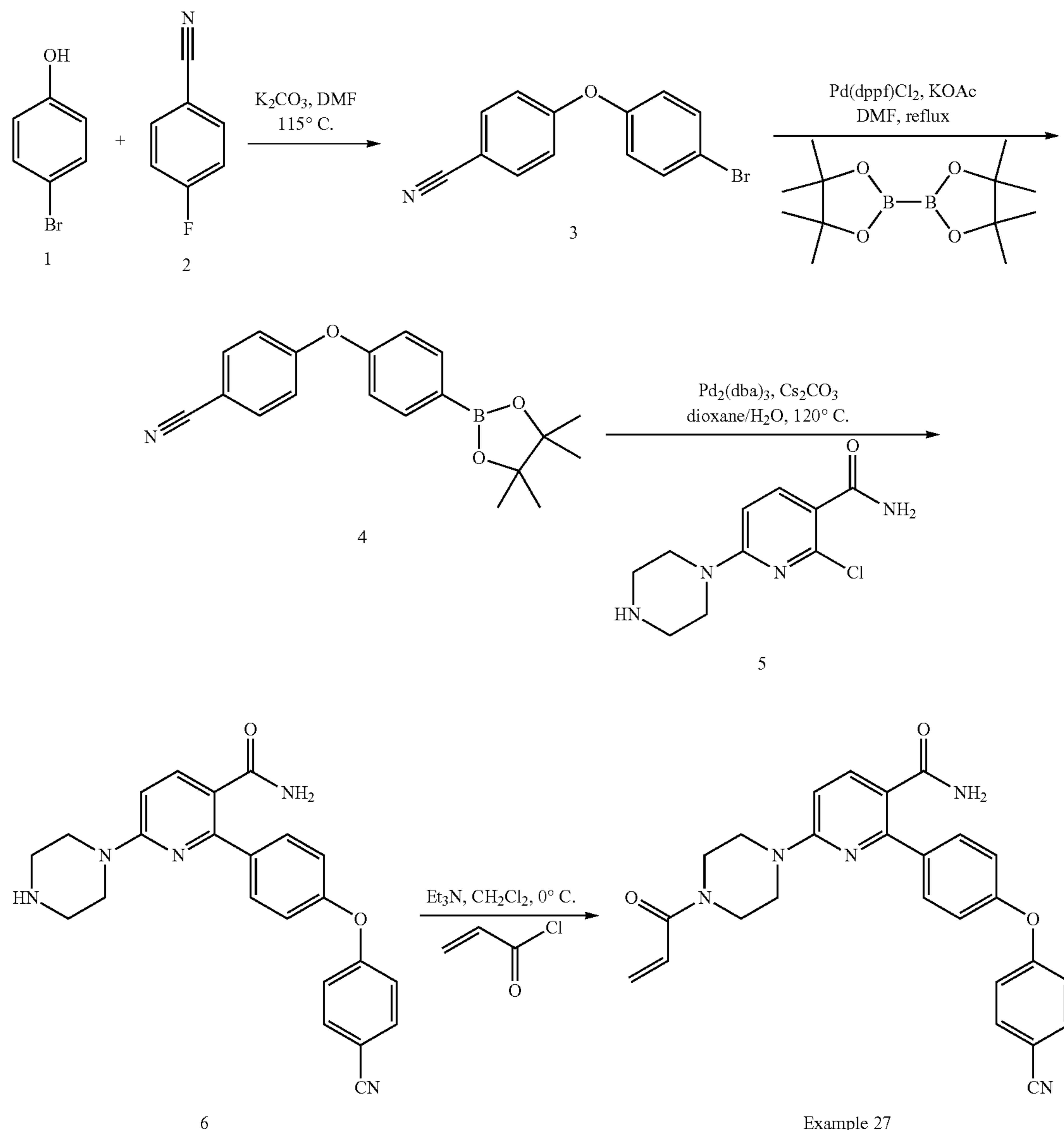
Scheme 16
