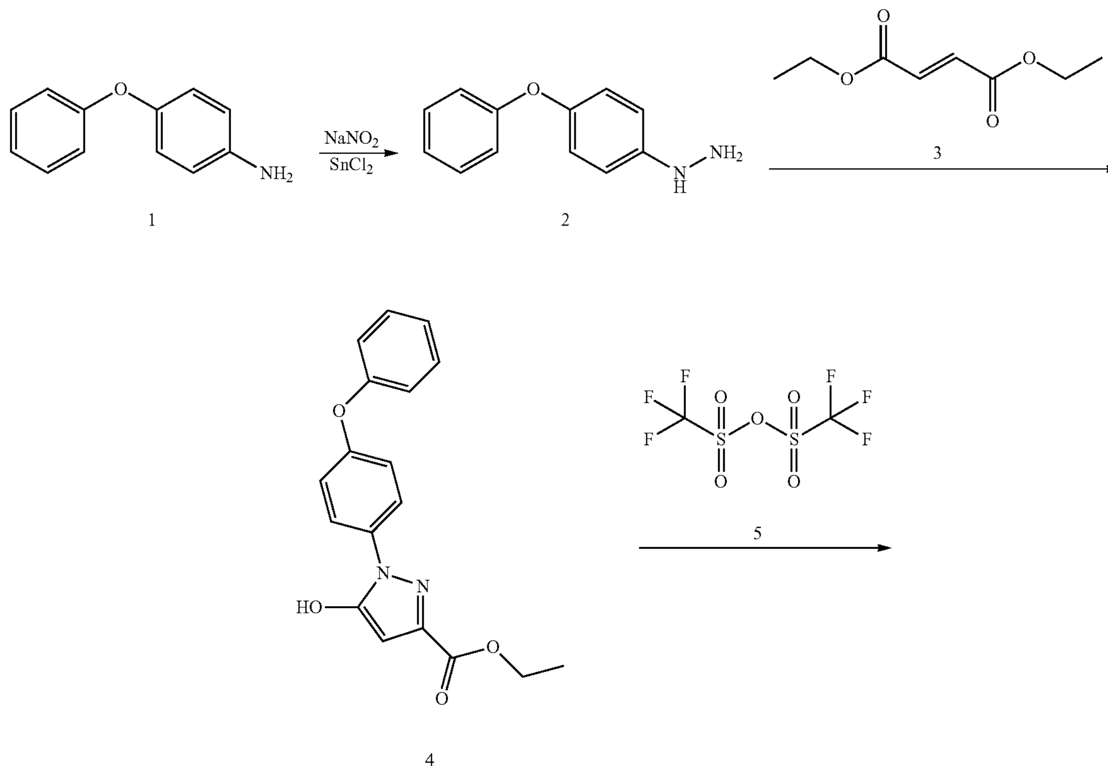
Scheme 46
