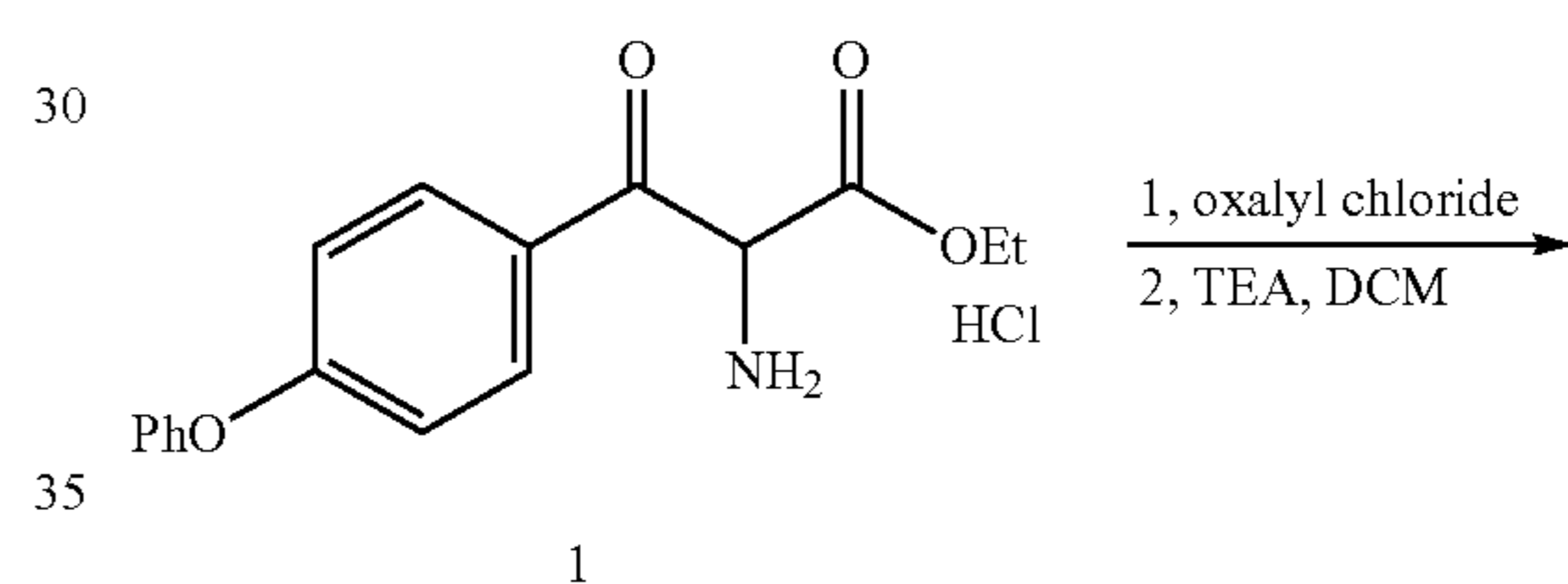
Scheme 44
