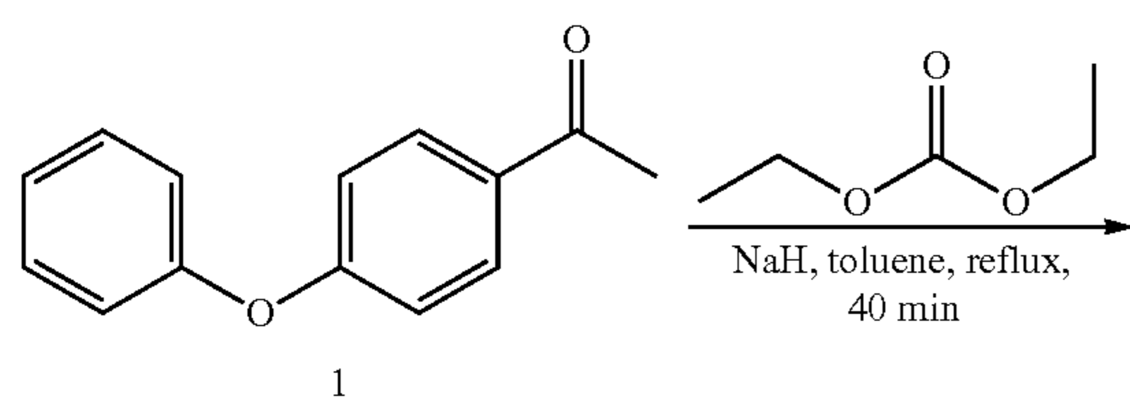
Scheme 32
