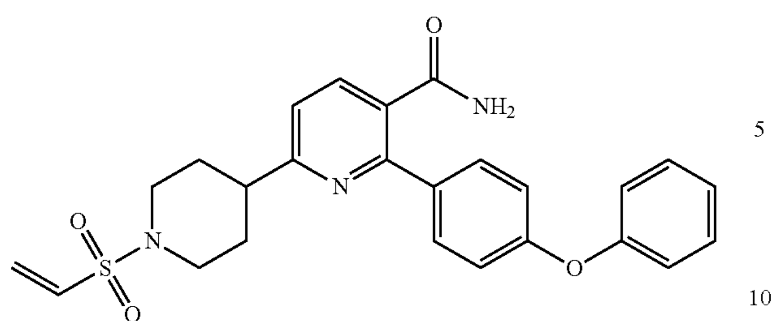
2-(4-phenoxyphenyl)-6-(1-(vinylsulfonyl)piperidin-4-yl) nicotinamide.
