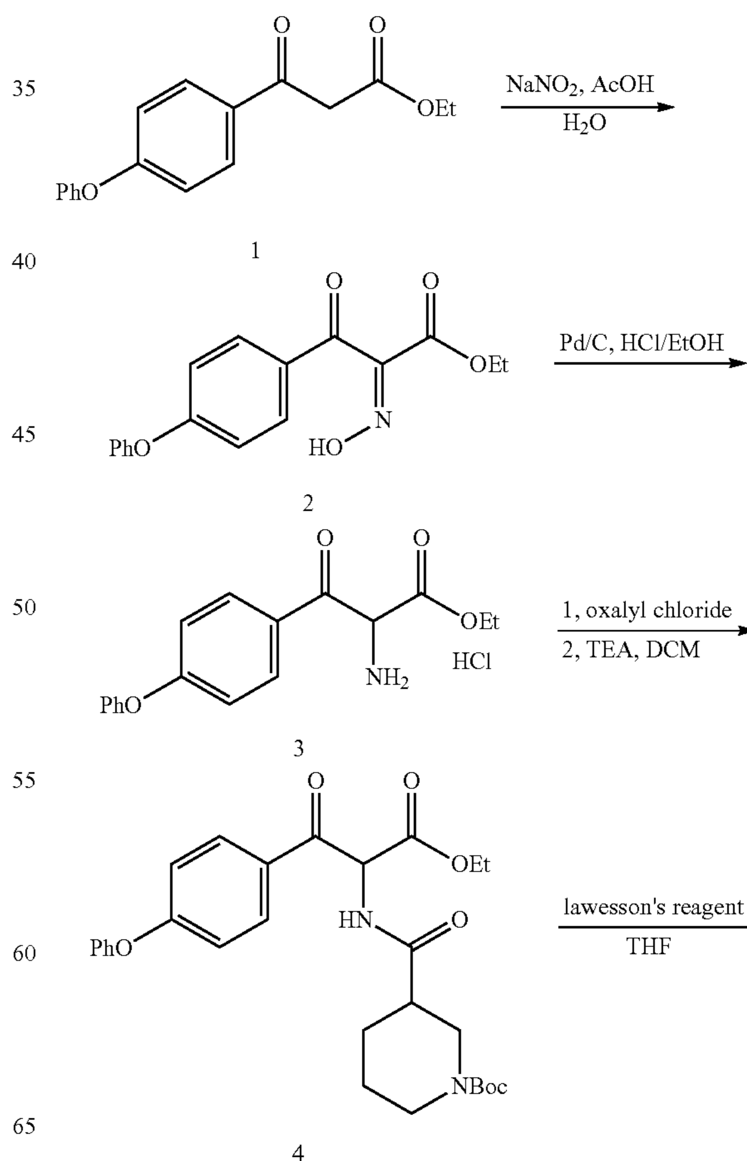
Scheme 35
