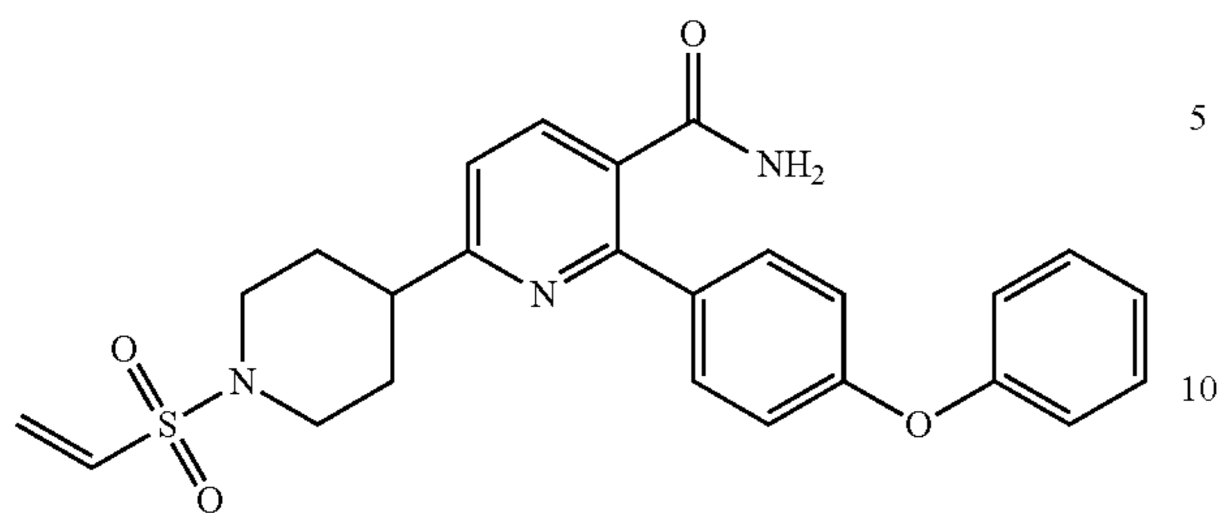
Example 63
