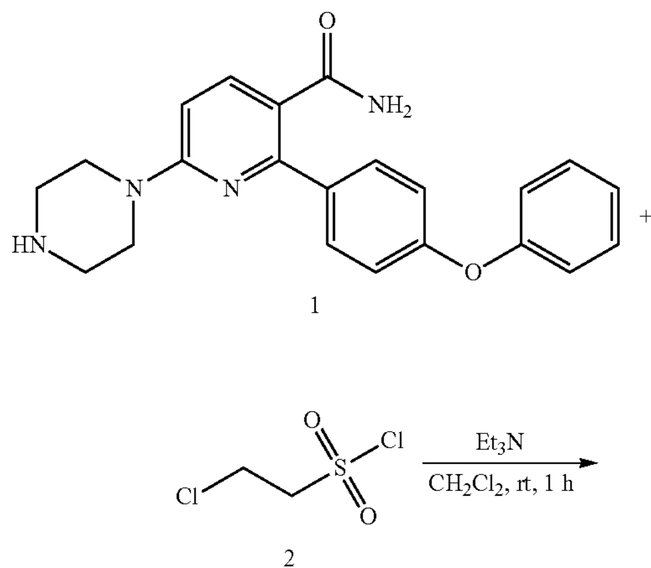
Scheme 52
