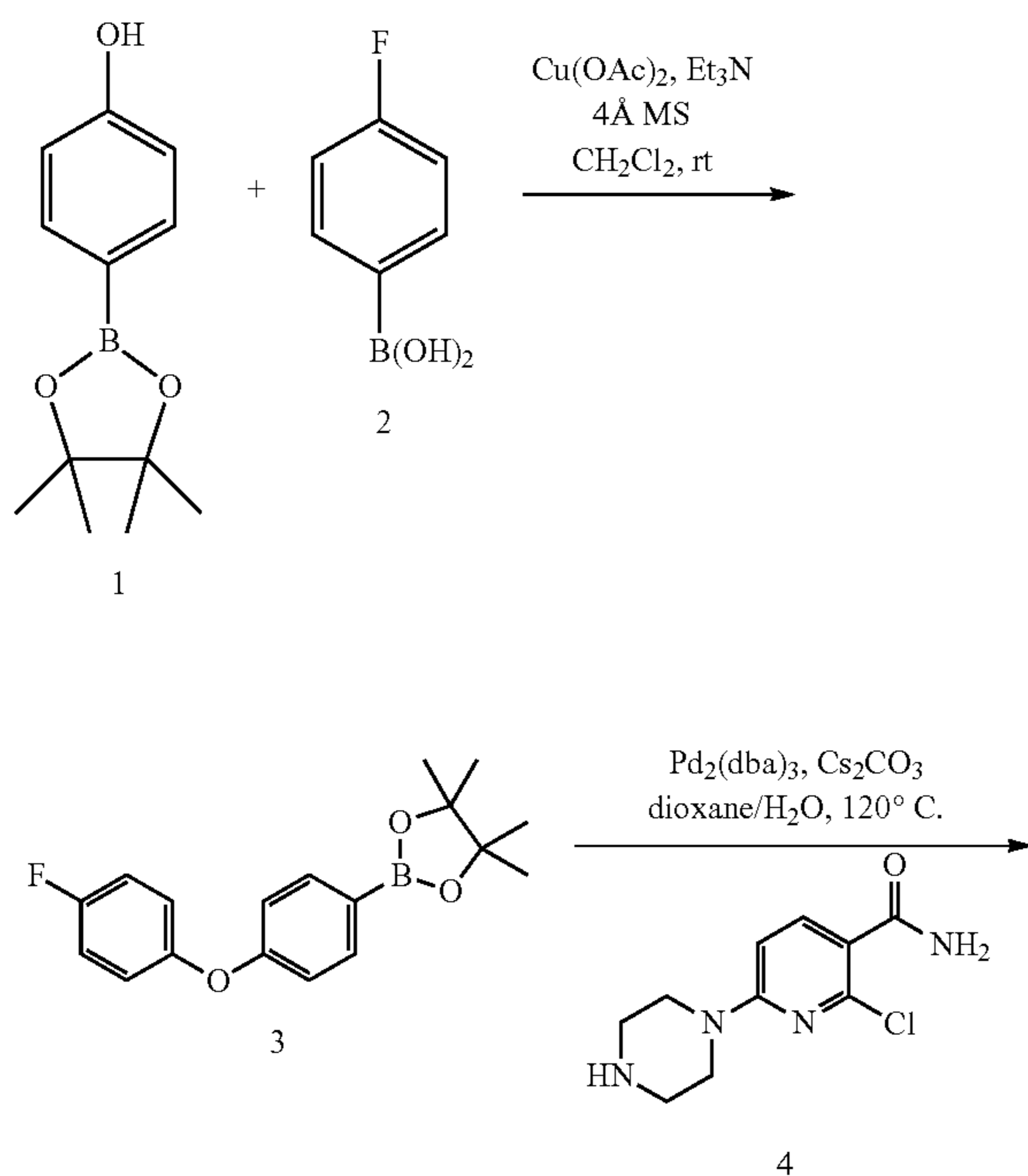
Scheme 27
