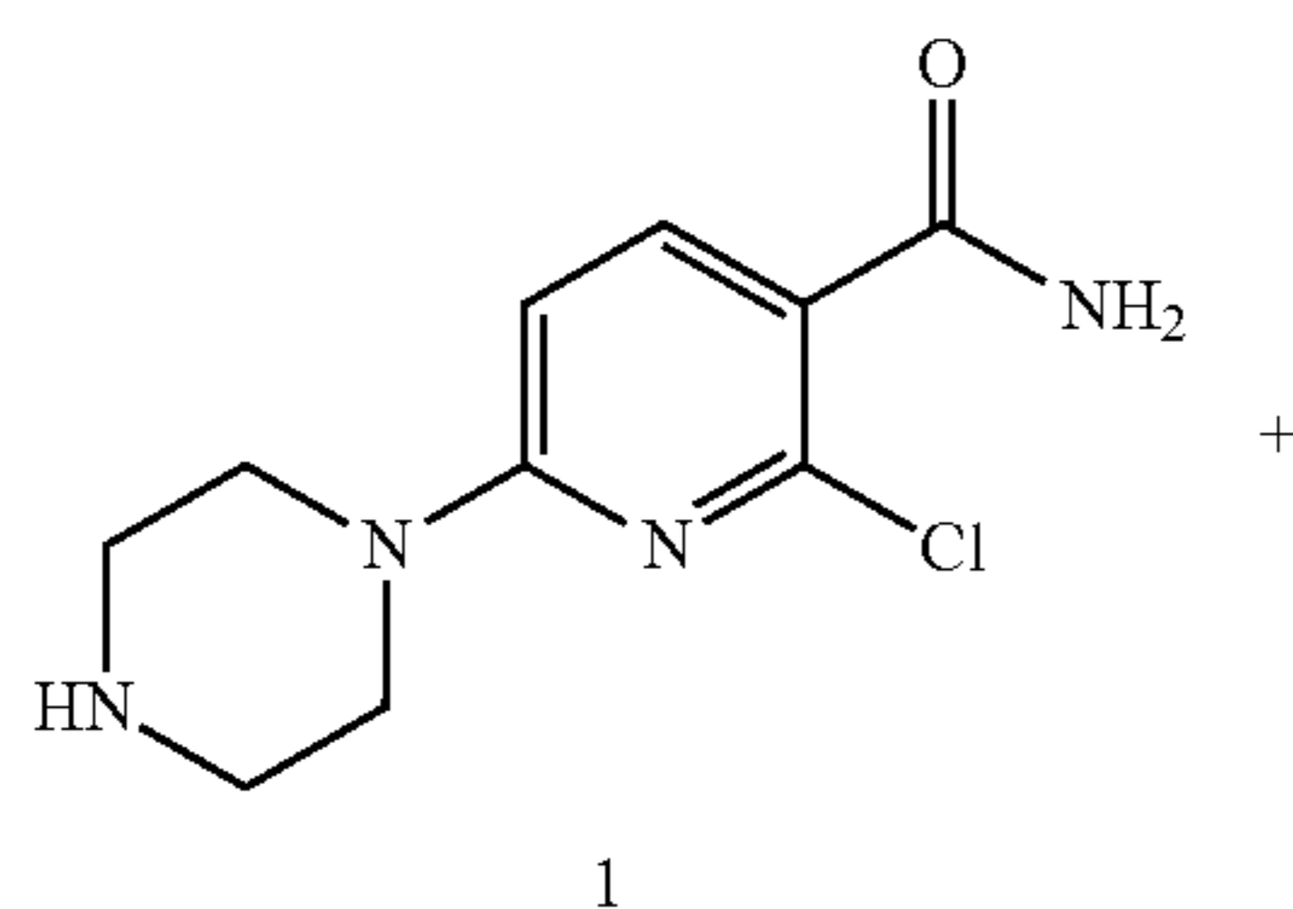
Scheme 18
