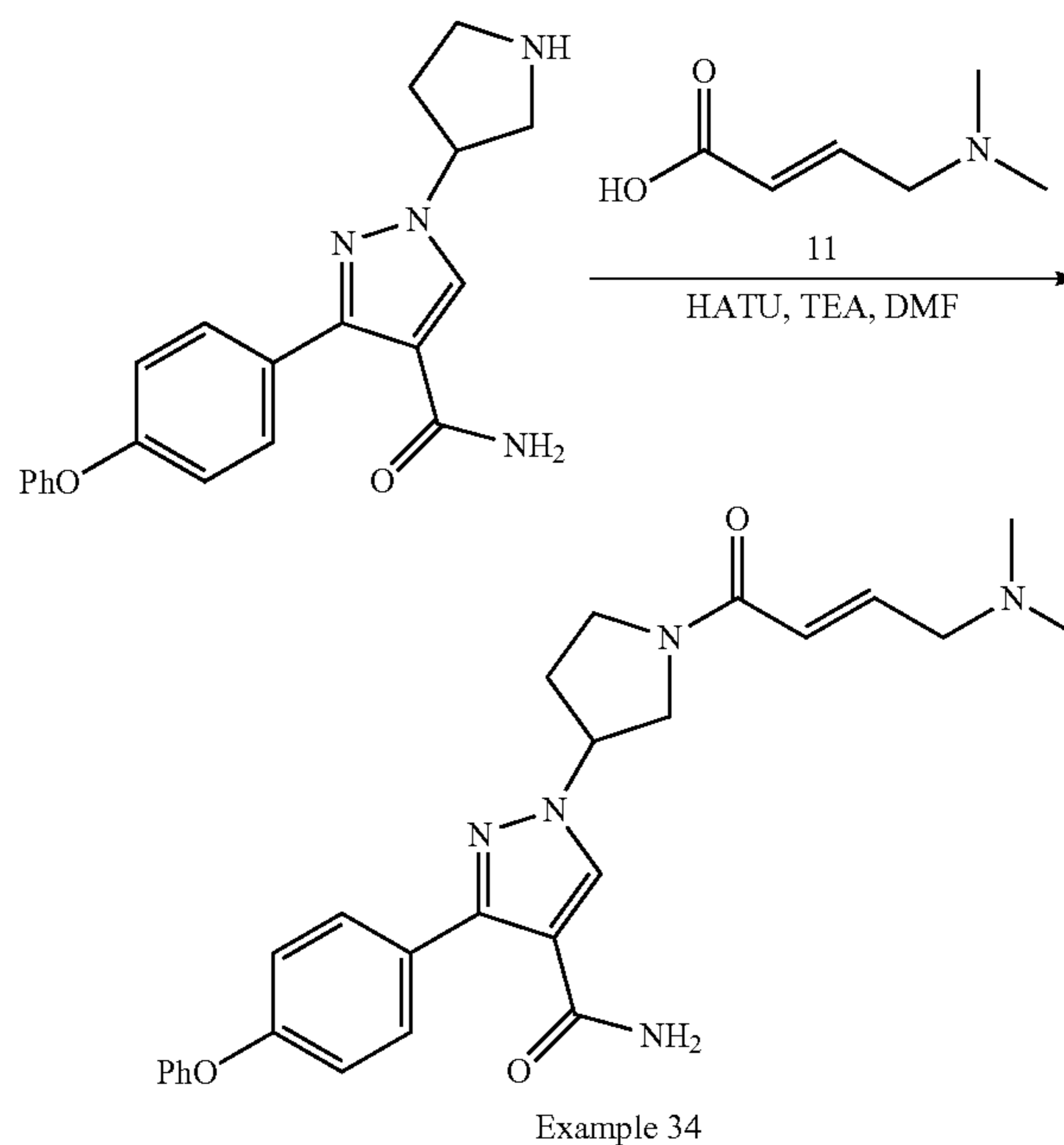
Scheme 24
