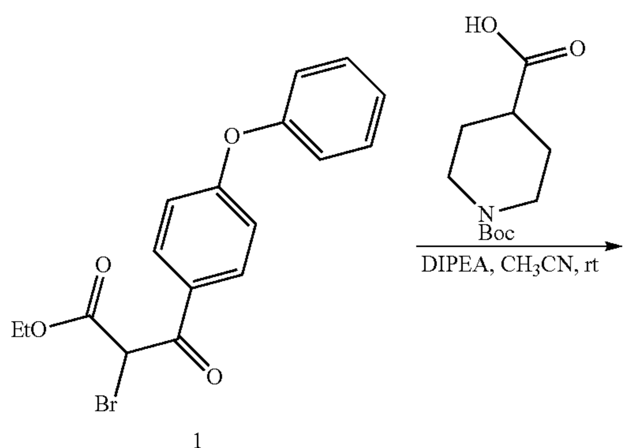
Scheme 36
