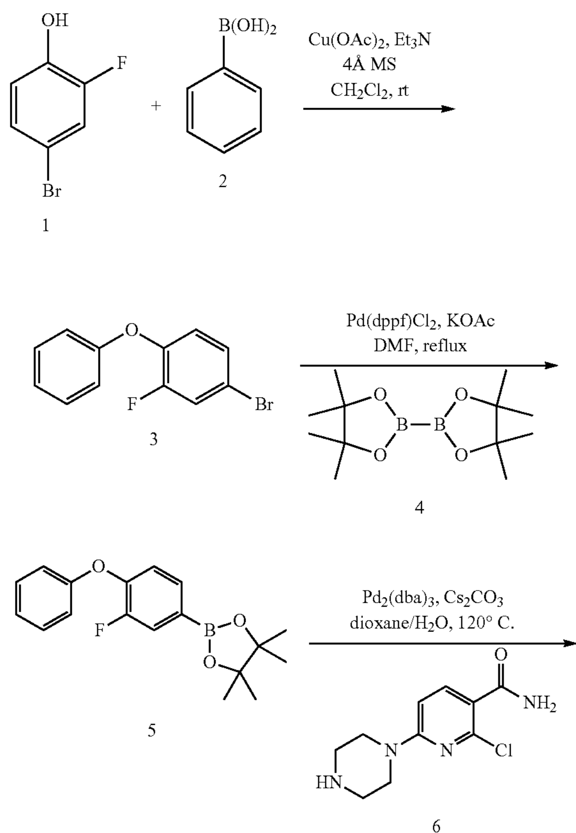
Scheme 26
