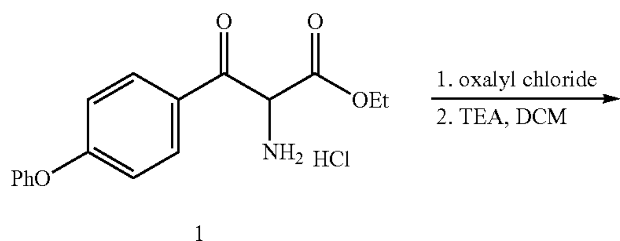
Scheme 34
