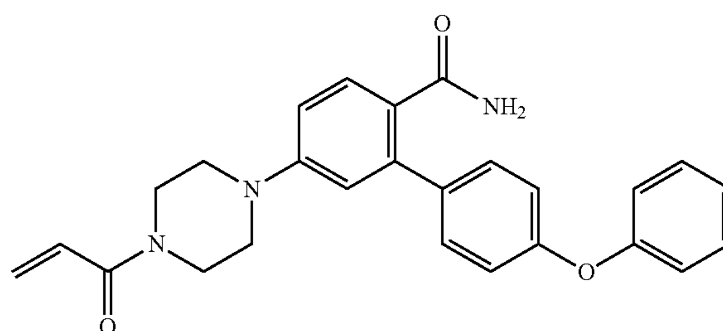
5-(4-acryloylpiperazin-1-yl)-4'-phenoxybiphenyl-2-carboxamide.
