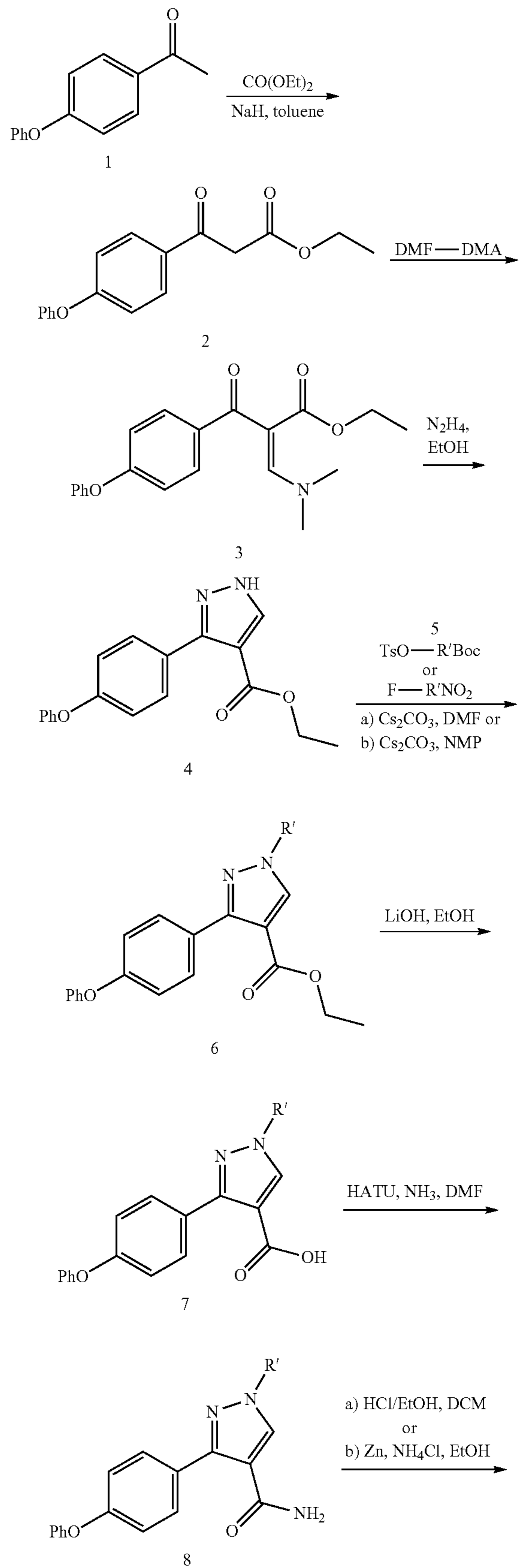
Scheme 23
