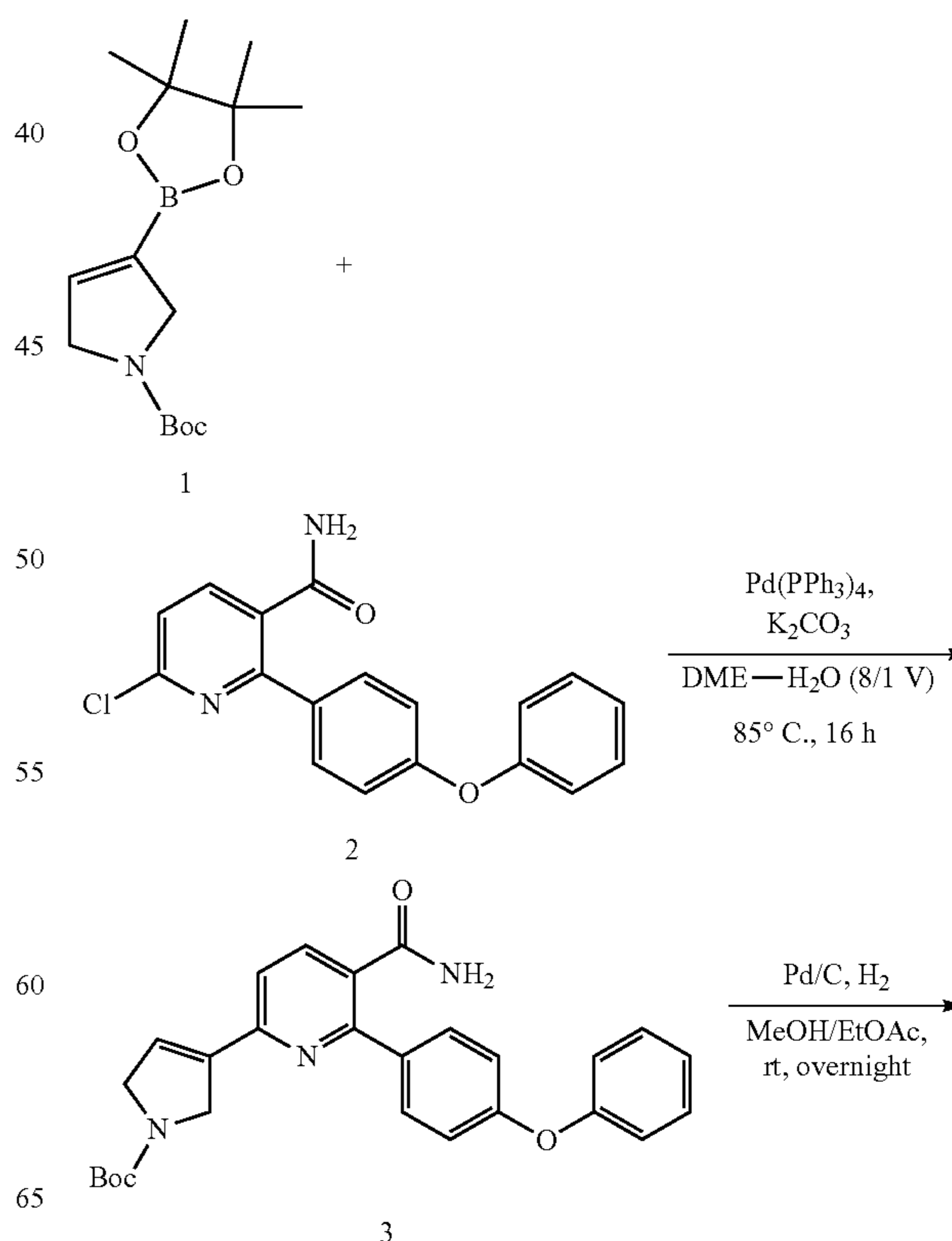
Scheme 12
