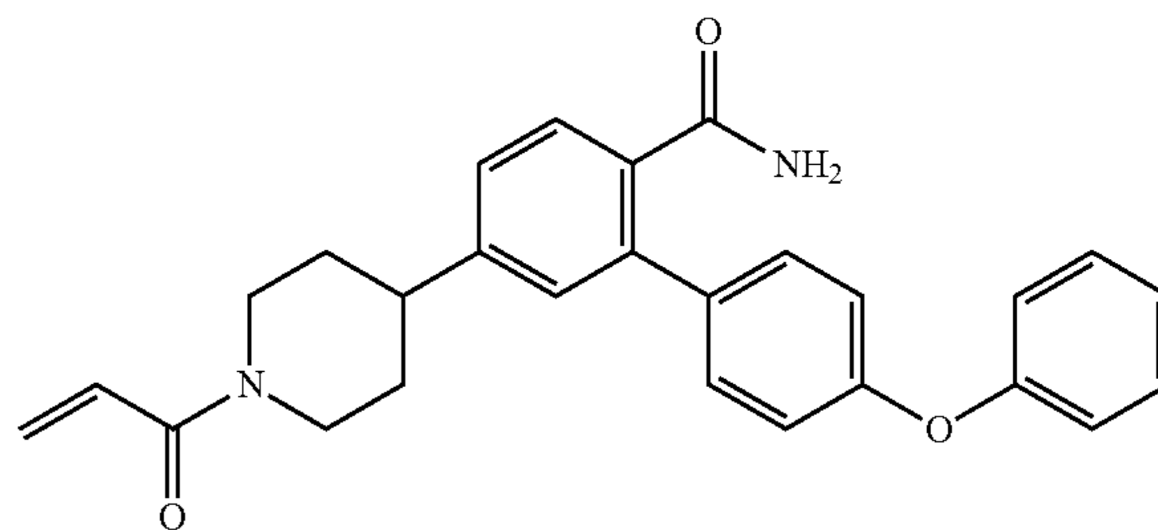
5-(1-acryloylpiperidin-4-yl)-4'-phenoxybiphenyl-2-carboxamide
