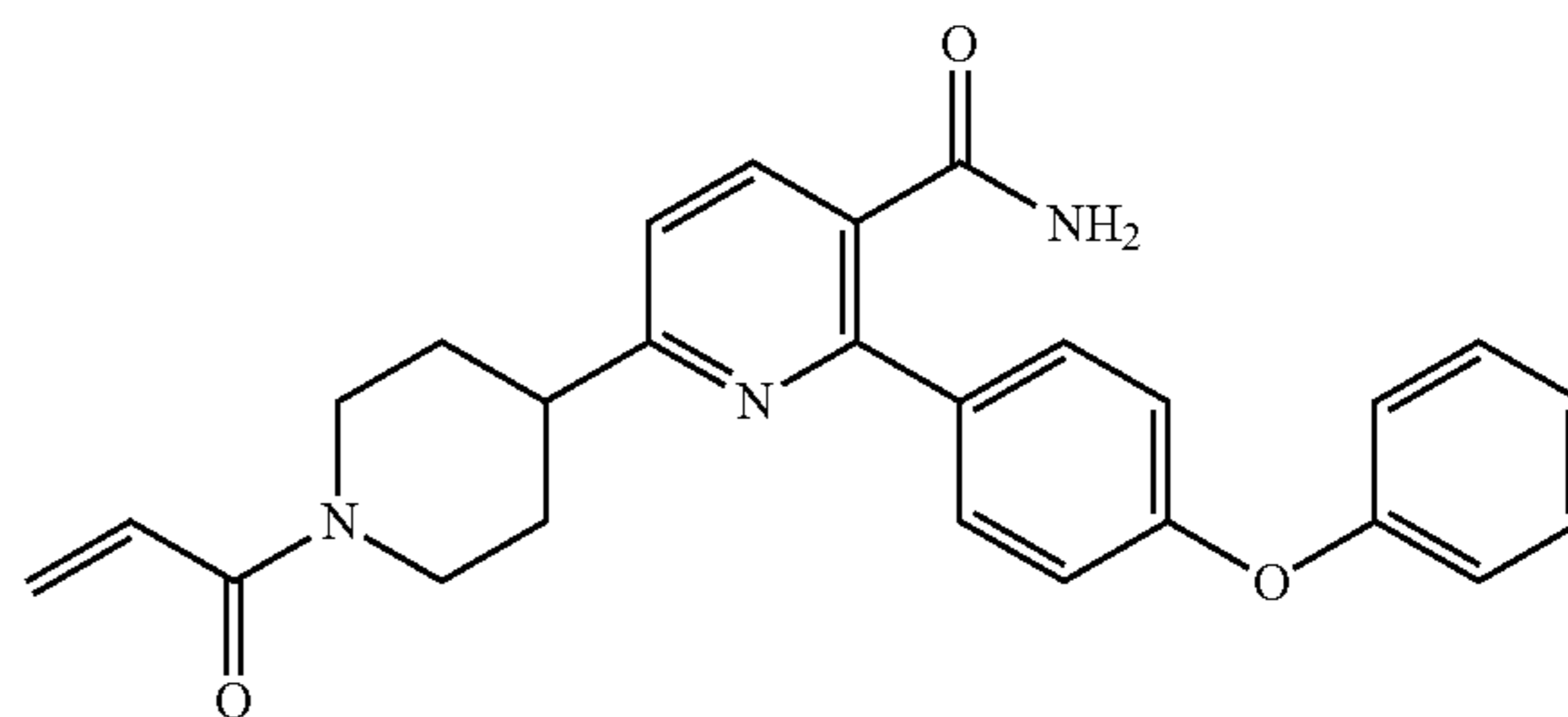
6-(1-acryloylpiperidin-4-yl)-2-(4-phenoxyphenyl)nicotinamide.
