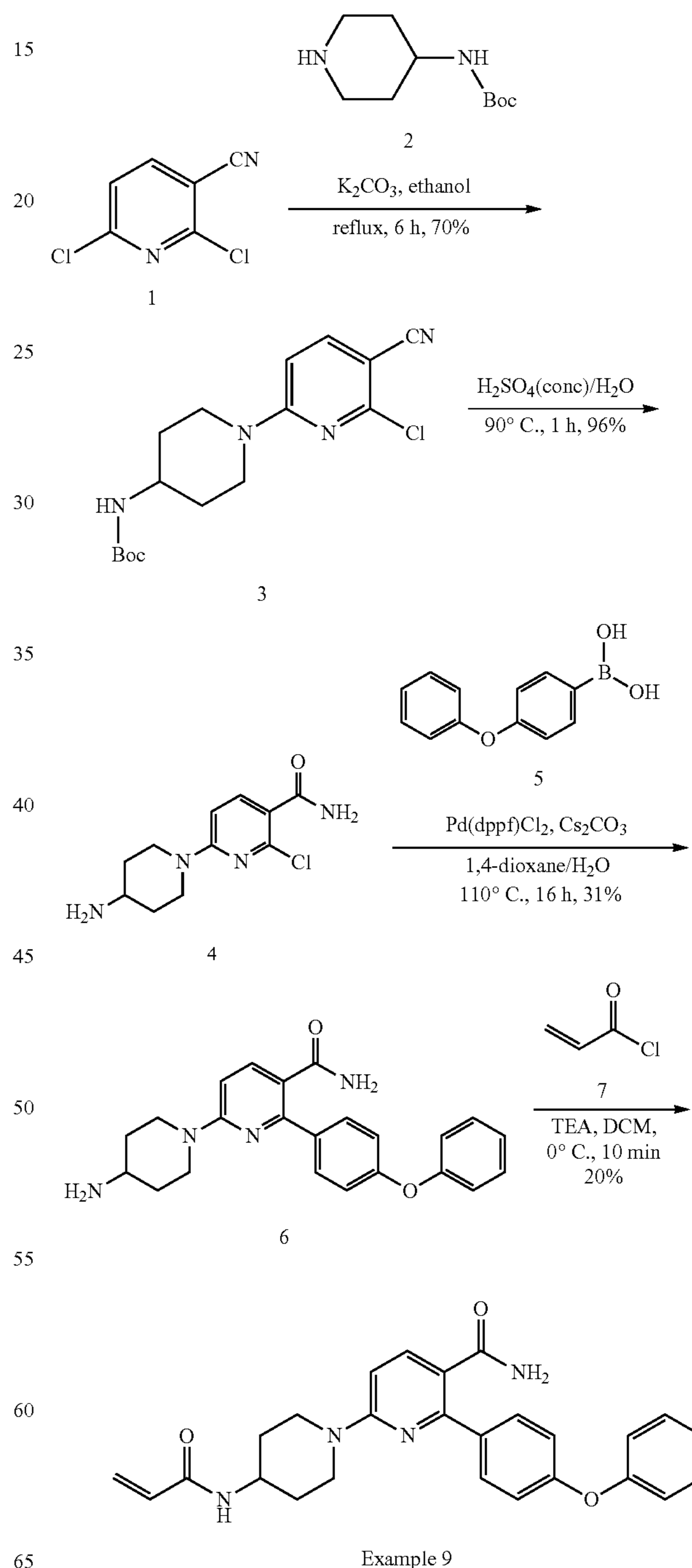
Scheme 7
