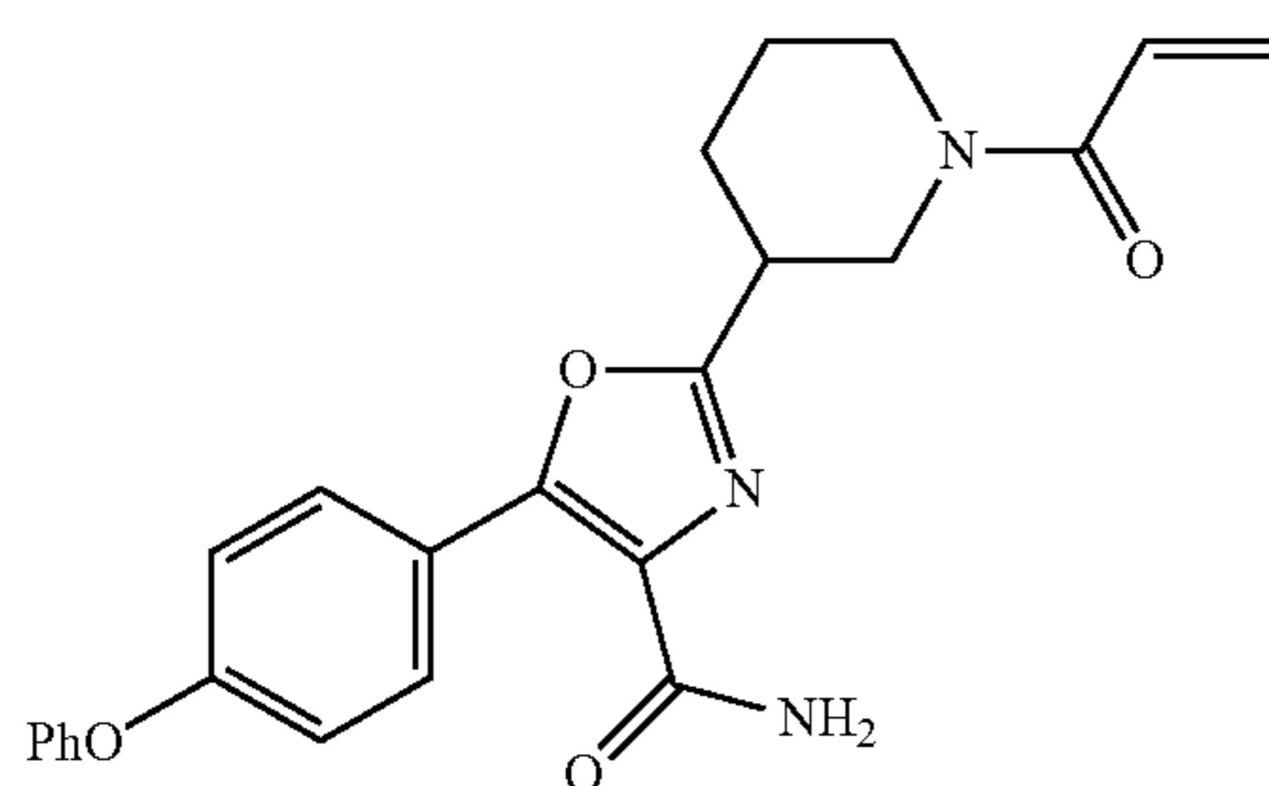
Example 54
