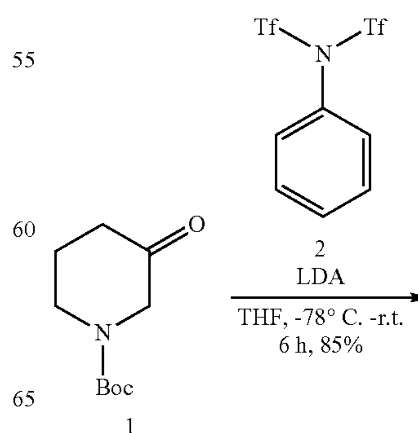
Scheme 6
