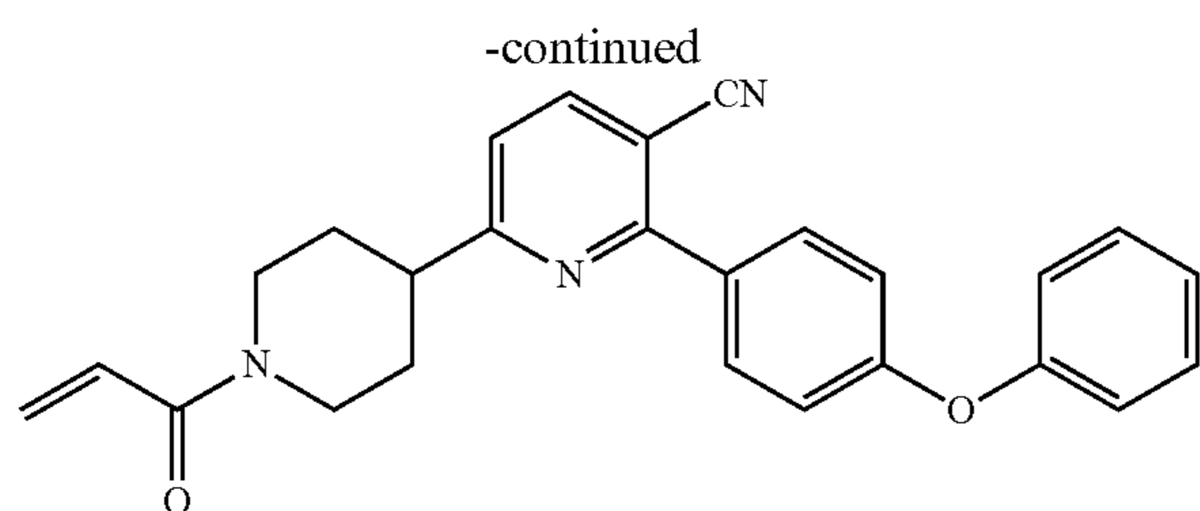
Example 24
