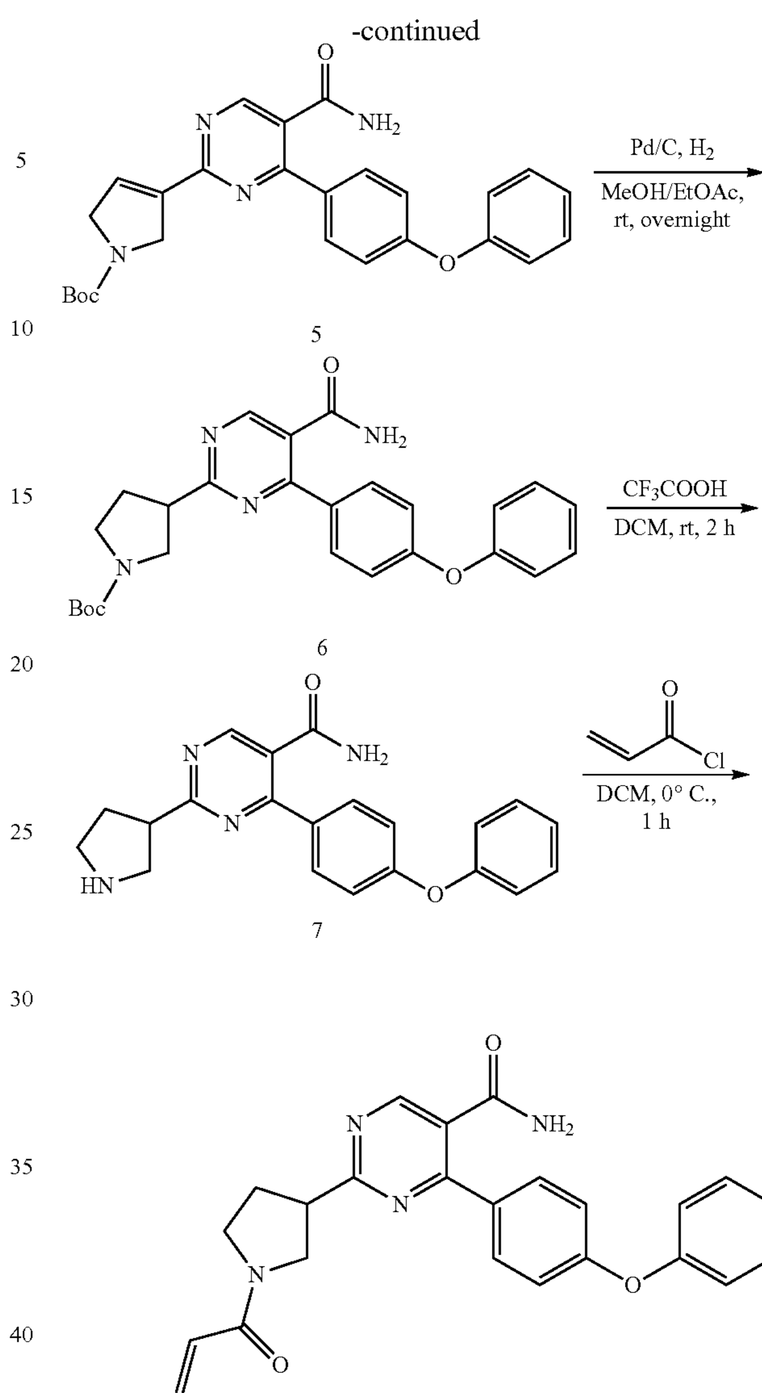
Example 22
