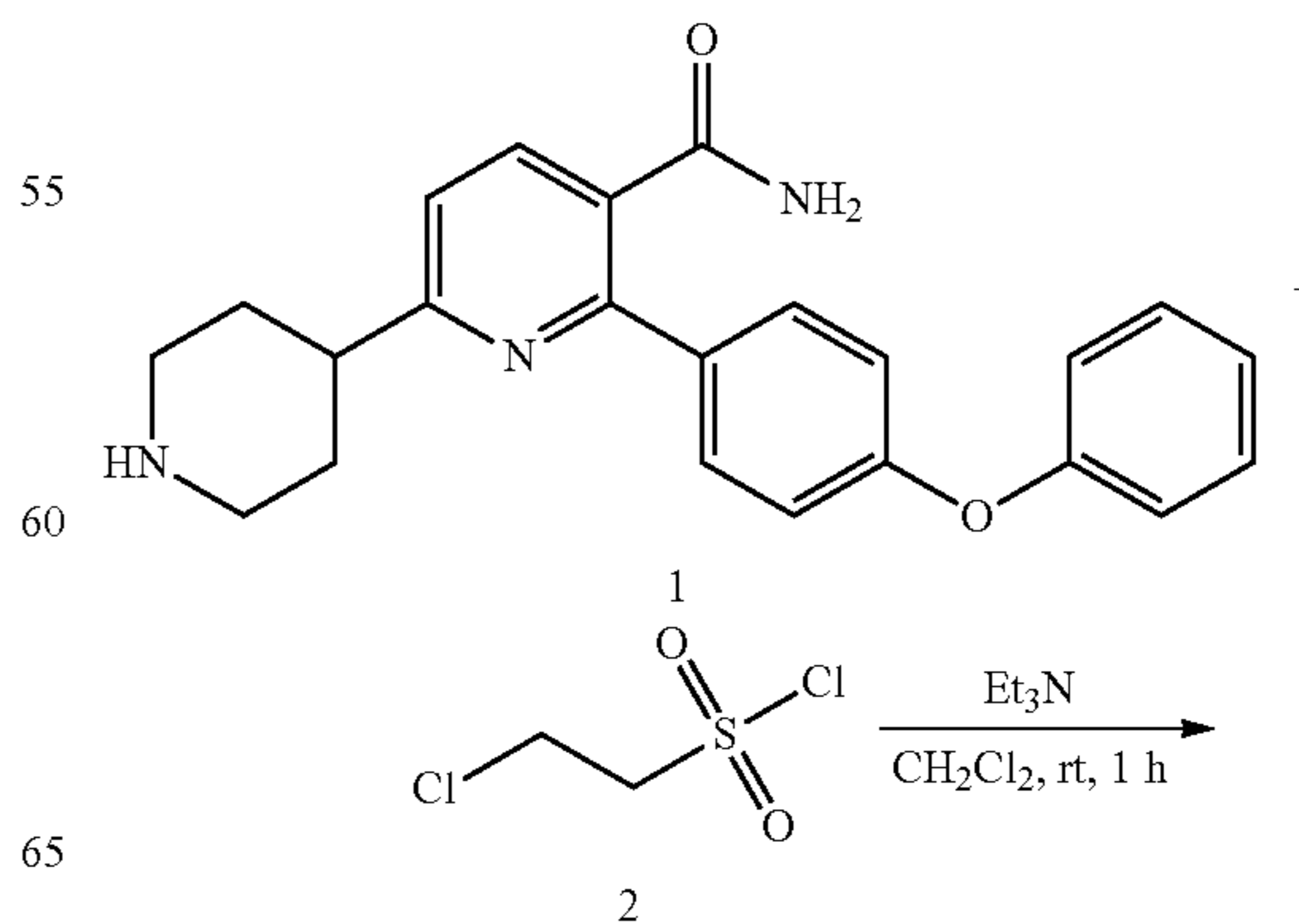
Scheme 53
