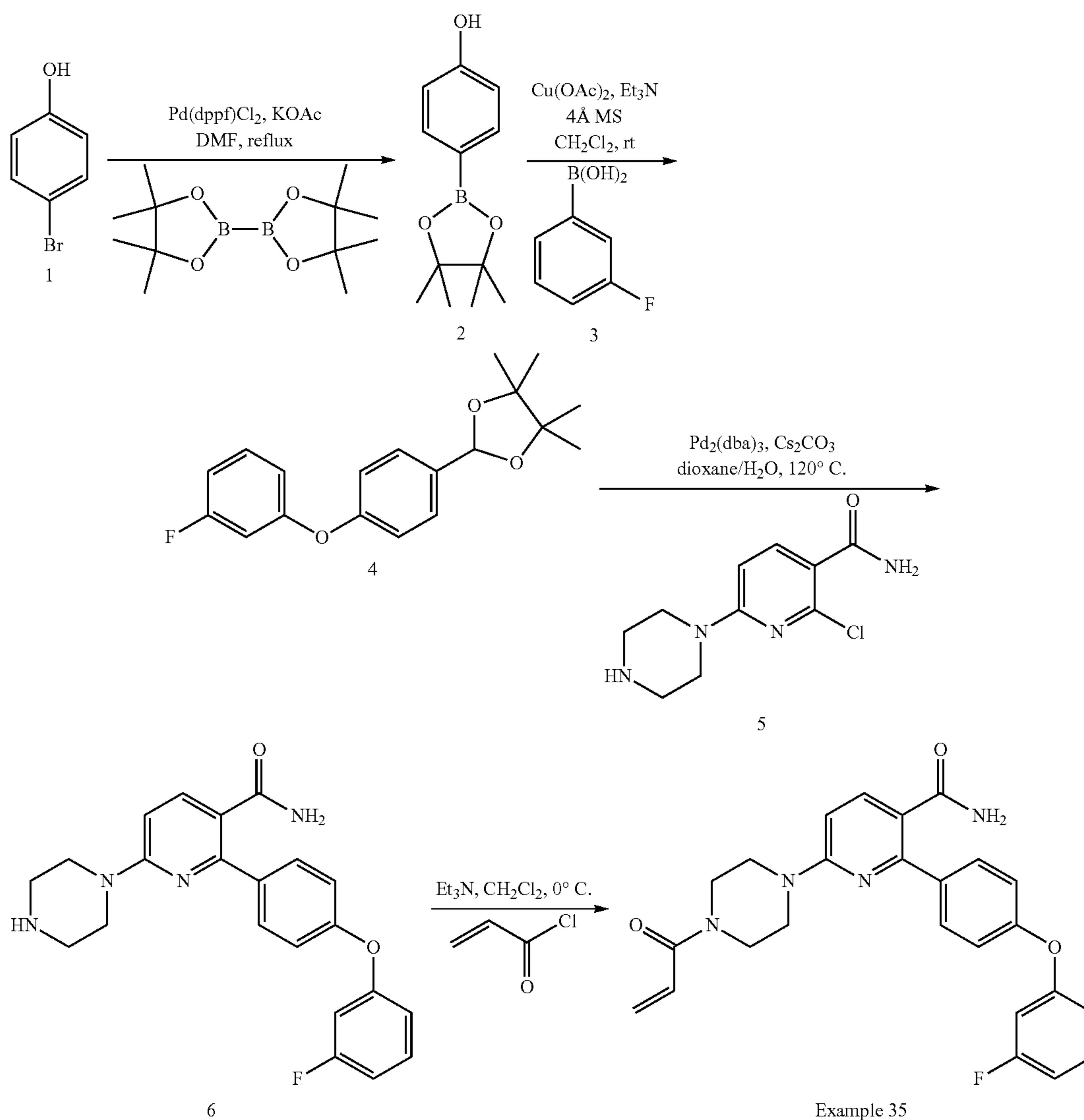
Scheme 25
