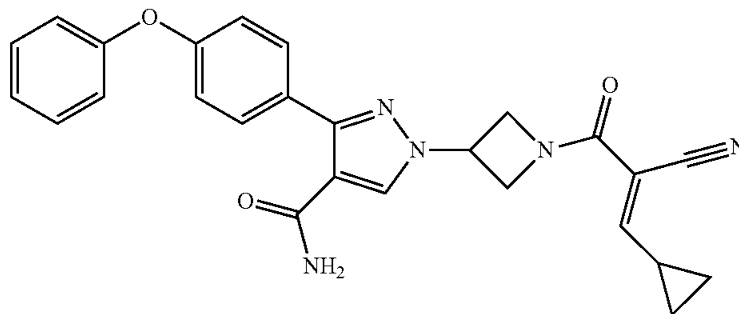
Example 53
