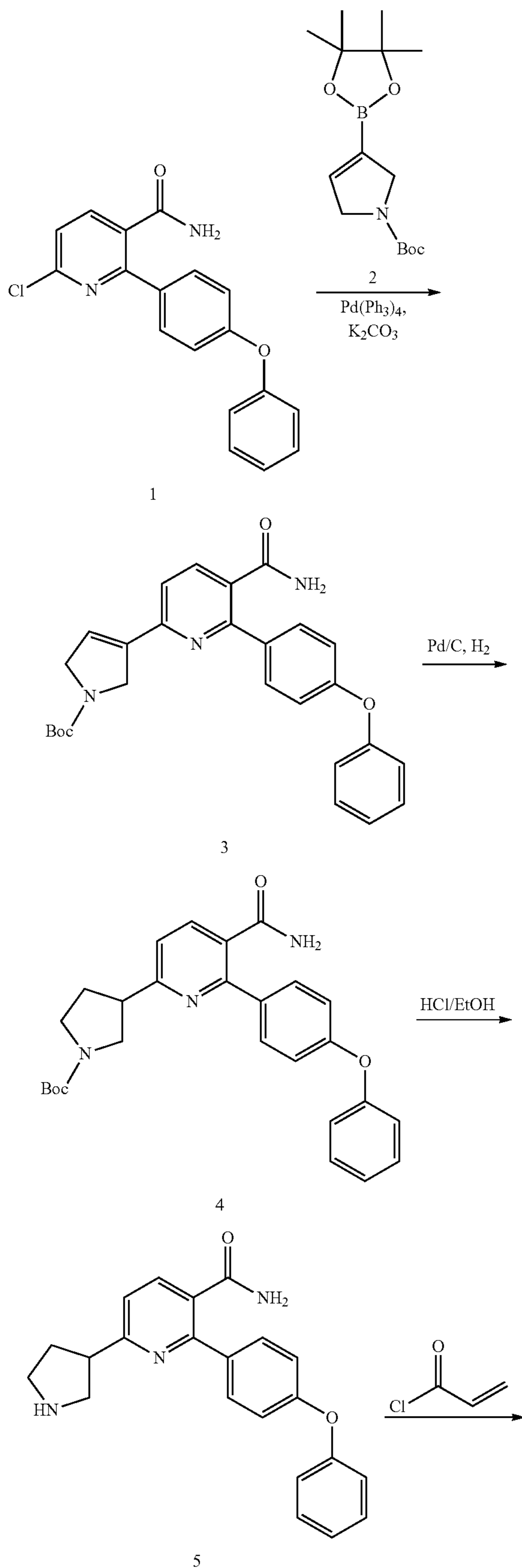
Scheme 4
