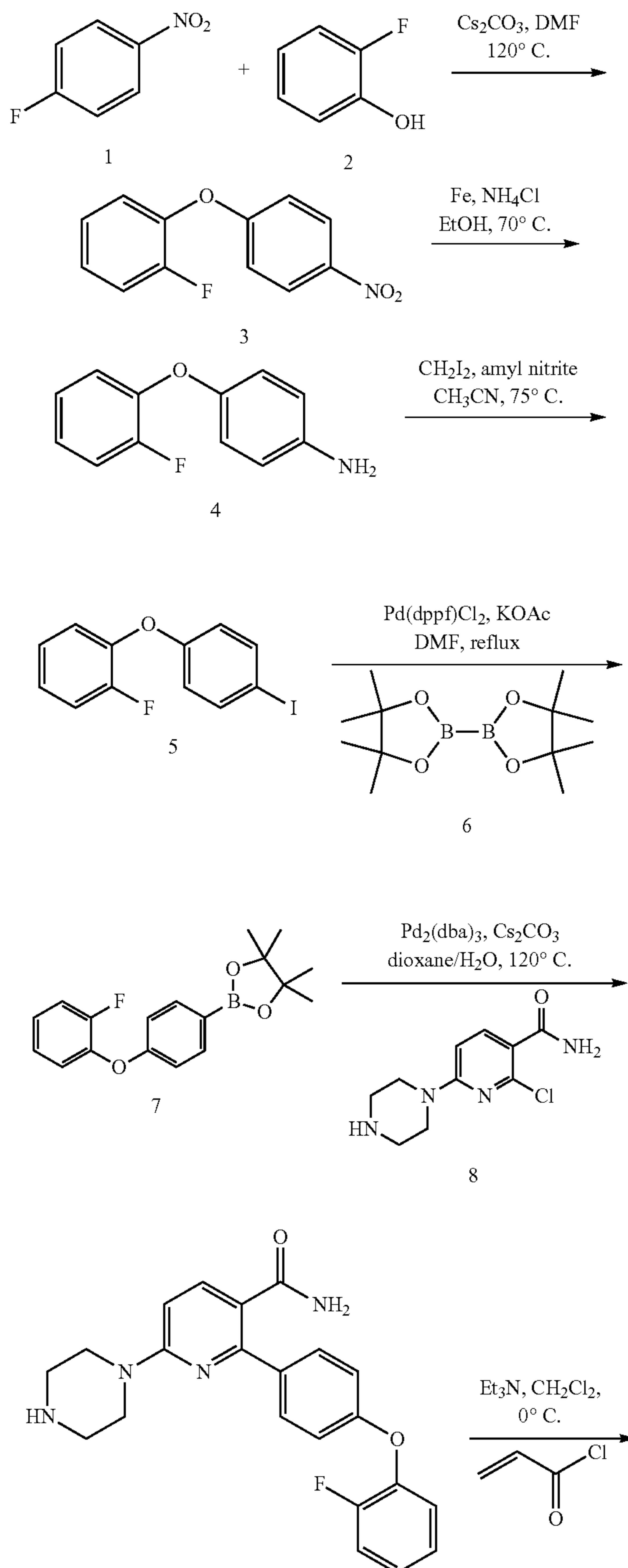
Scheme 28
