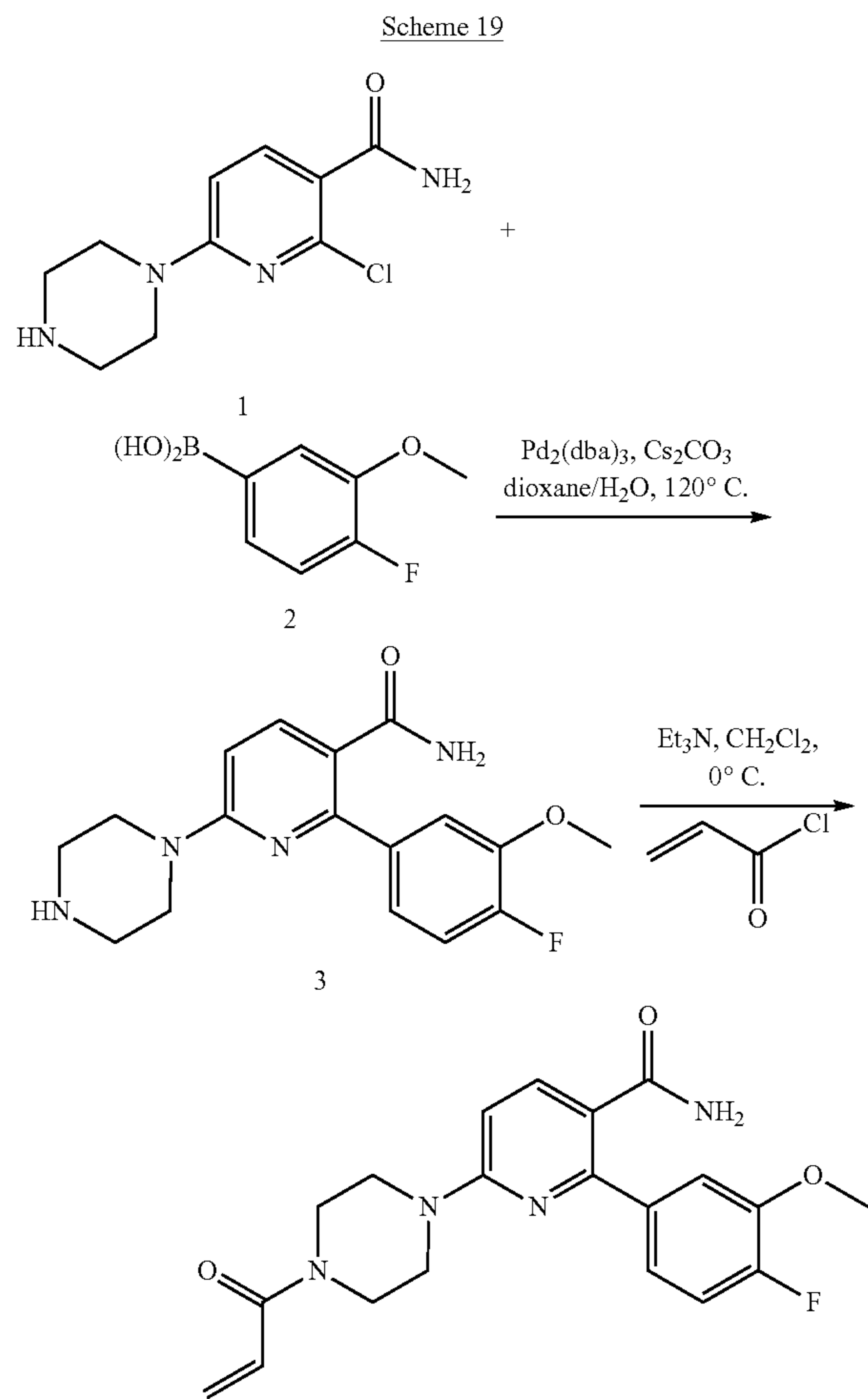
Example 30
