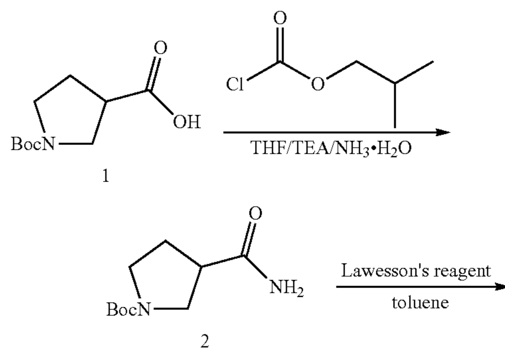
Scheme 31
