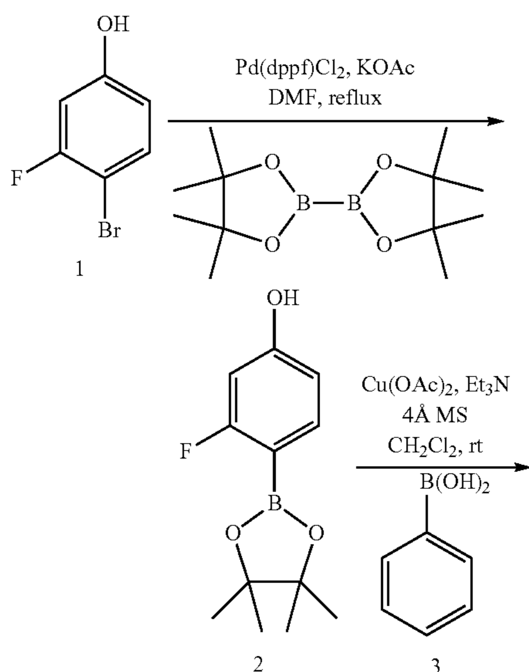
Scheme 29
