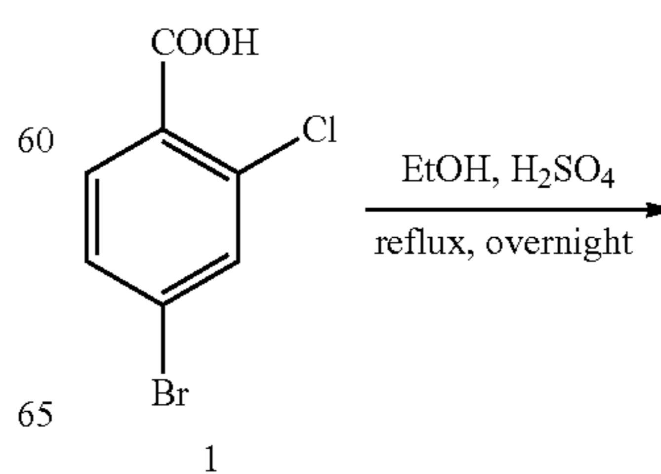
Scheme 45
