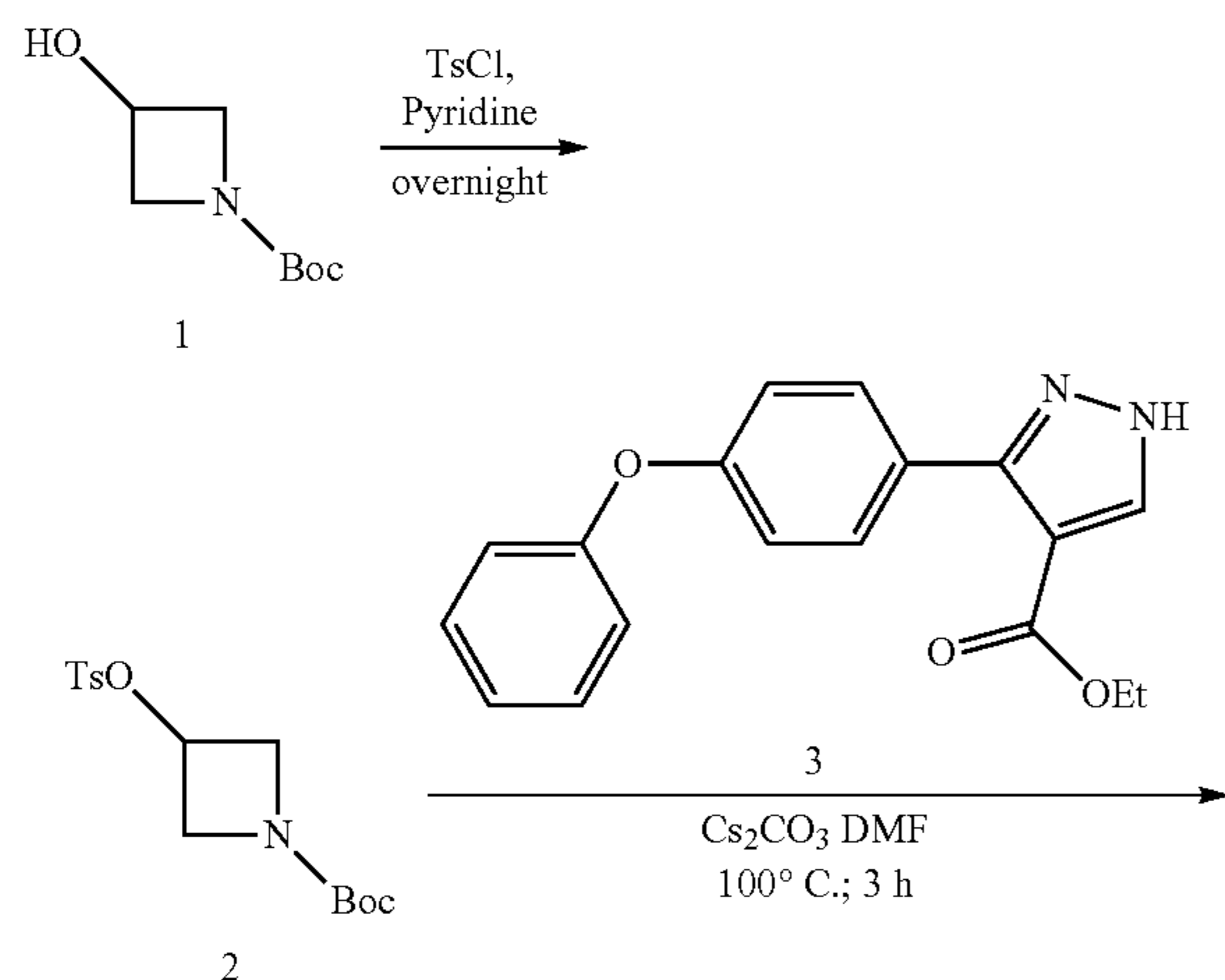
Scheme 9
