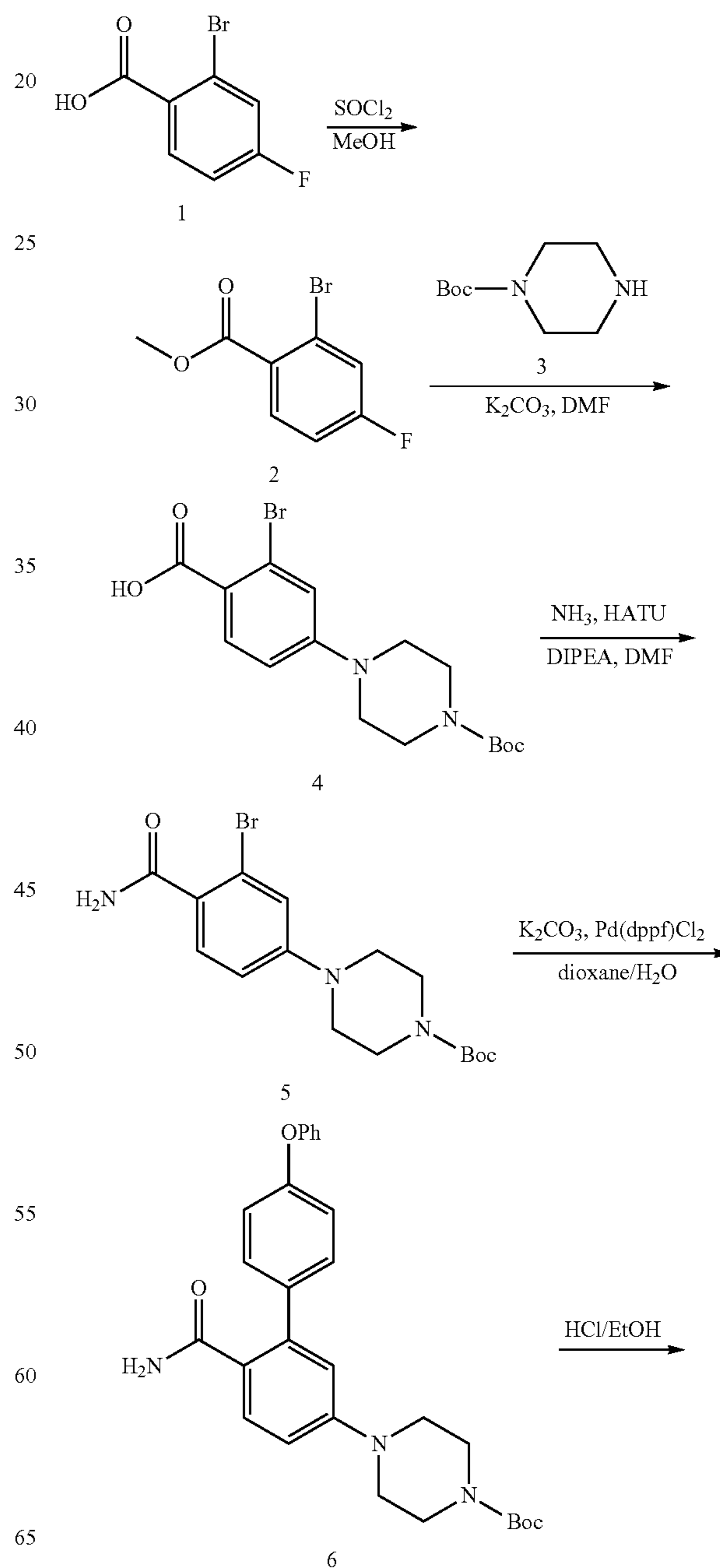
Scheme 47
