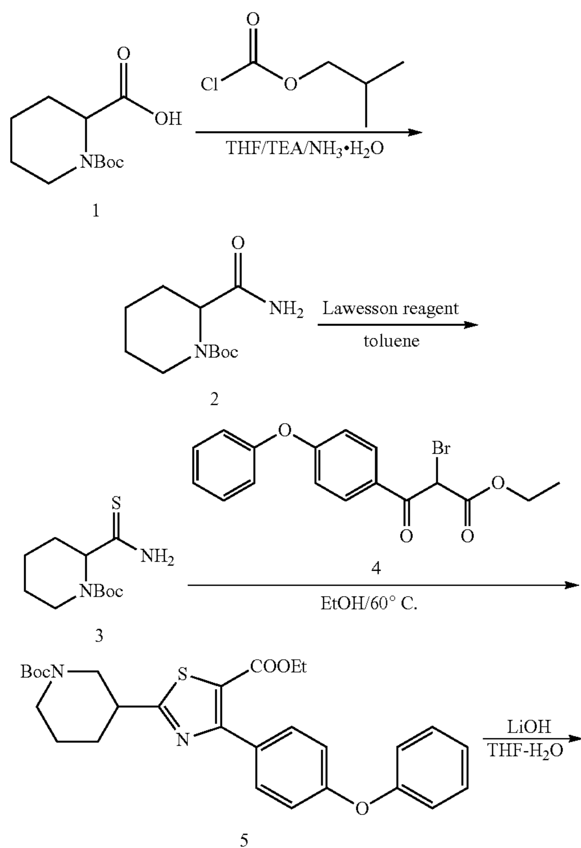
Scheme 30
