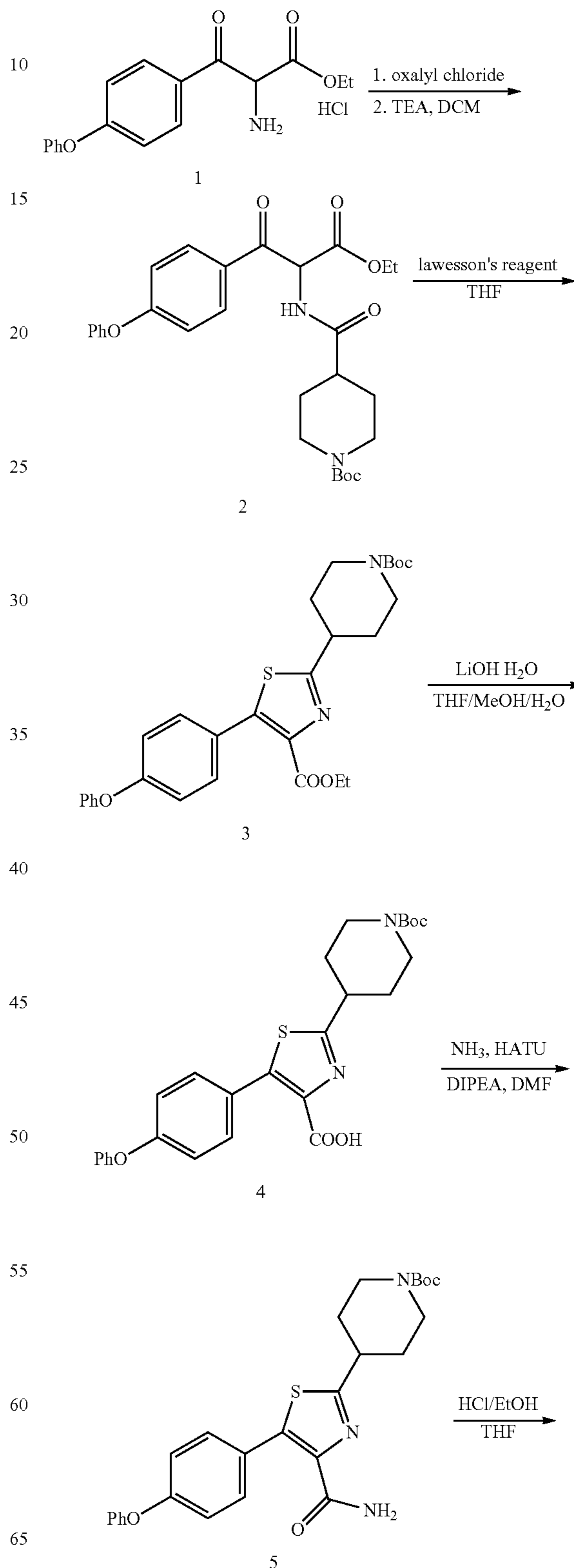
Scheme 39
