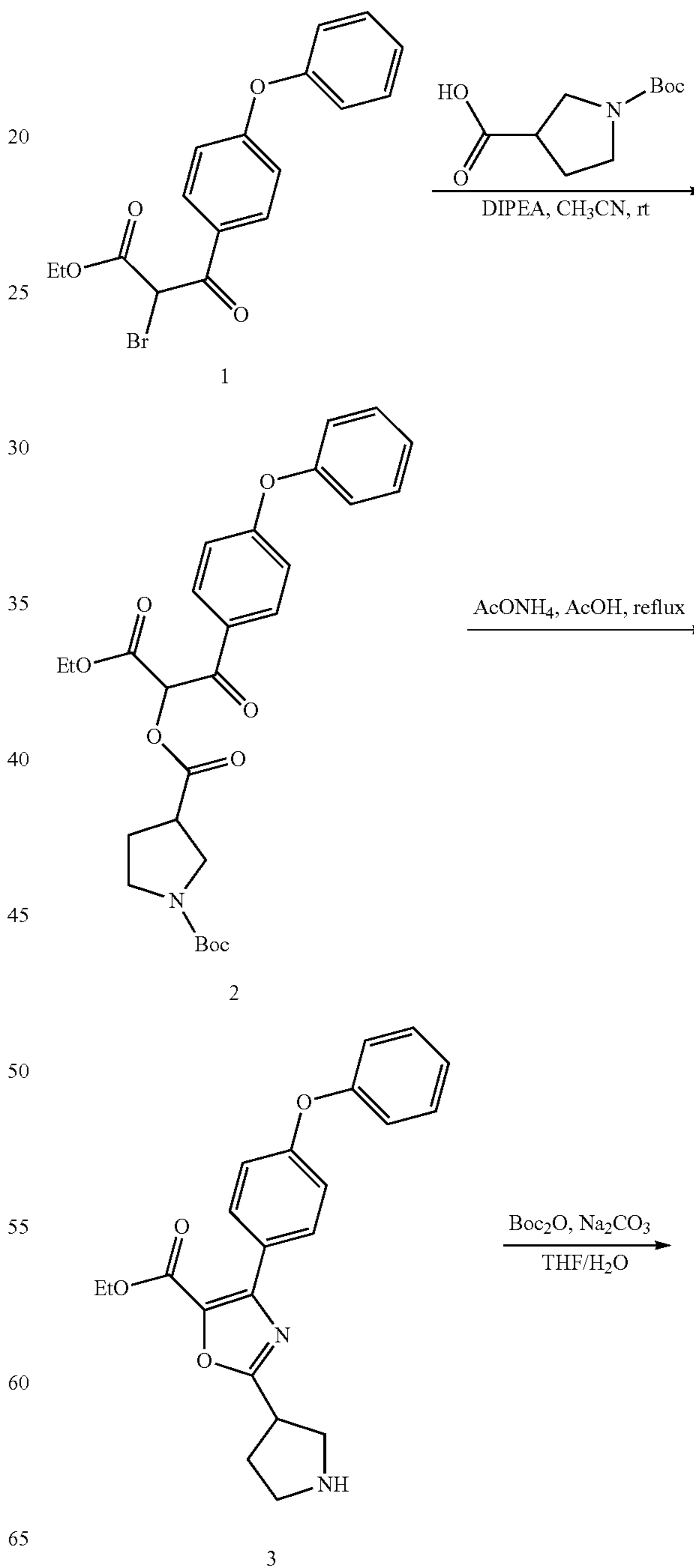
Scheme 33
