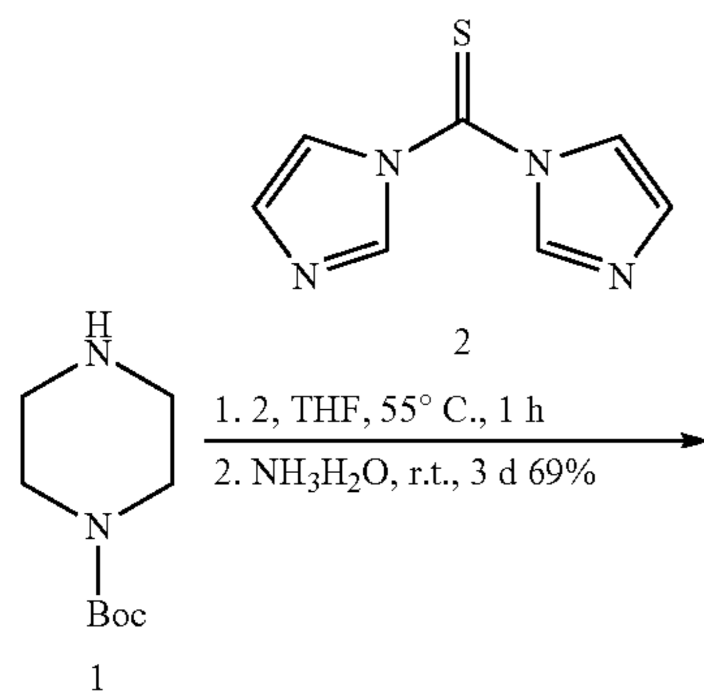
Scheme 41
