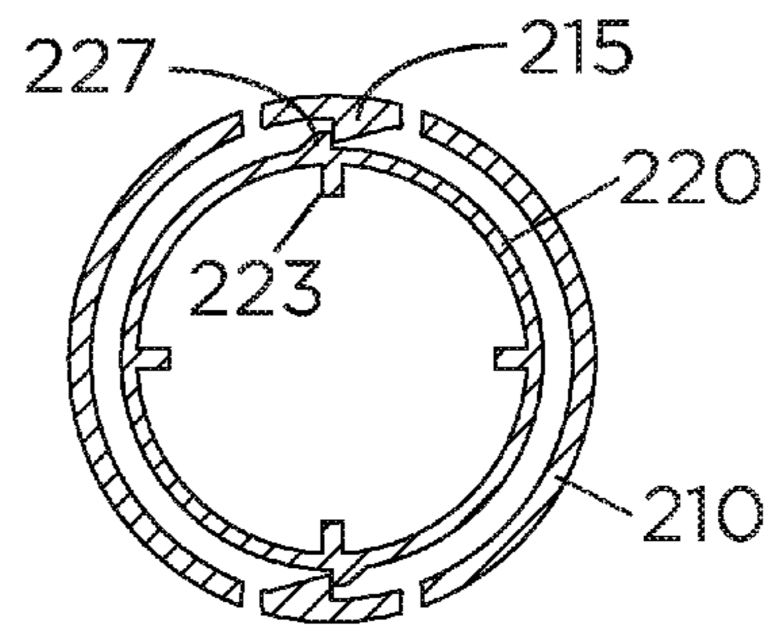
SECTION 13-13
