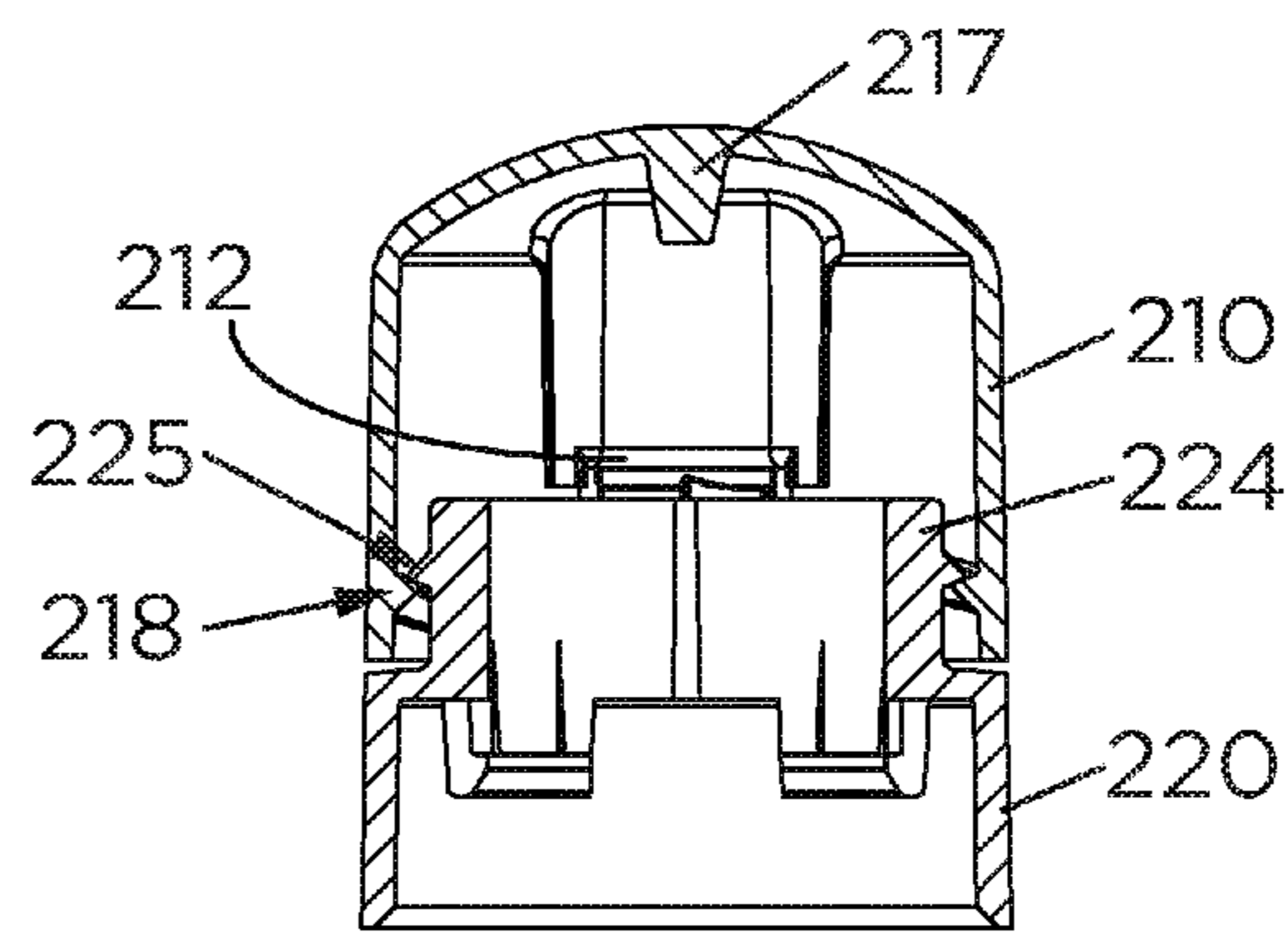
SECTION 11-11
