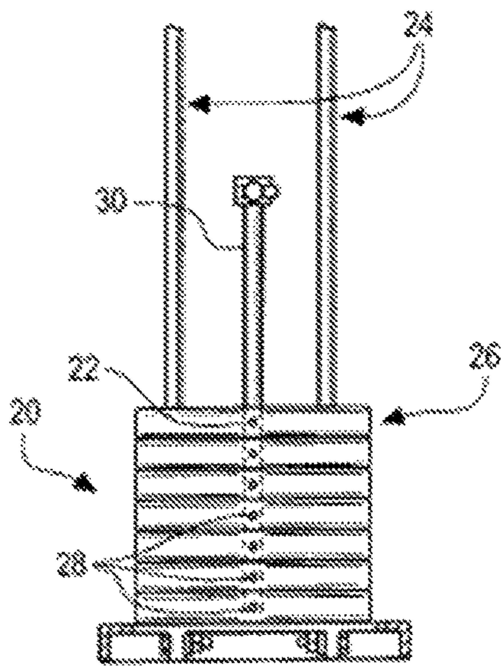
Fig. 2 PRIOR ART
