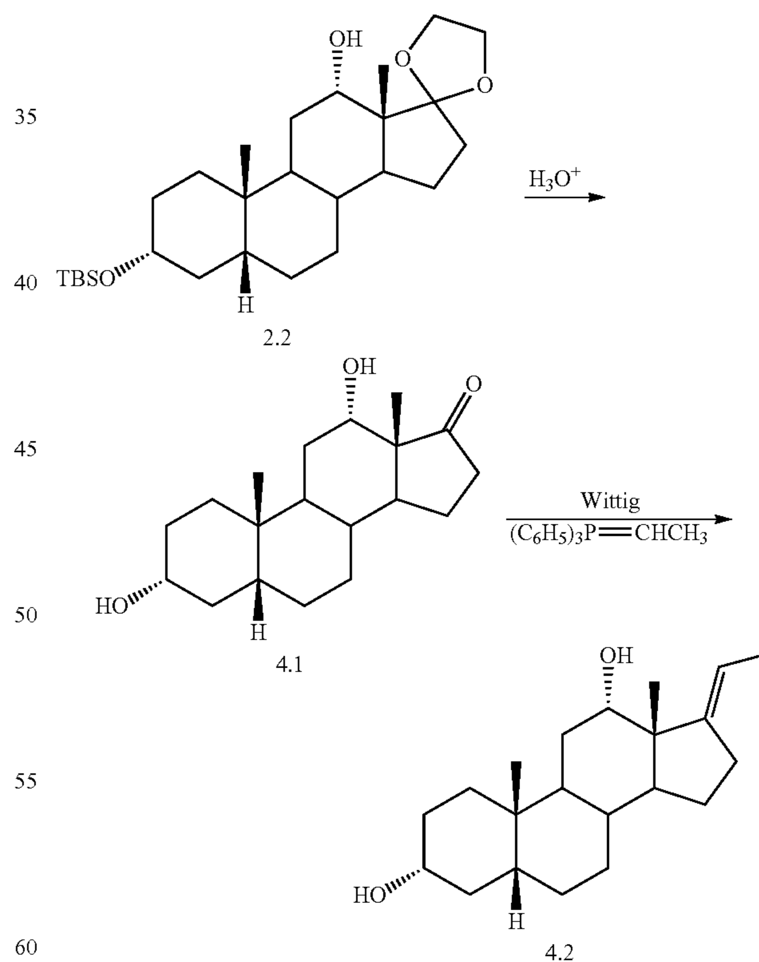
Scheme 4. Deprotection and Wittig Reaction
