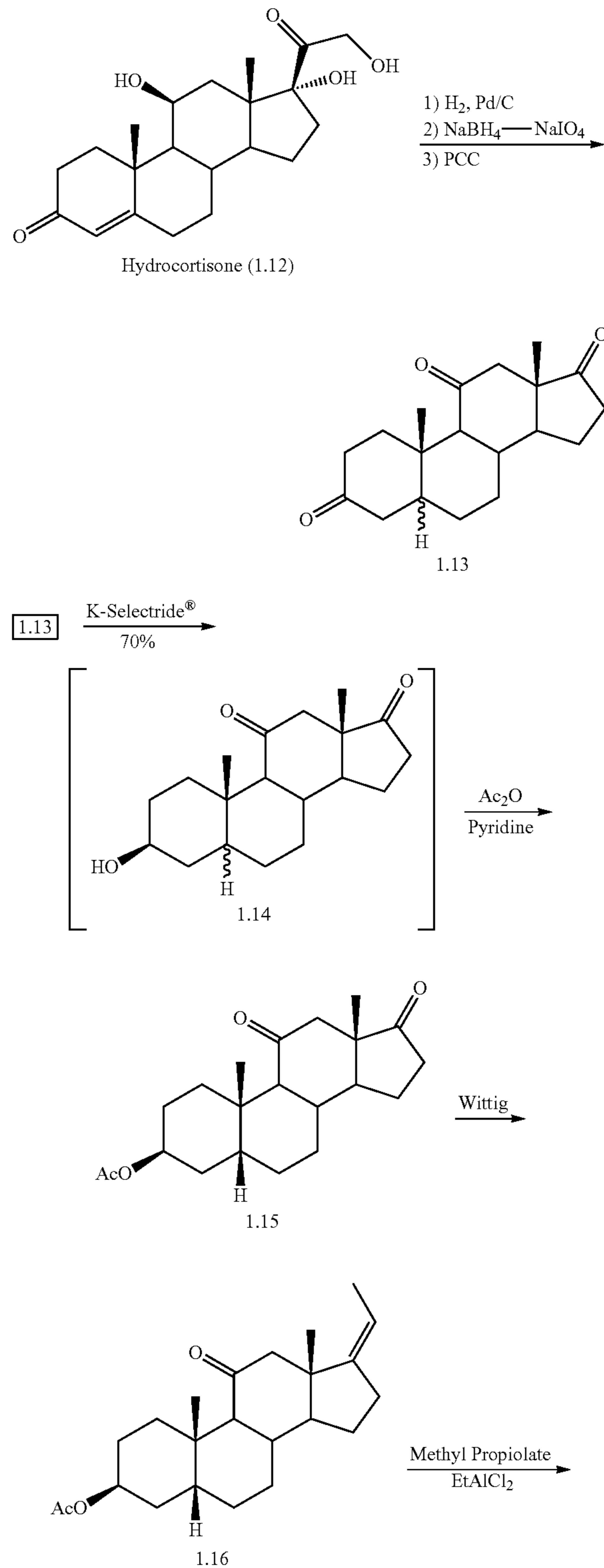
Scheme 1B. Synthesis of DCA from Hydrocortisone
