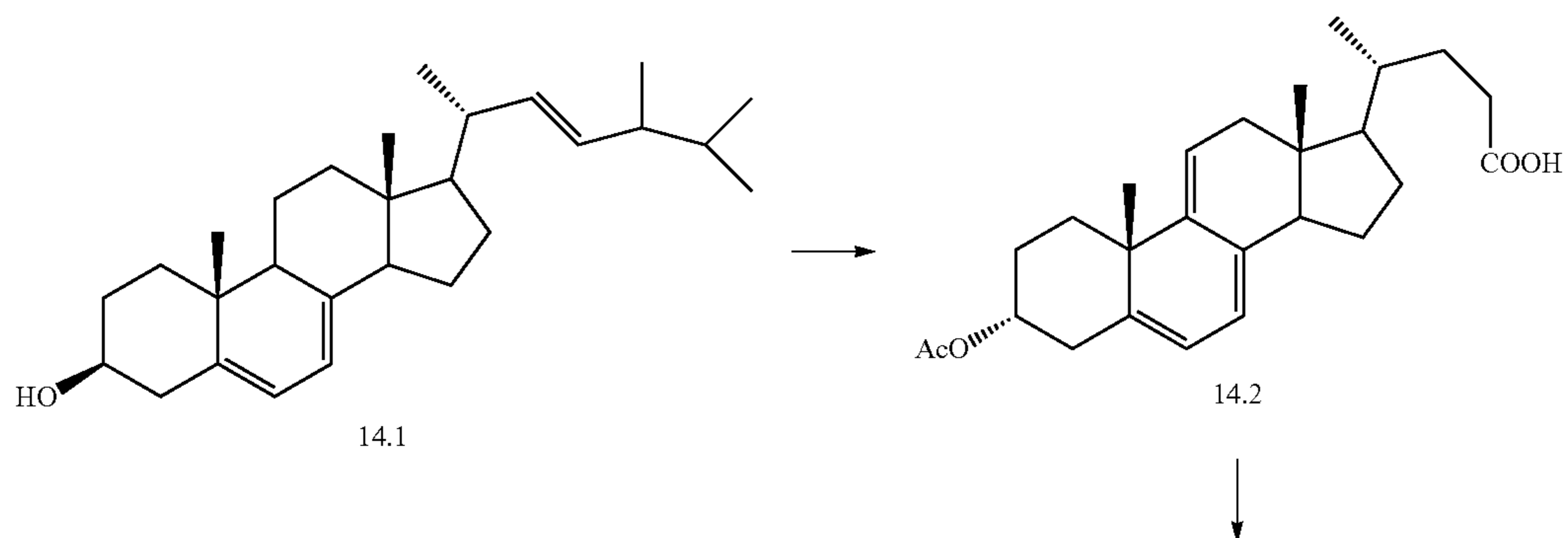
Scheme 14. Triene formation from Ergosterol
