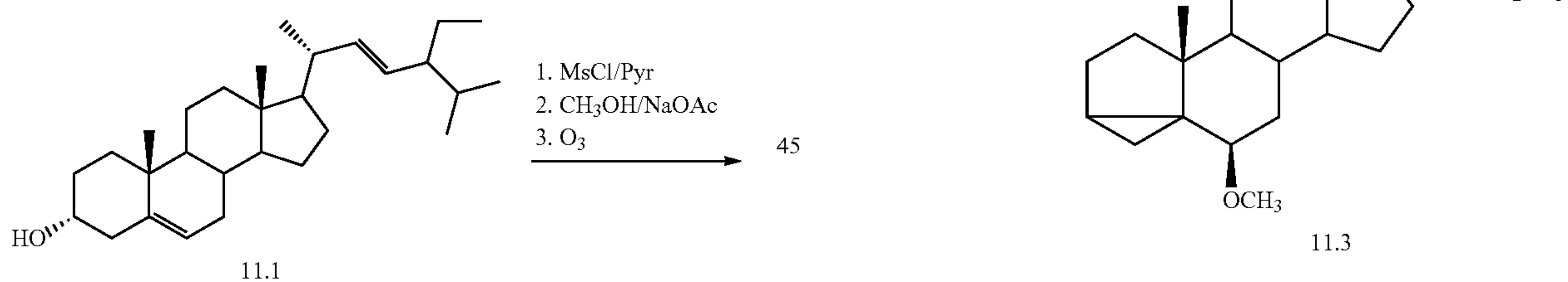
Scheme 11. Ozonolysis of i-steroid and side chain reduction
