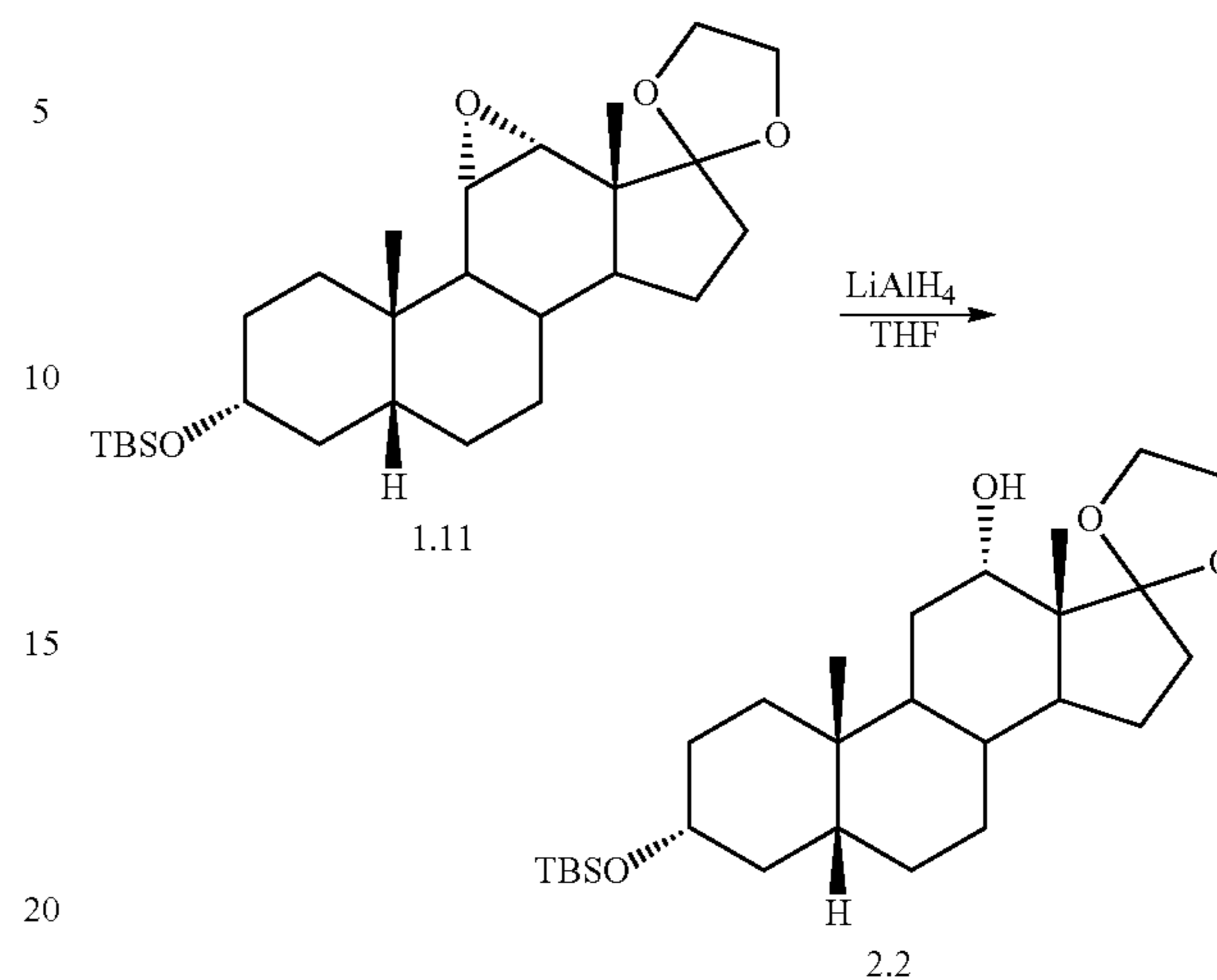
Scheme 3. Stereoselective Reduction of C 11 -C 12 epoxide.
