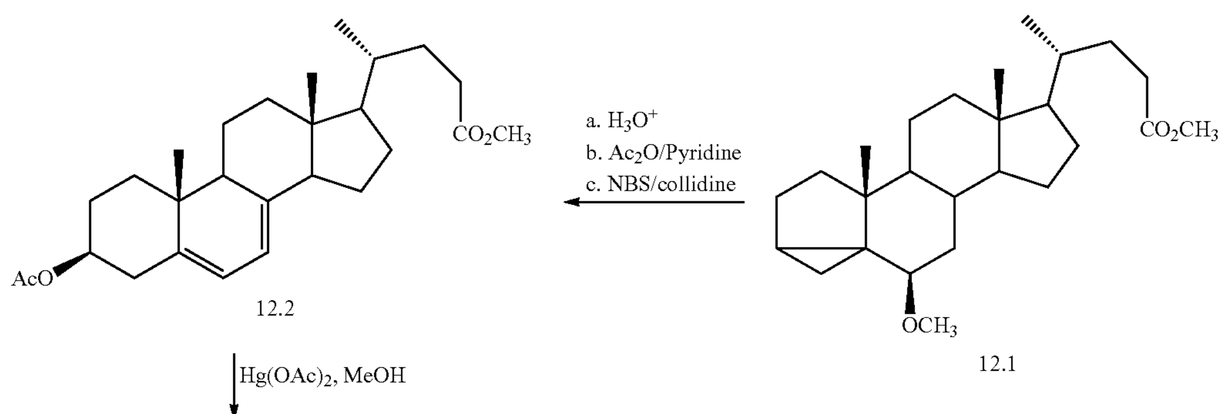
Scheme 12. Triene formation and allylic oxidation
