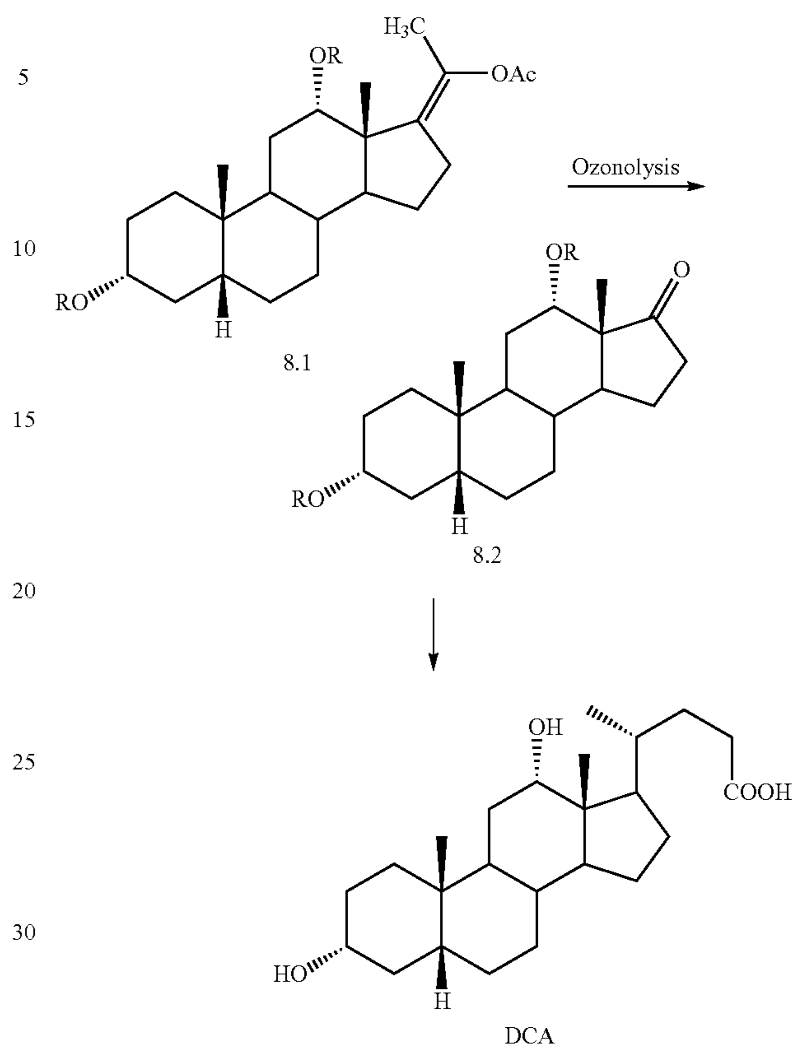
Scheme 8. Side-chain introduction
