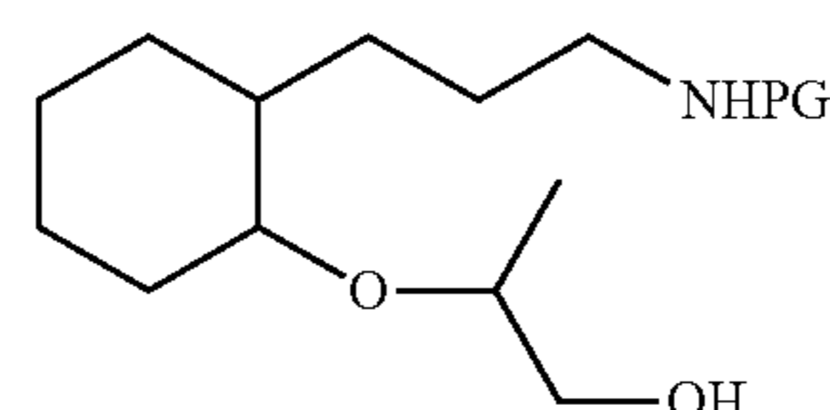
T102a [(2R,9R)-isomer] T102b [(2S,9S)-isomer]
