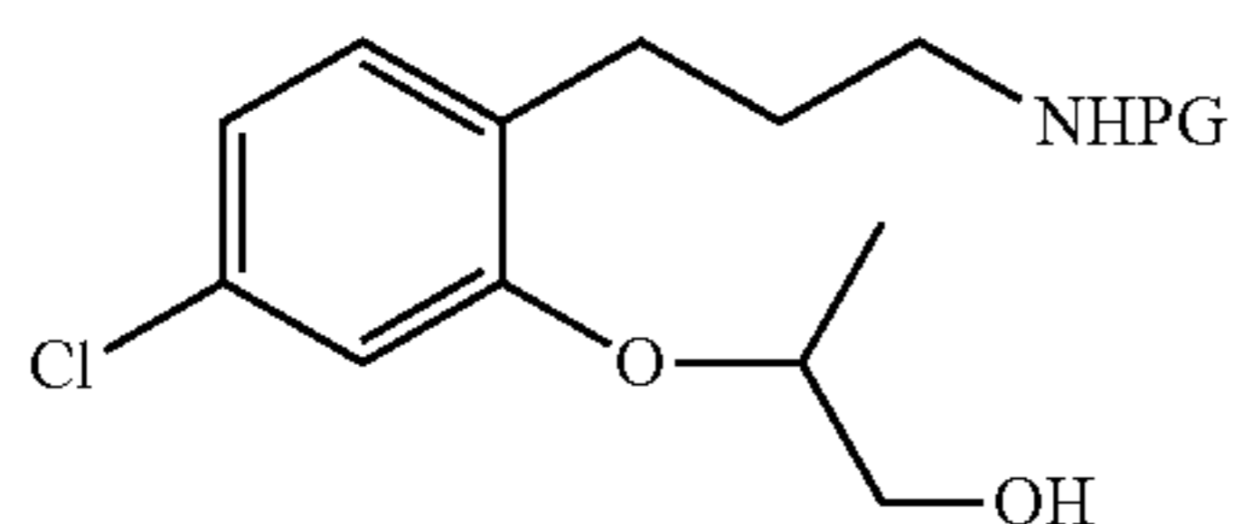
T111a [(R)-isomer] T111b [(S)-isomer]
