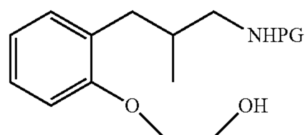
T40a [(R)-isomer] T40b [(S)-isomer]
