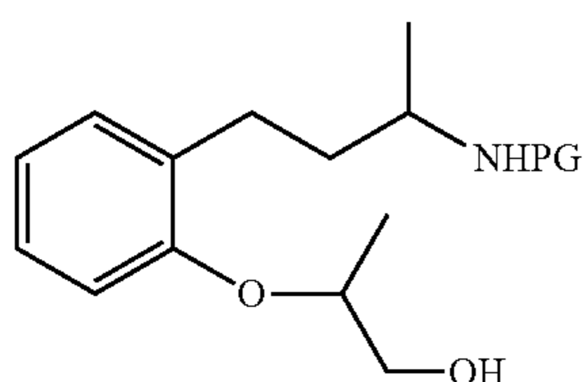
T125a [(R)-isomer] T125b [(S)-isomer]
