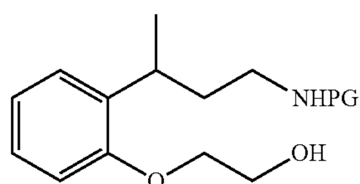
T39a [(R)-isomer] T39b [(S)-isomer]
