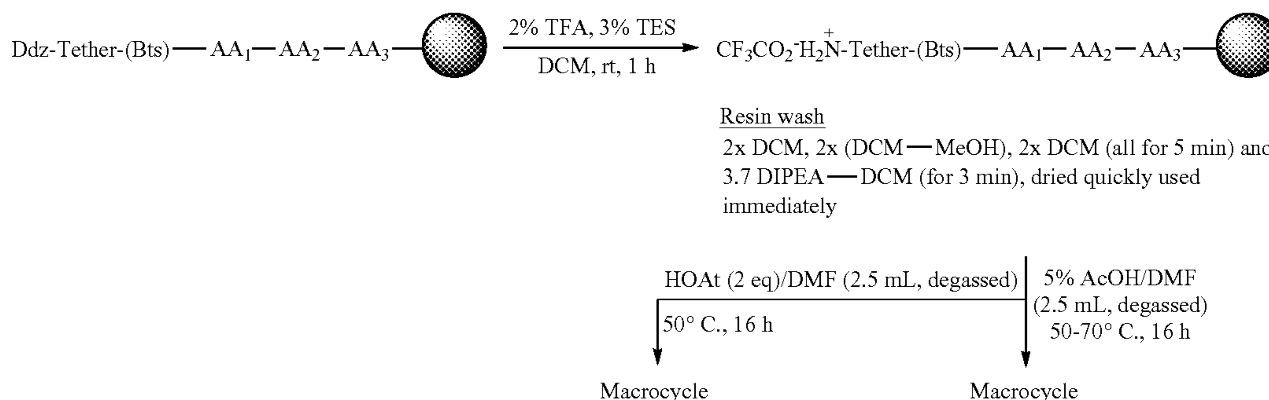
Scheme 2: Alternative Cyclization Methodologies
