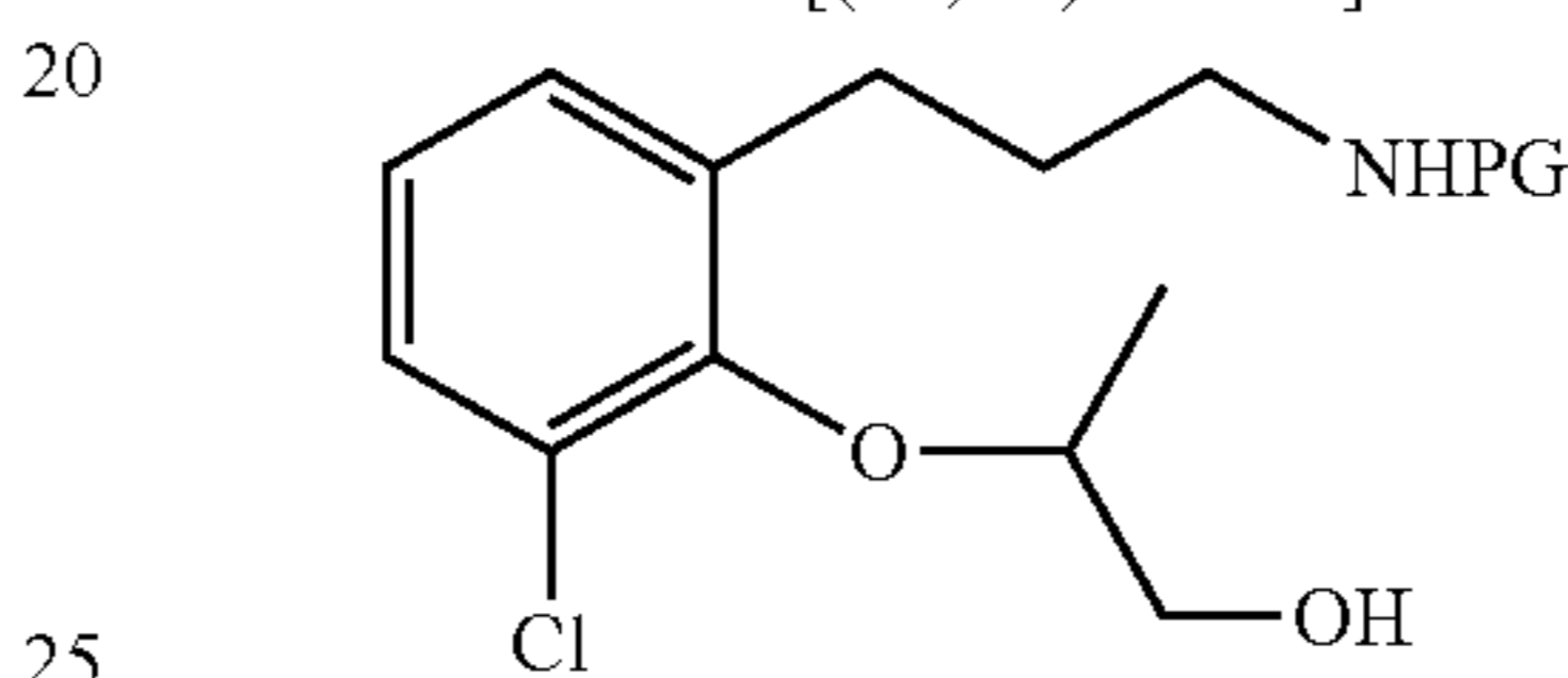
T115a [(R)-isomer] T115b [(S)-isomer]
