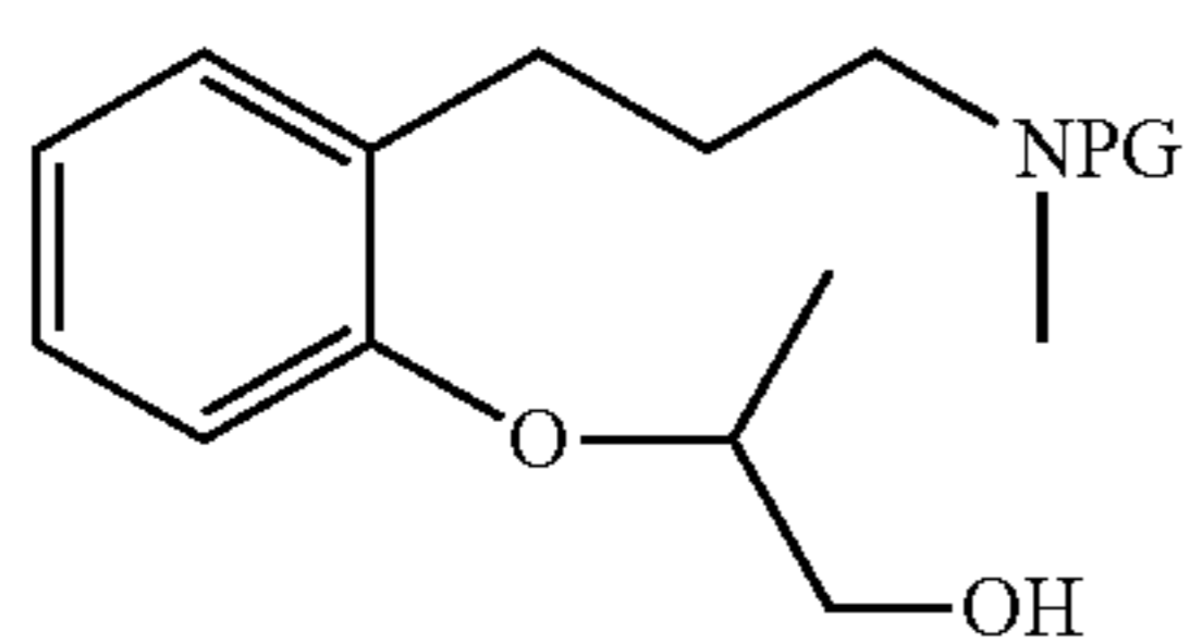
T122a [(R)-isomer] T122b [(S)-isomer]
