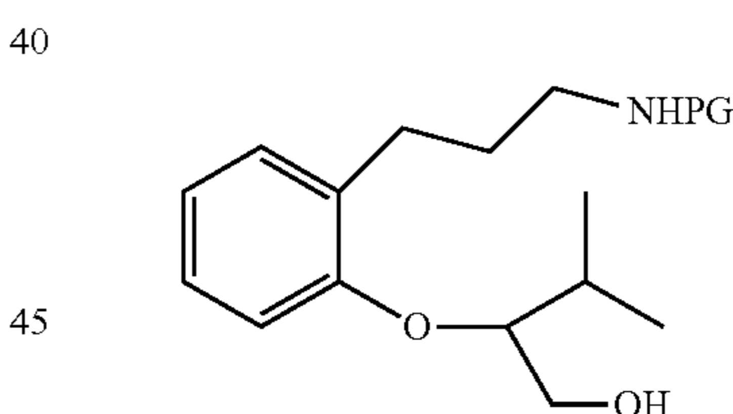
T117a [(R)-isomer] T117b [(S)-isomer]
