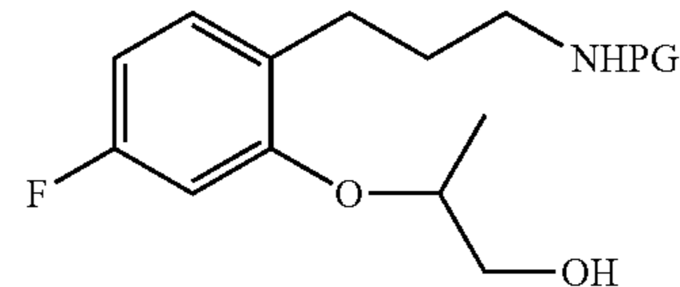
T75a [(R)-isomer] T75b [(S)-isomer]
