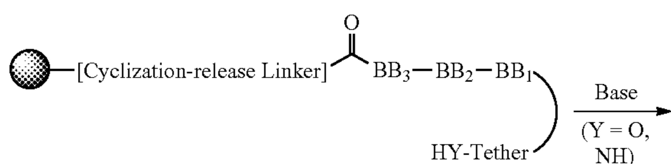
Scheme 1. Cyclization-release Strategy
