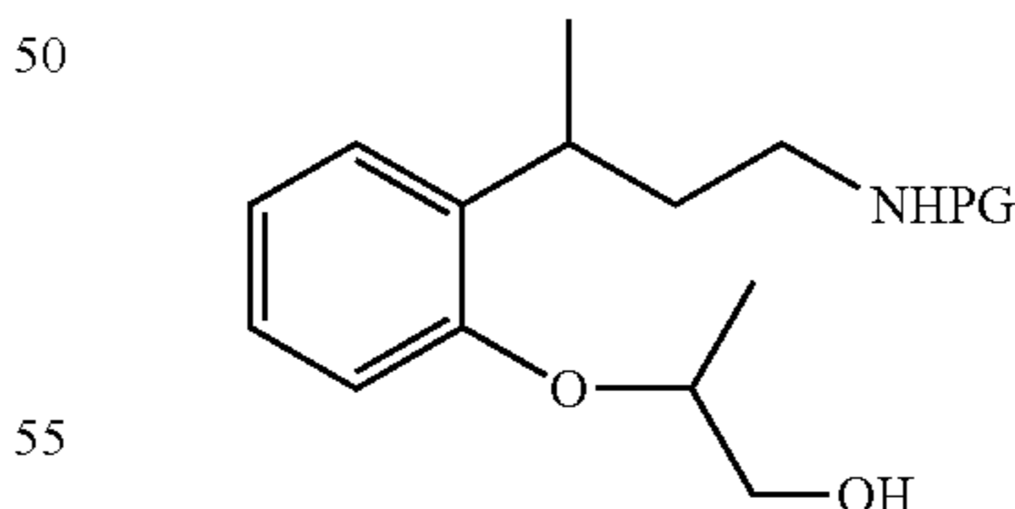
T118a [(2R,7R)-isomer] T118b [(2S,7S)-isomer] T118c [(2R,7S)-isomer] T118d [(2S,7R)-isomer]
