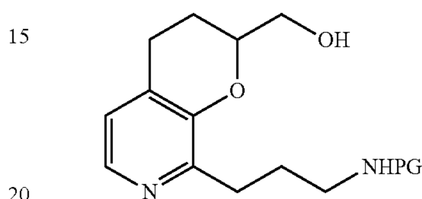
T131a [(R)-isomer] T131b [(S)-isomer]
