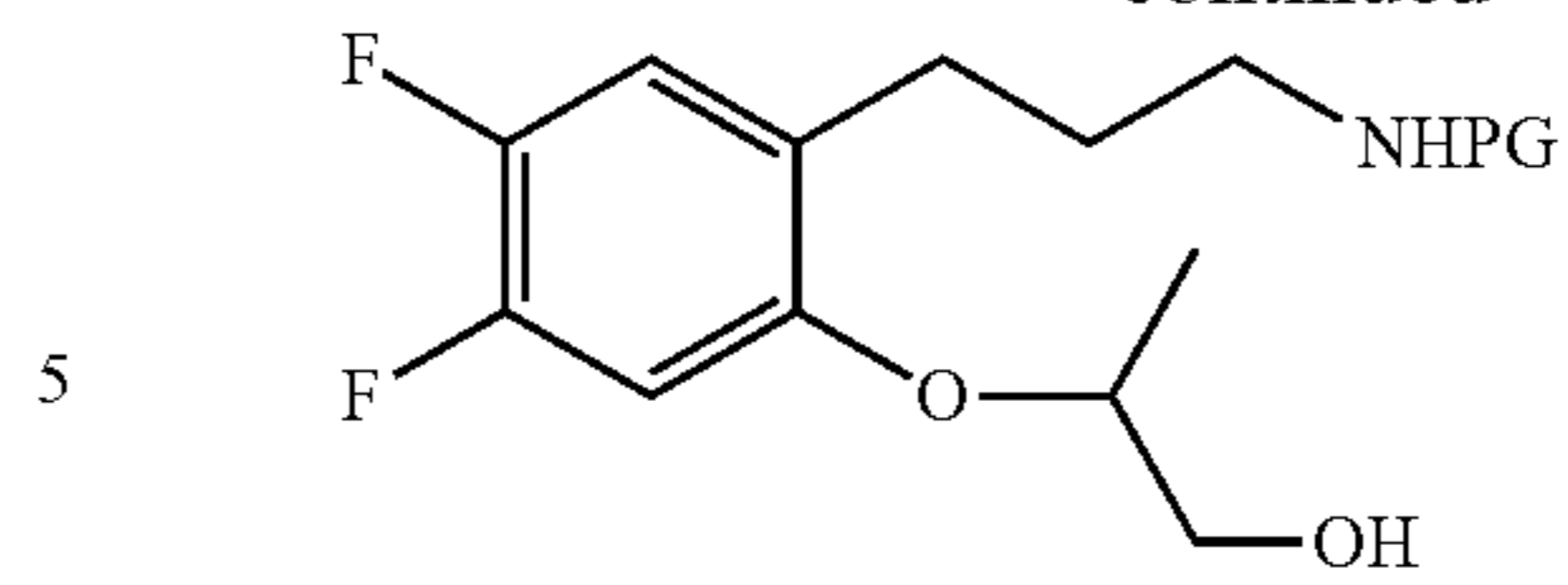
T112a [(R)-isomer] T112b [(S)-isomer]
