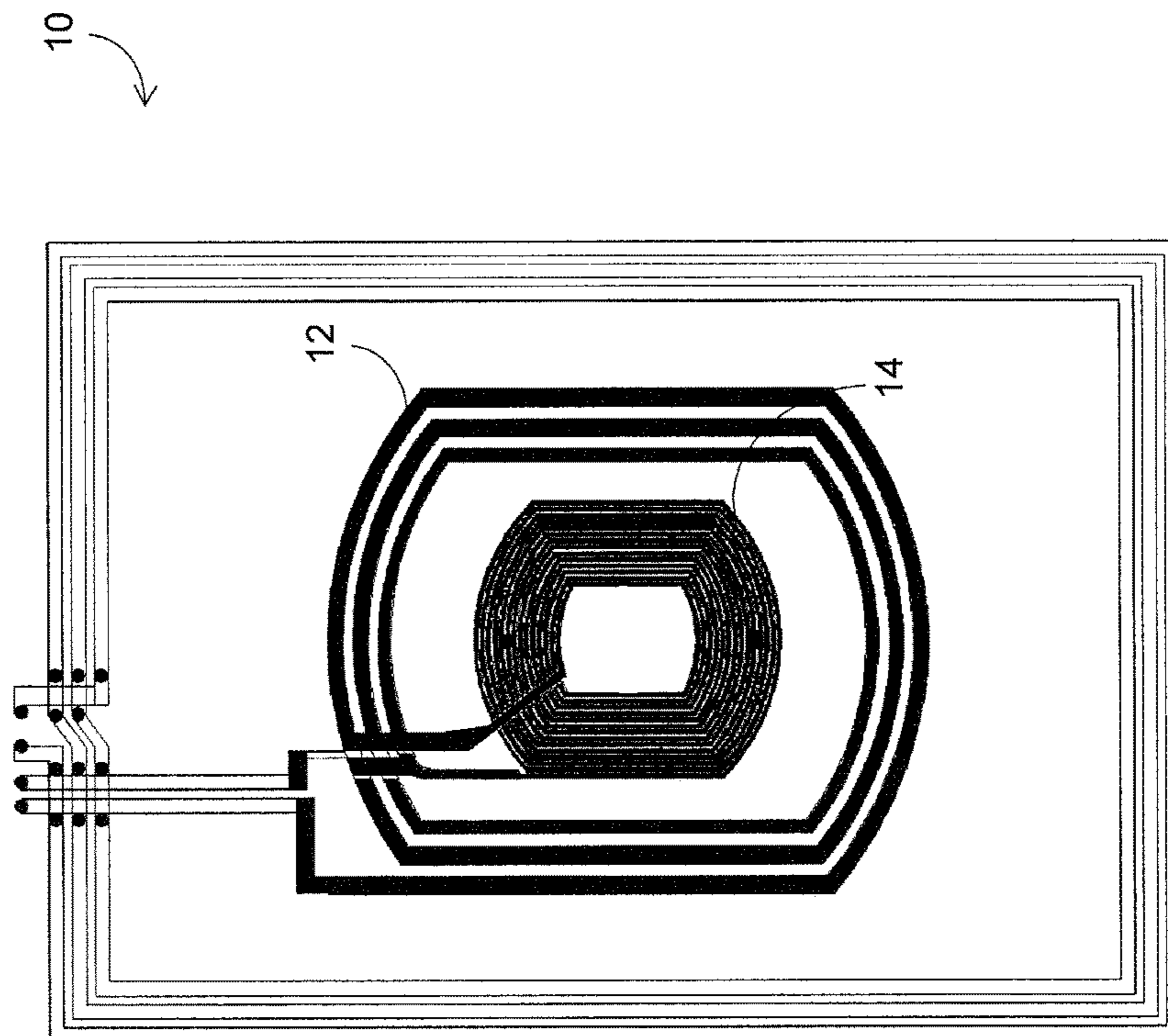
FIG. 1 PRIOR ART
