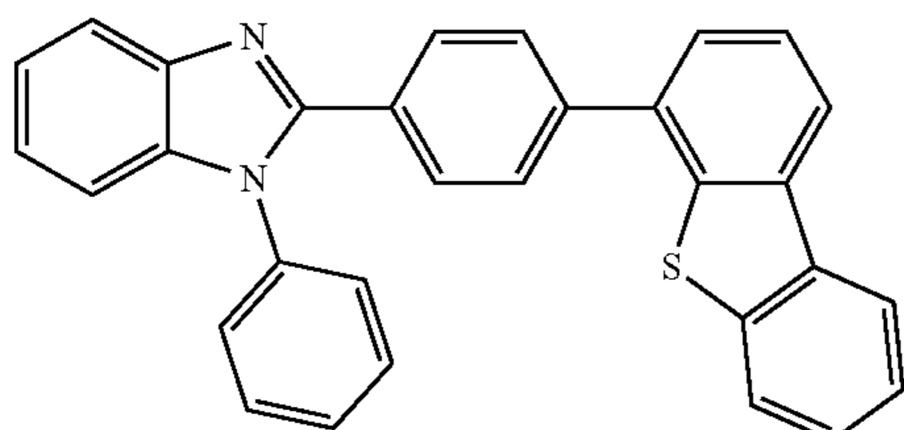
DBTBIIm-II
