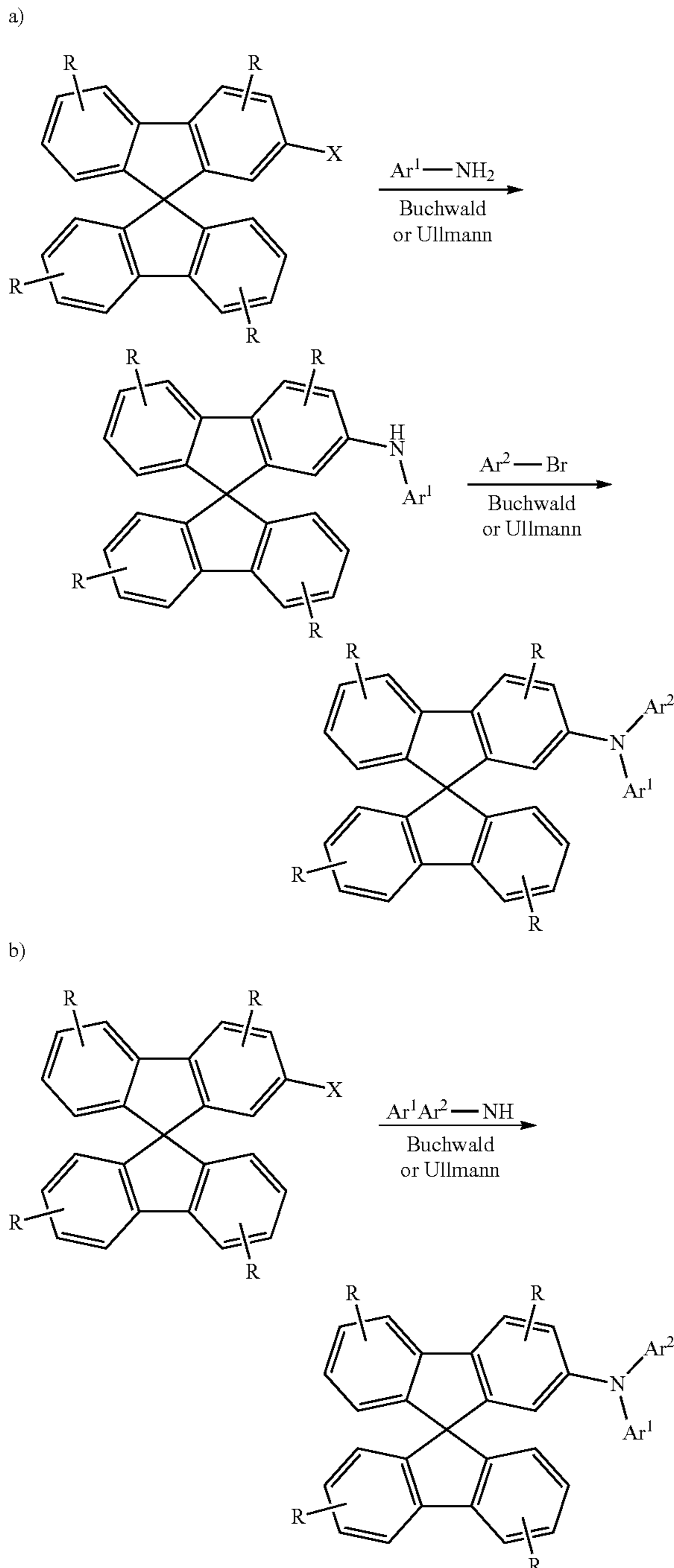
Scheme 1
