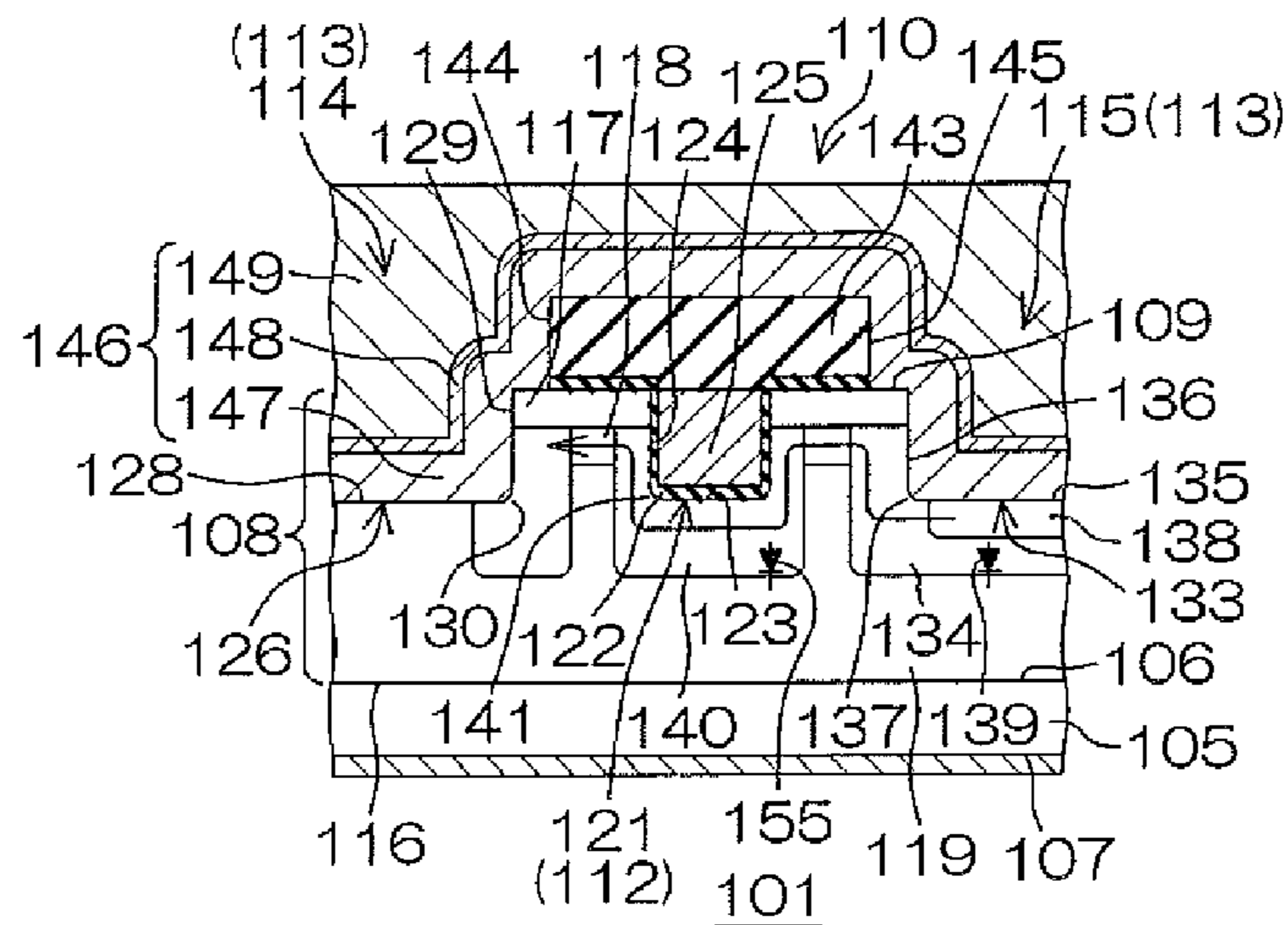
CROSS SECTION H-H
