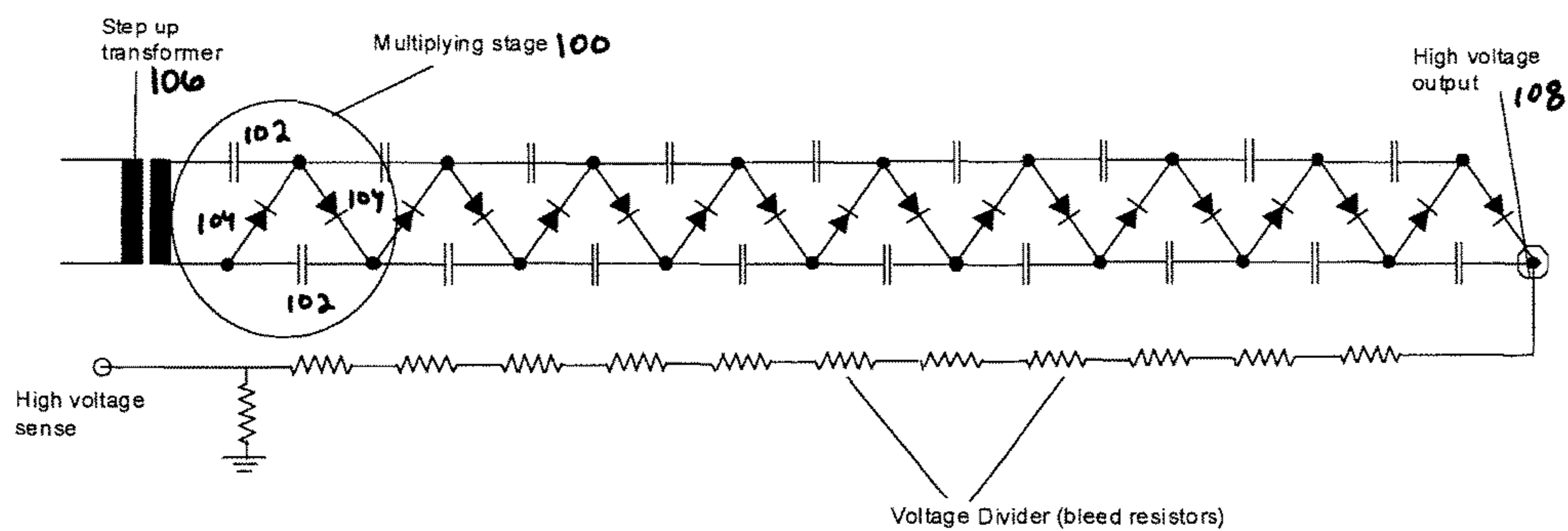
FIG. 1 (Prior Art)
