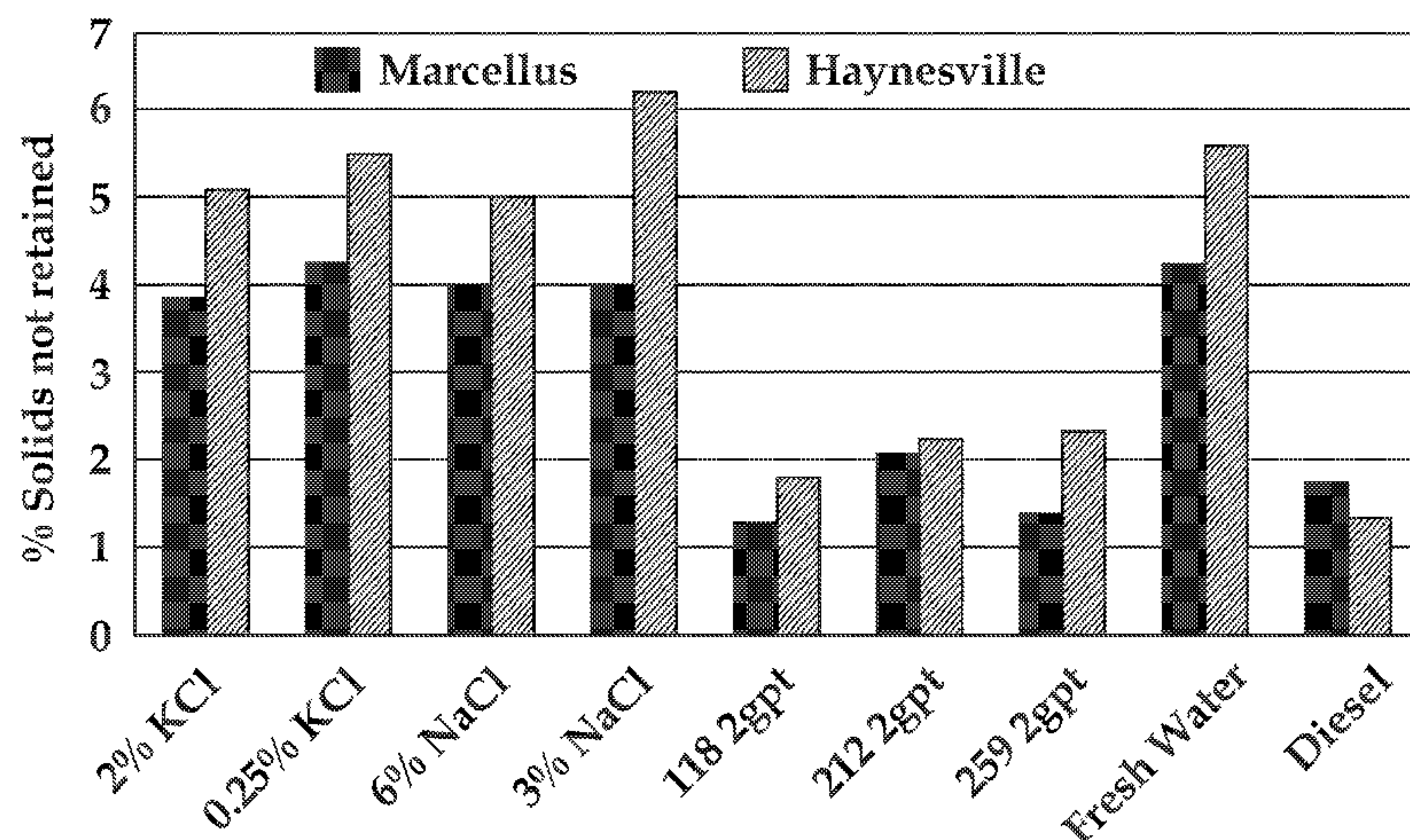
Roller Oven Shale Stability
