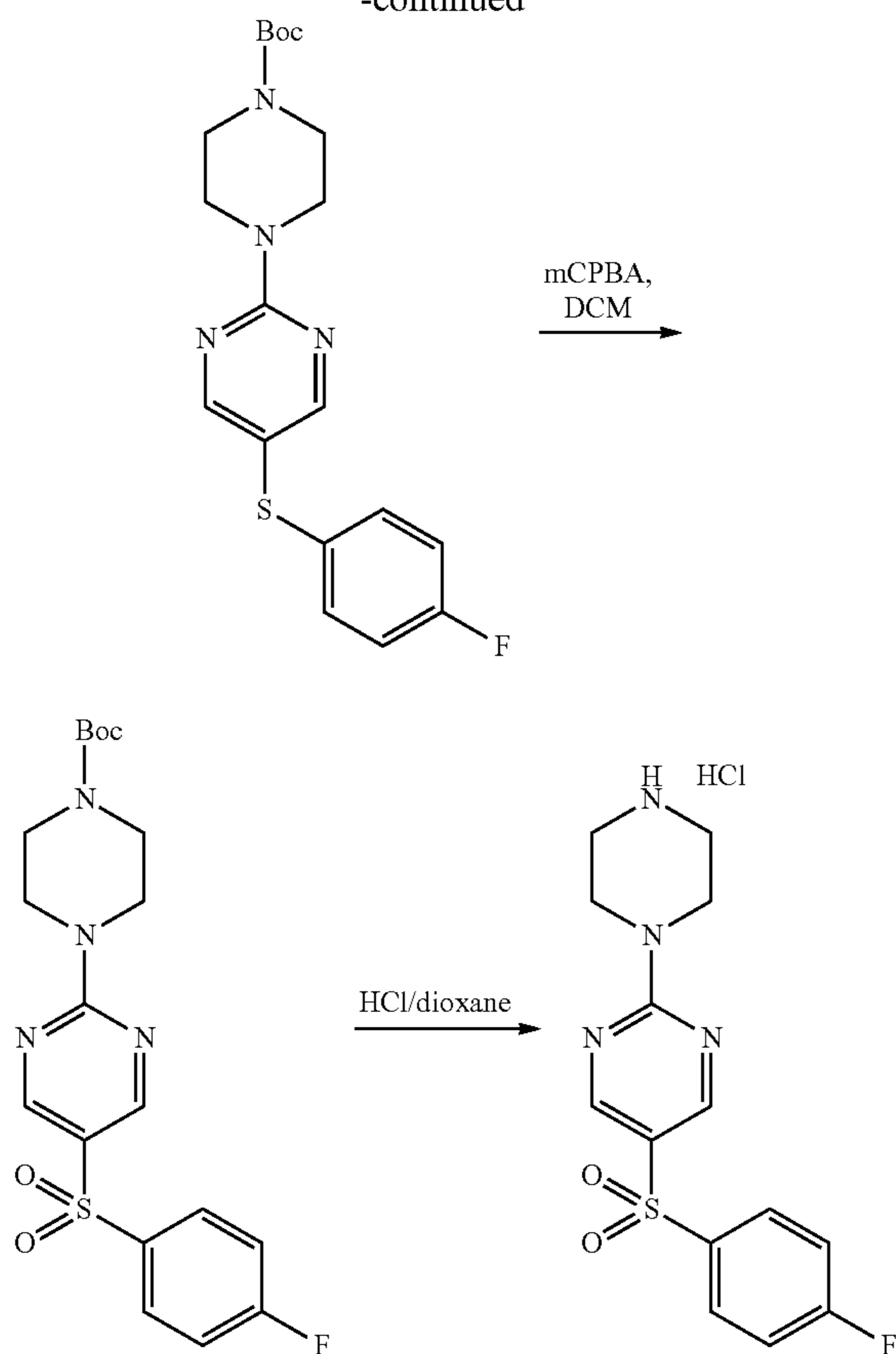
Step 1: Synthesis of tert-butyl 4-(5-(4-fluorophenylthio)pyrimidin-2-yl)piperazine-1-carboxylate
