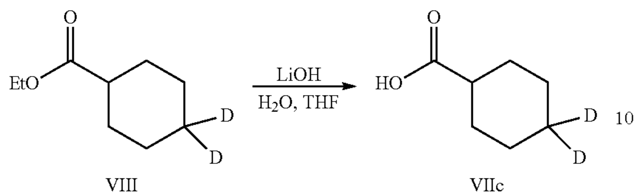
Scheme 3: Method for Preparation of Intermediate VIIc
