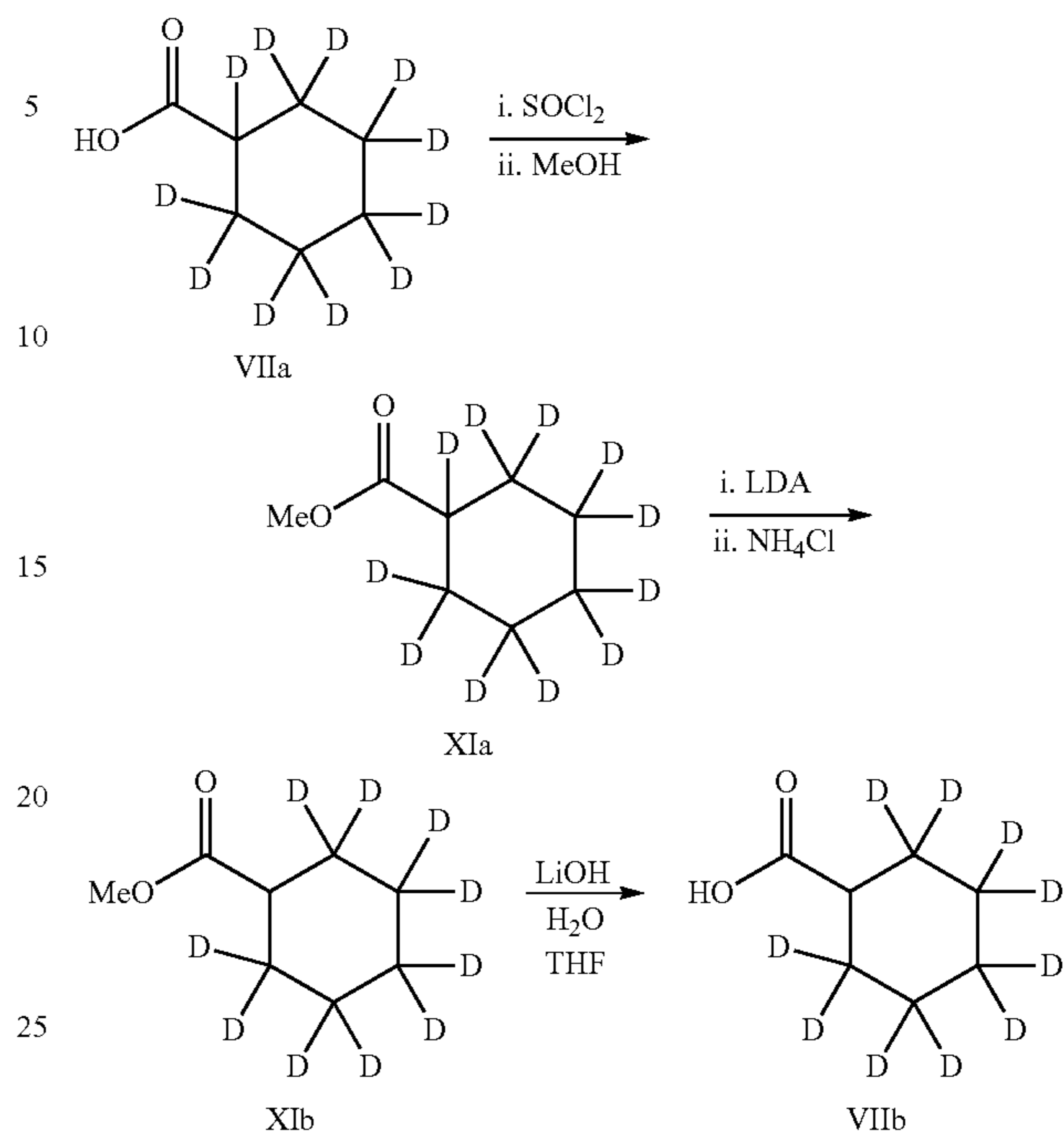
Scheme 2a: Alternative Method for Preparation of Intermediate VIIb:
