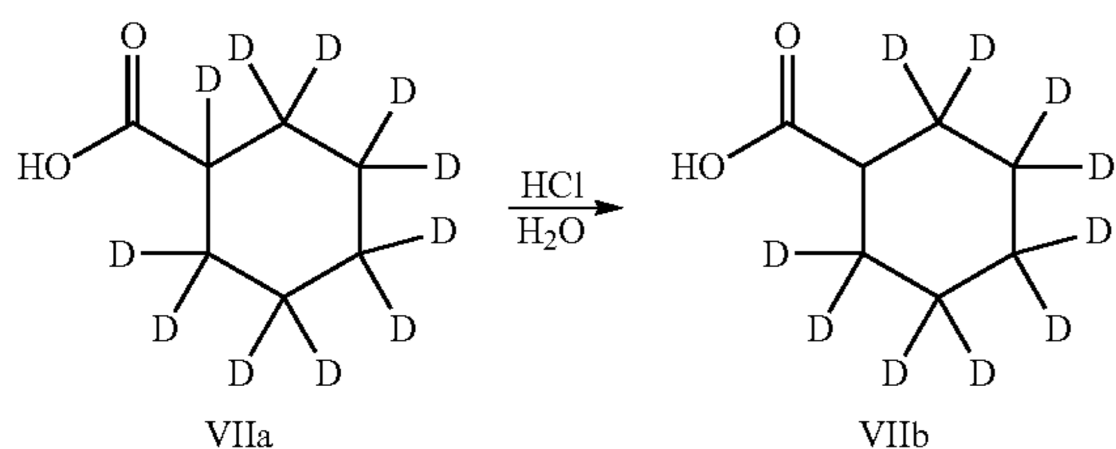
Scheme 2: Method for Preparing of Intermediate VIIb
