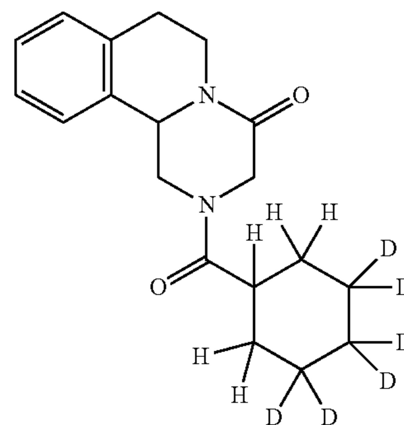
2-(Cyclohexane-3,3,4,4,5,5-d6-carbonyl)-2,3,6,7-tetrahydro-1H-pyrazino[2,1-a]isoquinolin-4(11bH)-one (Compound 109)
