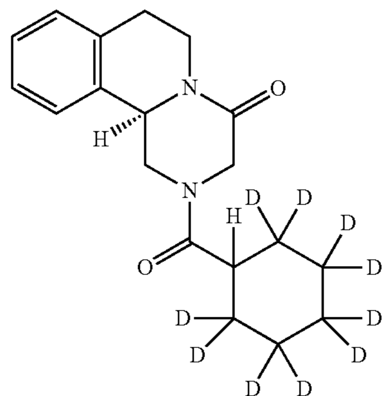
(R)-2-(2,2,3,3,4,4,5,5,6,6-d 10 -Cyclohexanecarbonyl)-2,3,6,7-tetrahydro-1H-pyrazino[2,1-a]isoquinolin-4(11bH)-one (103a)
