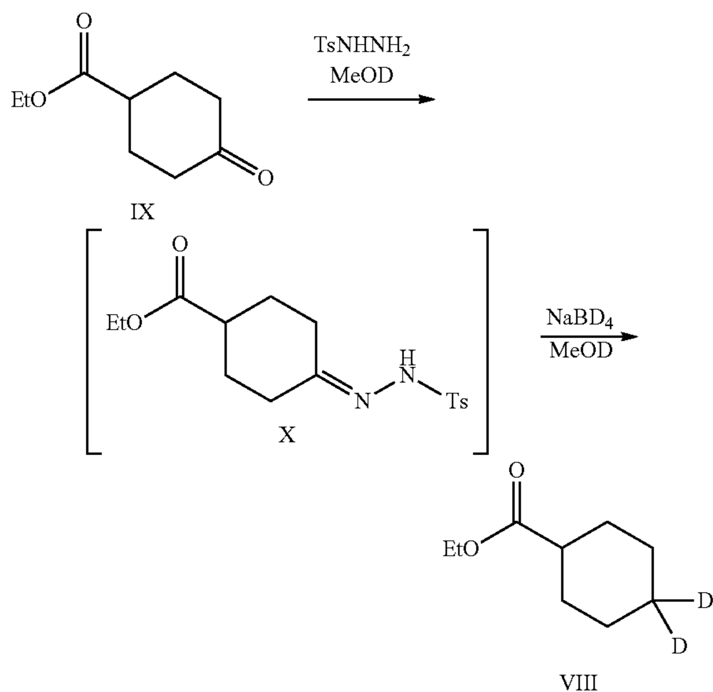
Scheme 3a: Method for Preparation of Intermediate VIII
