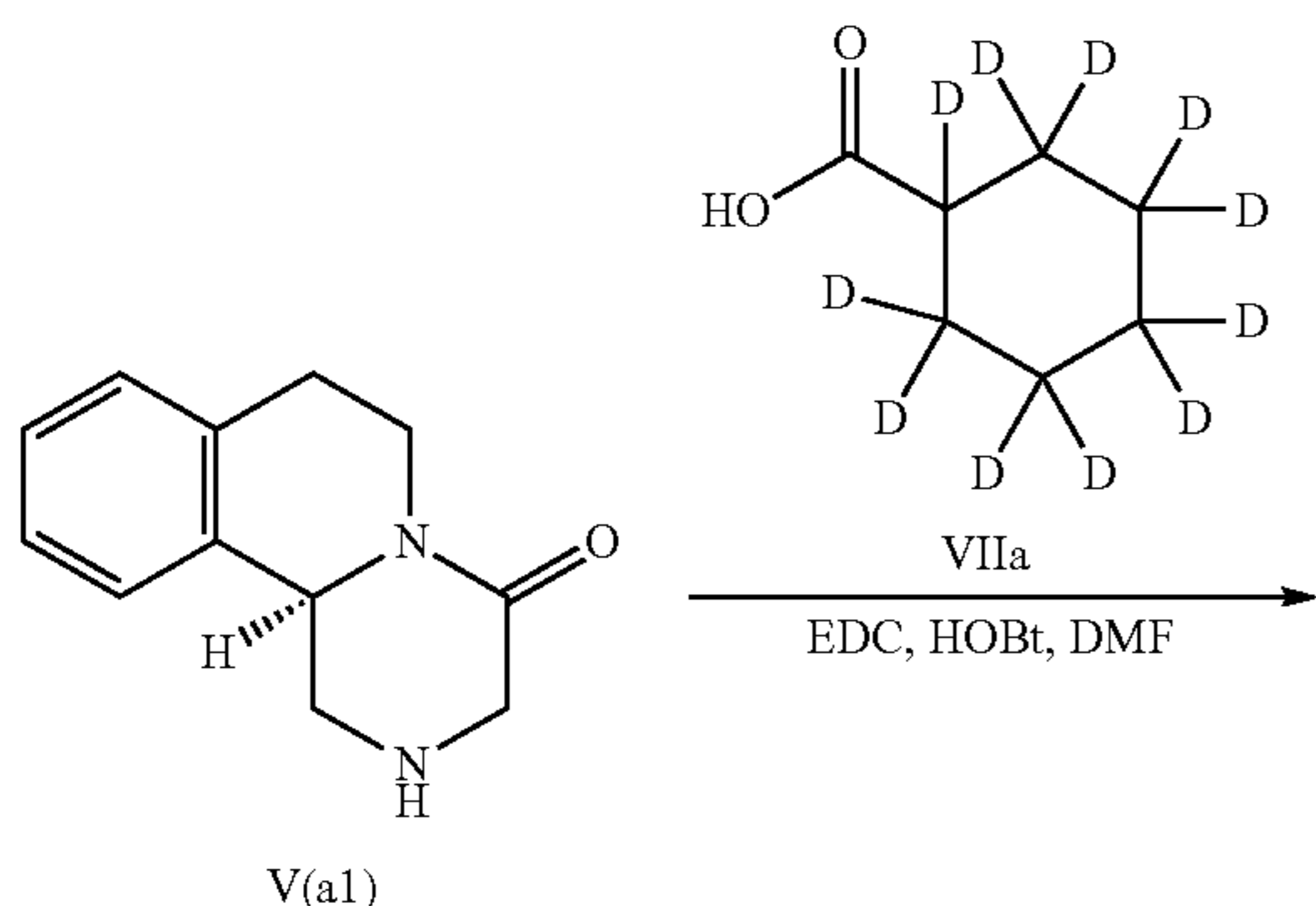
Scheme 10. Preparation of Compound 102a
