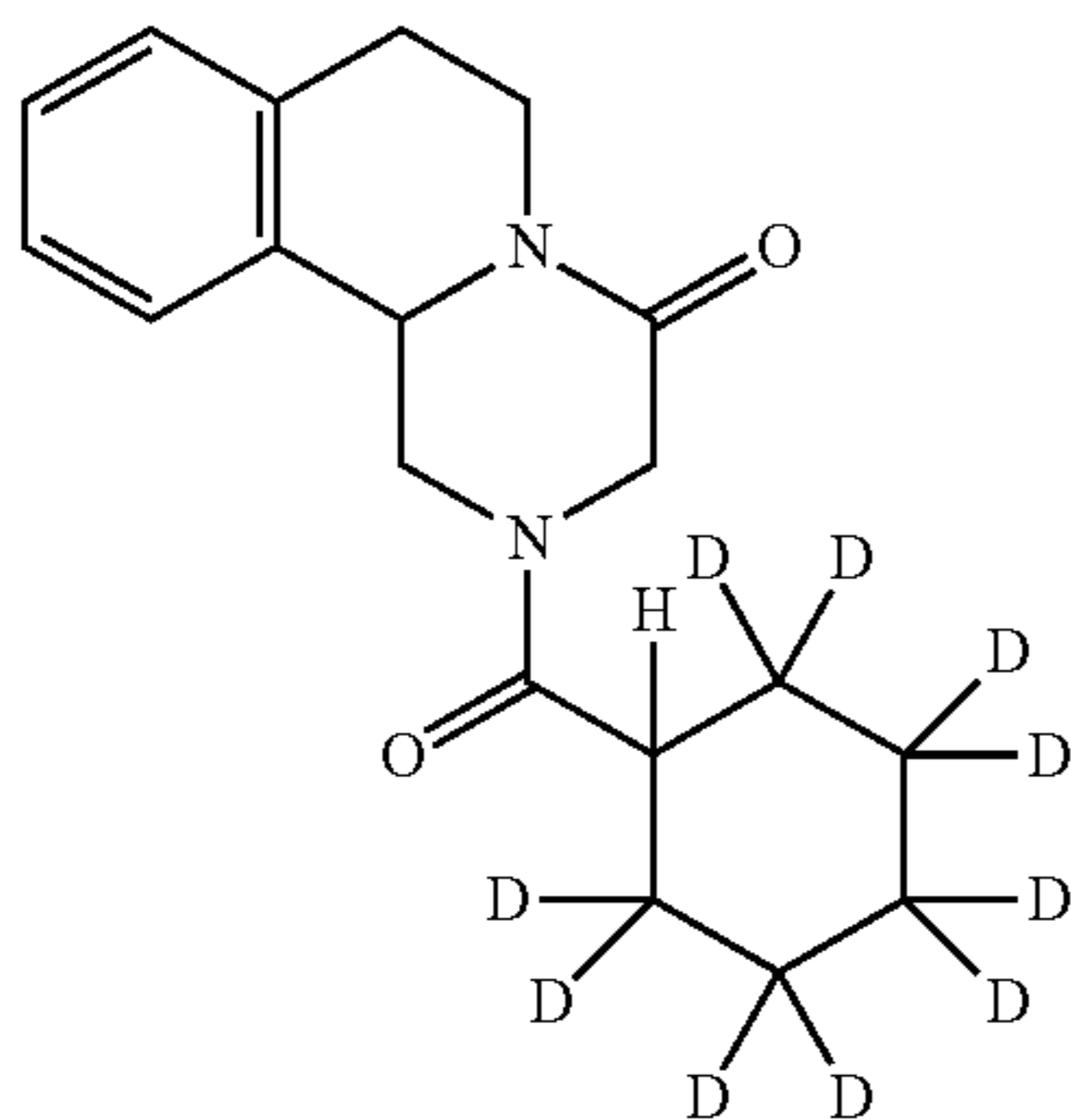
2-(Cyclohexane-2,2,3,3,4,4,5,5,6,6-d10-carbonyl)-2,3,6,7-tetrahydro-1H-pyrazino[2,1-a]isoquinolin-4(11bH)-one (Compound 103)
