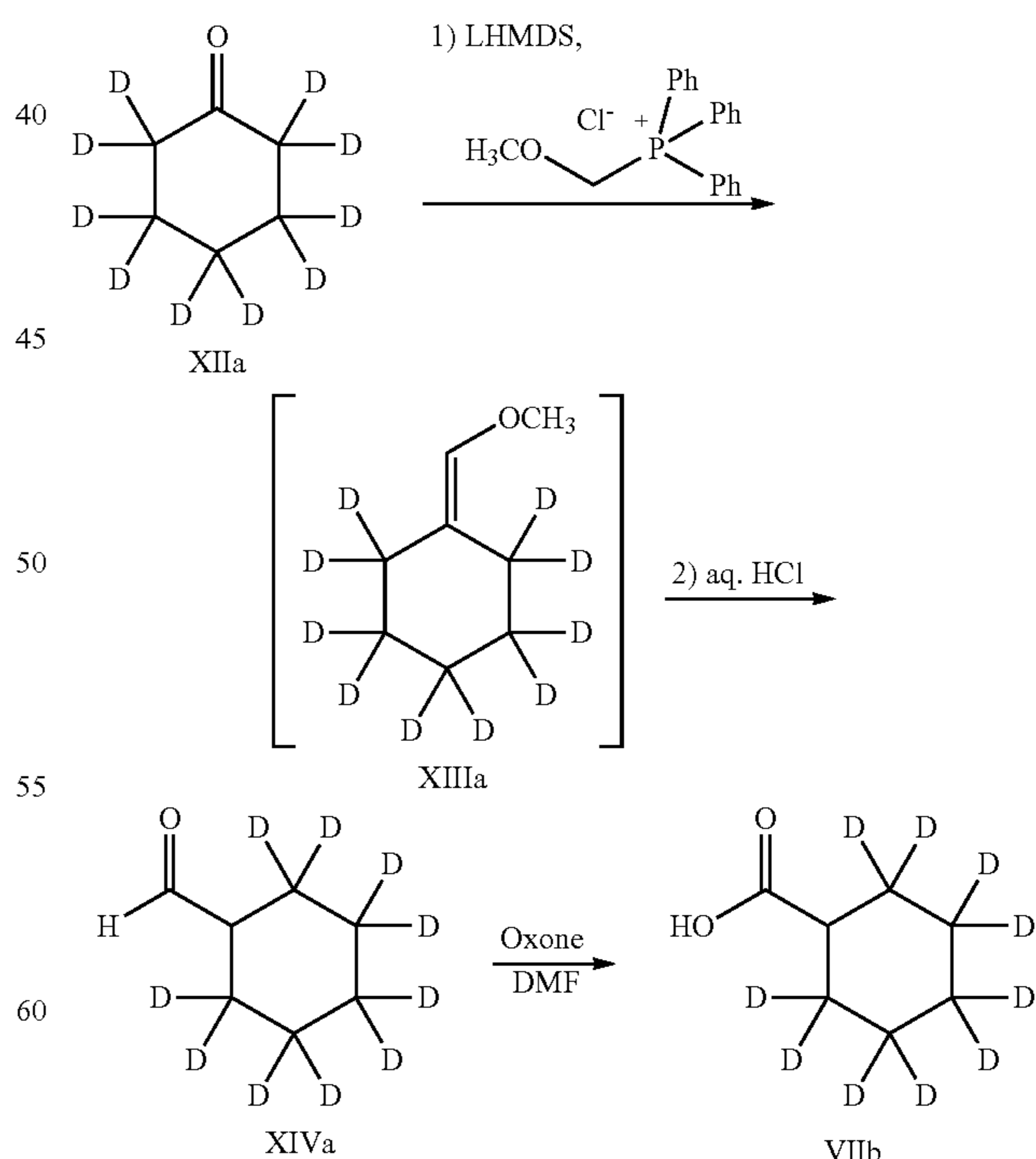
Scheme 2b: Alternative Method for Preparation of Intermediate VIIb:
