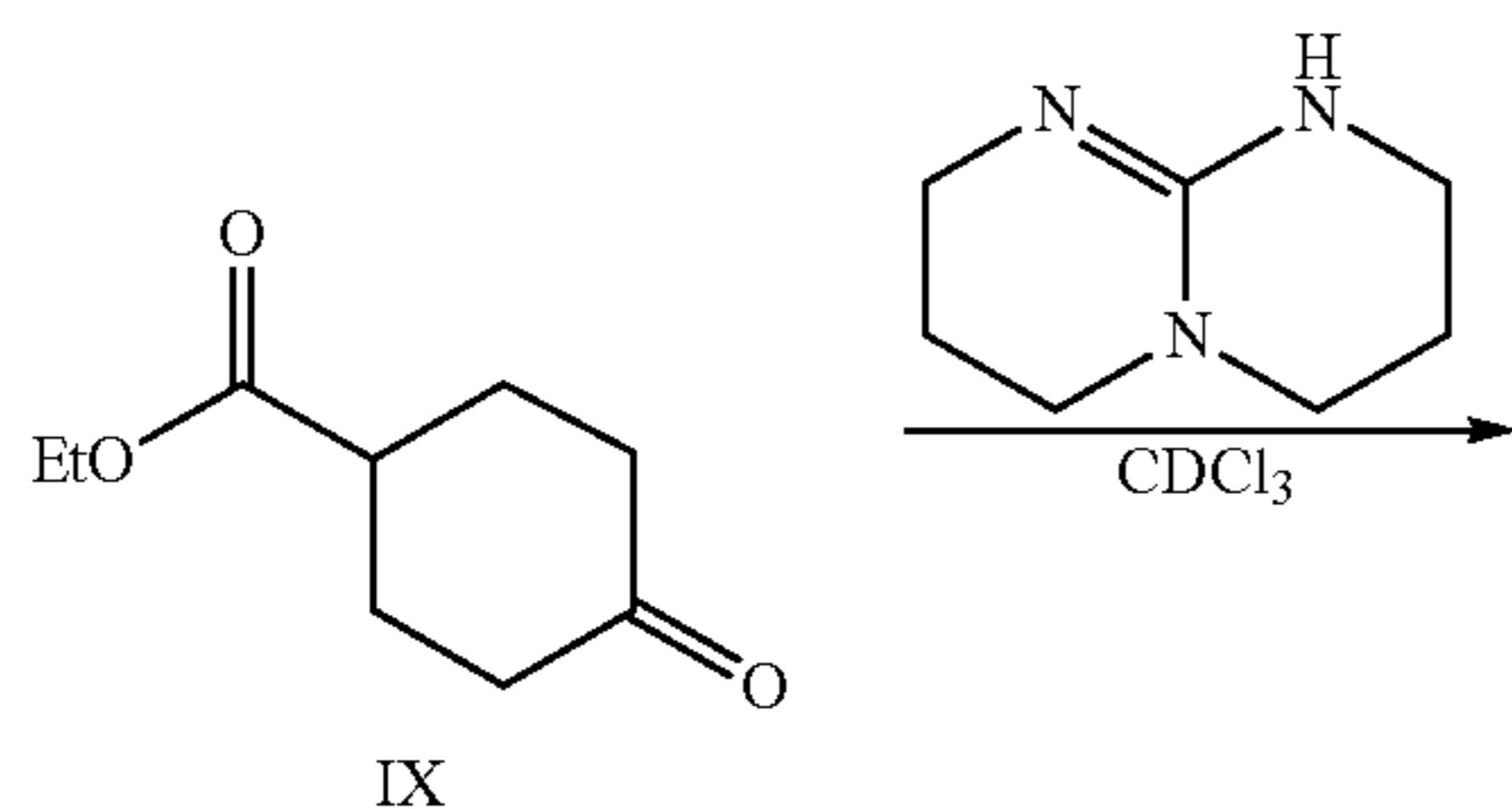
Scheme 4: Method for Preparation of Intermediate VIId:
