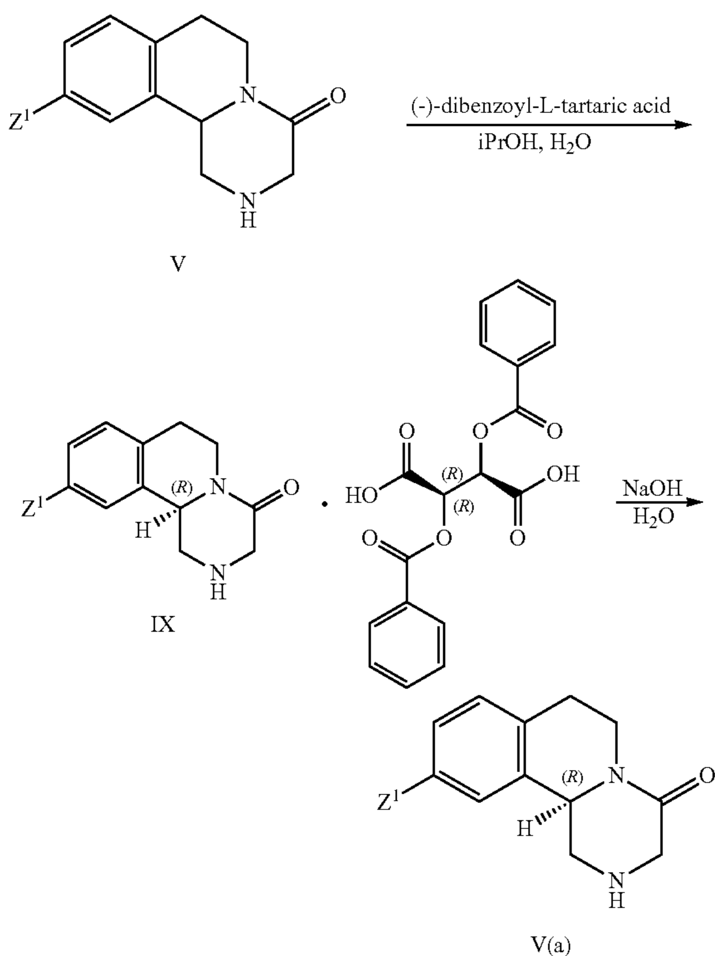
Scheme 5: Method for the Preparation of Intermediates V(a)
