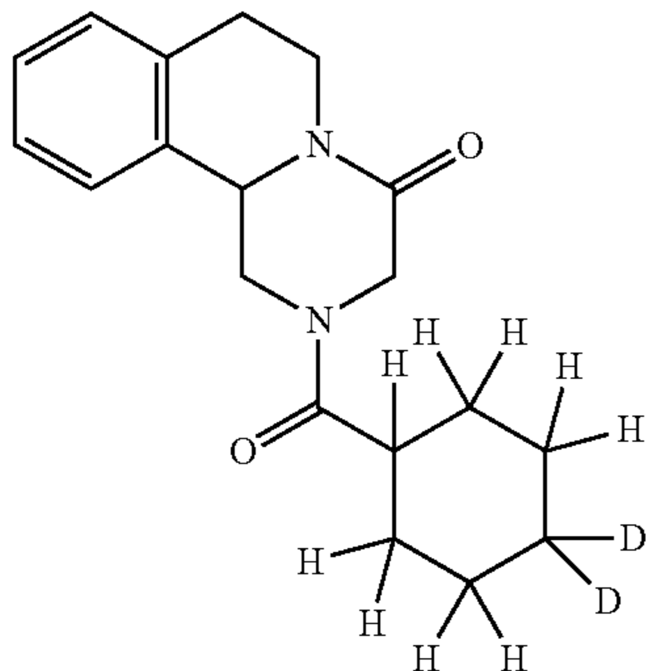
2-(Cyclohexane-4,4-d2-carbonyl)-2,3,6,7-tetrahydro-1H-pyrazino[2,1-a]isoquinolin-4(11bH)-one (Compound 101)
