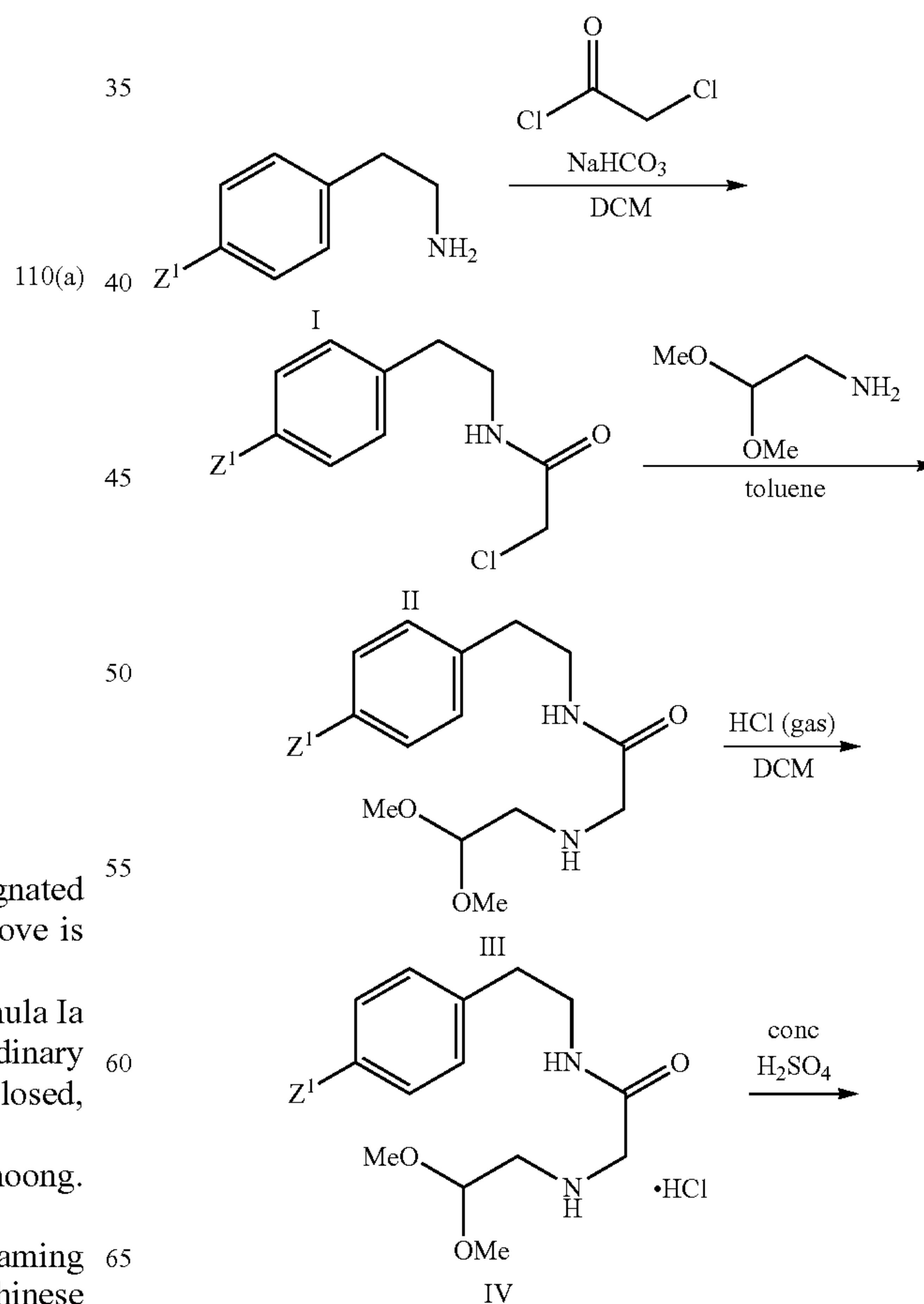
Scheme 1: Method for Preparing Compounds of Formula I
