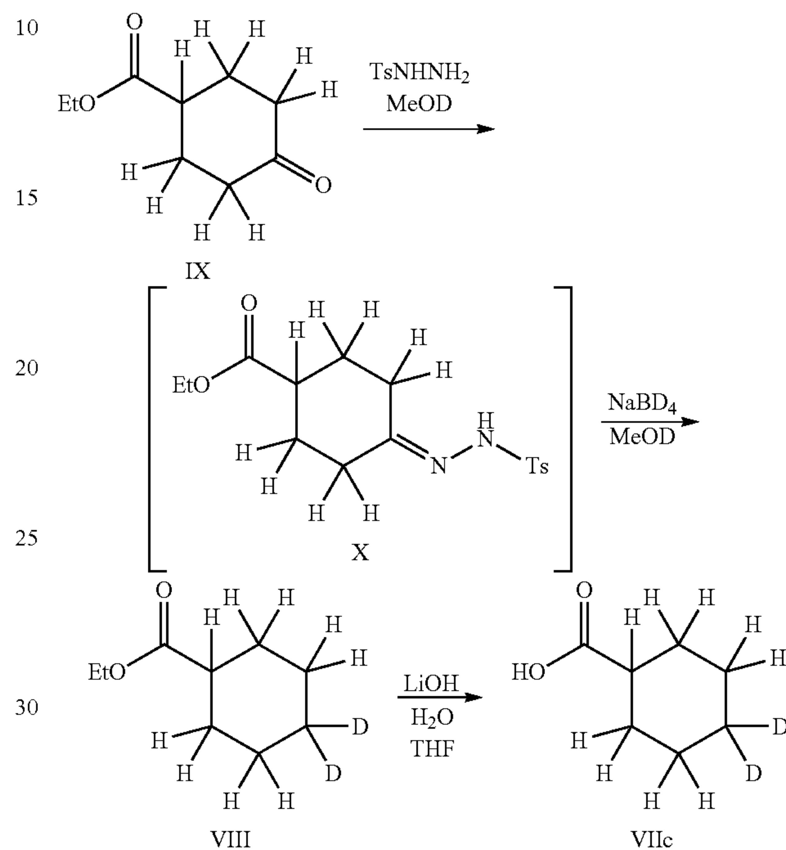
Scheme 7. Preparation of Intermediate VIIc
