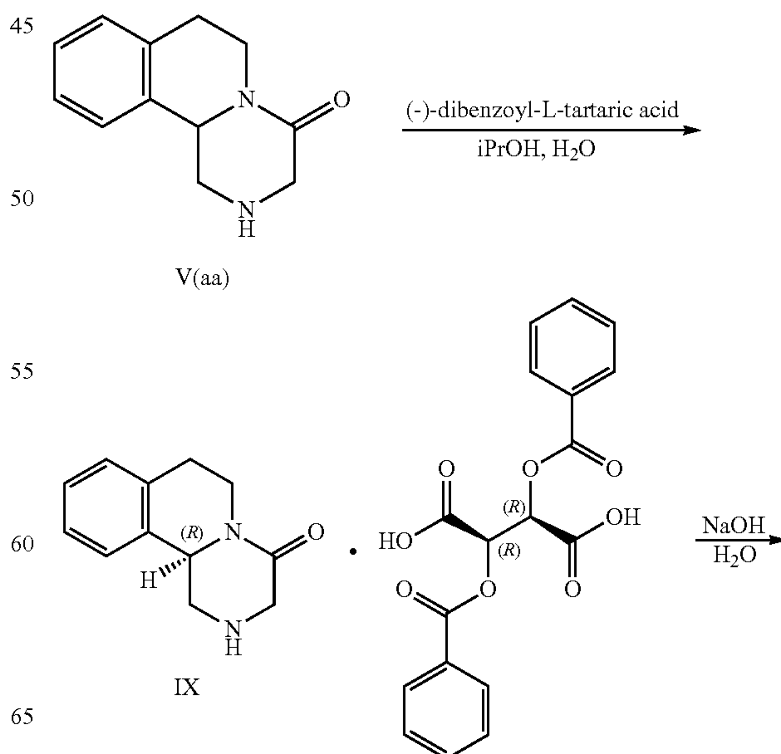
Scheme 5: Preparation of Intermediates V(a1)
