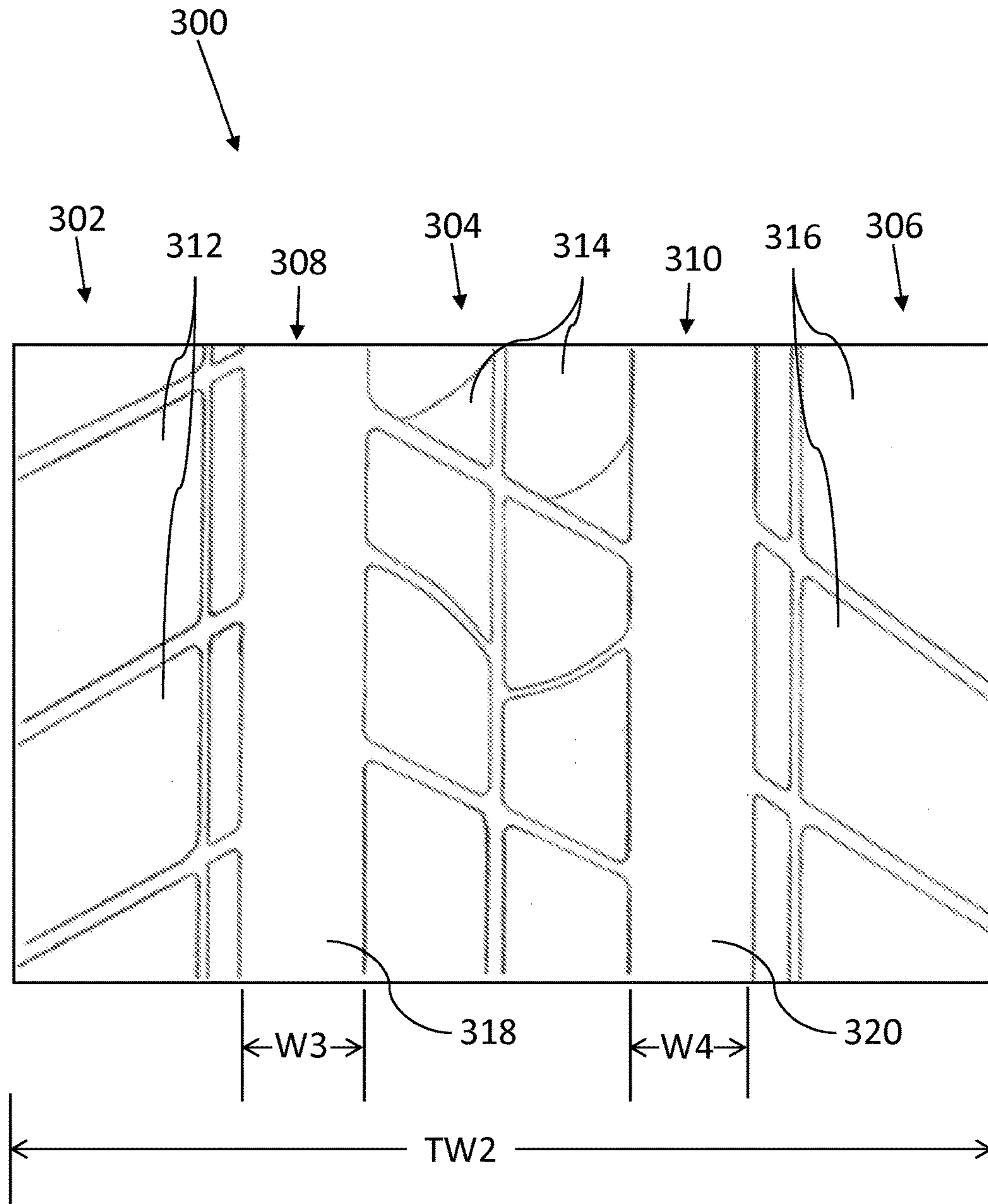
FIG. 3 PRIOR ART
