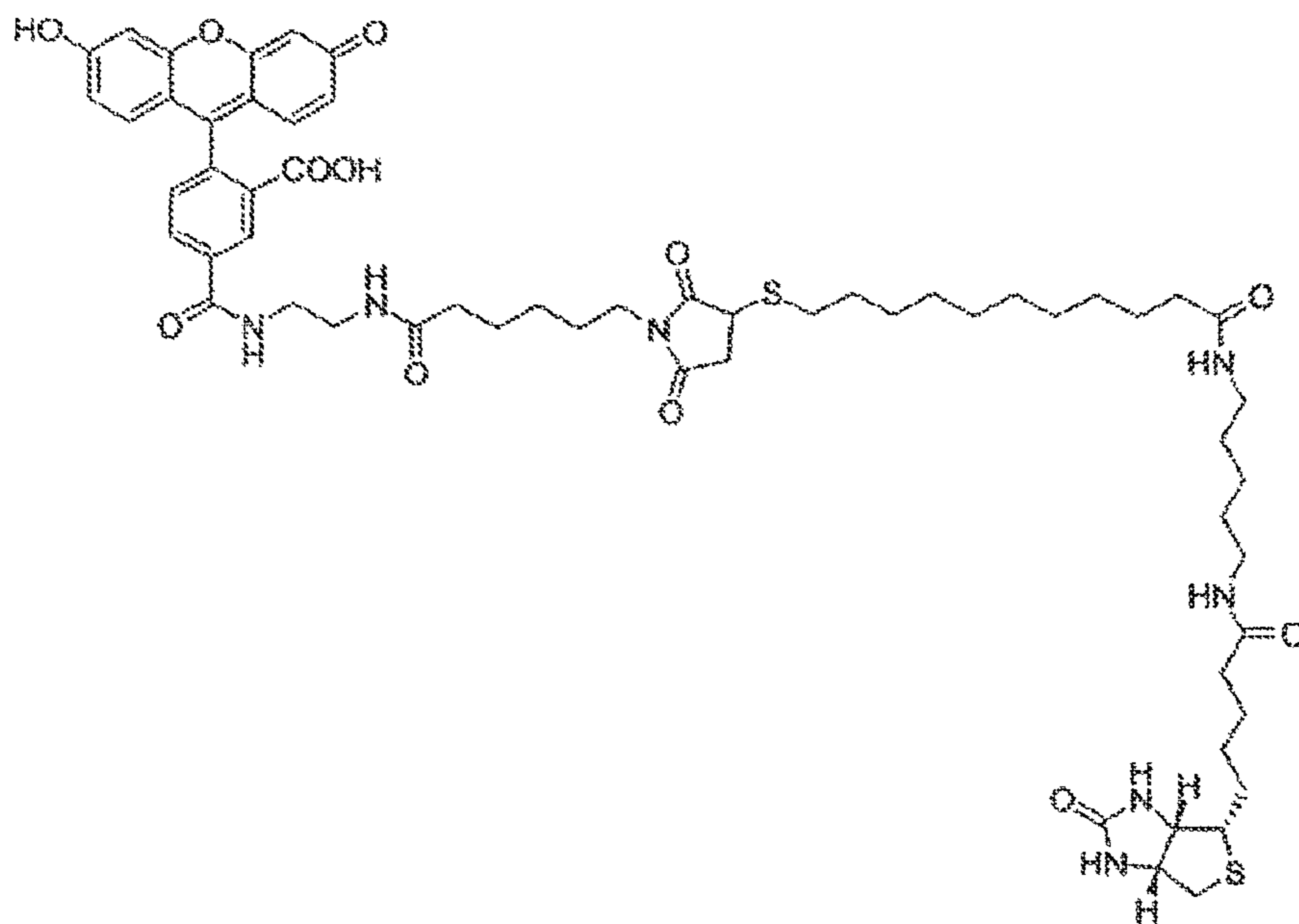
Pro27-biotin
