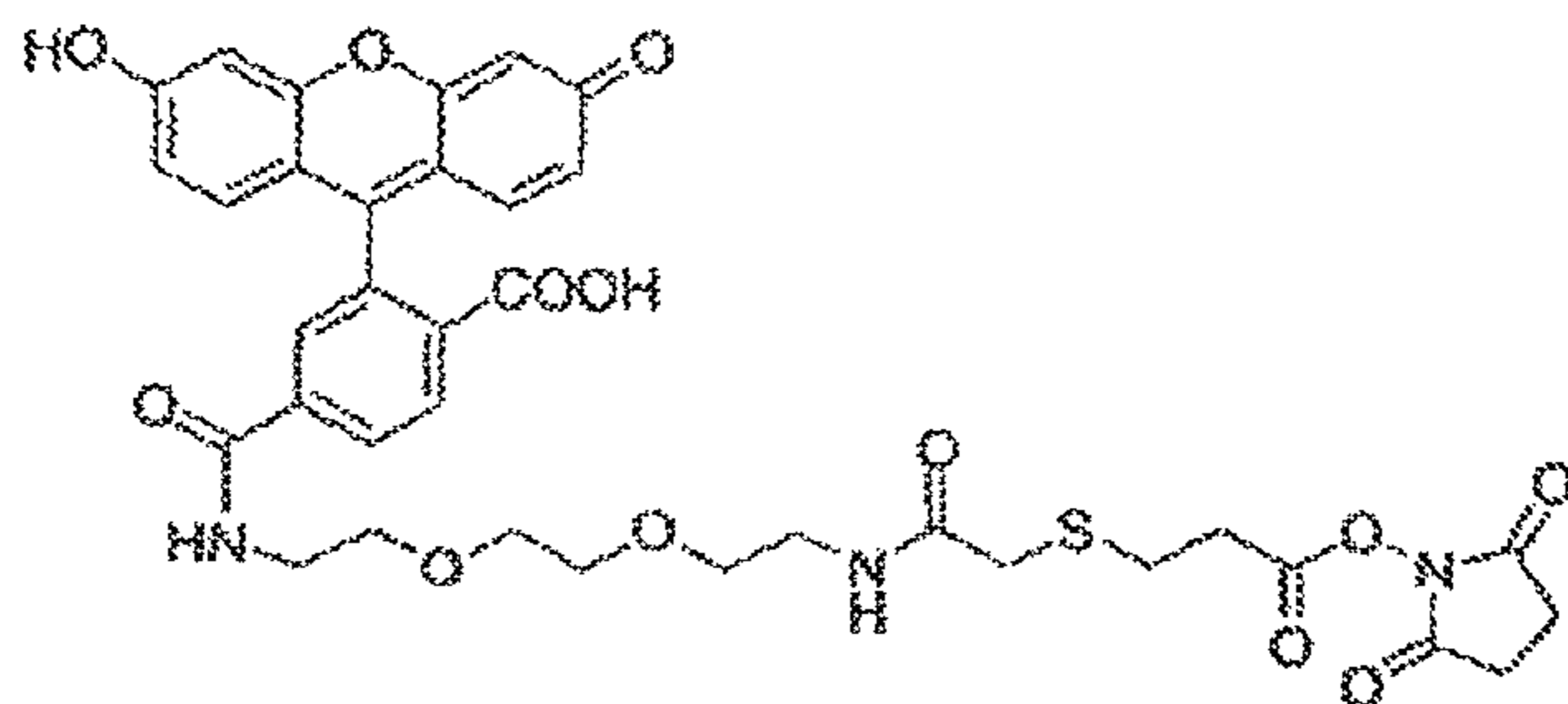
Pro12-NHS
