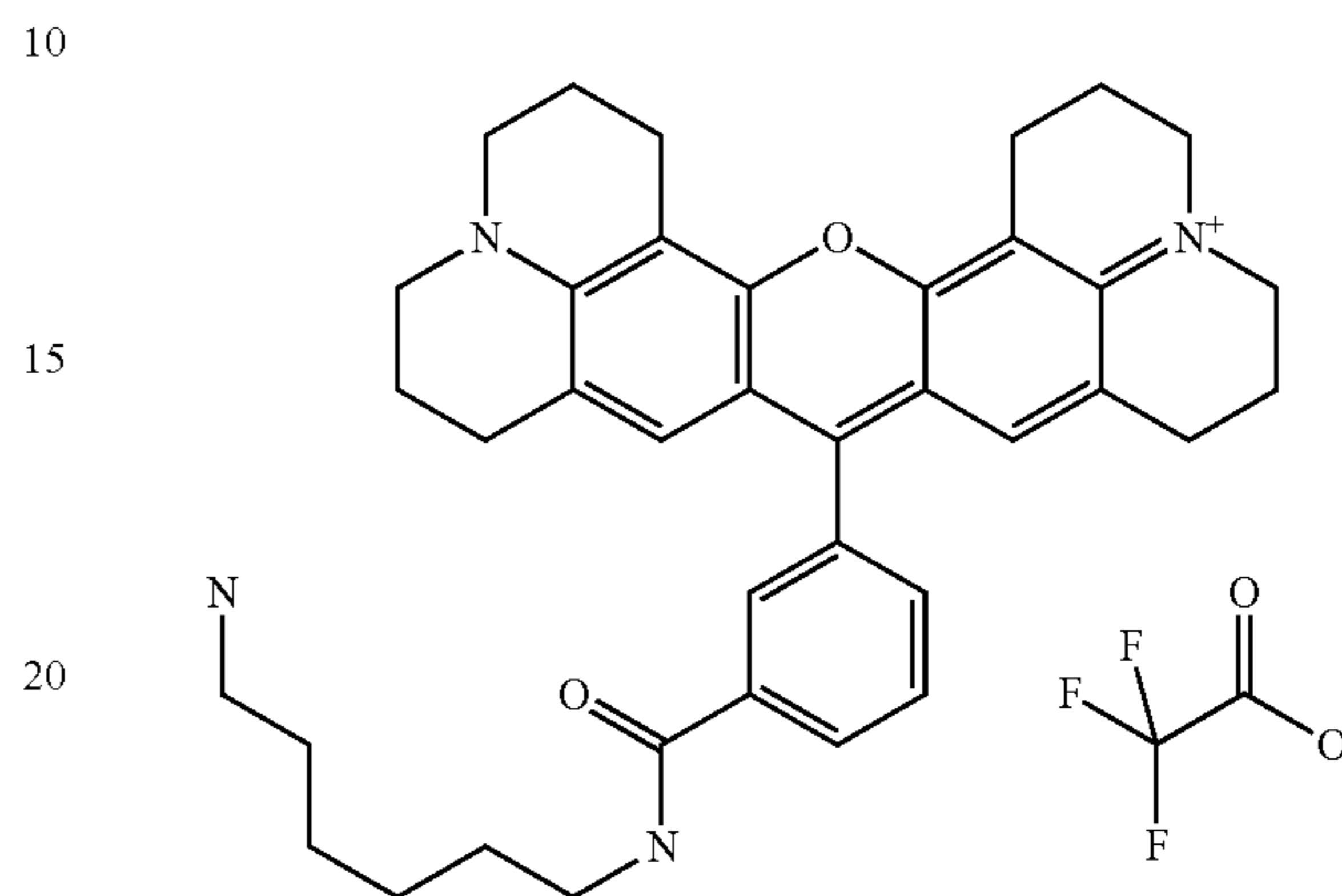
Compound 11
