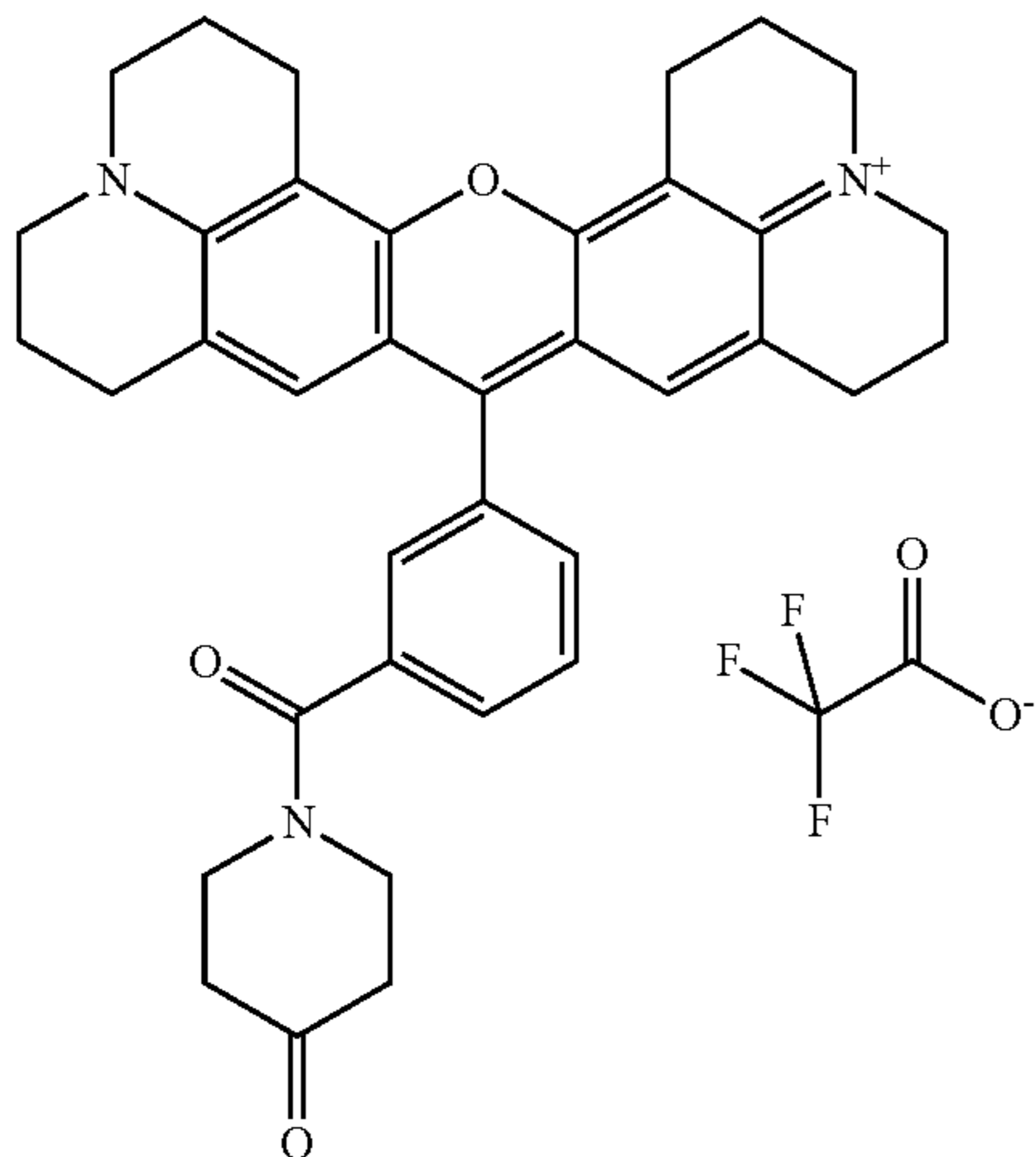
Compound 13
