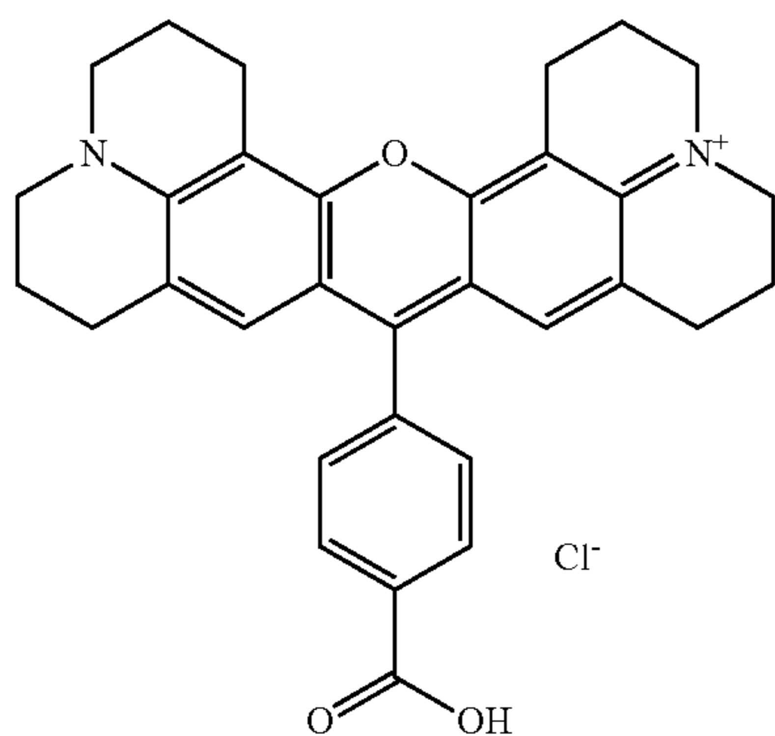
Intermediate 2
