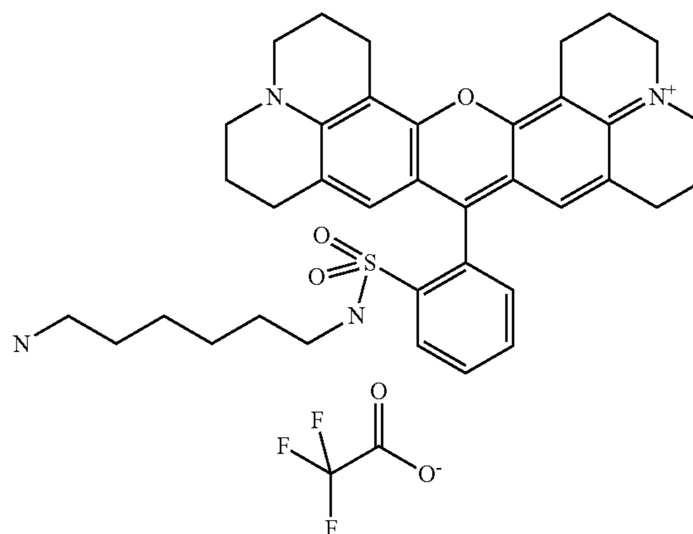
Compound 1
