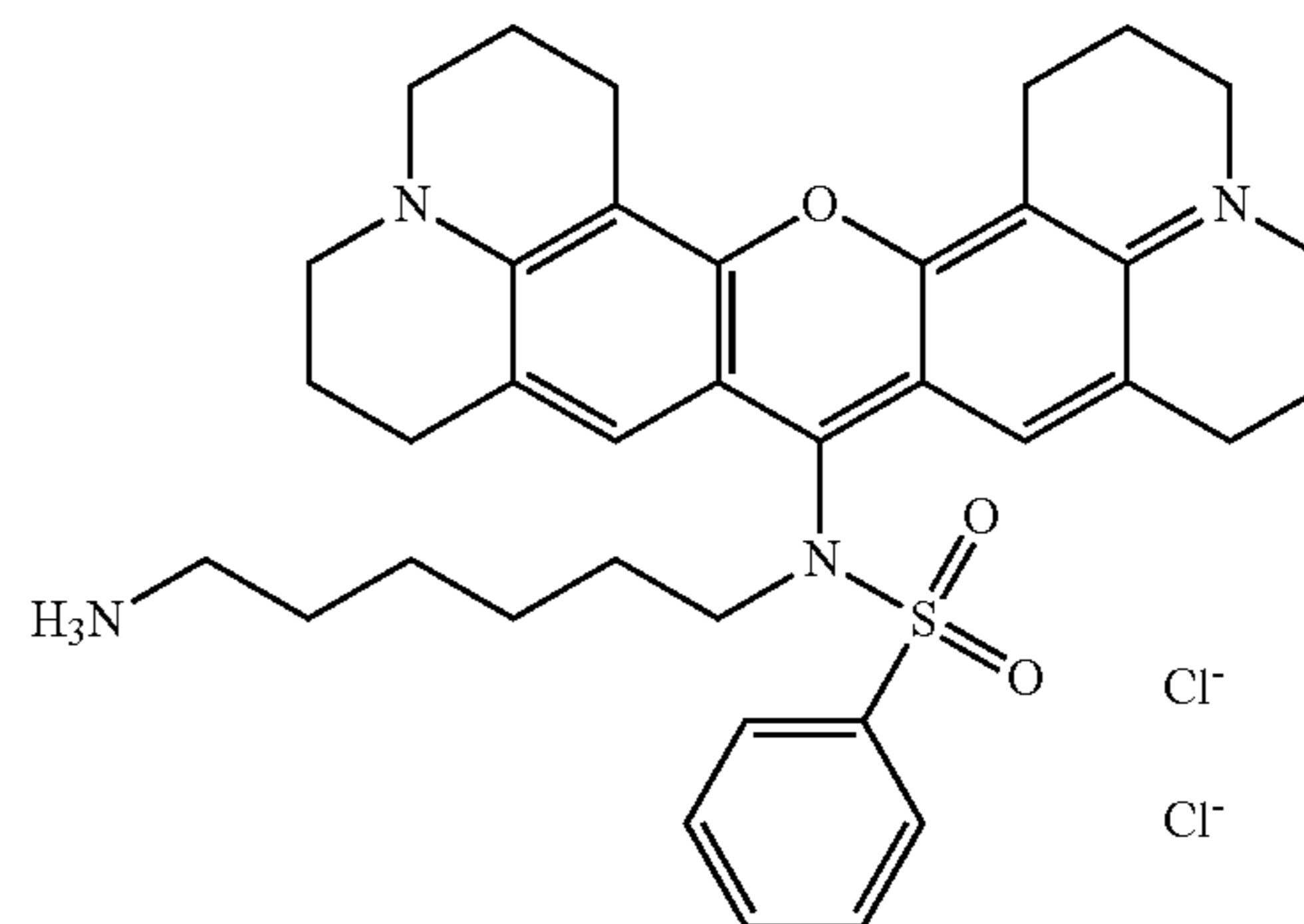
Compound 19
