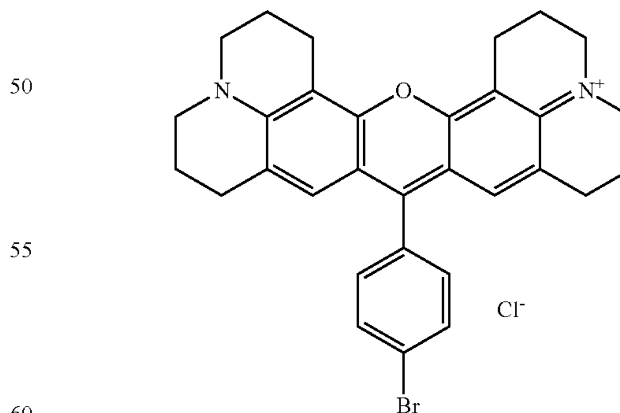
Intermediate 4
