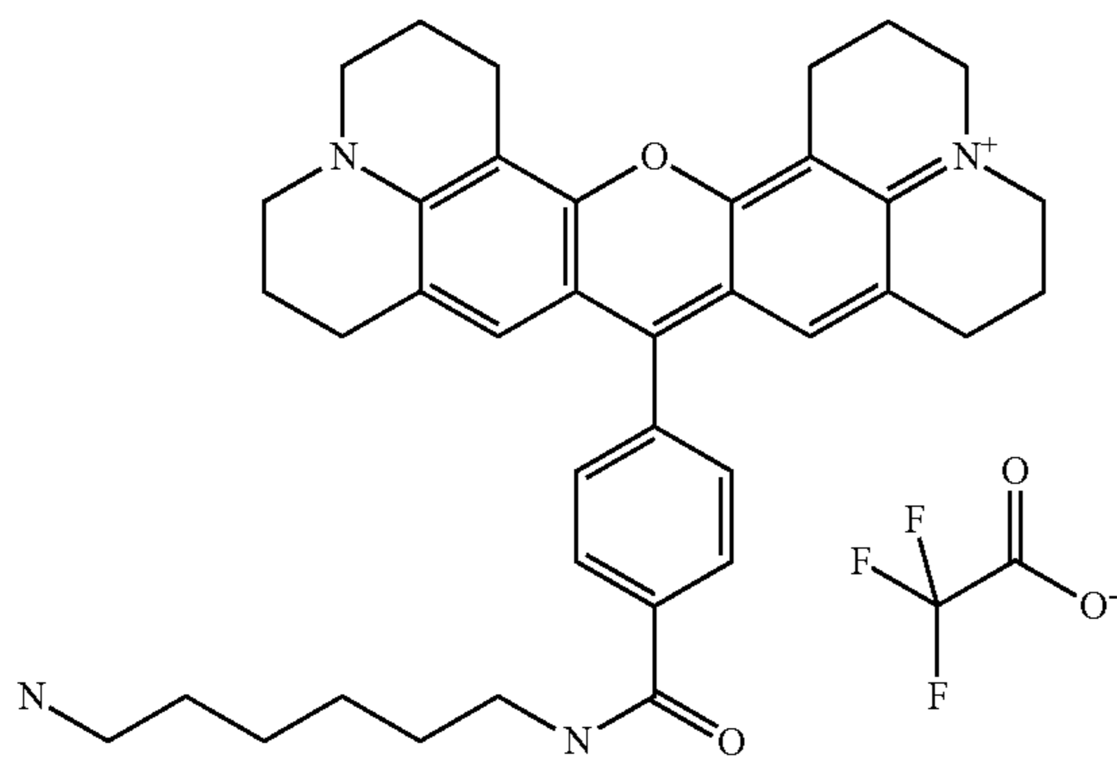
Compound 6
