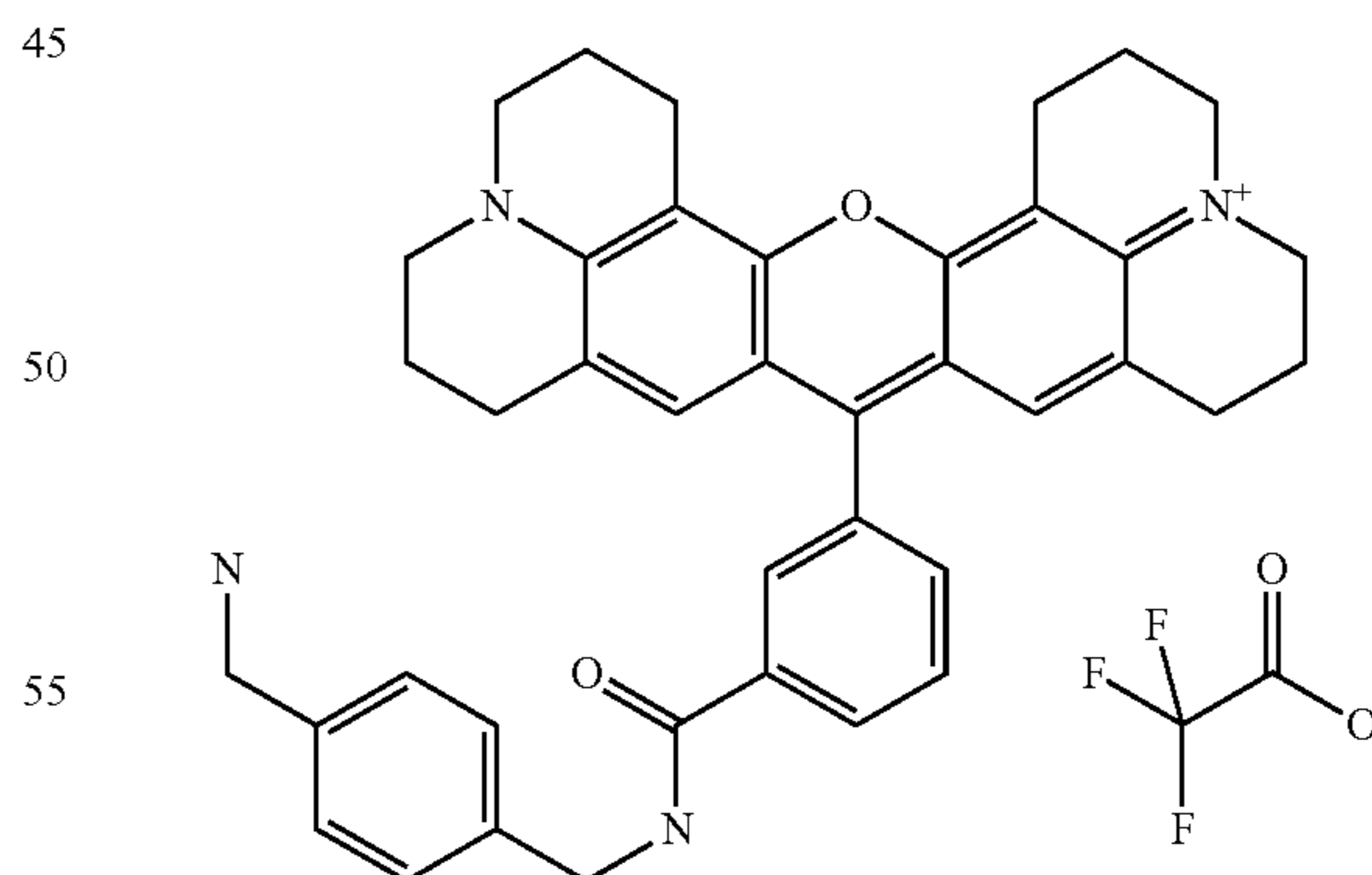
Compound 12
