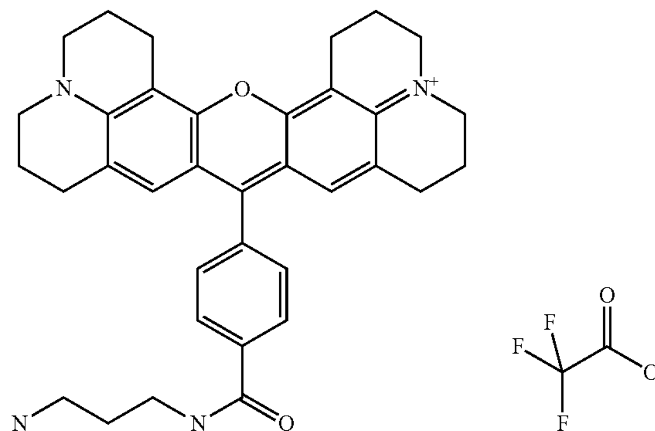
Compound 4
