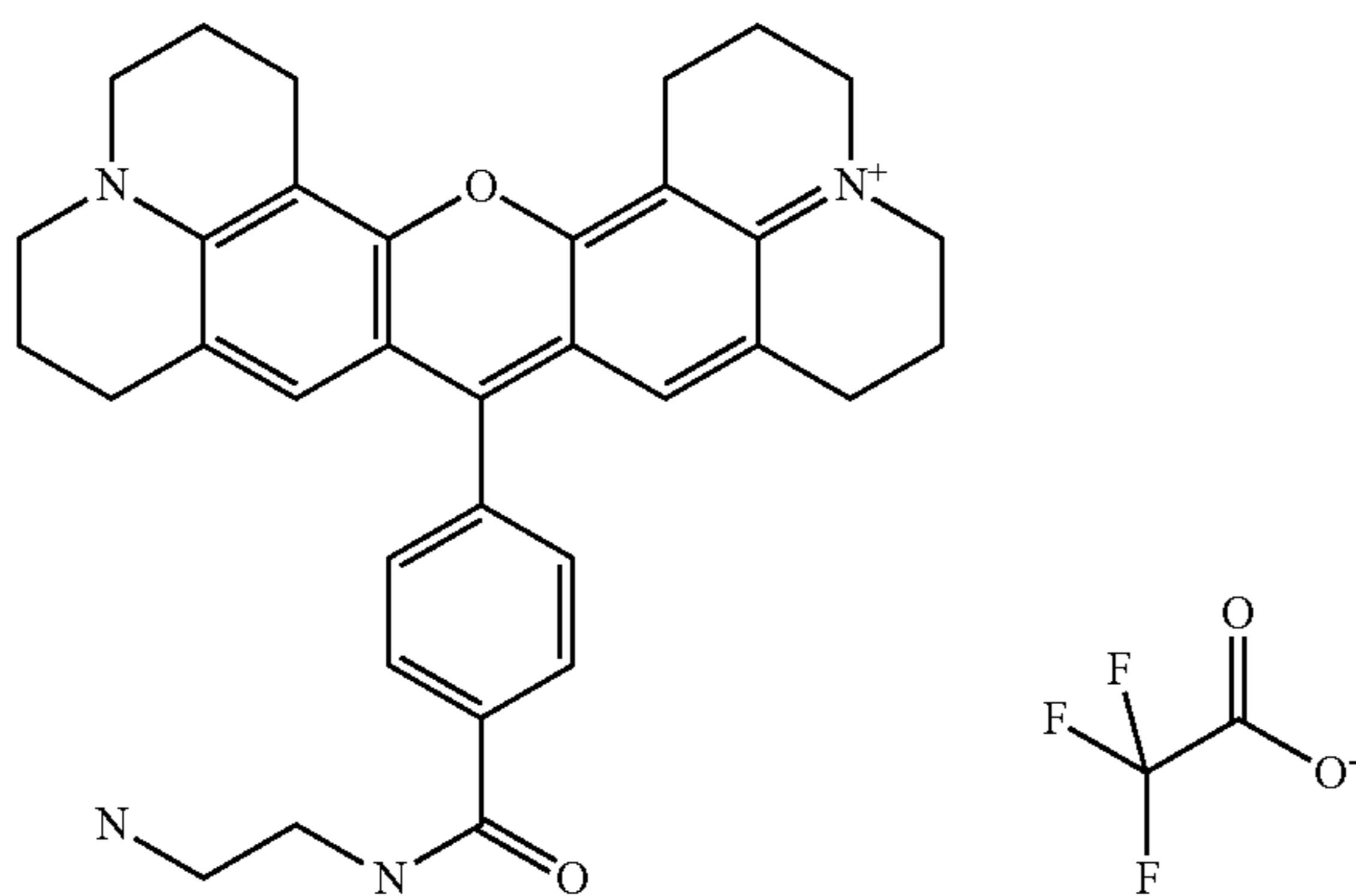
Compound 3
