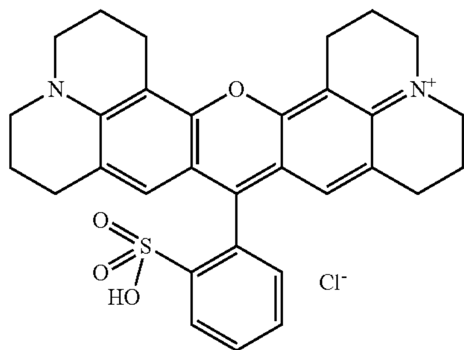
Intermediate 1
