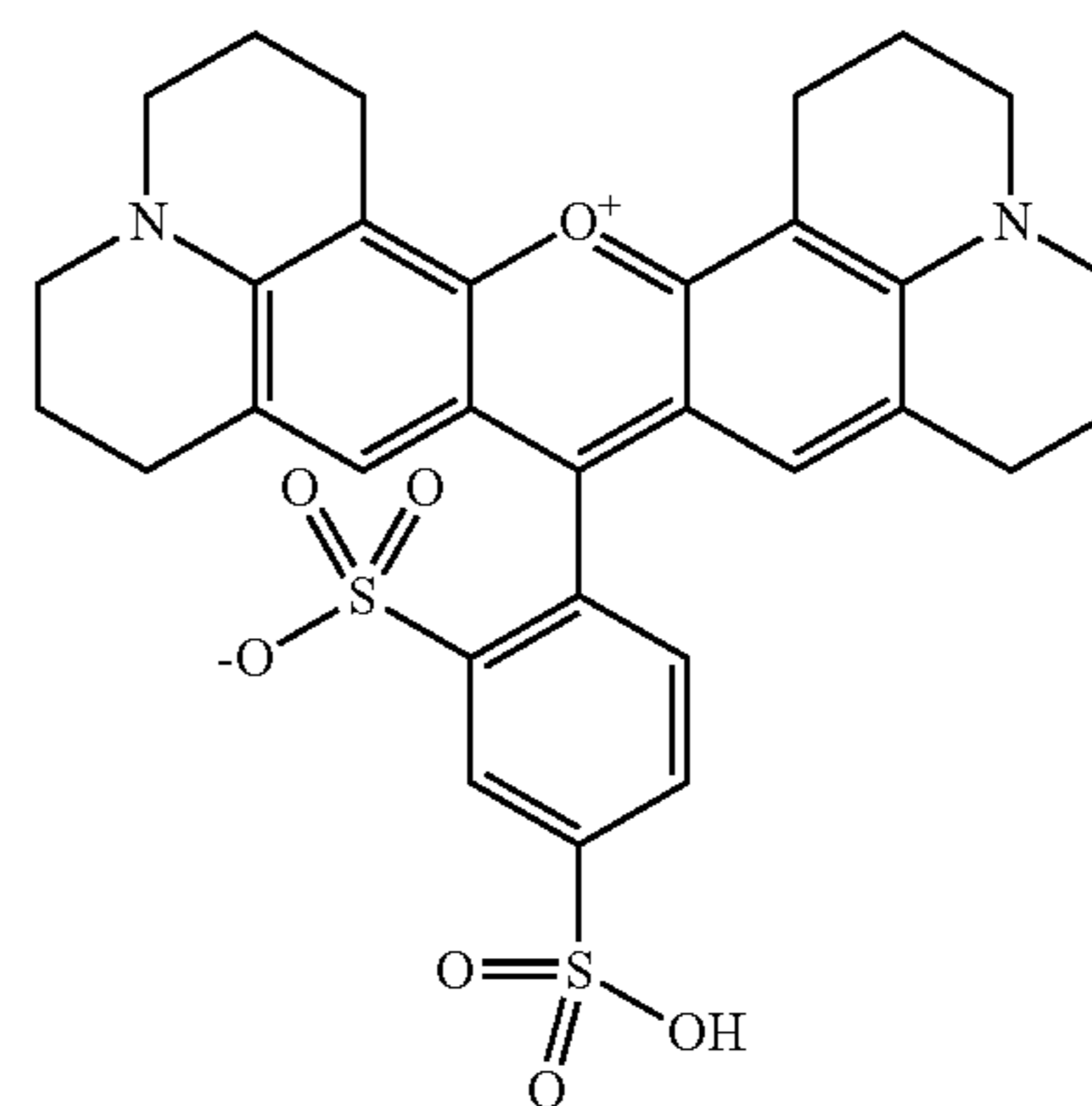
Sulforhodamine 101
