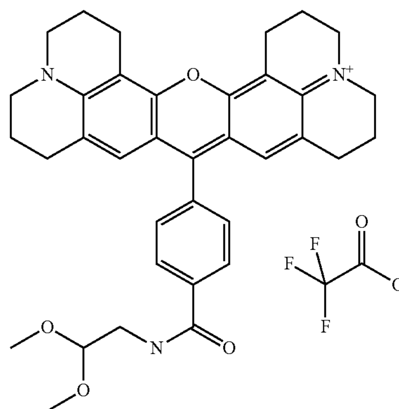
Compound 5
