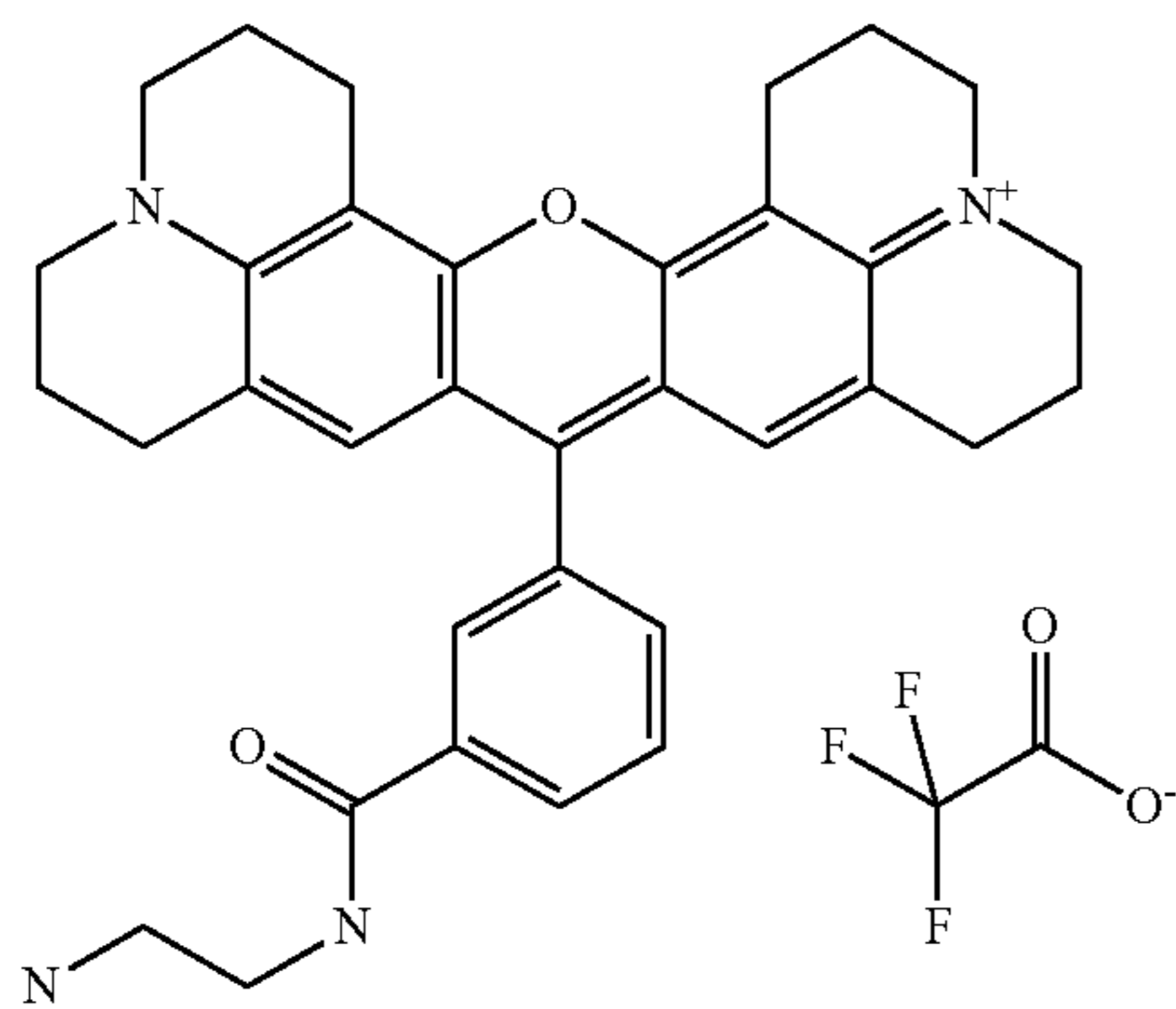
Compound 9
