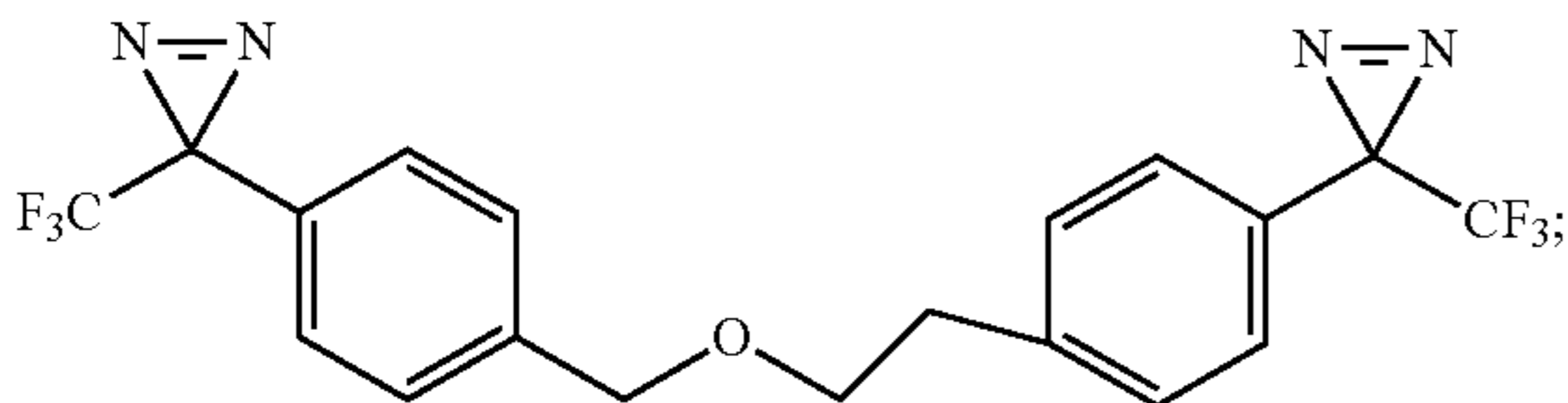
3-(trifluoromethyl)-3-(4-(2-((4-(3-(trifluoromethyl)-3H-diazirin-3-yl)benzyl)oxy)ethyl)phenyl)-3H-diazirine
