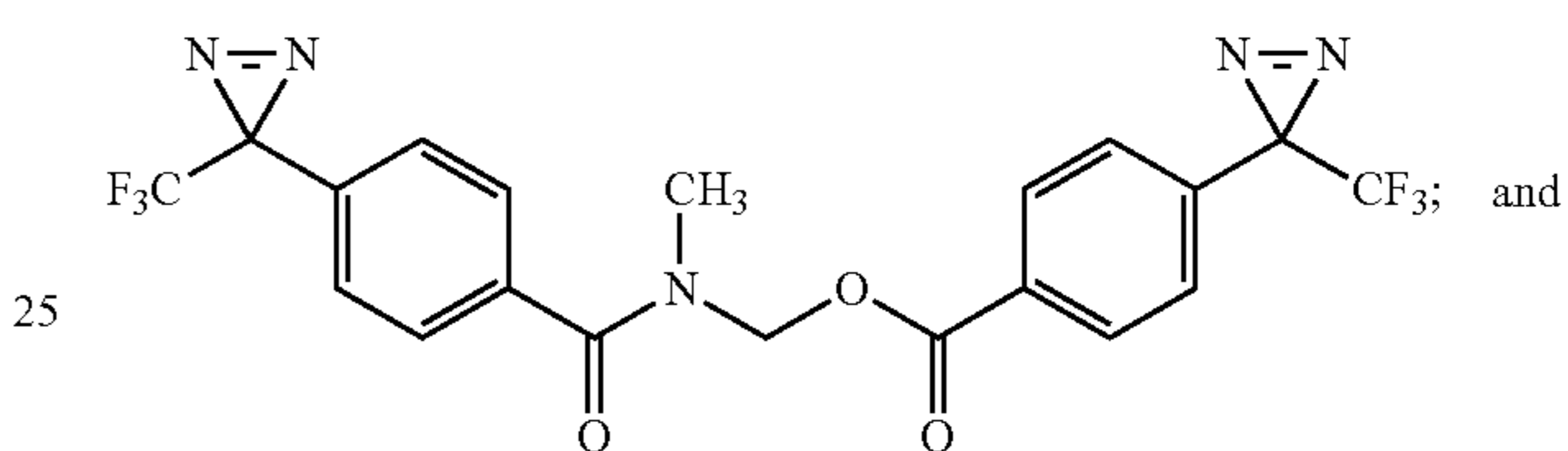
(N-methyl-4-(3-(trifluoromethyl)-3H-diazirin-3-yl)benzamido)methyl 4-(3-(trifluoromethyl)-3H-diazirin-3-yl)benzoate
