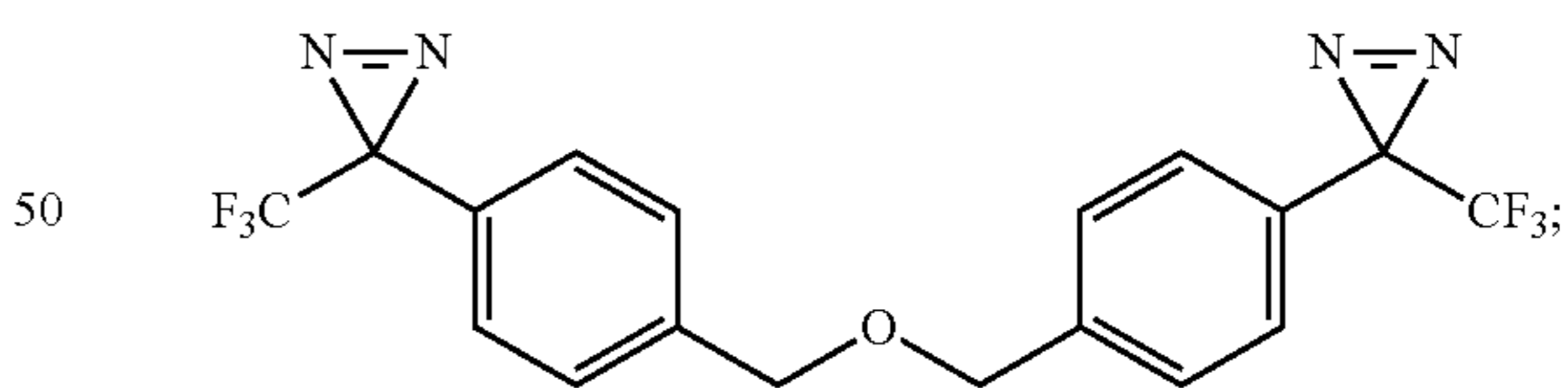
3,3'-((oxybis(methylene))bis(4,1-phenylene))bis(3-(trifluoromethyl)-3H-diazirine)
