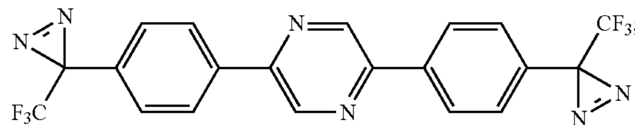
2,5-bis(4-(3-(trifluoromethyl)-3H-diazirin-3-yl)phenyl)pyrazine
