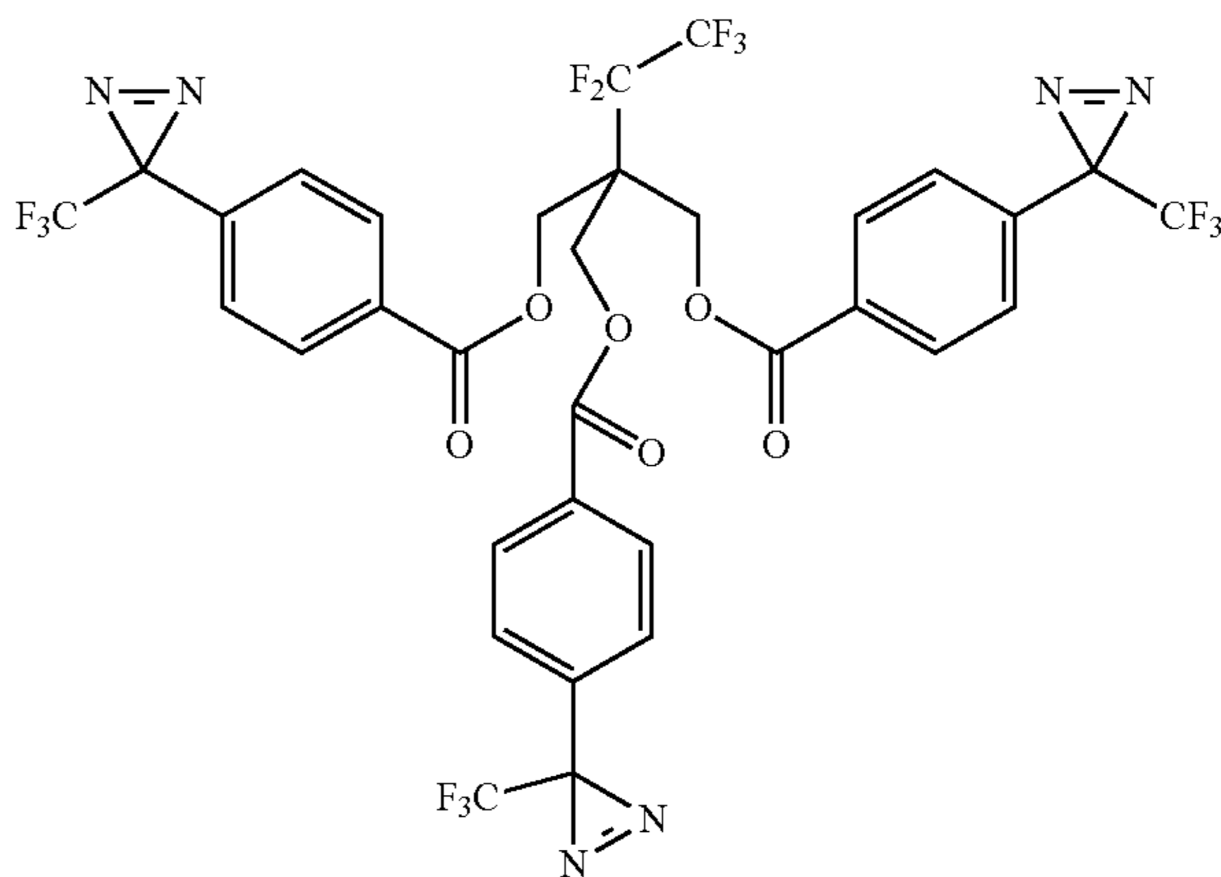
2-(perfluoroethyl)-2-(((4-(3-(trifluoromethyl)-3H-diazirin-3-yl)benzoyl)oxy)methyl)propane-1,3-diyl bis(4-(3-(trifluoromethyl)-3H-diazirin-3-yl)benzoate)
