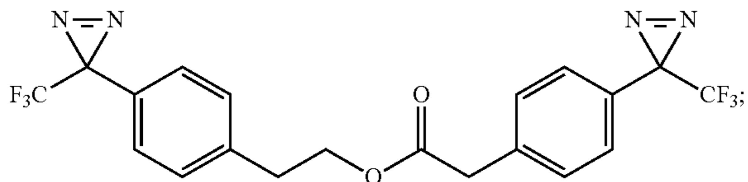
4-(3-(trifluoromethyl)-3H-diazirin-3-yl)phenethyl 2-(4-(3-(trifluoromethyl)-3H-diazirin-3-yl)phenyl)acetate
