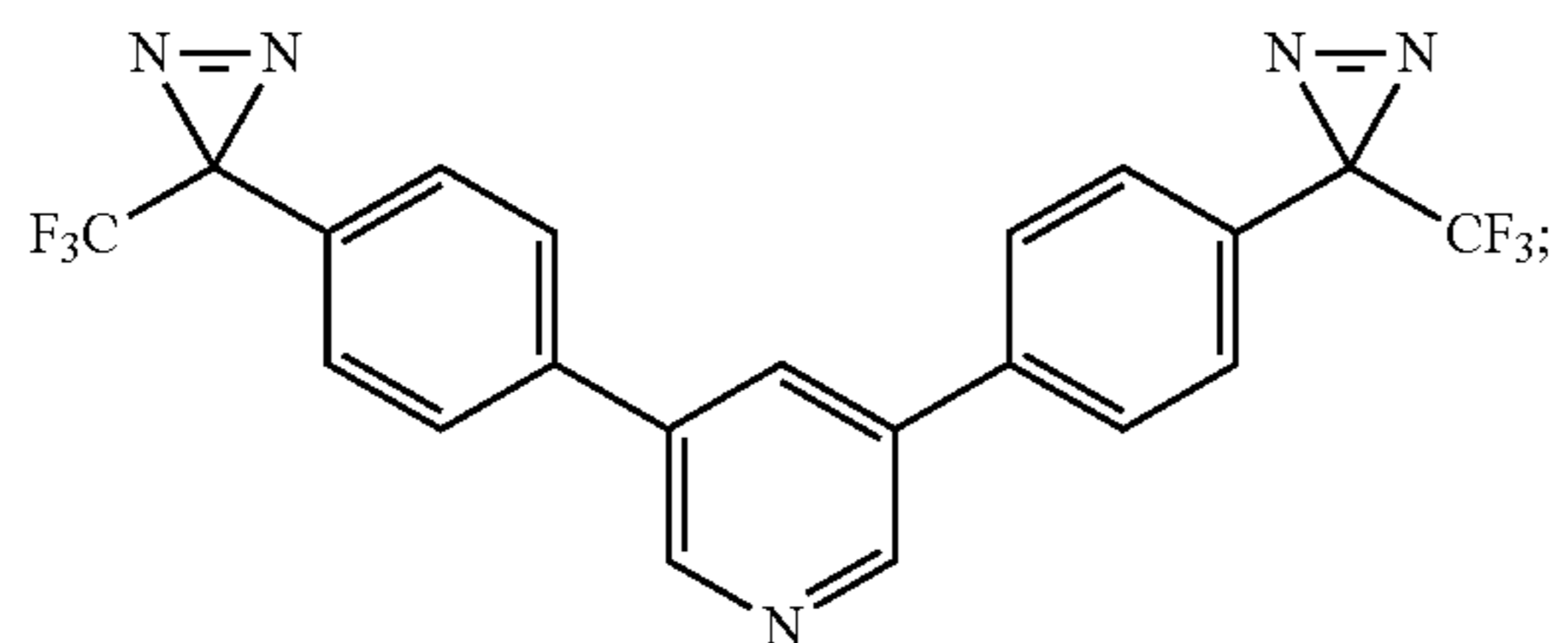
3,5-bis(4-(3-(trifluoromethyl)-3H-diazirin-3-yl)phenyl)pyridine
