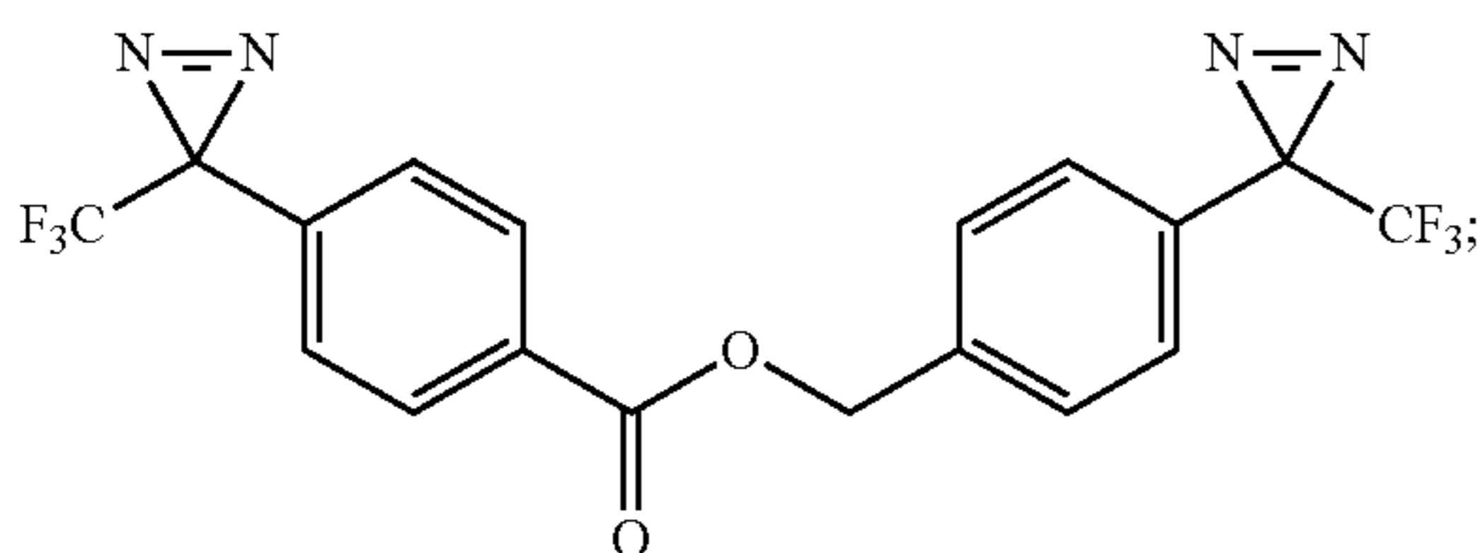
4-(3-(trifluoromethyl)-3H-diazirin-3-yl)benzyl 4-(3-(trifluoromethyl)-3H-diazirin-3-yl)benzoate
