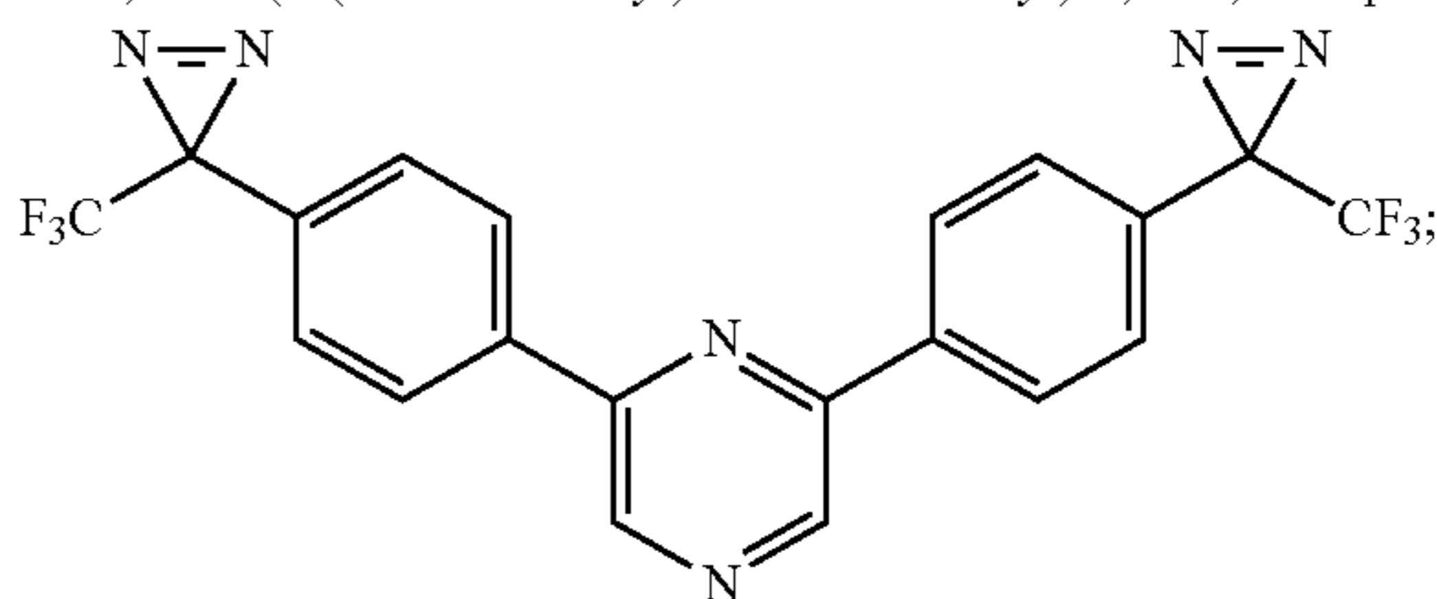
2,6-bis(4-(3-(trifluoromethyl)-3H-diazirin-3-yl)phenyl)pyrazine
