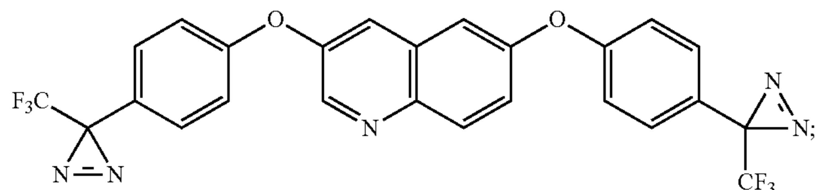
3,6-bis(4-(3-(trifluoromethyl)-3H-diazirin-3-yl)phenoxy)quinoline
