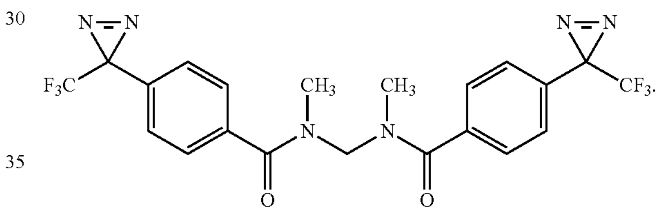
N,N'-methylenebis(N-methyl-4-(3-(trifluoromethyl)-3H-diazirin-3-yl)benzamide)
