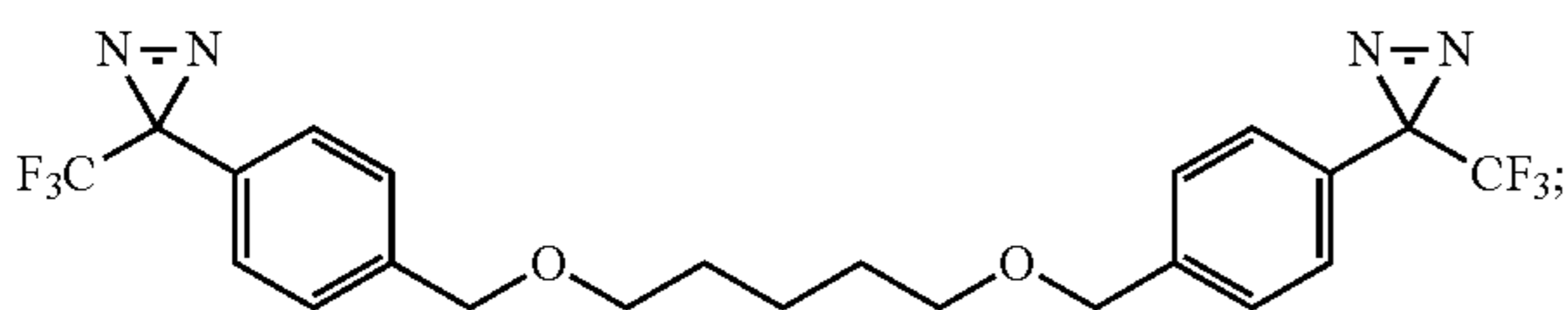
1,5-bis((4-(3-(trifluoromethyl)-3H-diazirin-3-yl)benzyl)oxy)pentane
