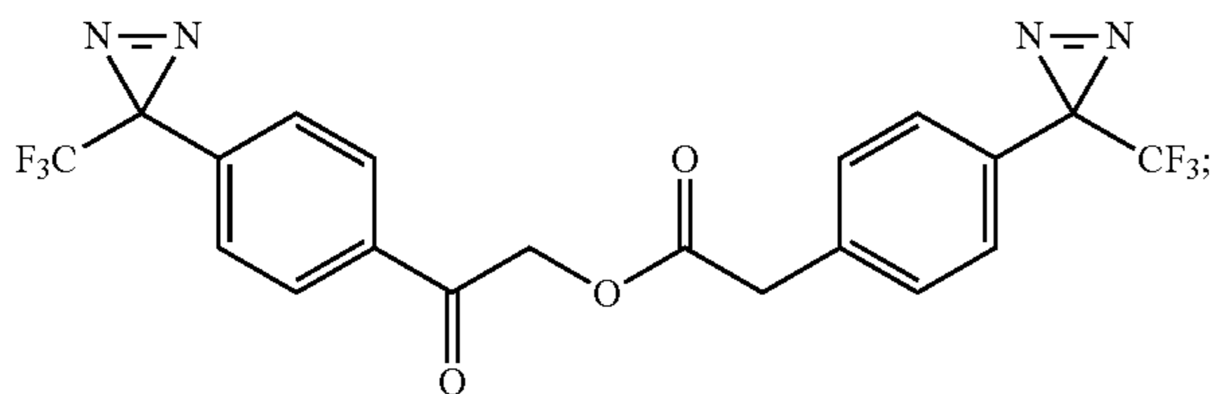
2-oxo-2-(4-(3-(trifluoromethyl)-3H-diazirin-3-yl)phenyl)ethyl 3-(3-(trifluoromethyl)-3H-diazirin-3-yl)benzoate
