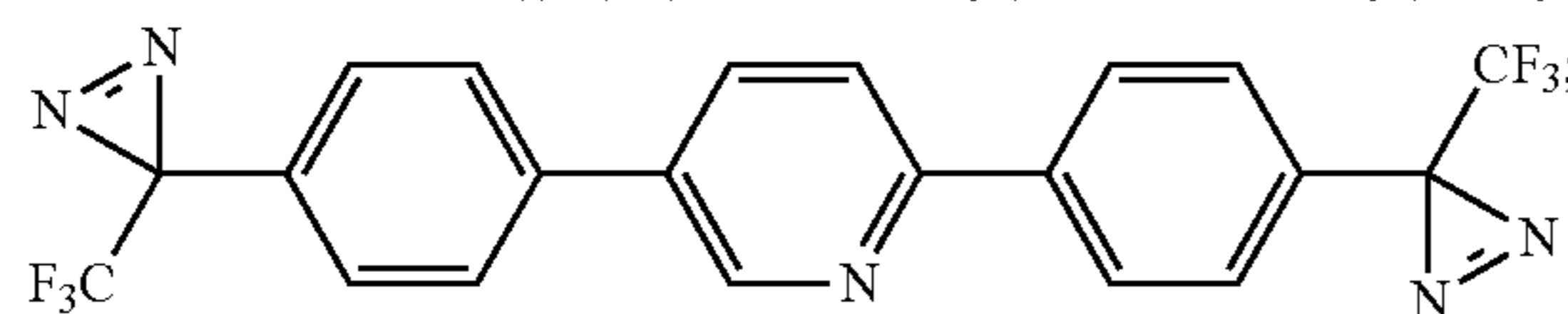
2,5-bis(4-(3-(trifluoromethyl)-3H-diazirin-3-yl)phenyl)pyridine
