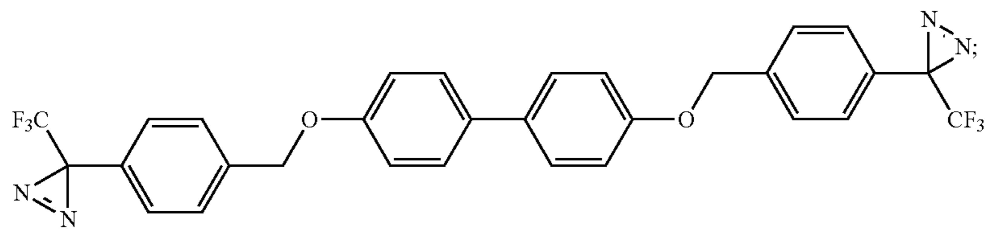
4,4'-bis((4-(3-(trifluoromethyl)-3H-diazirin-3-yl)benzyl)oxy)-1,1'-biphenyl
