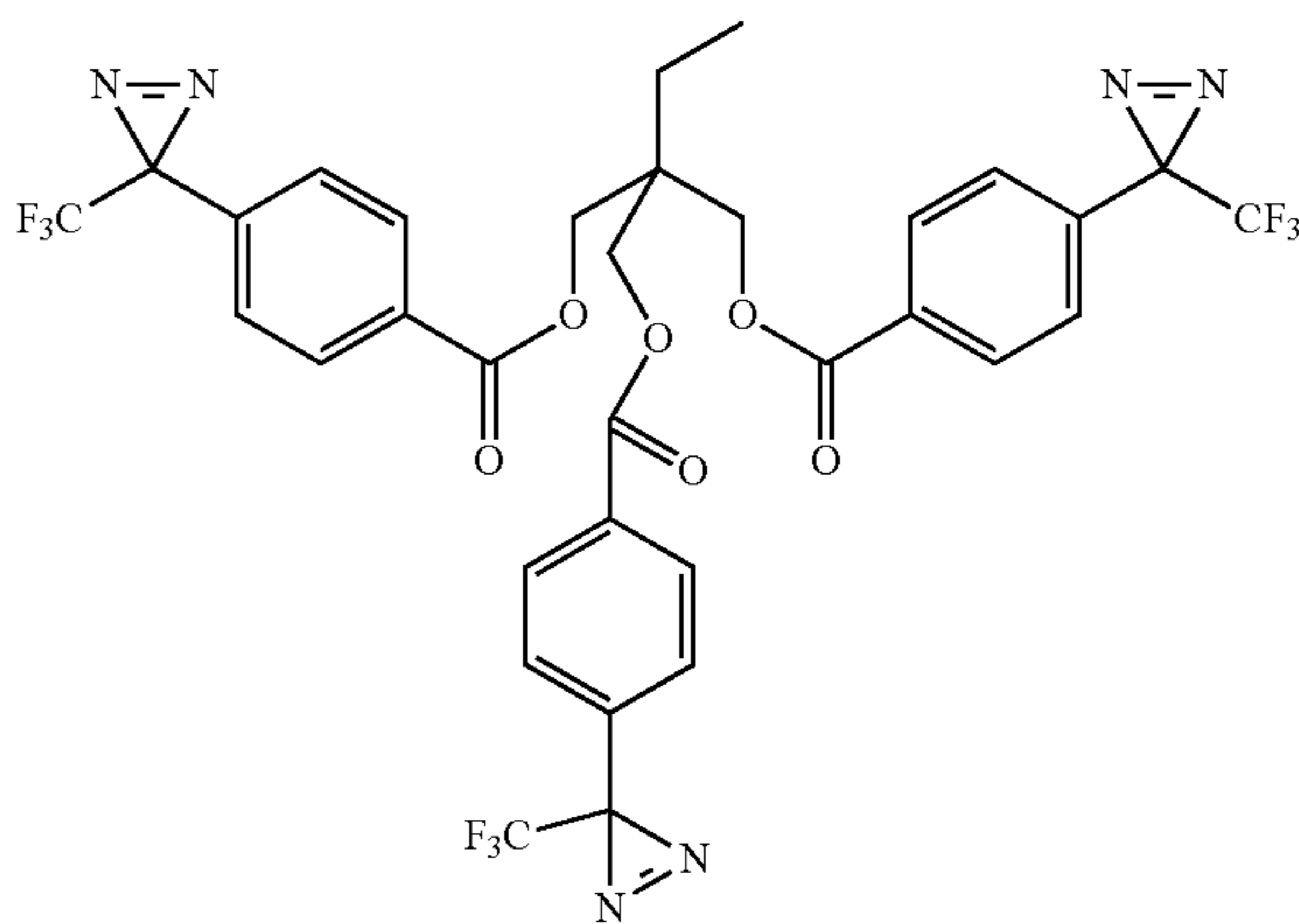
2-ethyl-2-(((4-(3-(trifluoromethyl)-3H-diazirin-3-yl)benzoyl)oxy)methyl)propane-1,3-diyl bis(4-(3-(trifluoromethyl)-3H-diazirin-3-yl)benzoate)
