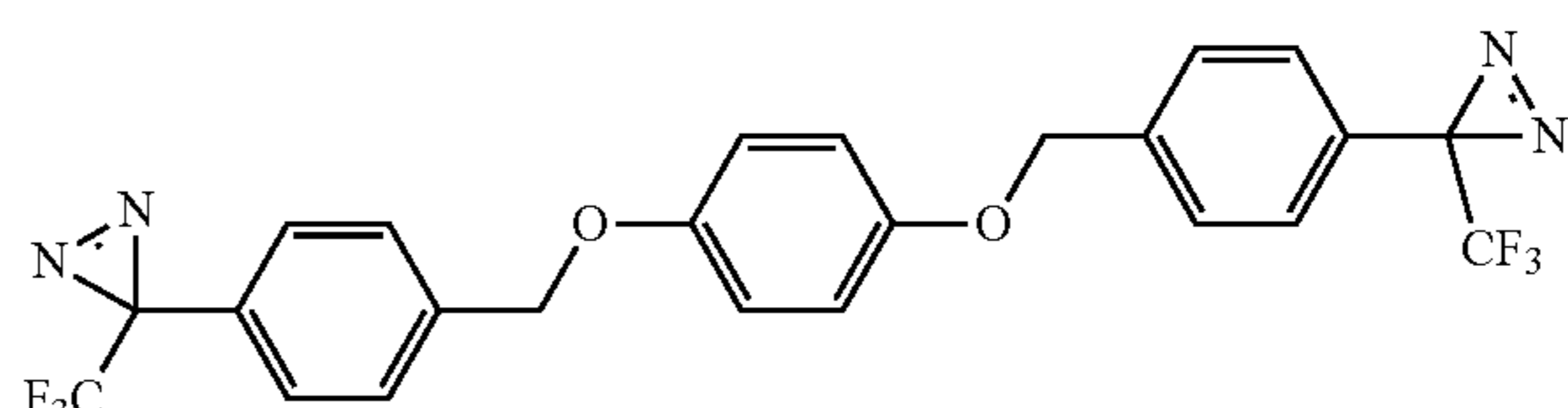
1,4-bis((4-(3-(trifluoromethyl)-3H-diazirin-3-yl)benzyl)oxy)benzene
