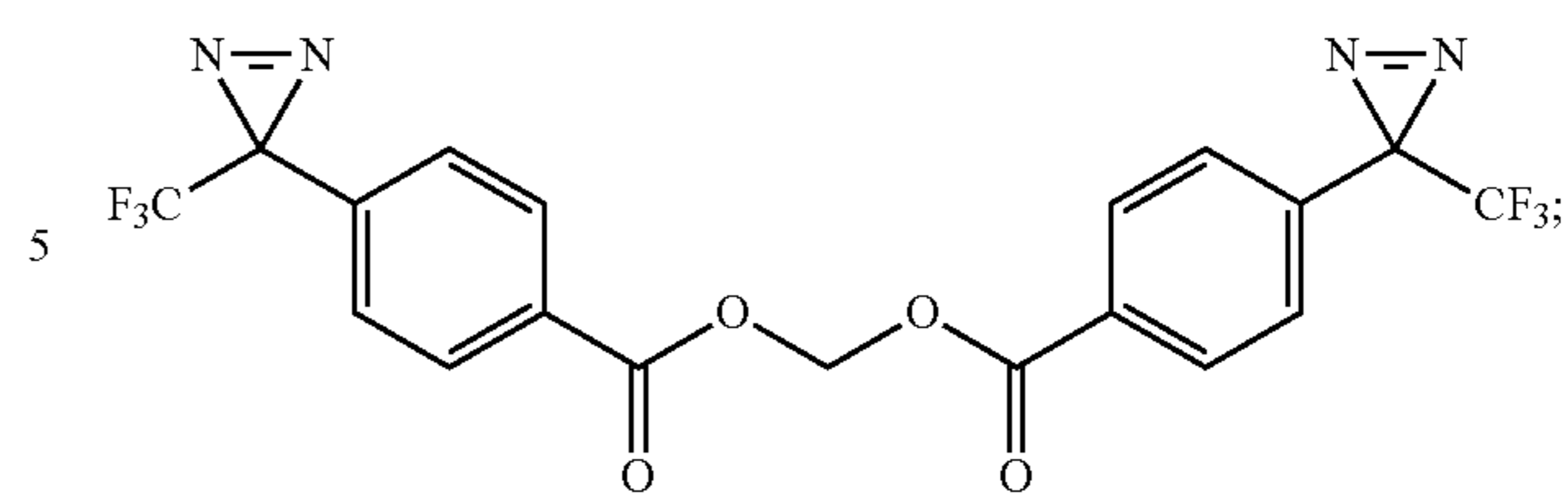
methylene bis(4-(3-(trifluoromethyl)-3H-diazirin-3-yl)benzoate)
