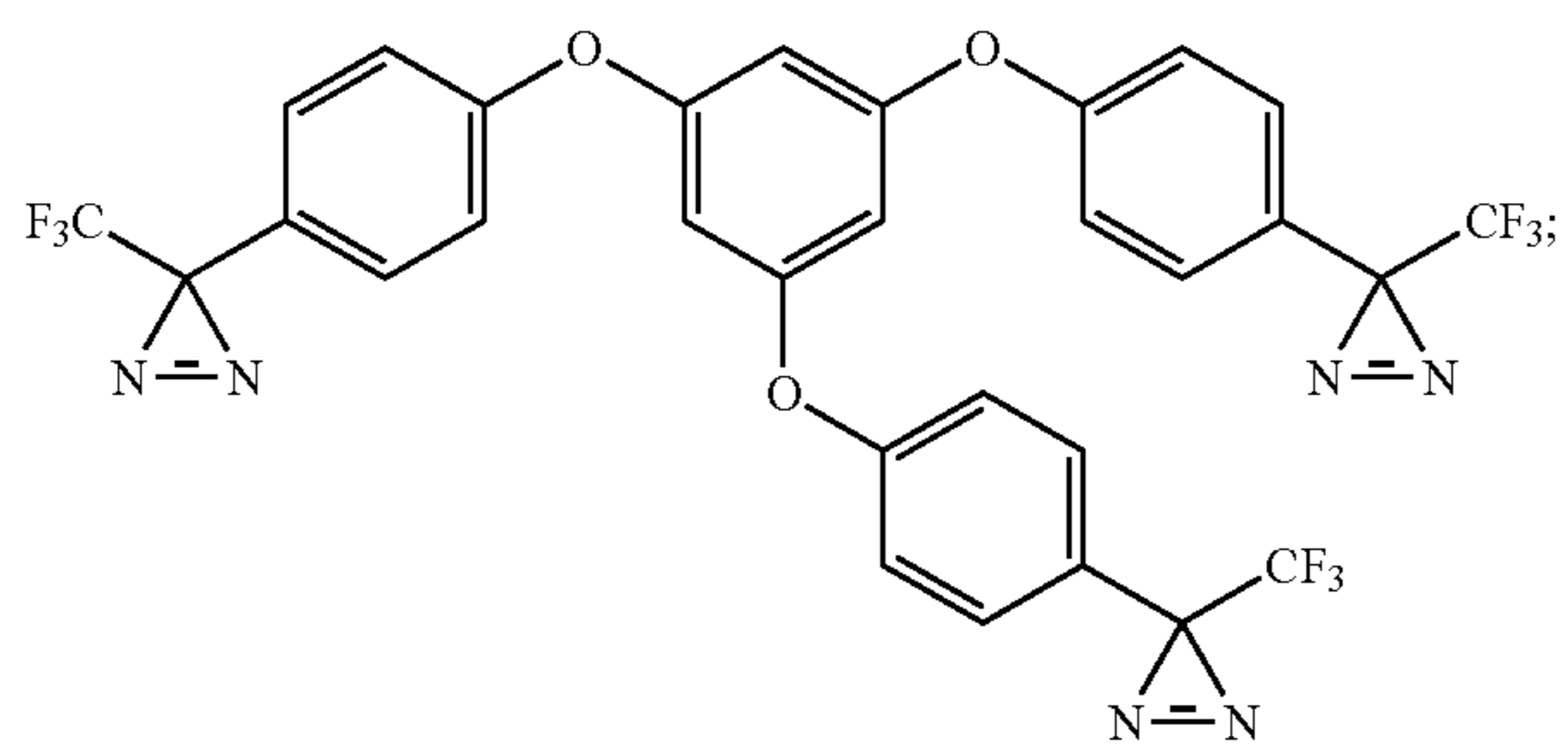
1,3,5-tris(4-(3-(trifluoromethyl)-3H-diazirin-3-yl)phenoxy)benzene
