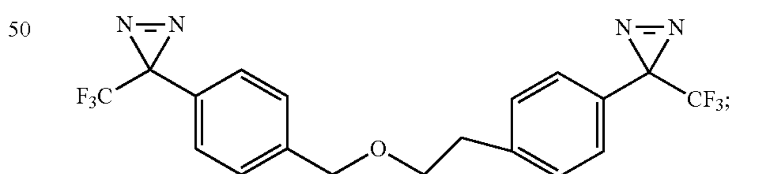
3-(trifluoromethyl)-3-(4-(2-((4-(3-(trifluoromethyl)-3H-diazirin-3-yl)benzyl)oxy)ethyl)phenyl)-3H-diazirine
