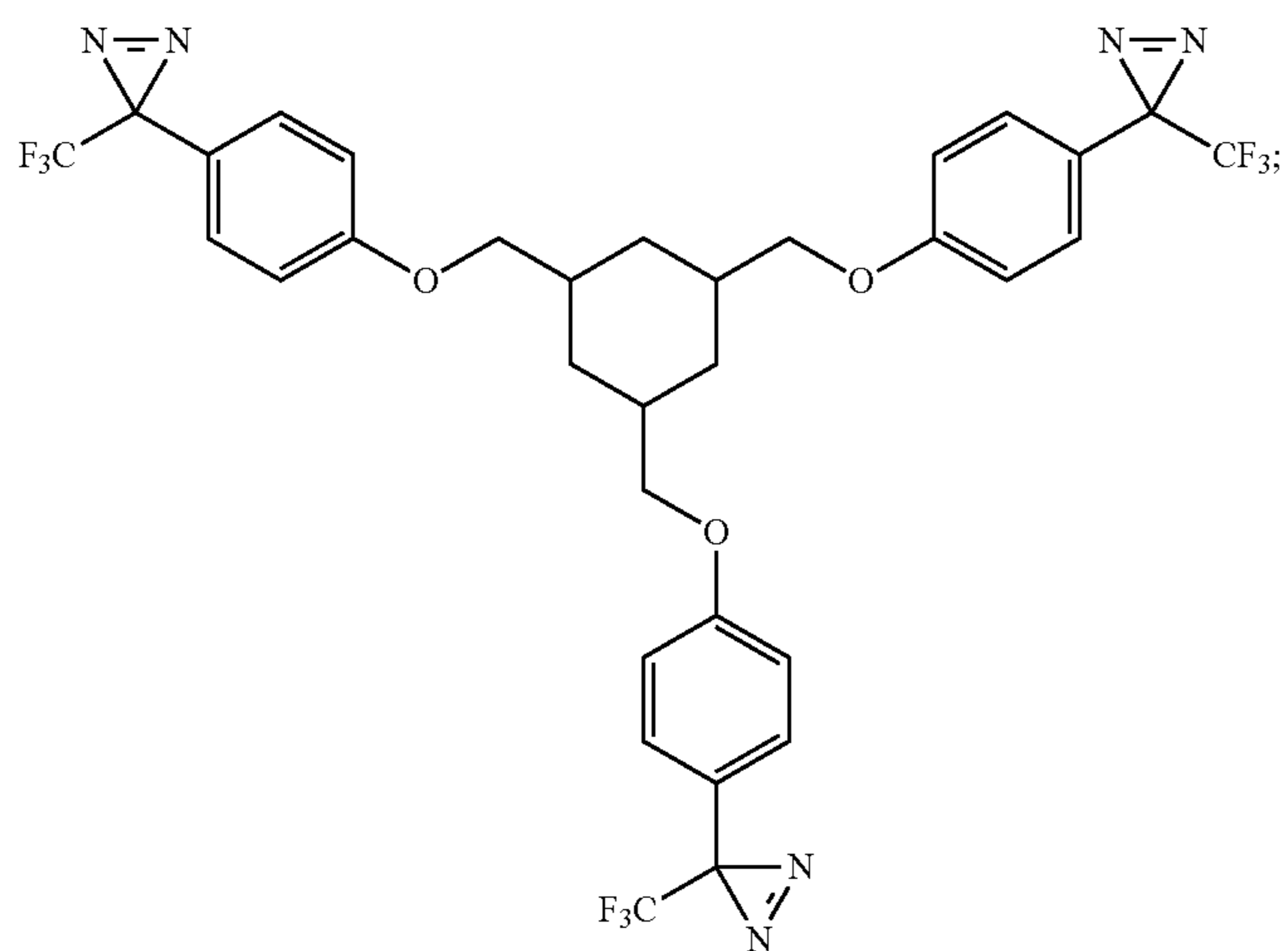
1,3,5-tris((4-(3-(trifluoromethyl)-3H-diazirin-3-yl)phenoxy)methyl)cyclohexane
