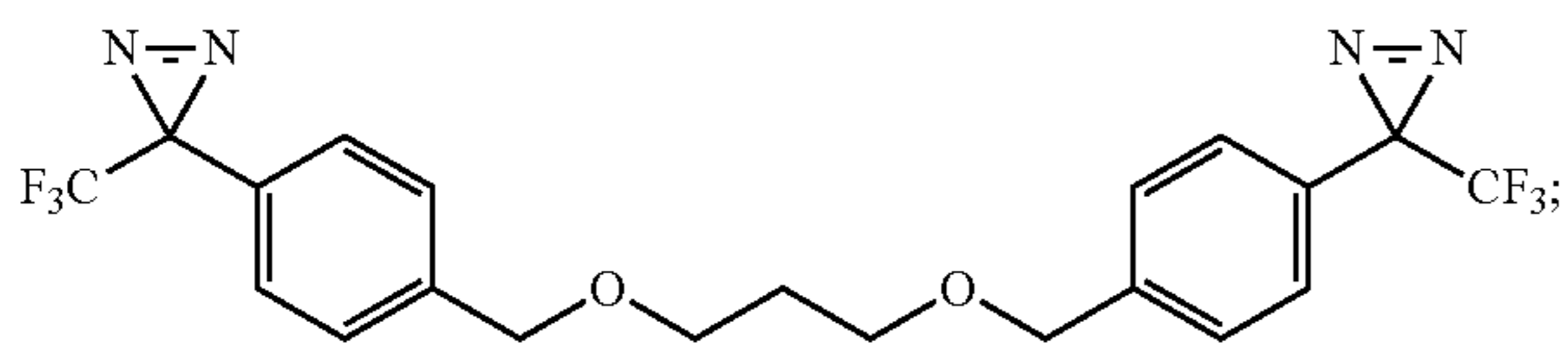
1,3-bis((4-(3-(trifluoromethyl)-3H-diazirin-3-yl)benzyl)oxy)propane
