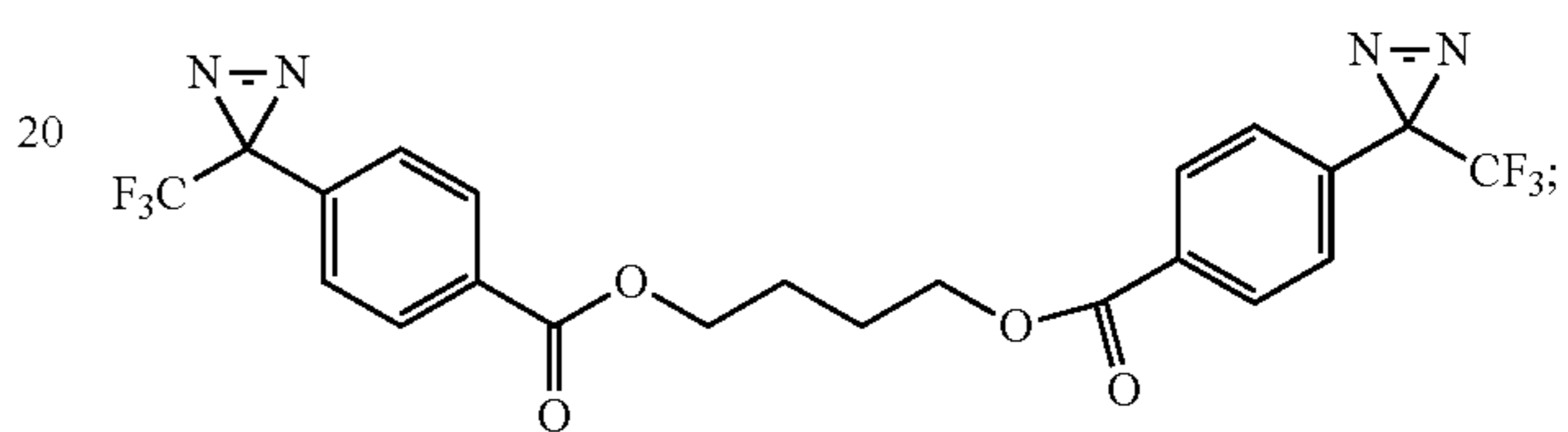
butane-1,4-diyl bis(4-(3-(trifluoromethyl)-3H-diazirin-3-yl)benzoate)
