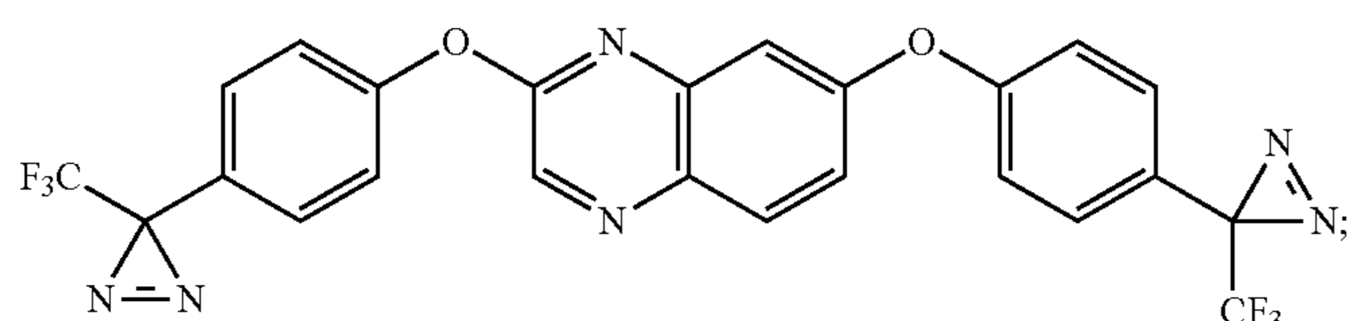
2,7-bis(4-(3-(trifluoromethyl)-3H-diazirin-3-yl)phenoxy)quinoxaline
