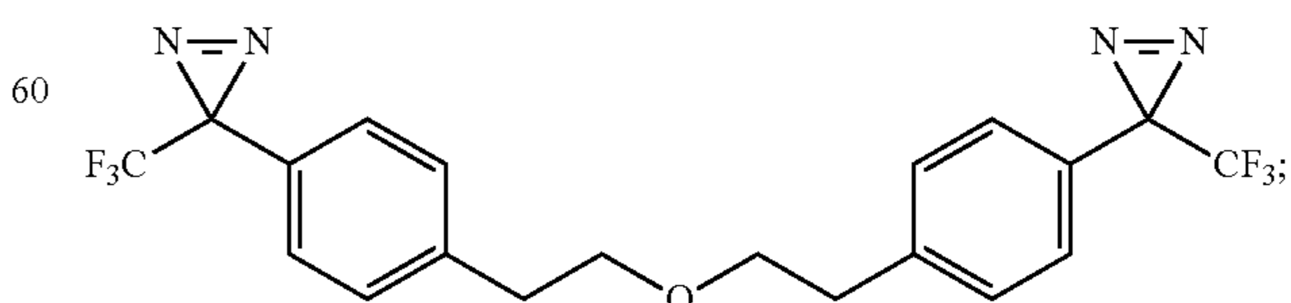
3,3'-((oxybis(ethane-2,1-diyl))bis(4,1-phenylene))bis(3-(trifluoromethyl)-3H-diazirine)
