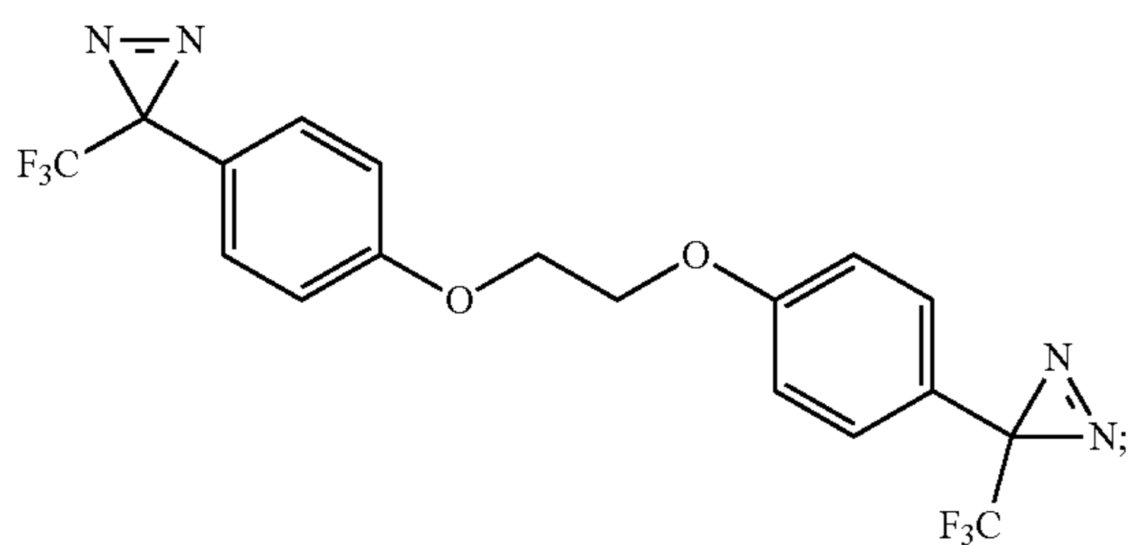
1,2-bis(4-(3-(trifluoromethyl)-3H-diazirin-3-yl)phenoxy)ethane
