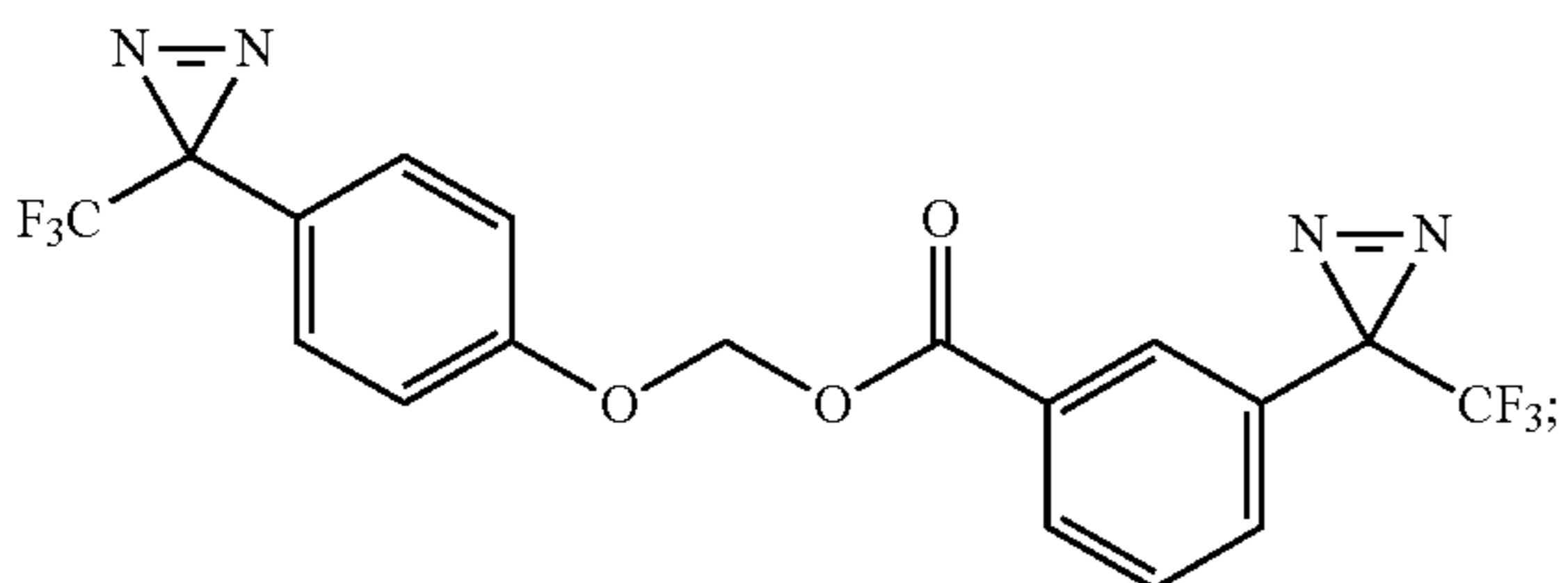
(4-(3-(trifluoromethyl)-3H-diazirin-3-yl)phenoxy)methyl 3-(3-(trifluoromethyl)-3H-diazirin-3-yl)benzoate
