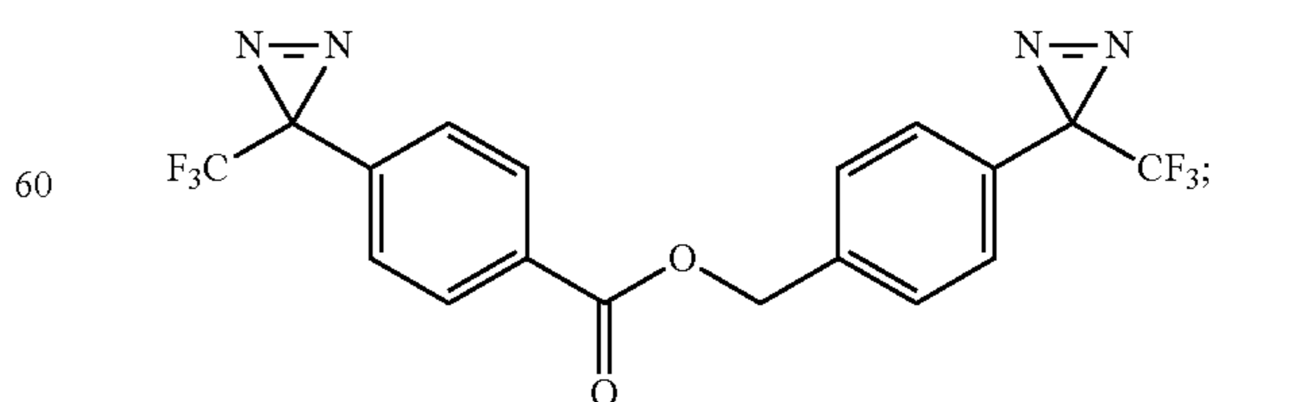
4-(3-(trifluoromethyl)-3H-diazirin-3-yl)benzyl 4-(3-(trifluoromethyl)-3H-diazirin-3-yl)benzoate
