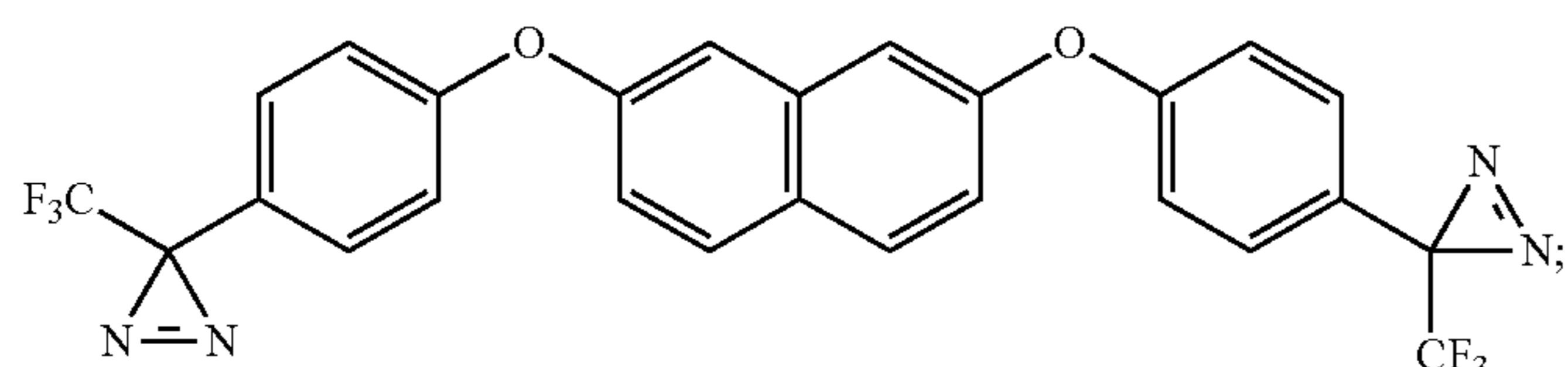
2,7-bis(4-(3-(trifluoromethyl)-3H-diazirin-3-yl)phenoxy)naphthalene
