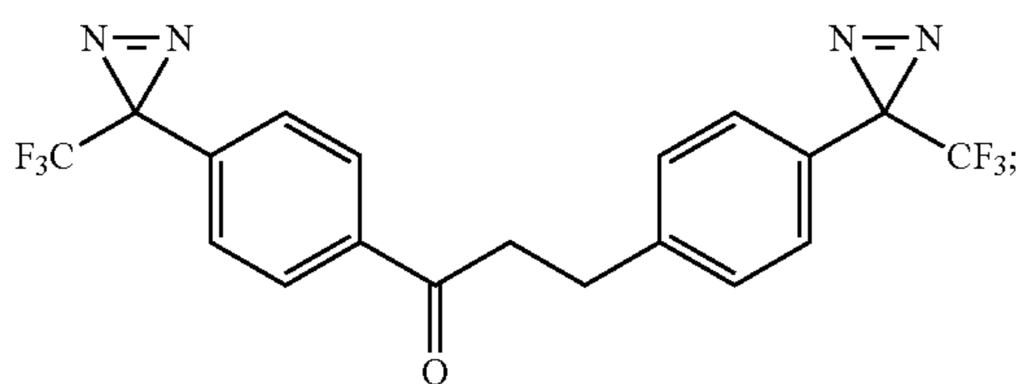
1,3-bis(4-(3-(trifluoromethyl)-3H-diazirin-3-yl)phenyl)propan-1-one
