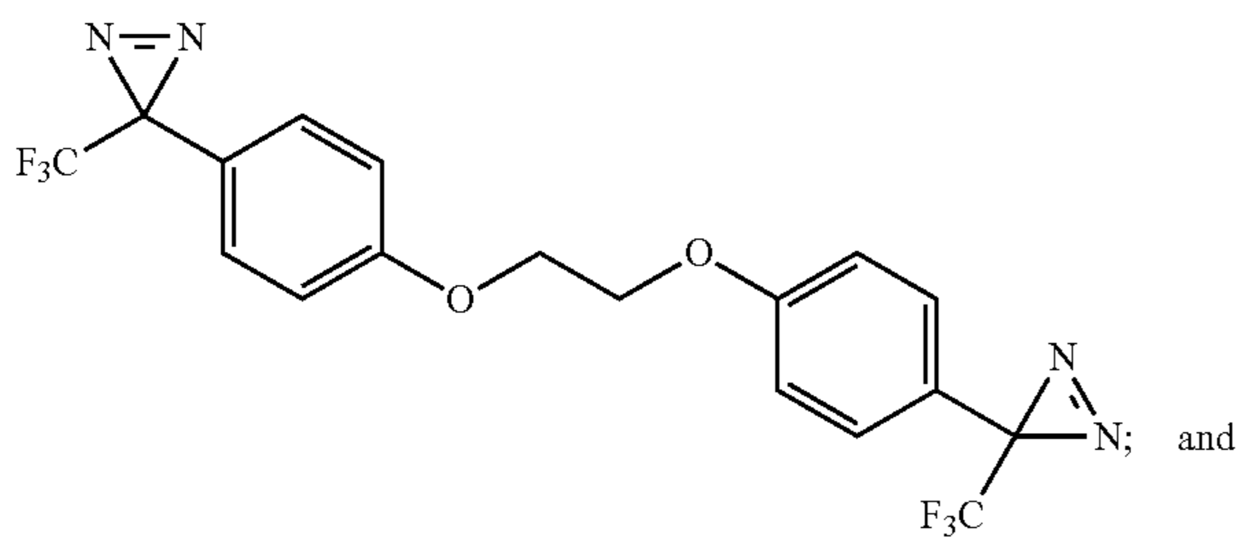
1,2-bis(4-(3-(trifluoromethyl)-3H-diazirin-3-yl)phenoxy)ethane
