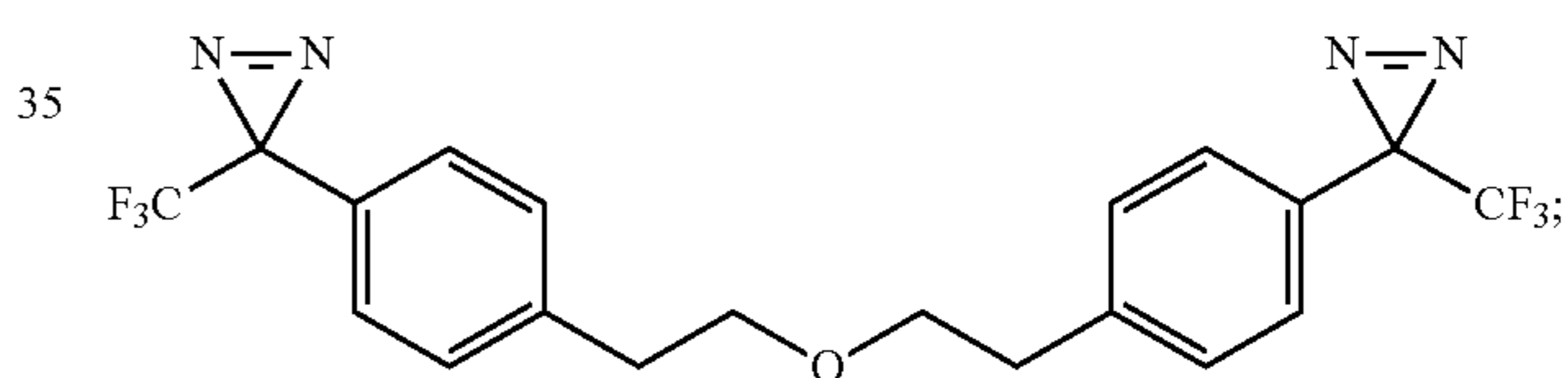
3,3'-((oxybis(ethane-2,1-diyl))bis(4,1-phenylene))bis(3-(trifluoromethyl)-3H-diazirine)
