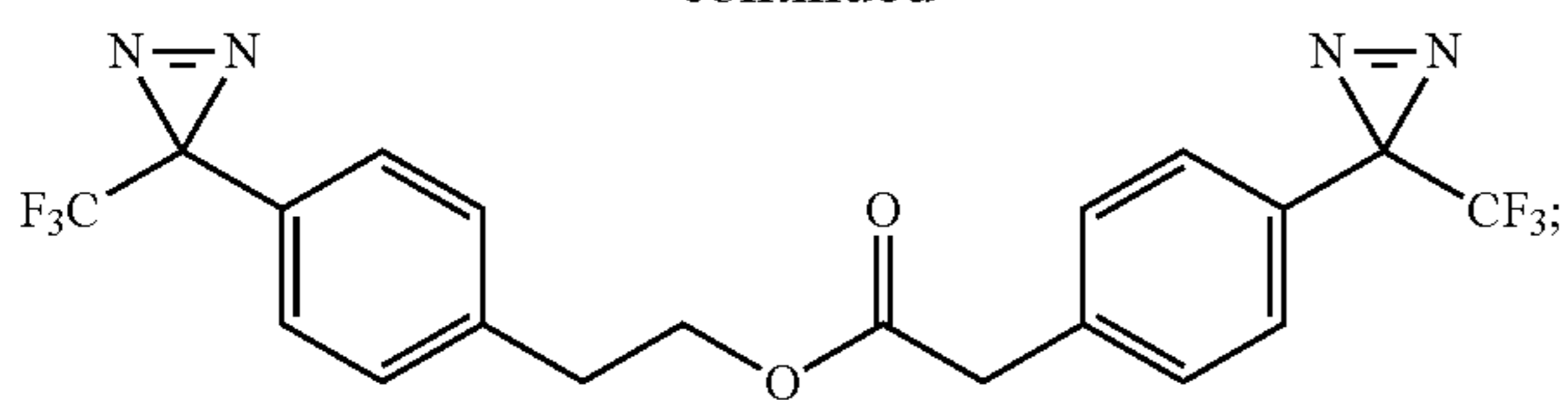
4-(3-(trifluoromethyl)-3H-diazirin-3-yl)phenethyl 2-(4-(3-(trifluoromethyl)-3H-diazirin-3-yl)phenyl)acetate
