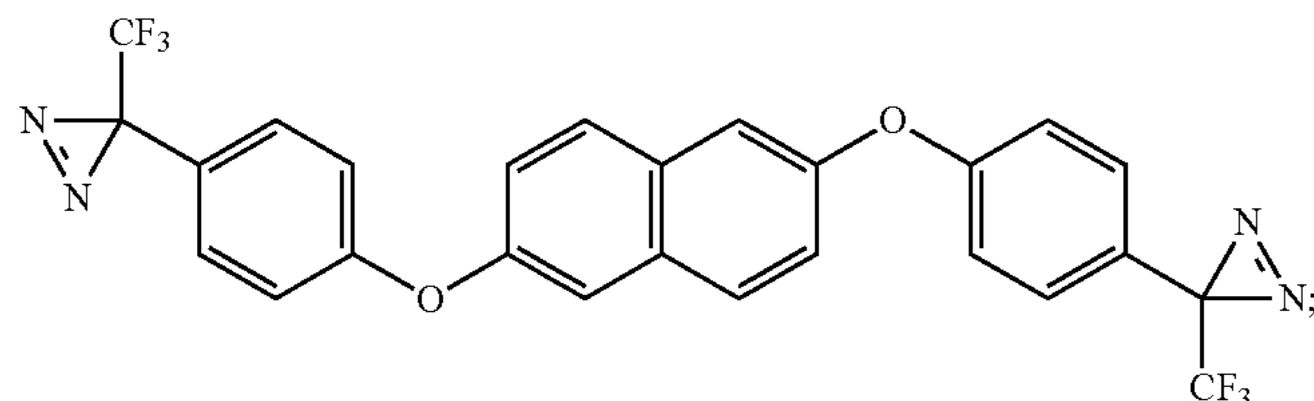
2,6-bis(4-(3-(trifluoromethyl)-3H-diazirin-3-yl)phenoxy)naphthalene
