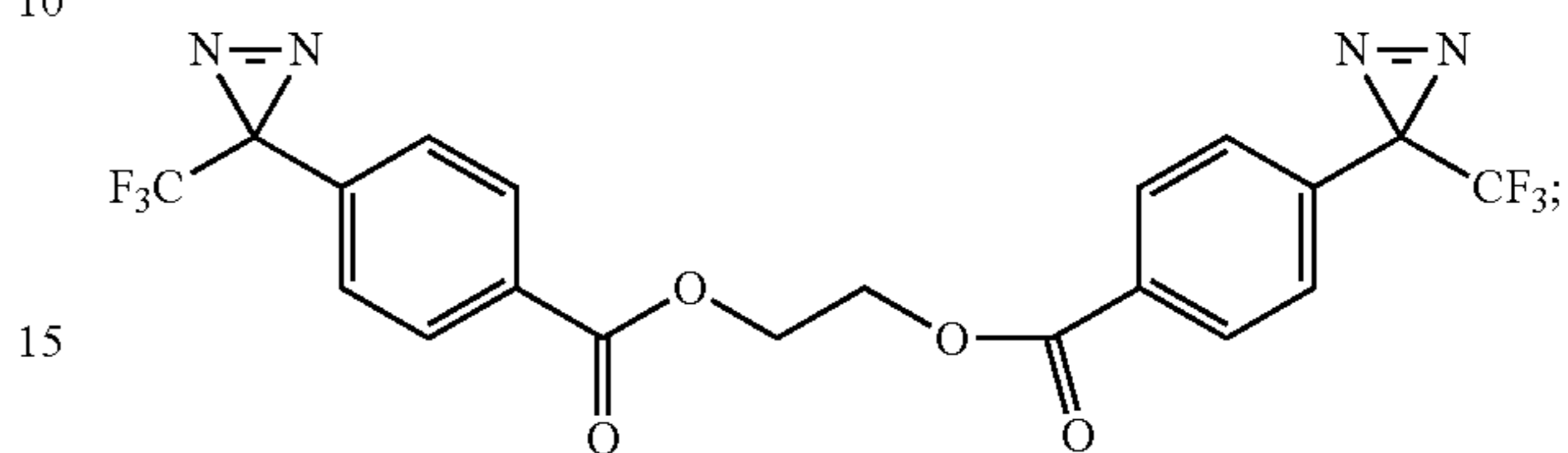
ethane-1,2-diyl bis(4-(3-(trifluoromethyl)-3H-diazirin-3-yl)benzoate)
