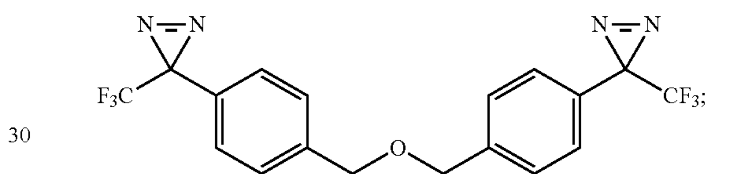
3,3'-((oxybis(methylene))bis(4,1-phenylene))bis(3-(trifluoromethyl)-3H-diazirine)
