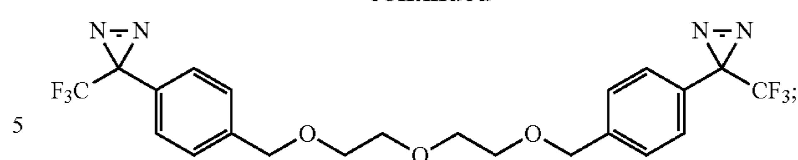
3,3'-((((oxybis(ethane-2,1-diyl))bis(oxy))bis(methylene))bis(4,1-phenylene))bis(3-(trifluoromethyl)-3H-diazirine)
