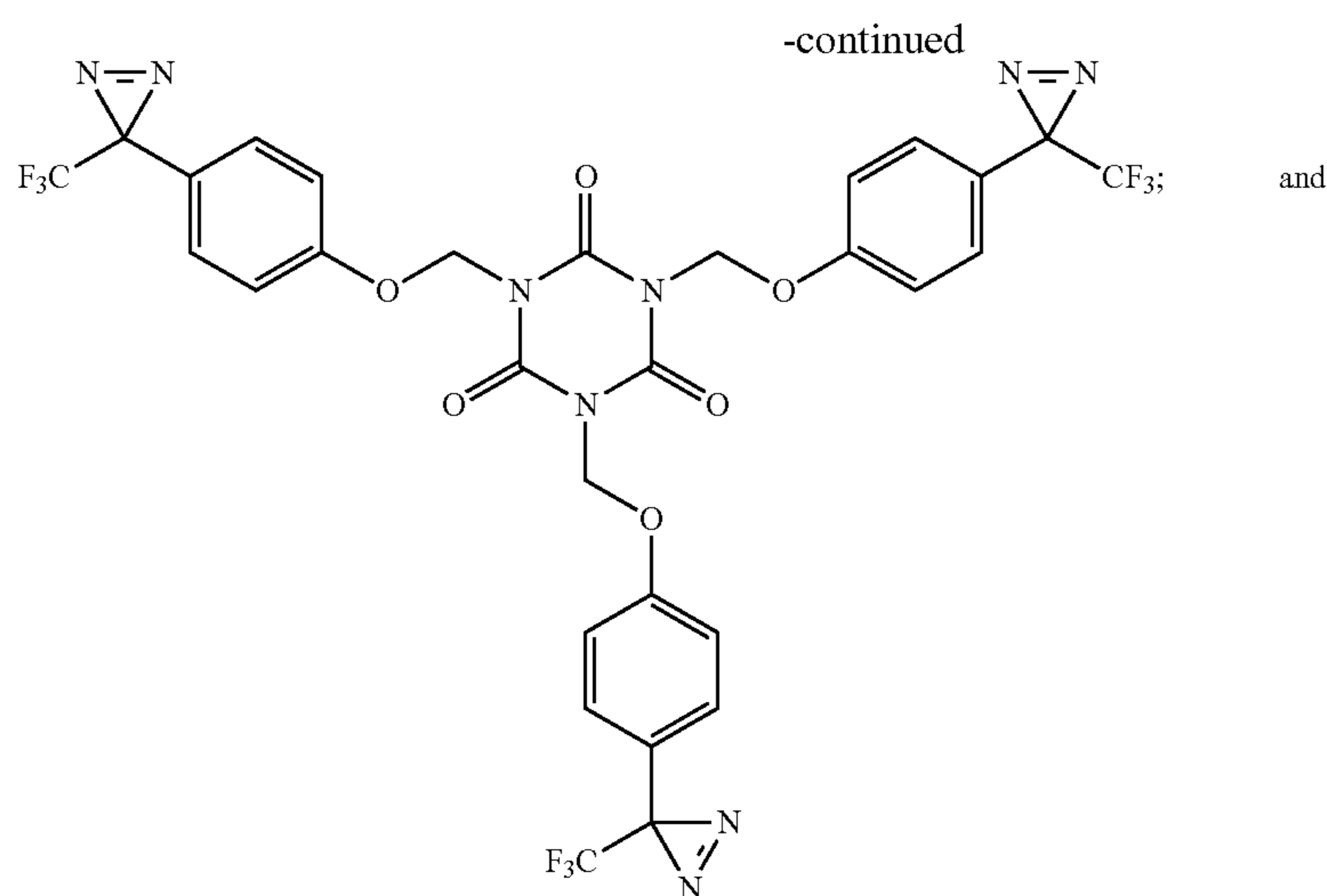
1,3,5-tris((4-(3-(trifluoromethyl)-3H-diazirin-3-yl)phenoxy)methyl)-1,3,5-triazinane-2,4,6-trione
