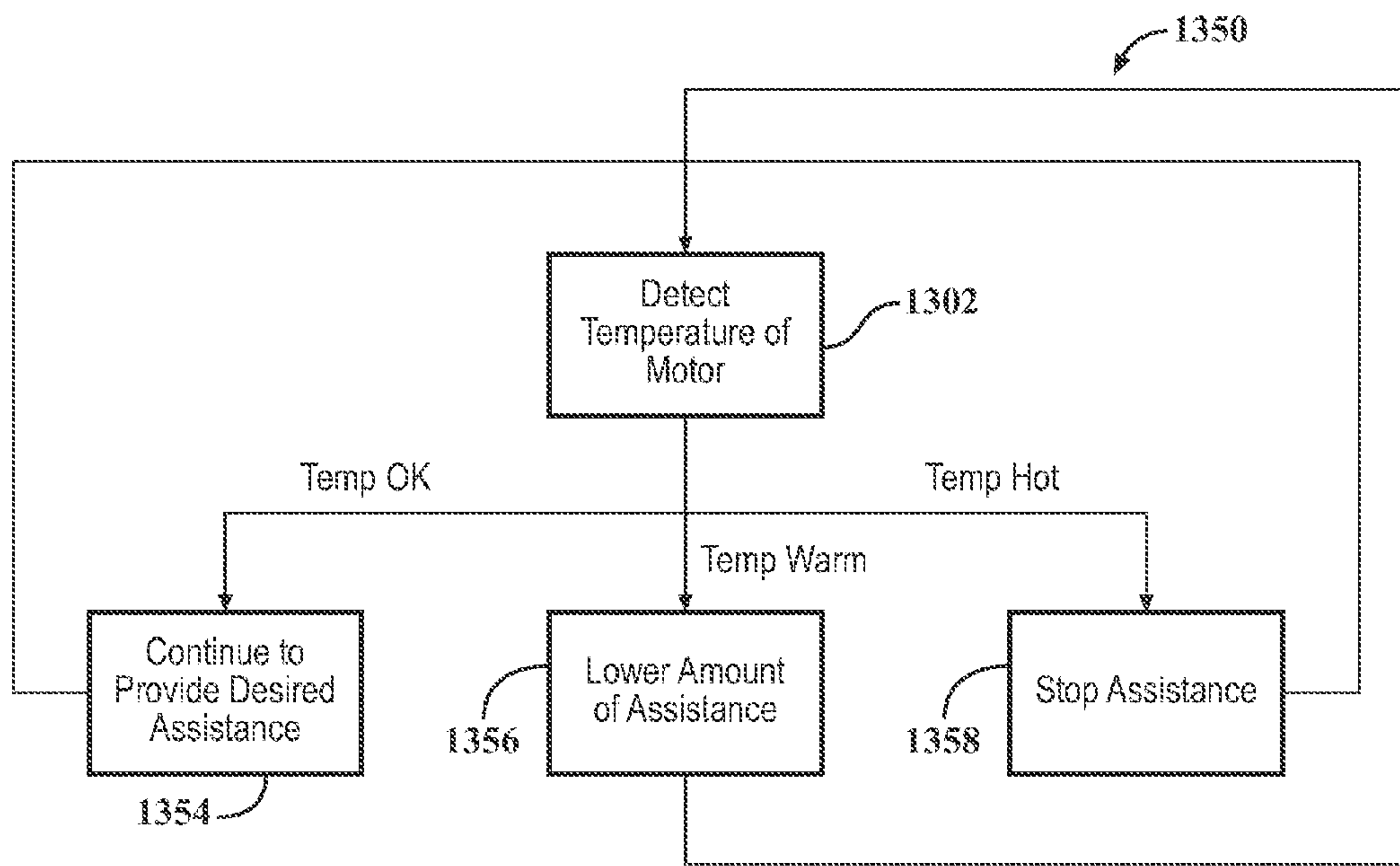
Thermal Motor Control
