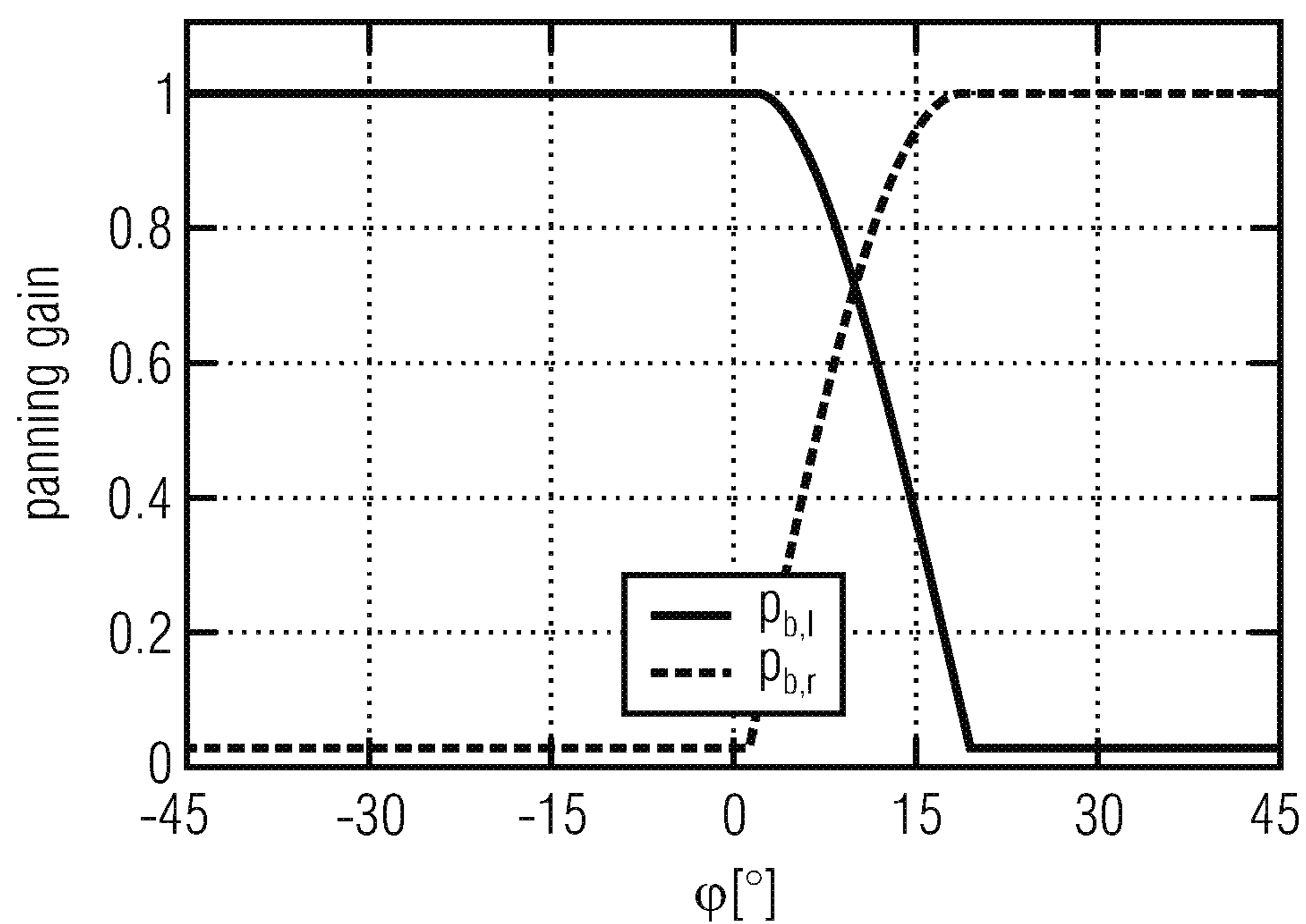
panning function after zooming with a shift
