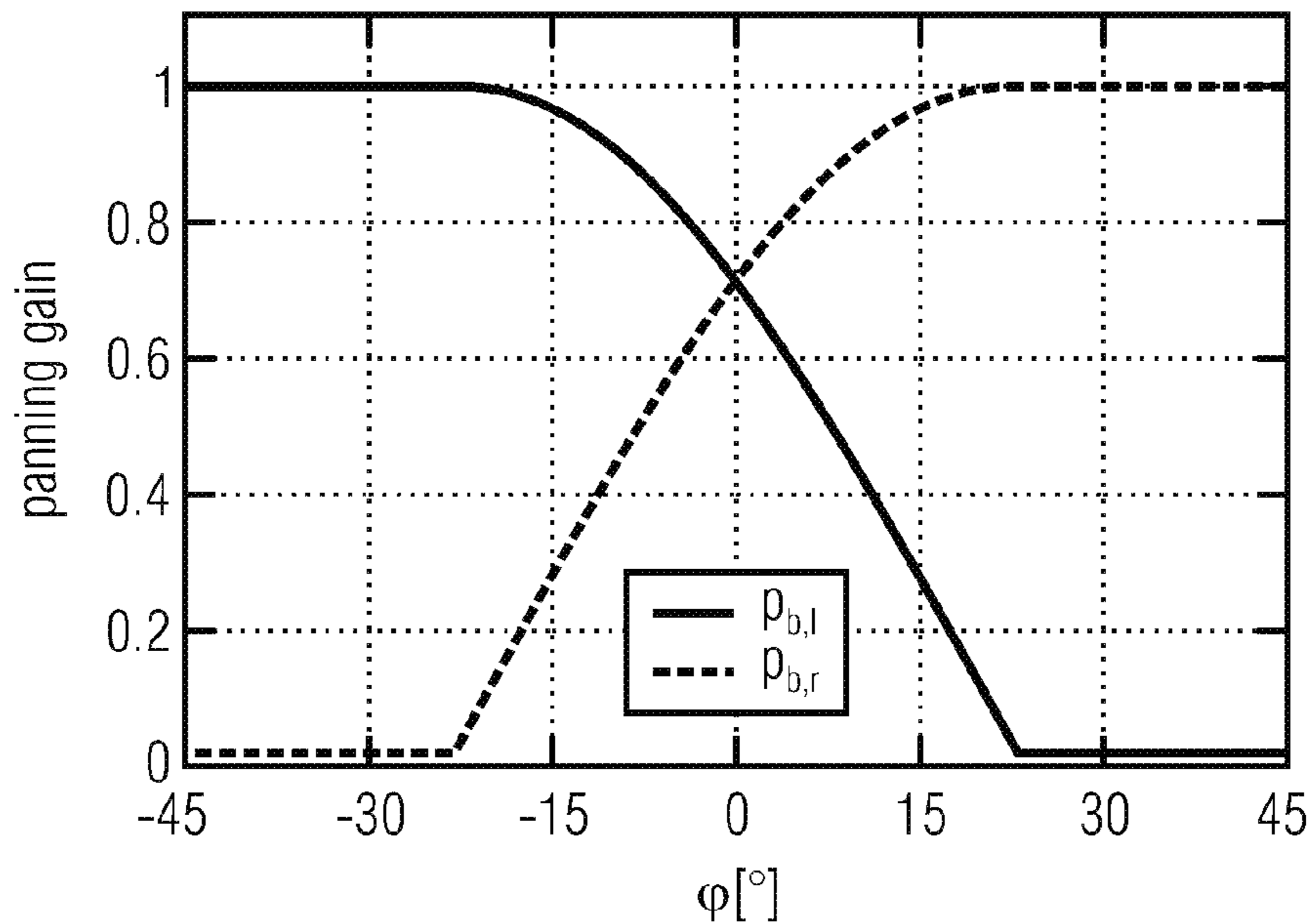
panning function for consistent reproduction
