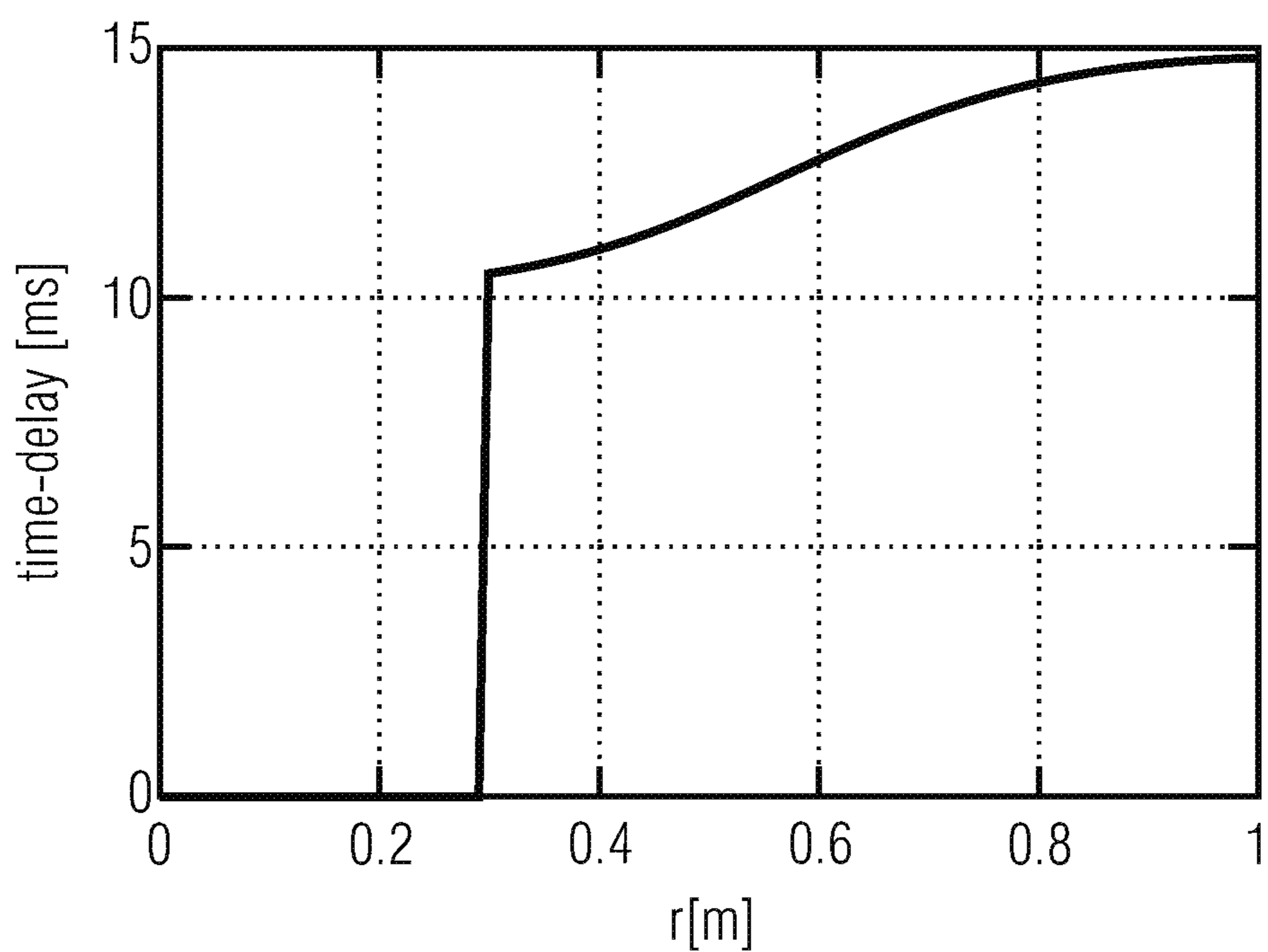
time-delay of the repeated direct sound
