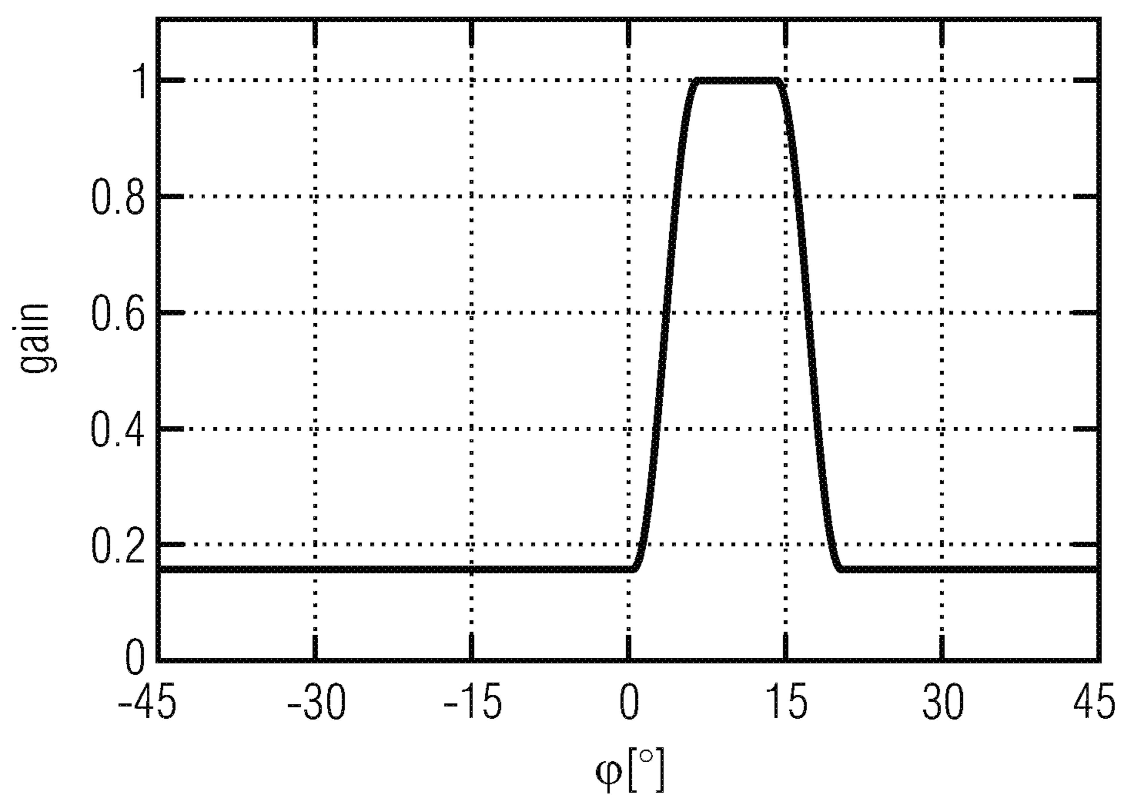
window function after zooming with a shift
