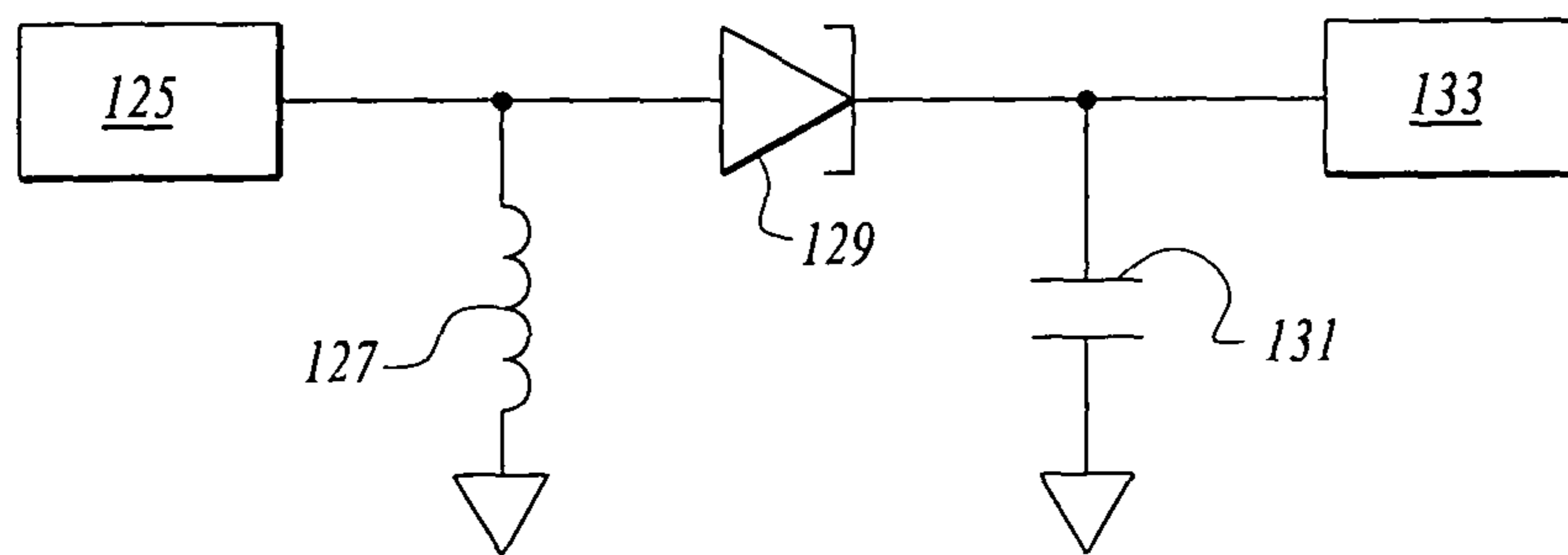
PRIOR TUNNEL DIODE DETECTOR SETUP
