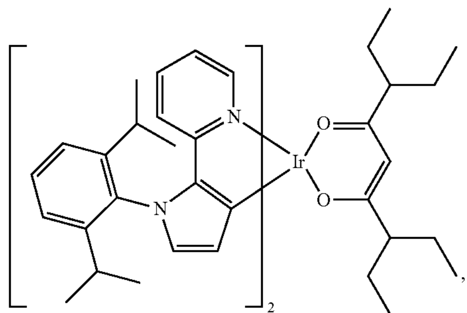
Compound 58
