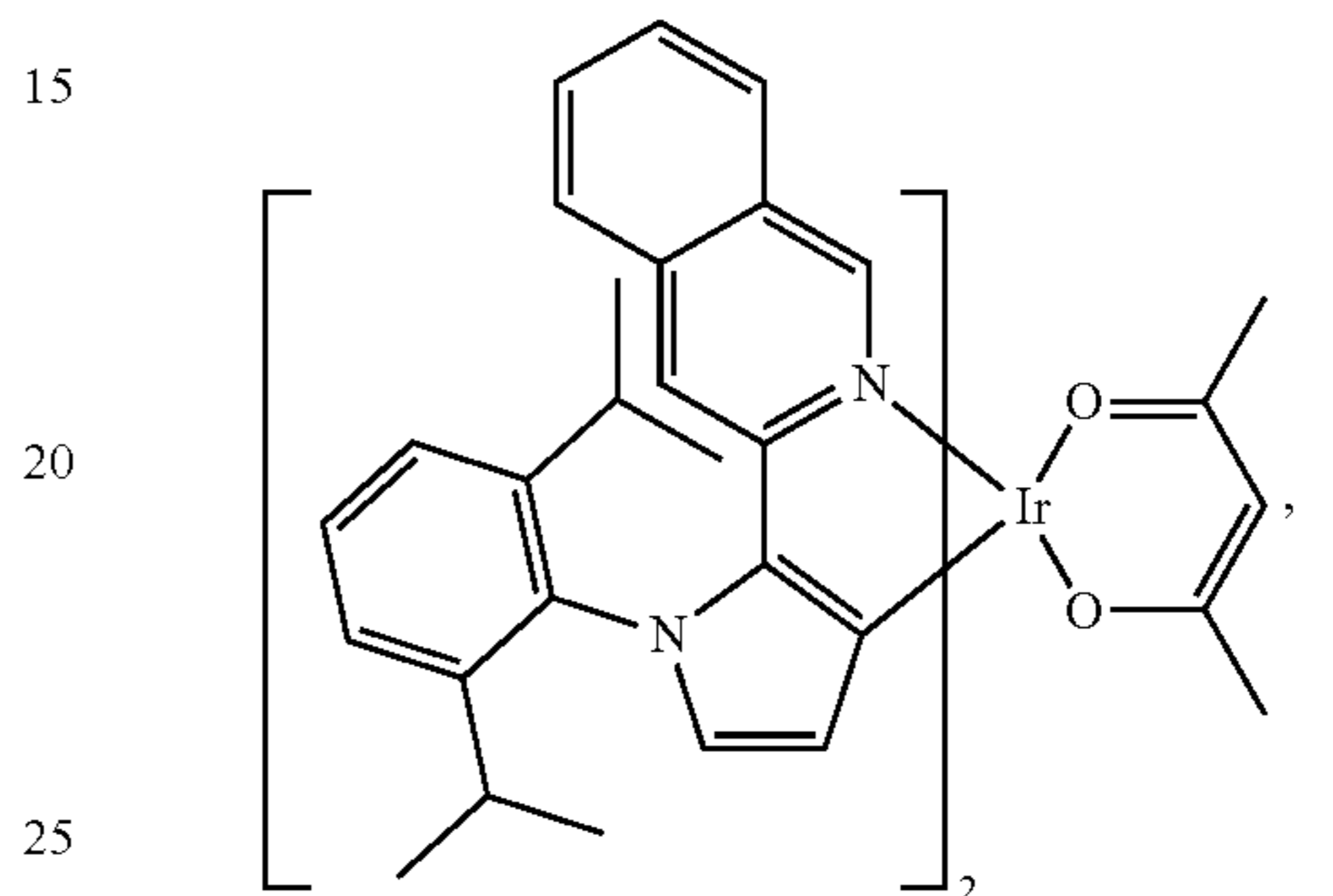
Compound 58
