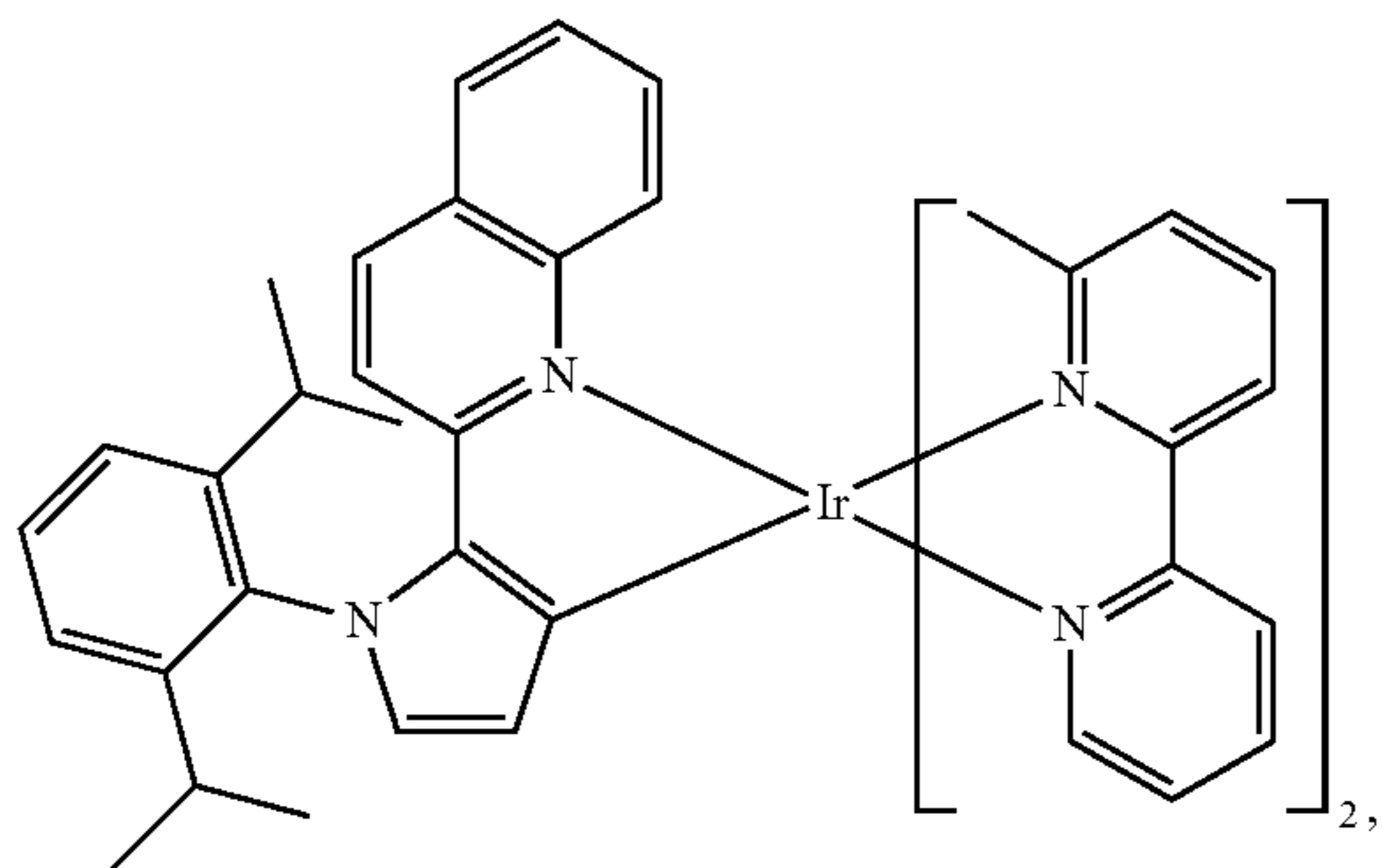
Compound 80
