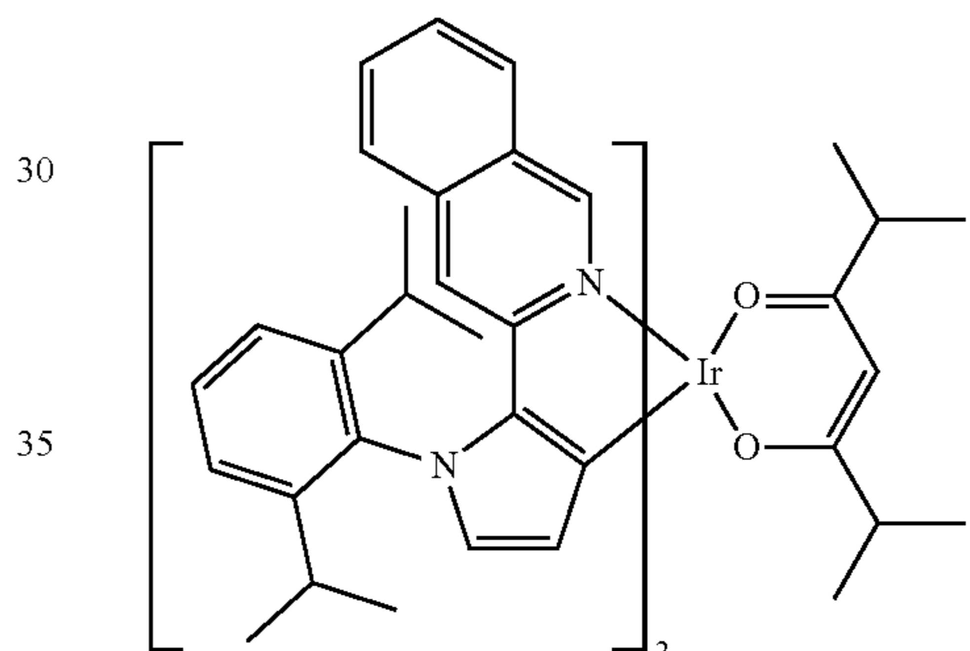
Compound 59
