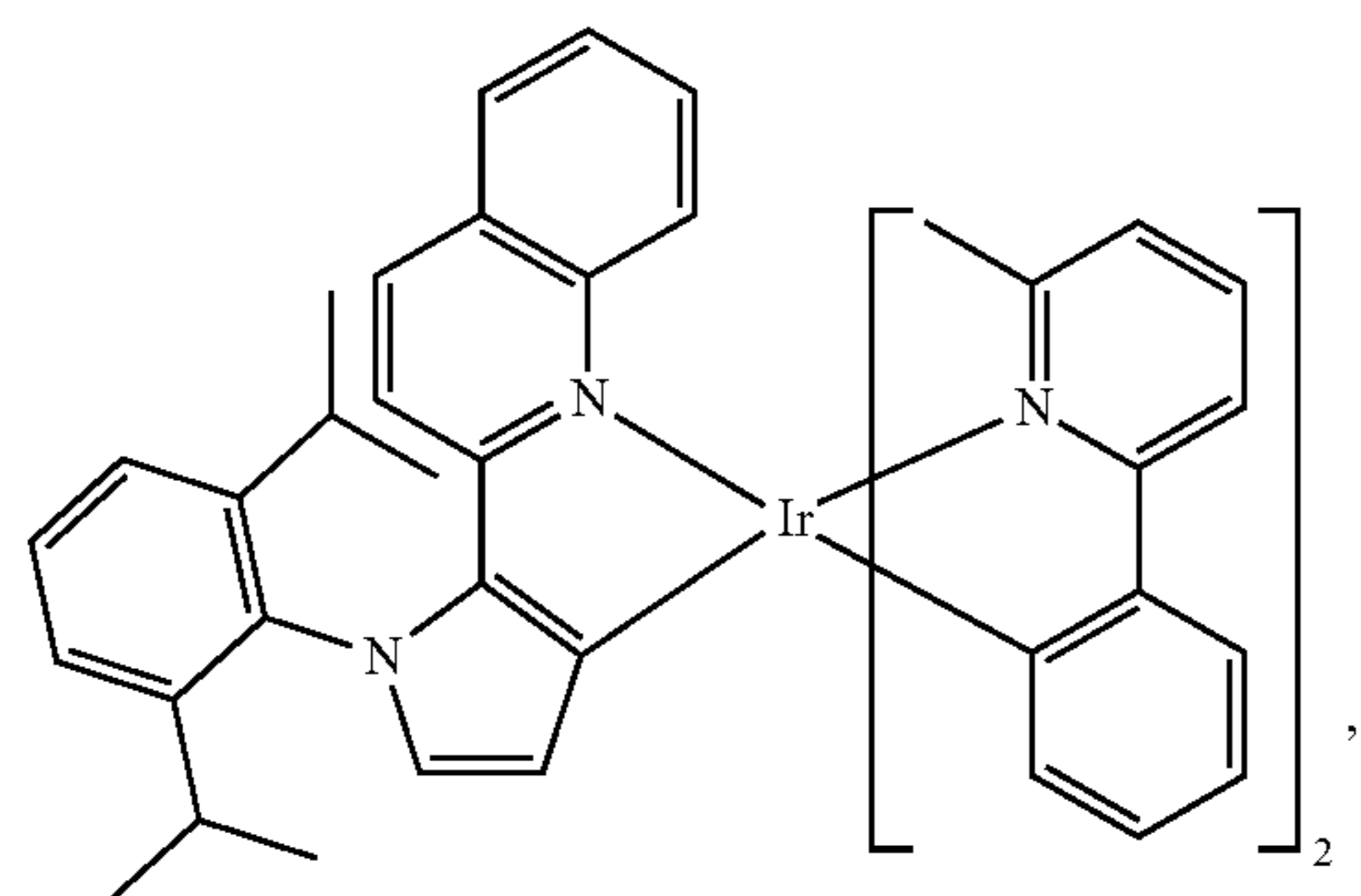
Compound 80
