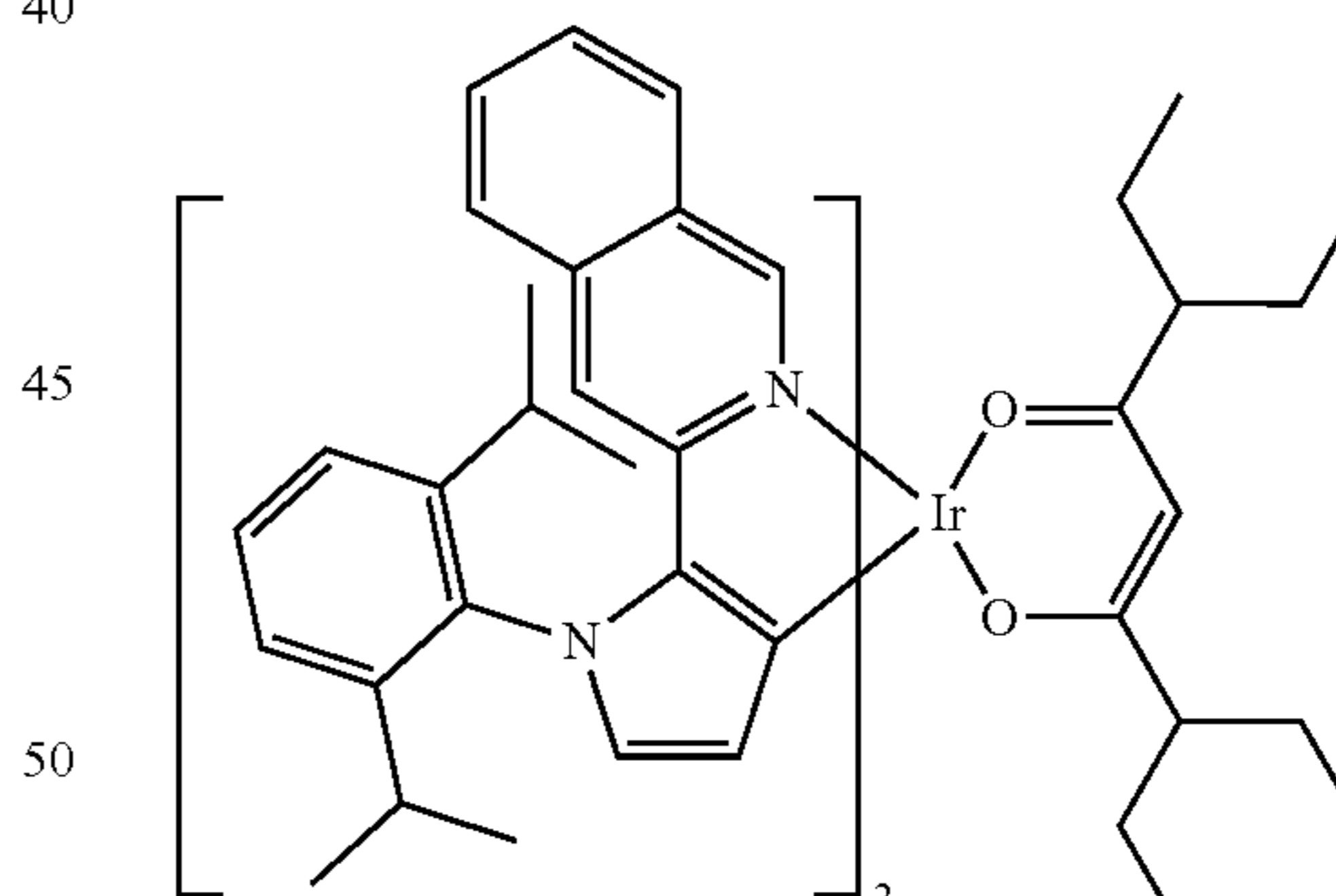
Compound 60
