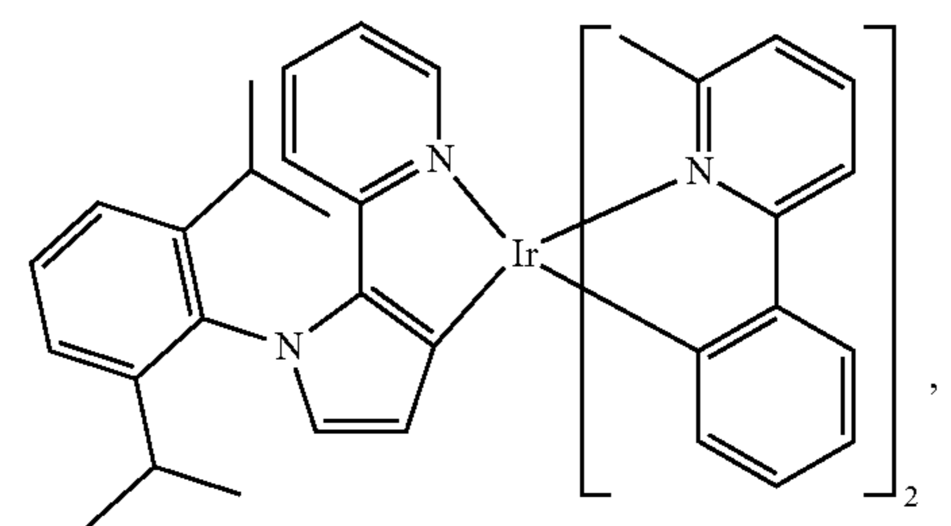
Compound 61
