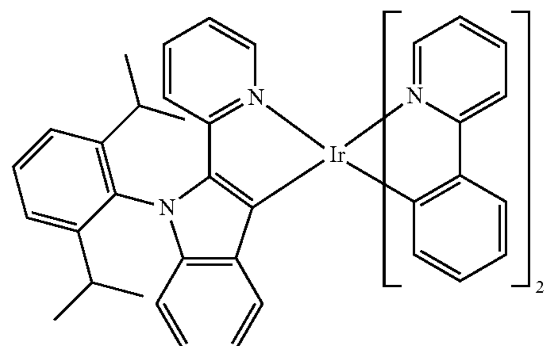
Compound 62
