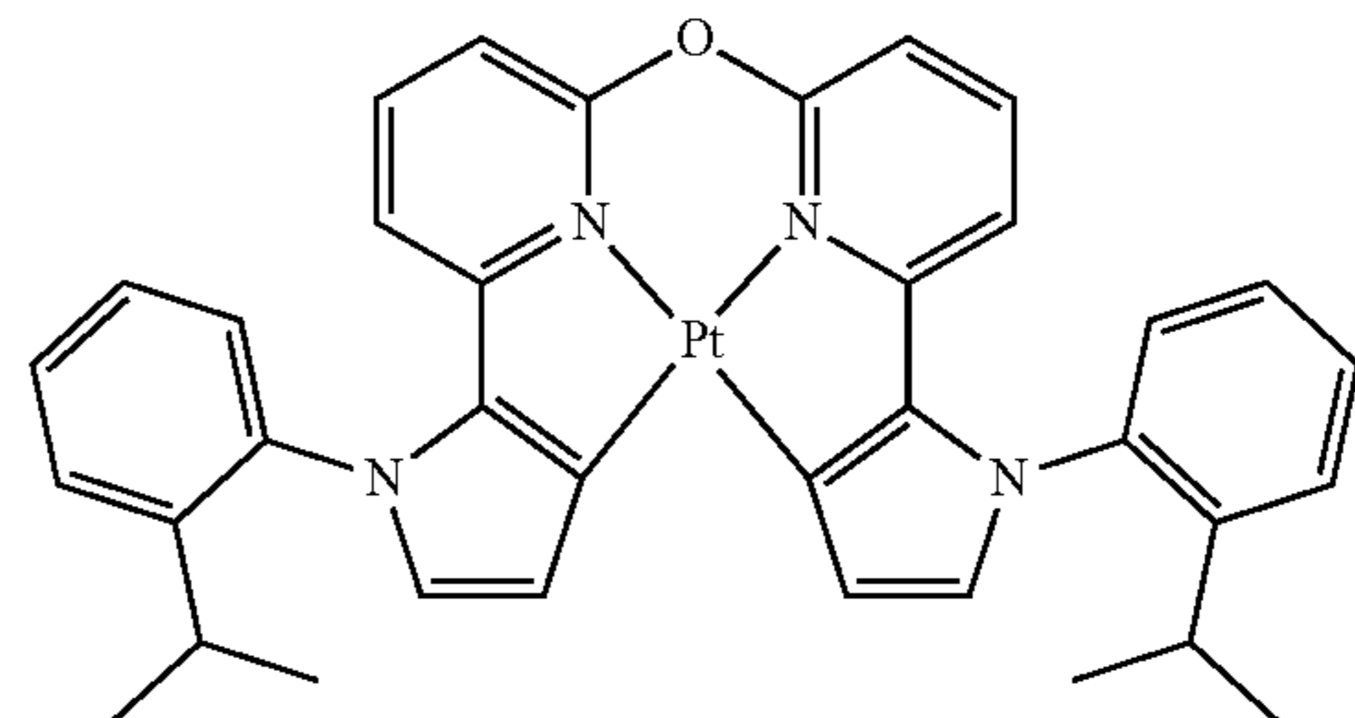
Compound 103
