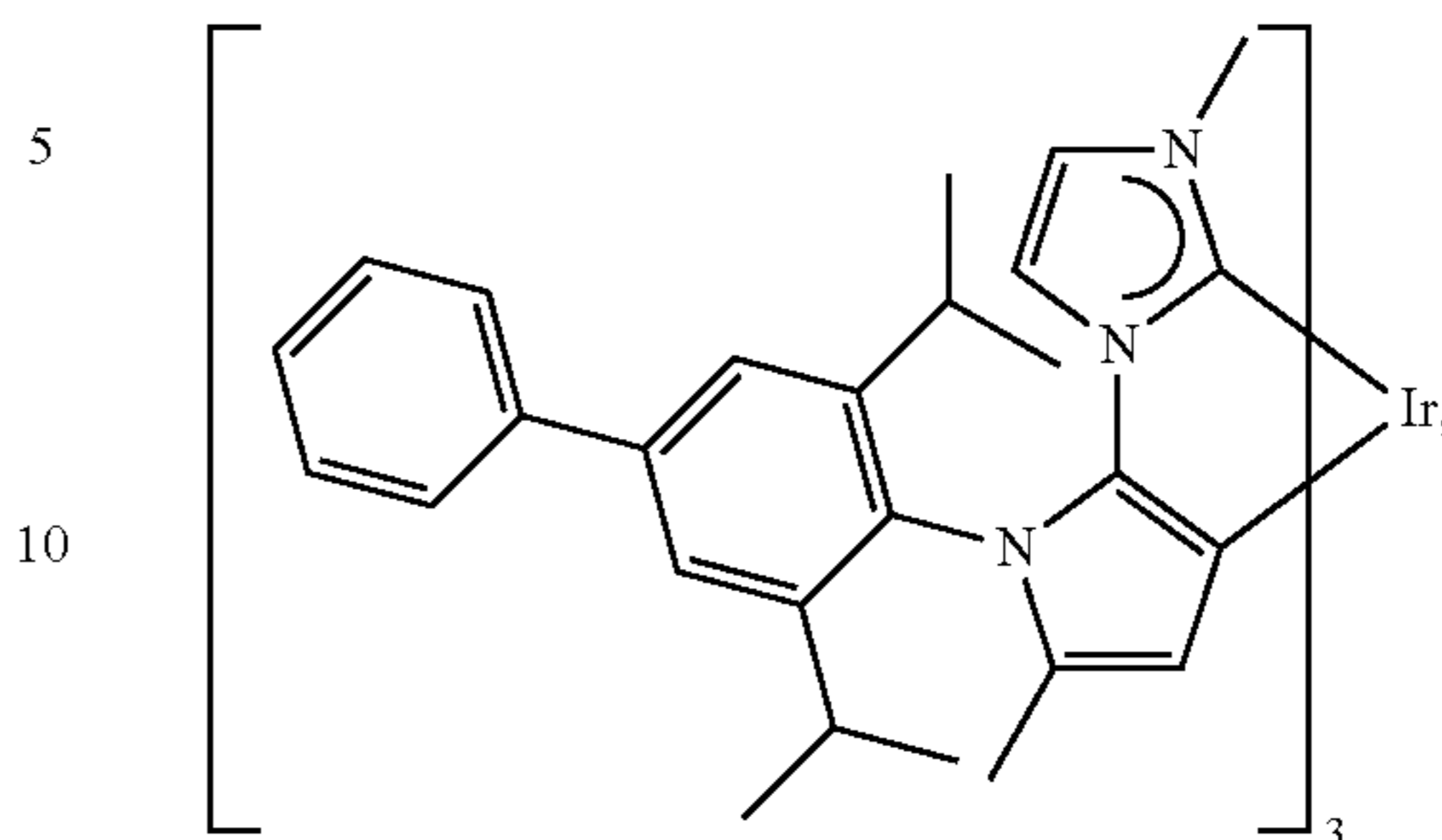
Compound 1
