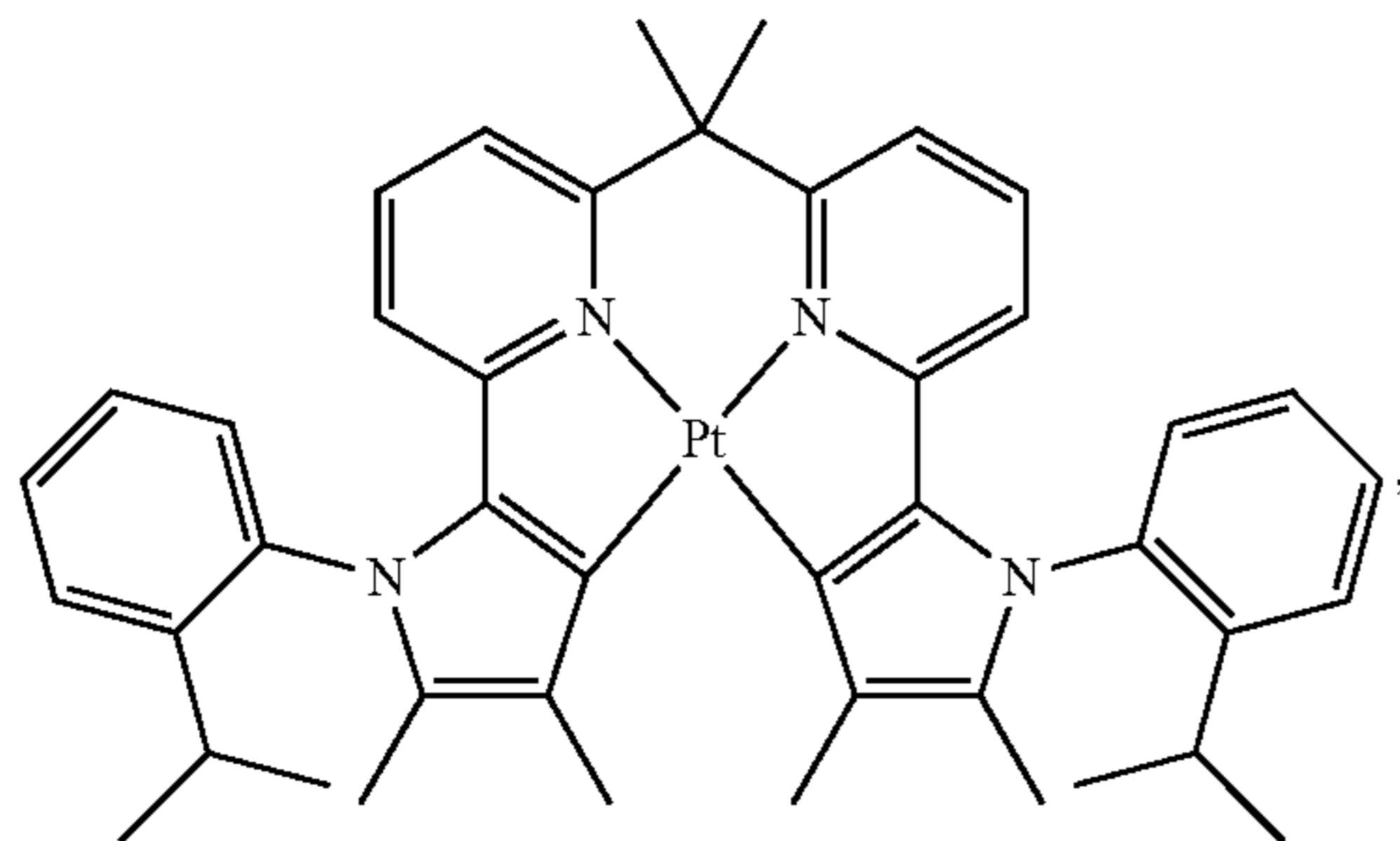
Compound 100
