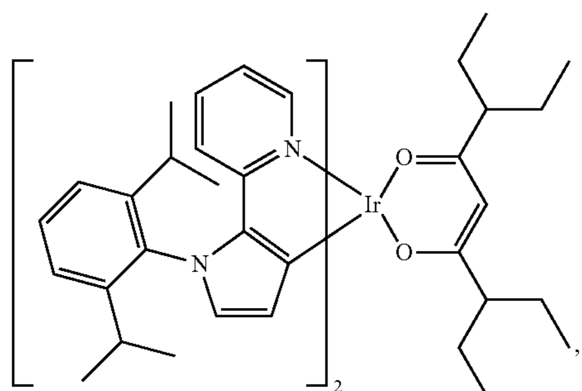
Compound 56
