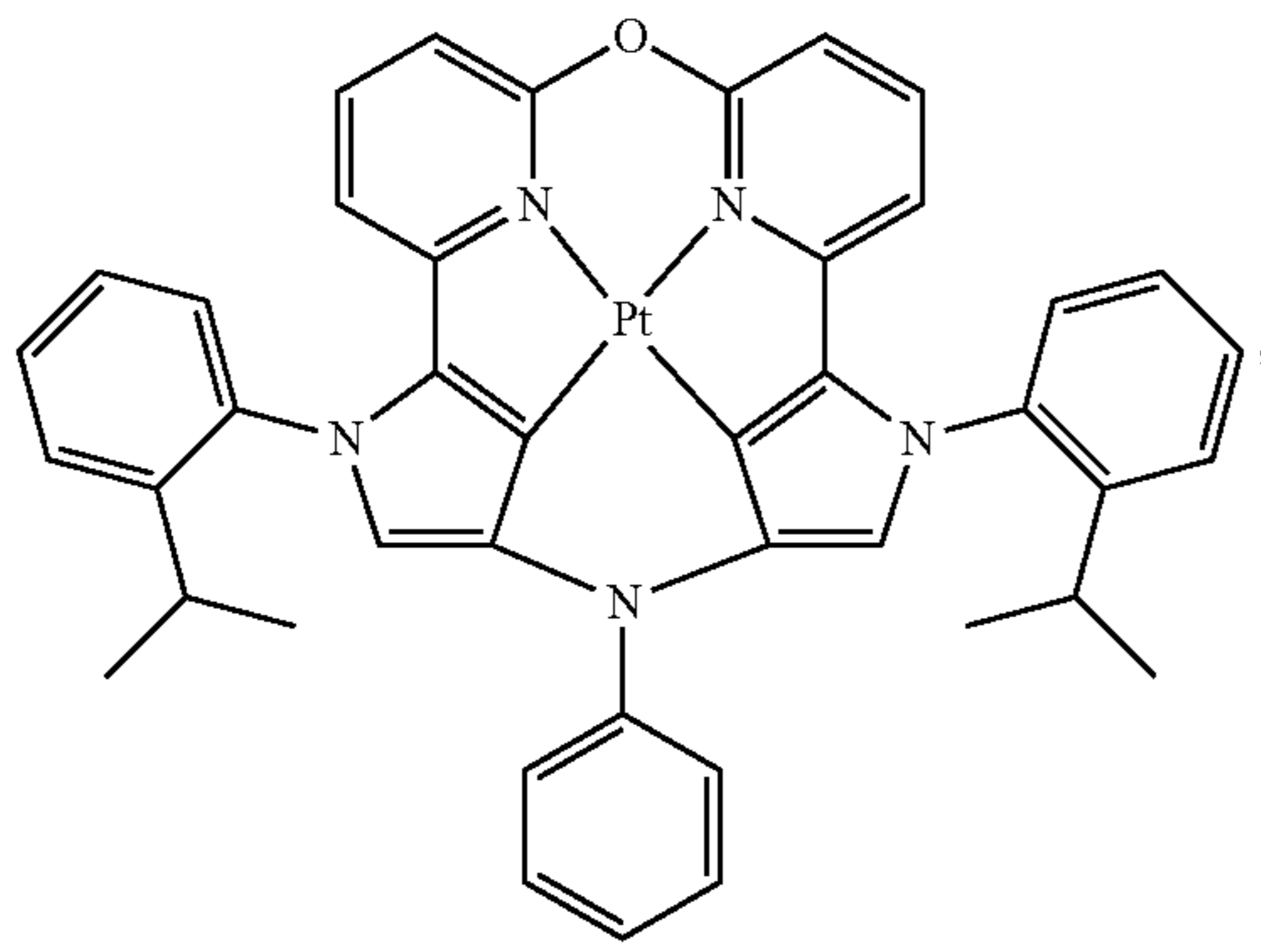
Compound 110
