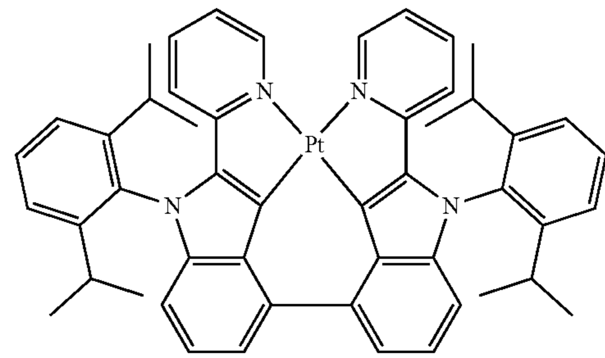
Compound 113
