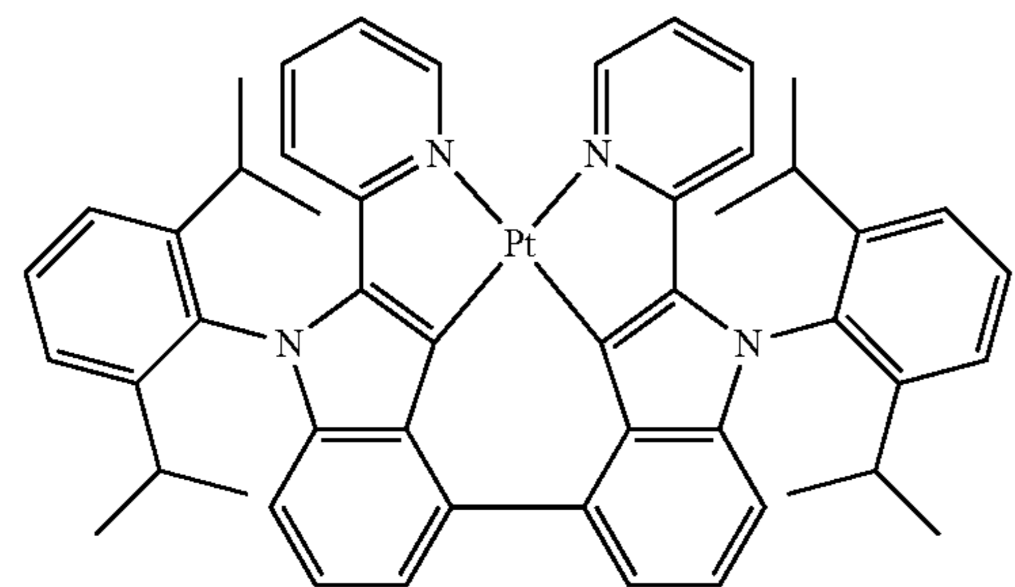
Compound 113
