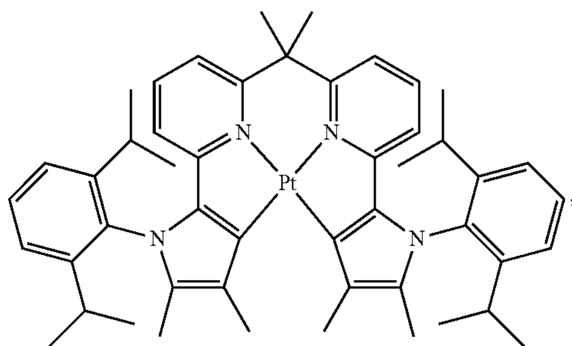
Compound 102
