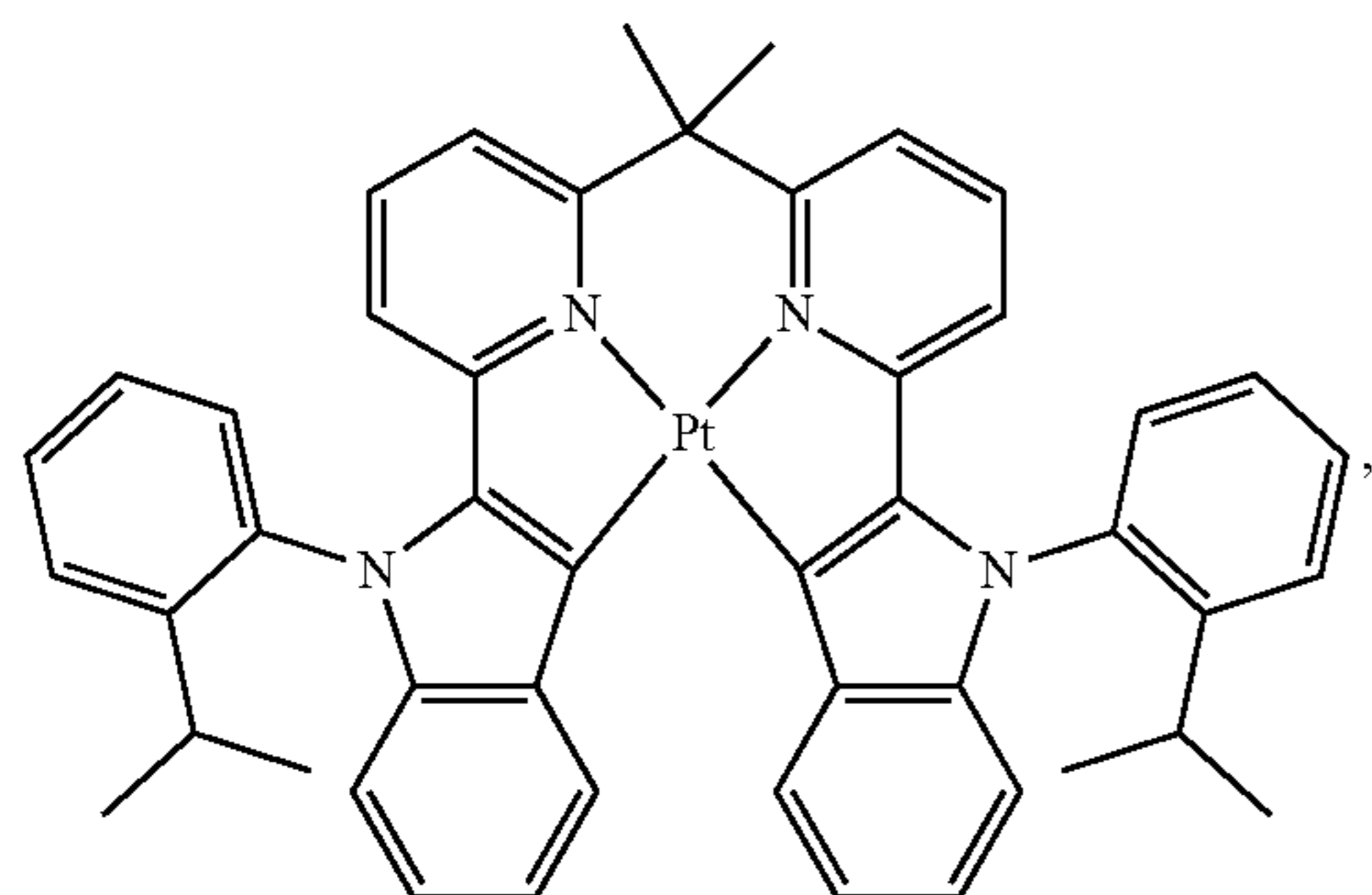
Compound 95
