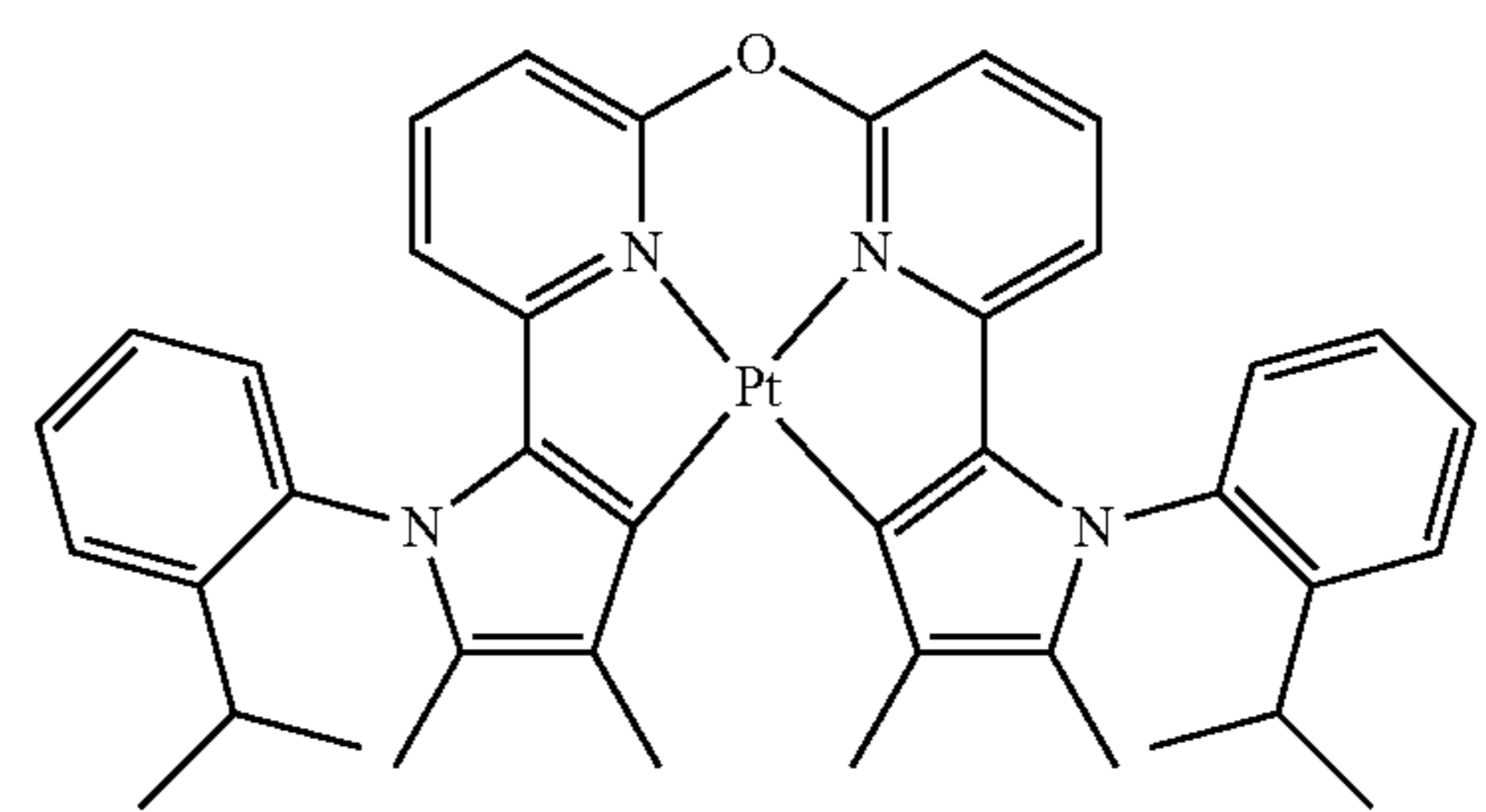
Compound 108
