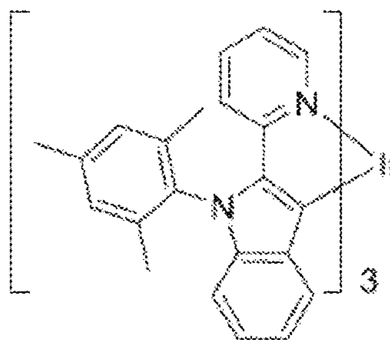
Compound 48
