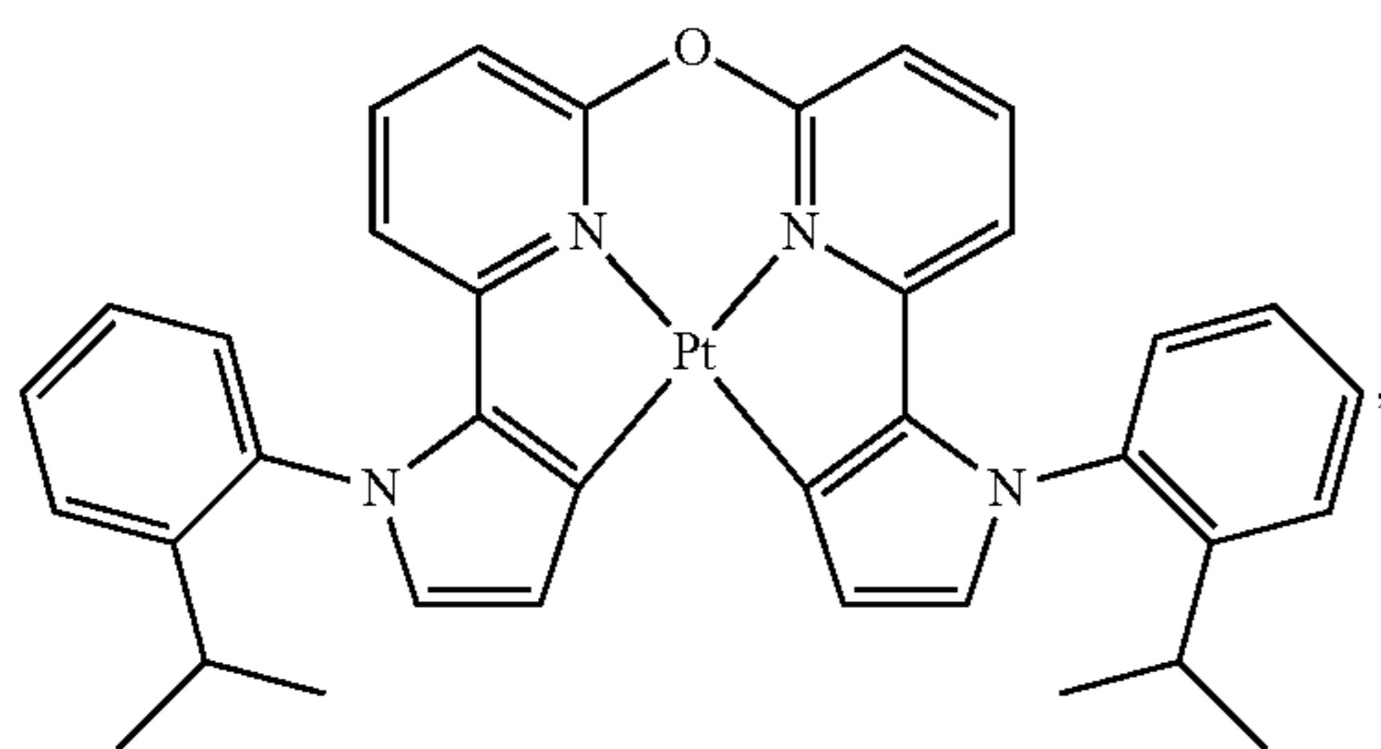
Compound 104
