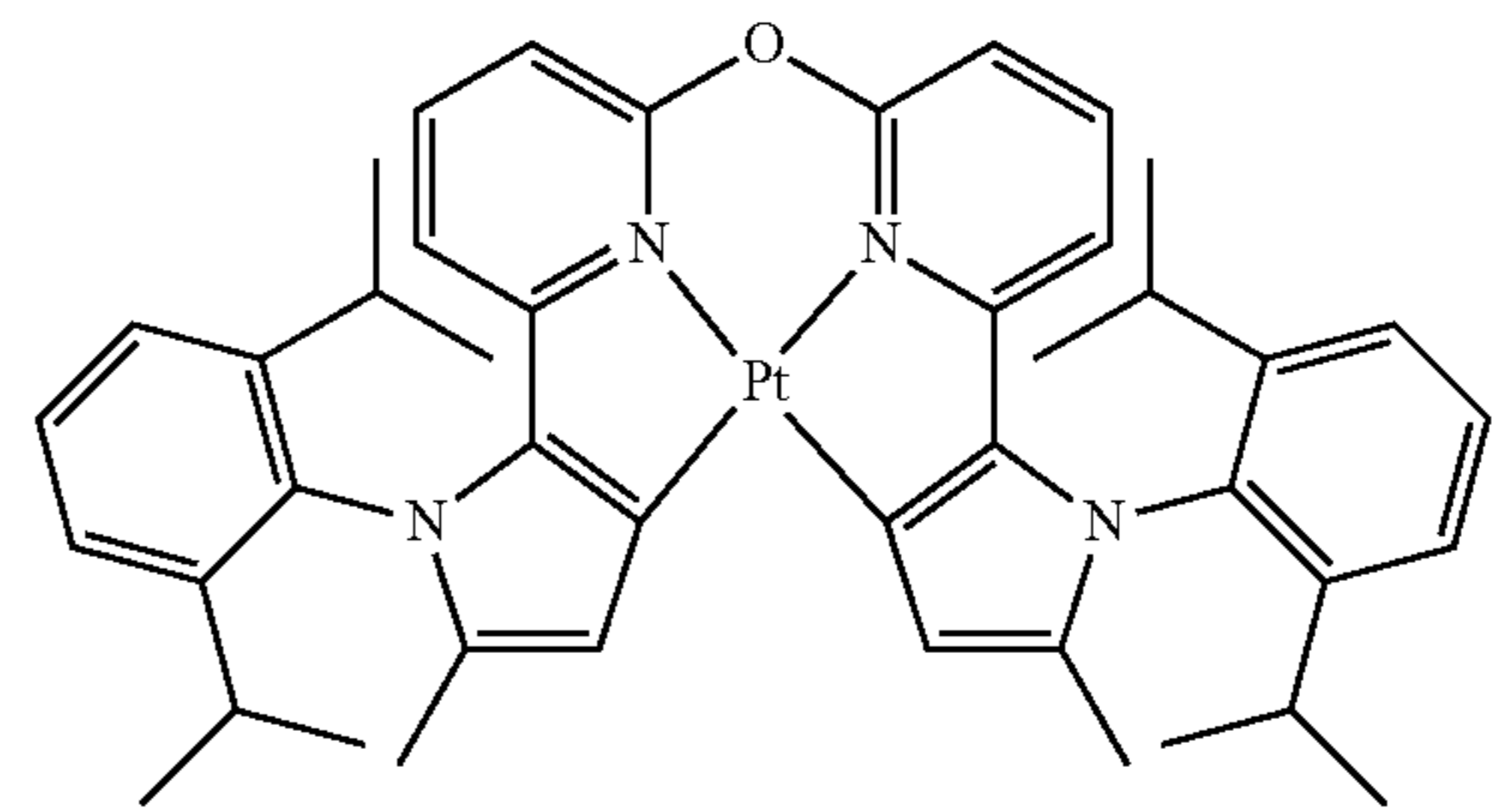
Compound 108
