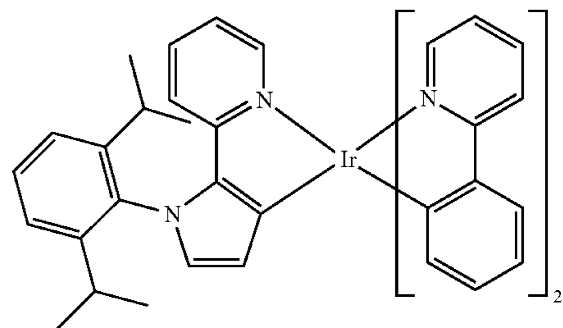
Compound 59
