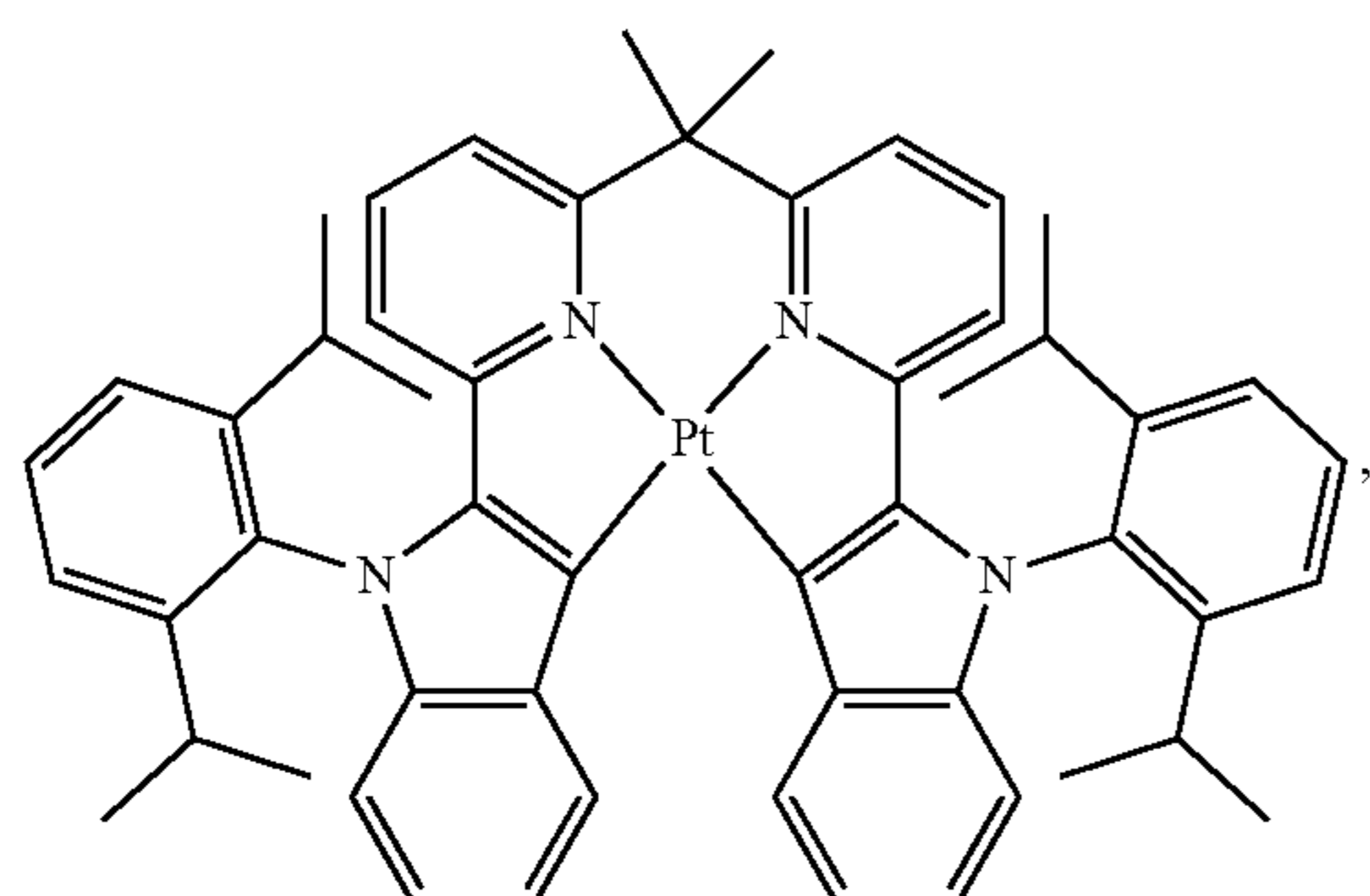
Compound 97
