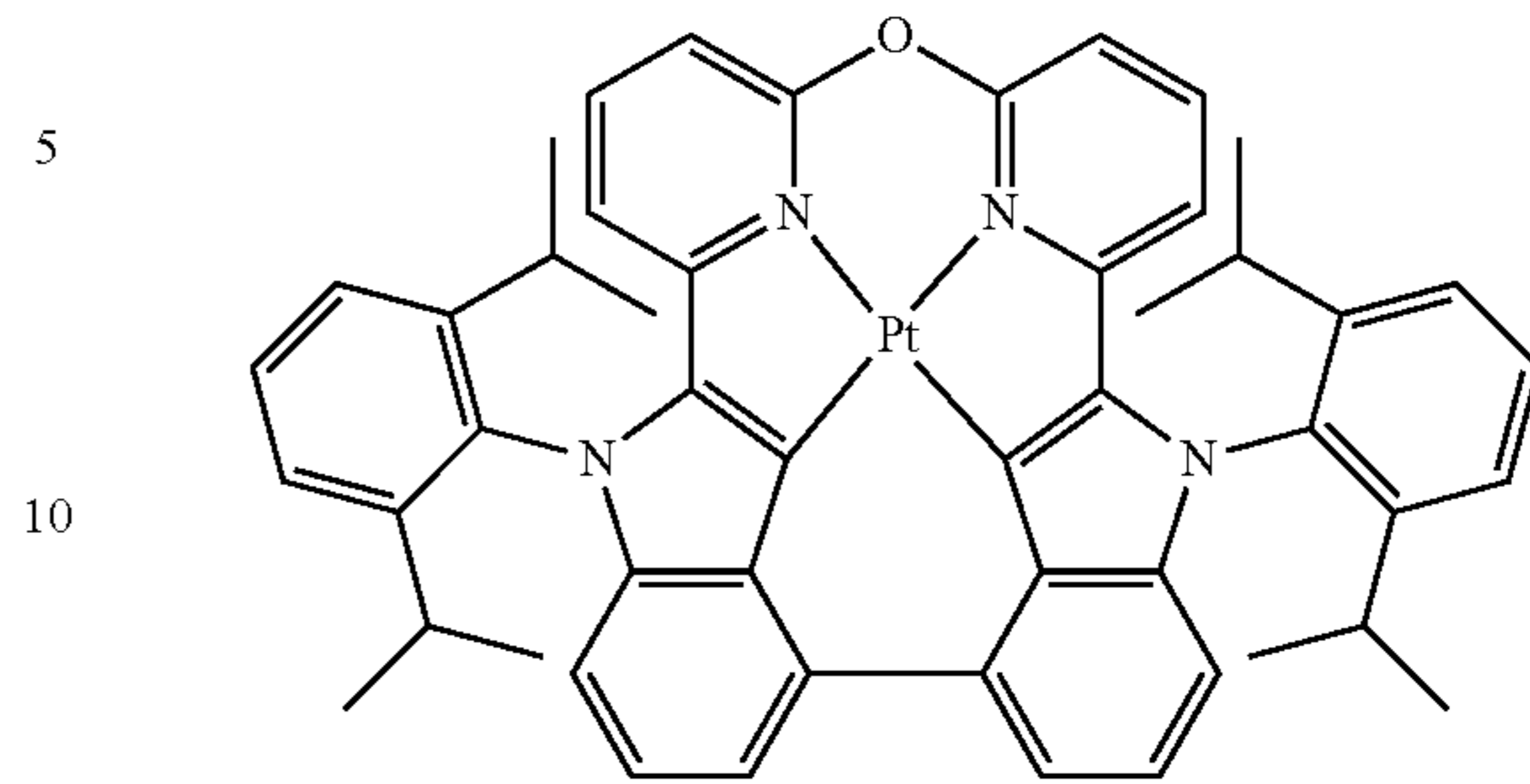
Compound 113
