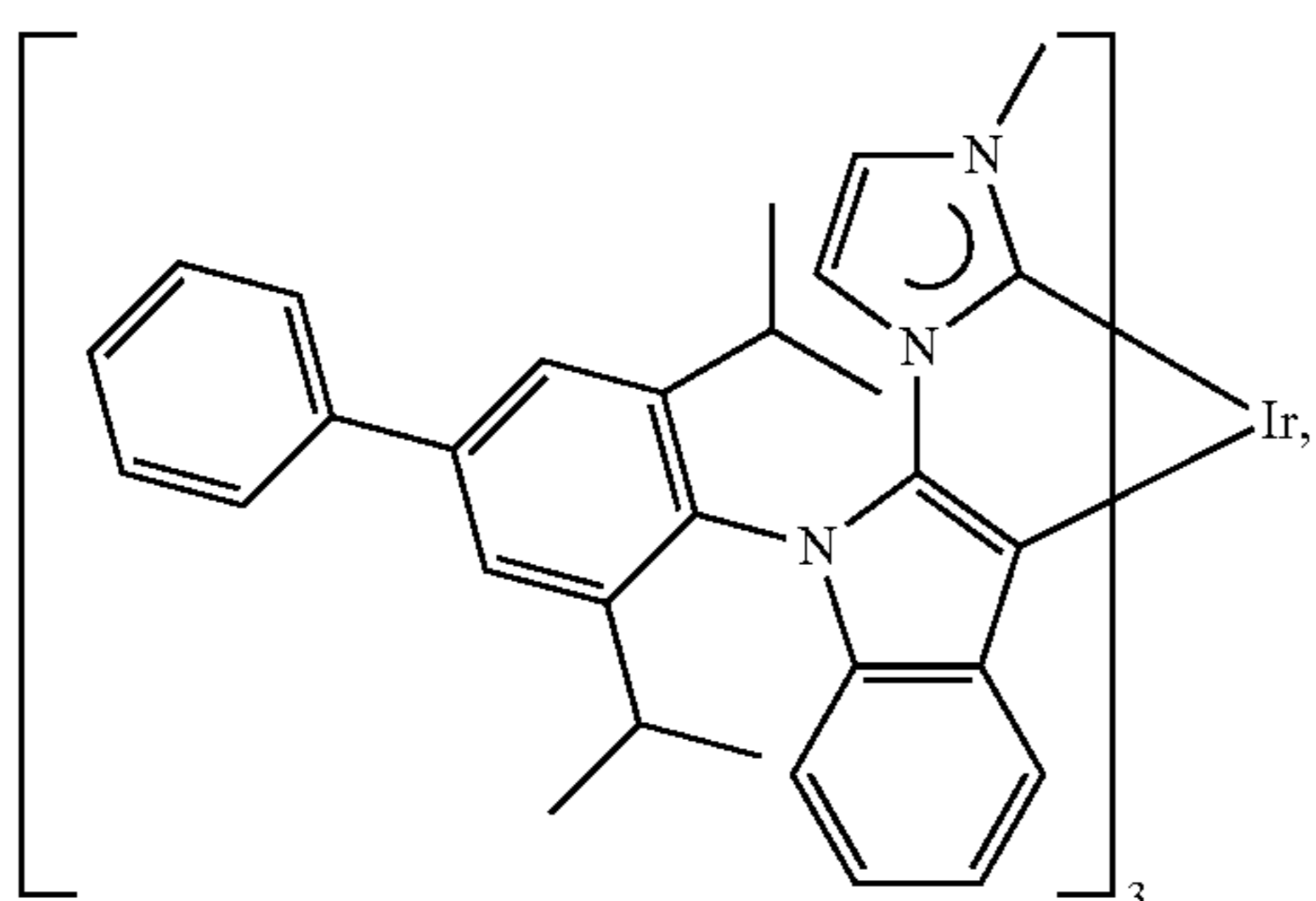
Compound 13
