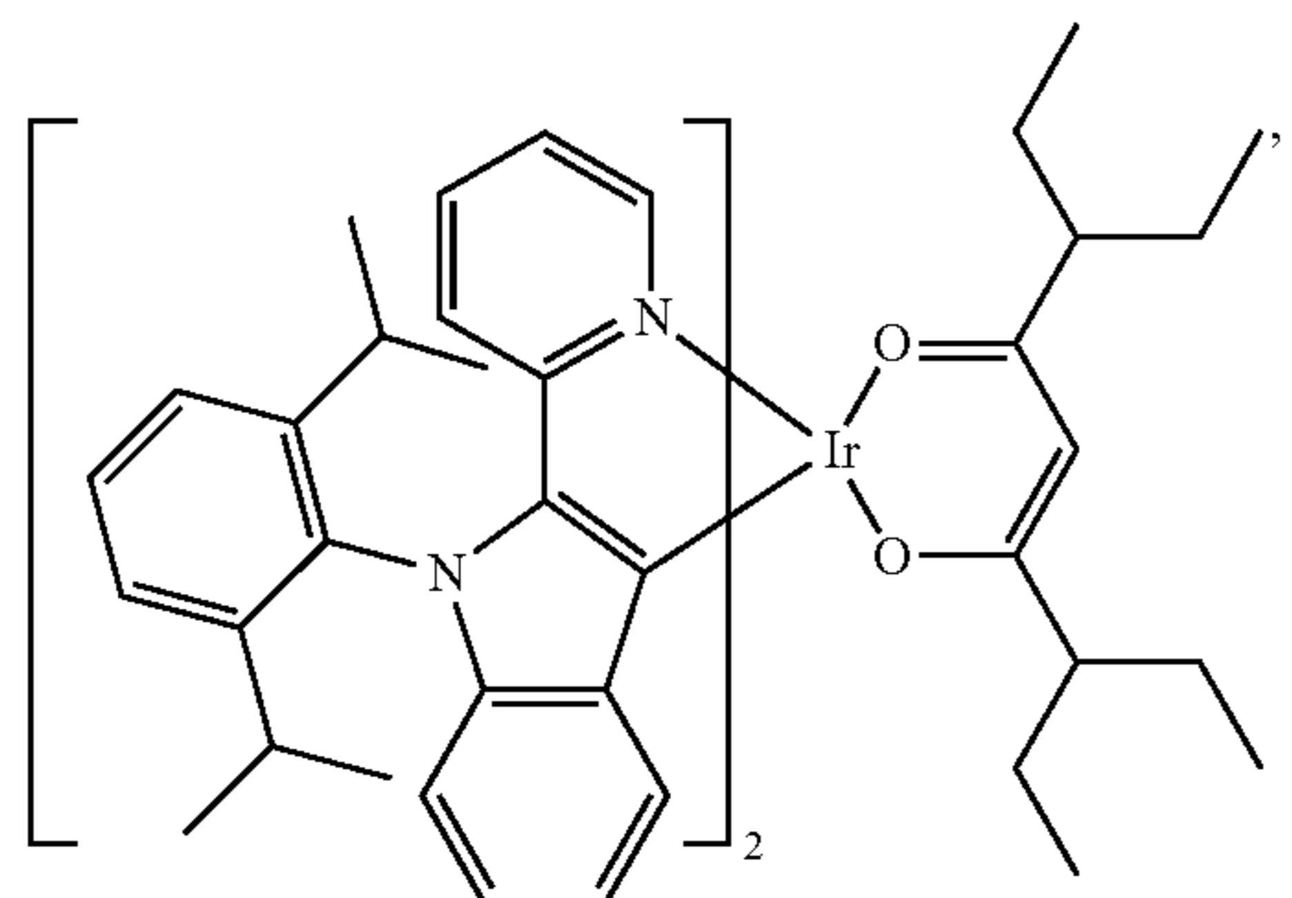
Compound 58
