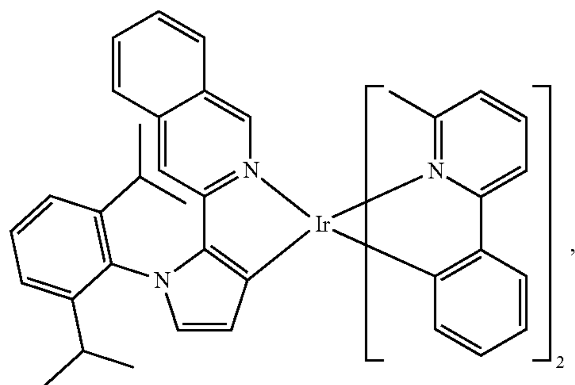
Compound 70
