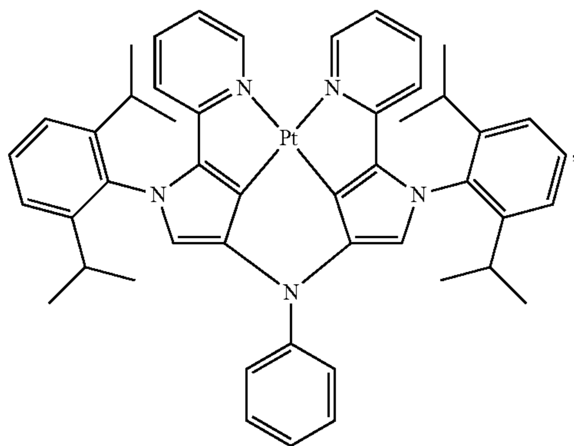
Compound 112
