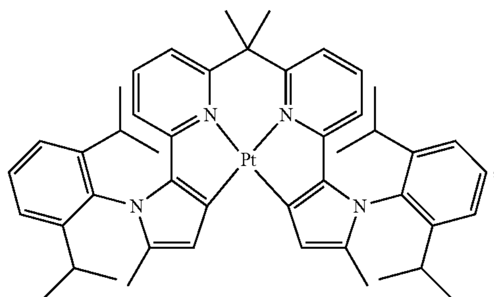
Compound 99
