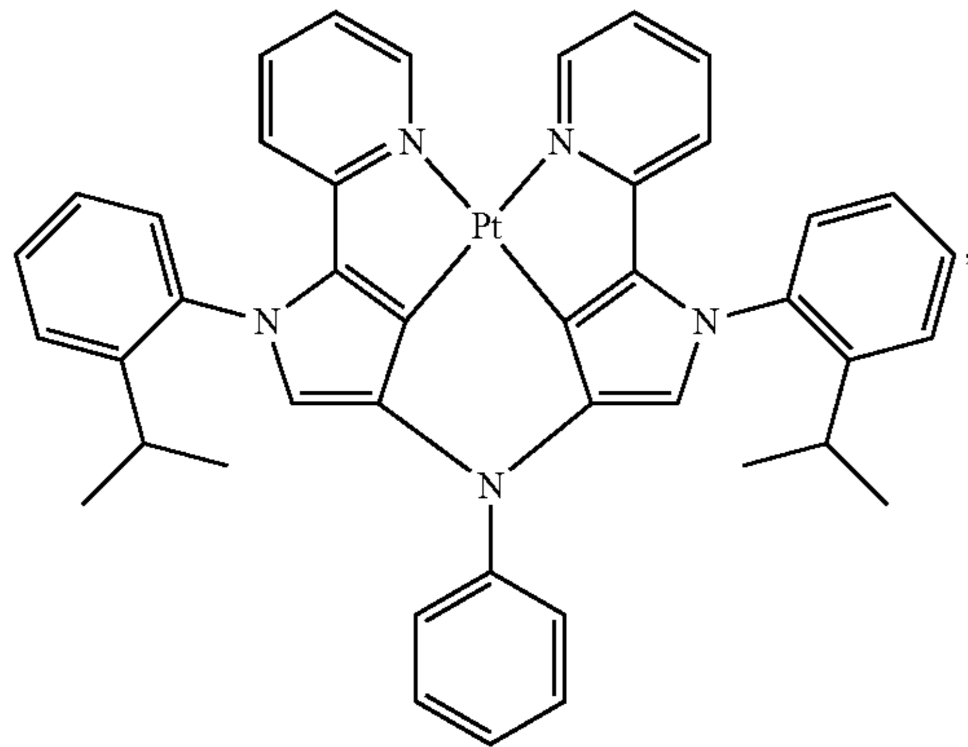
Compound 111
