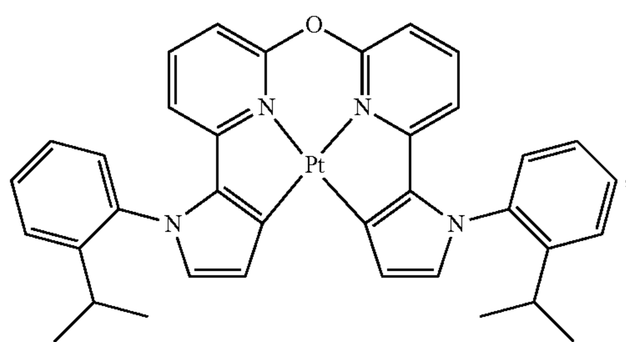
Compound 103
