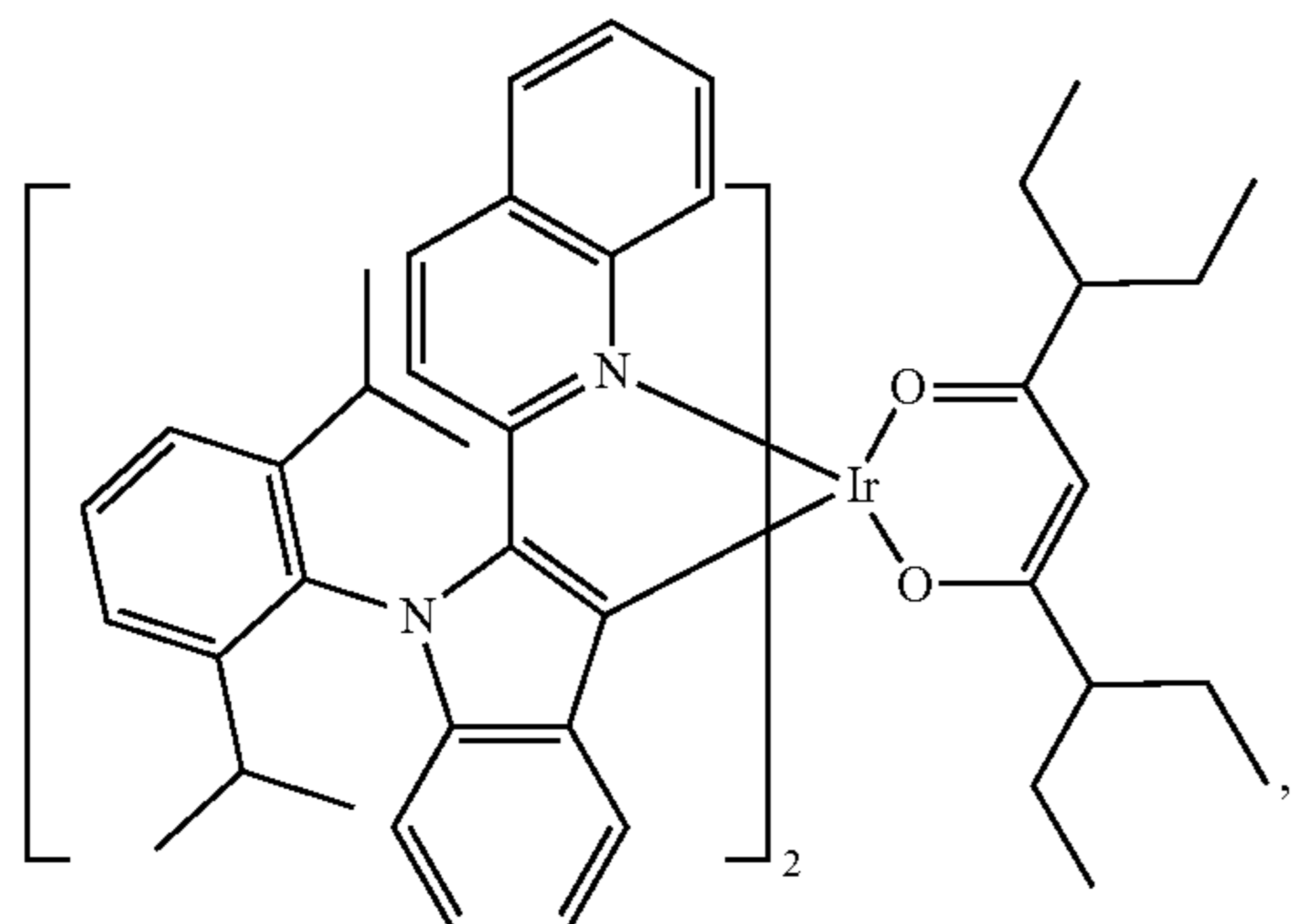
Compound 78
