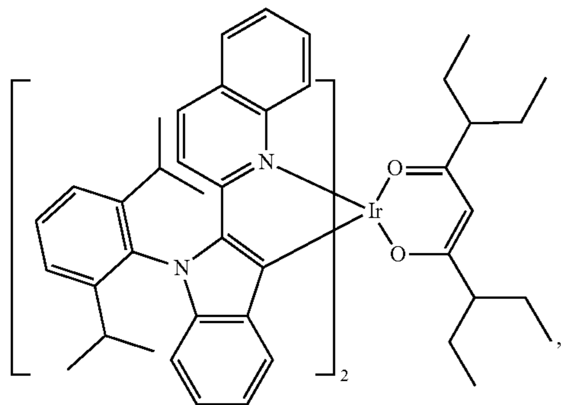
Compound 78
