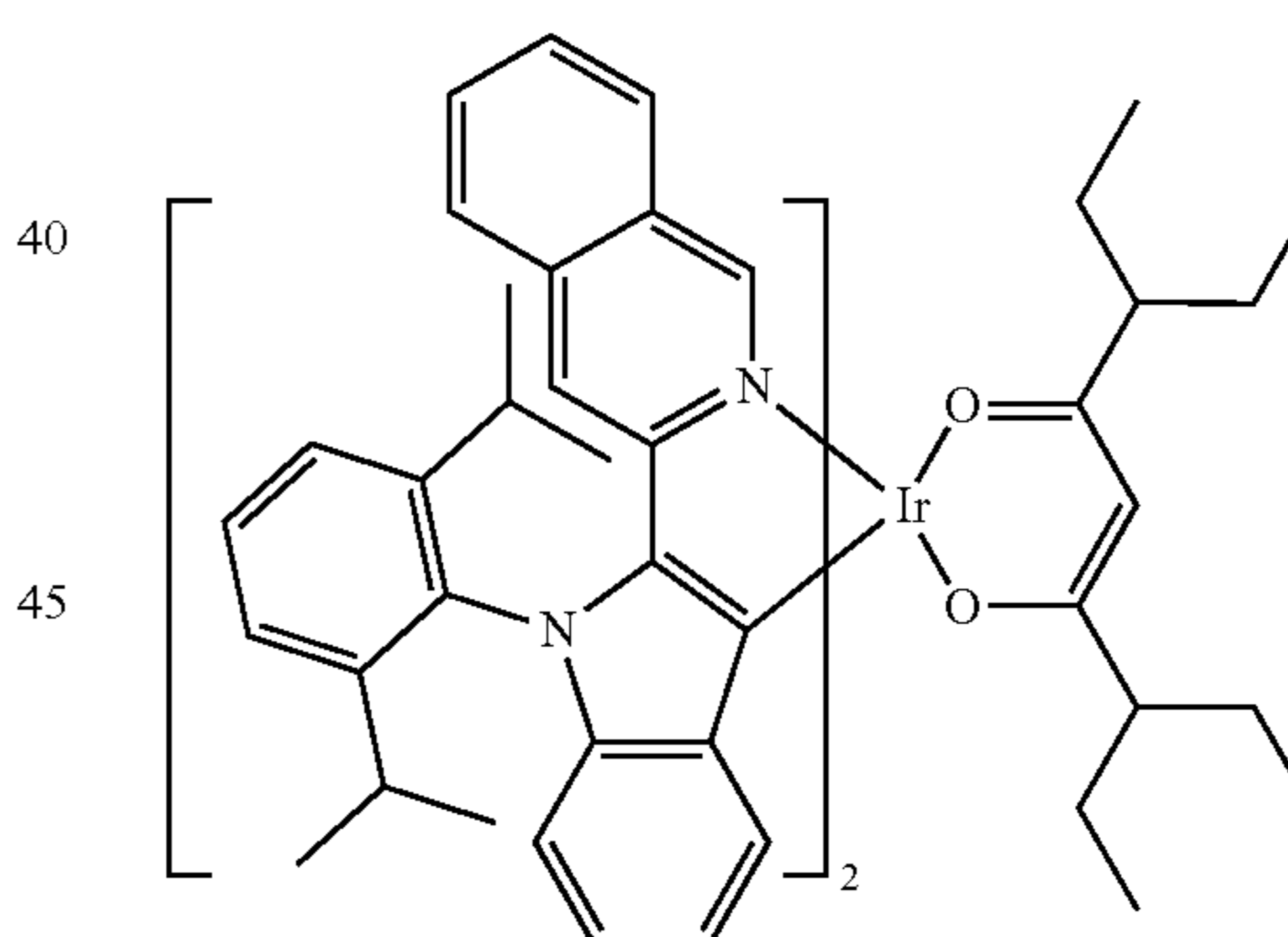
Compound 64
