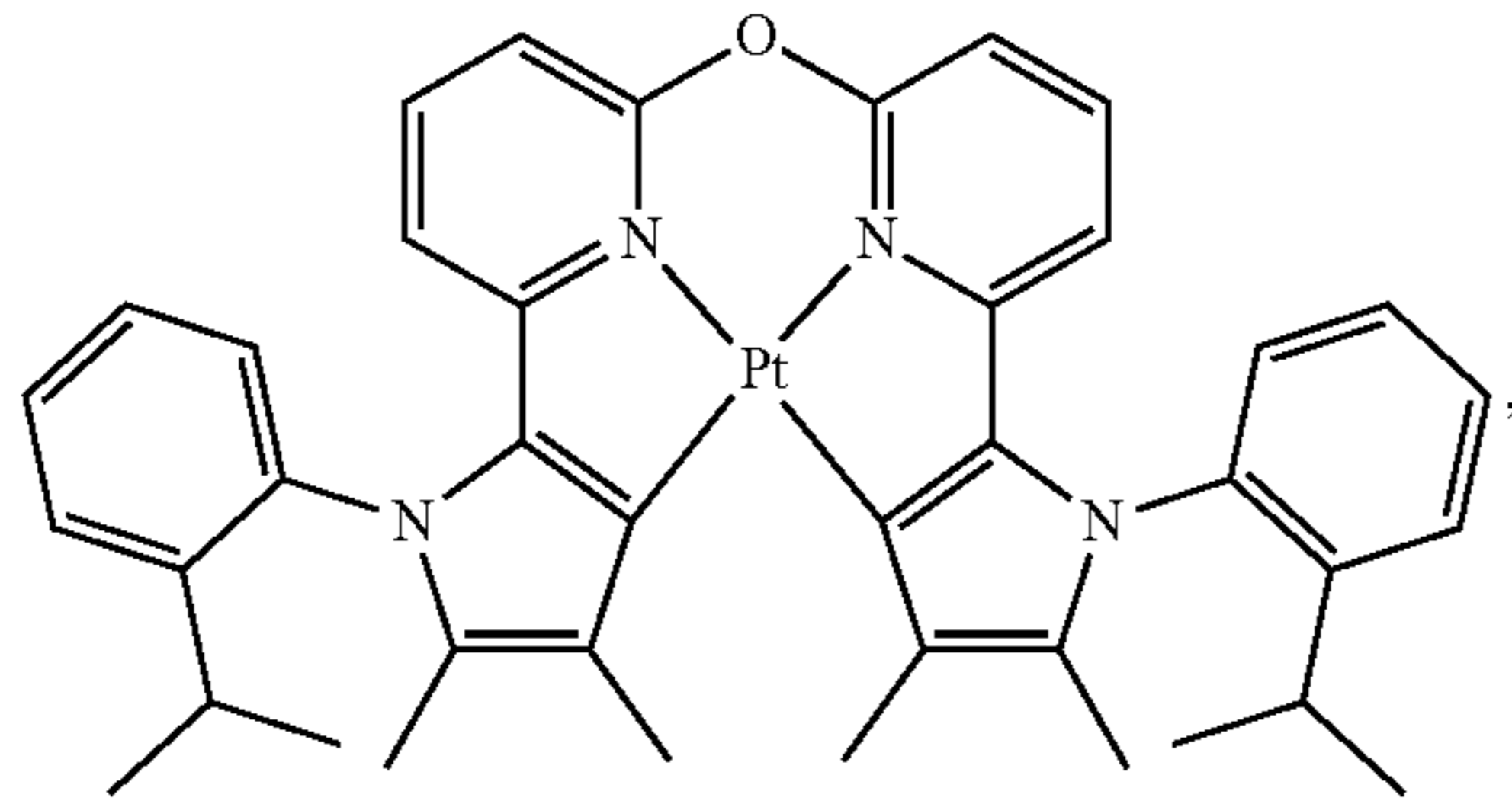
Compound 109
