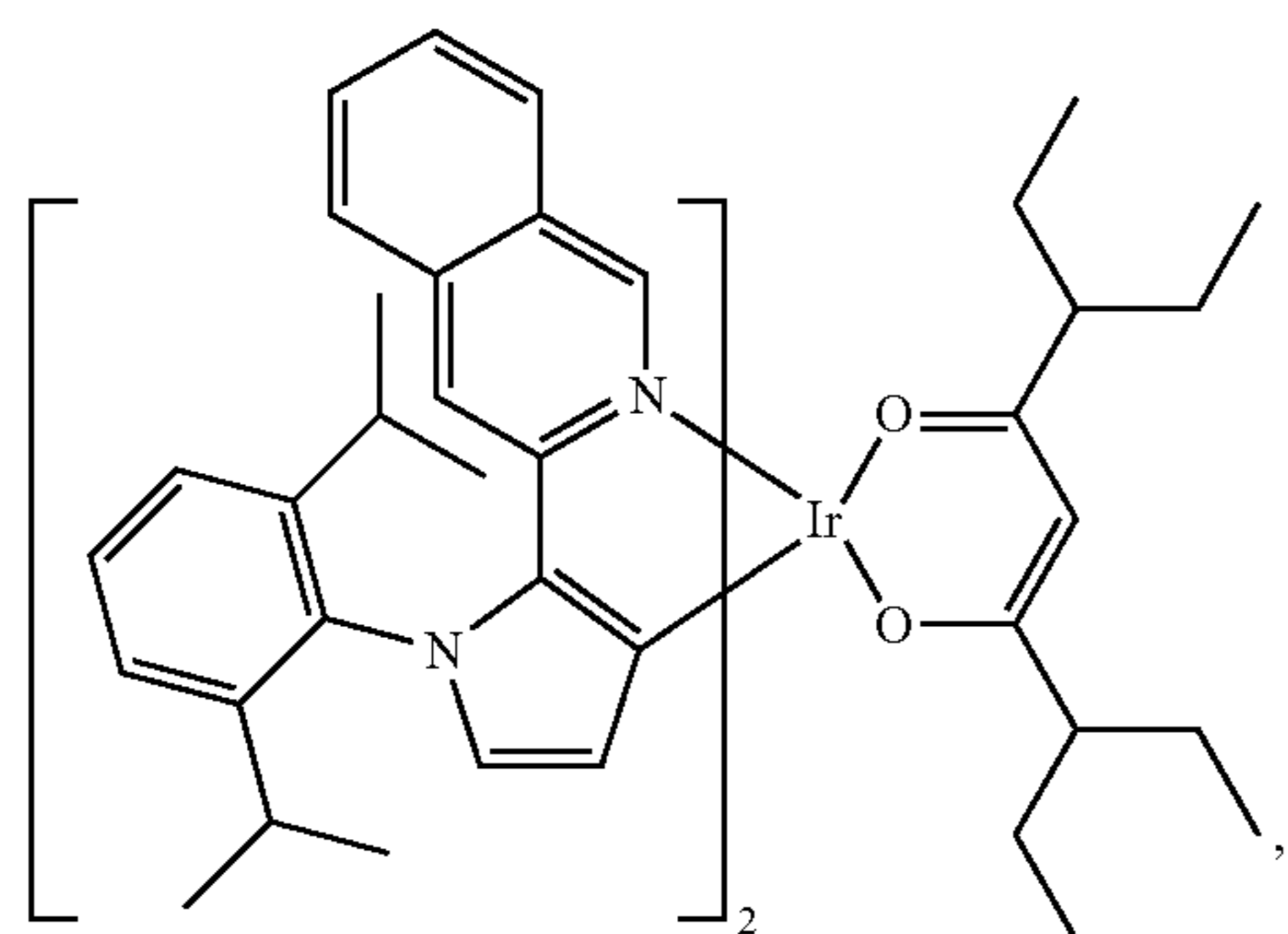
Compound 65
