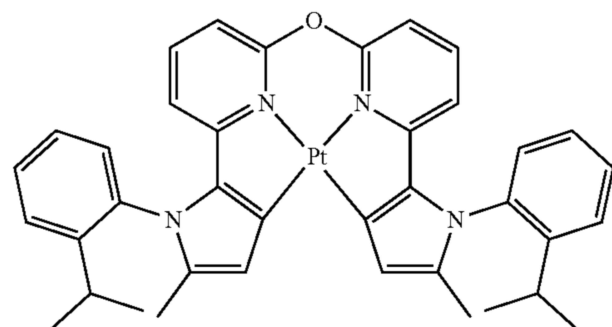
Compound 106
