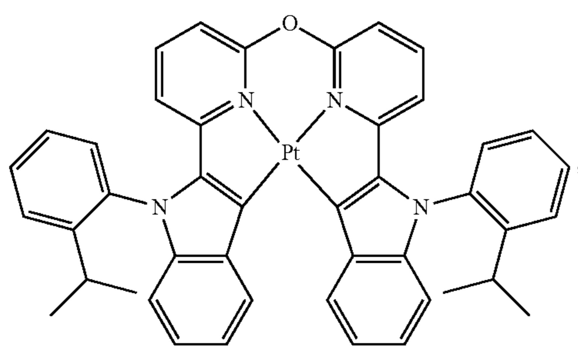
Compound 103
