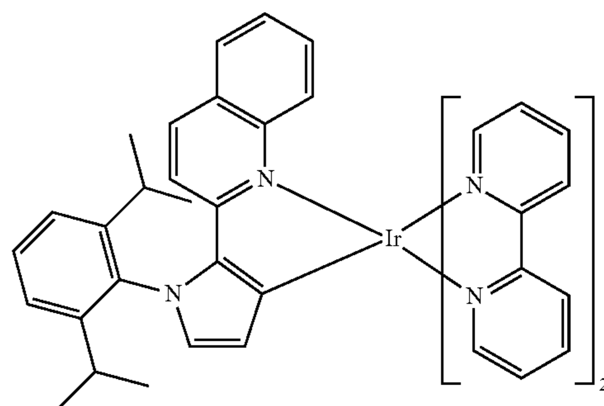
Compound 79
