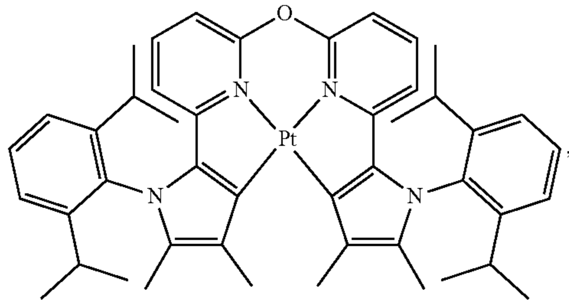
Compound 110
