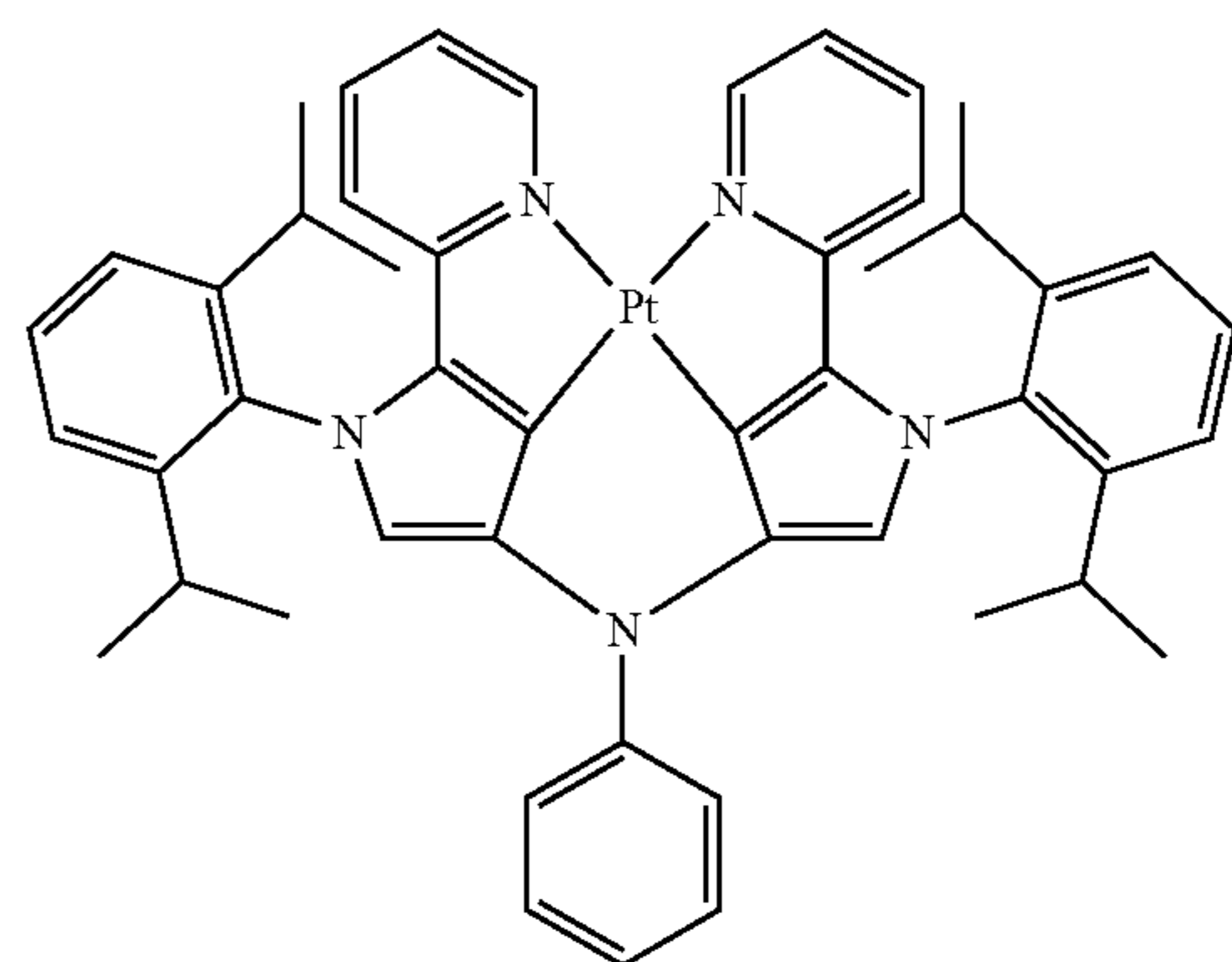
Compound 111
