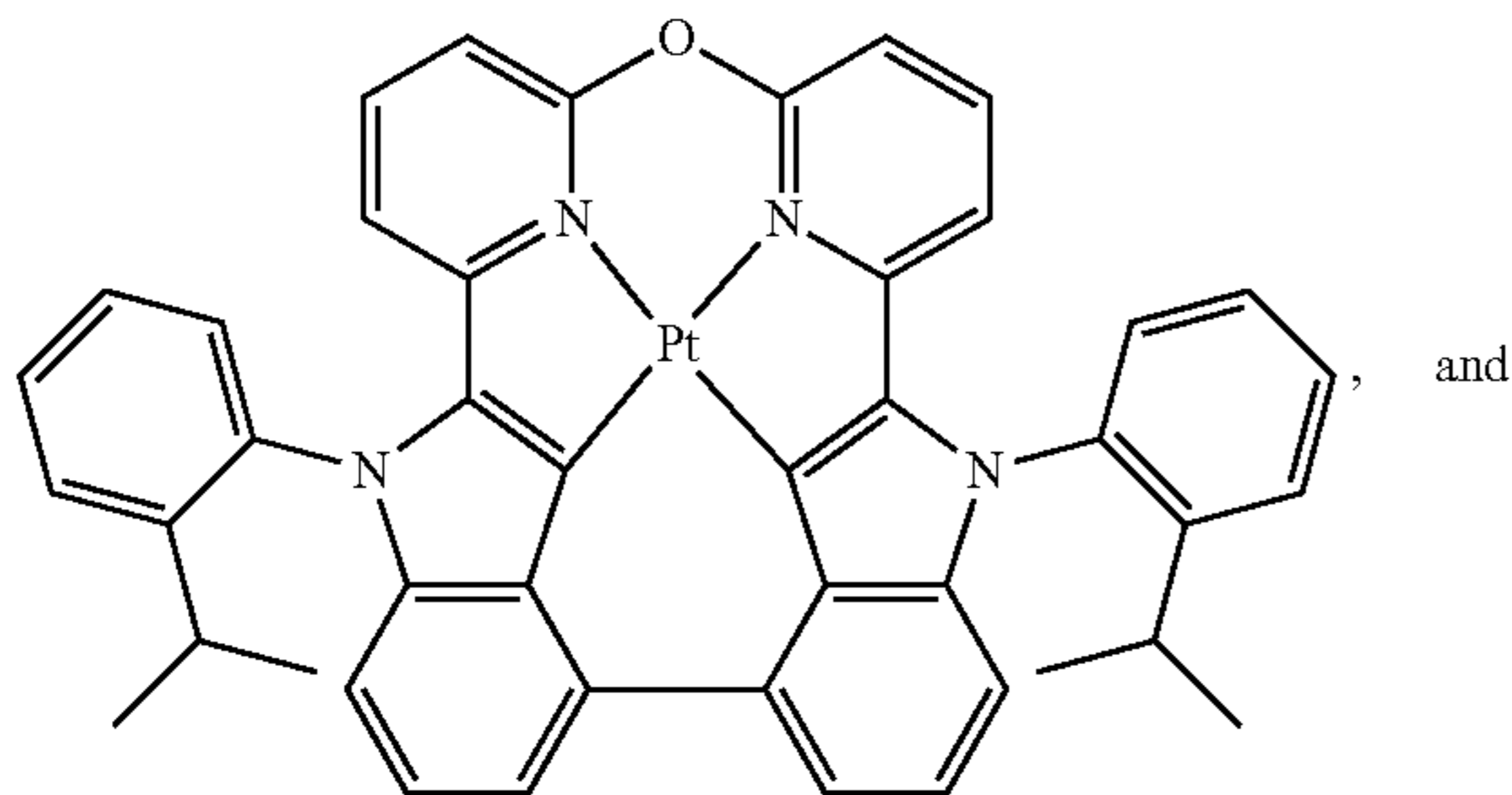
Compound 112
