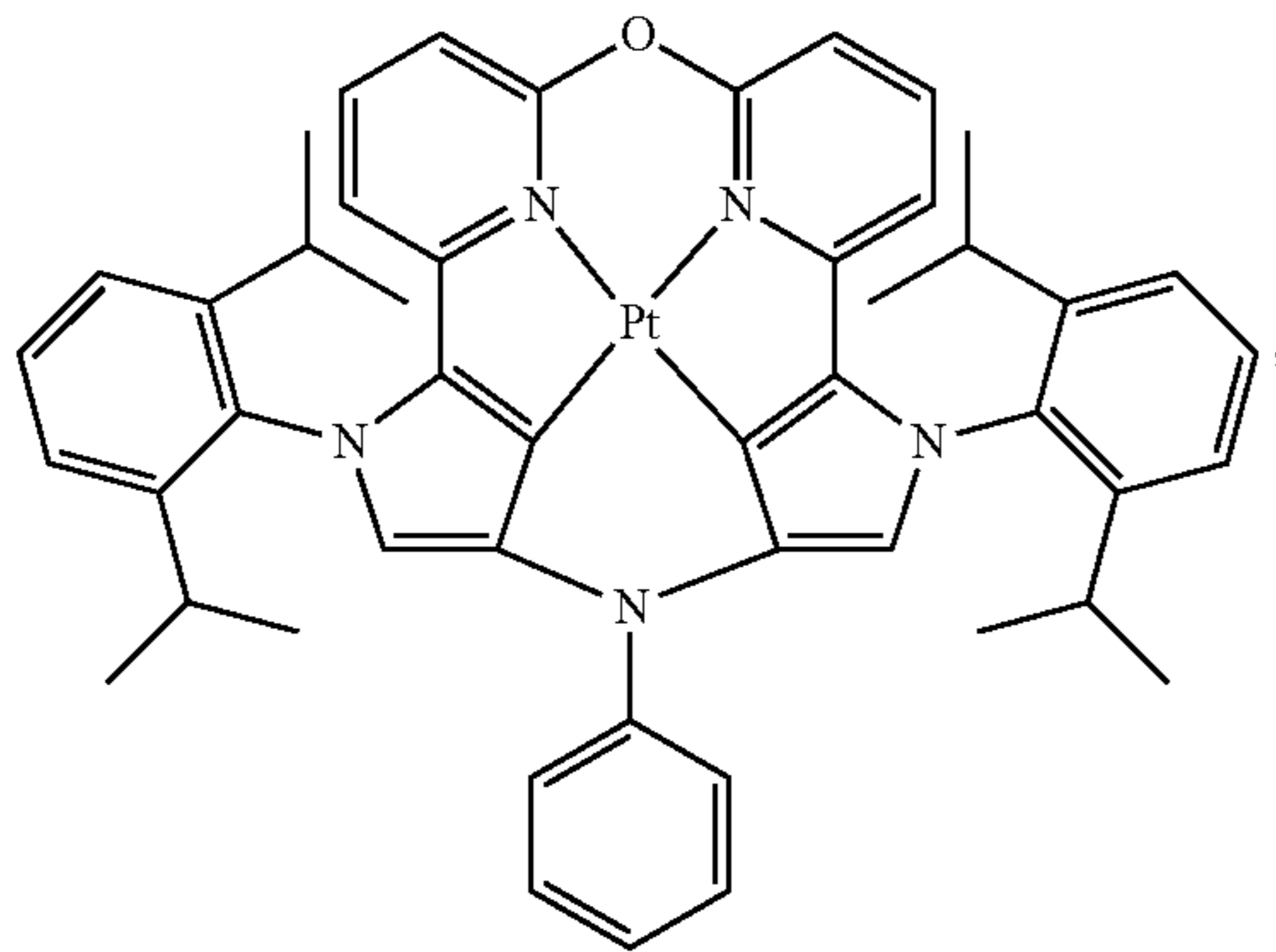
Compound 111
