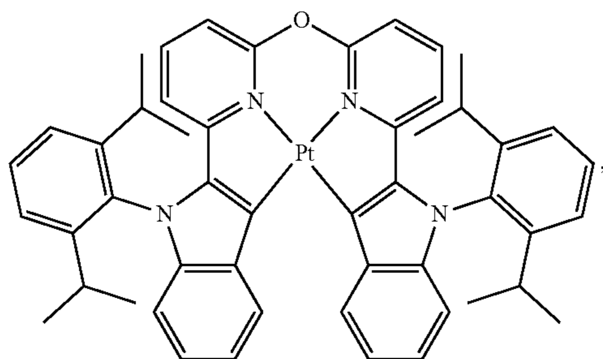
Compound 104
