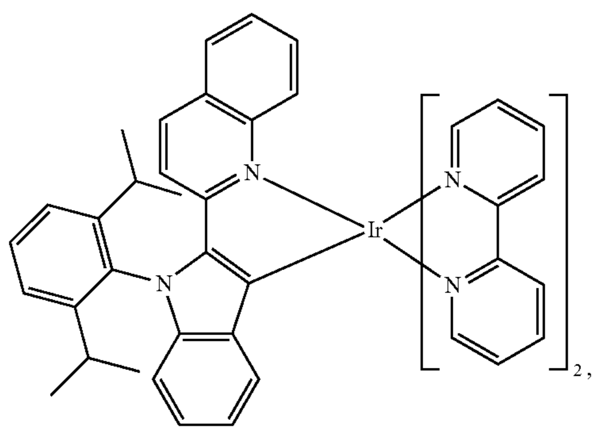
Compound 81
