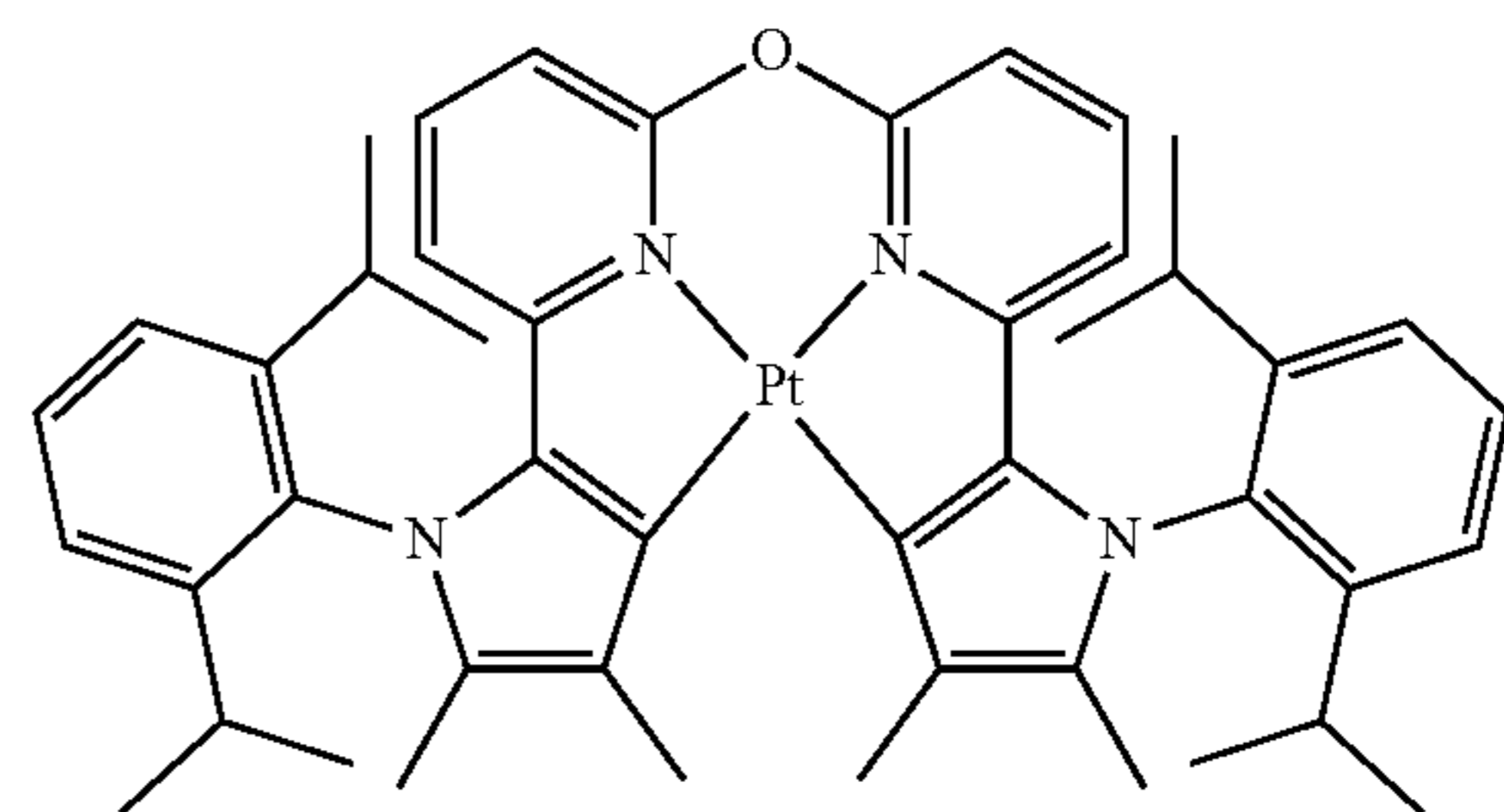
Compound 109
