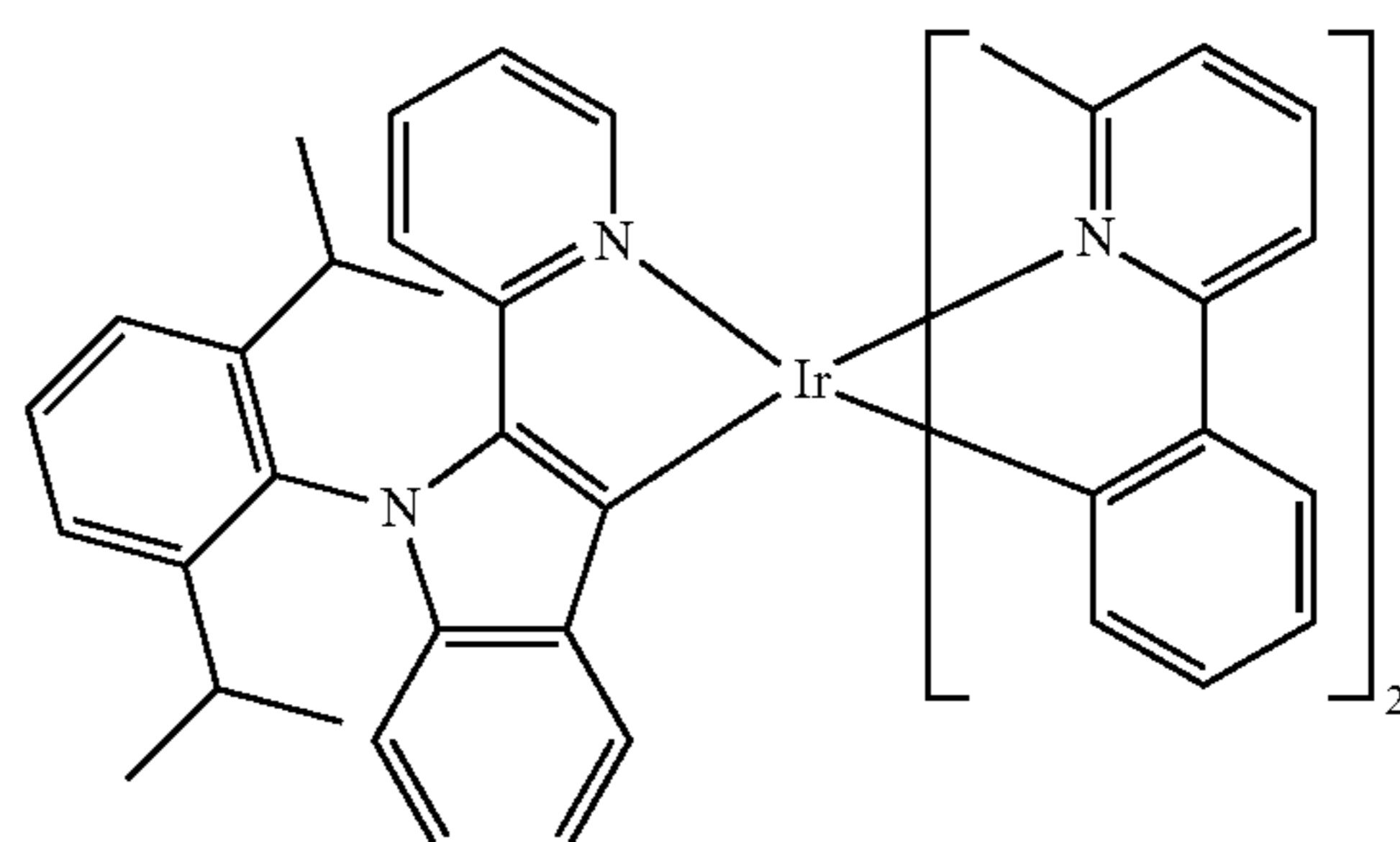
Compound 63
