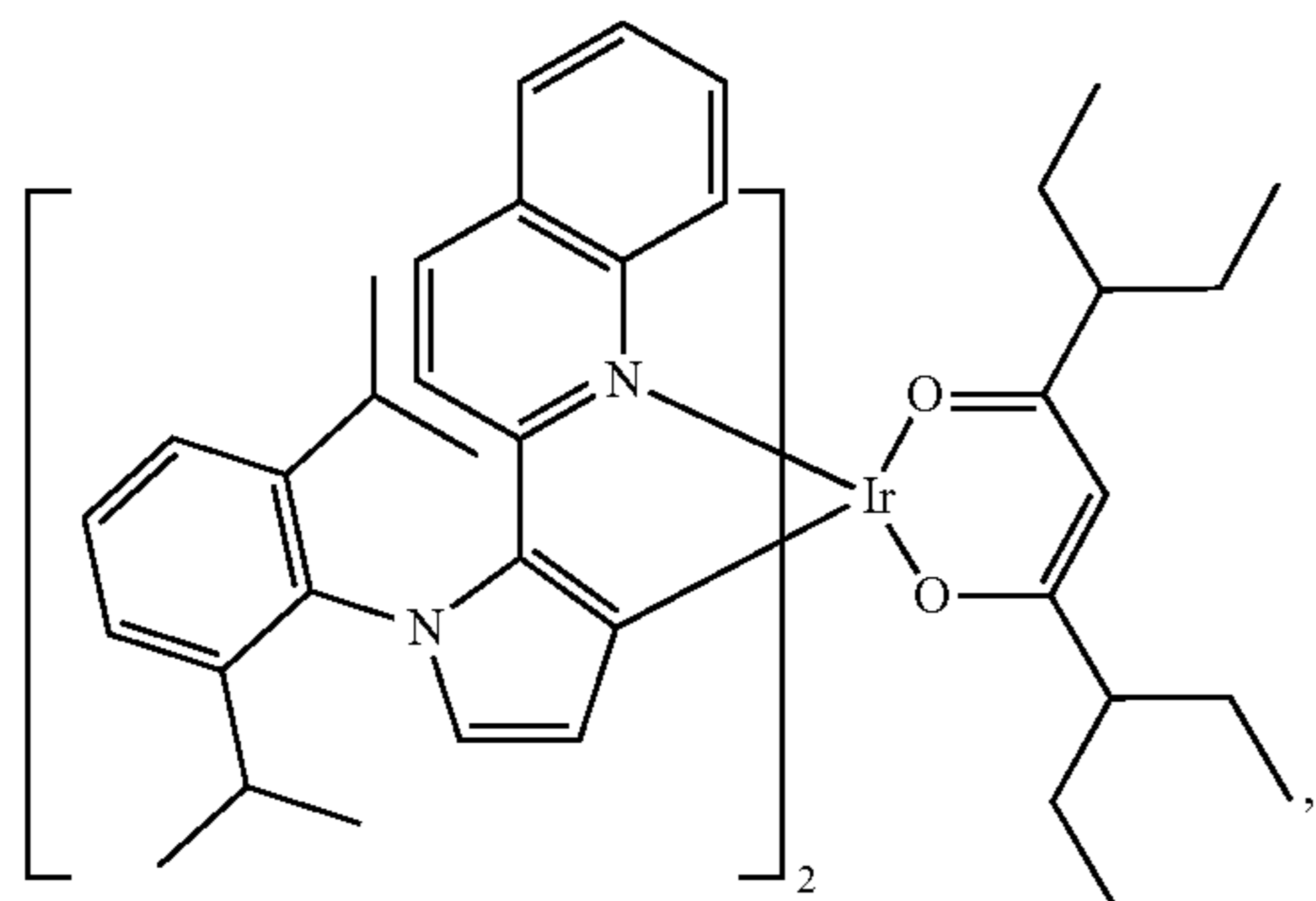
Compound 75
