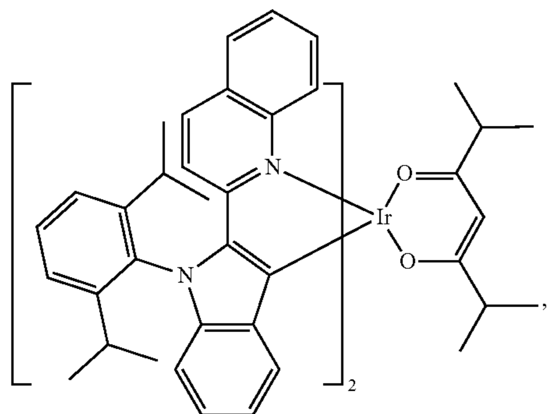
Compound 78
