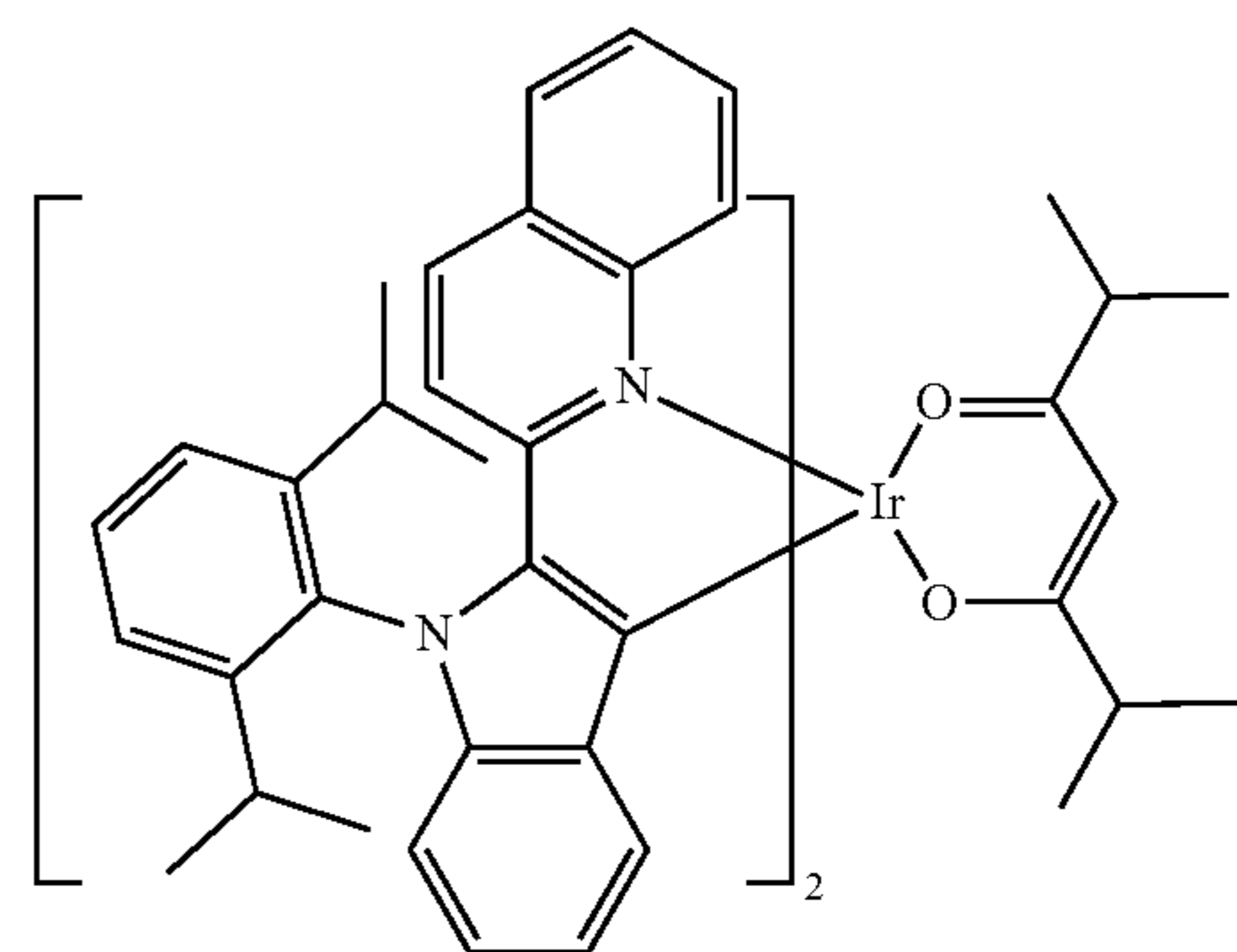
Compound 77
