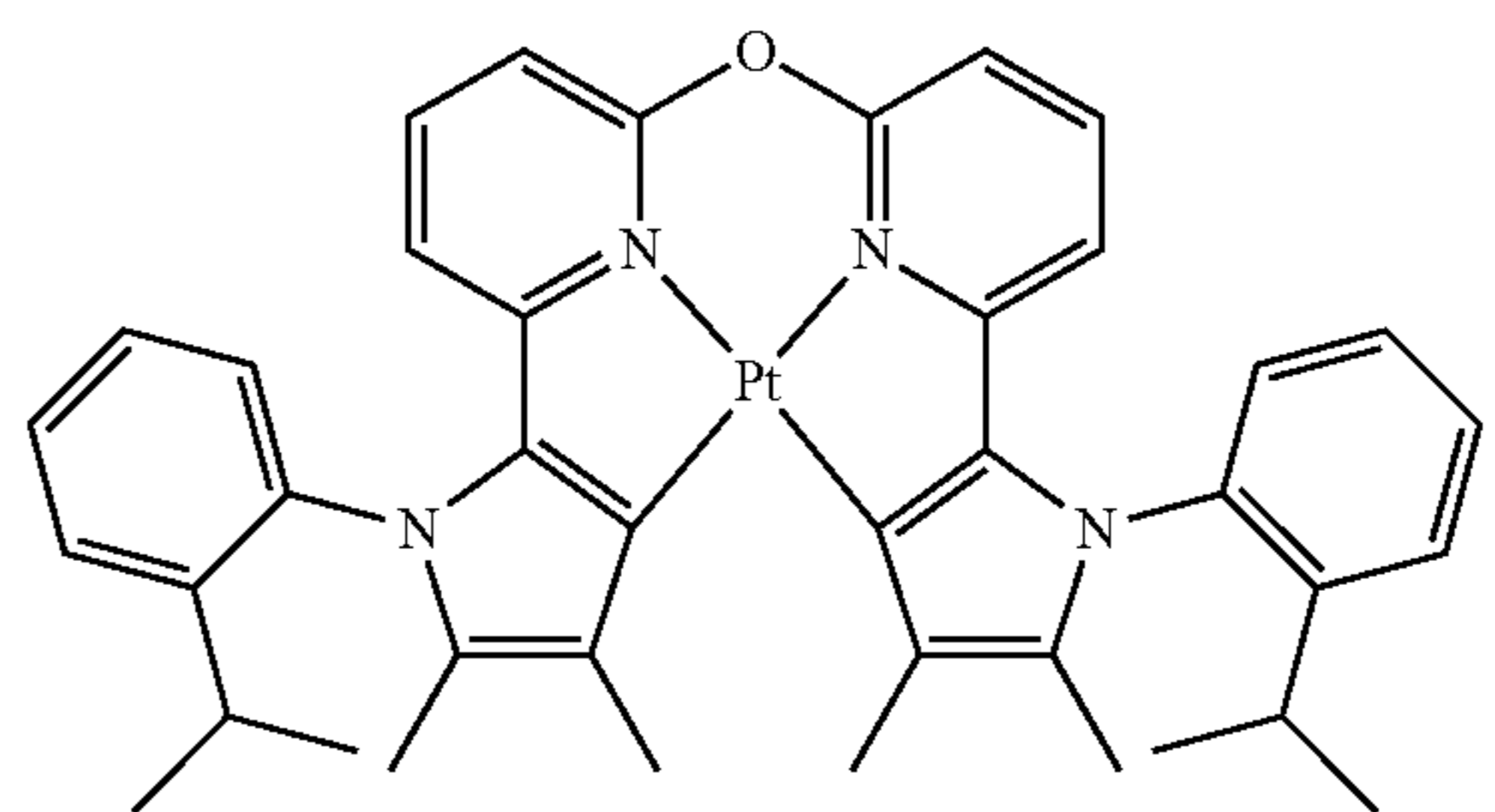
Compound 109
