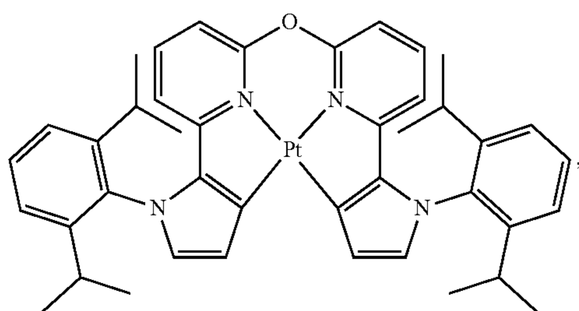
Compound 105
