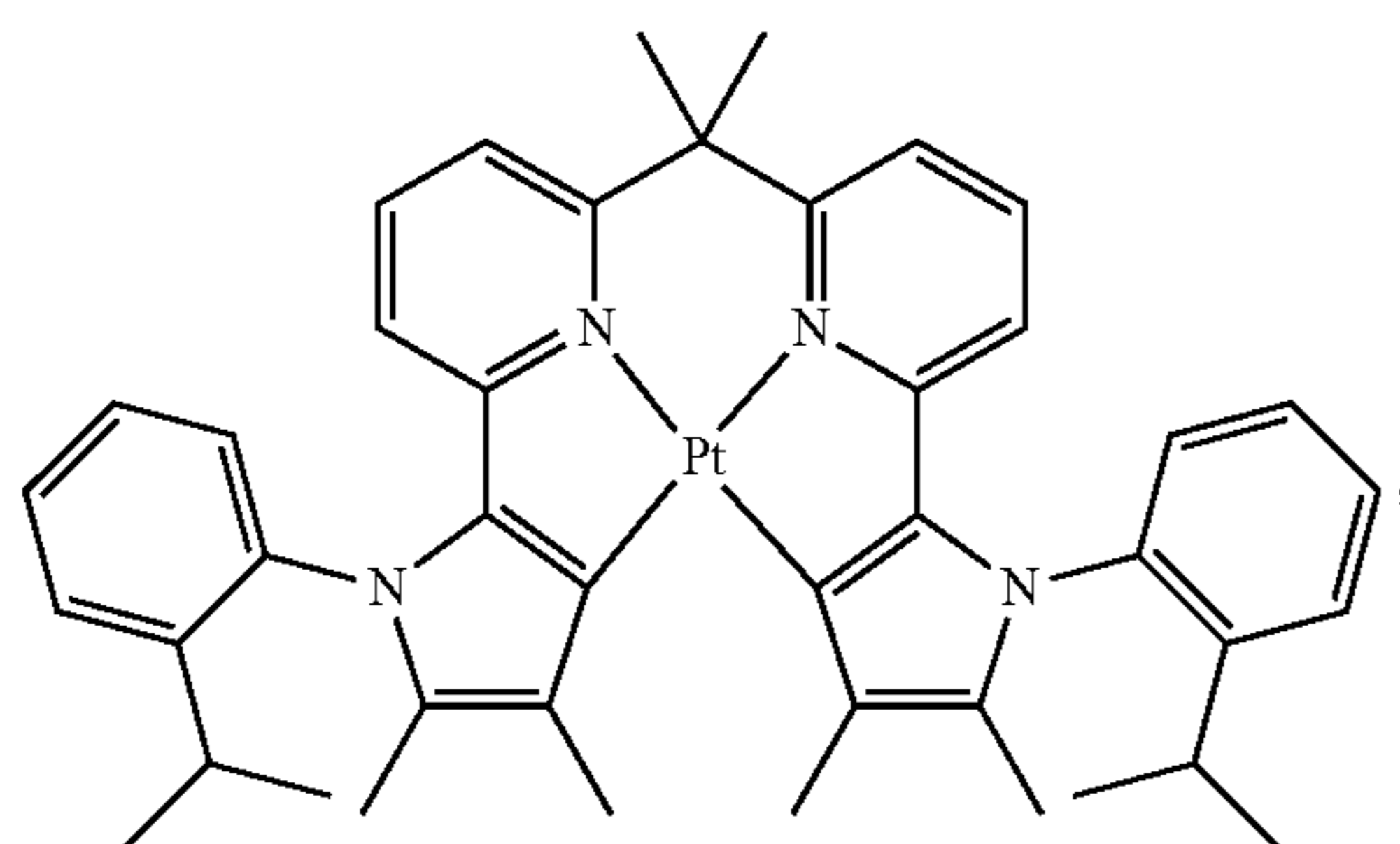
Compound 101
