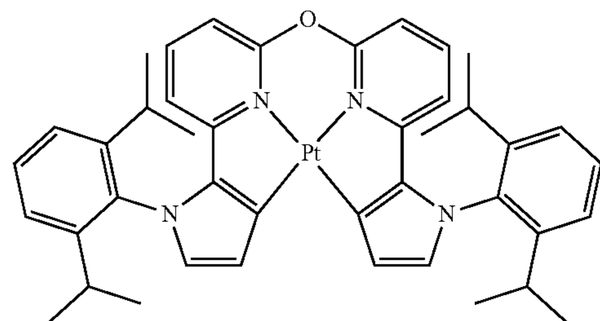
Compound 106
