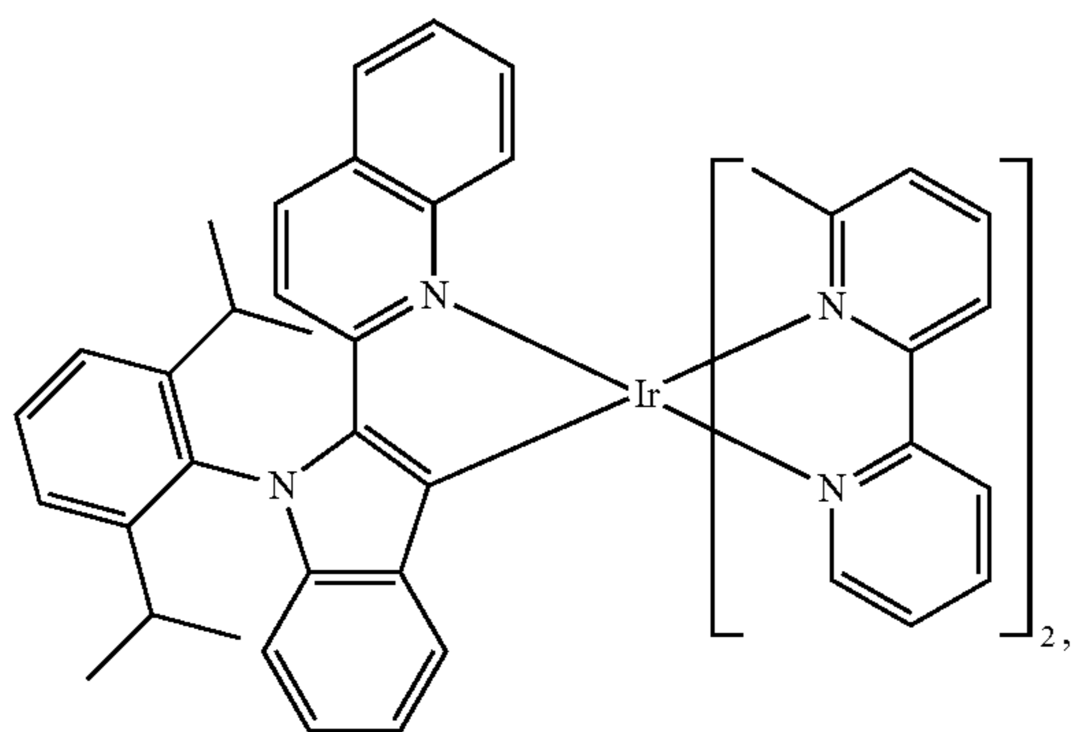
Compound 82
