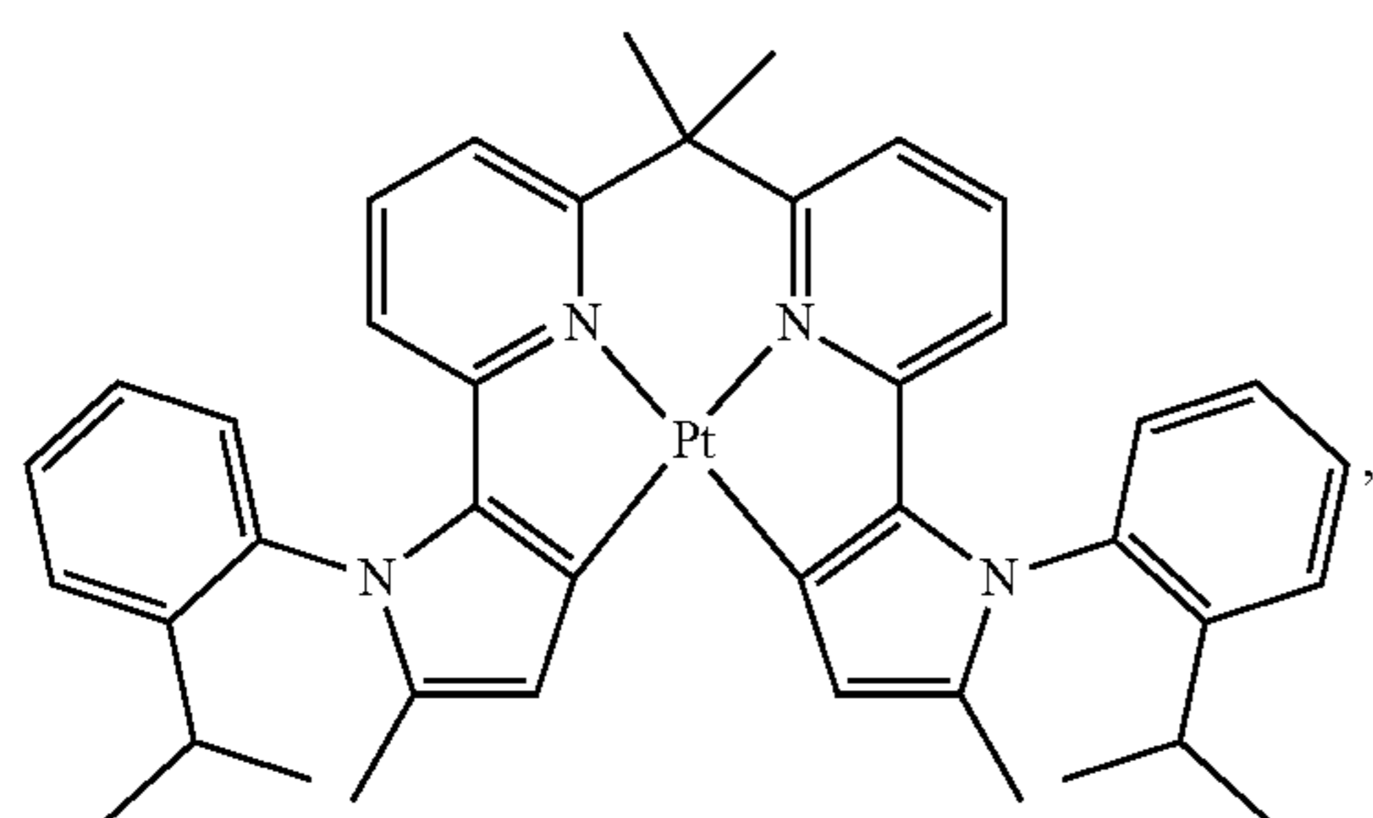
Compound 98
