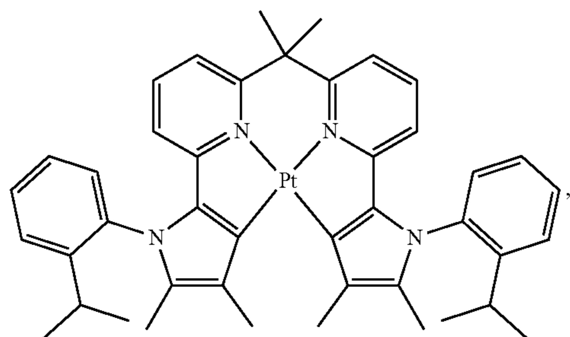
Compound 101
