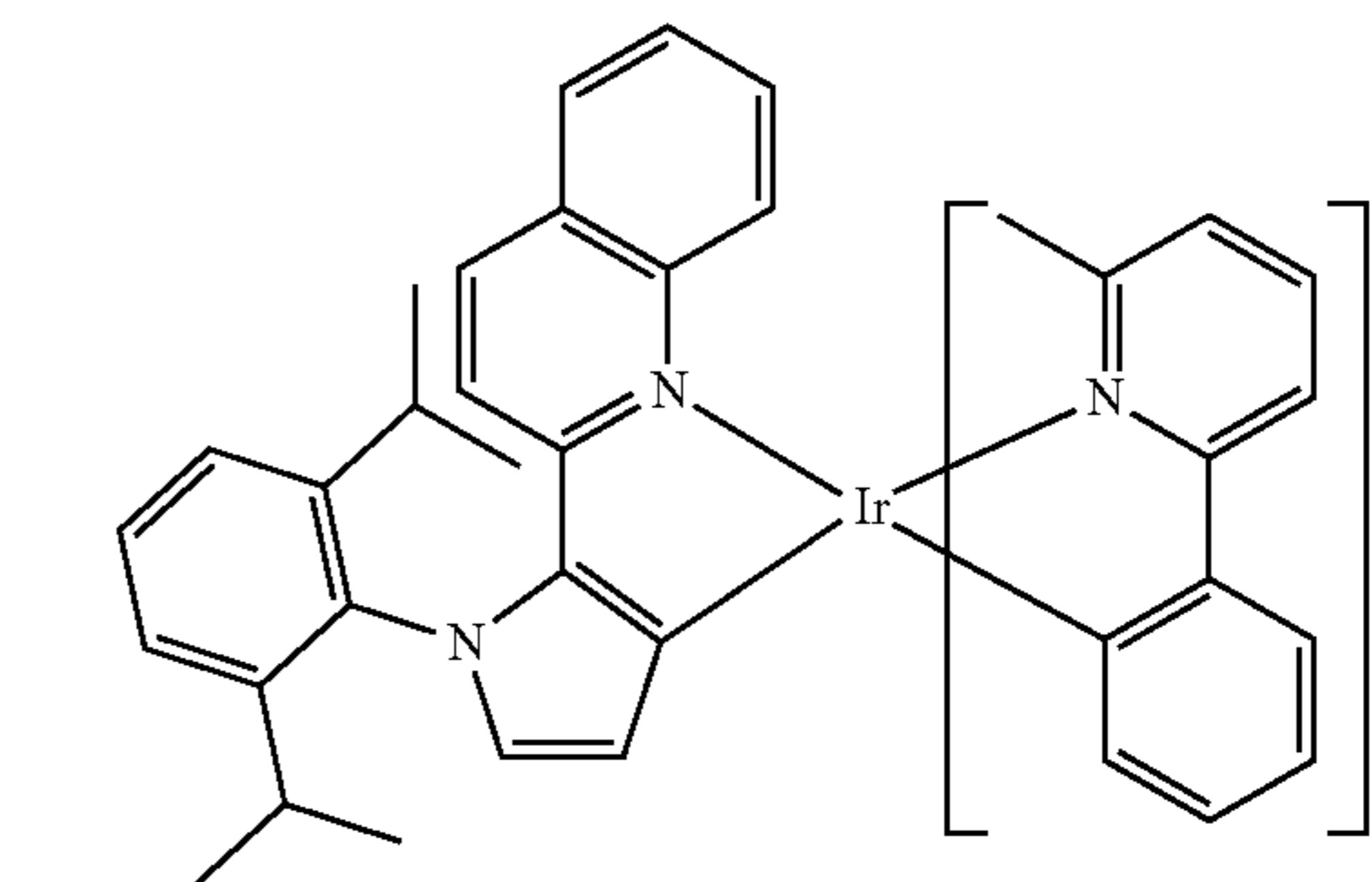
Compound 81
