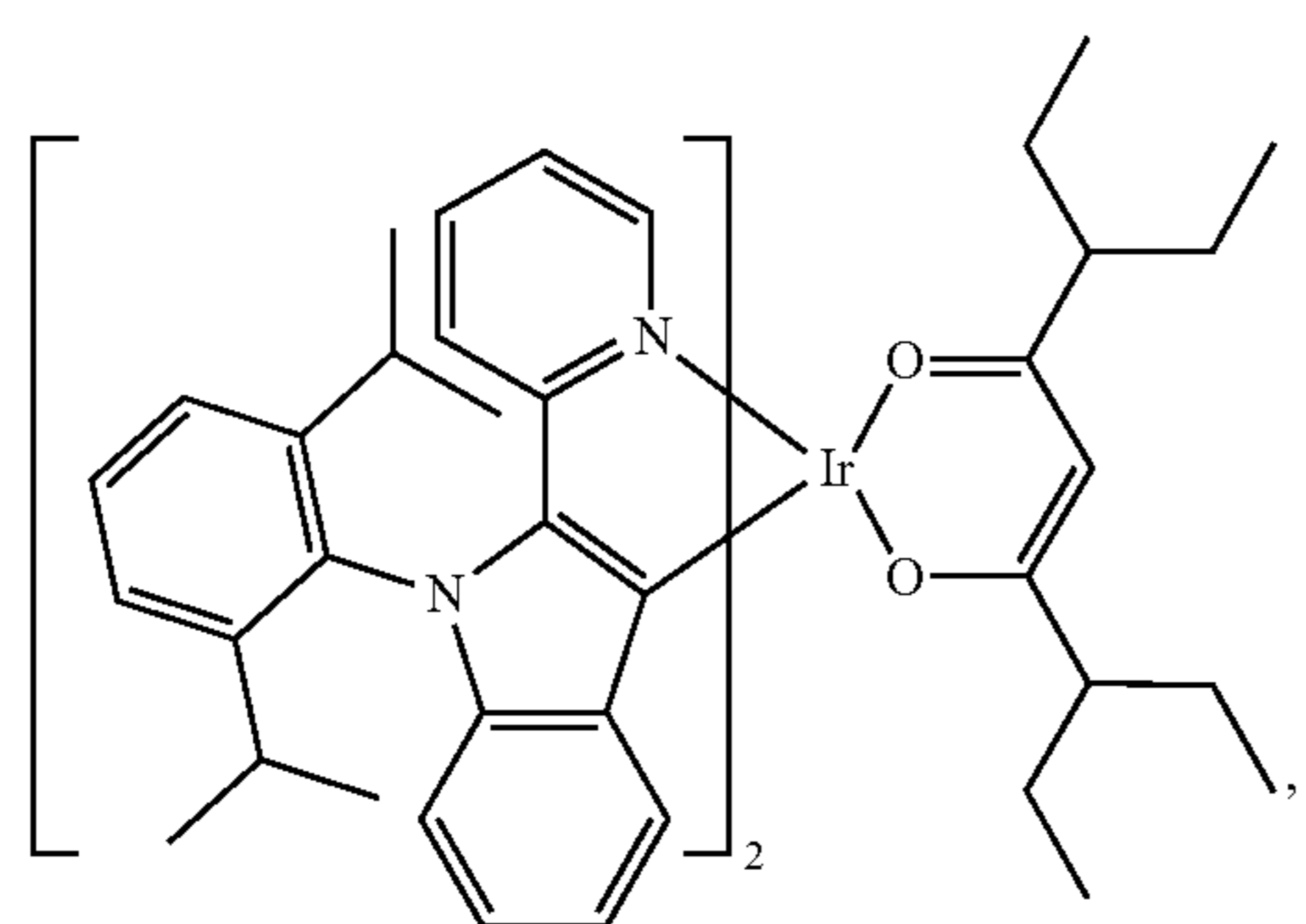
Compound 58
