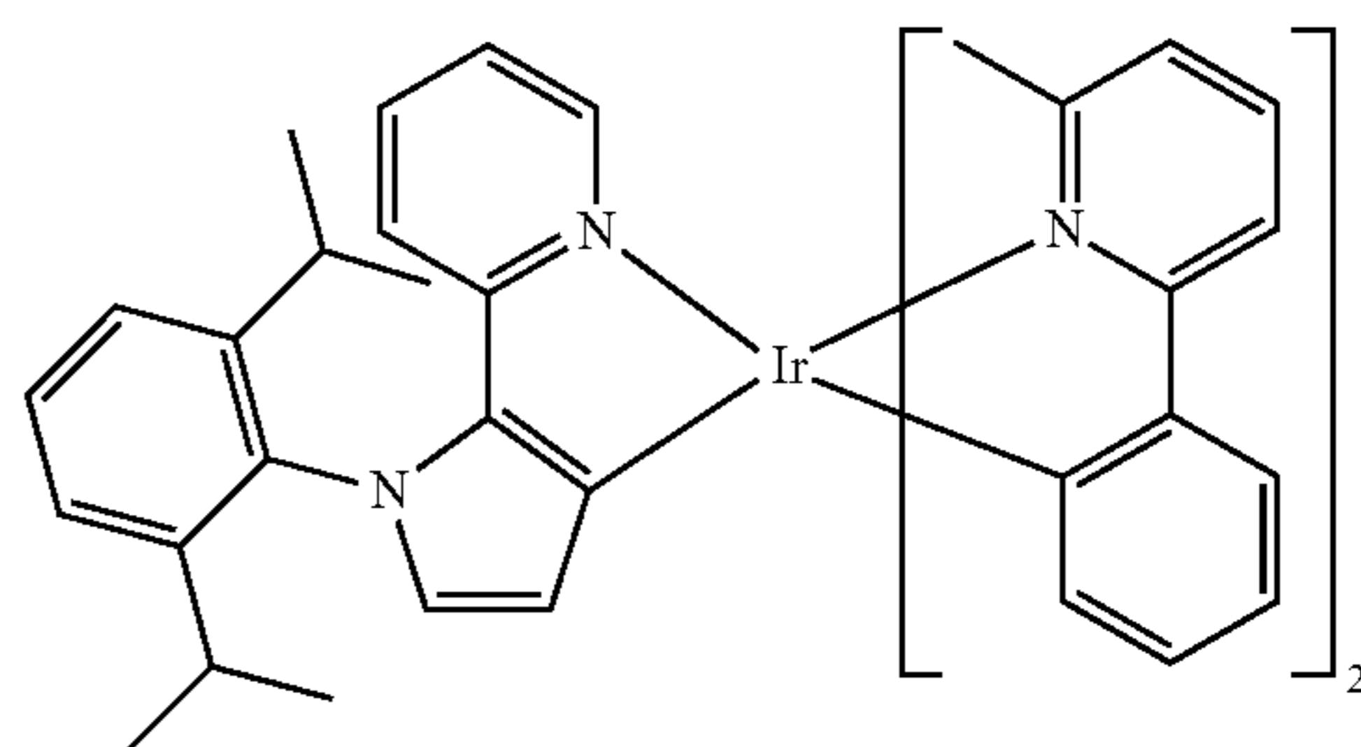
Compound 61
