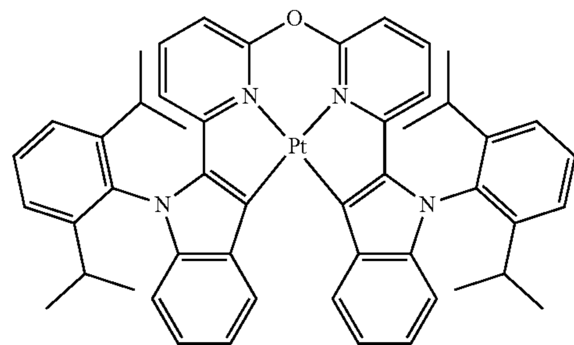
Compound 105
