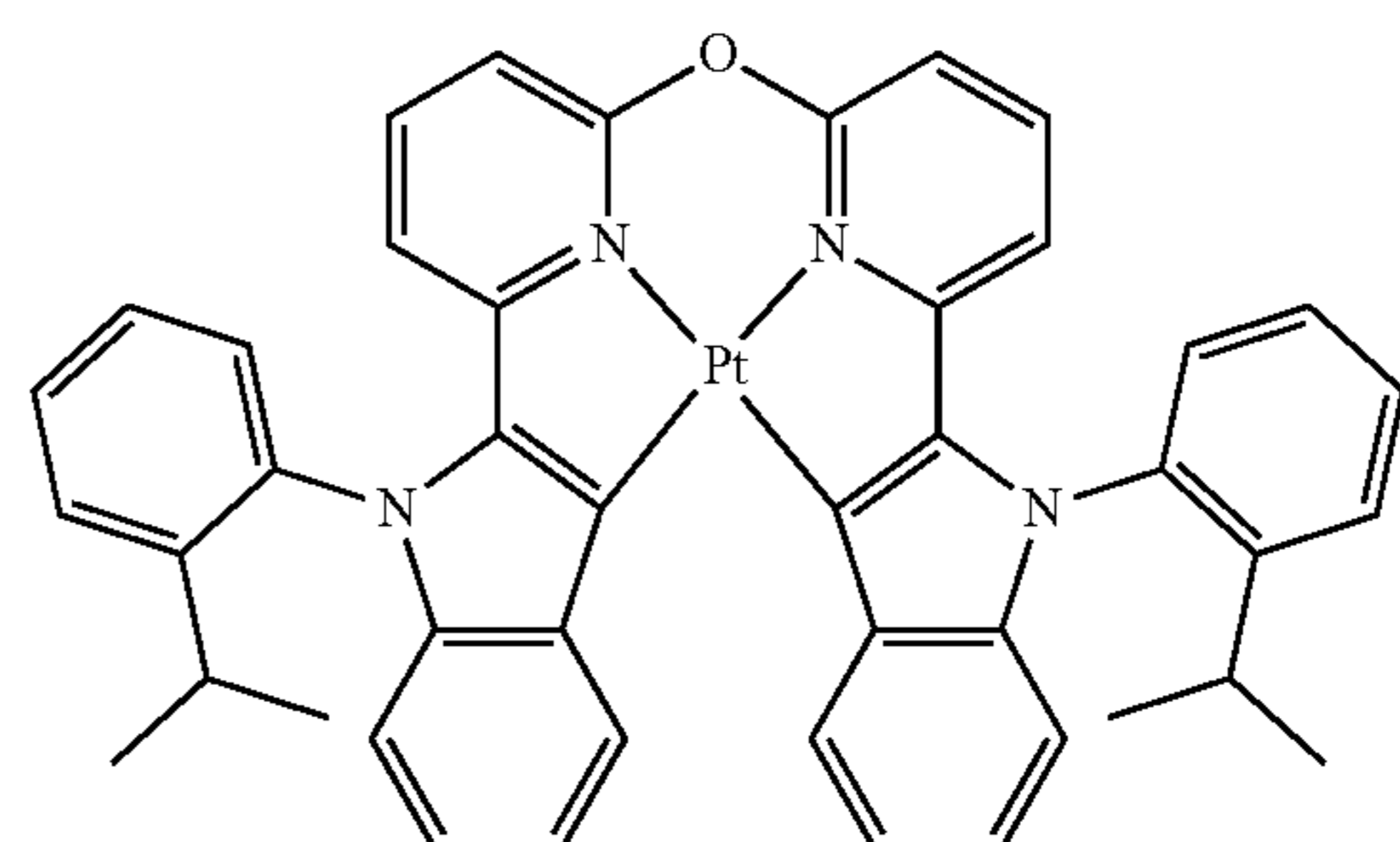
Compound 103
