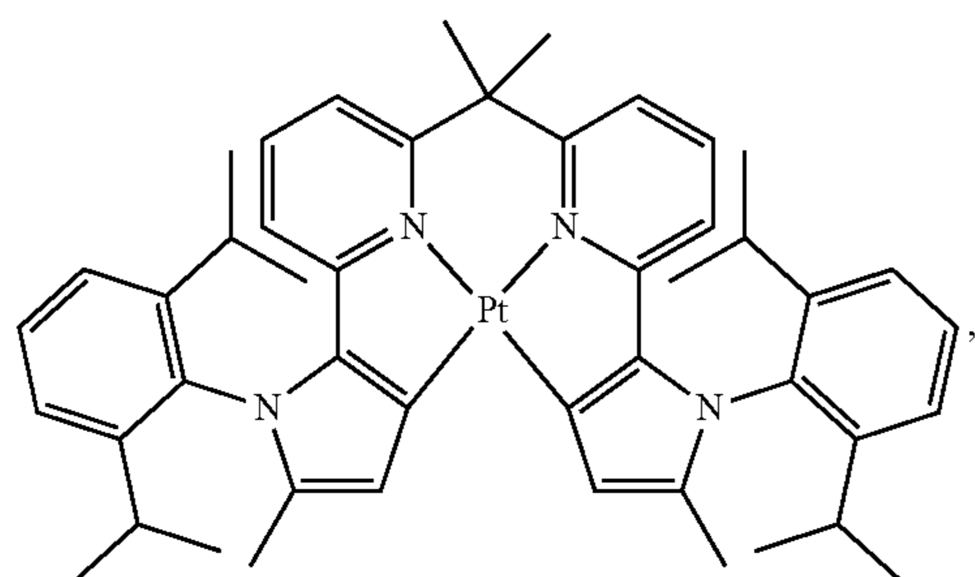
Compound 100
