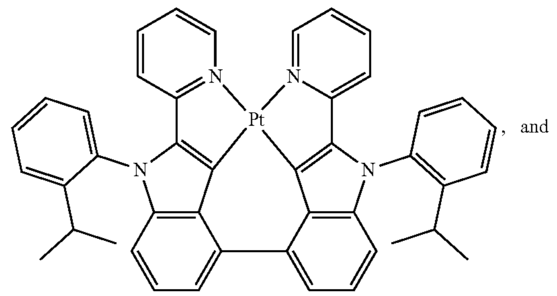
Compound 112
