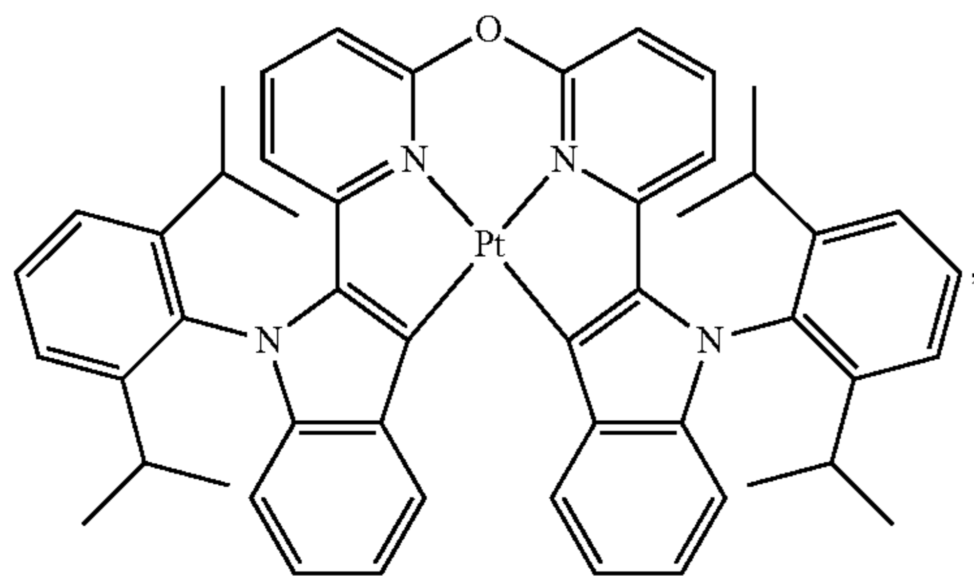
Compound 104
