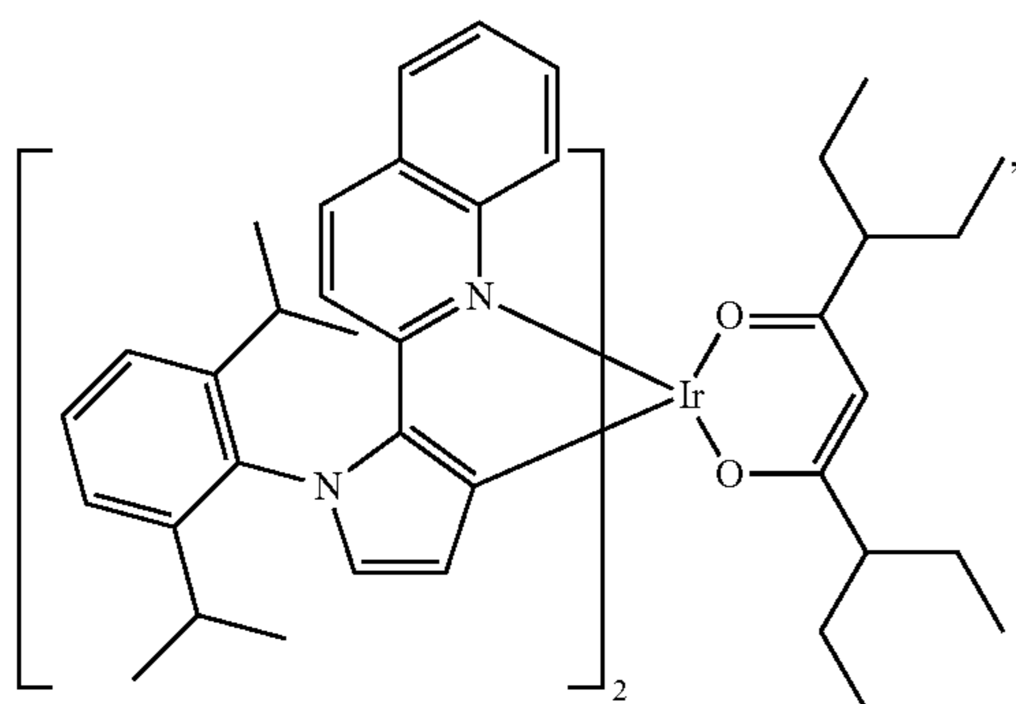
Compound 75
