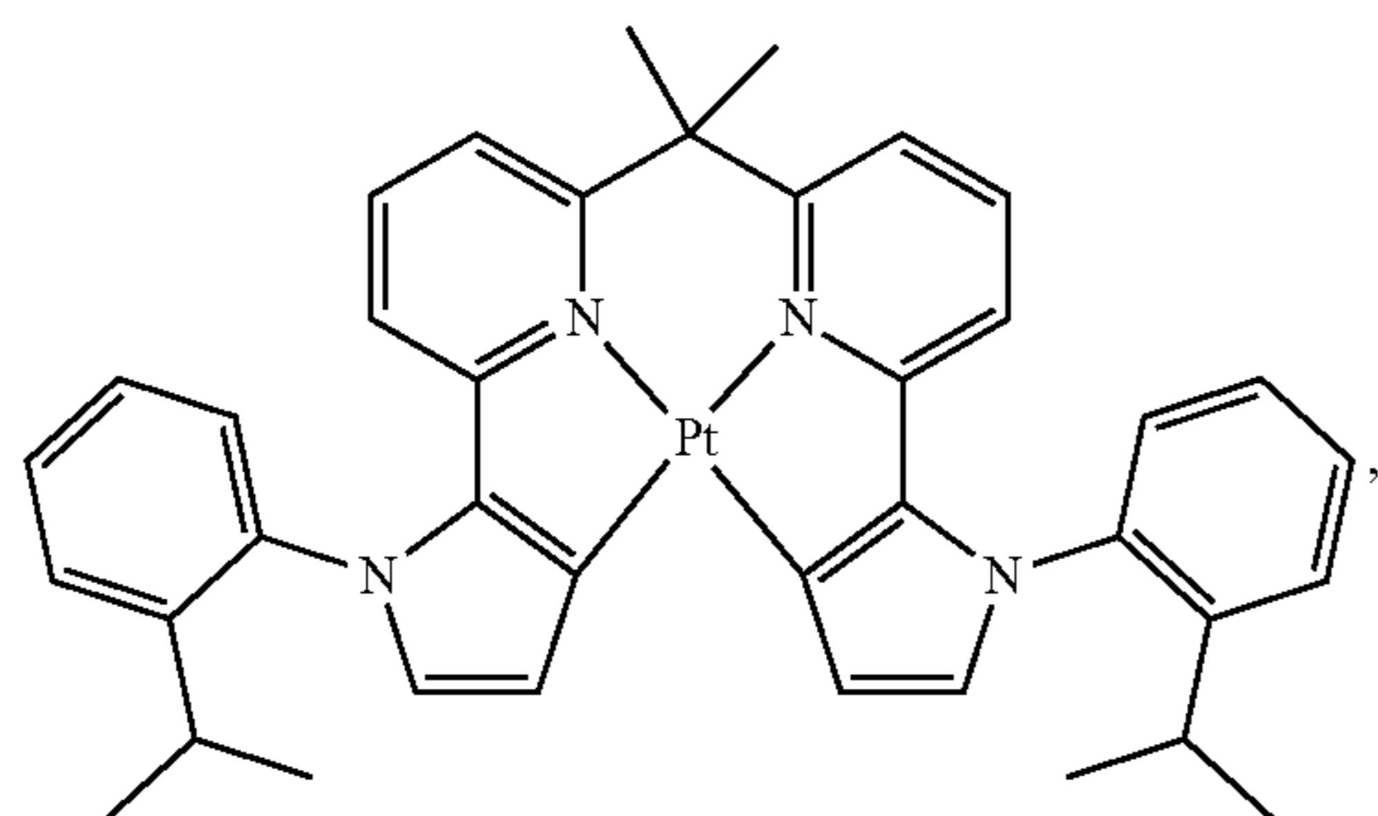
Compound 96
