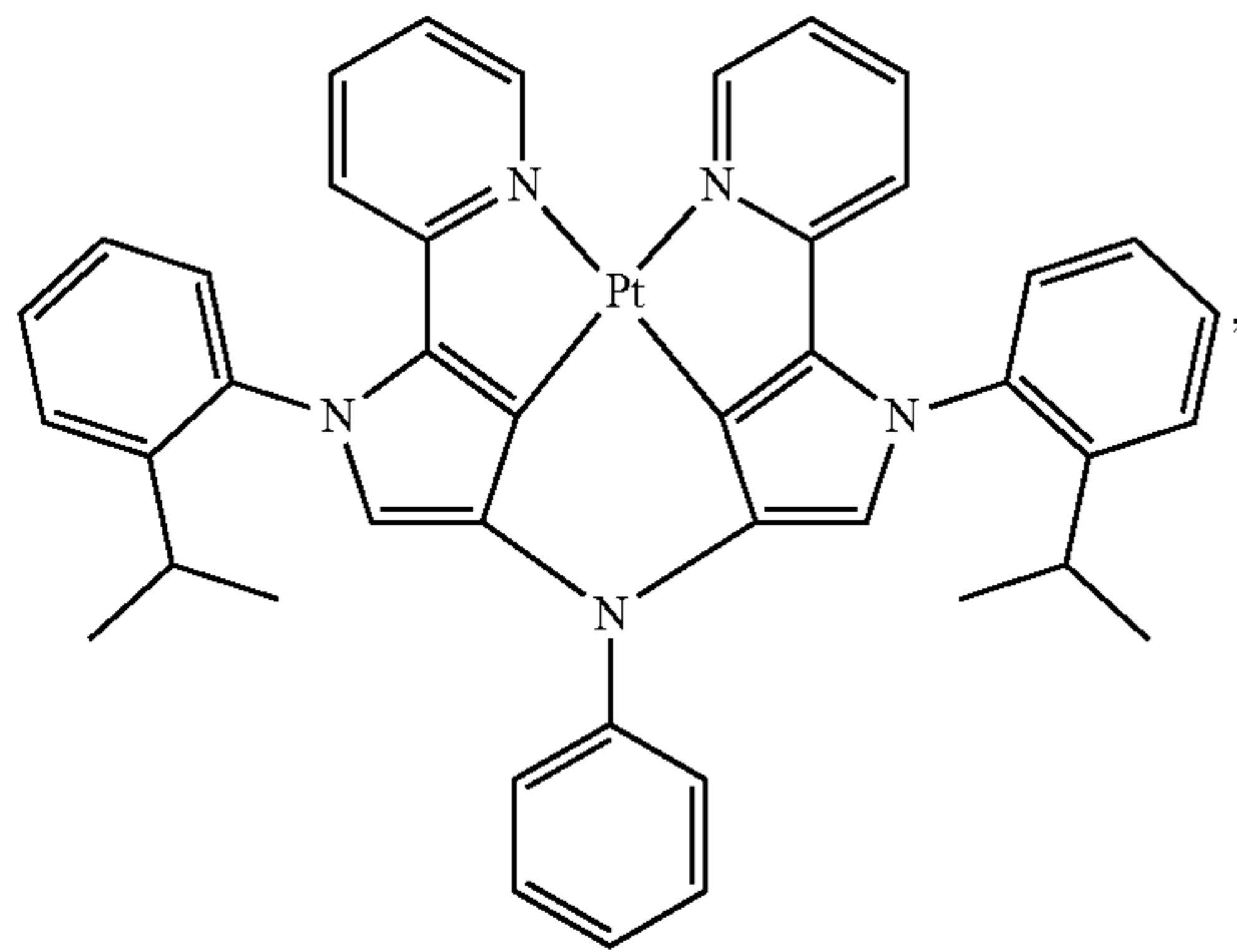
Compound 111
