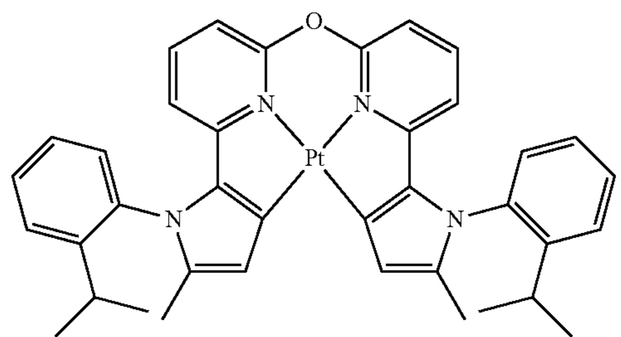
Compound 106
