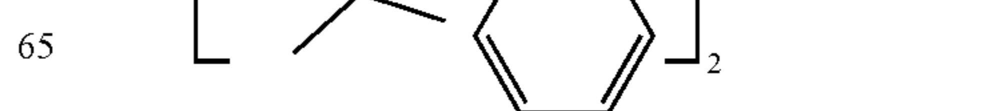
Compound 62
