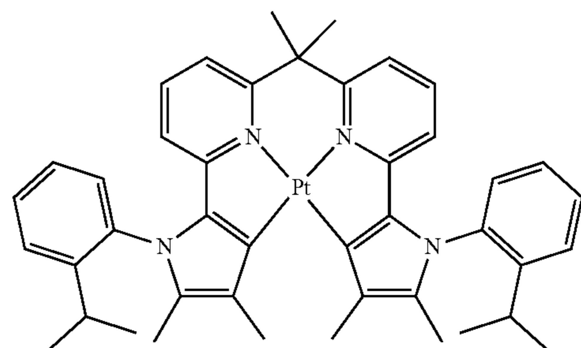
Compound 101
