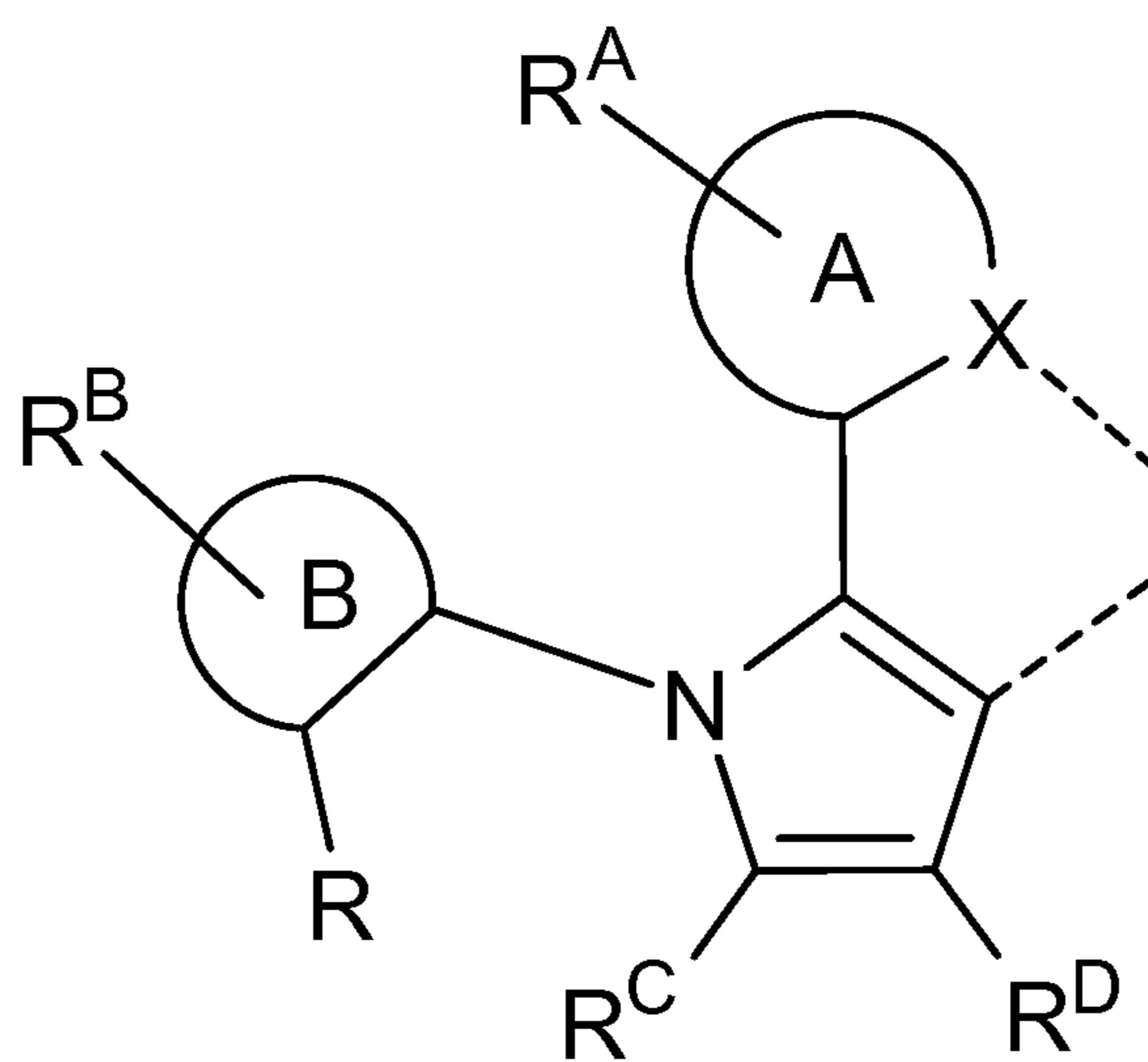
Formula I
