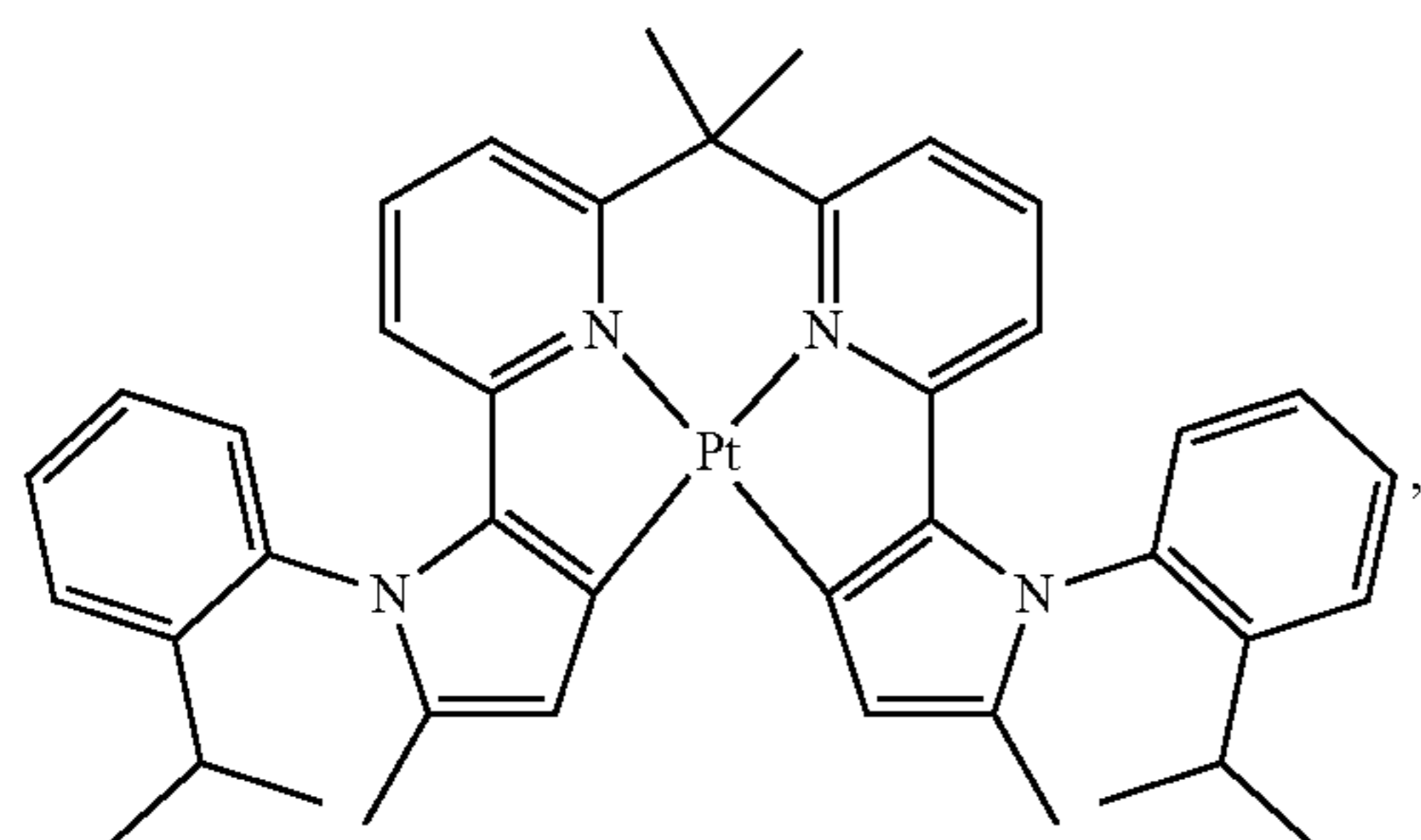
Compound 99
