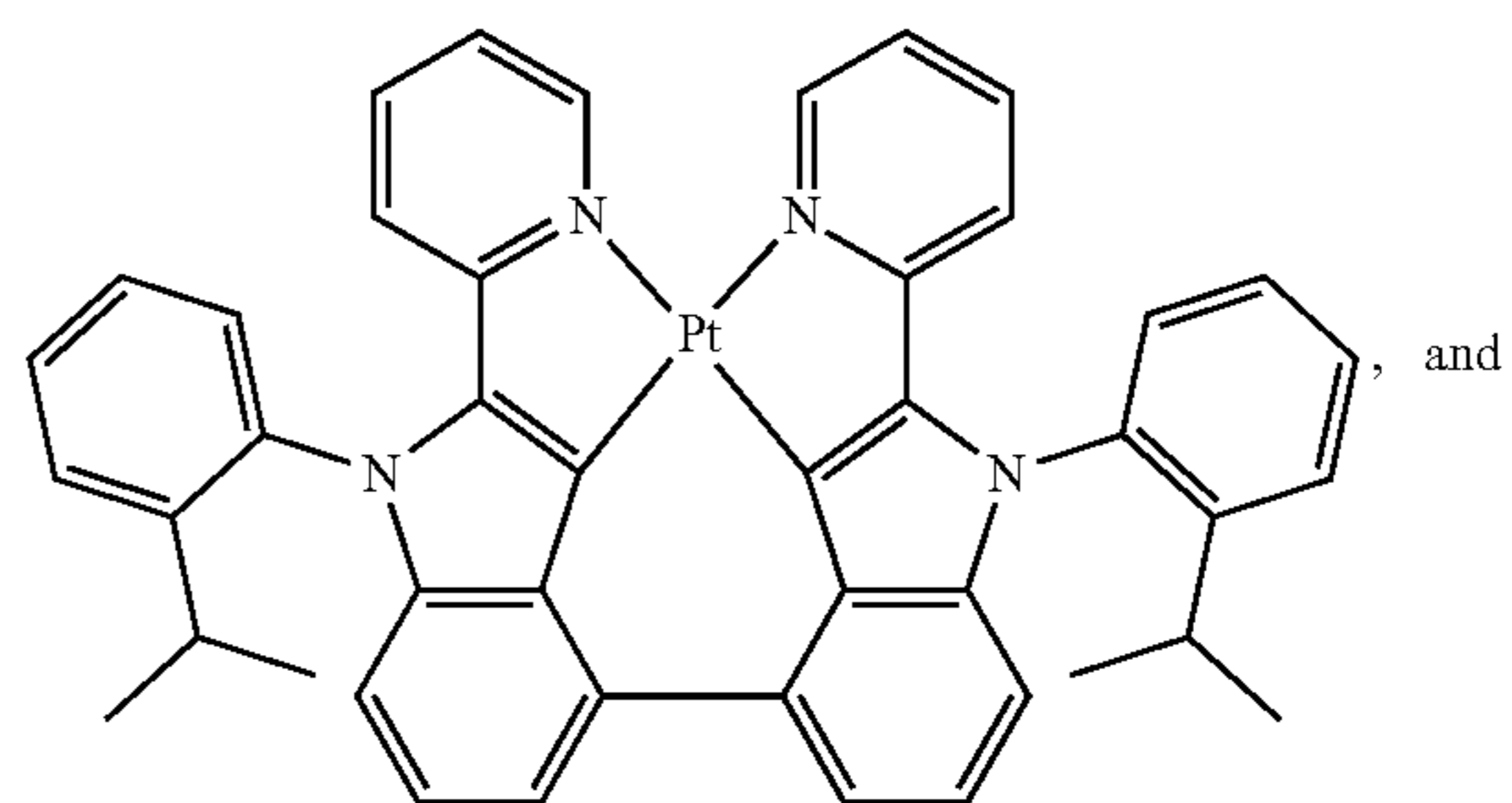
Compound 112
