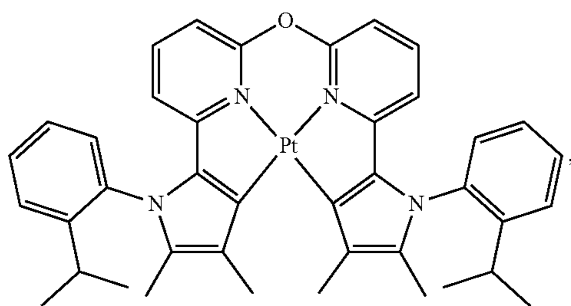
Compound 108
