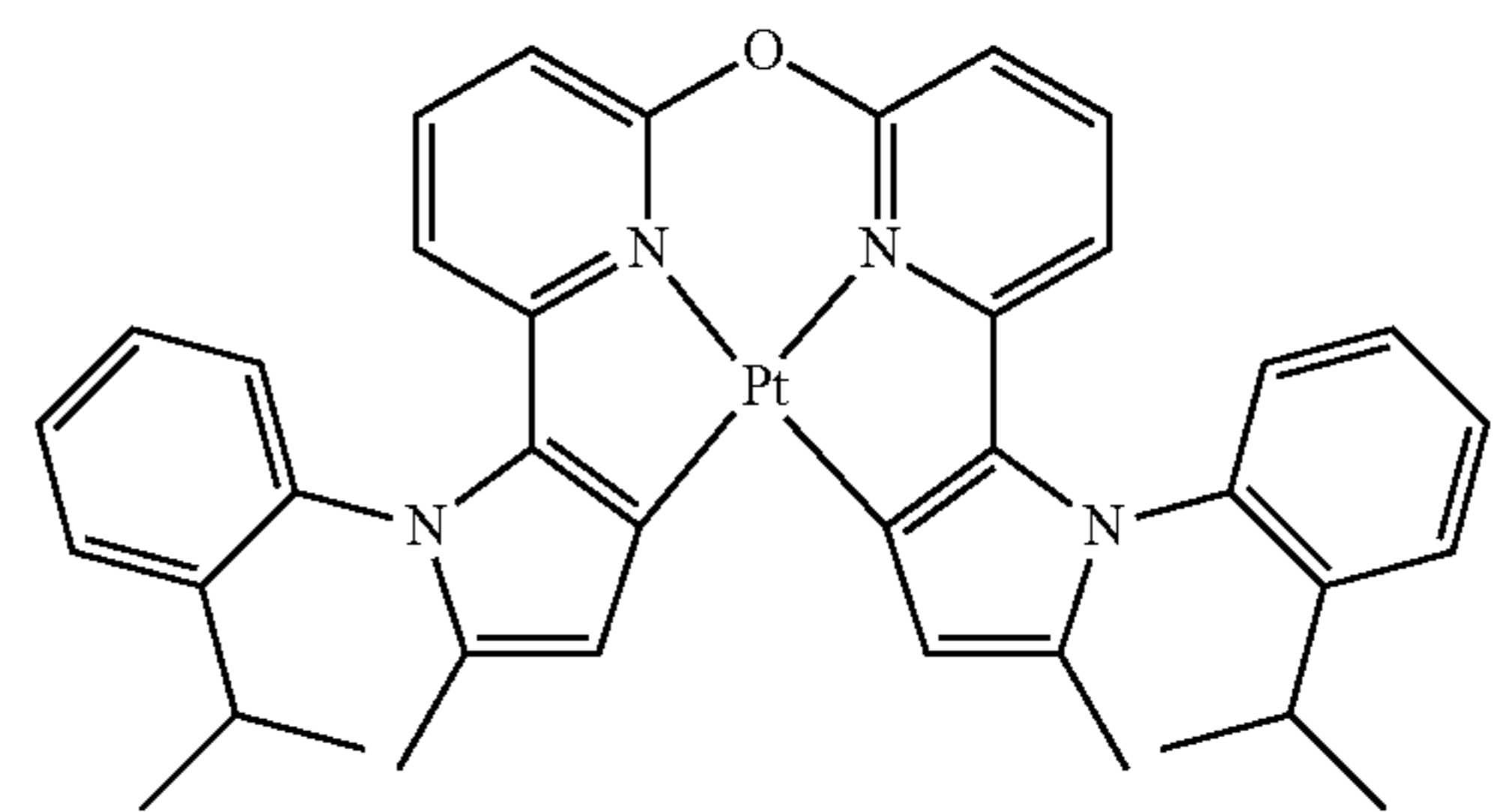
Compound 107
