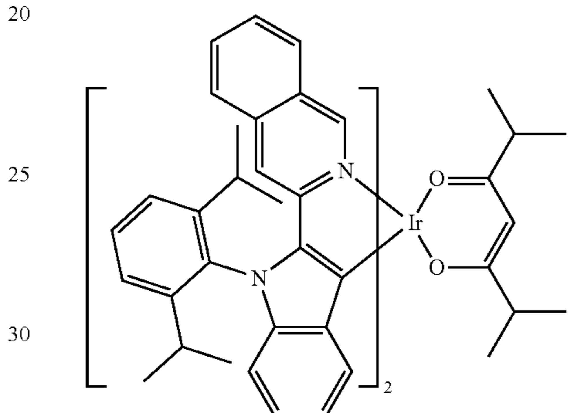
Compound 63
