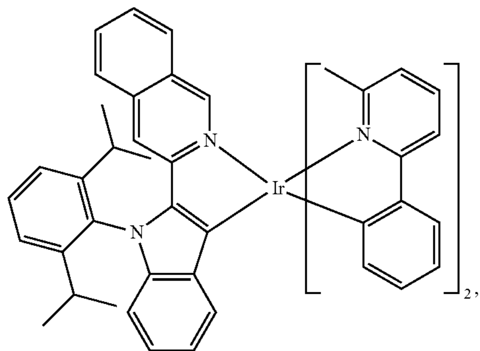
Compound 72
