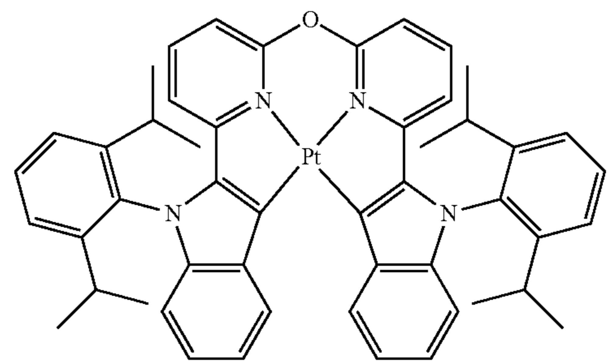
Compound 104
