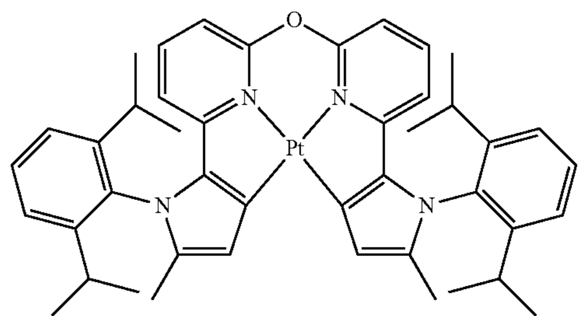
Compound 107
