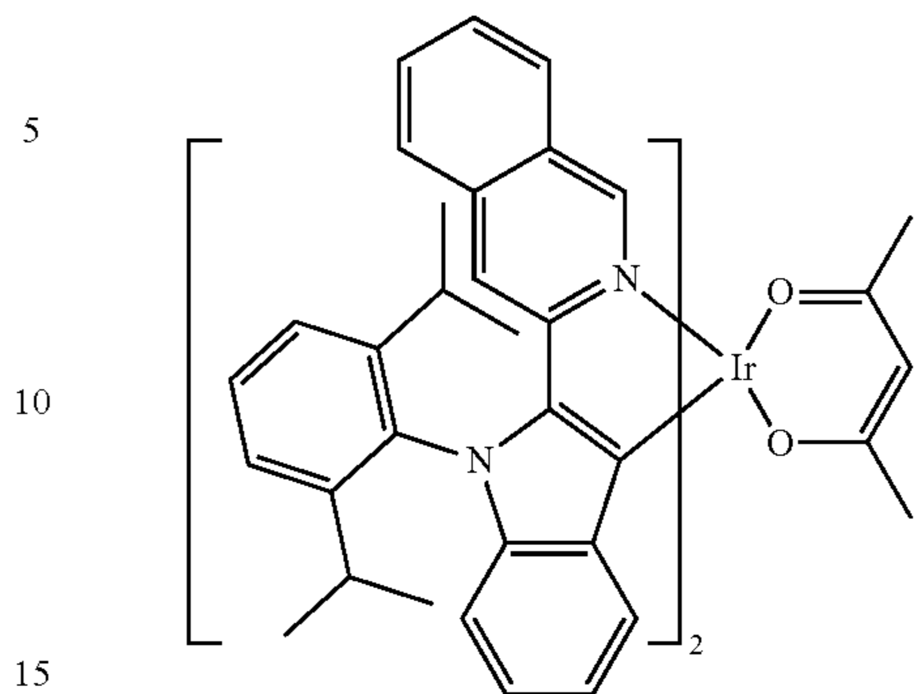
Compound 62
