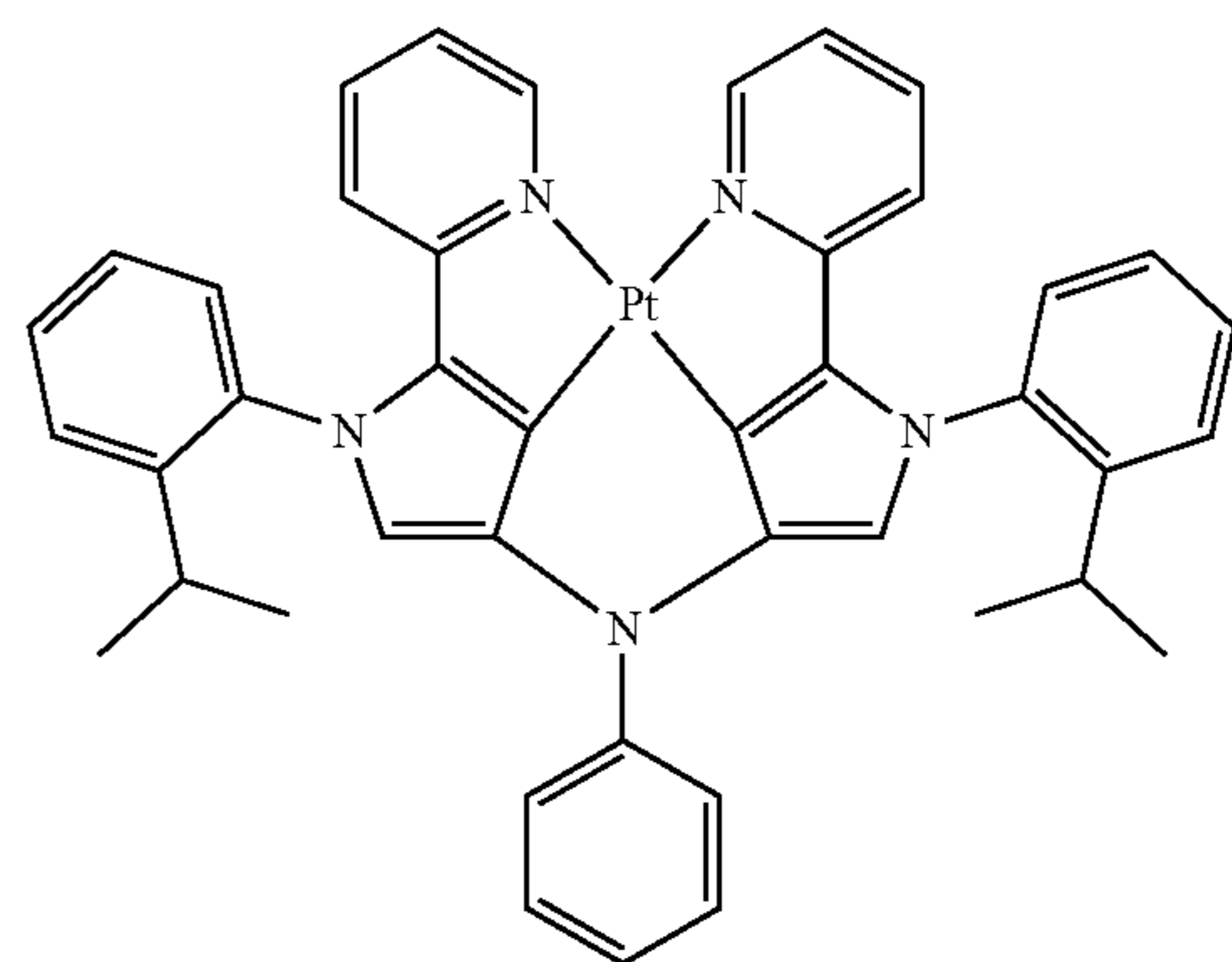
Compound 110
