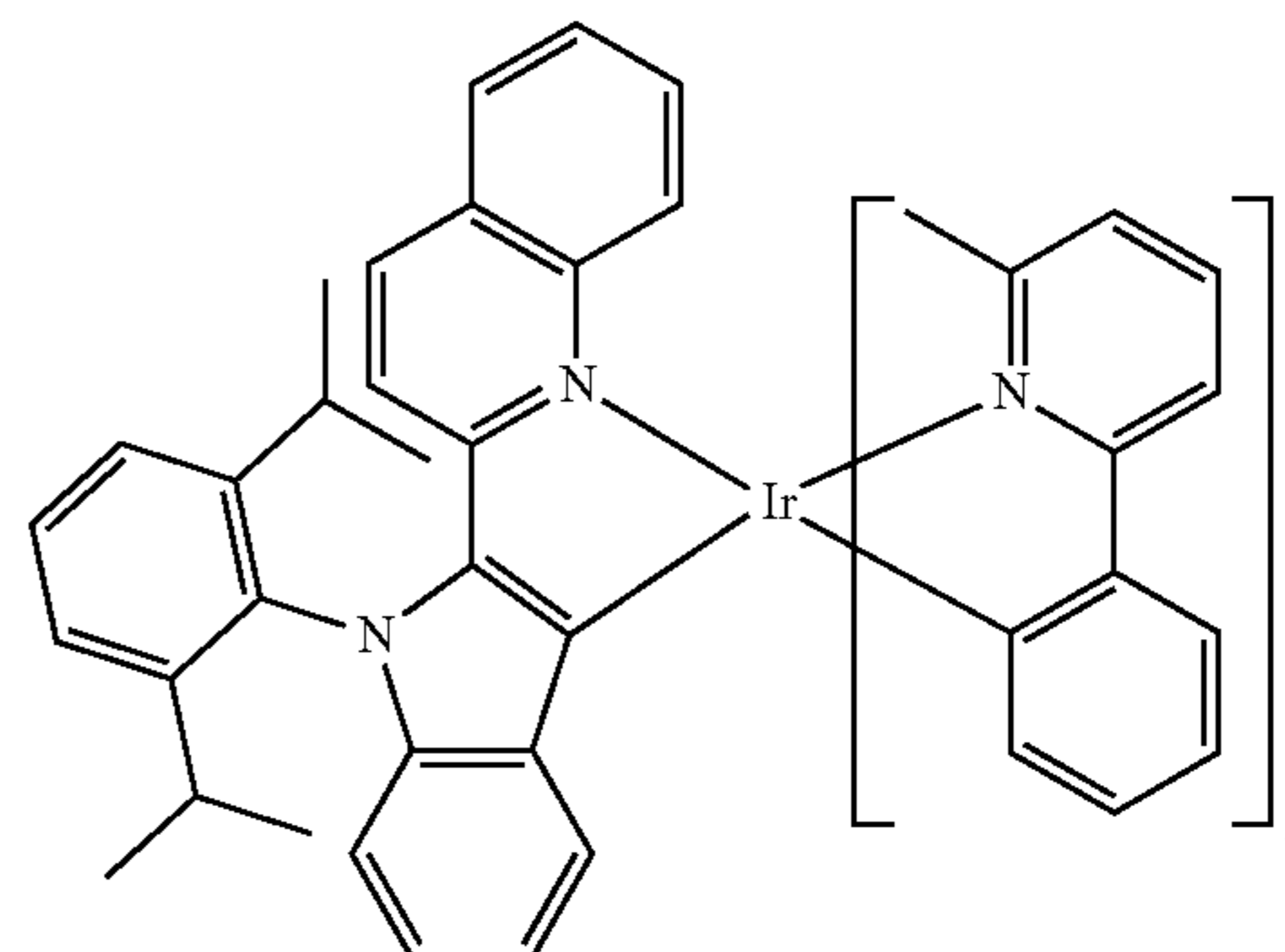
Compound 82
