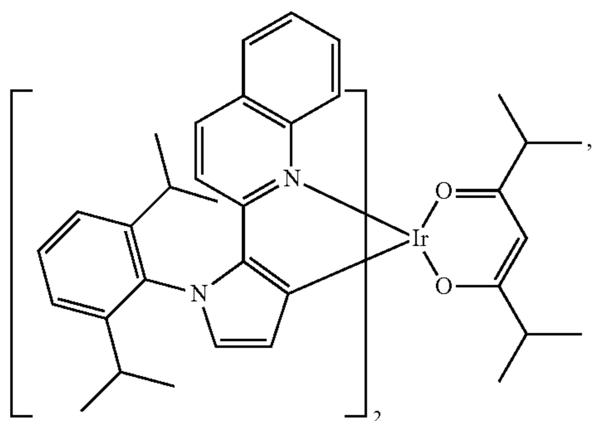
Compound 74
