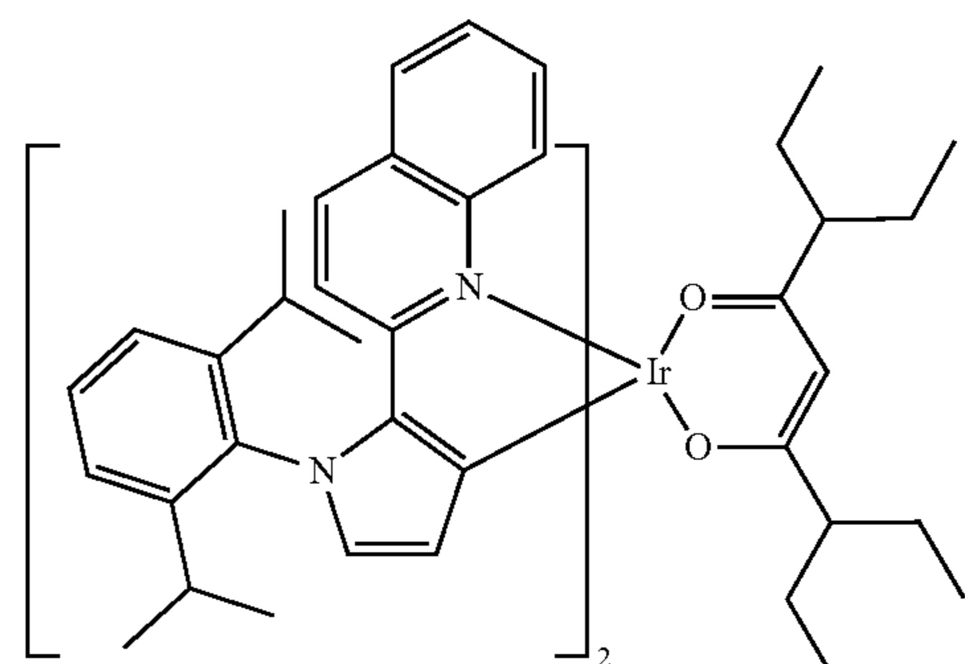
Compound 75
