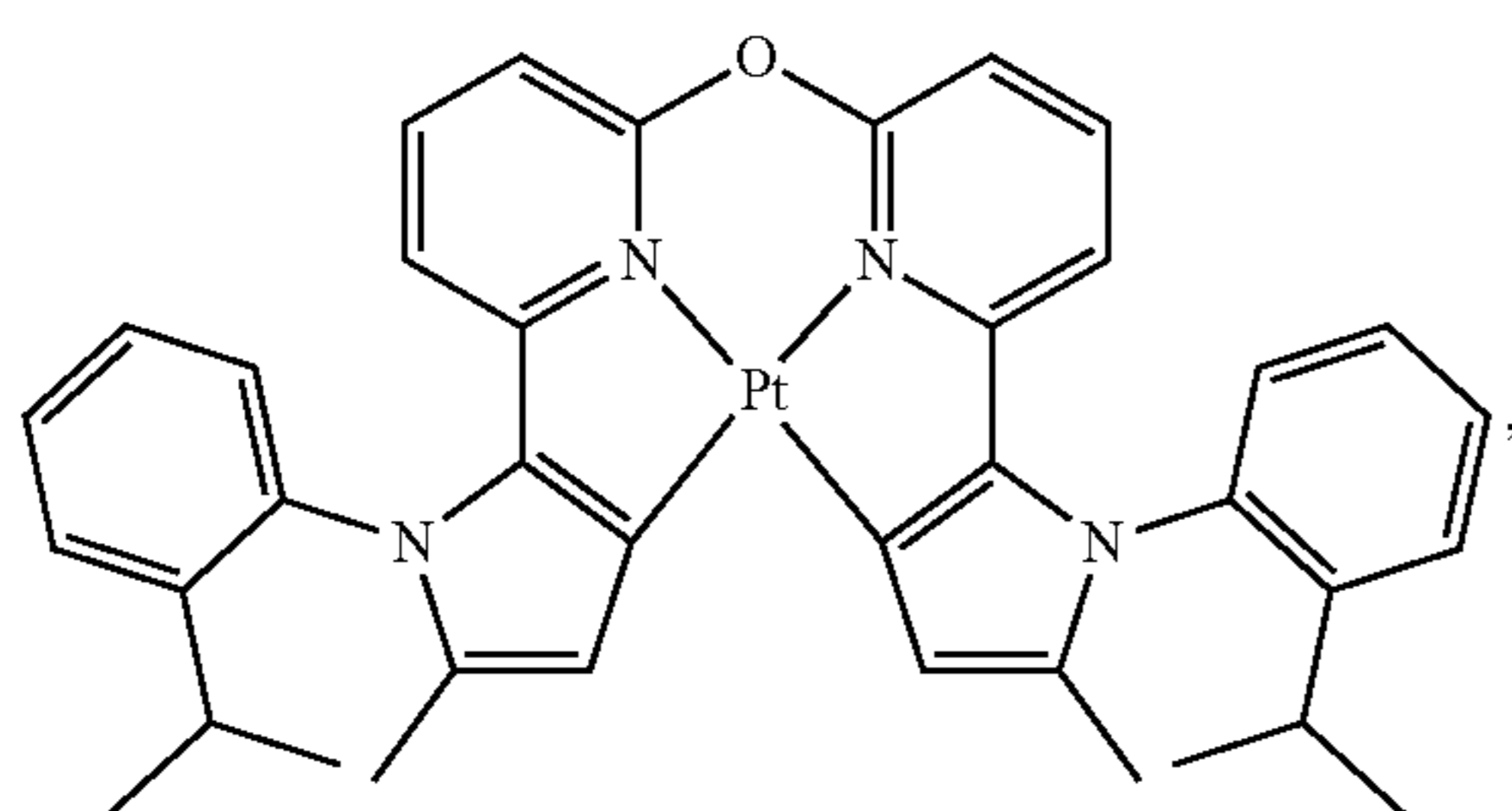
Compound 107
