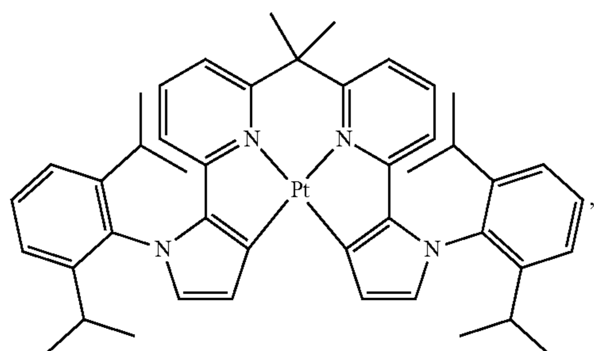
Compound 98
