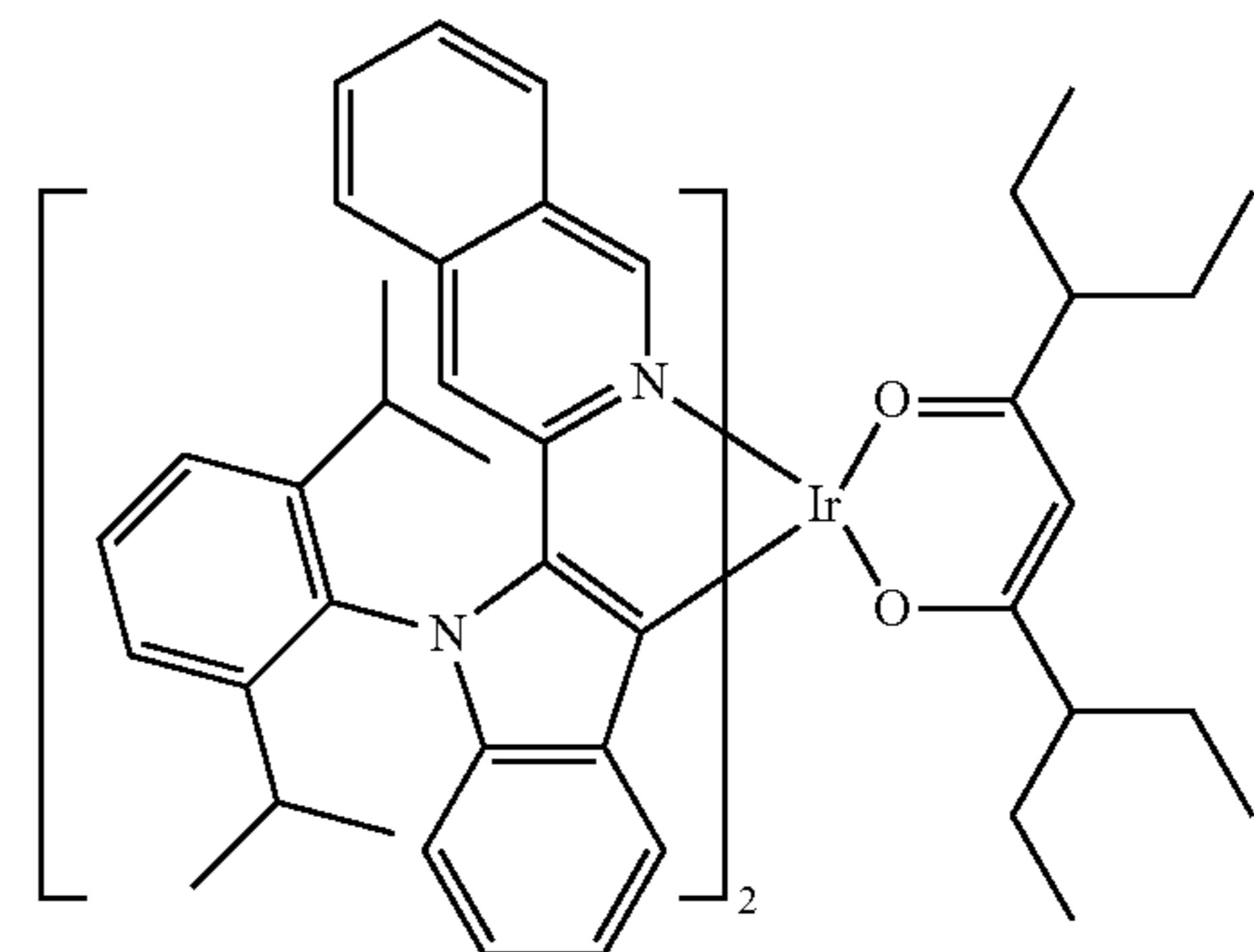
Compound 68
