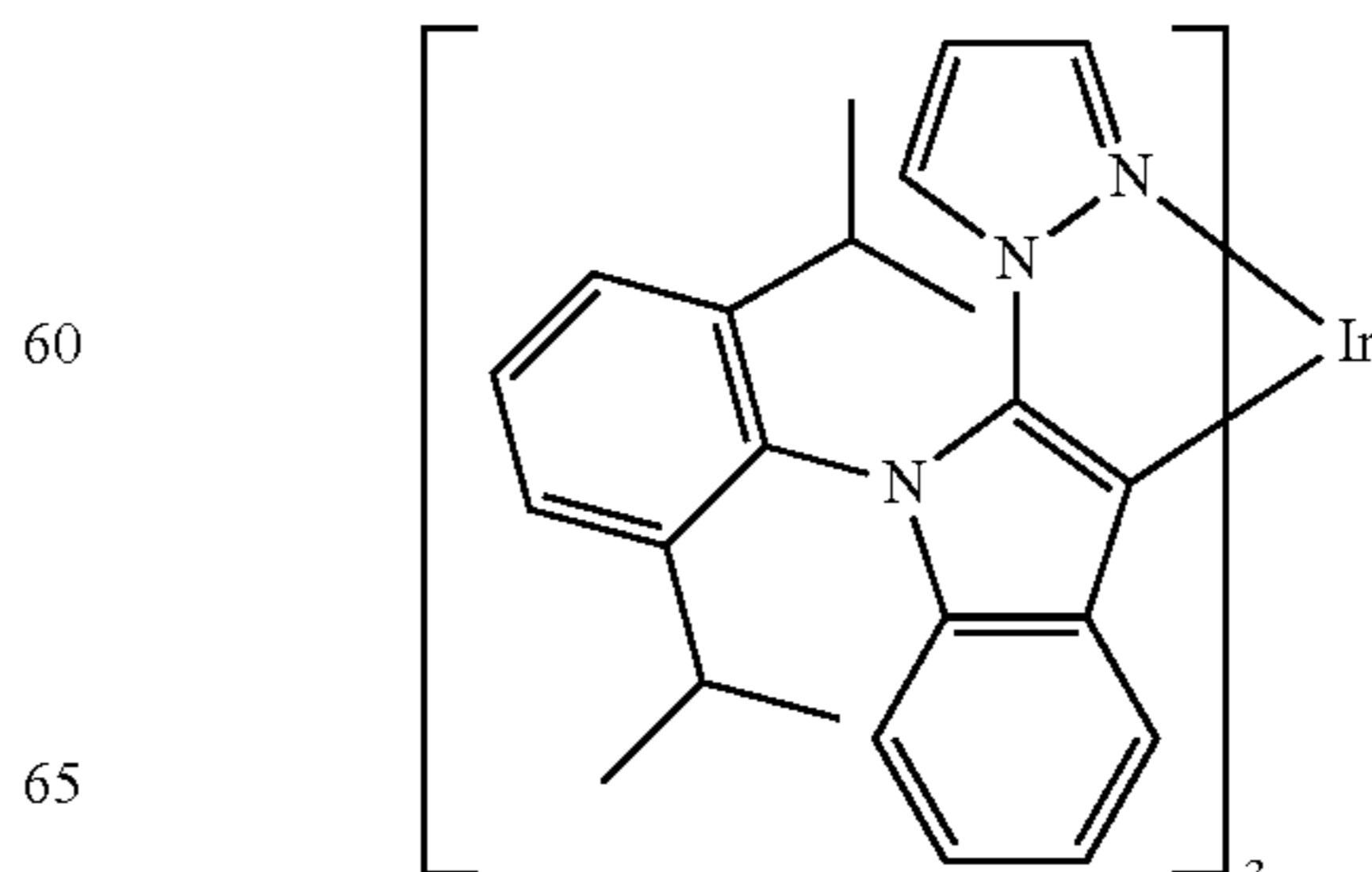
Compound 14
