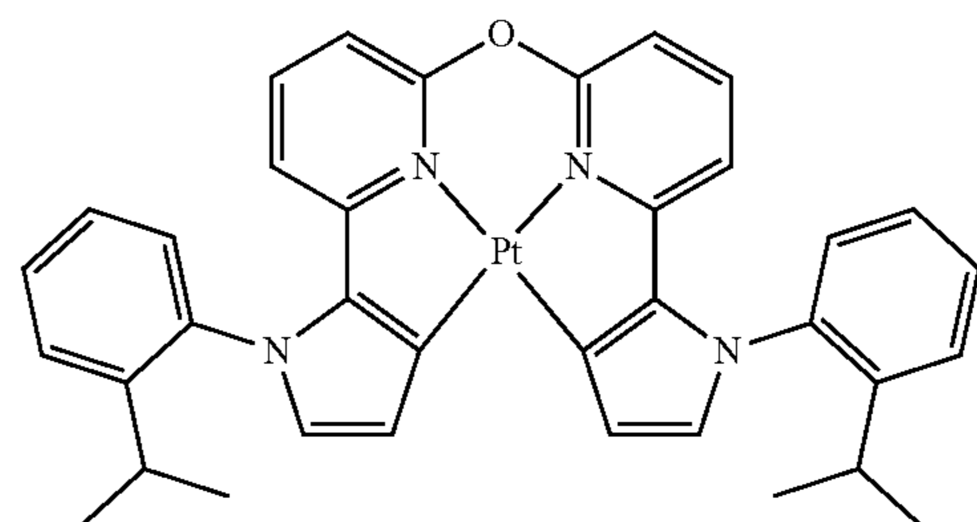
Compound 103
