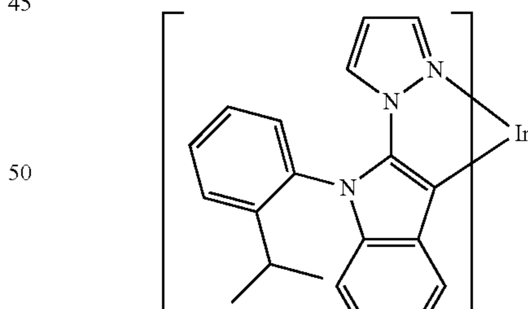
Compound 13
