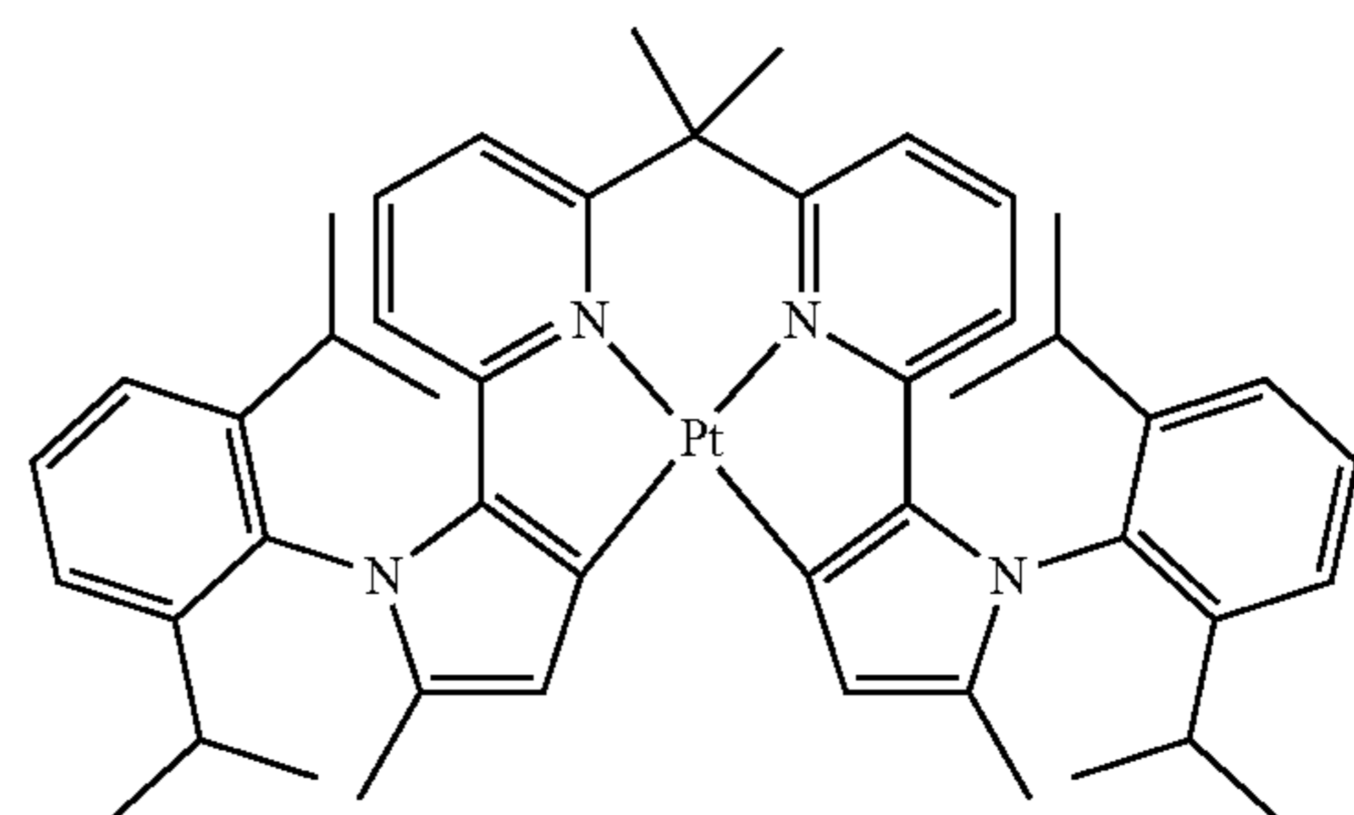
Compound 99
