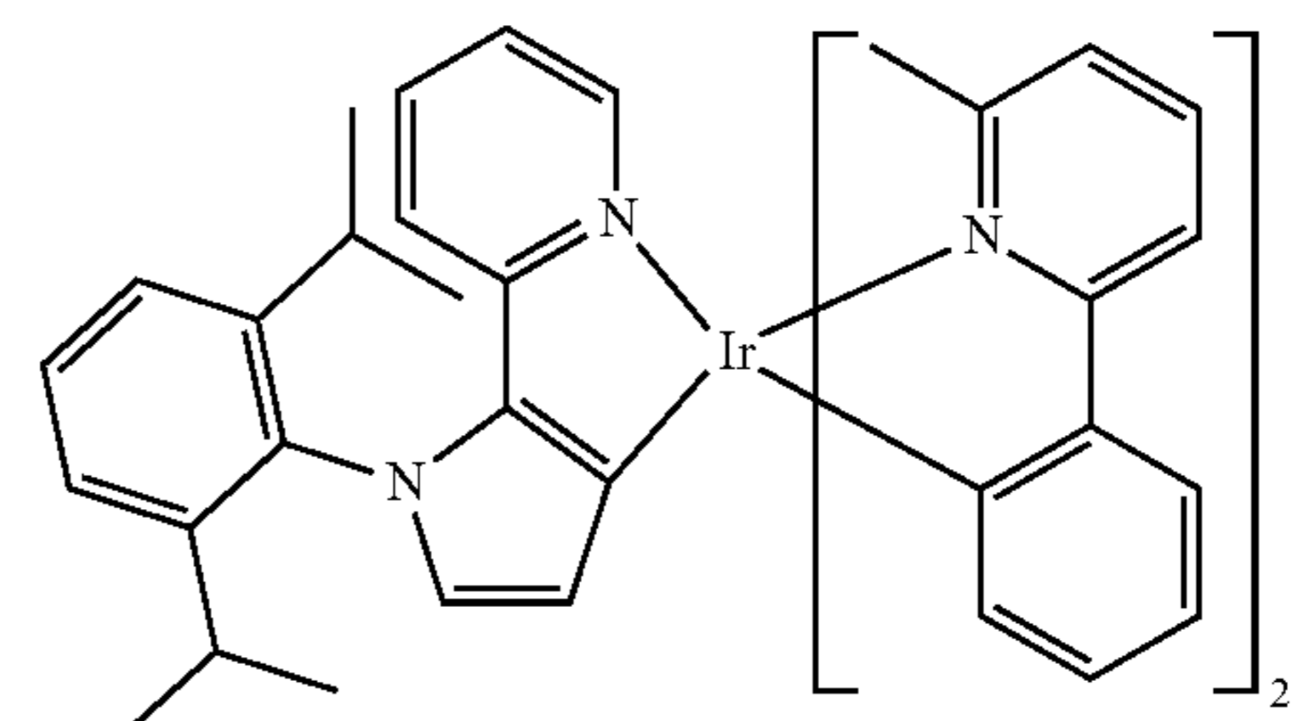
Compound 60
