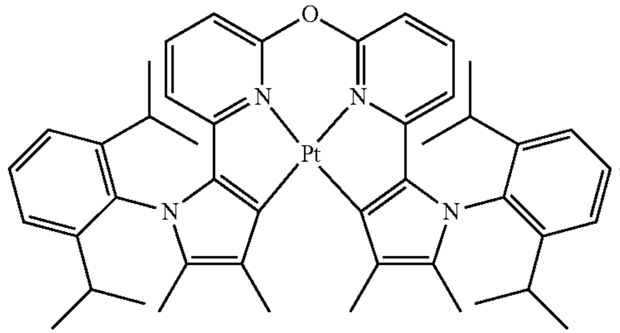
Compound 109
