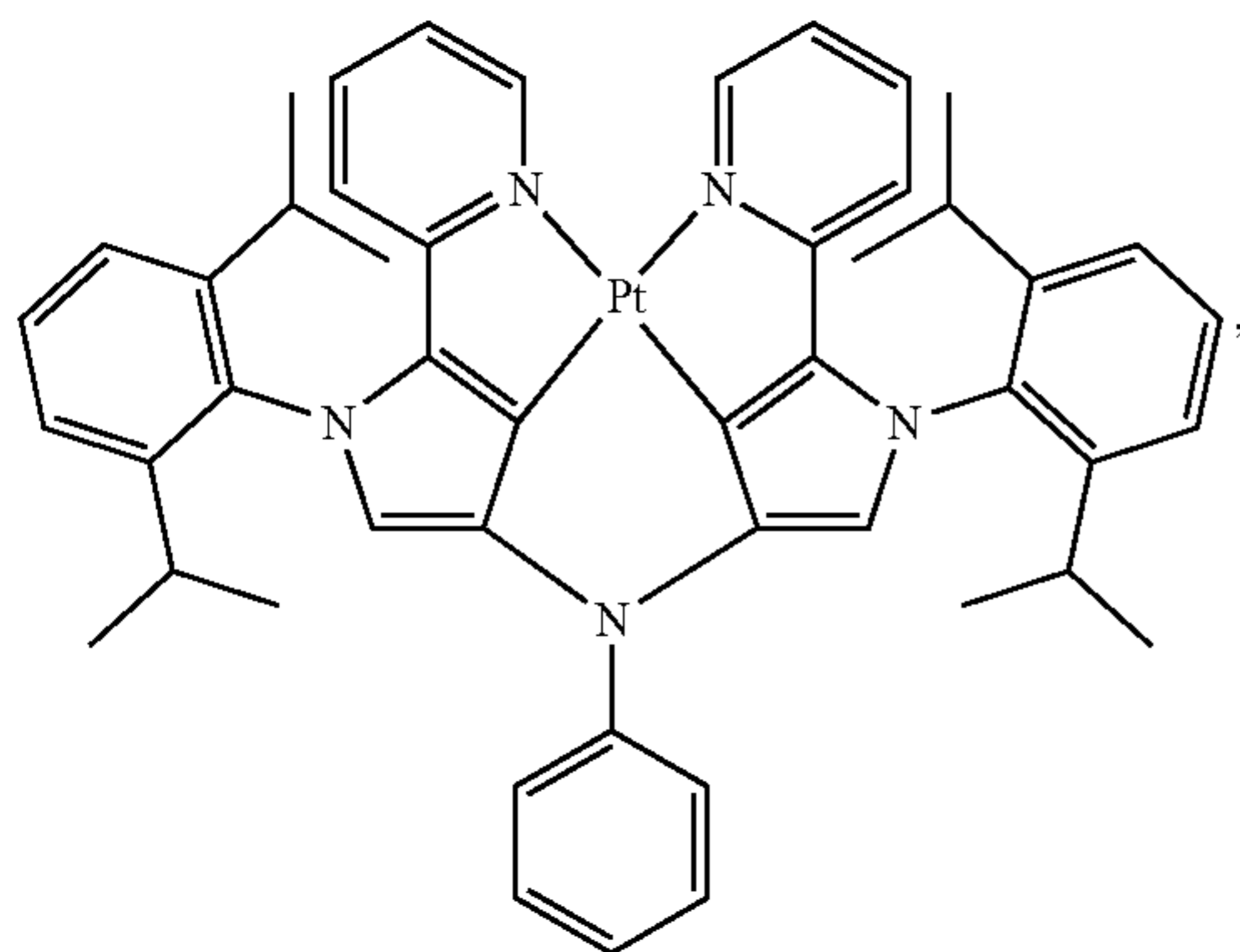
Compound 111
