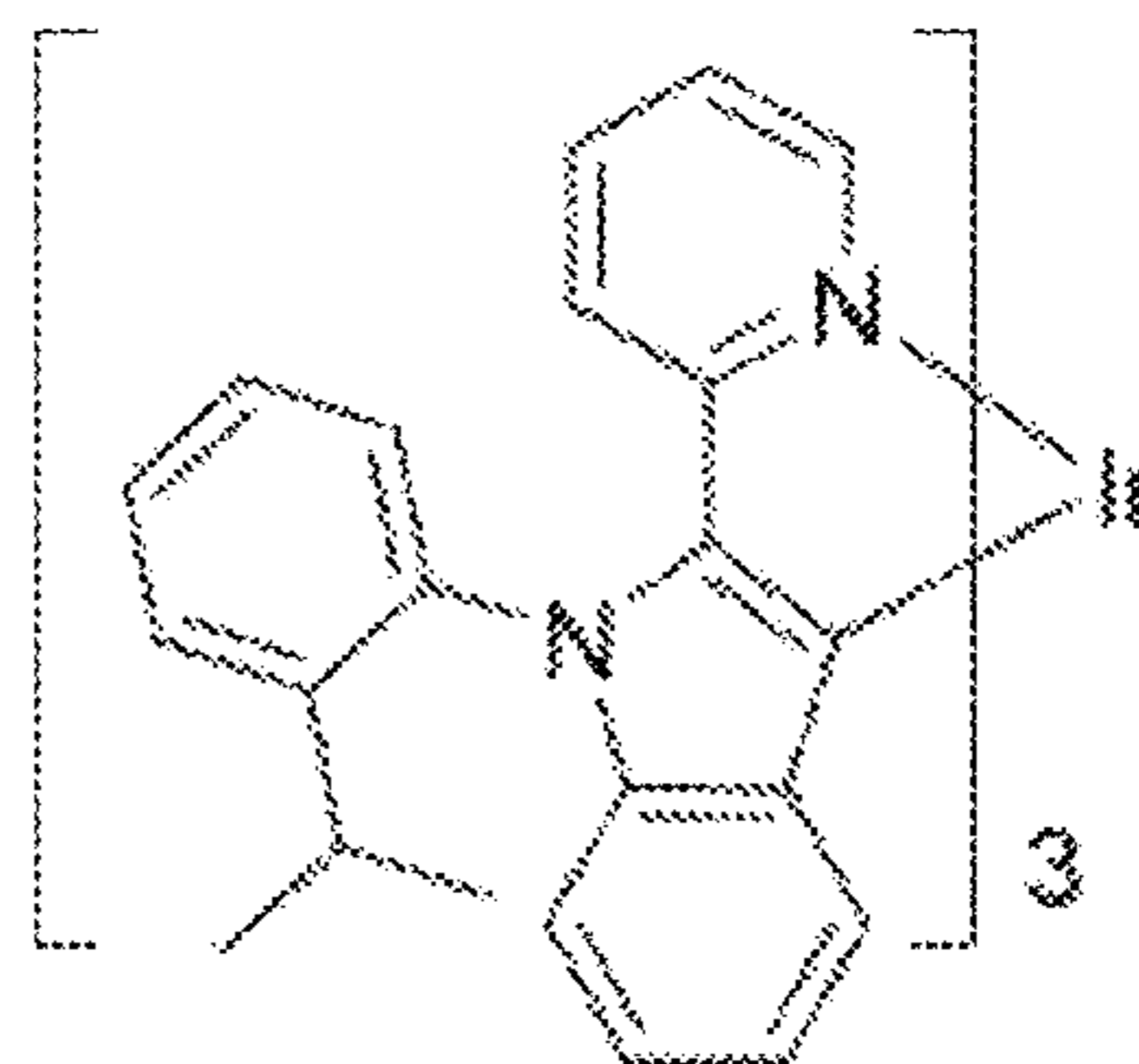
Compound 49
