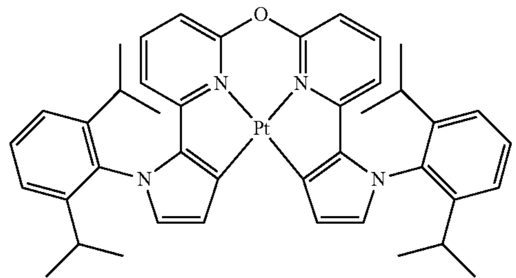
Compound 105
