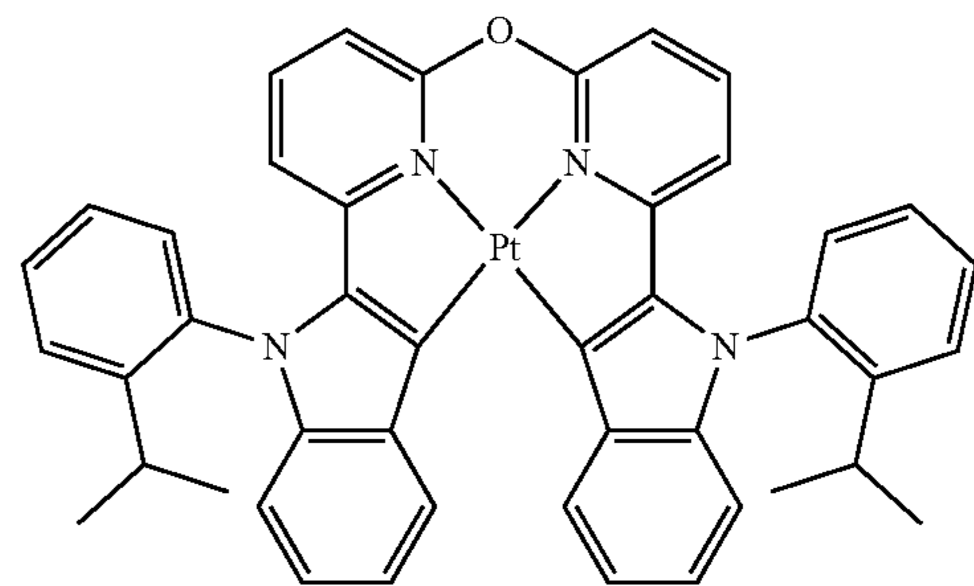
Compound 102
