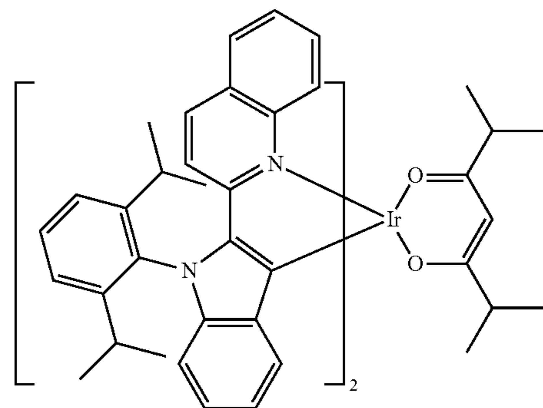
Compound 77
