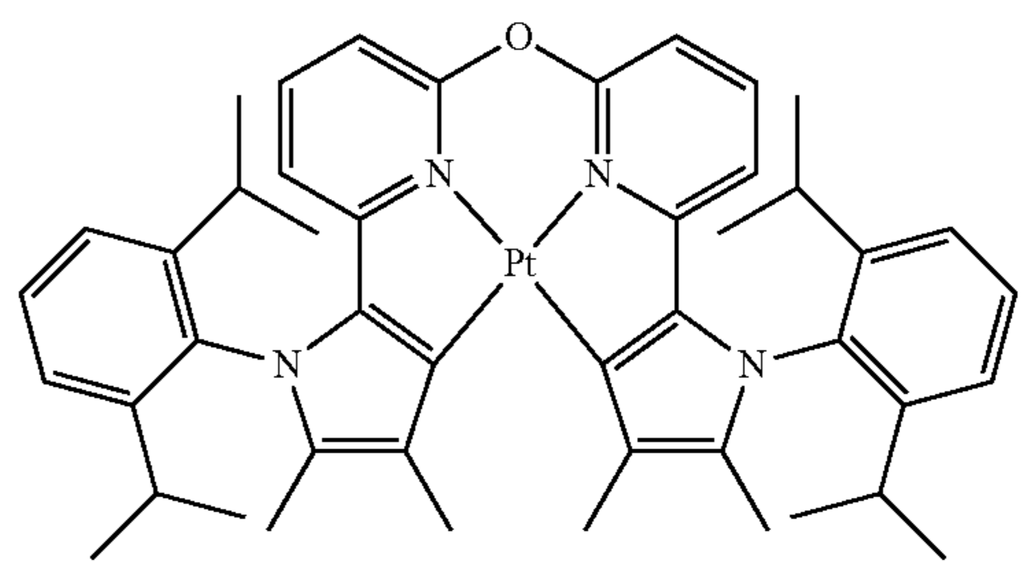
Compound 109
