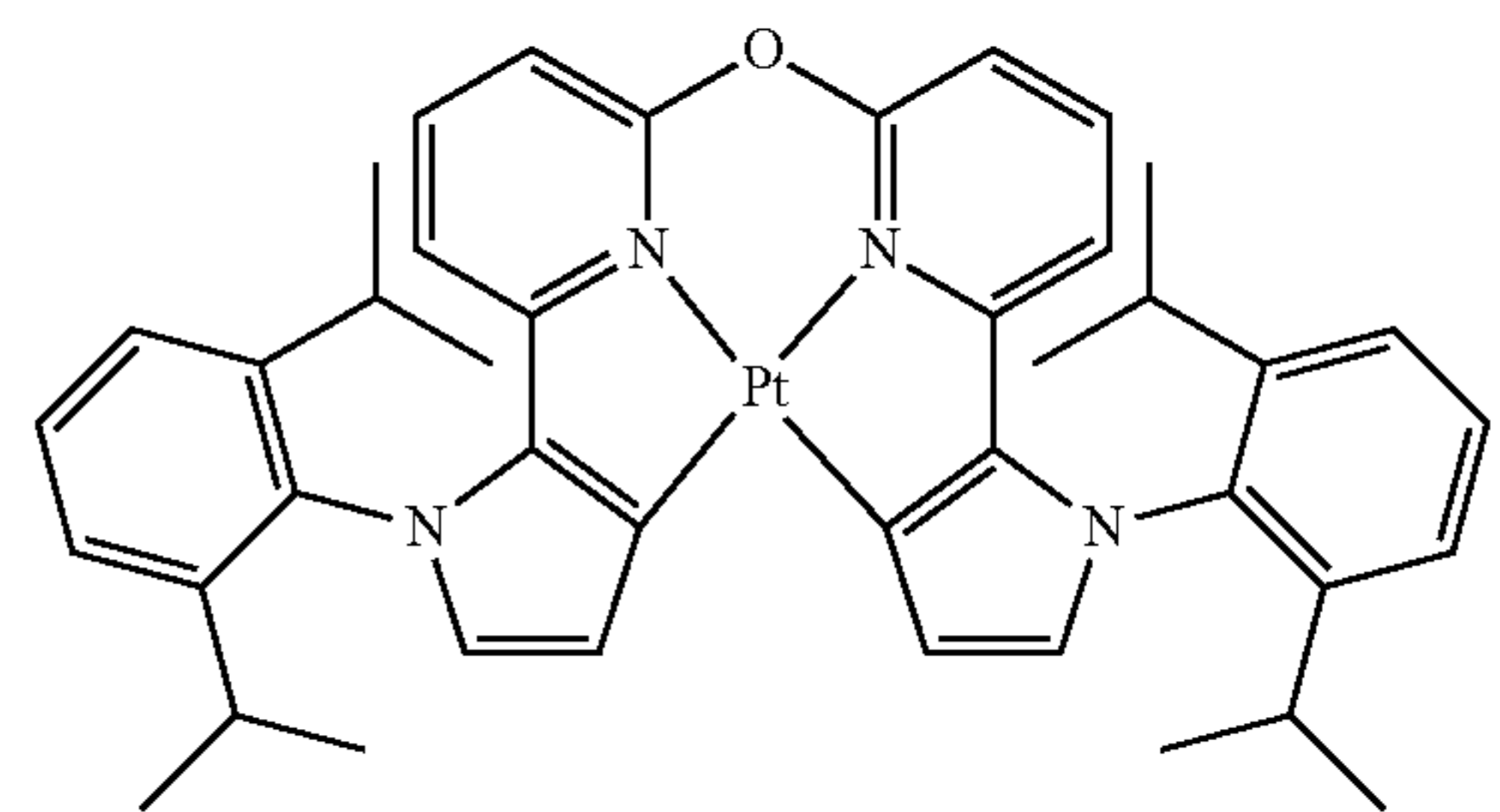
Compound 105
