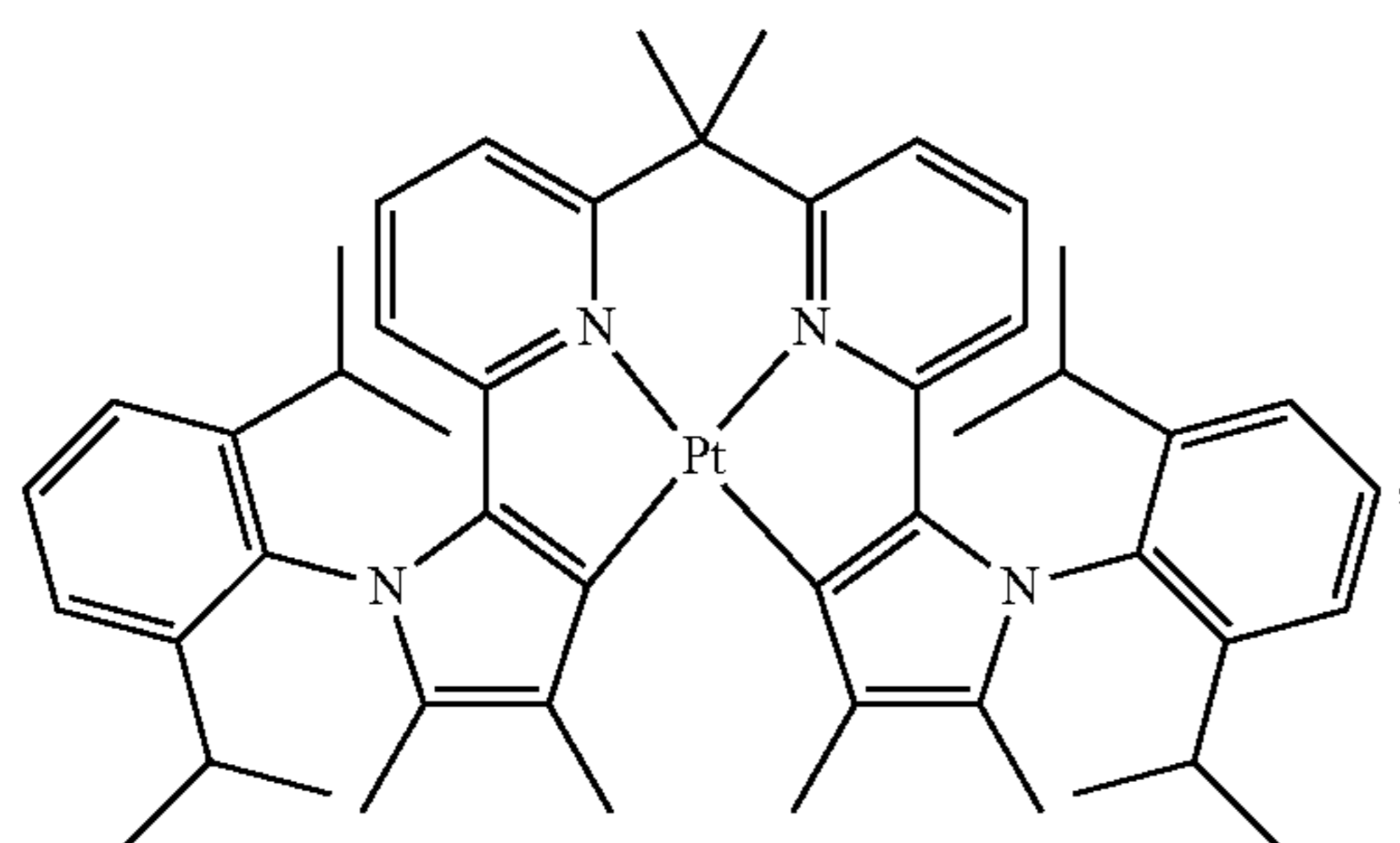
Compound 102
