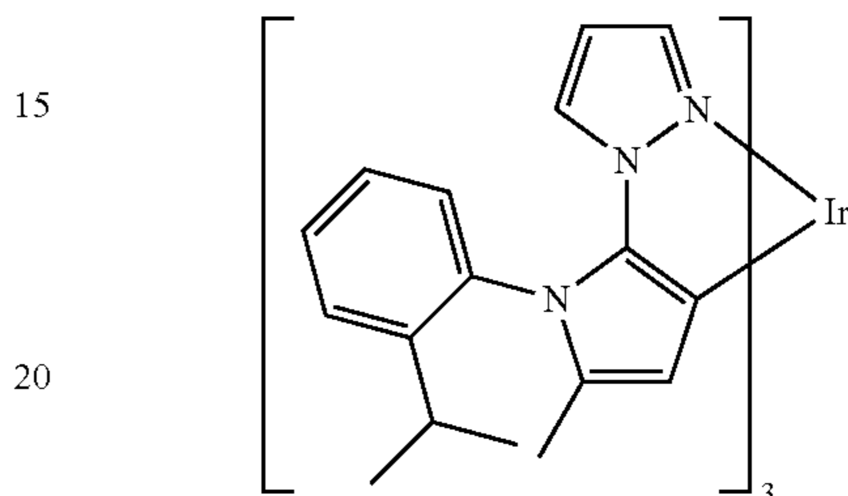
Compound 11
