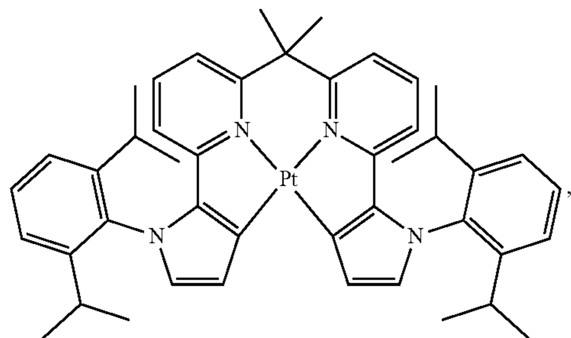
Compound 97
