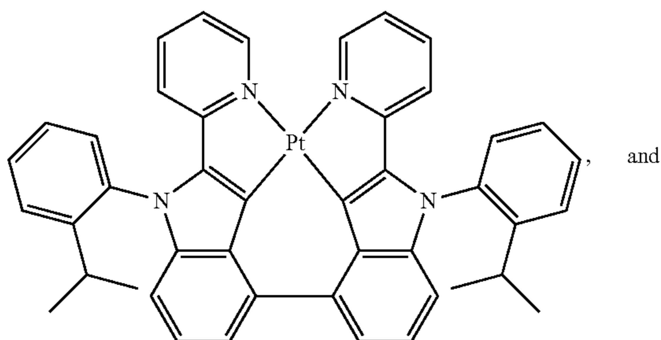
Compound 113
