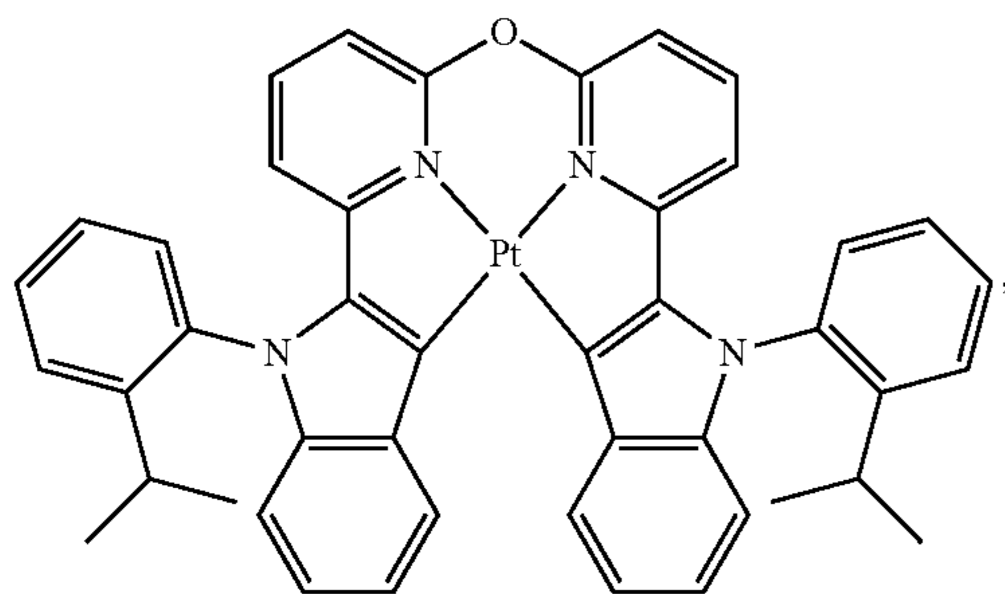
Compound 103
