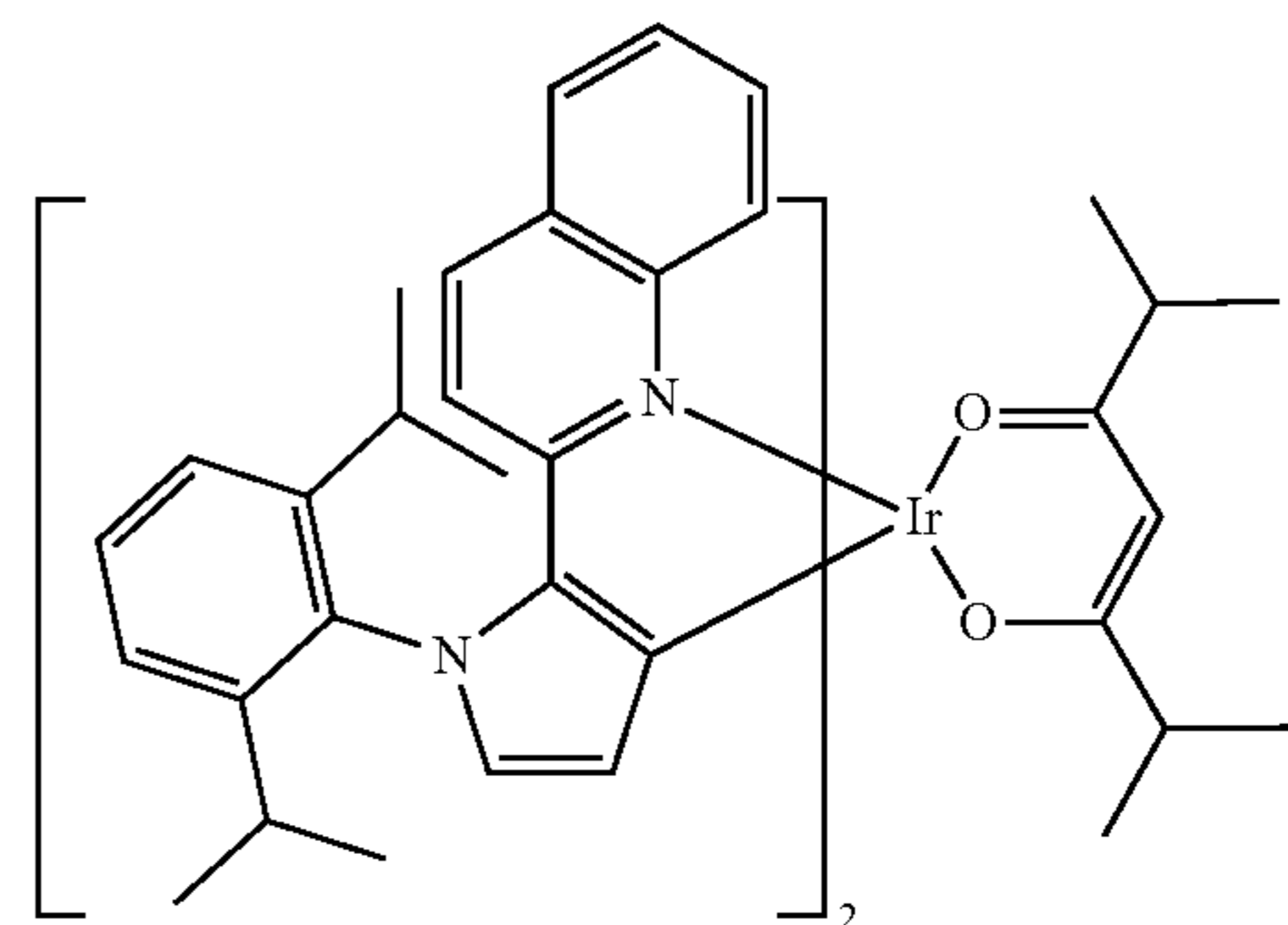
Compound 74
