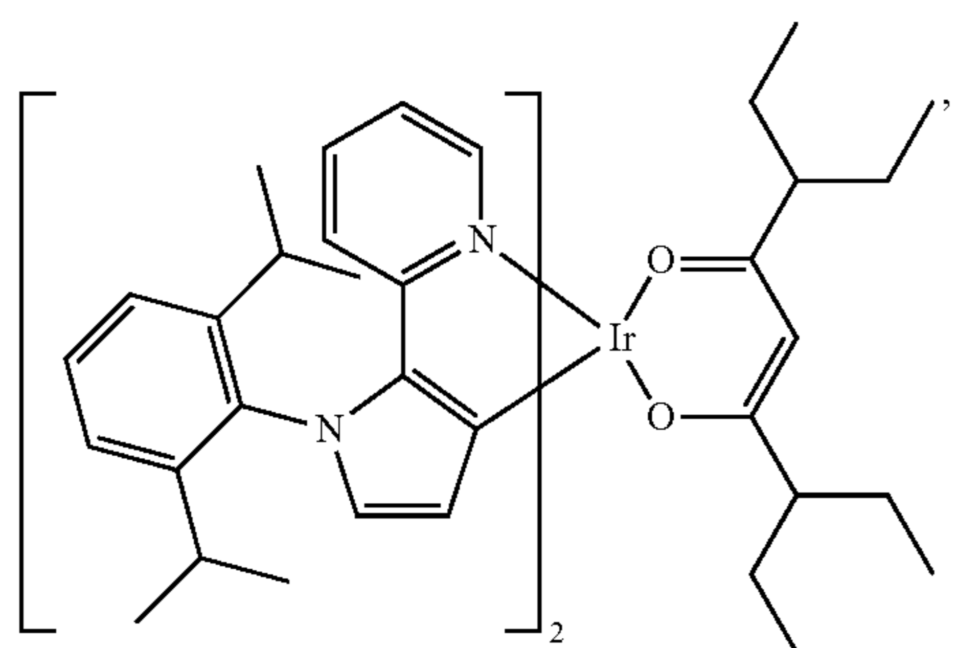
Compound 56
