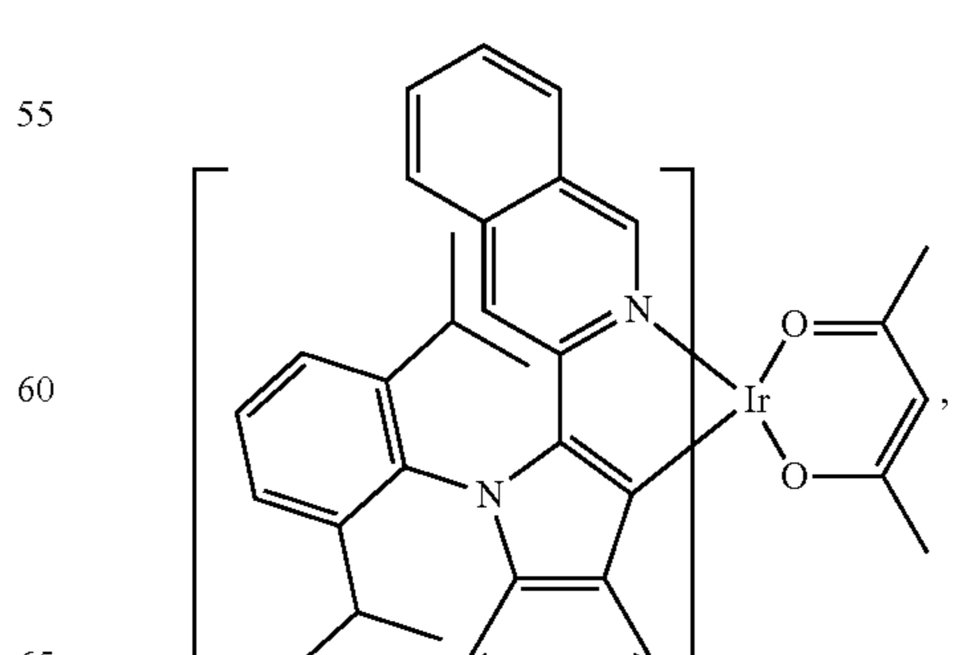
Compound 61
