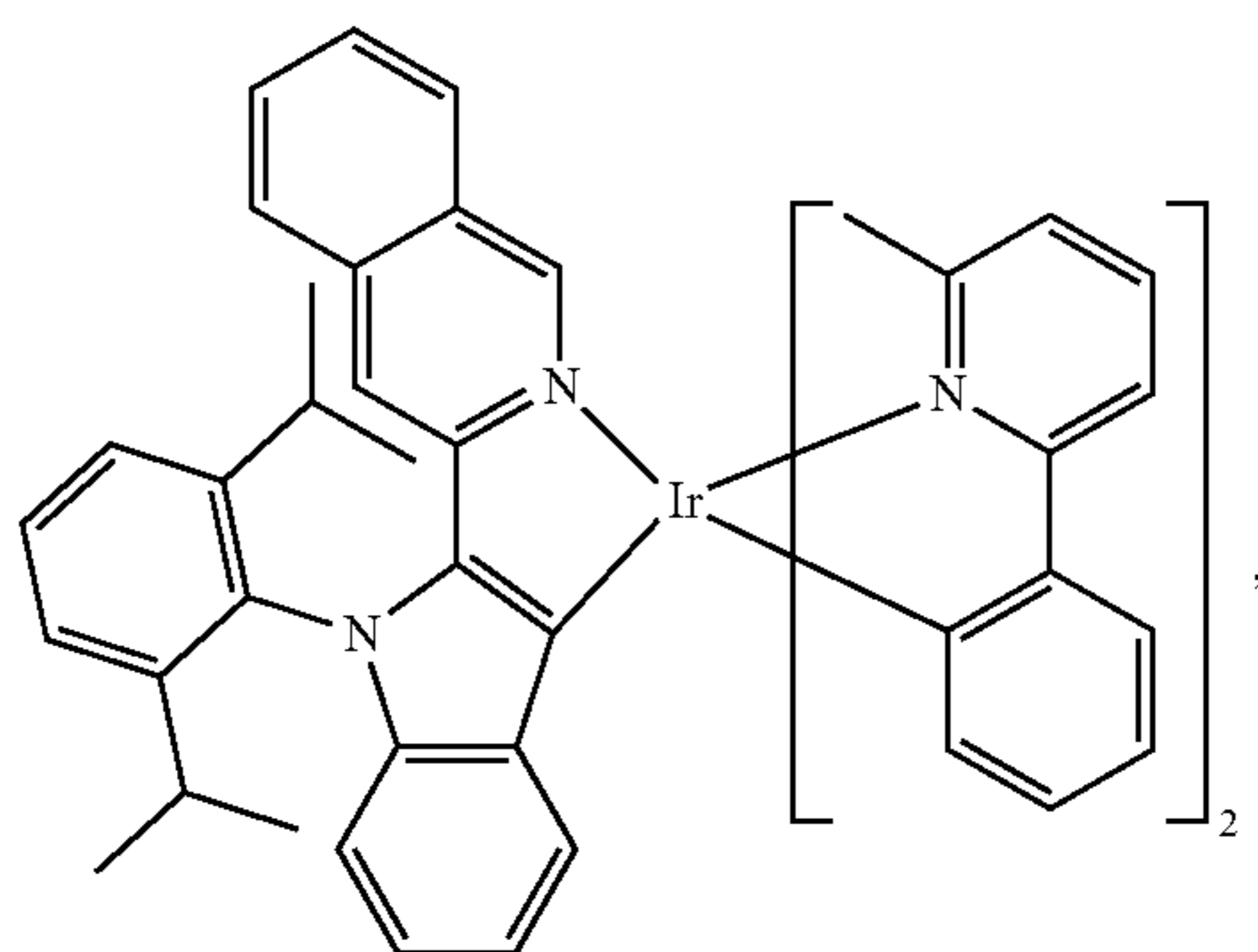
Compound 72
