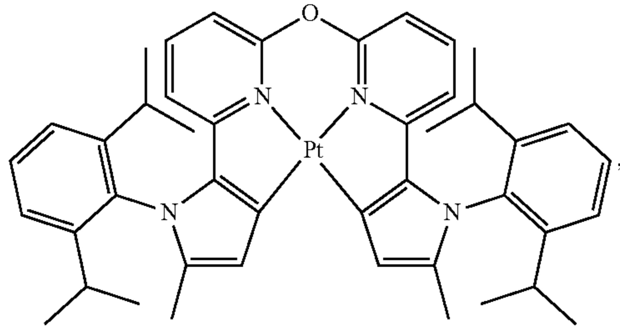
Compound 108
