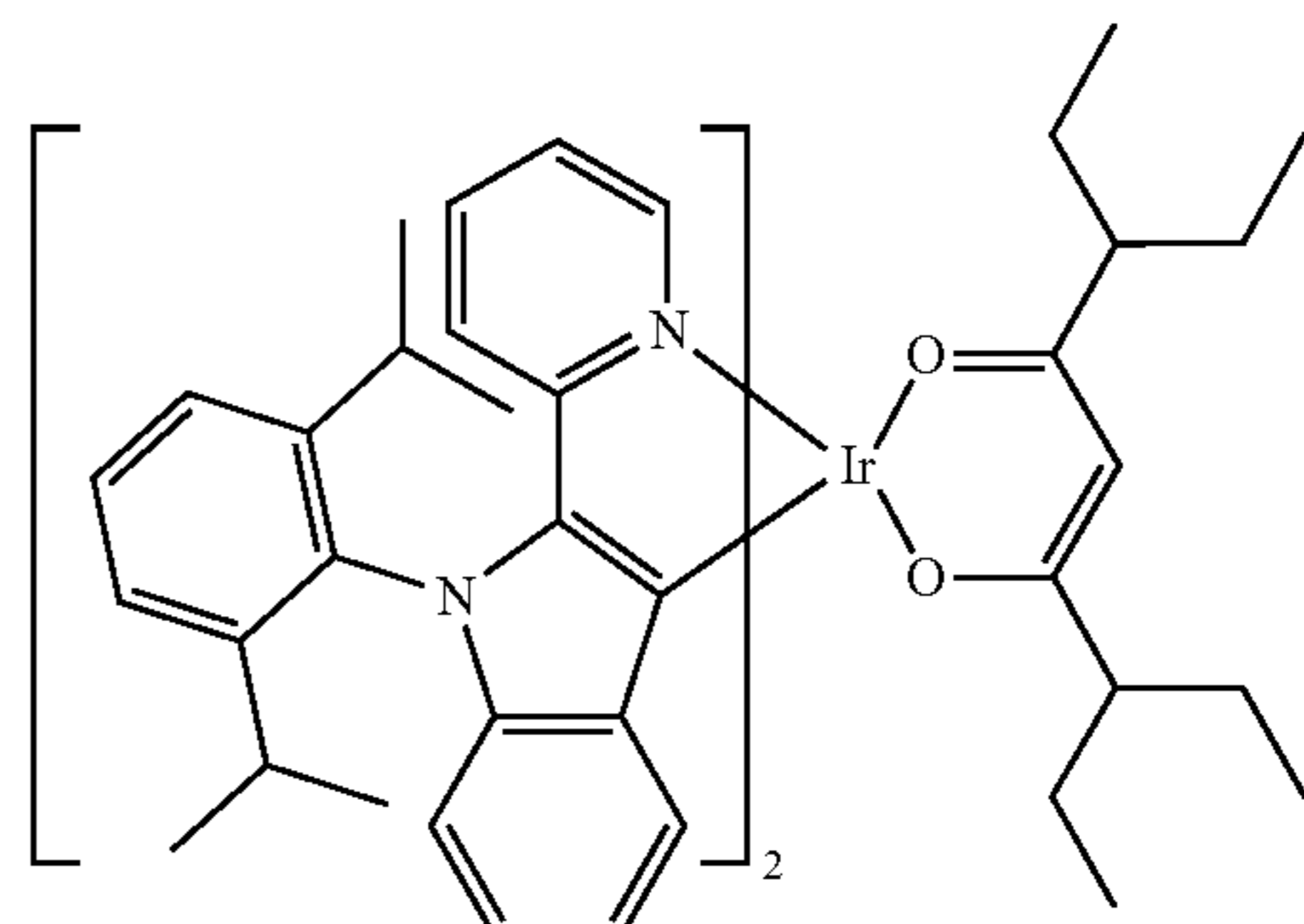
Compound 59
