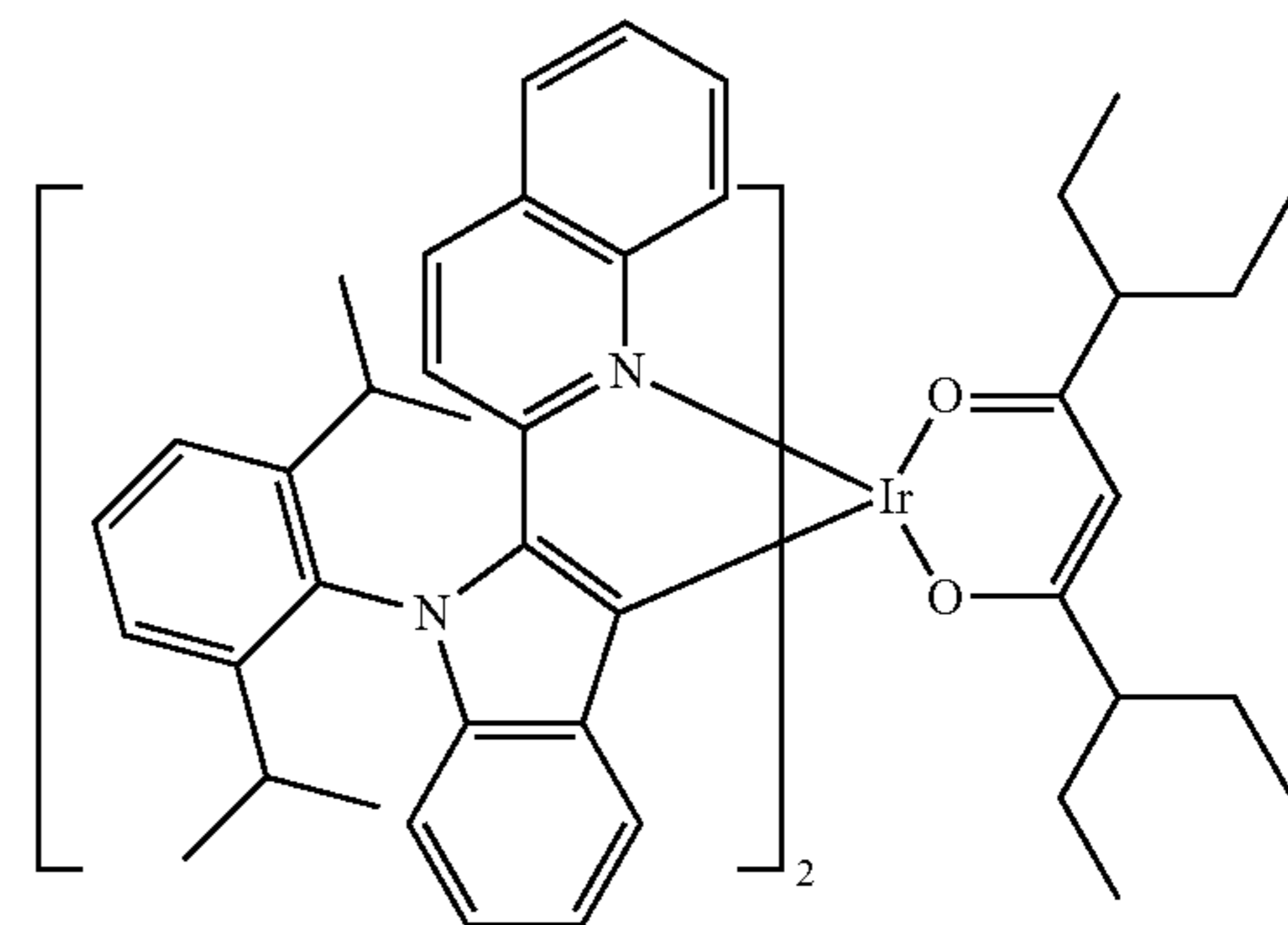
Compound 78
