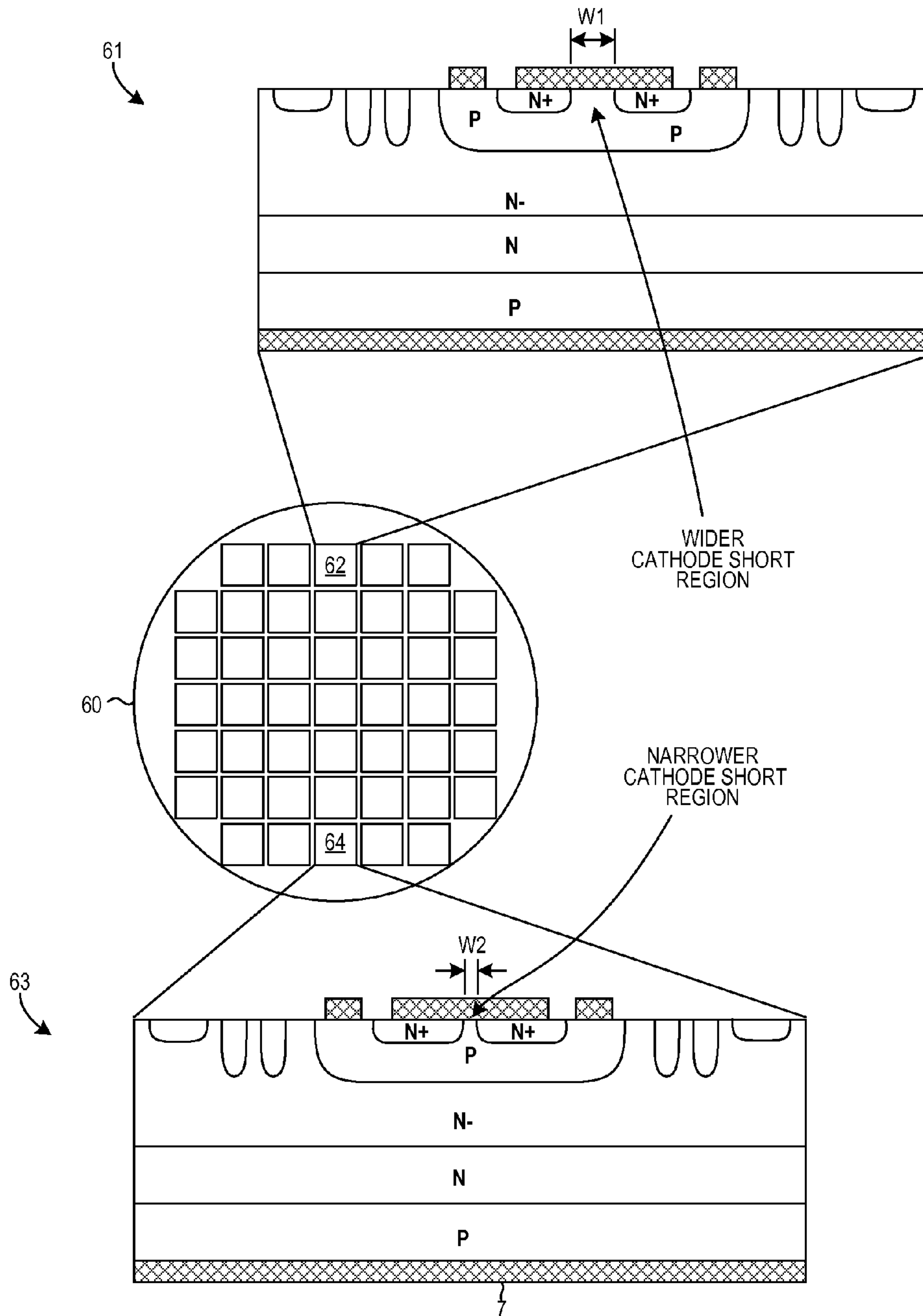
ONE WAFER YIELDS BOD DEVICES WITH DIFFERENT TRIGGERING CURRENTS
