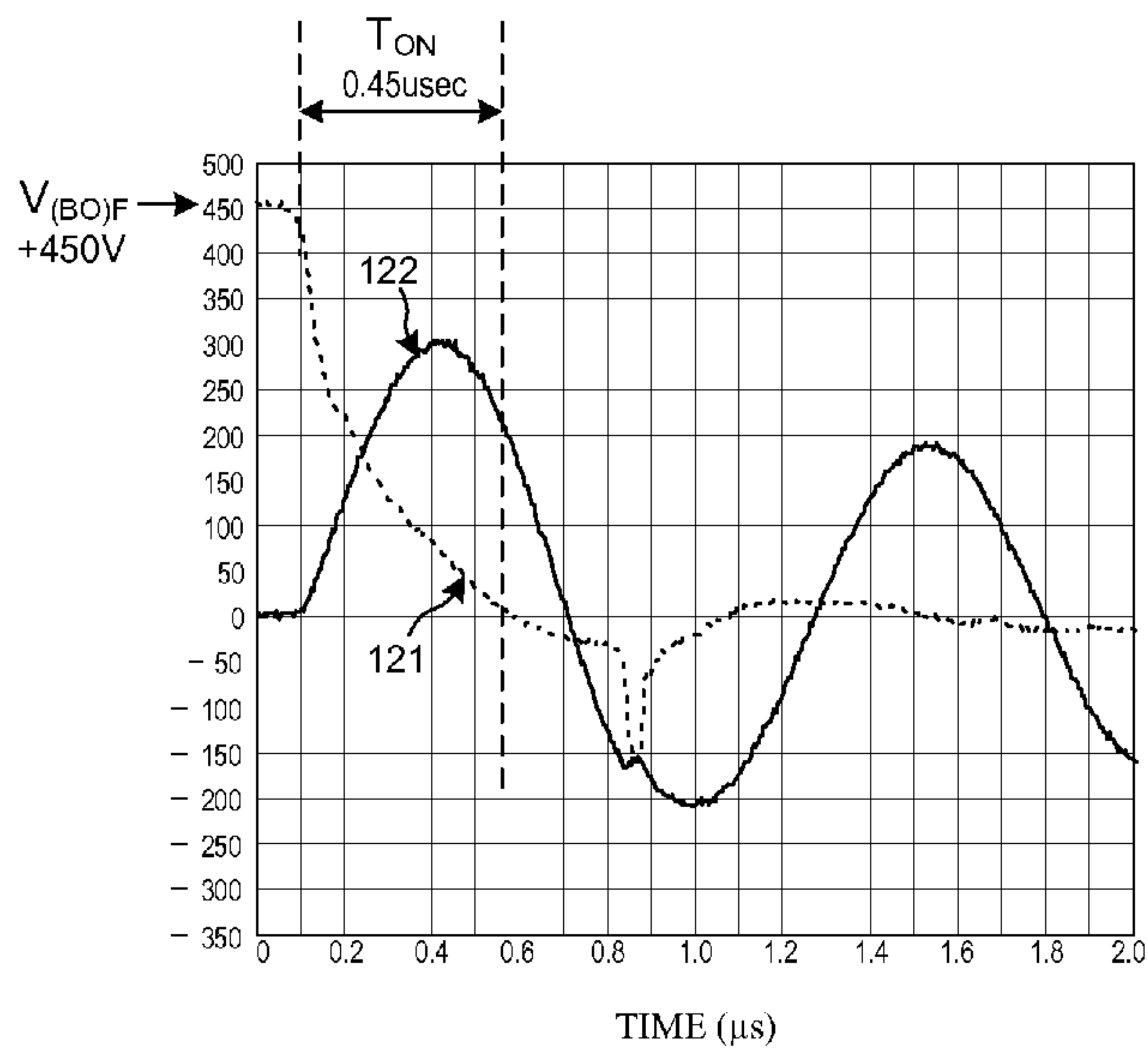
SWITCHING DIAGRAM OF THE BOD OF FIG. 22
