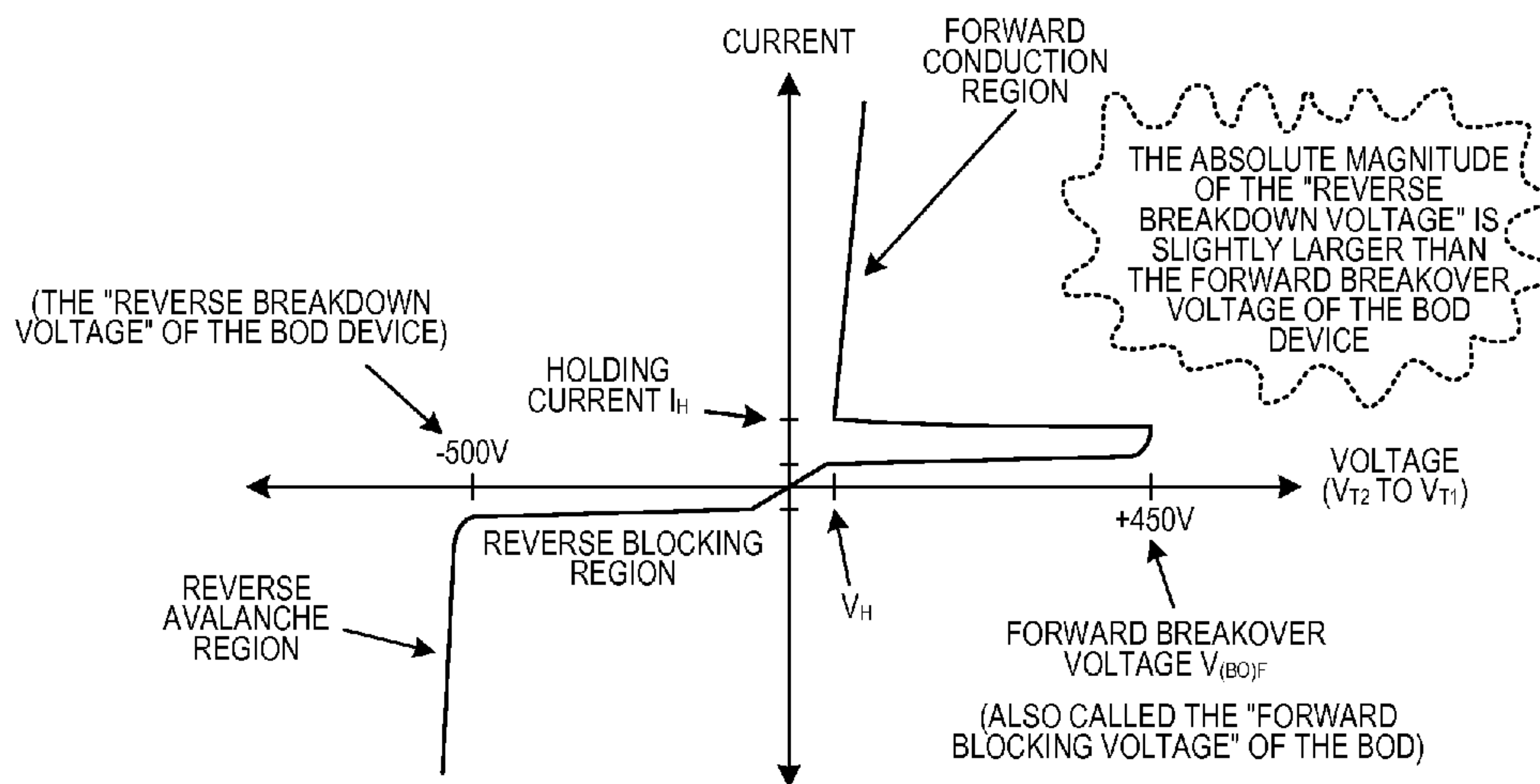
V-I CHARACTERISTICS OF BOD OF FIG. 22
