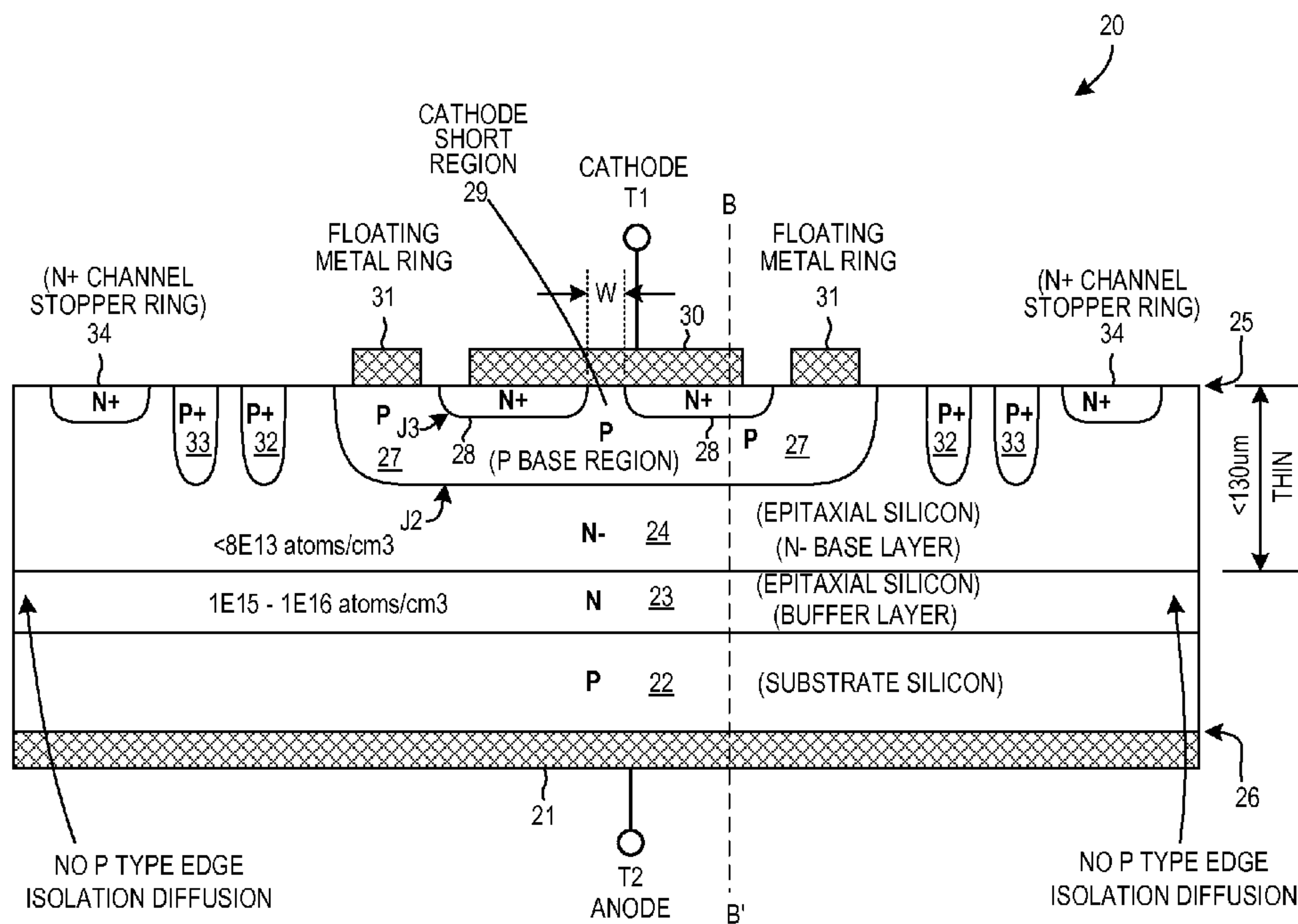
BREAKOVER DIODE DEVICE
