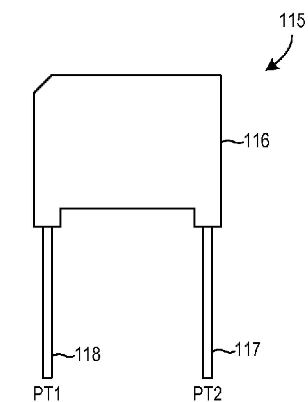
PACKAGED BOD OF FIG. 22
