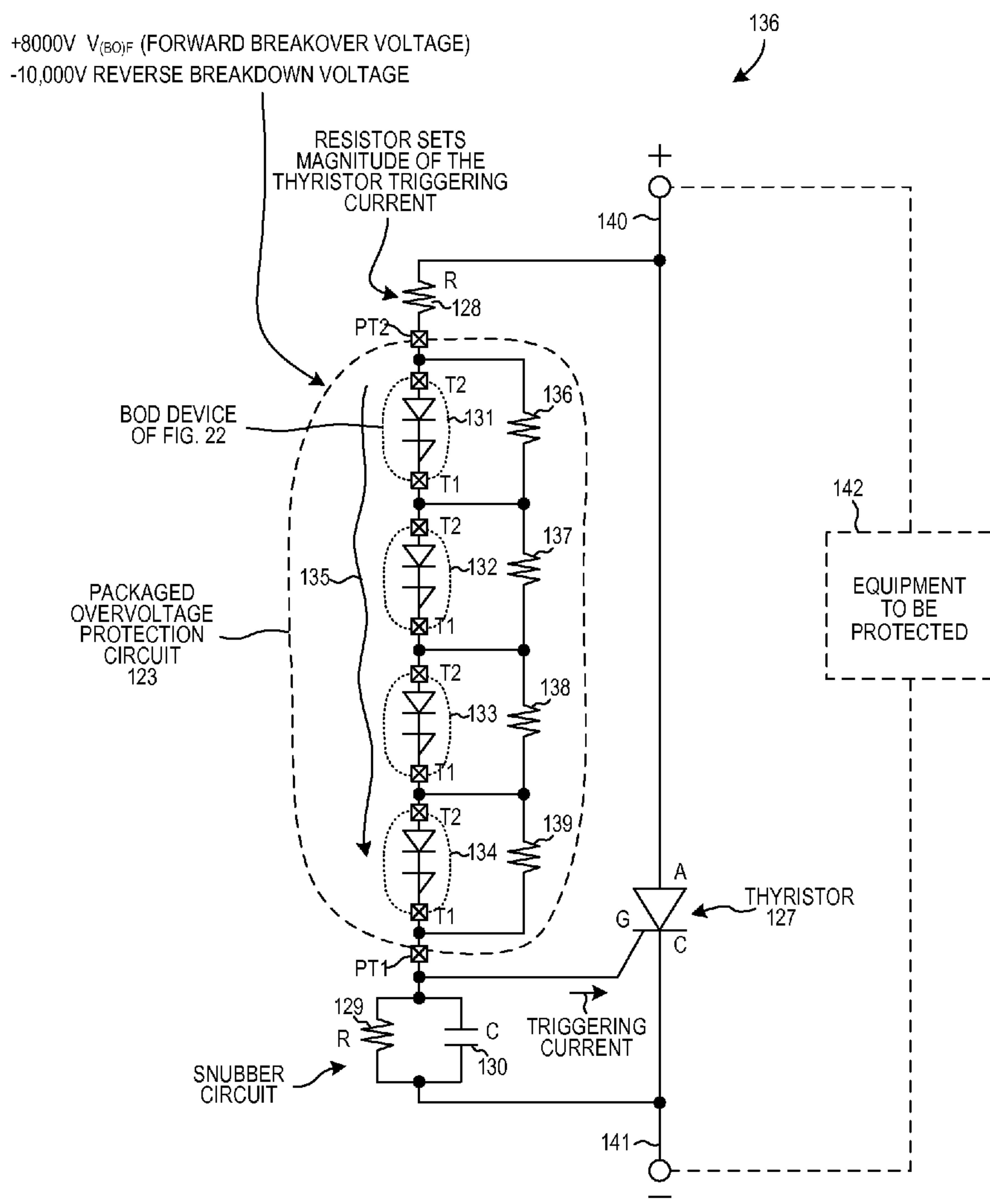
PACKAGED OVERVOLTAGE PROTECTION CIRCUIT AND A THYRISTOR
