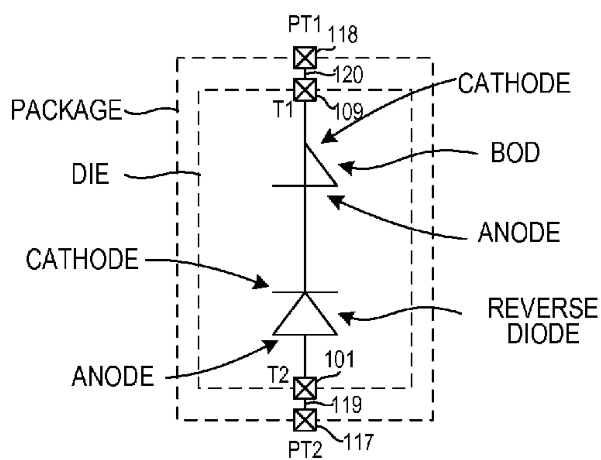
SYMBOL OF PACKAGED BOD OF FIG. 22
