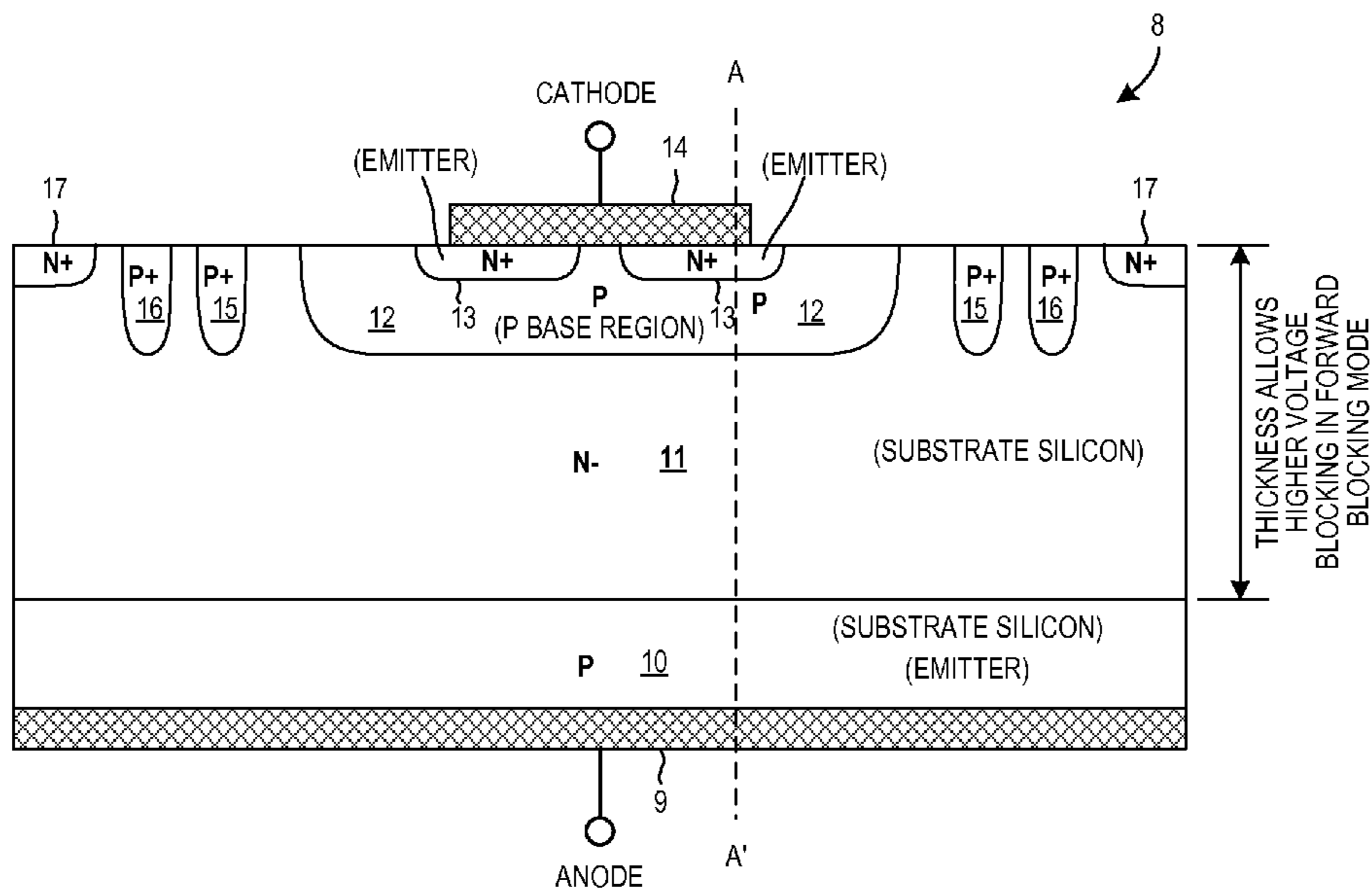
ANODE BULK BOD (PRIOR ART) FIG. 4
