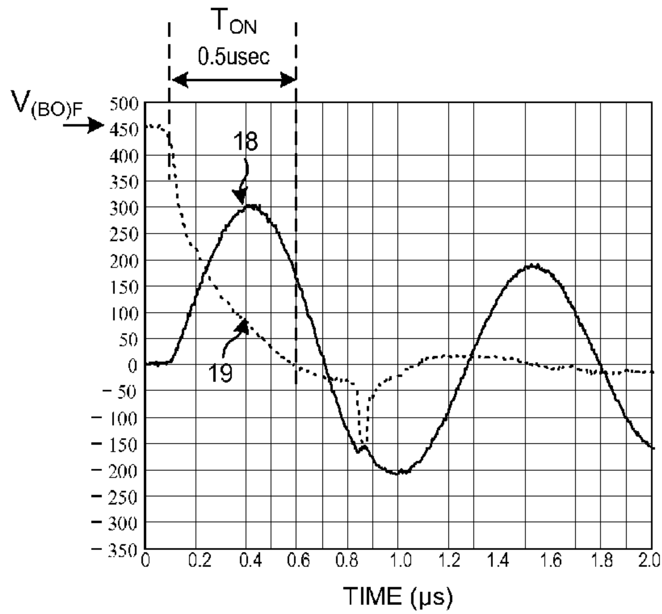
SWITCHING (PRIOR ART)
