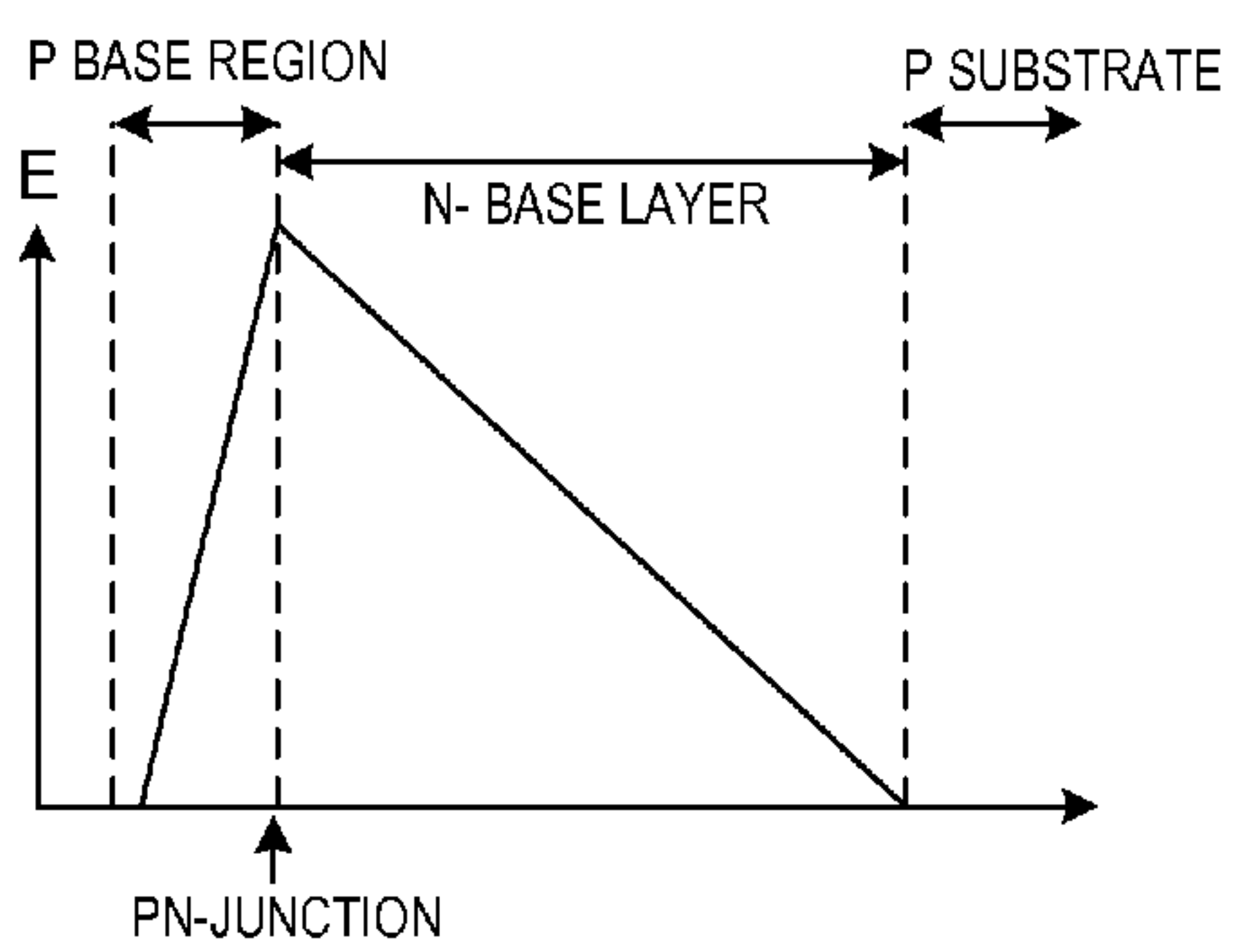
ELECTRIC FIELD ALONG LINE A-A' (PRIOR ART)
