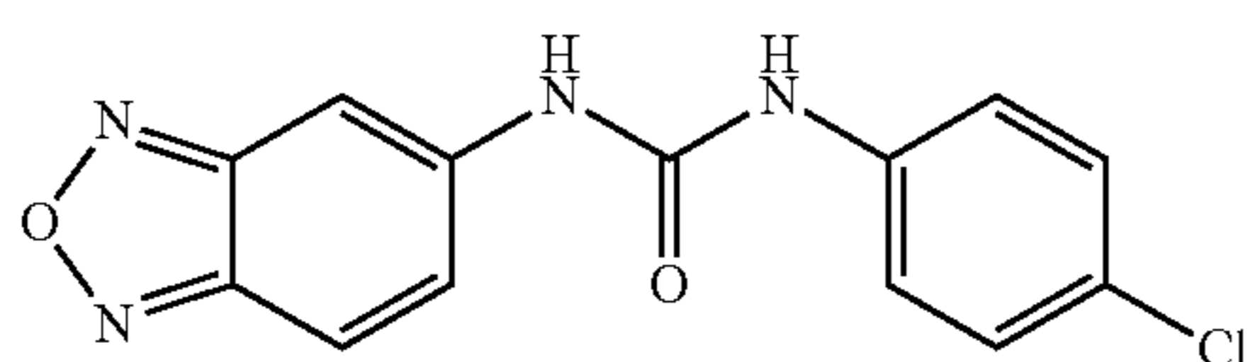
Compound KM09748
