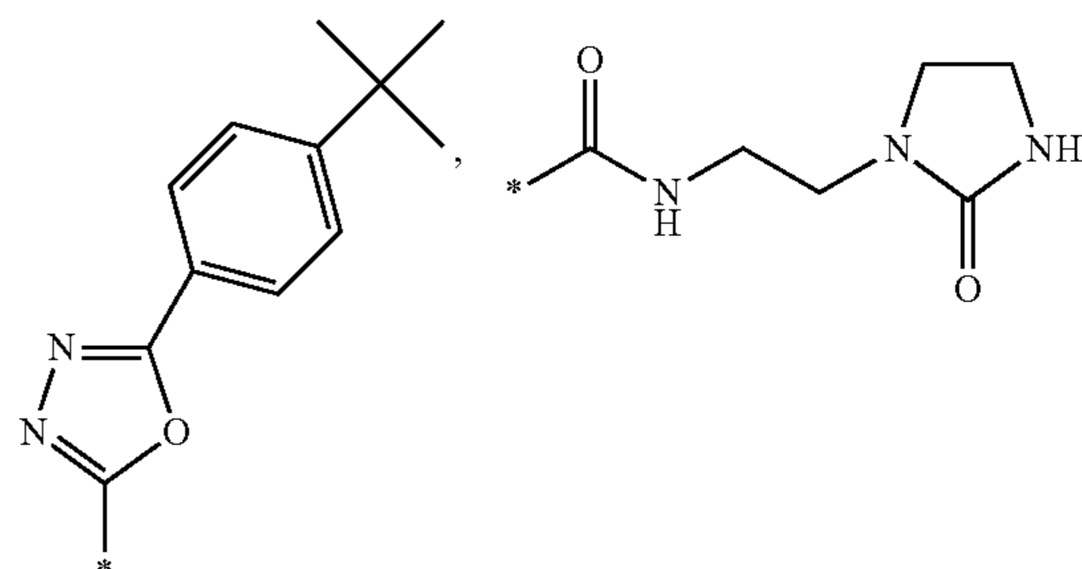
Formula I
