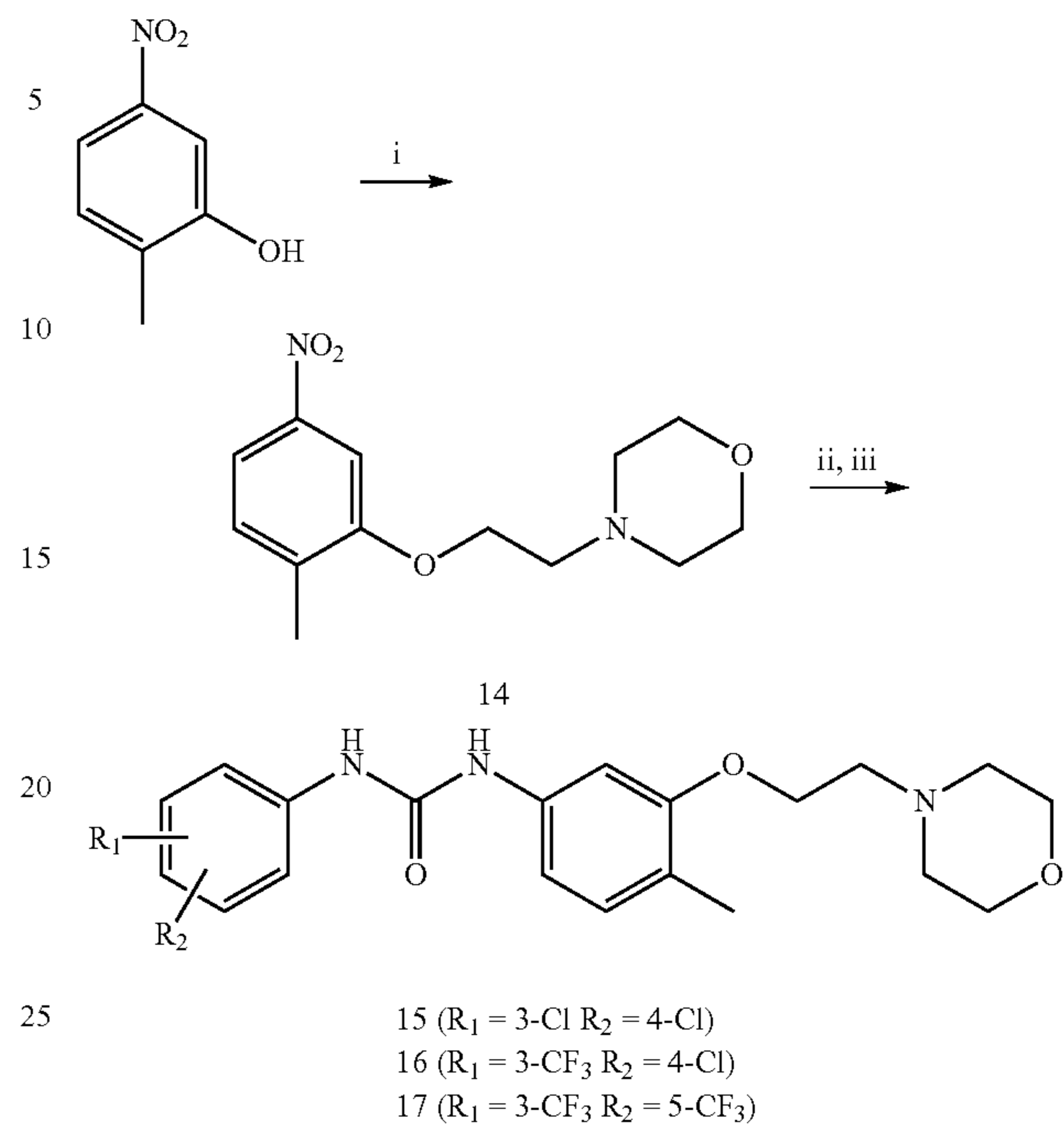
Scheme 4:
