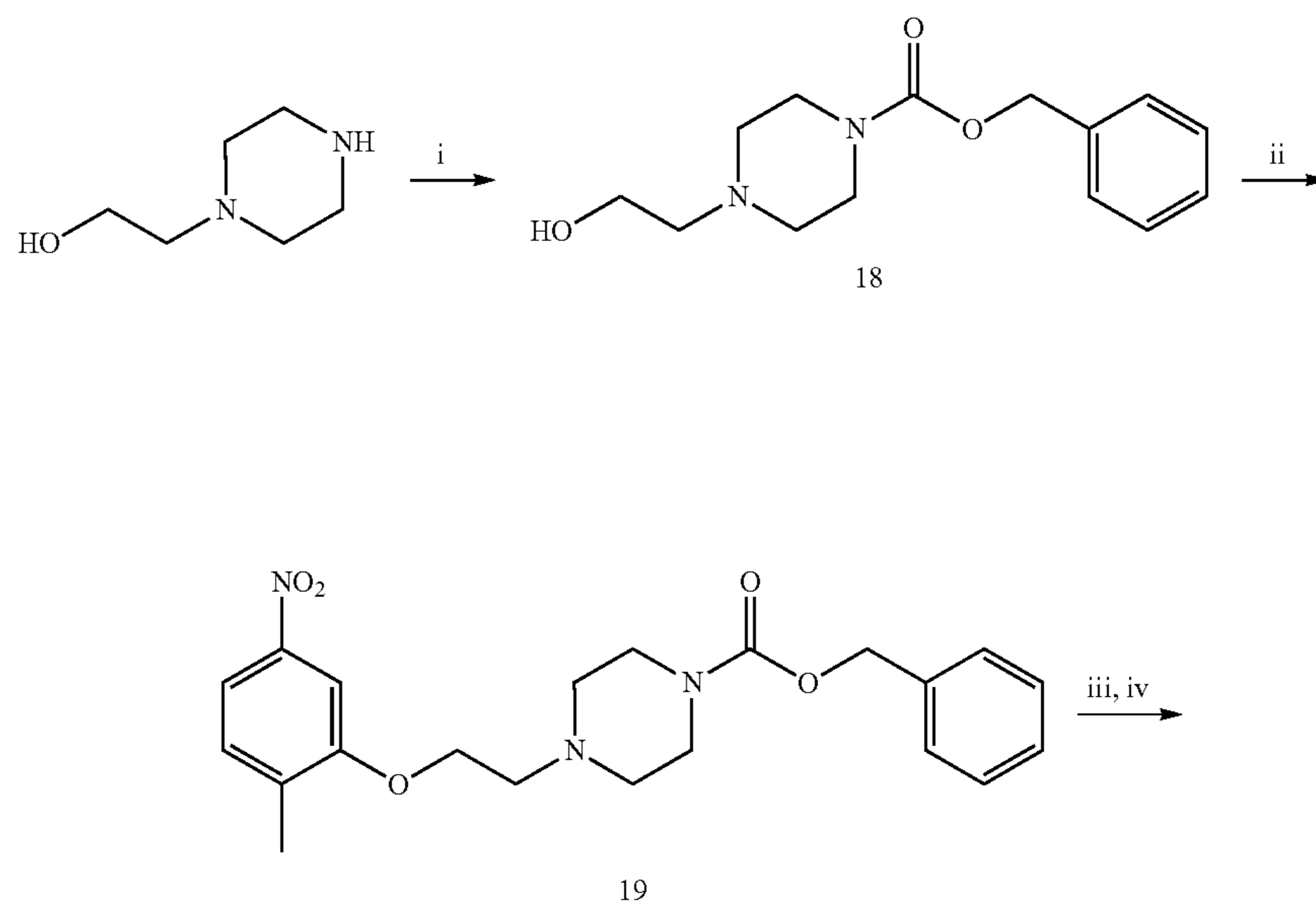
Scheme 5:
