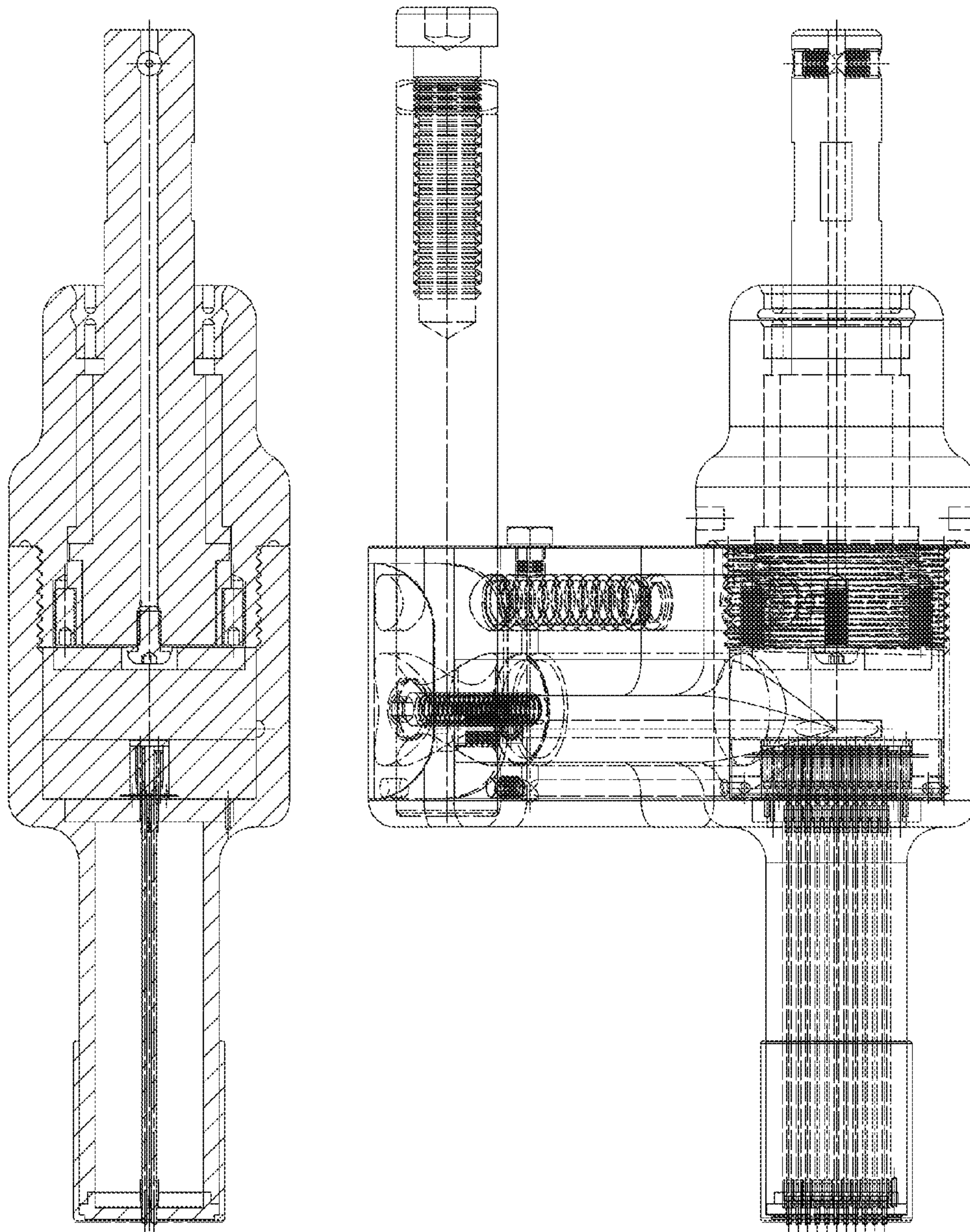
Rechargeable Spindle Rotation Programmable Programmable 2X11 Detachable Stylus Guide (Vertical Stylus Center Line Section View) Selectable Character Multiple Stylus Orbital Engraving Tool's Typical Components and Assembly
