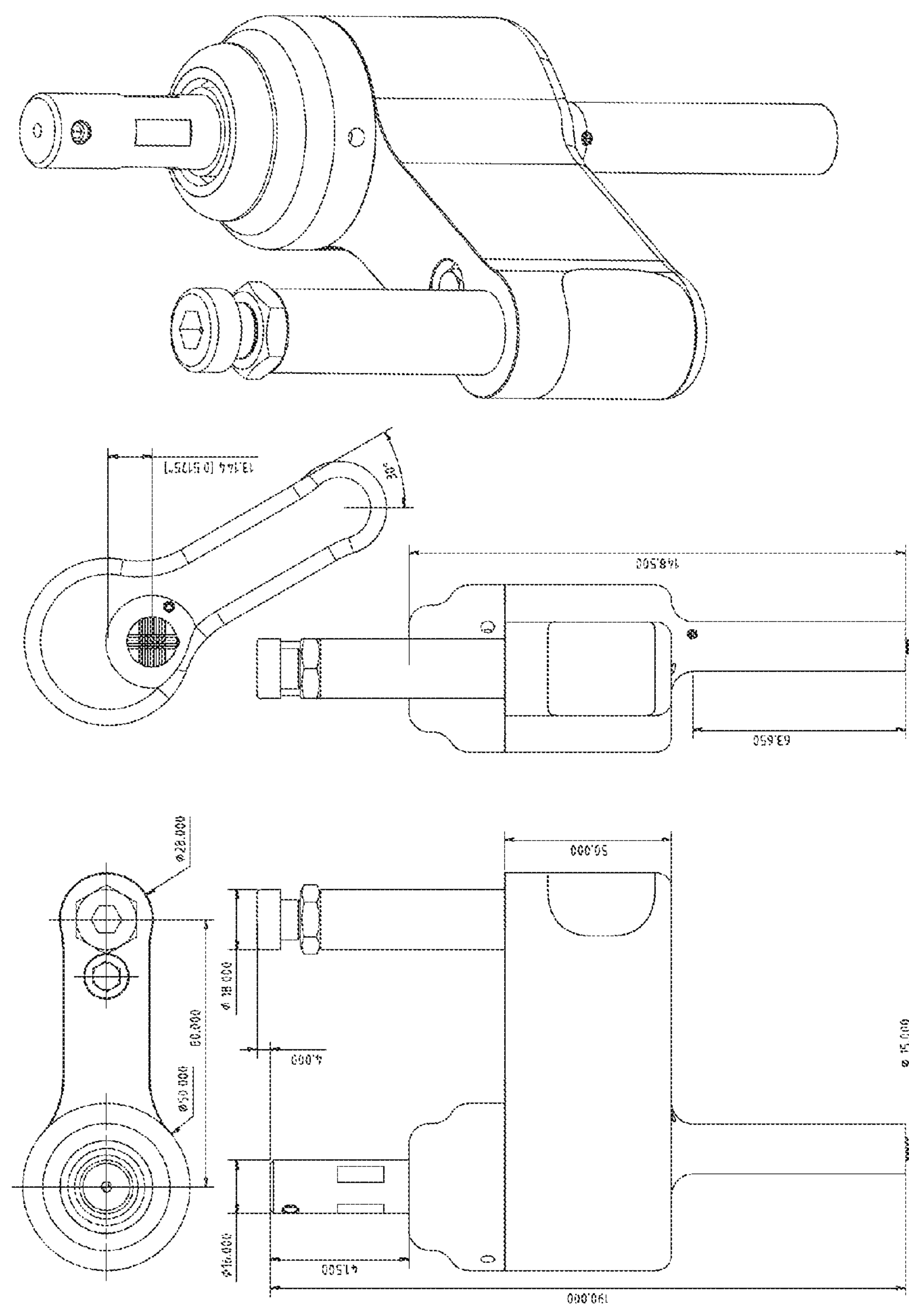
Fig.11 (Dimensioned Assembled View) Typical Components and Assembly of the Selectable Character Multiple Stylus Orbital Engraving Tool
