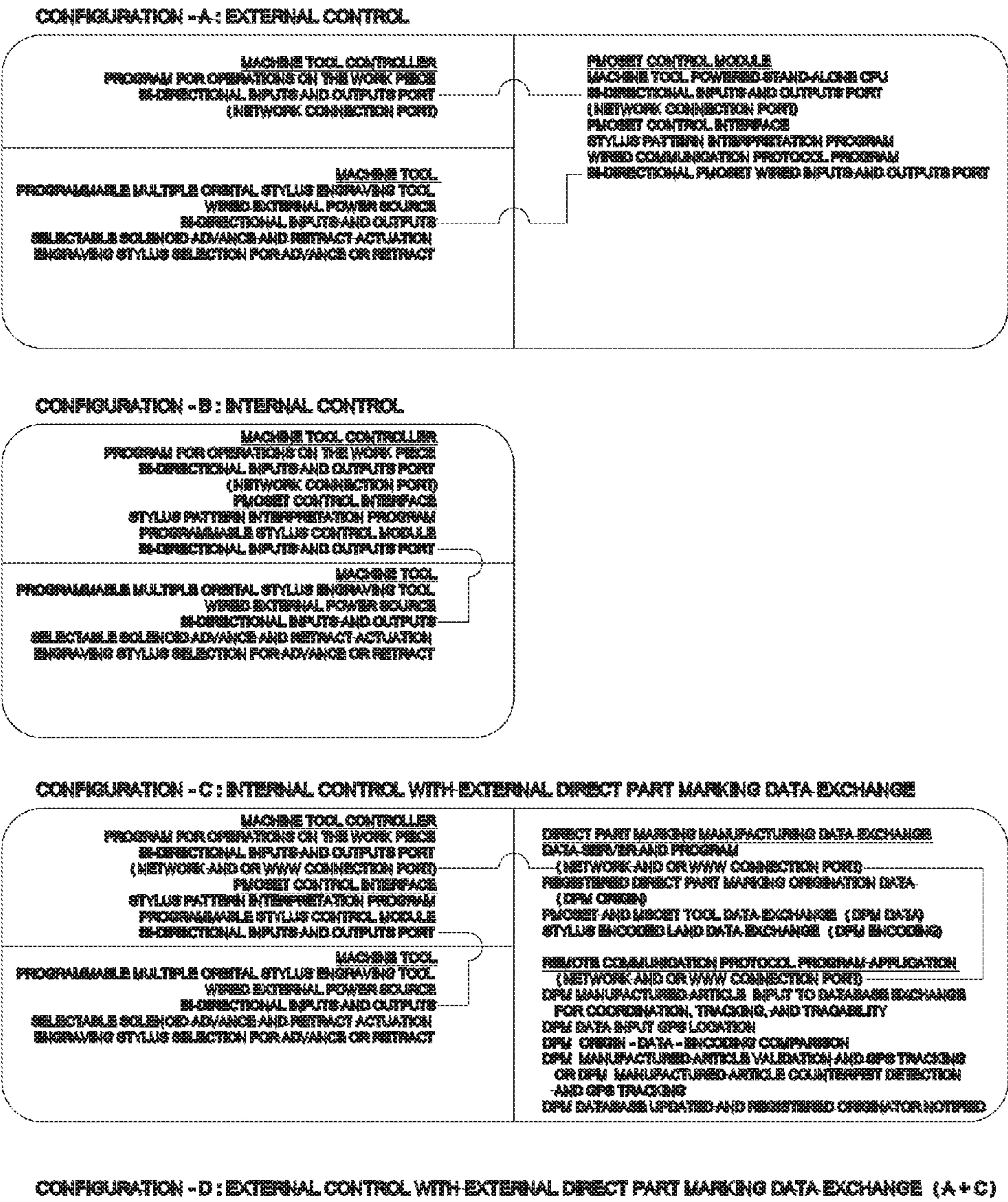
DIRECT PART MARKING DIRECT CONTROL MODULE AND DATA EXCHANGE SCHEMAS PROGRAMMABLE OR SELECTABLE MULTIPLE ORBITAL STYLUS ENGRAVING TOOL (PMOSET) OR (MOSET) CONTROLS AND DATA EXCHANGE SCHEMAS FOR THE STRAIGHT OR ENCODED LAND, SINGLE OR MULTI FLUTE STYLUS Figure-61
