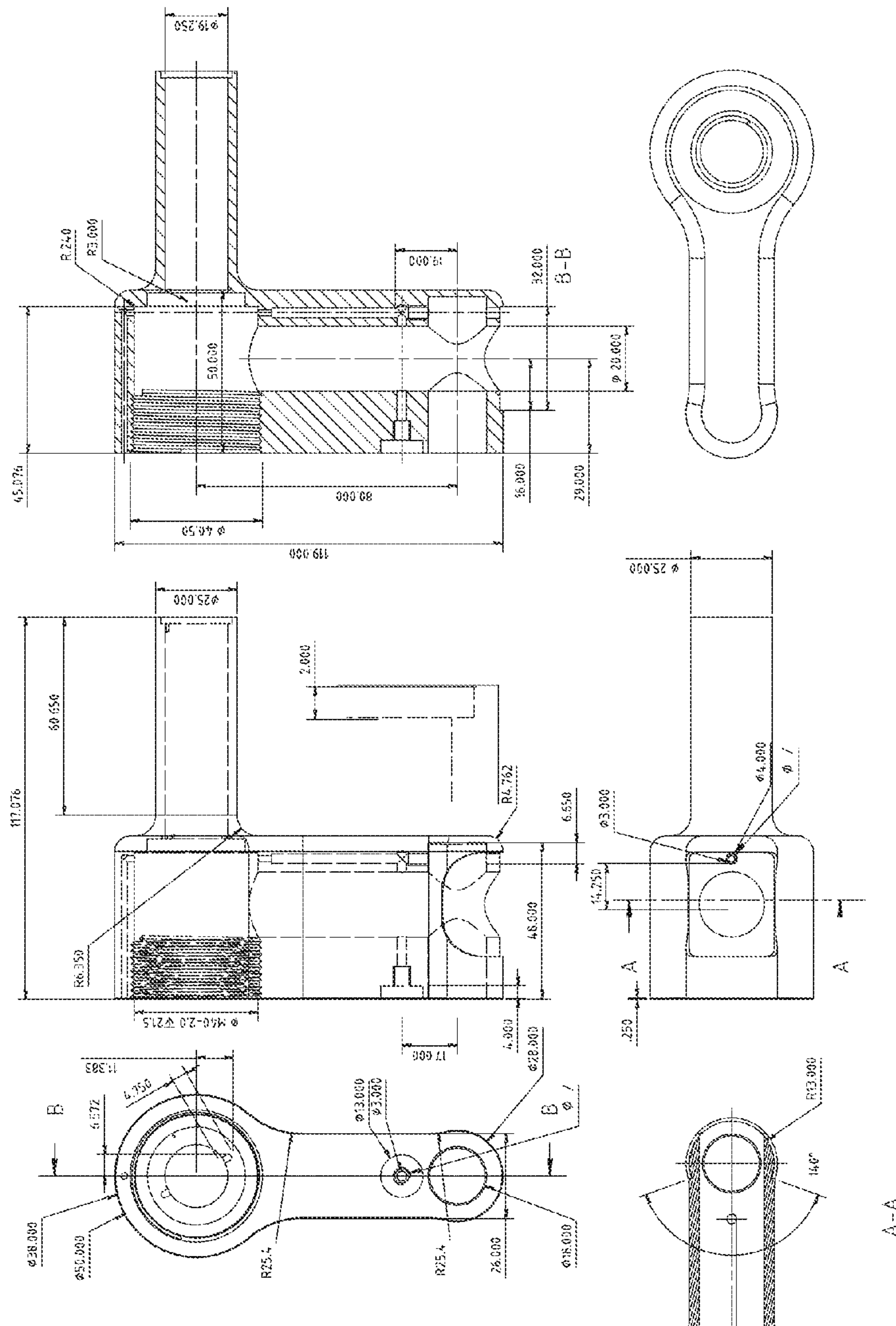
Part 6.211 (2X11) Main Housing:
