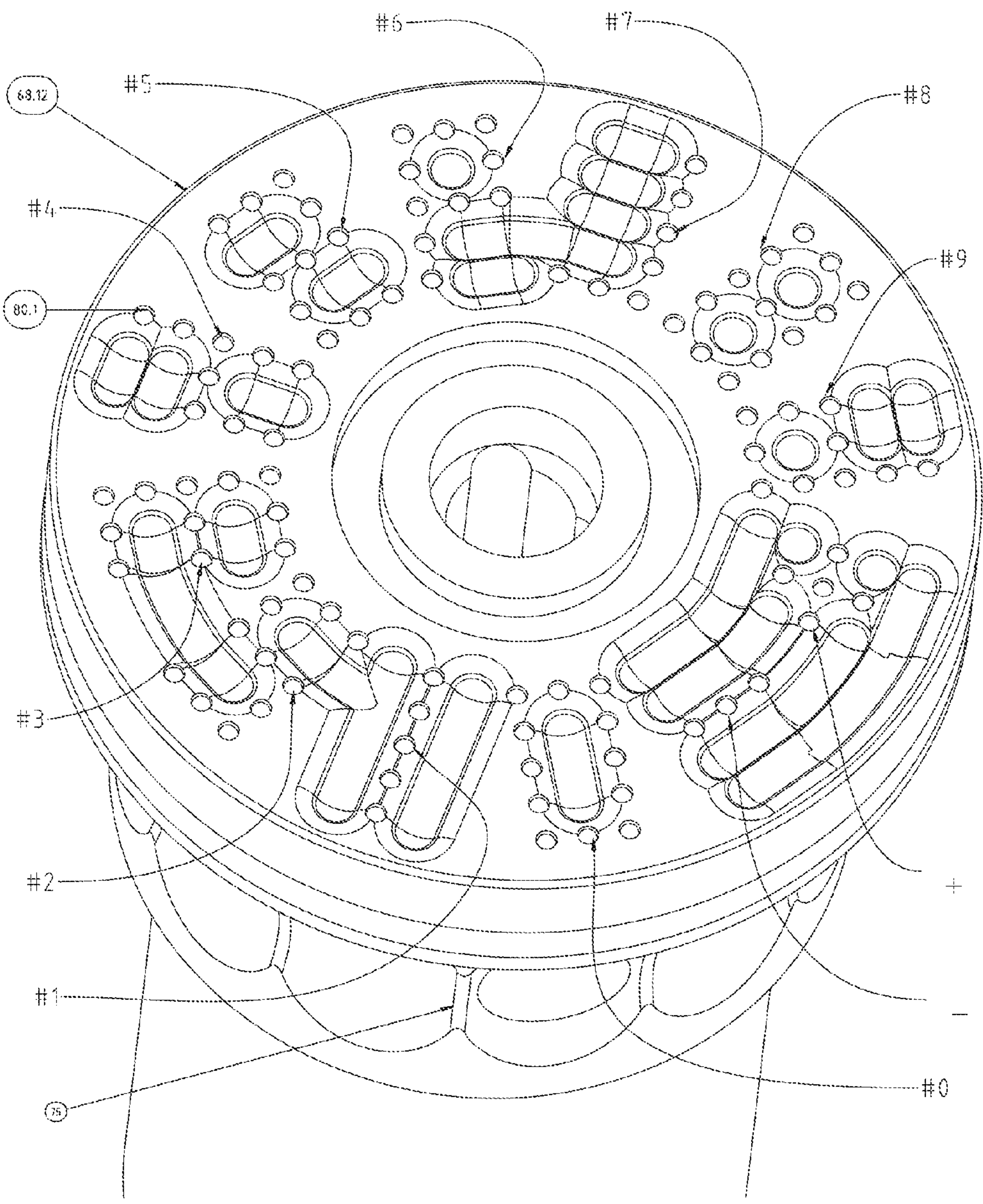
Part-68.12 12-Character for 12-Position Stylus Pattern Disk Component for the Selectable Character Multiple Stylus Orbital Engraving Tool
