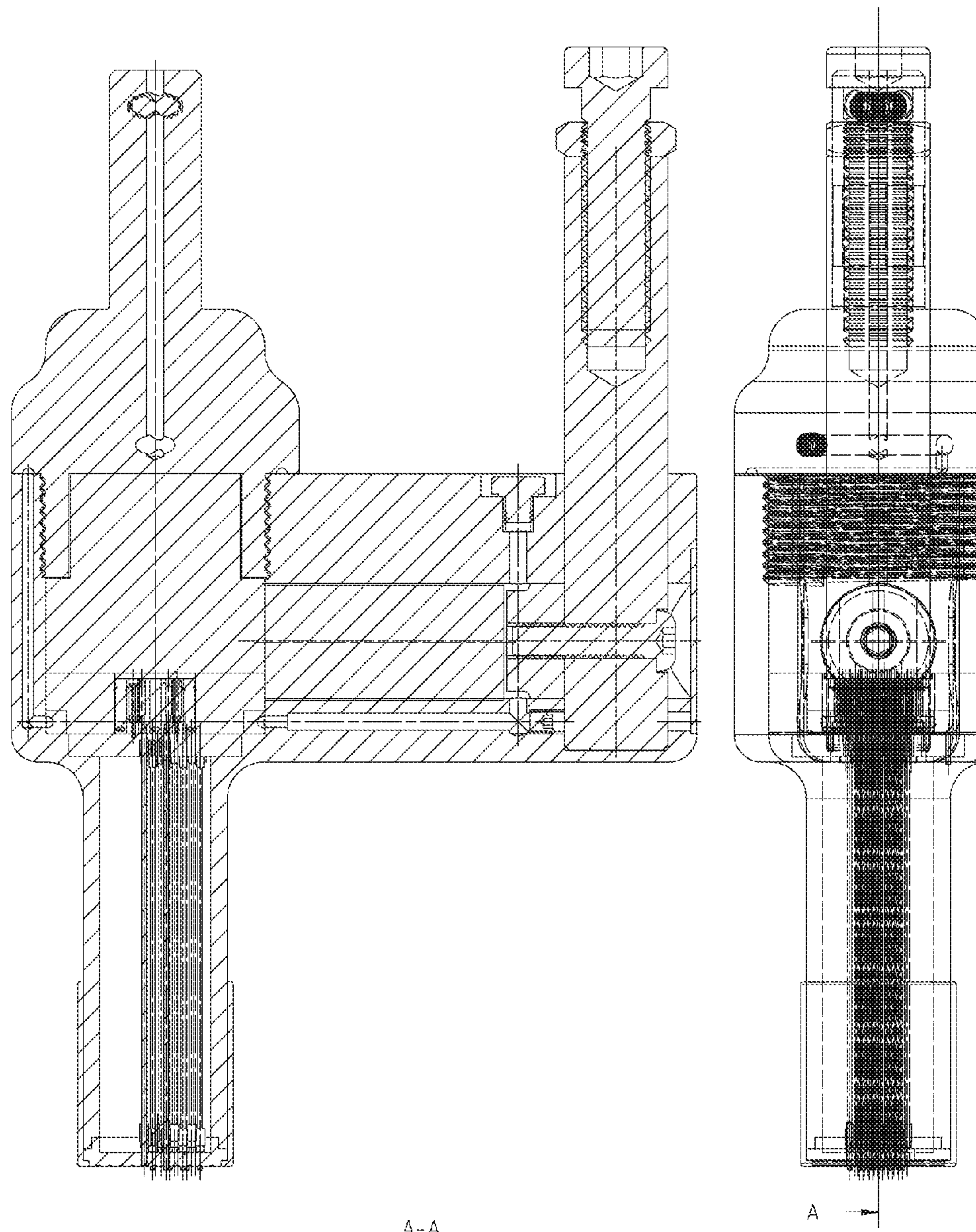
Wireless Programmable 2X11 Detachable Stylus Guide (Arm - Stylus Center Line Section View) Selectable Character Multiple Stylus Orbital Engraving Tool's Typical Components and Assembly
