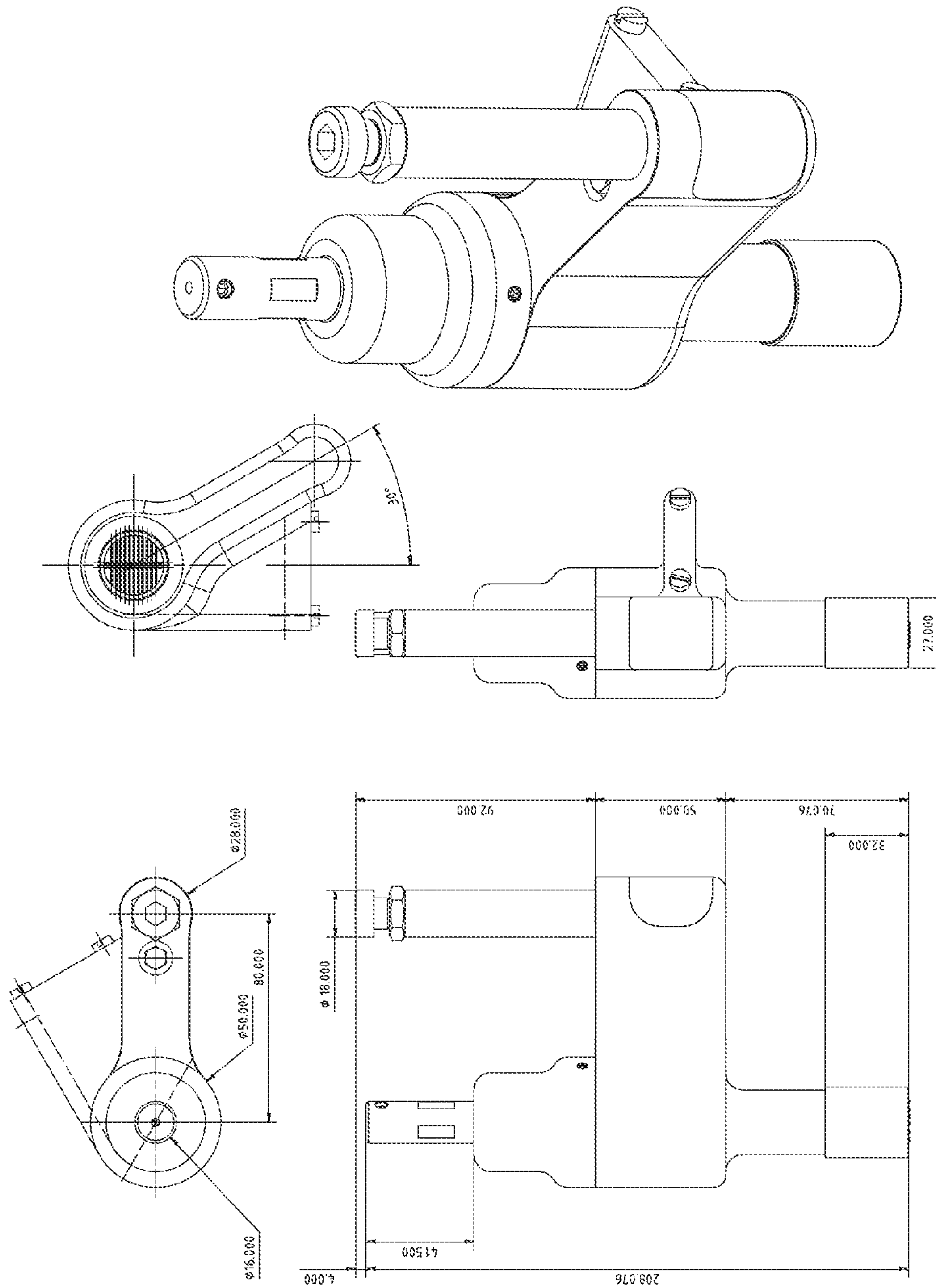
Rechargeable Wireless Programmable ZXR Detachable Stylus Guide (Dimensioned Assembled View)
