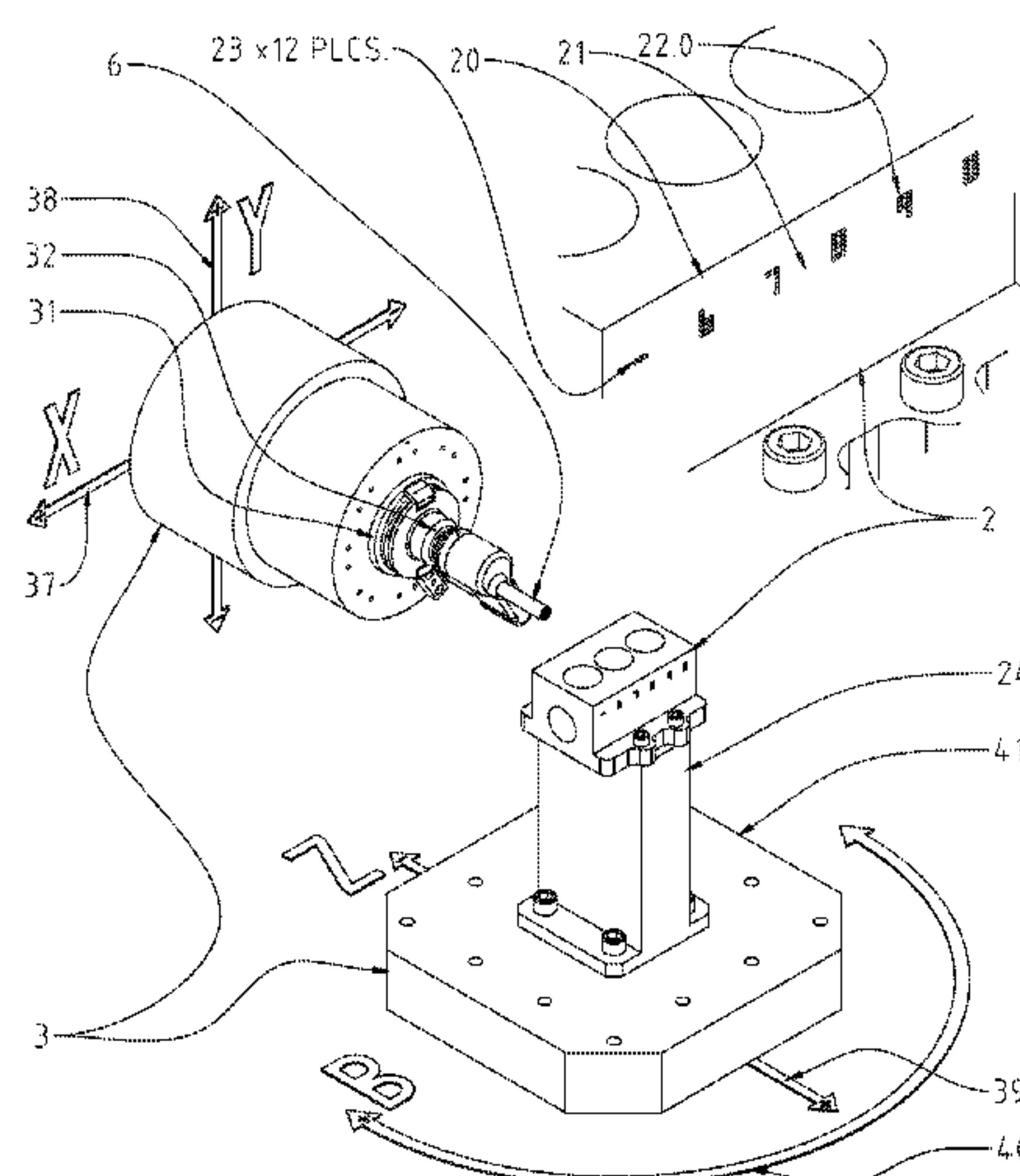
(X+ Iso. View) Typical Horizontal Machine Tool for the Selectable Character Multiple Stylus Orbital Engraving Tool
