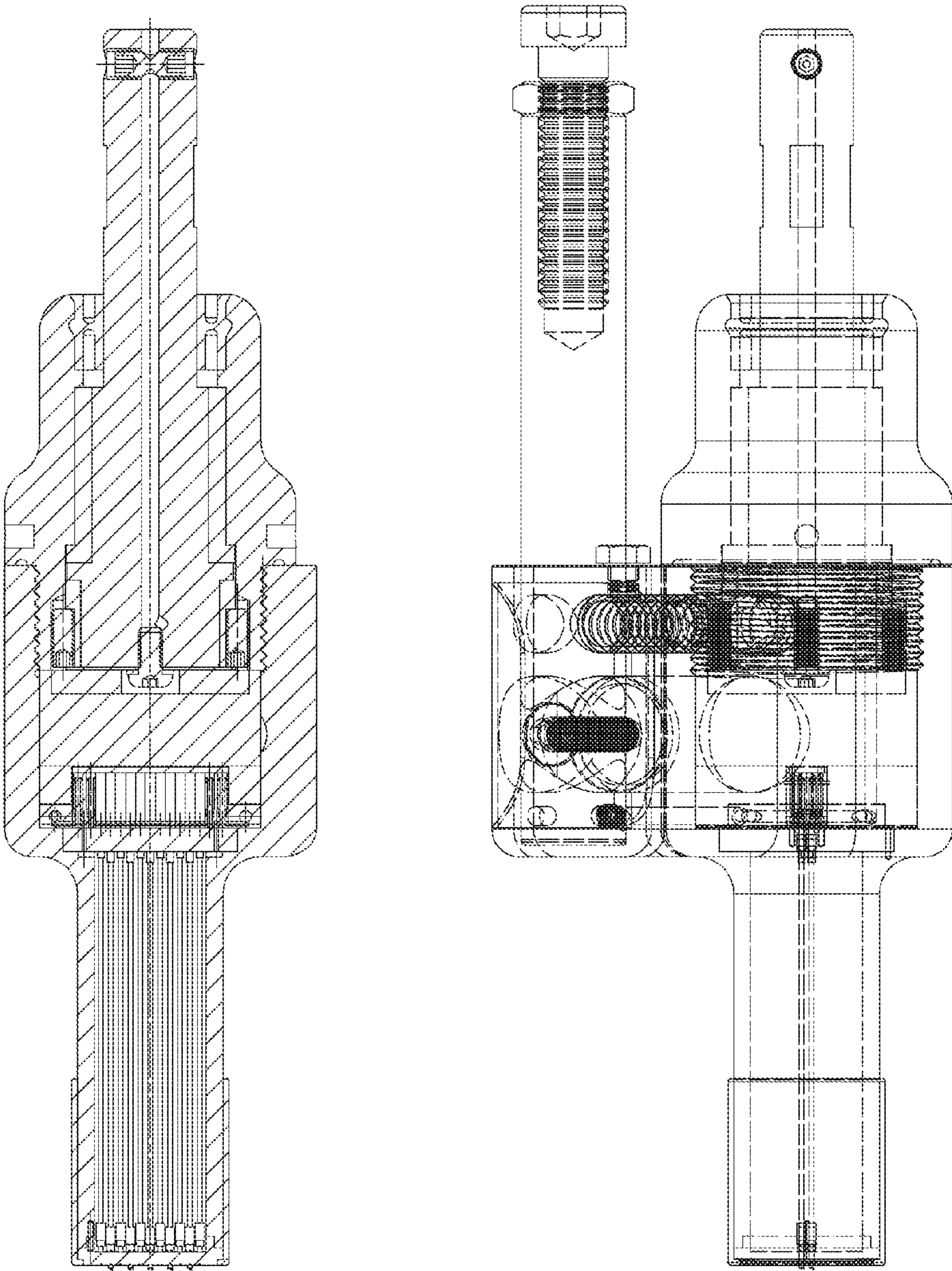
Spindle Rotation Programmable 2X11 Detachable Stylus Guide (Horizontal Stylus Center Line Section View) Selectable Character Multiple Stylus Orbital Engraving Tool's Typical Components and Assembly
