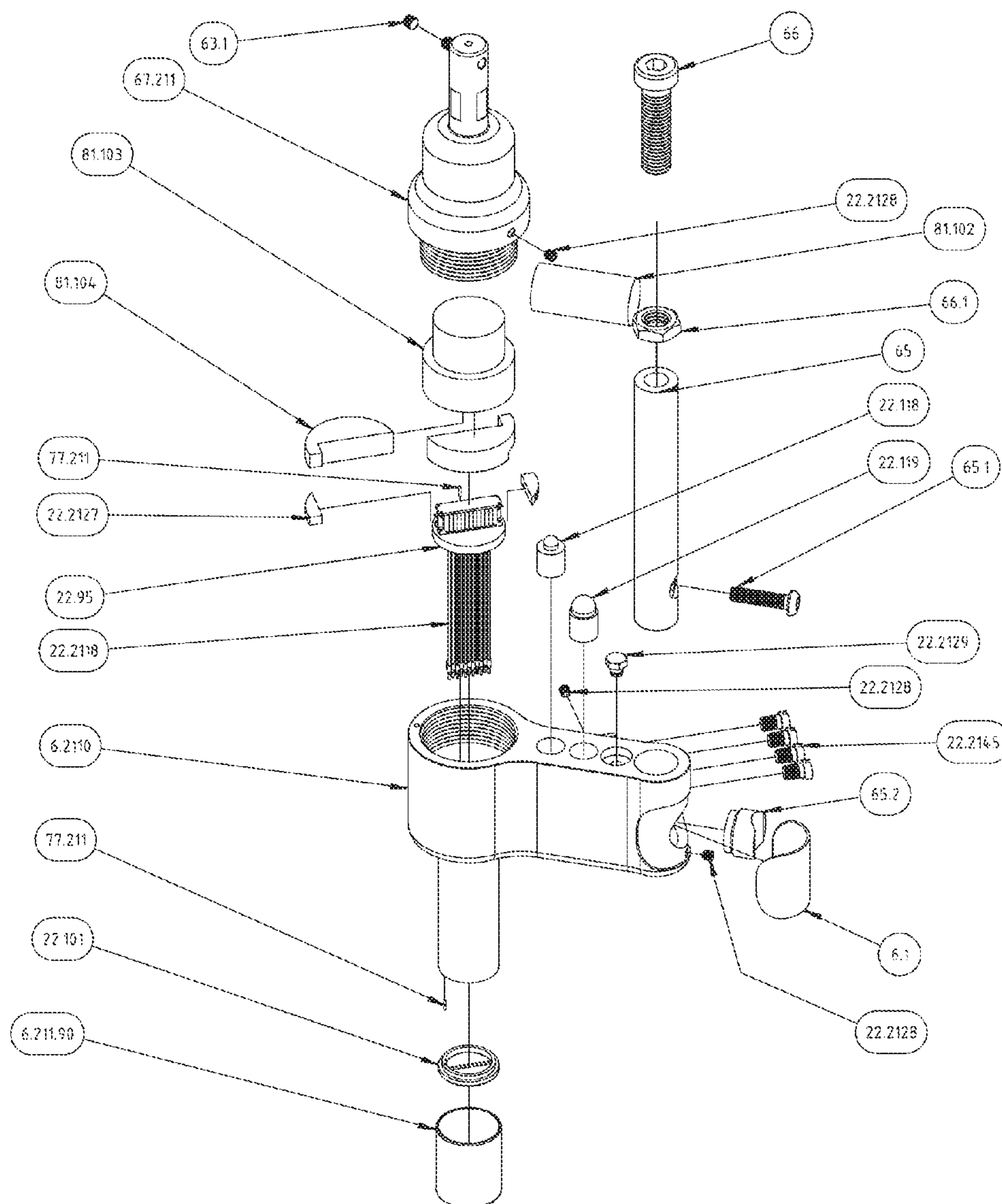
Rechargeable Contact and Optical Programmable 2X11 Detachable Stylus Guide (Exploded Parts View) Selectable Character Multiple Stylus Orbital Engraving Tool's Typical Components and Assembly
