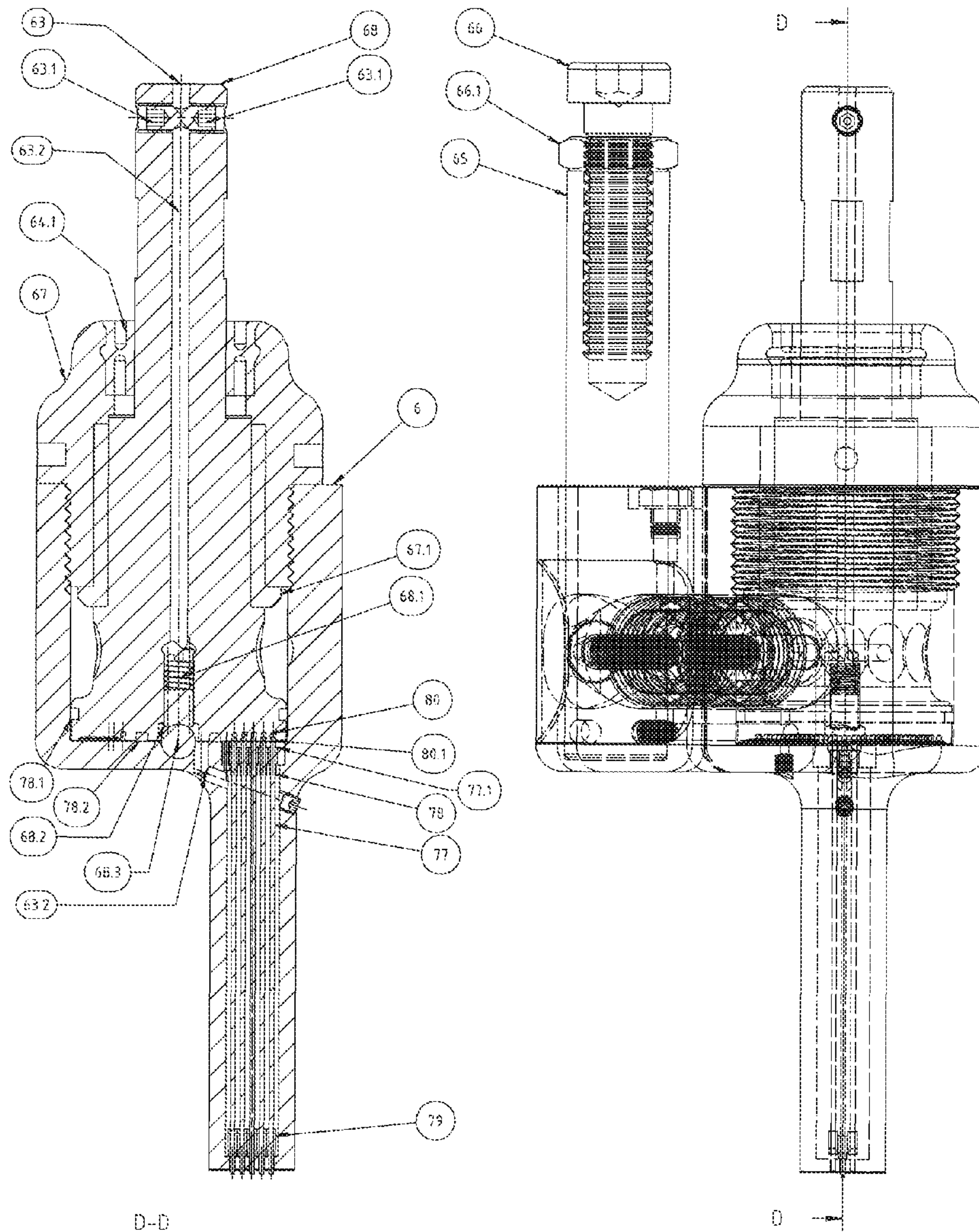
Fig. 15 (Stylus Center Line Section View) Character Pattern #1 Stylus Activation of the Selectable Character Multiple Stylus Orbital Engraving Tool
