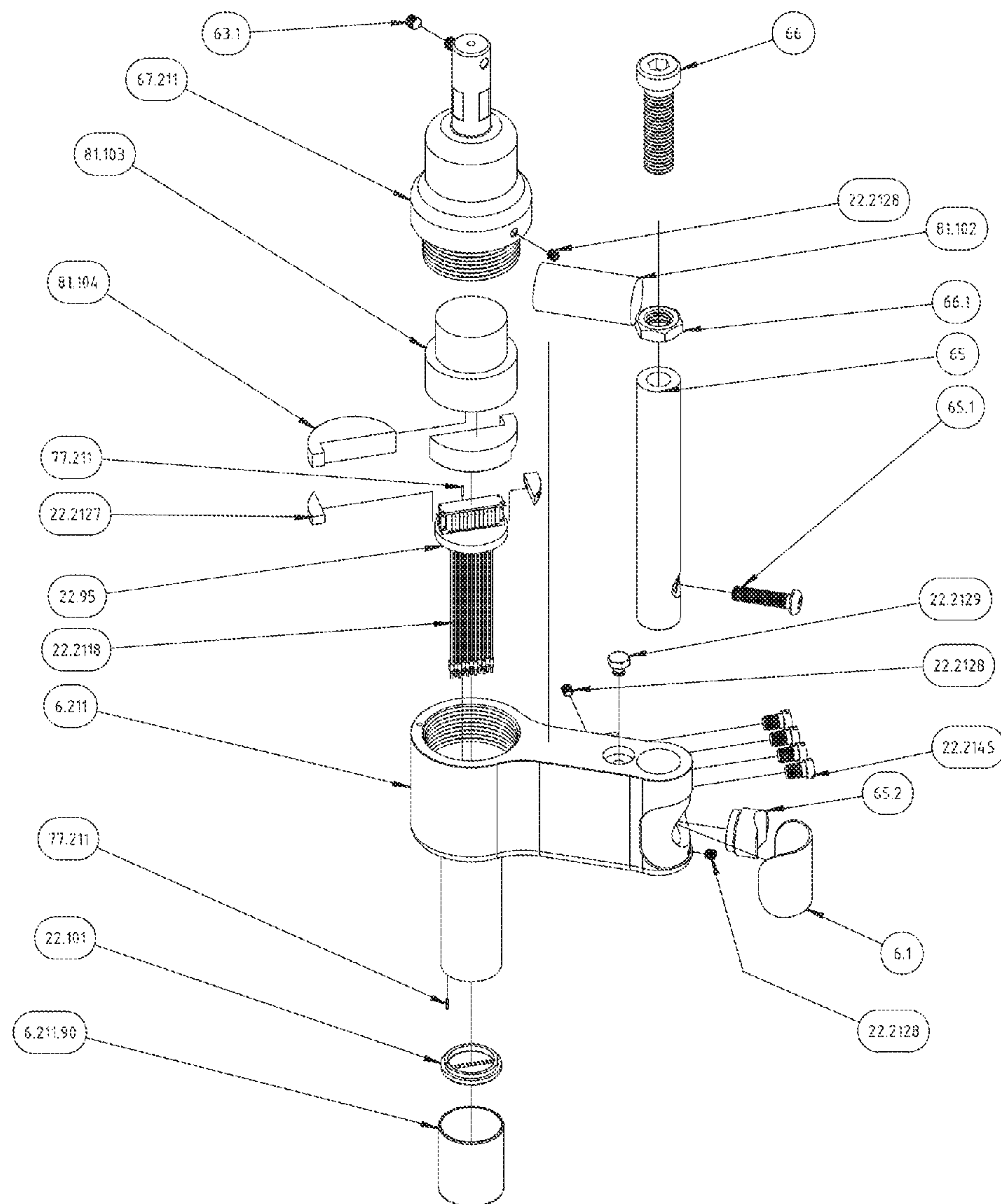
Rechargeable Contact Programmable 2X11 Detachable Stylus Guide (Exploded Parts View) Selectable Character Multiple Stylus Orbital Engraving Tool's Typical Components and Assembly
