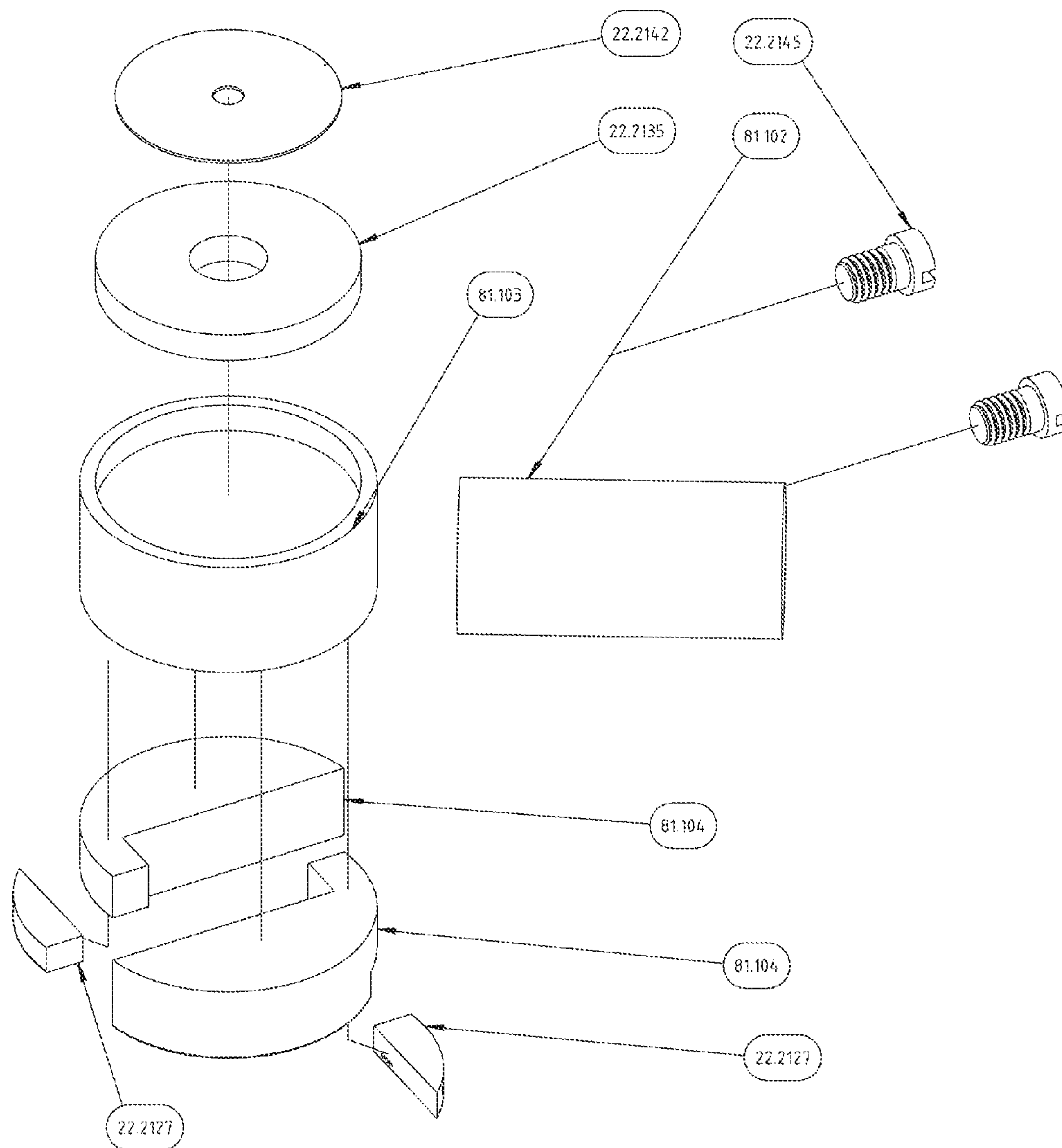
Rechargeable Spindle Rotation Programmable Programmable 2X11 Detachable Stylus Guide (Exploded Electrical Module View) Selectable Character Multiple Stylus Orbital Engraving Tool's Typical Components and Assembly
