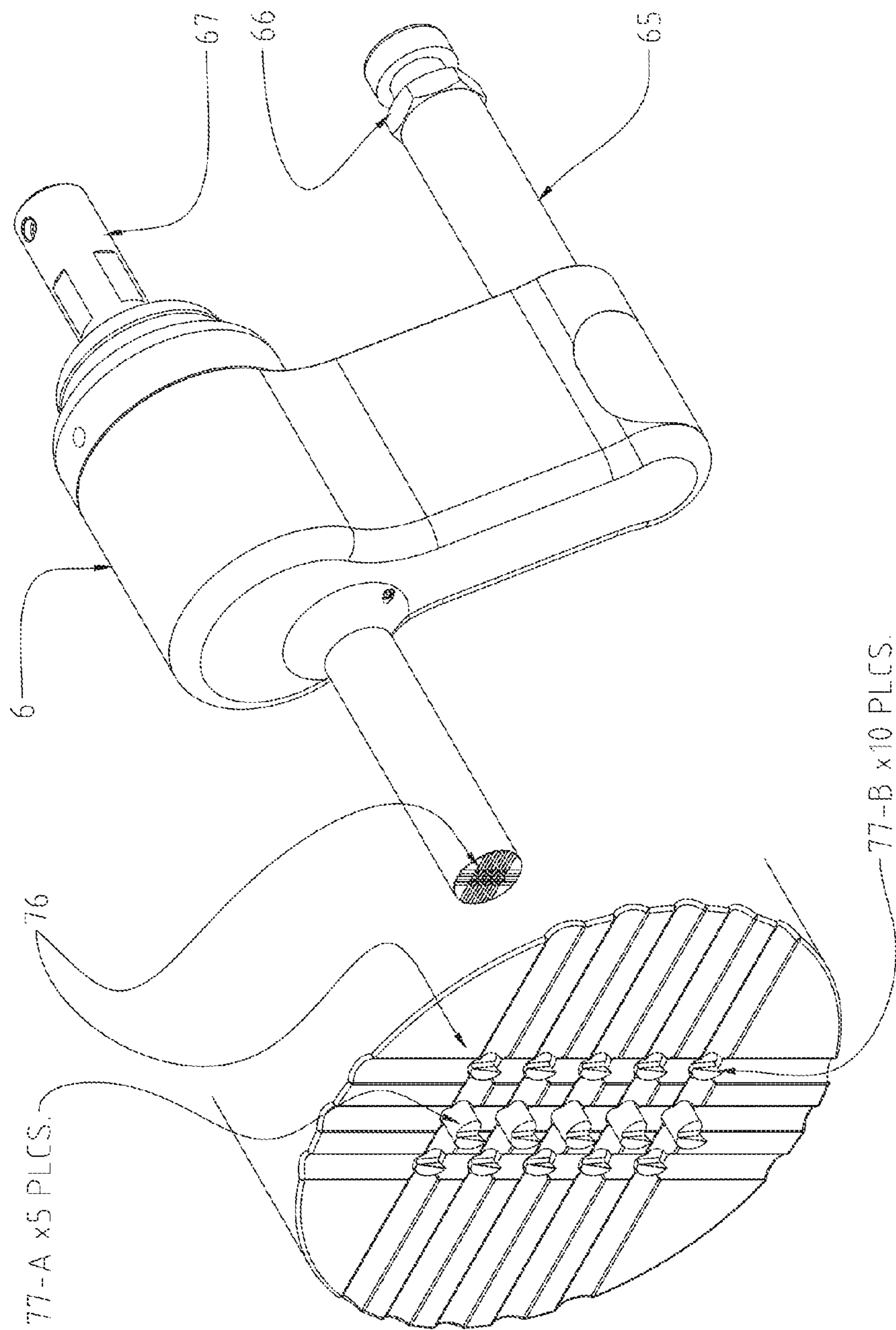
FIGURE 8 (X- Iso. View) Character "1" Selected for the Selectable Character Multiple Stylus Orbital Engraving Tool
