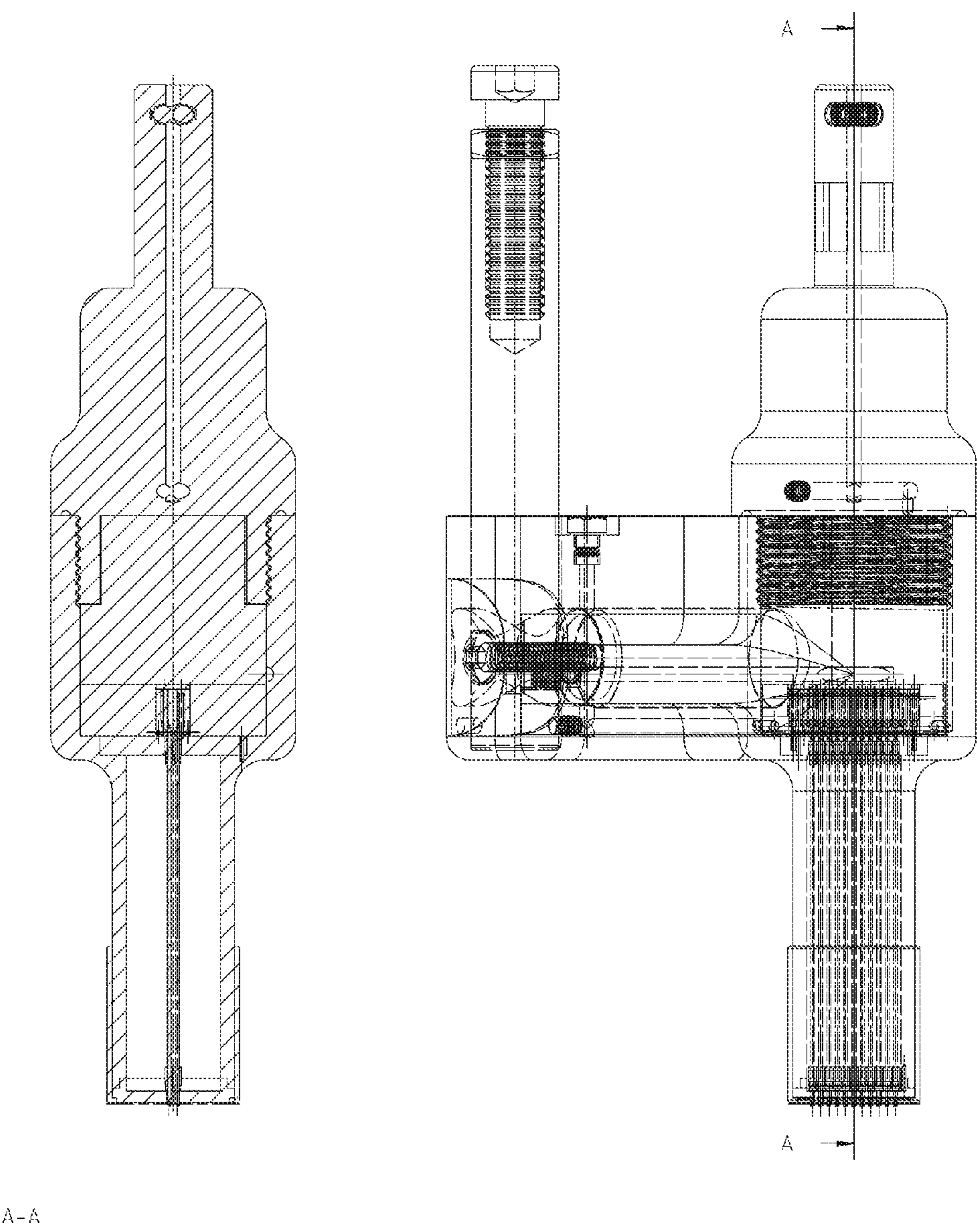
Rechargeable Contact Programmable 2X11 Detachable Stylus Guide (Vertical Stylus Center Line Section View) Selectable Character Multiple Stylus Orbital Engraving Tool's Typical Components and Assembly
