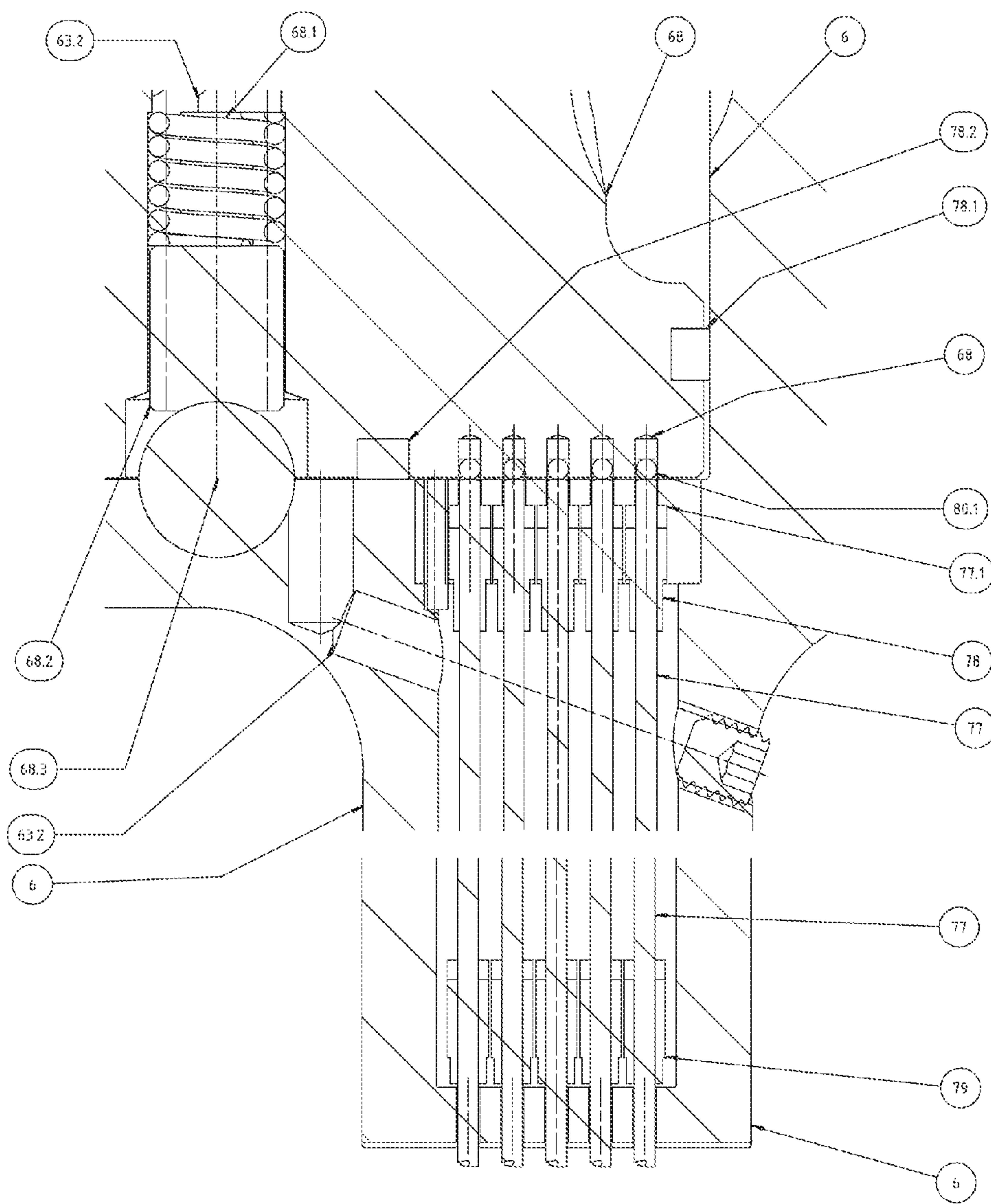
Fig. 16 (Stylus Center Line Detail Section View) Character Pattern #1 Stylus Activation of the Selectable Character Multiple Stylus Orbital Engraving Tool
