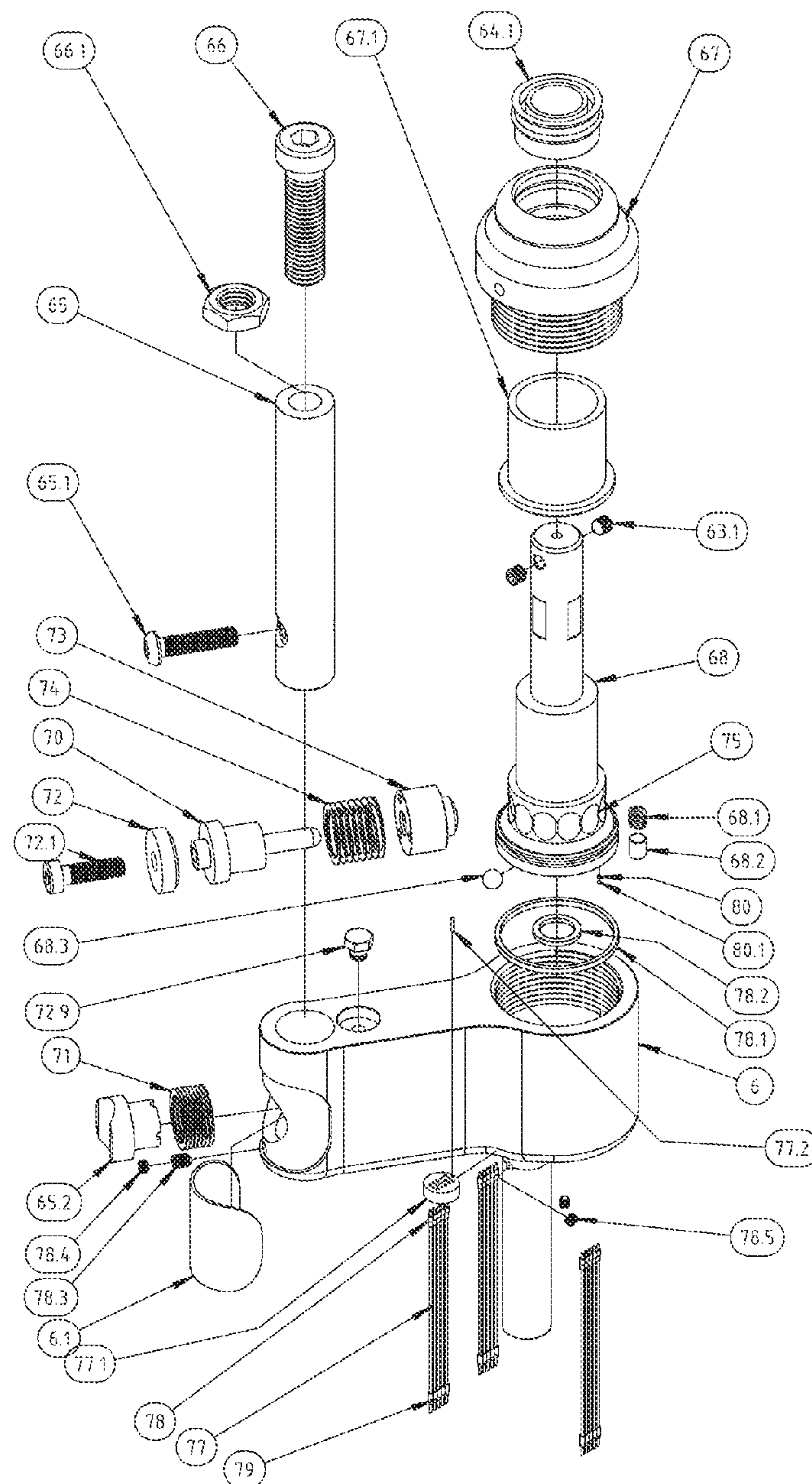
Fig.12 (Exploded Parts View) Typical Components and Assembly of the Selectable Character Multiple Stylus Orbital Engraving Tool
