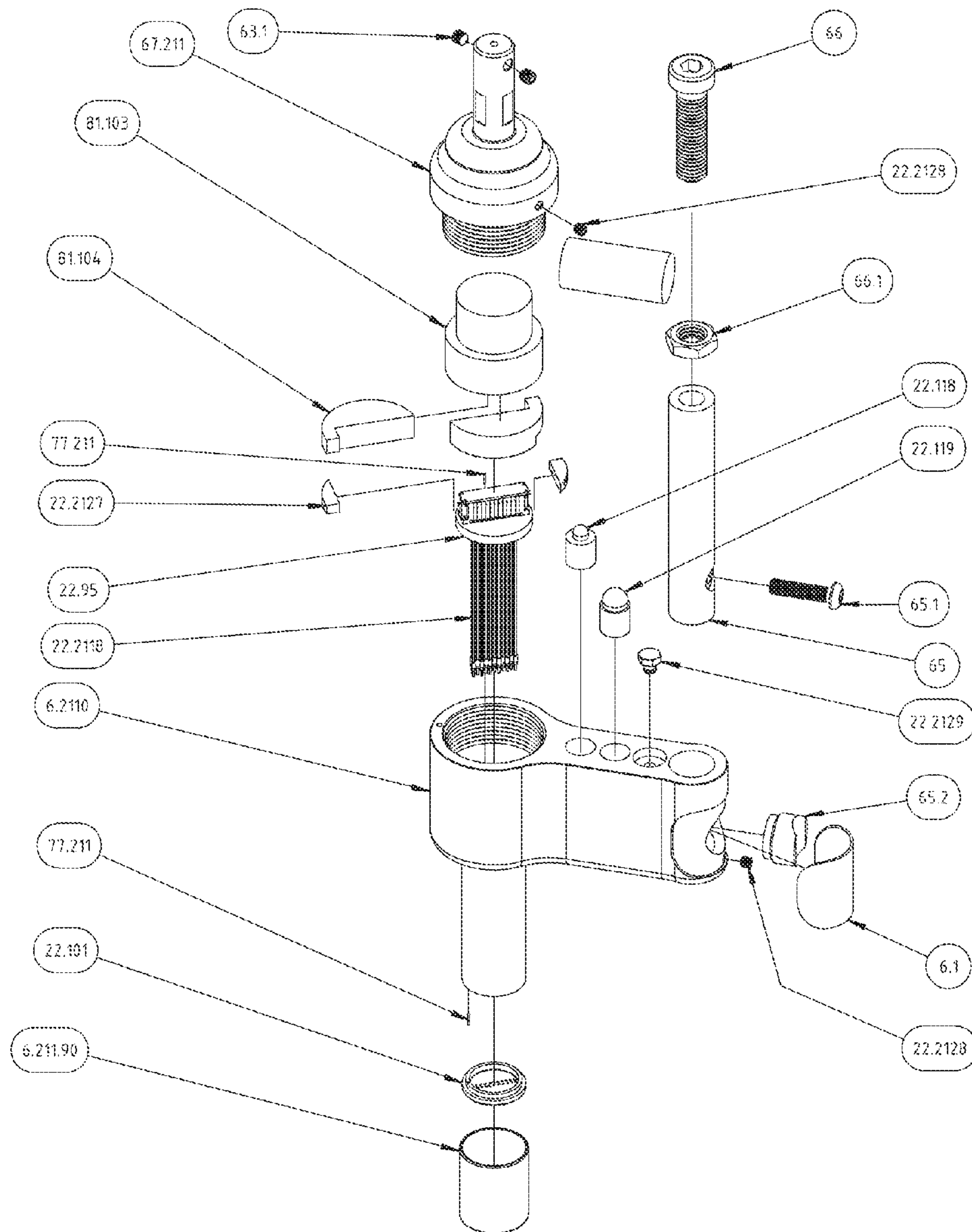
Optical Programmable 2X11 Detachable Stylus Guide (Exploded Parts View) Selectable Character Multiple Stylus Orbital Engraving Tool's Typical Components and Assembly
