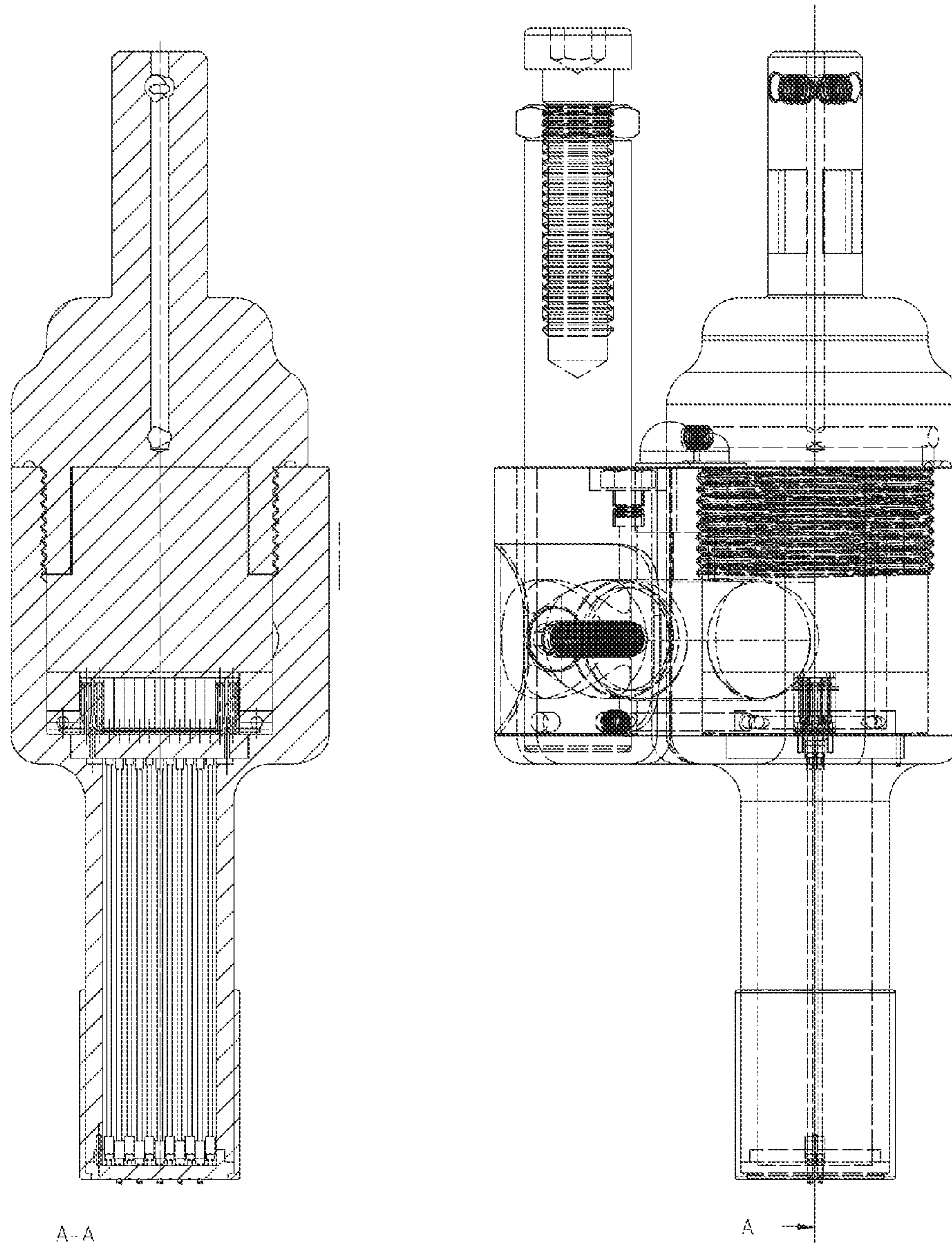
Optical Programmable 2X11 Detachable Stylus Guide (Horizontal Stylus Center Line Section View) Selectable Character Multiple Stylus Orbital Engraving Tool's Typical Components and Assembly
