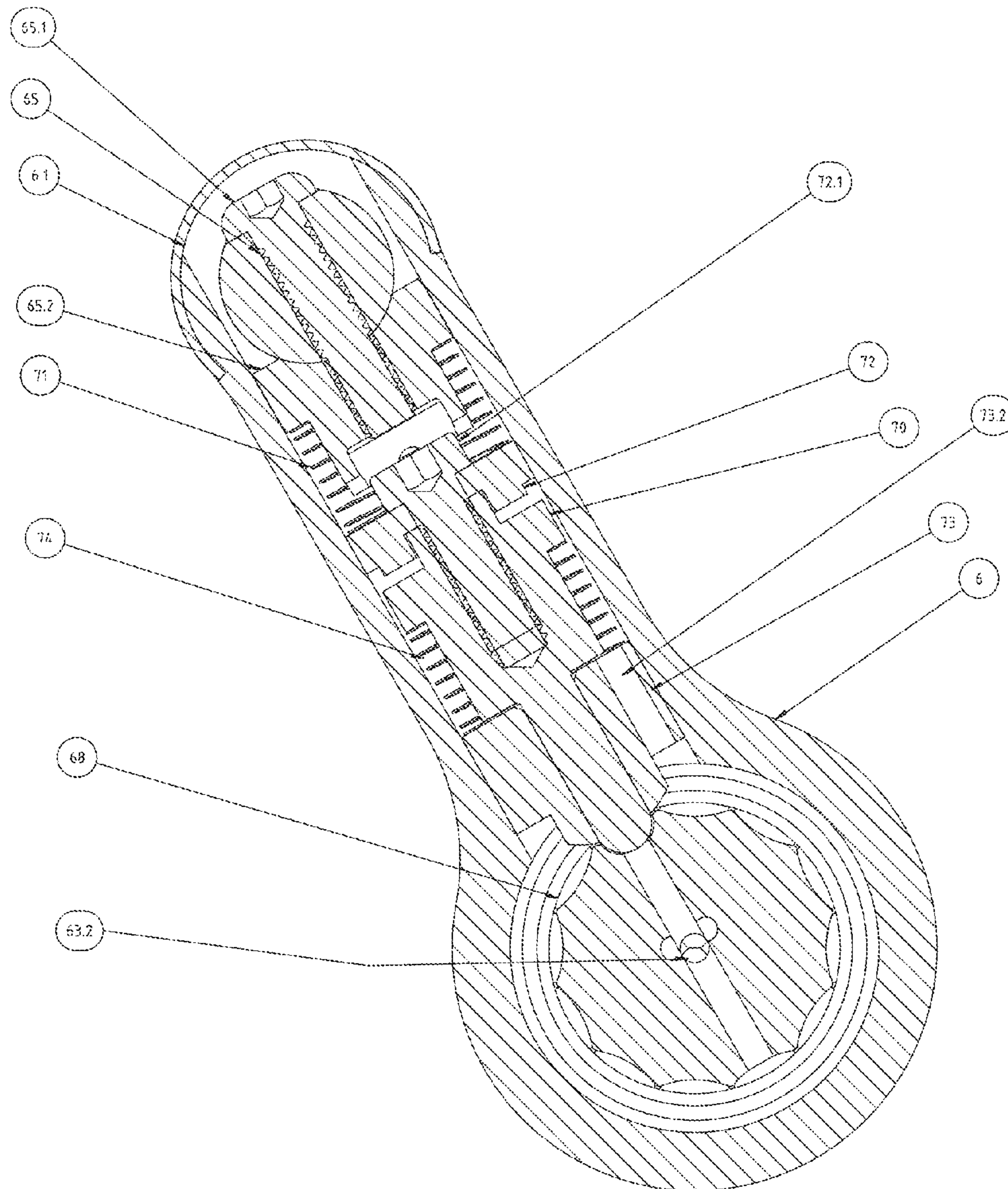
Fig. 17 (Index Lock Center Line Section View) Character Pattern Selection Disk in the Locked Position for the Selectable Character Multiple Stylus Orbital Engraving Tool
