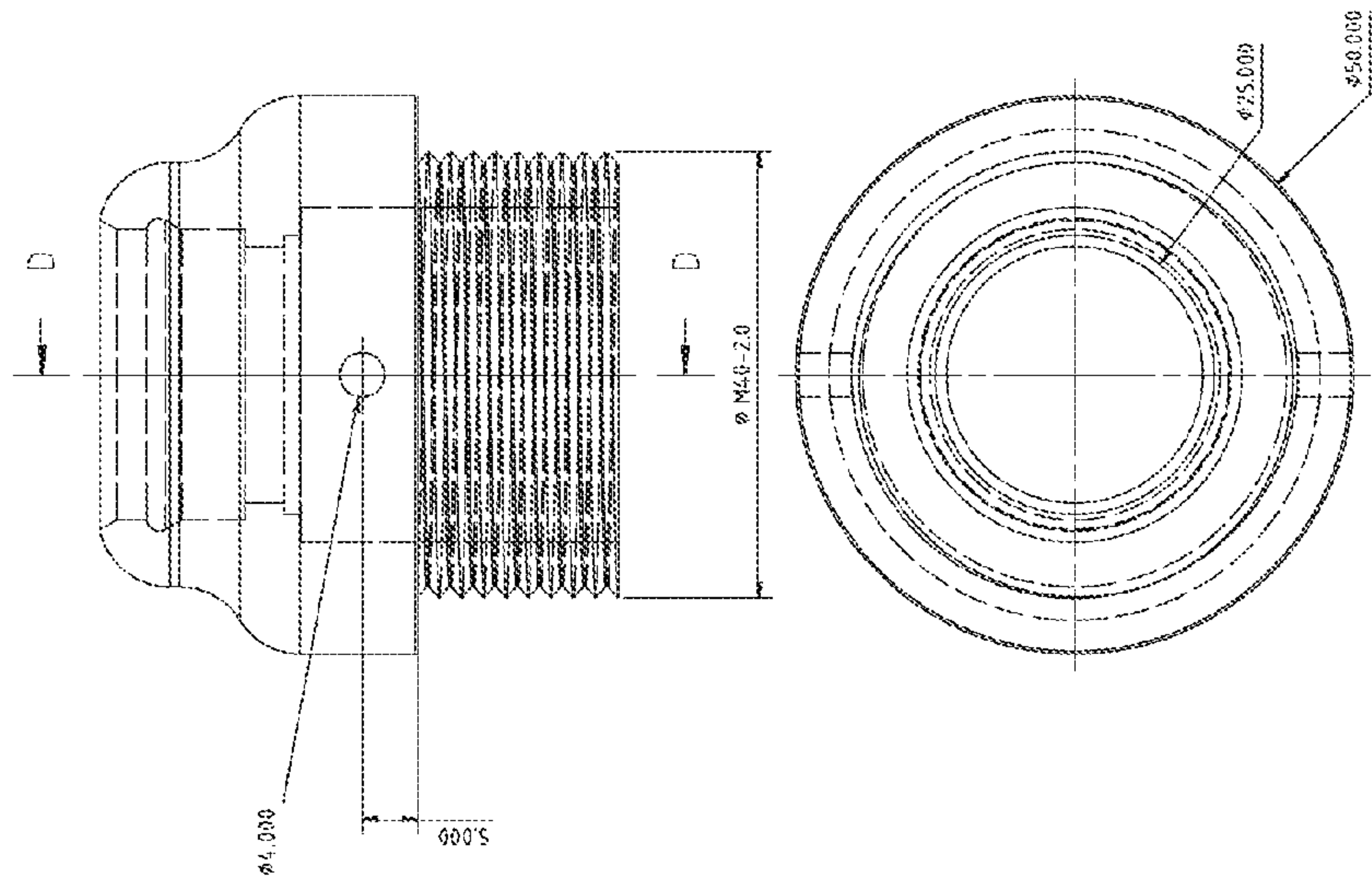
Part-67 MOSET Main Housing Shaft Collar Component for the Selectable Character Multiple Stylus Orbital Engraving Tool
