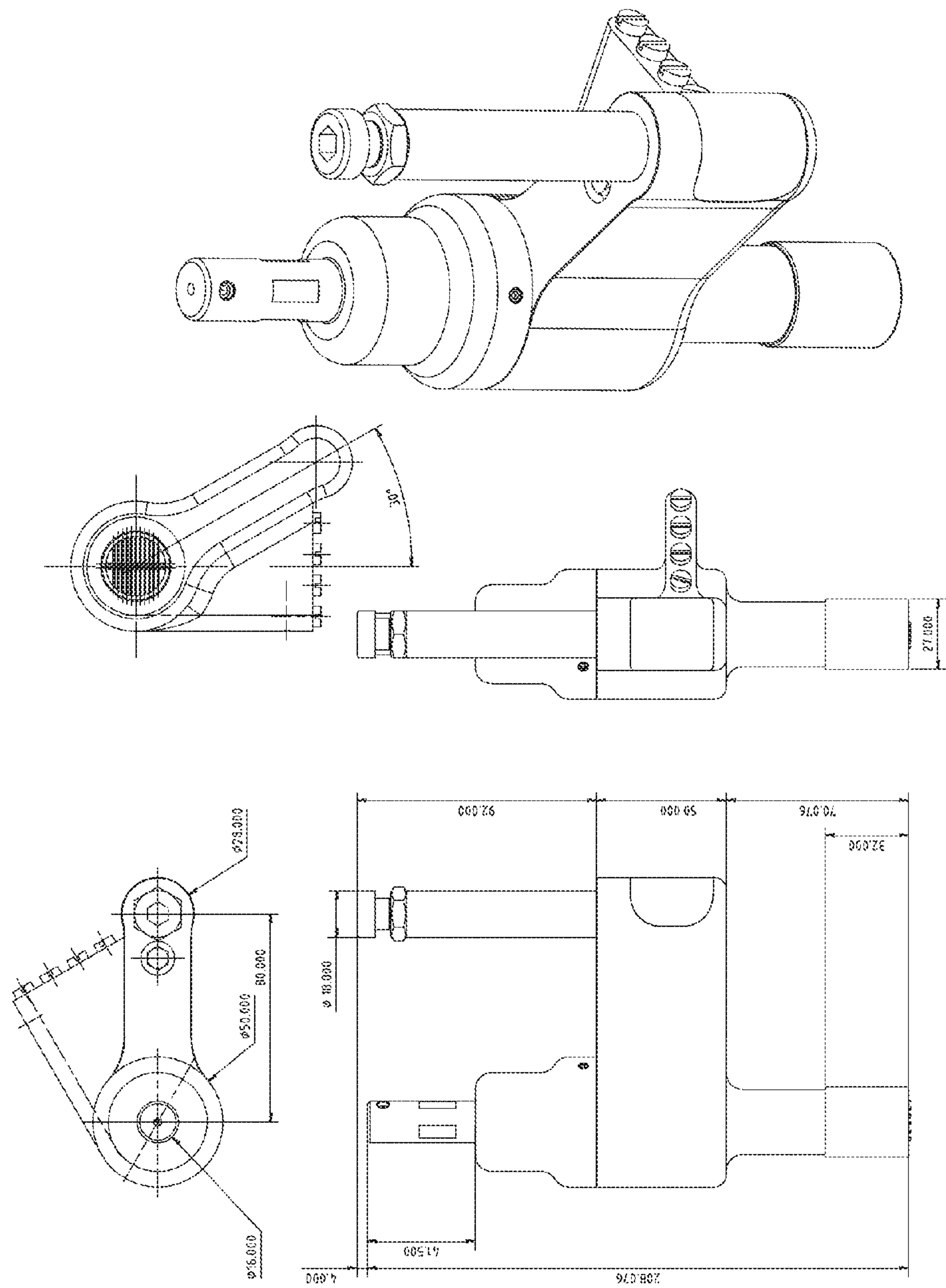
Rechargeable Contact Programmable 2X11 Detachable Stylus Guide (Dimensioned Assembled View) Selectable Character Multiple Stylus 0-bit Engraving Tool's Typical Components and Assembly
