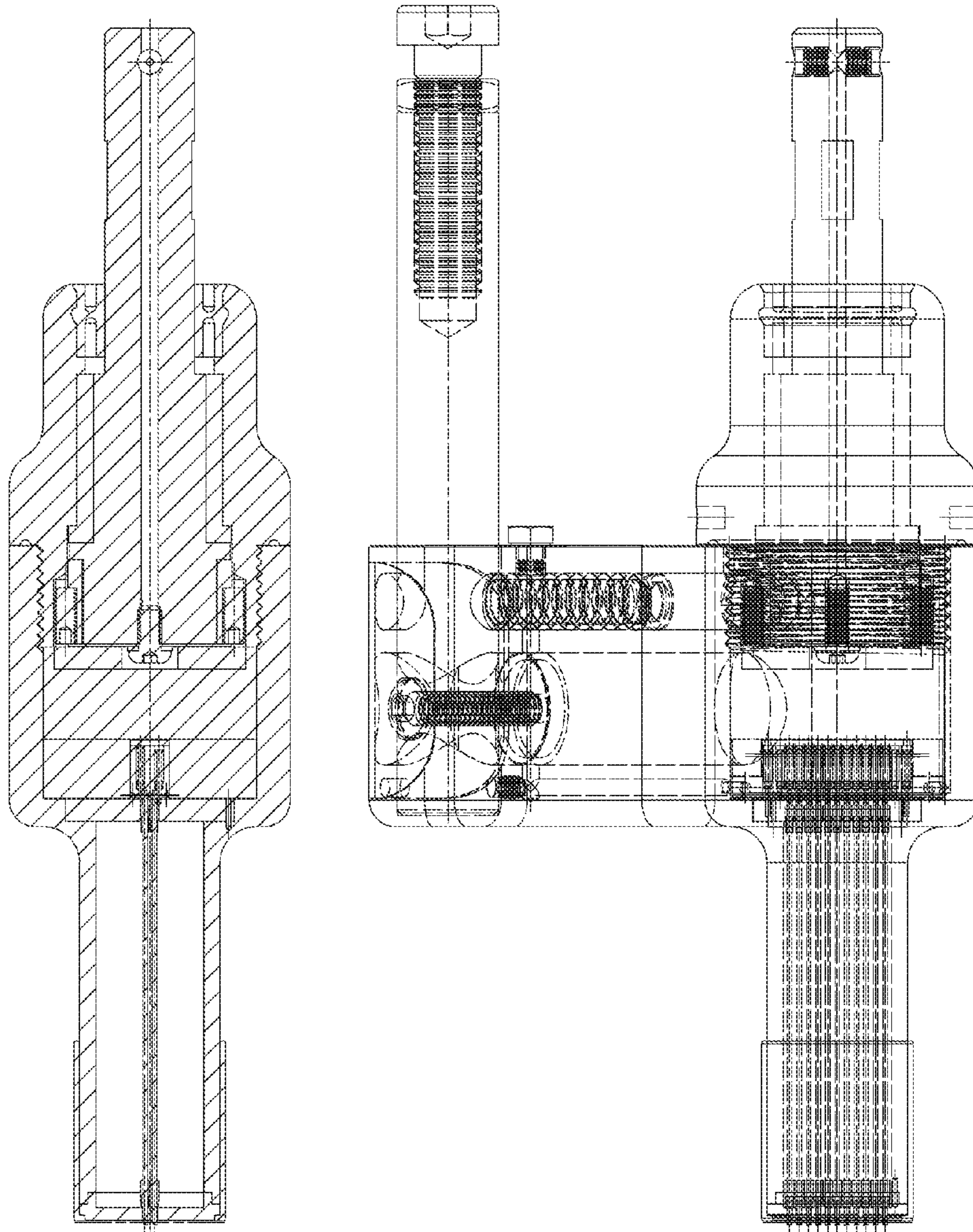
Spindle Rotation Programmable 2K11 Detachable Stylus Guide (Vertical Stylus Center Line Section View) Selectable Character Multiple Stylus Orbital Engraving Tool's Typical Components and Assembly
