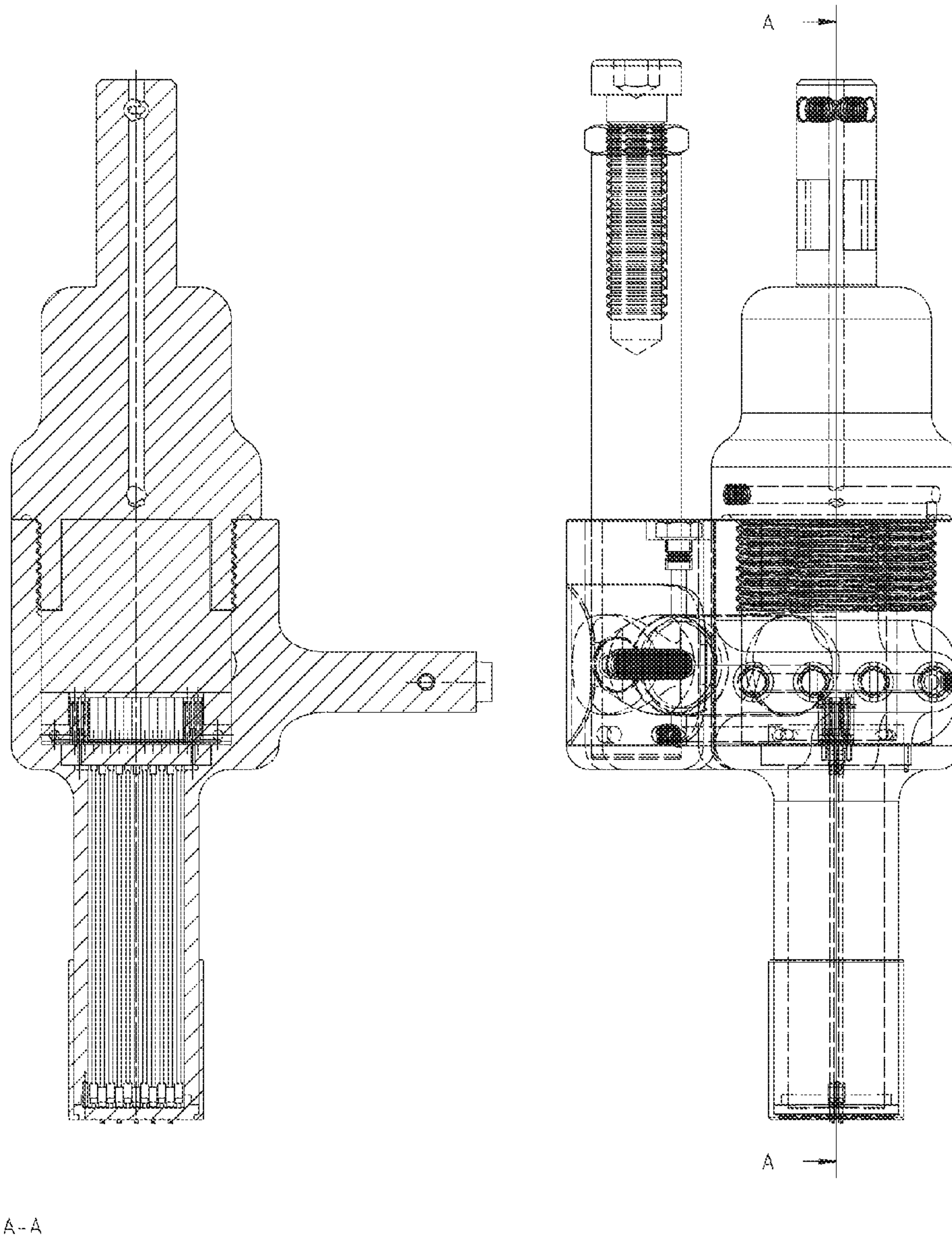
Rechargeable Contact Programmable 2X11 Detachable Stylus Guide (Horizontal Stylus Center Line Section View) Selectable Character Multiple Stylus Orbital Engraving Tool's Typical Components and Assembly
