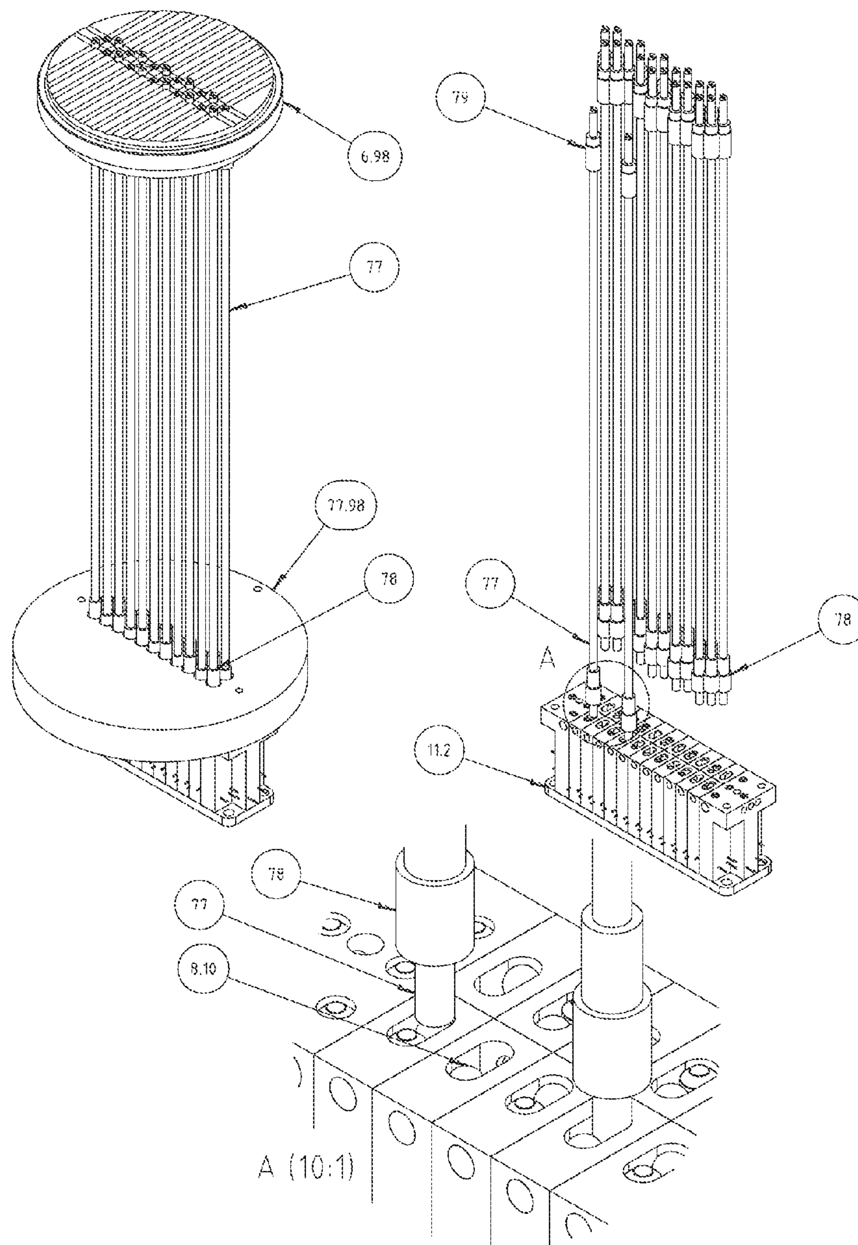
Programmable 2X11 STYLUS ACTUATION MODULE (ACTUATED STYLUS TEST PATTERN #1 SHOWN) For the Selectable Character Multiple Stylus Orbital Engraving Tool
