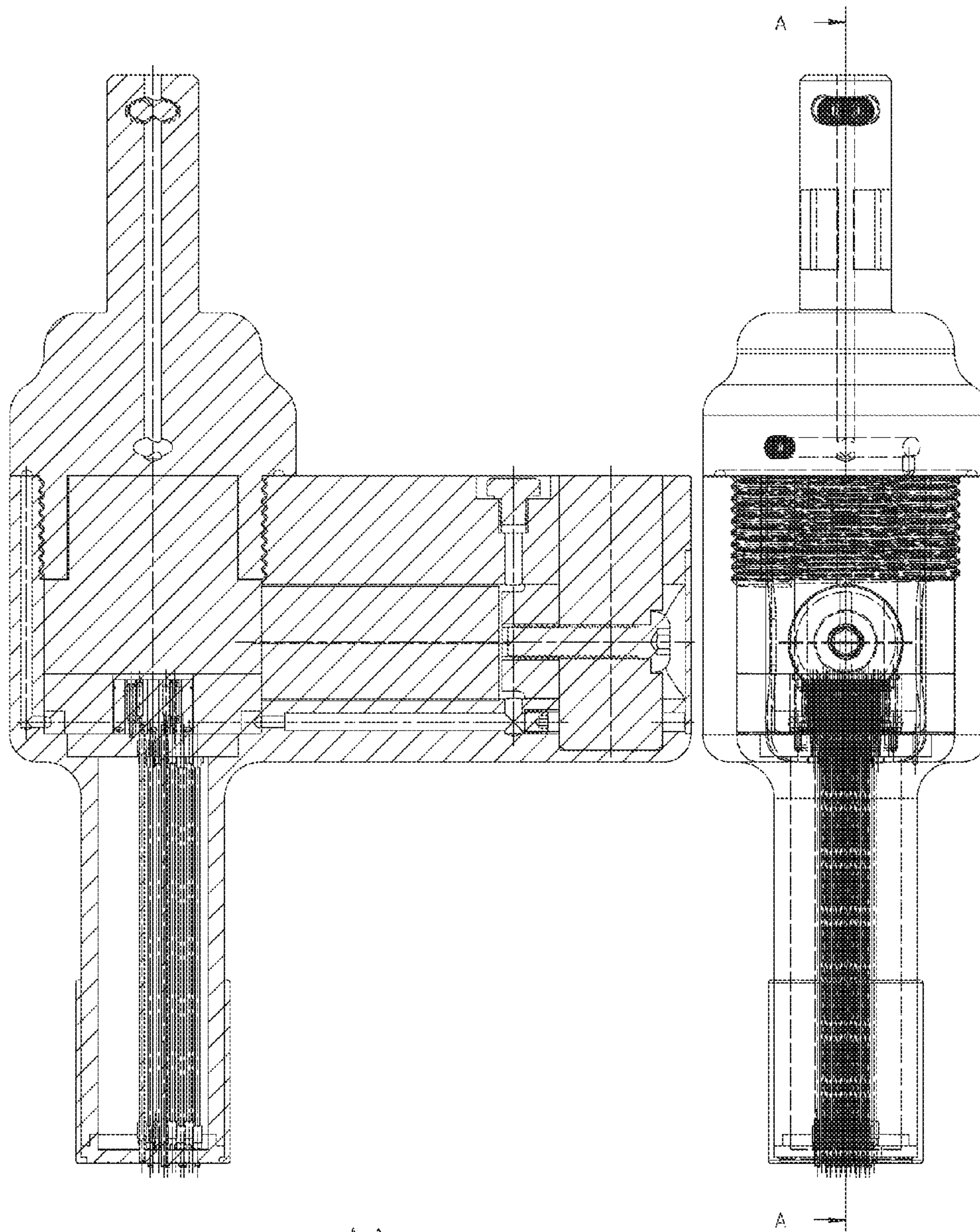
A-A Tool Rotation Programmable 2X11 Detachable Stylus Guide (Arm - Stylus Center Line Section View) Selectable Character Multiple Stylus Orbital Engraving Tool's Typical Components and Assembly
