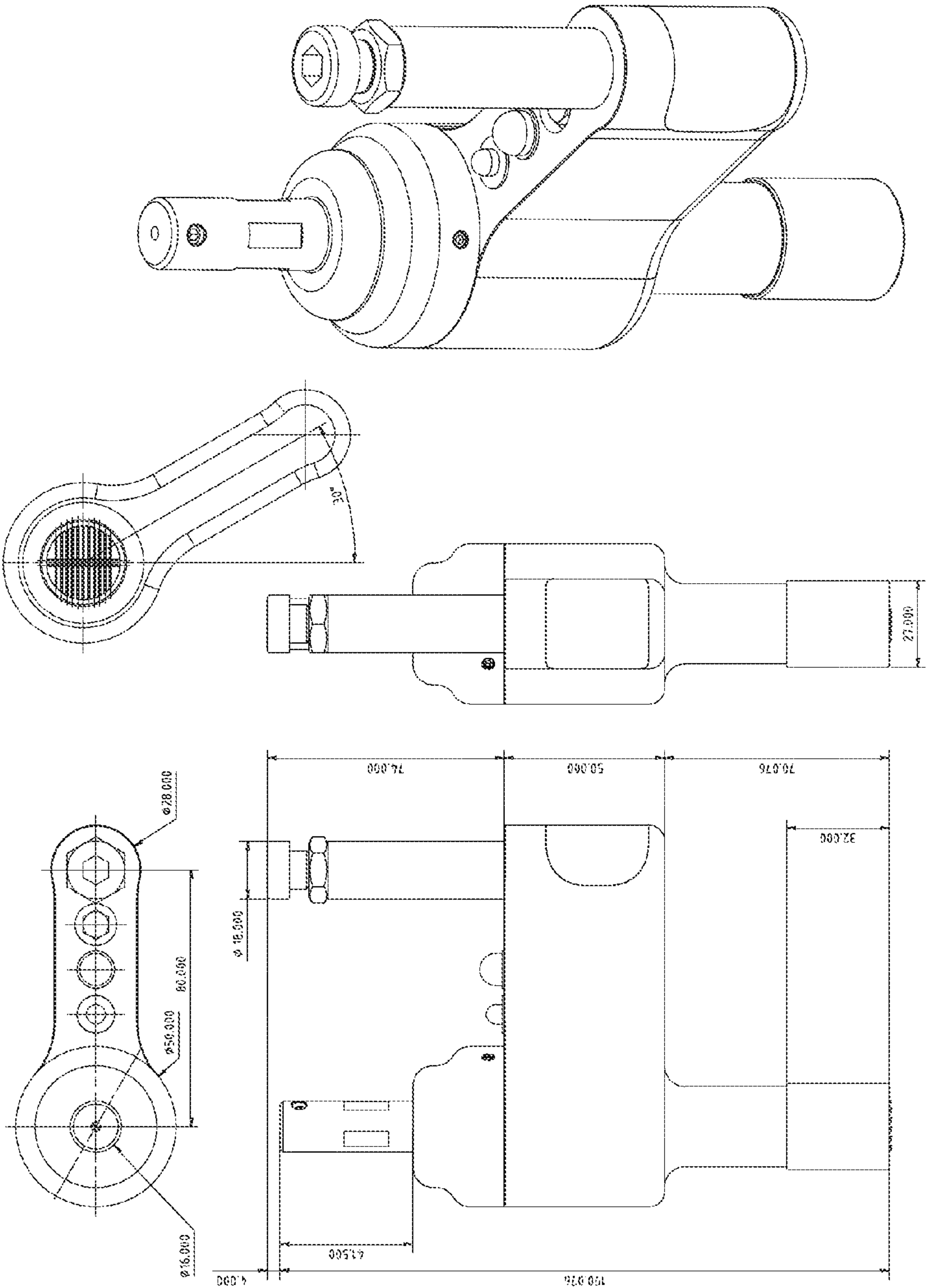
Optical Programmable 2X11 Detachable Stylus Guide (Dimensioned Assembled View) Selectable Character Multiple Stylus Orbital Engraving Tool's Typical Components and Assembly
