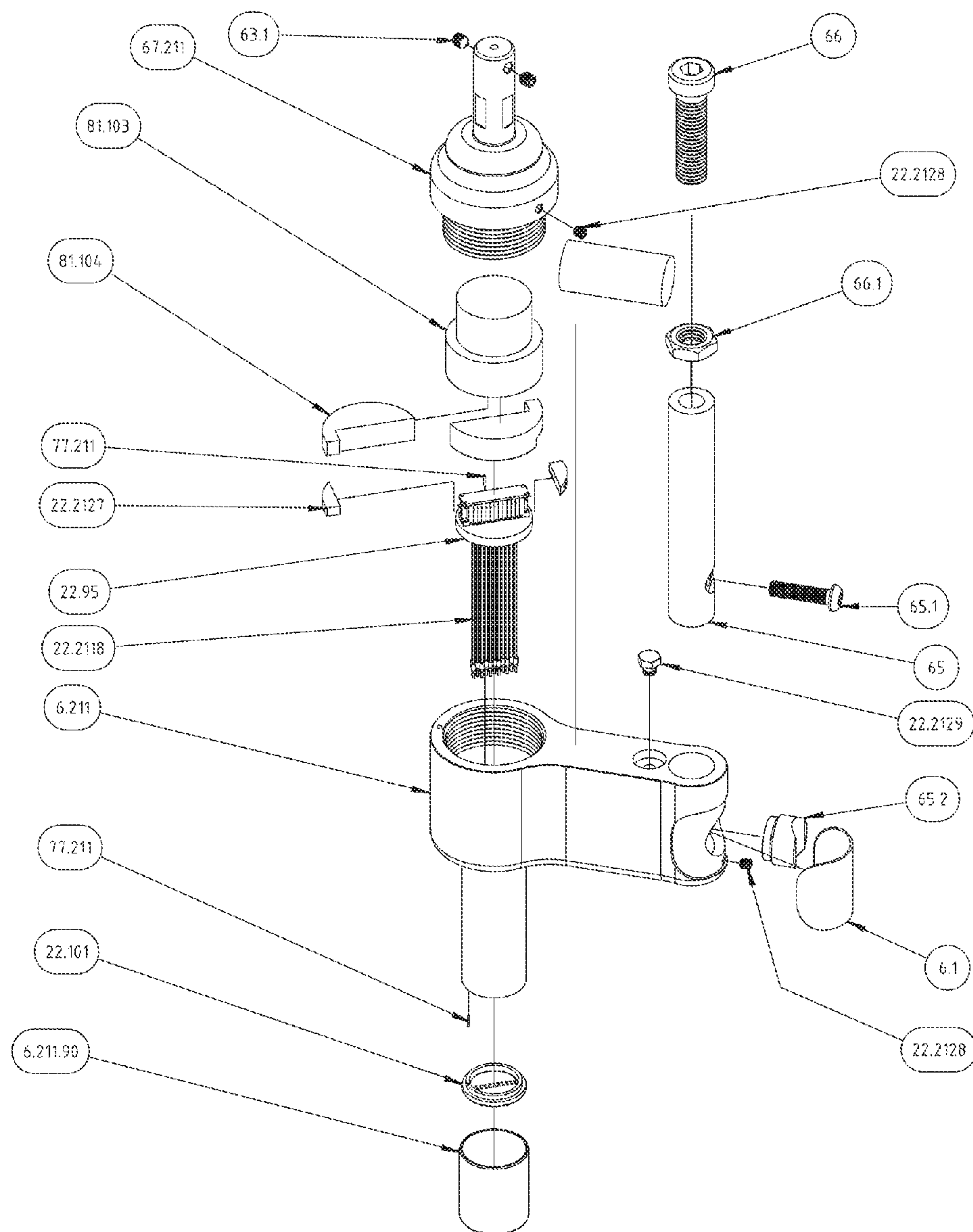
Wireless Programmable 2X11 Detachable Stylus Guide (Exploded Parts View) Selectable Character Multiple Stylus Orbital Engraving Tool's Typical Components and Assembly
