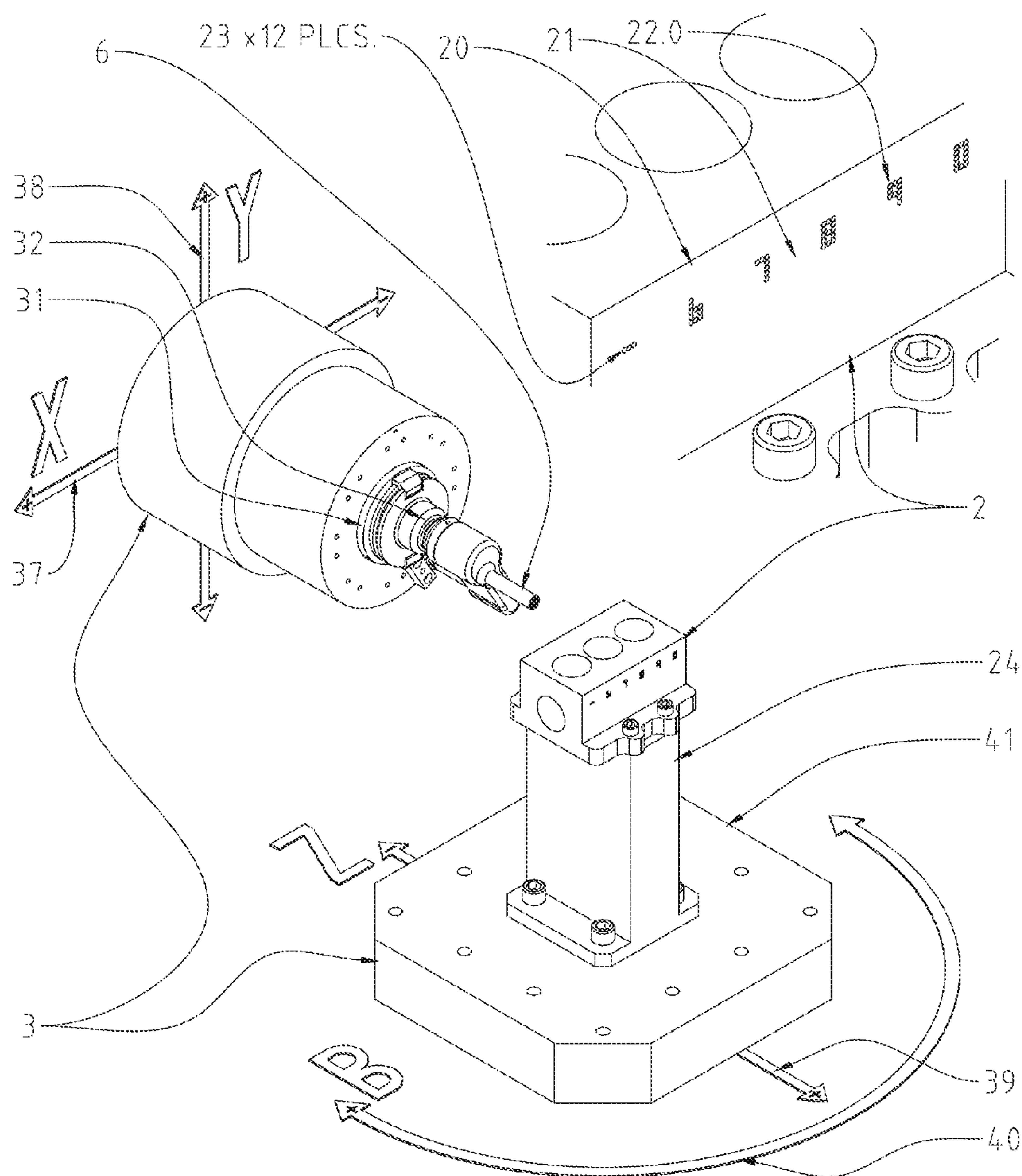
FIGURE 1 (X+ Iso. View) Typical Horizontal Machine Tool for the Selectable Character Multiple Stylus Orbital Engraving Tool
