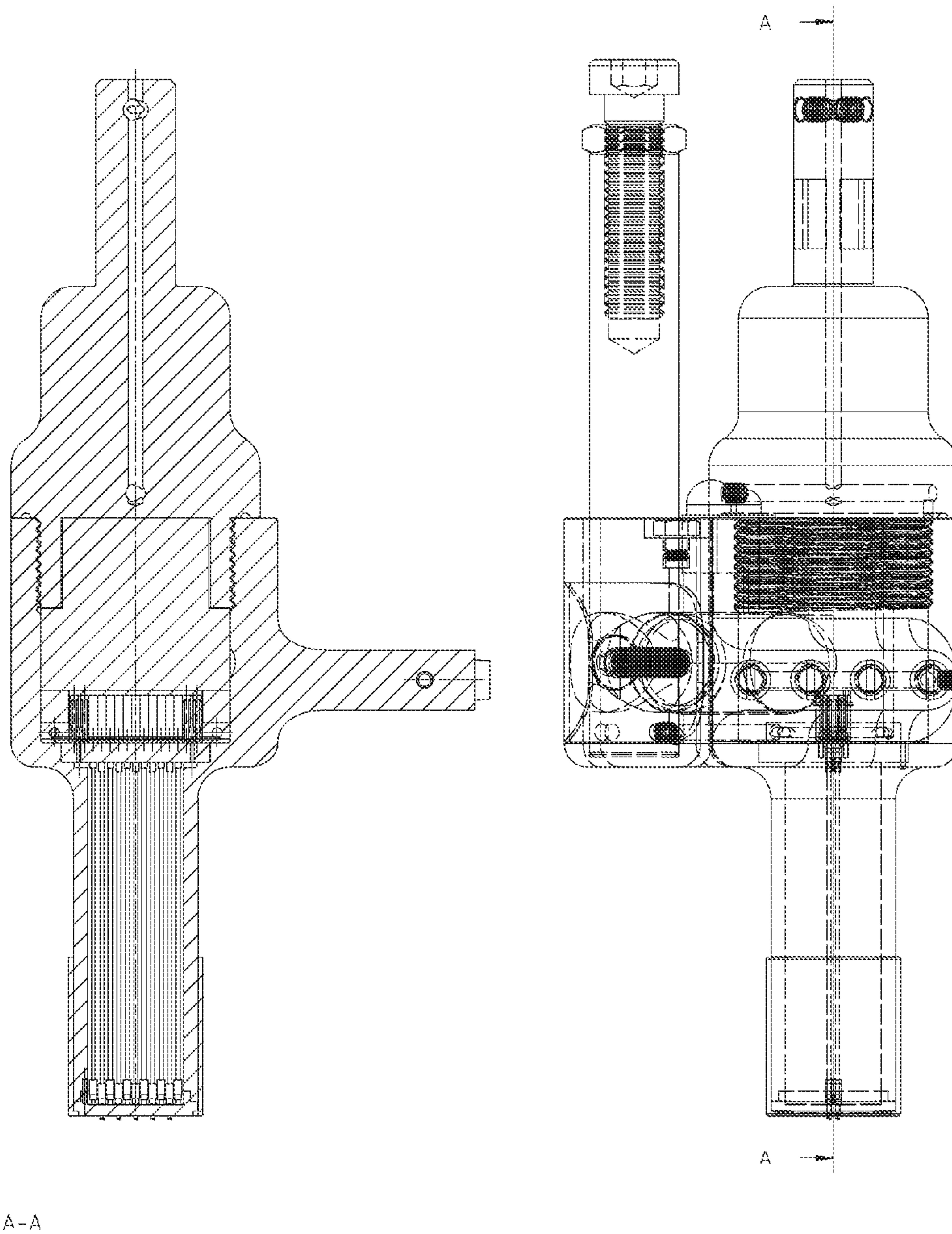
Rechargeable Contact and Optical Programmable 2X33 Detachable Stylus Guide (Horizontal Stylus Center Line Section View) Selectable Character Multiple Stylus Orbital Engraving Tool's Typical Components and Assembly
