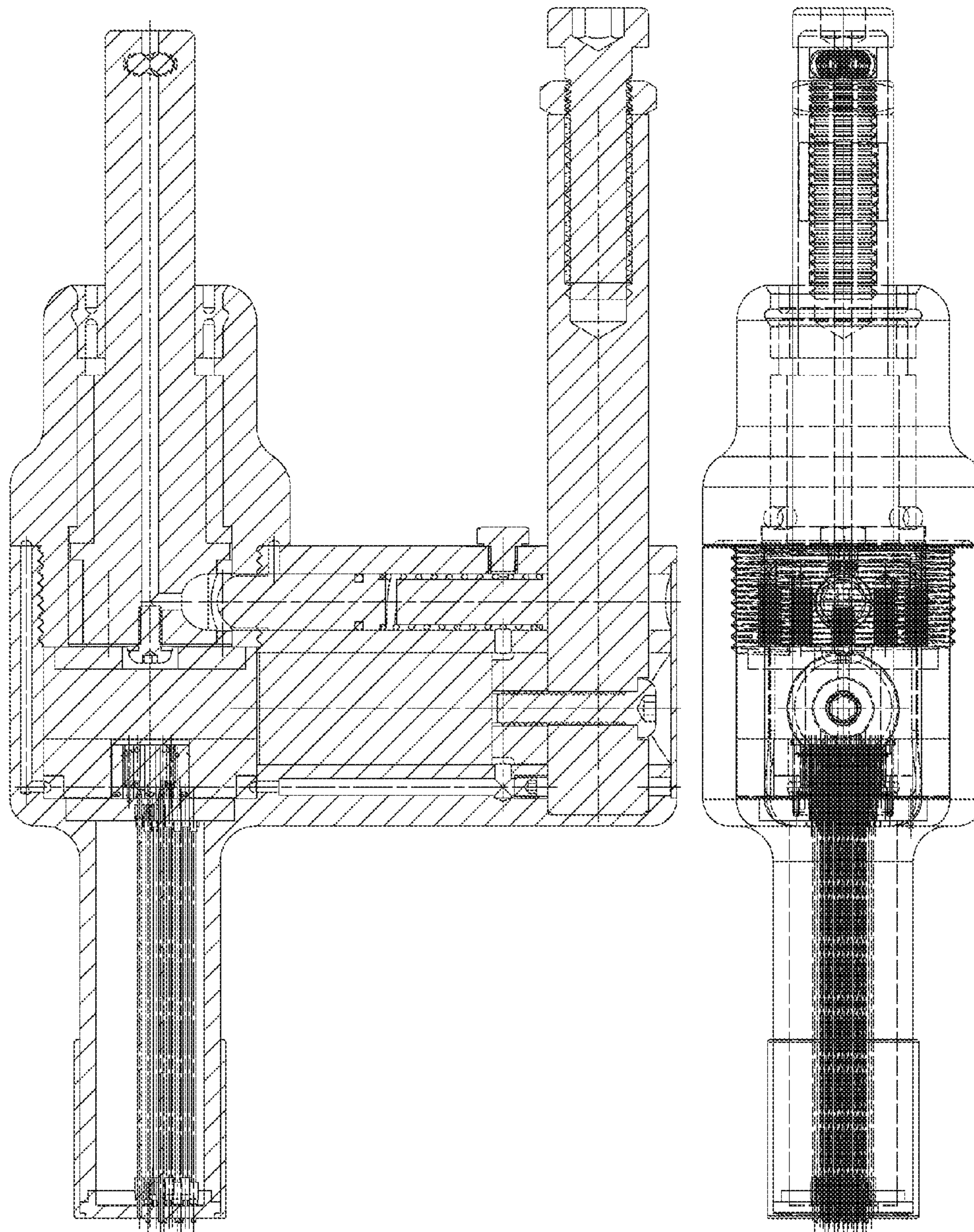
Spindle Rotation Programmable 2X11 Detachable Stylus Guide (Arm - Stylus Center Line Section View) Selectable Character Multiple Stylus Orbital Engraving Tool's Typical Components and Assembly
