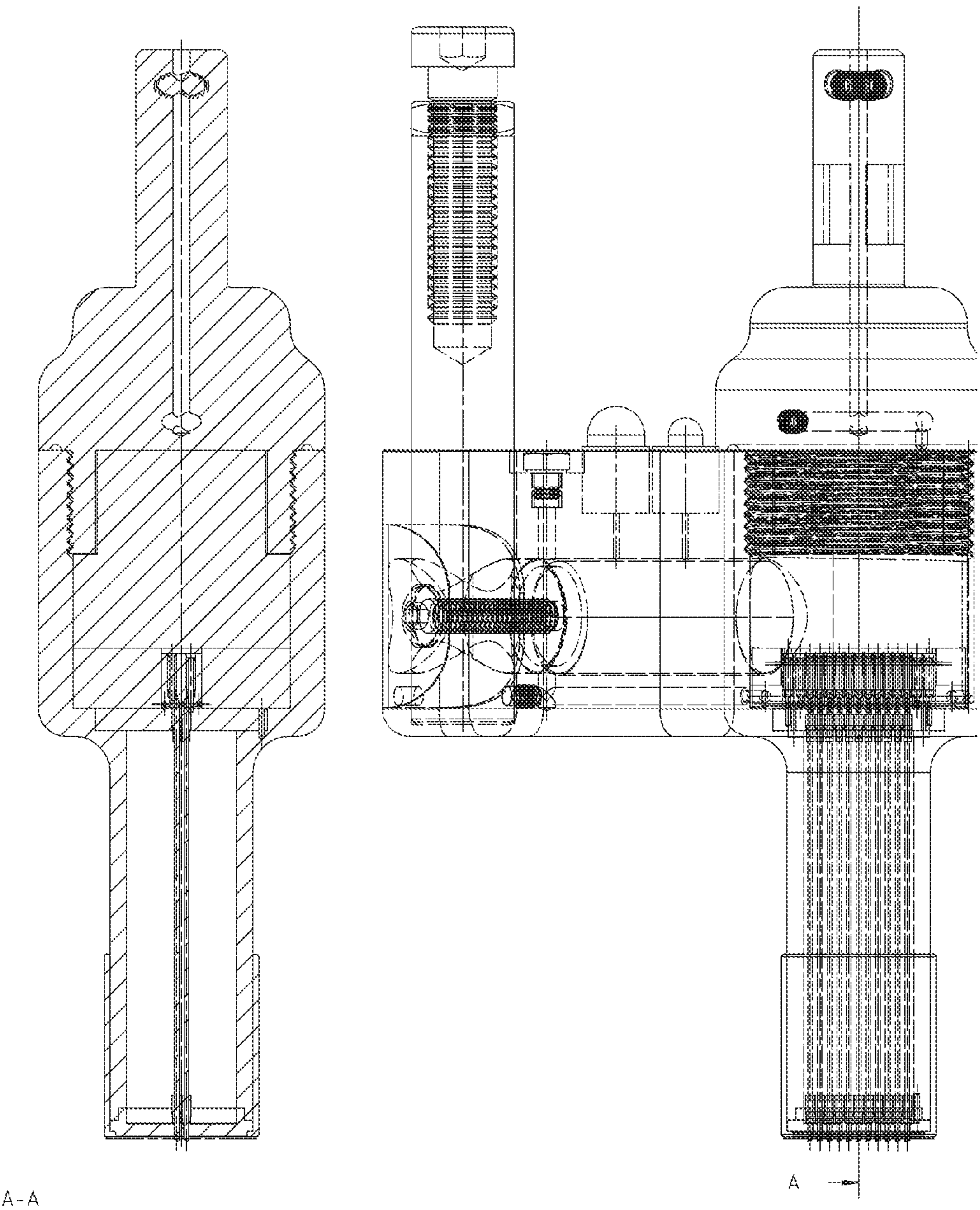
Optical Programmable 2X11 Detachable Stylus Guide (Vertical Stylus Center Line Section View) Selectable Character Multiple Stylus Orbital Engraving Tool's Typical Components and Assembly
