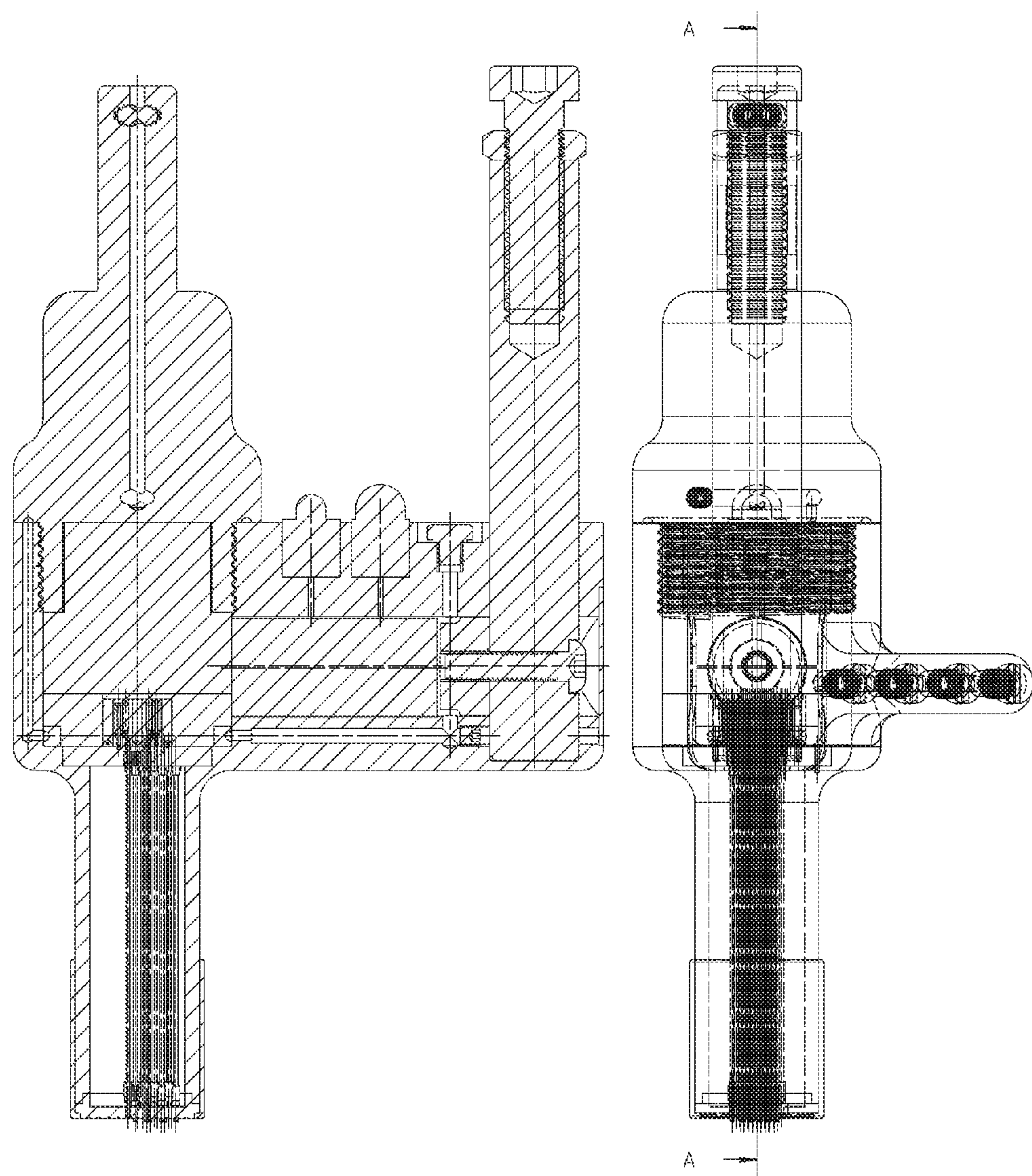
A-A Rechargeable Contact and Optical Programmable 2X11 Detachable Stylus Guide (Arm - Stylus Center Line Section View) Selectable Character Multiple Stylus Orbital Engraving Tool's Typical Components and Assembly
