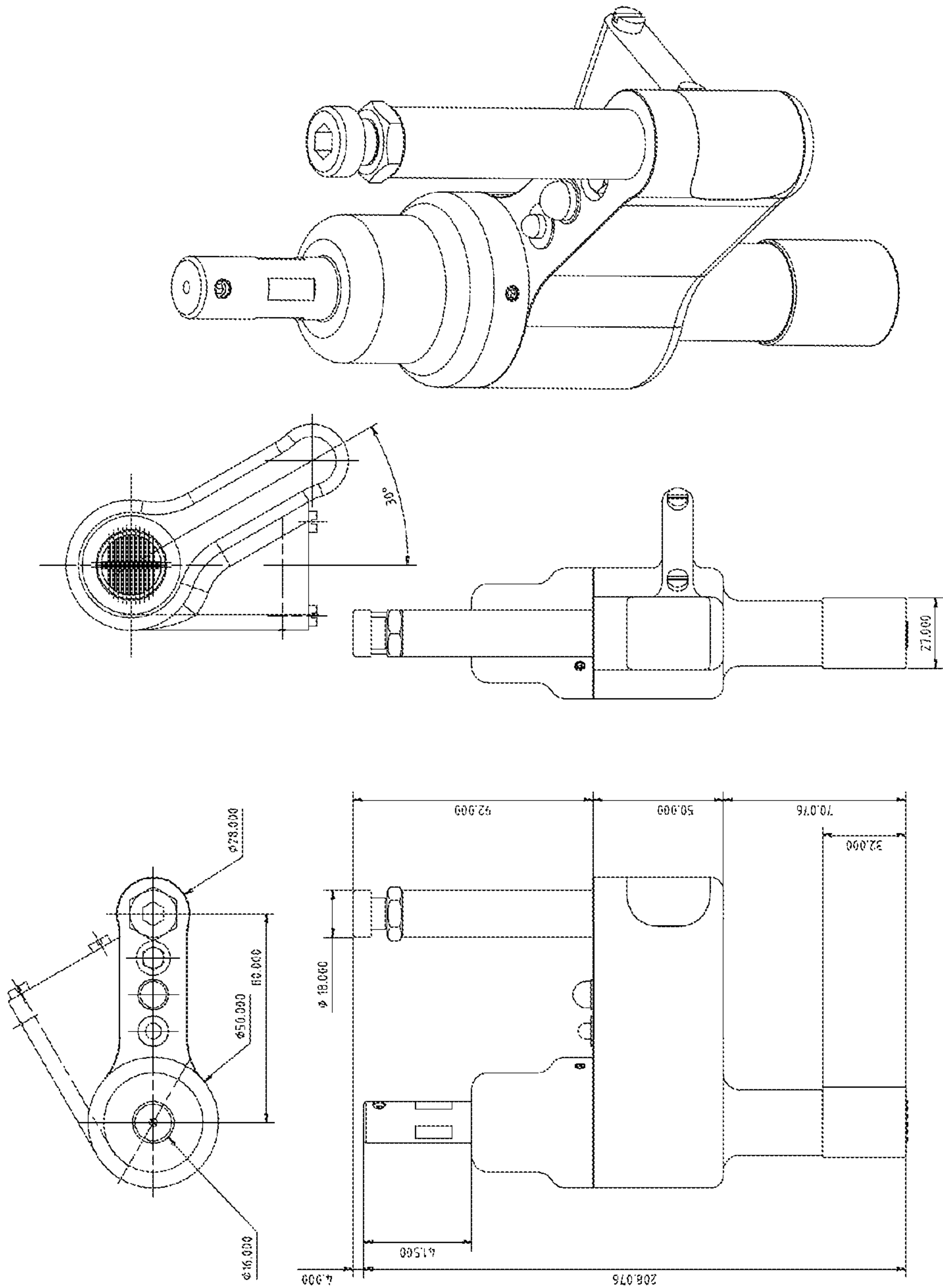
Rechargeable Optical Programmable 2X11 Detachable Stylus Guide (Dimensioned Assembled View) Selectable Character Multiple Stylus Orbital Engraving Tool's Typical Components and Assembly
