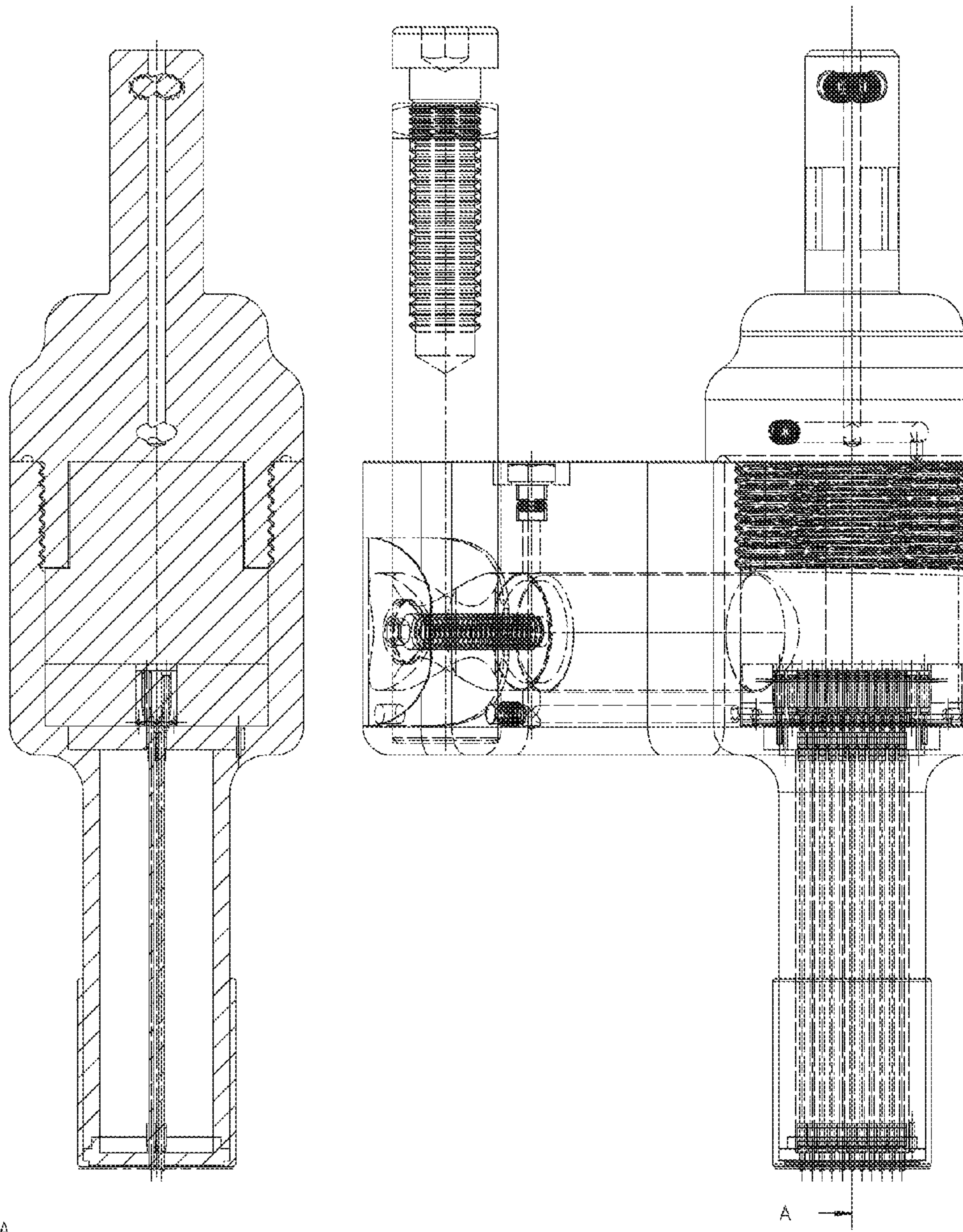
Wireless Programmable 2X11 Detachable Stylus Guide (Vertical Stylus Center Line Section View) Selectable Character Multiple Stylus Orbital Engraving Tool's Typical Components and Assembly
