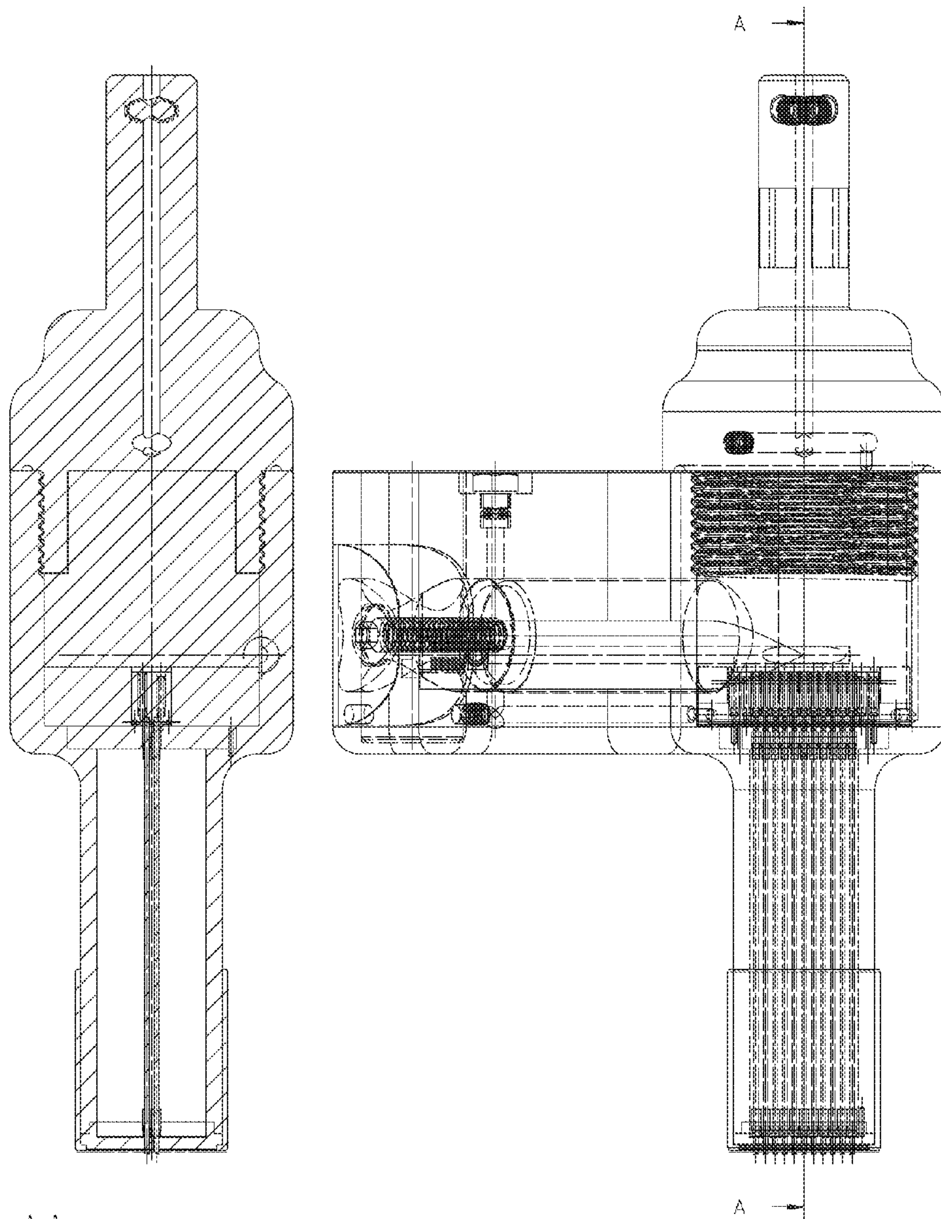
A--A Rechargeable Tool Rotational Programmable 2X11 Detachable Stylus Guide (Vertical Stylus Center Line Section View) Selectable Character Multiple Stylus Orbital Engraving Tool's Typical Components and Assembly
