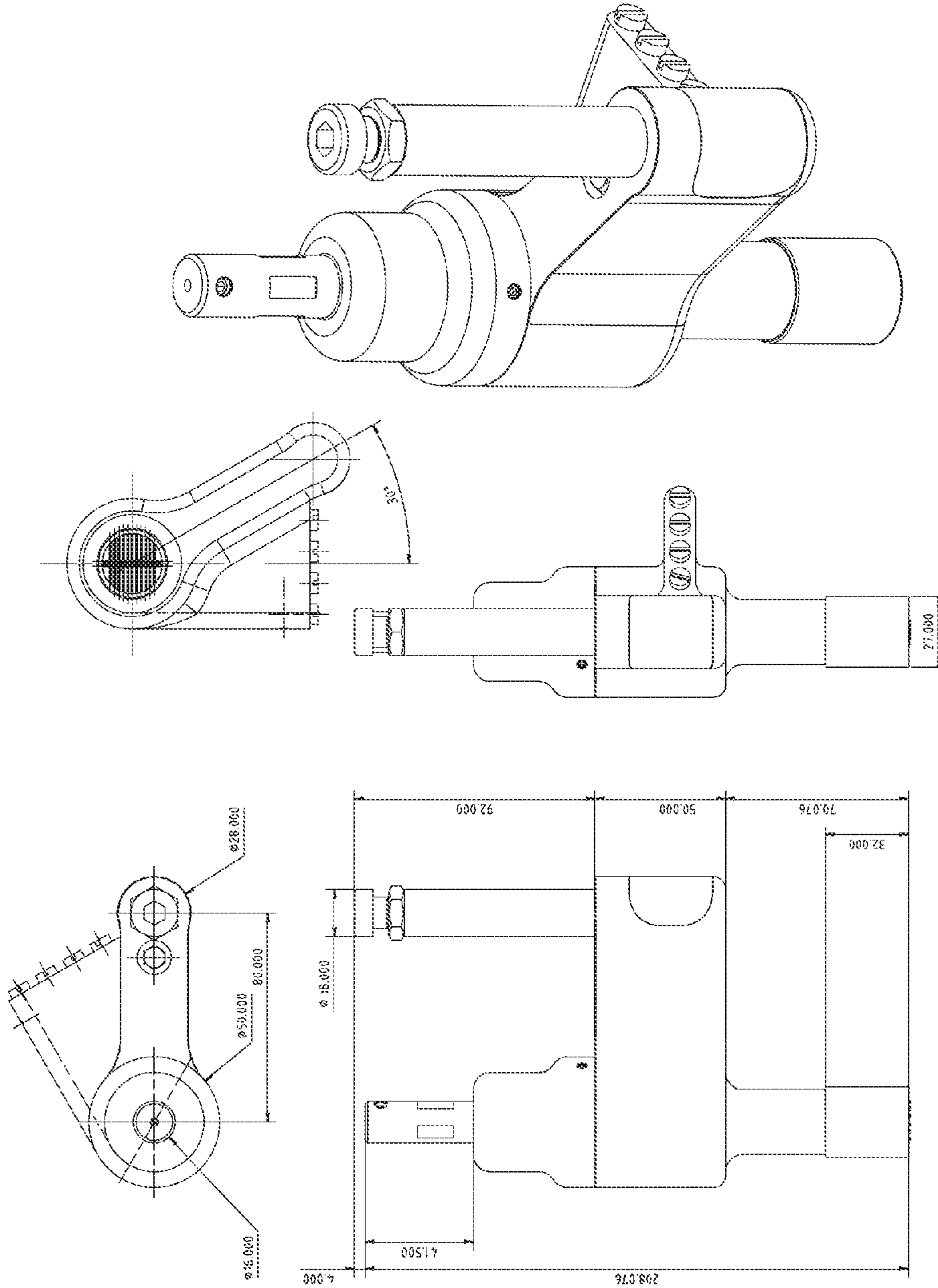
Rechargeable Contact and Wireless Programmable 2X11 Detachable Stylus Guide (Dimensioned Assembled View) Selectable Character Multiple Stylus (Orbital Engraving Tool's Typical Components and Assembly
