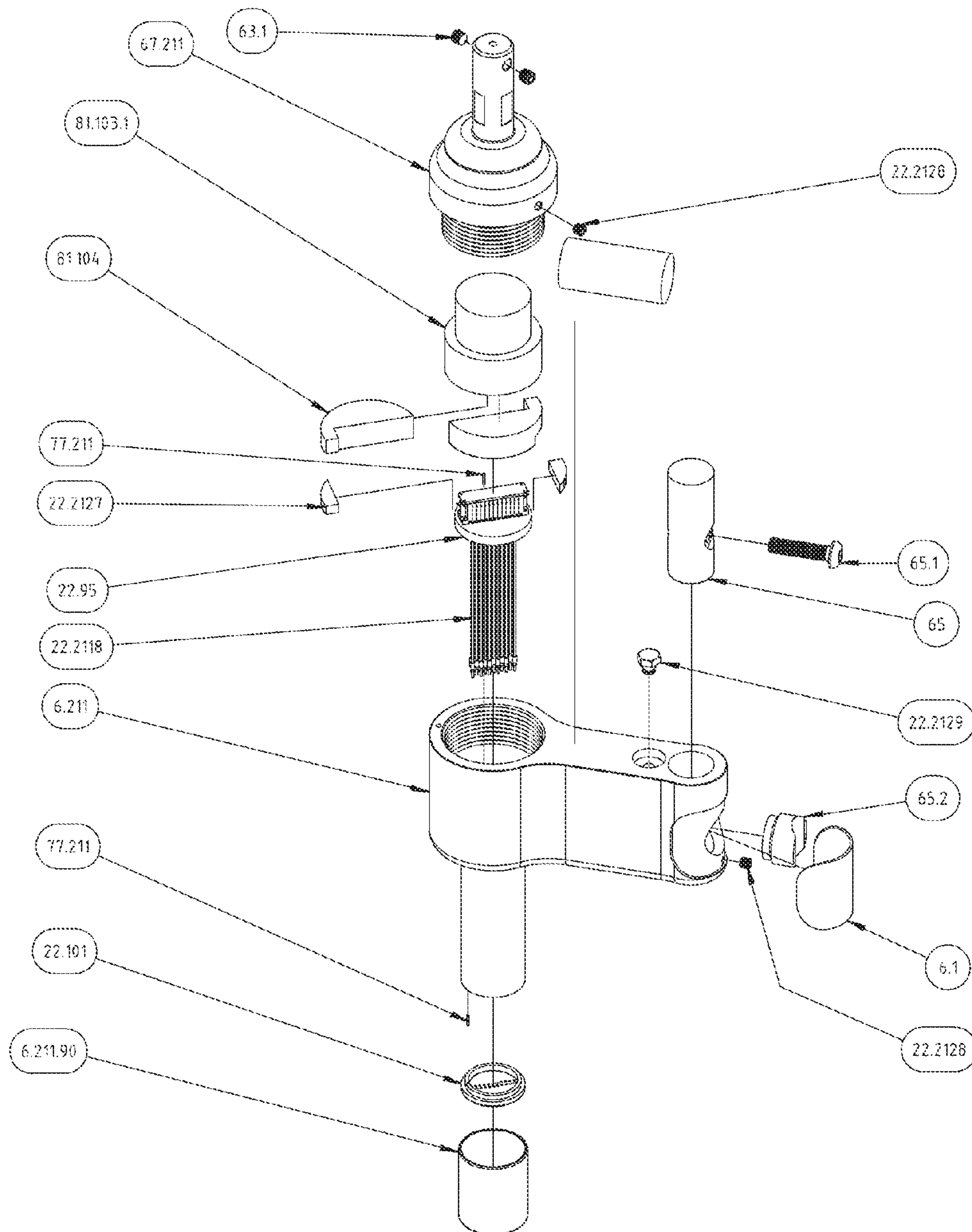
Tool Rotation Programmable 2X11 Detachable Stylus Guide (Exploded Parts View) Selectable Character Multiple Stylus Orbital Engraving Tool's Typical Components and Assembly
