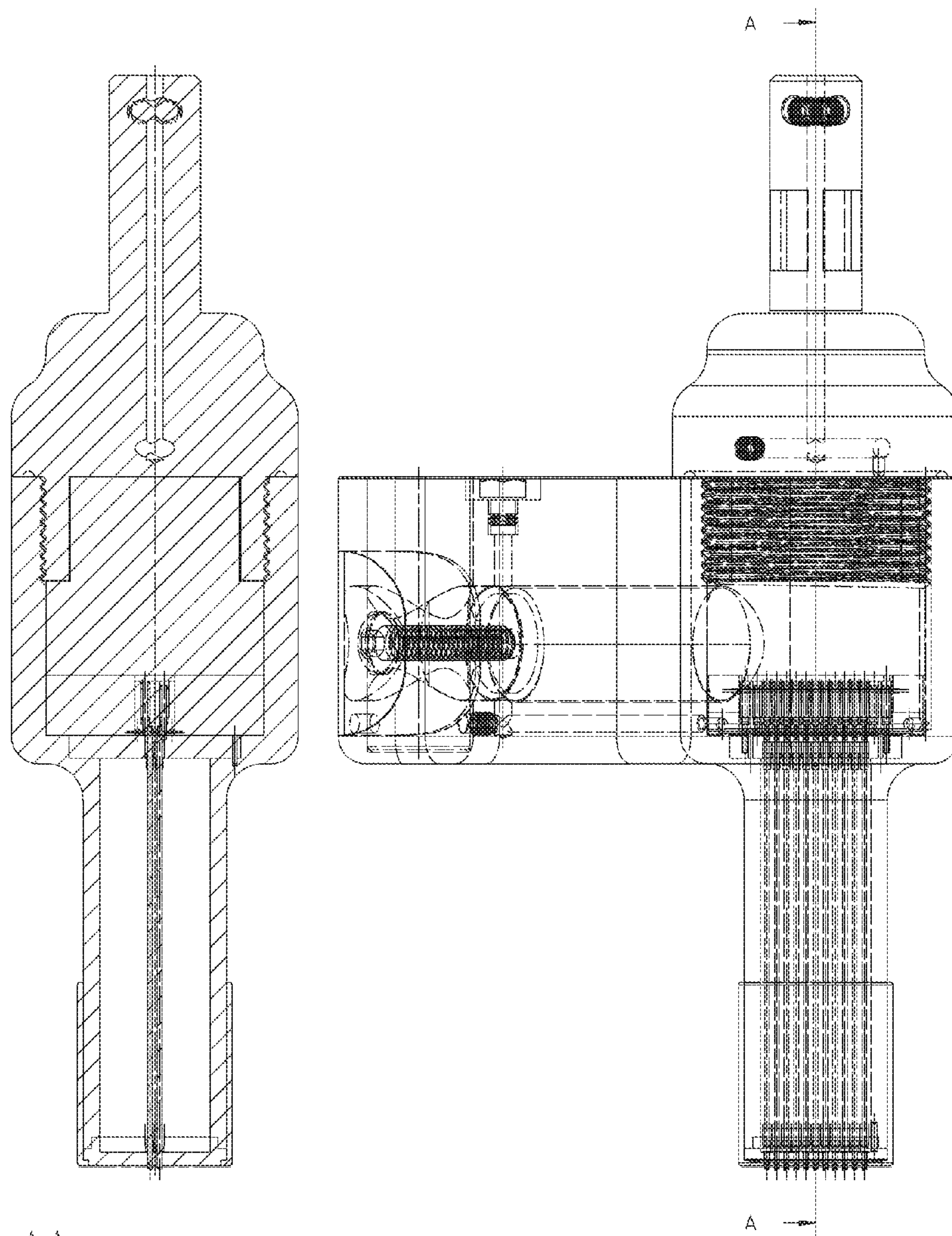
A-A Tool Rotation Programmable 2X11 Detachable Stylus Guide (Vertical Stylus Center Line Section View) Selectable Character Multiple Stylus Orbital Engraving Tool's Typical Components and Assembly
