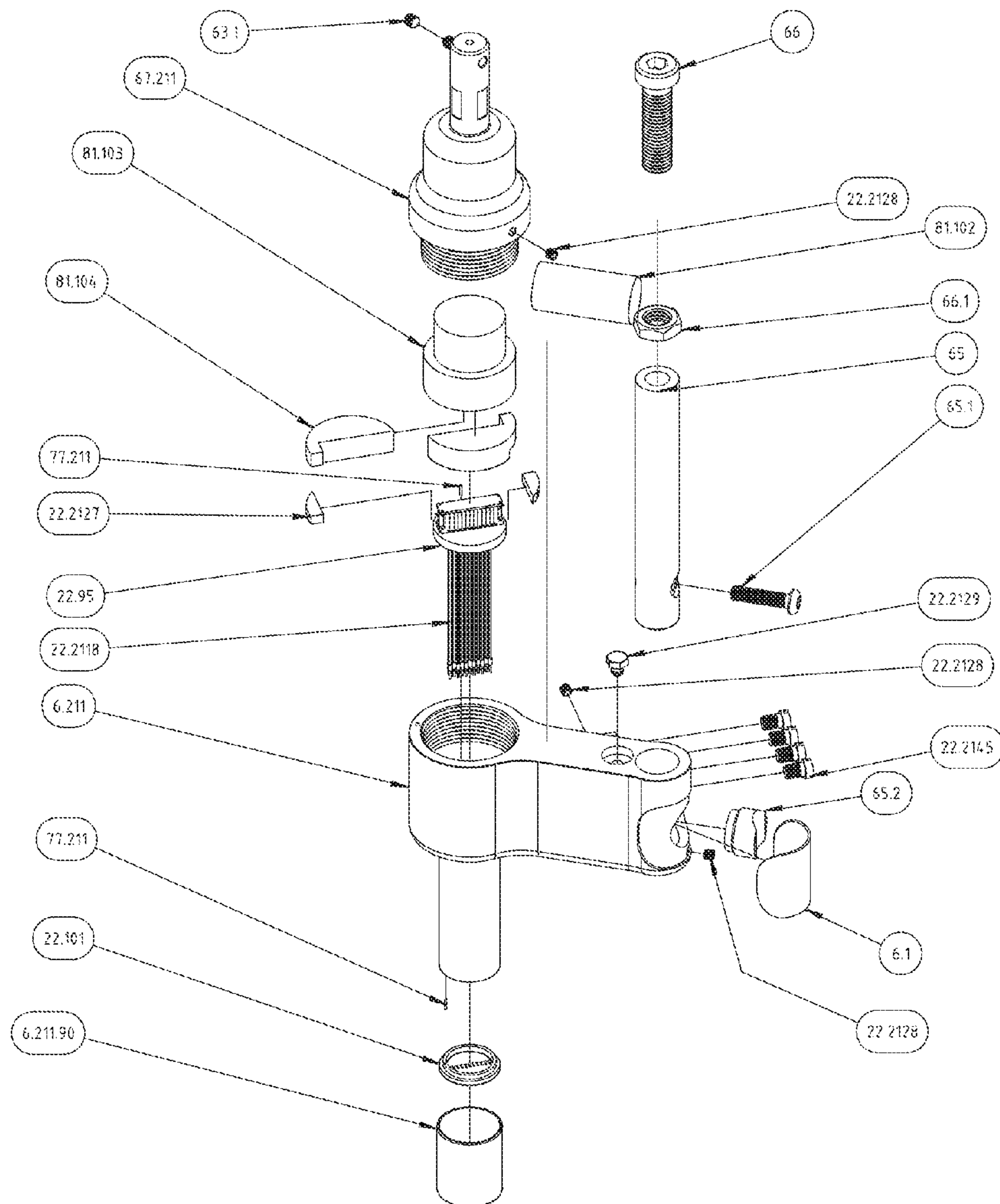
Rechargeable Contact and Wireless Programmable 2X11 Detachable Stylus Guide (Exploded Parts View) Selectable Character Multiple Stylus Orbital Engraving Tool's Typical Components and Assembly
