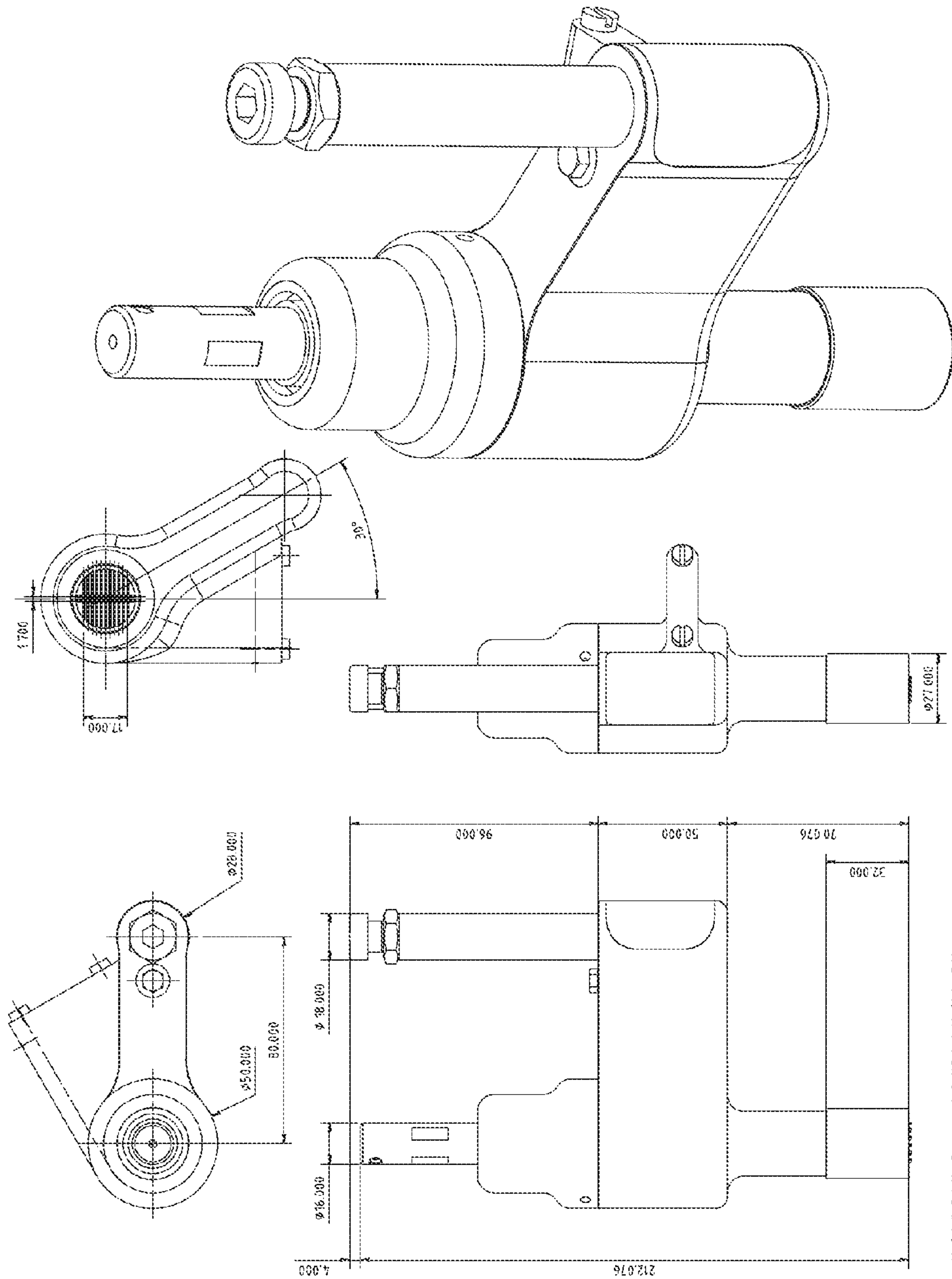
Rechargeable Stylus Rotated Programmable ZAM Detachable Stylus Guide Dimensions Assembled View Selectable Character Multiple Stylus Orbital Engraving Tool's Typical Components and Assembly
