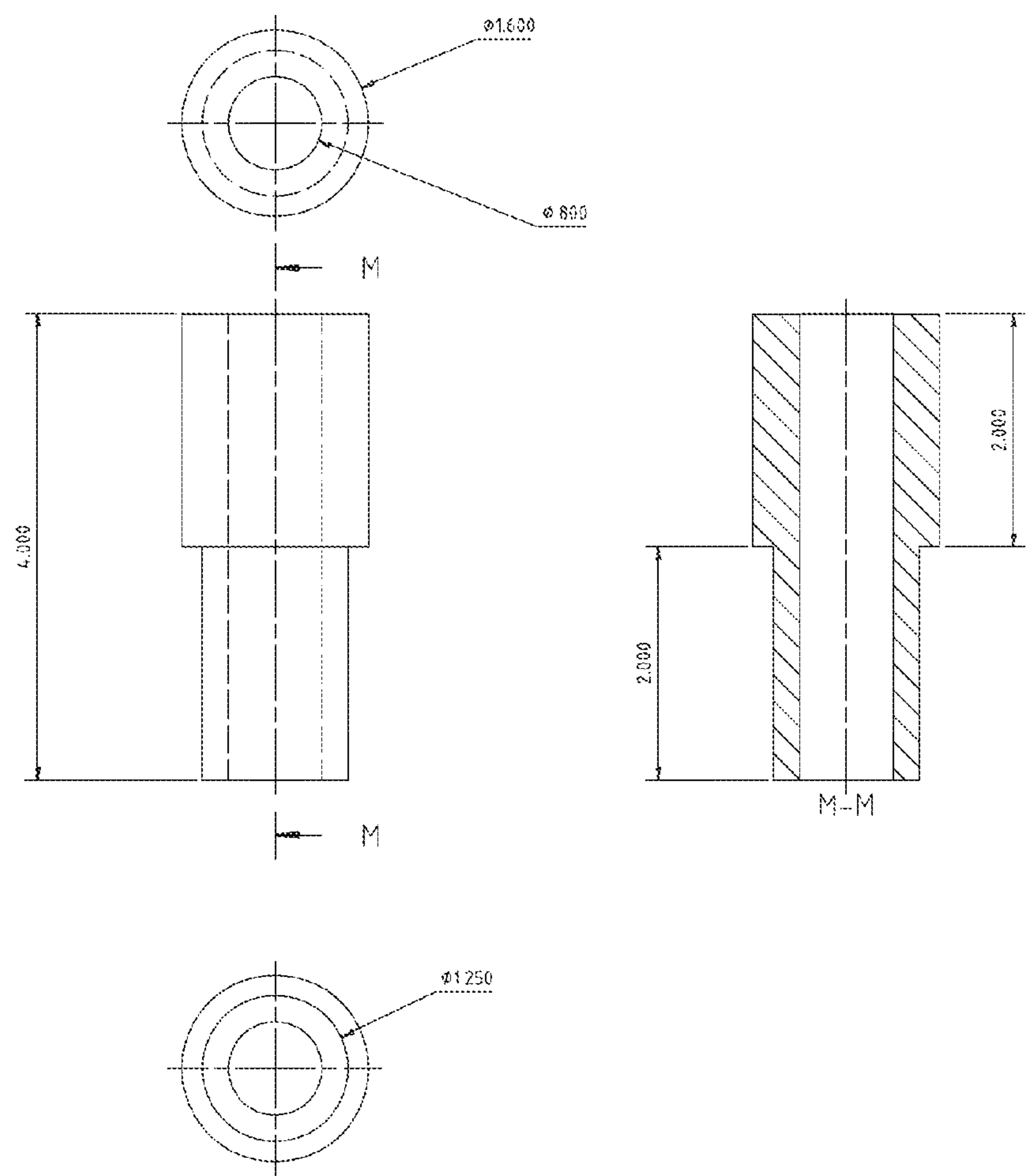
Part-78 Stylus Pneumatic Retraction Collar Component for the Selectable Character Multiple Stylus Orbital Engraving Tool
