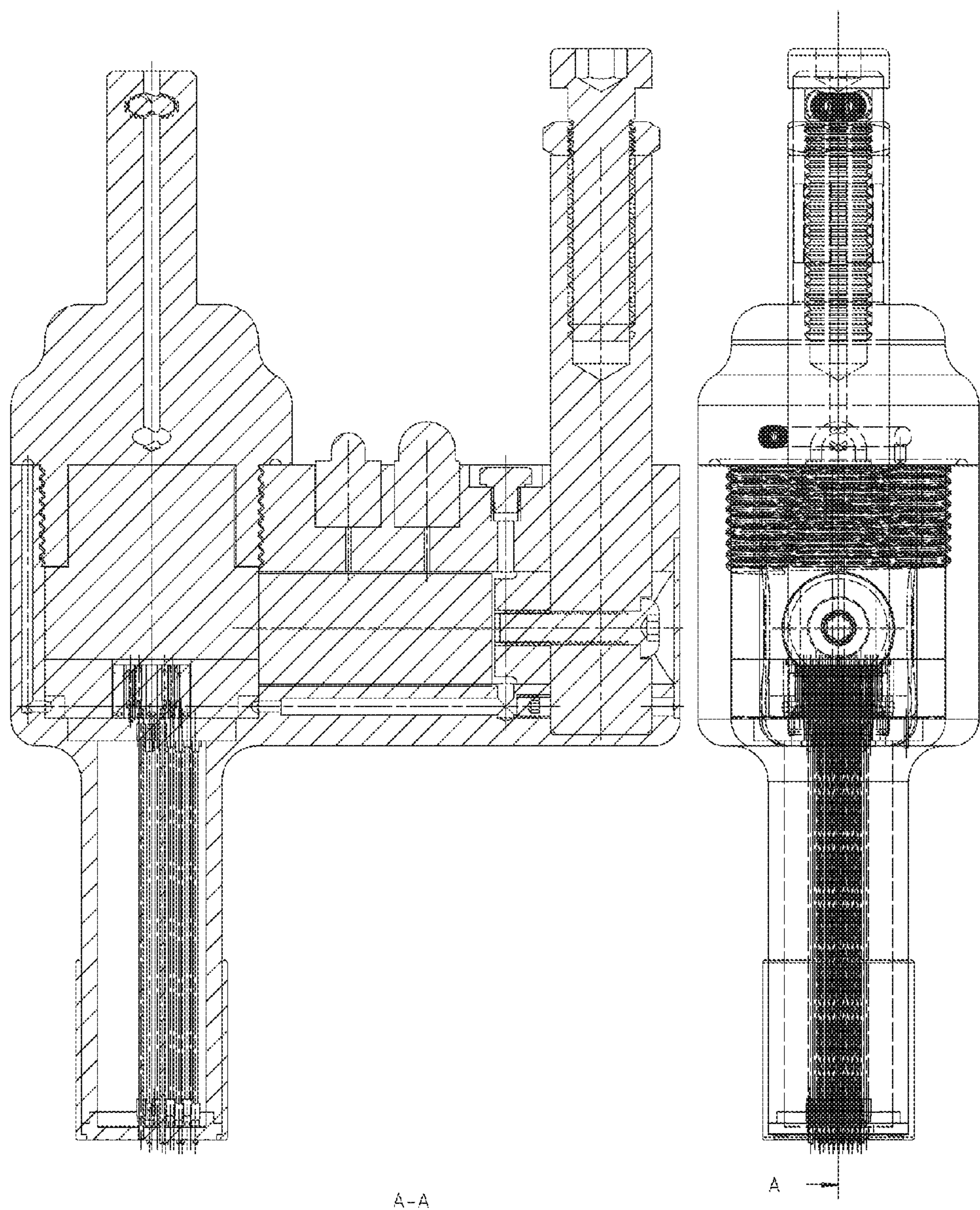
Optical Programmable ZX13 Detachable Stylus Guide (Arm - Stylus Center Line Section View) Selectable Character Multiple Stylus Orbital Engraving Tool's Typical Components and Assembly
