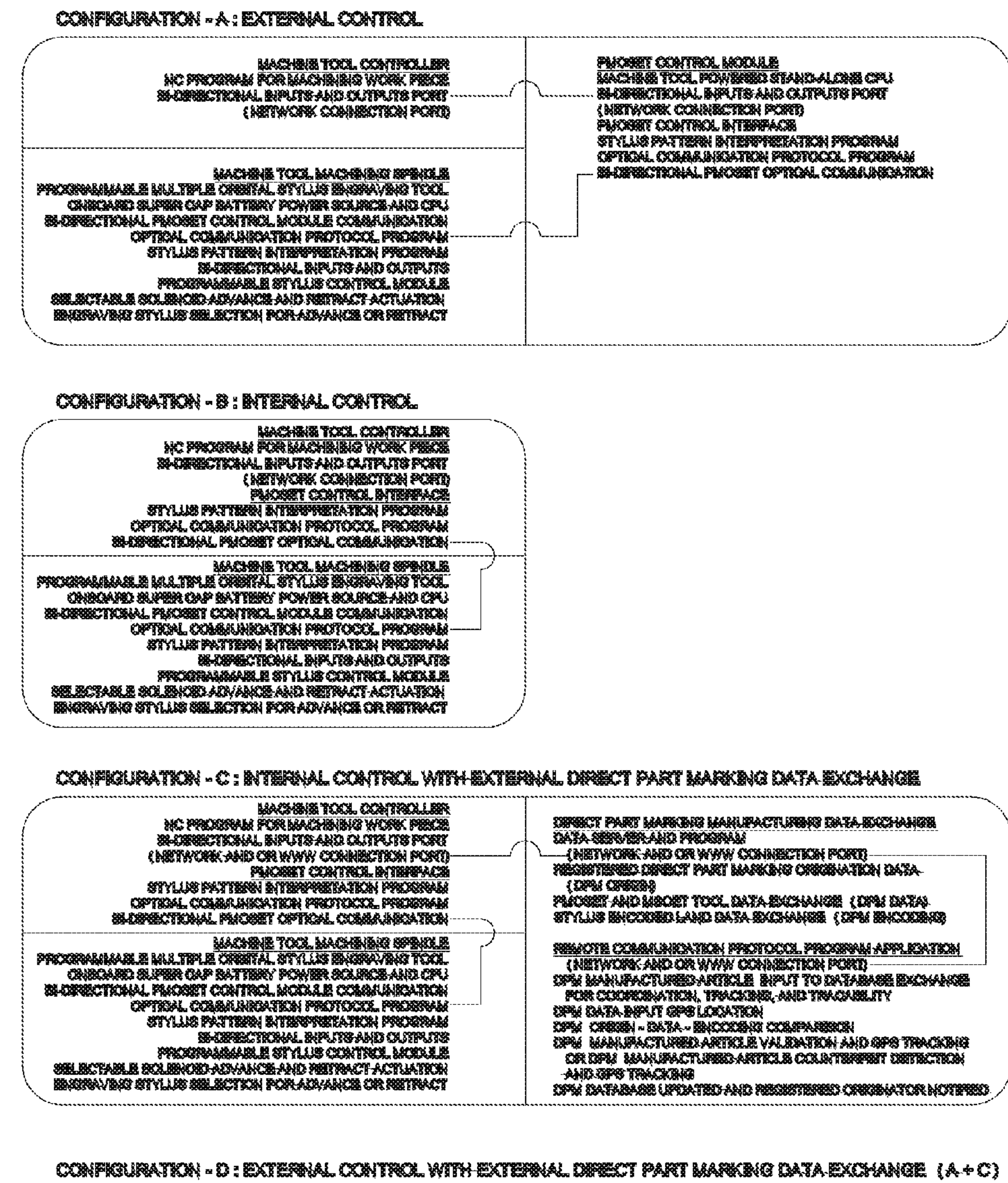
DIRECT PART MARKING OPTIC CONTROL MODULE AND DATA EXCHANGE SCHEMAS PROGRAMMABLE OR SELECTABLE MULTIPLE ORBITAL STYLUS ENGRAVING TOOL (PMOSSET) OR (MROSET) CONTROLS AND DATA EXCHANGE SCHEMAS FOR THE STRAIGHT OR ENCODED LAND, SINGLE OR MULTI FLUTE STYLUS Figure-62
