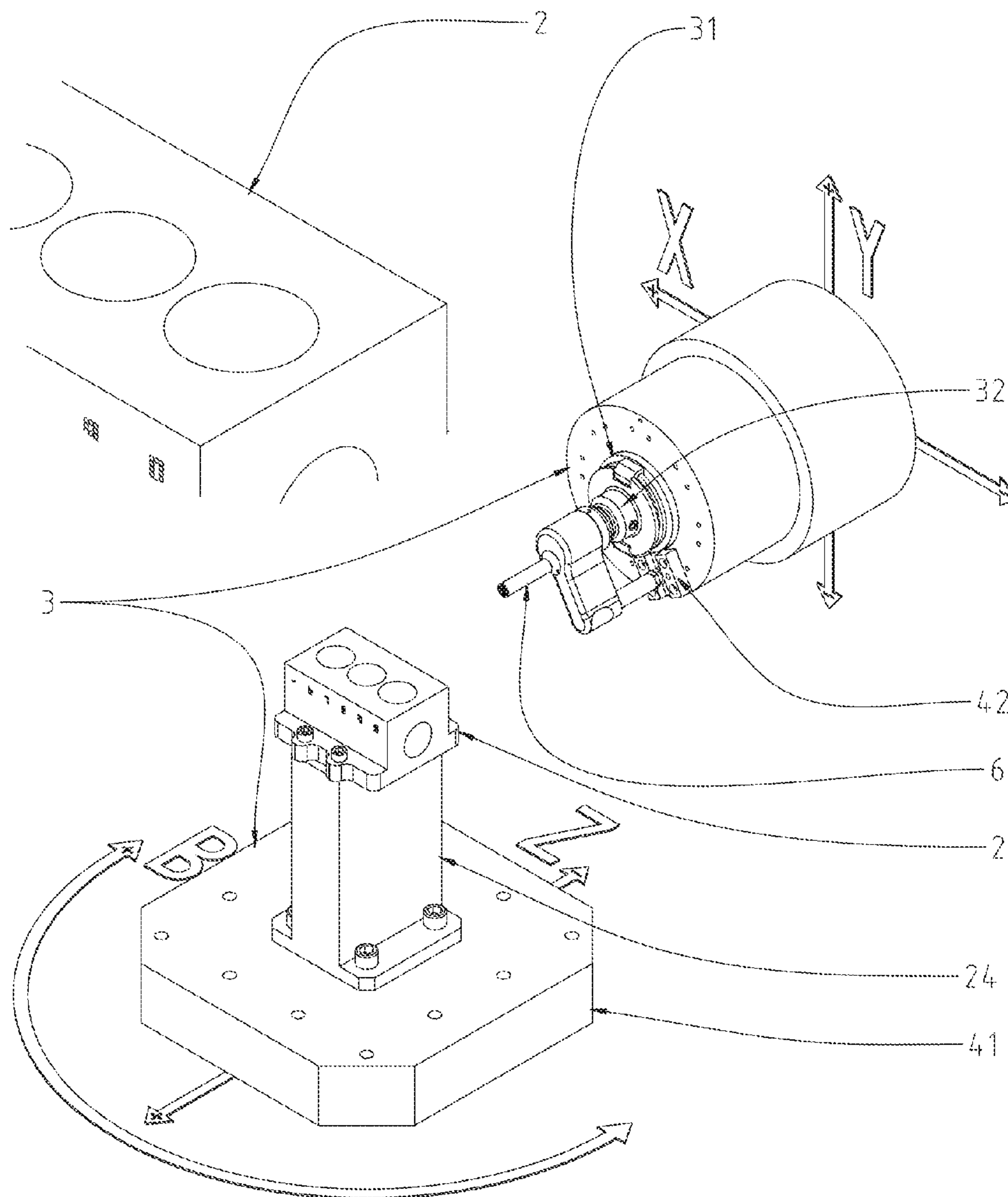
FIGURE 2 (X- Iso. View) Typical Horizontal Machine Tool for the Selectable Character Multiple Stylus Orbital Engraving Tool
