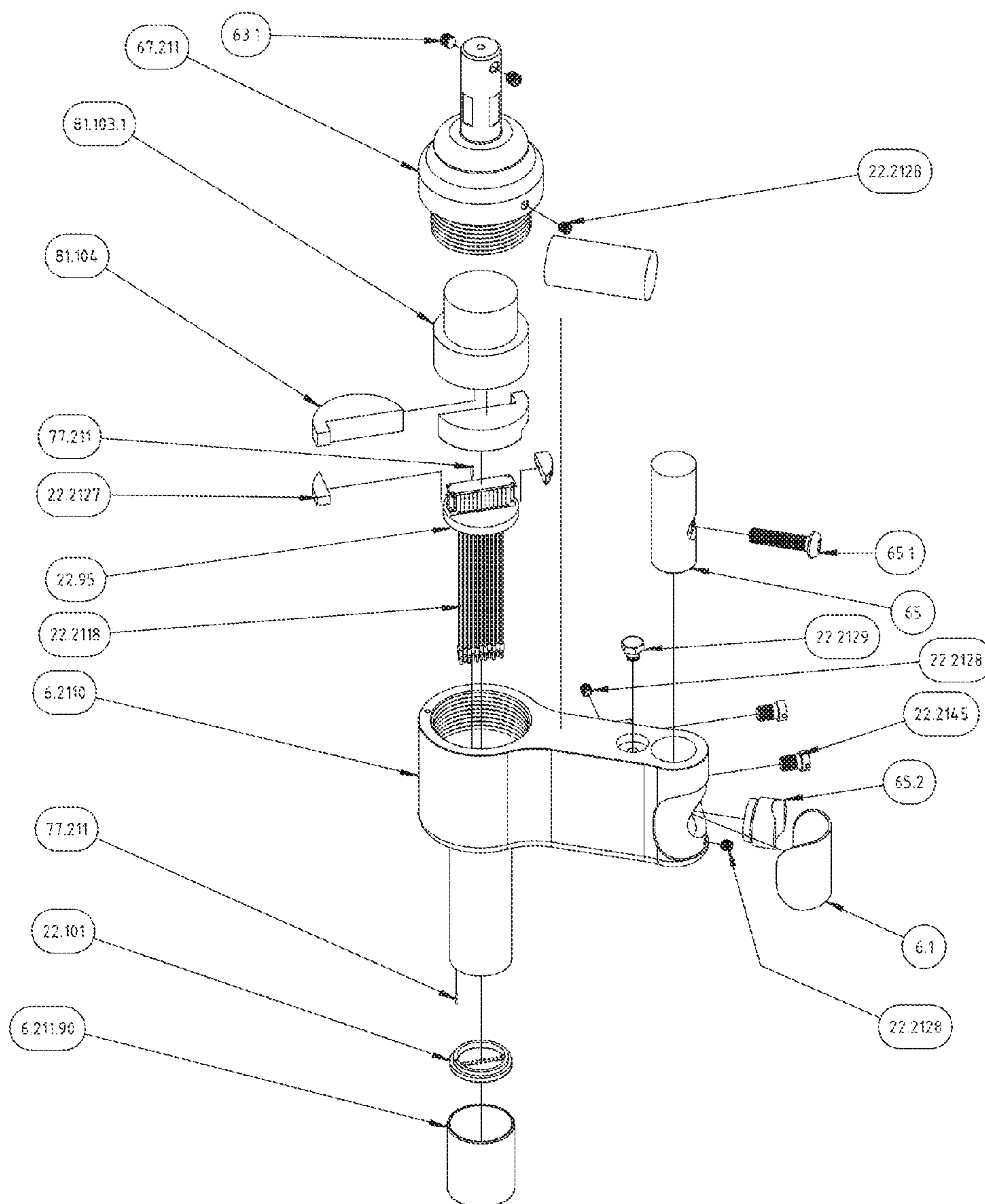
Rechargeable Tool Rotational Programmable 2X11 Detachable Stylus Guide (Exploded Parts View) Selectable Character Multiple Stylus Orbital Engraving Tool's Typical Components and Assembly Figure-140
