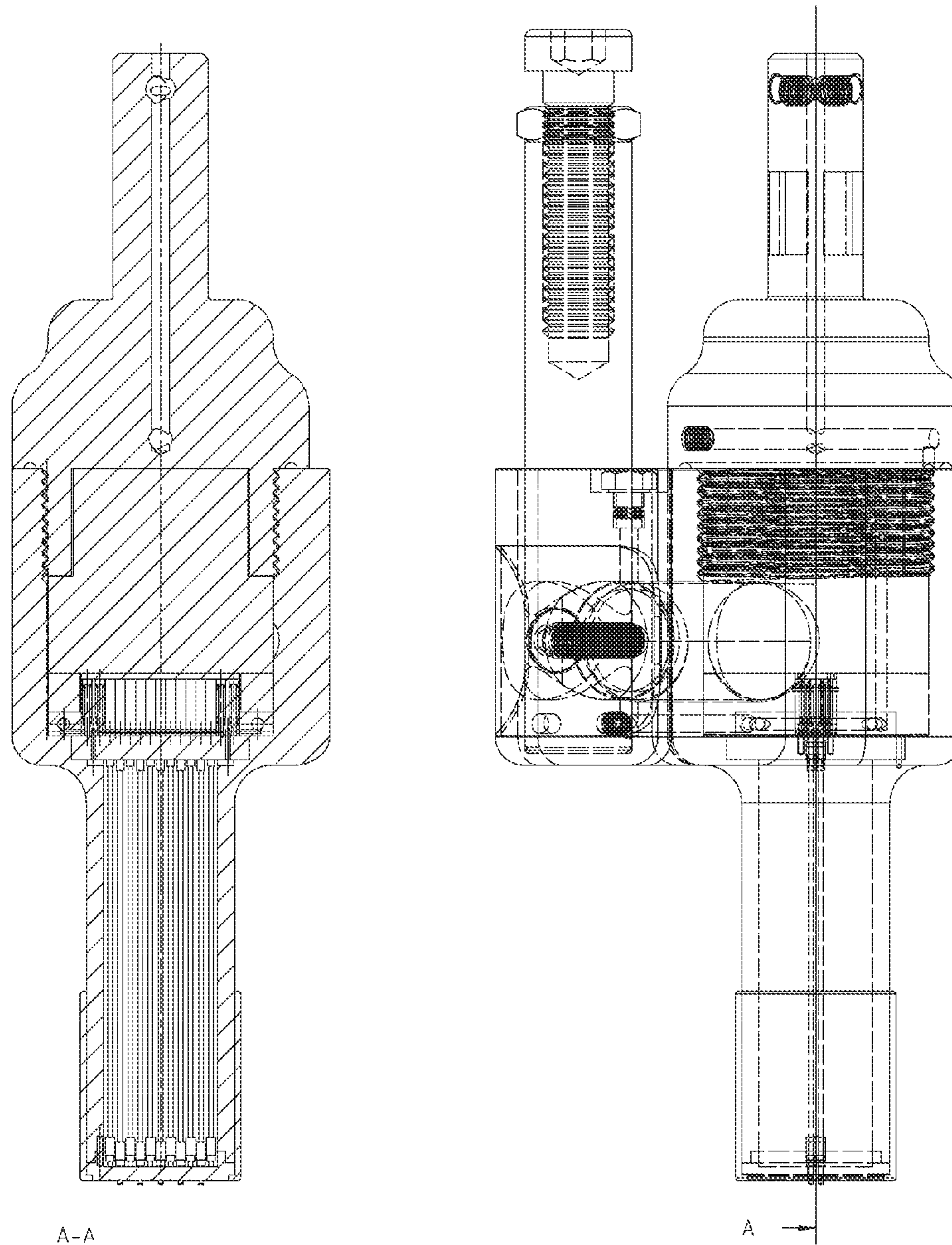
Wireless Programmable 2X11 Detachable Stylus Guide (Horizontal Stylus Center Line Section View) Selectable Character Multiple Stylus Orbital Engraving Tool's Typical Components and Assembly
