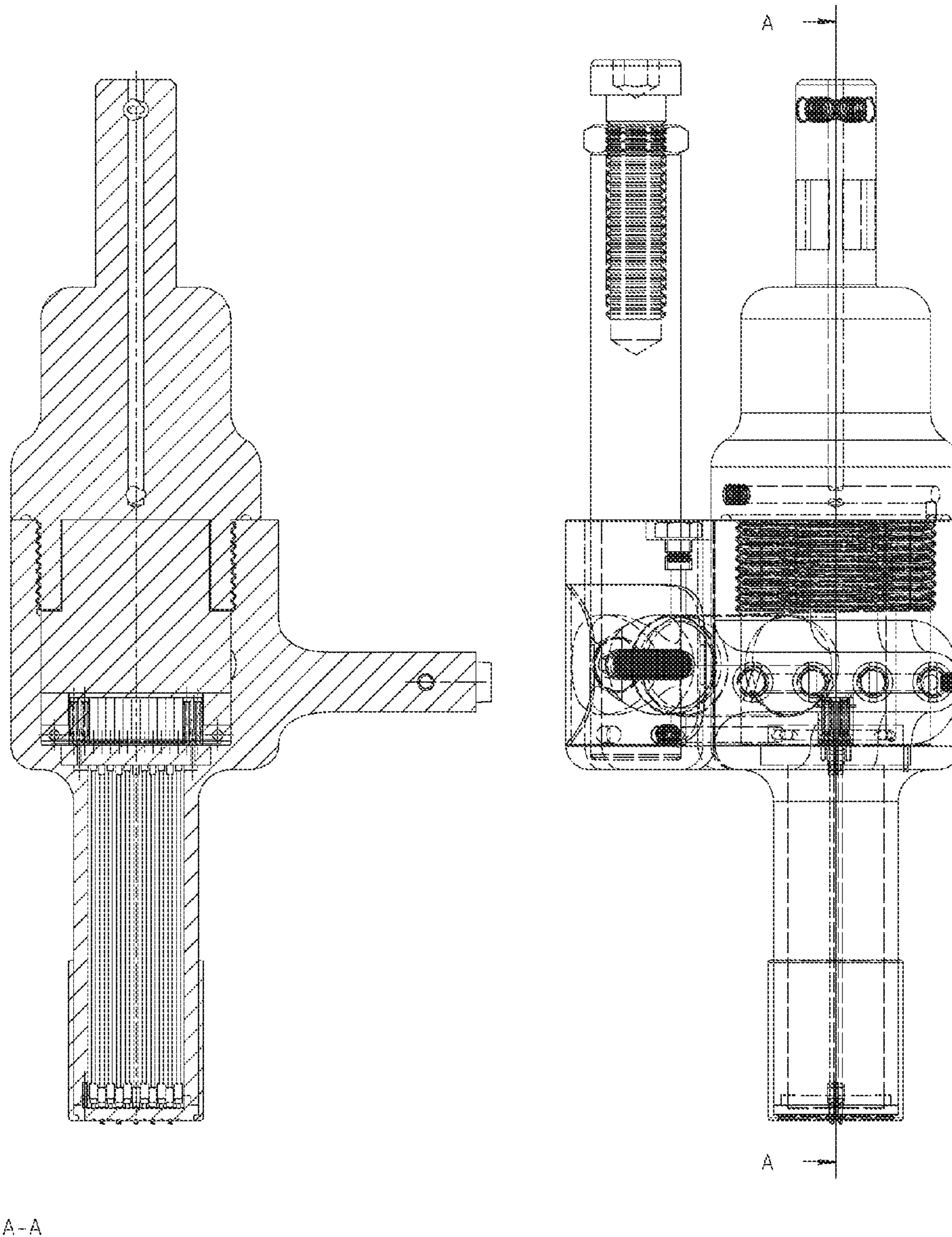
Rechargeable Contact and Wireless Programmable 2X11 Detachable Stylus Guide (Horizontal Stylus Center Line Section View) Selectable Character Multiple Stylus Orbital Engraving Tool's Typical Components and Assembly
